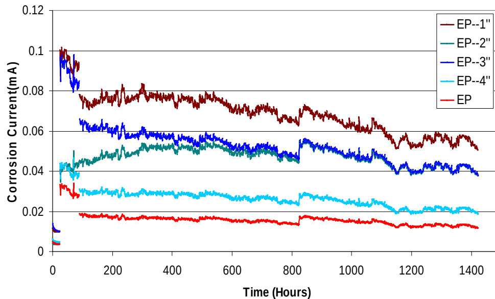
Figure 6.30 Corrosion current of epoxy-coated rebar.
