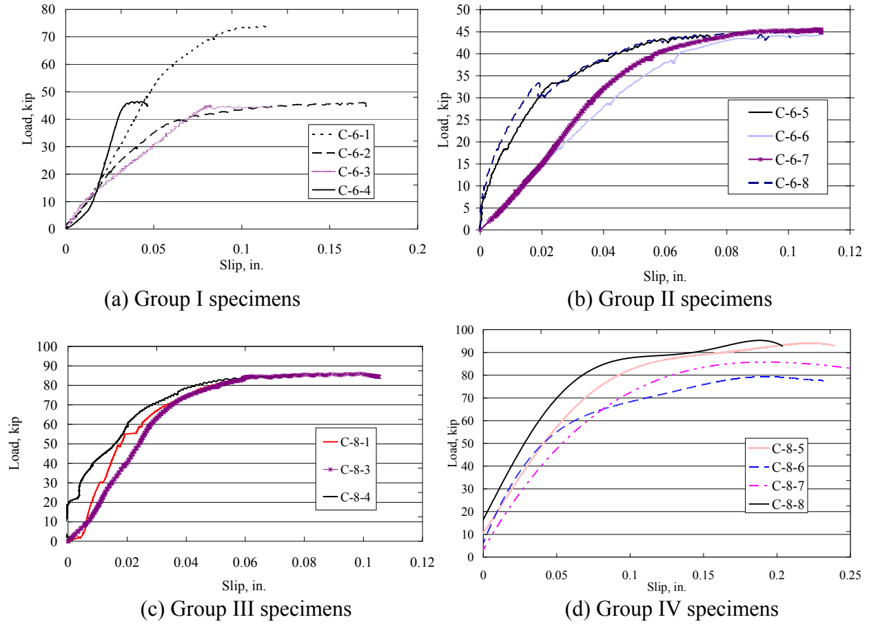
Figure 5.30 Load-slip curves of all tested specimens.
