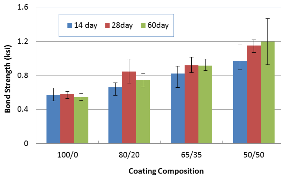
Figure 4.7 Concrete bonding to steel rods coated with various enamel coatings.
