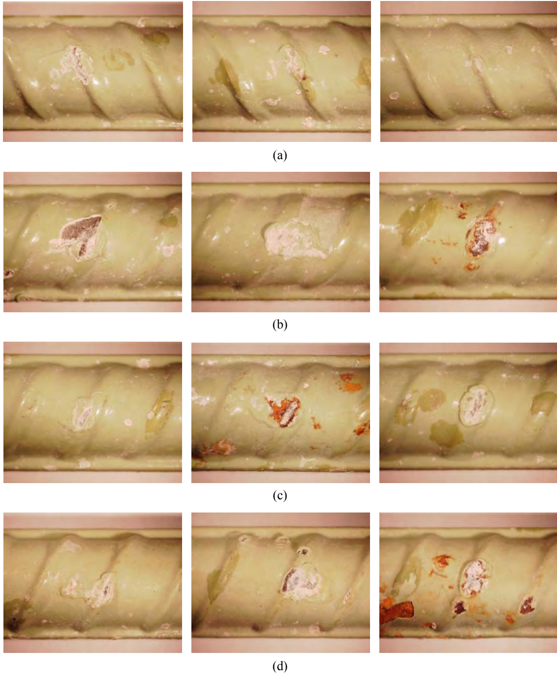
Figure C - 30: The three intentionally damaged areas along (a) bar-1; (b) bar-2; (c) bar-3; and (d) bar-4 of ponding specimen EP-D-2.
