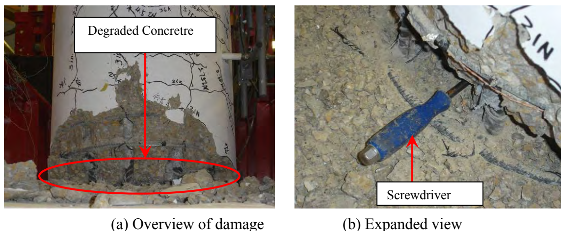
Figure 5.49 Concrete cover spalling and concrete core degradation of Column #1
