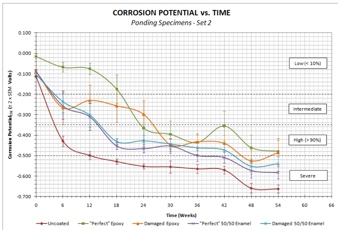
Figure C - 6: Average corrosion potential for (a) the first and second ponding specimen within each specimen group; (b) third and fourth ponding specimen within each specimen group.
