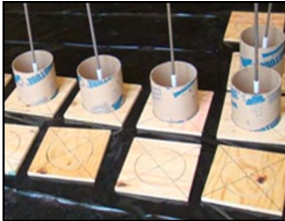
(a) Molds for specimen casting
