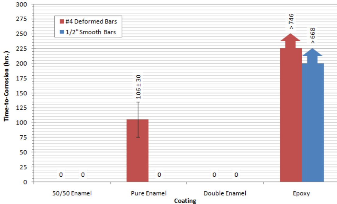
Figure 6.26 Test result summary for the non-grouted specimens.
