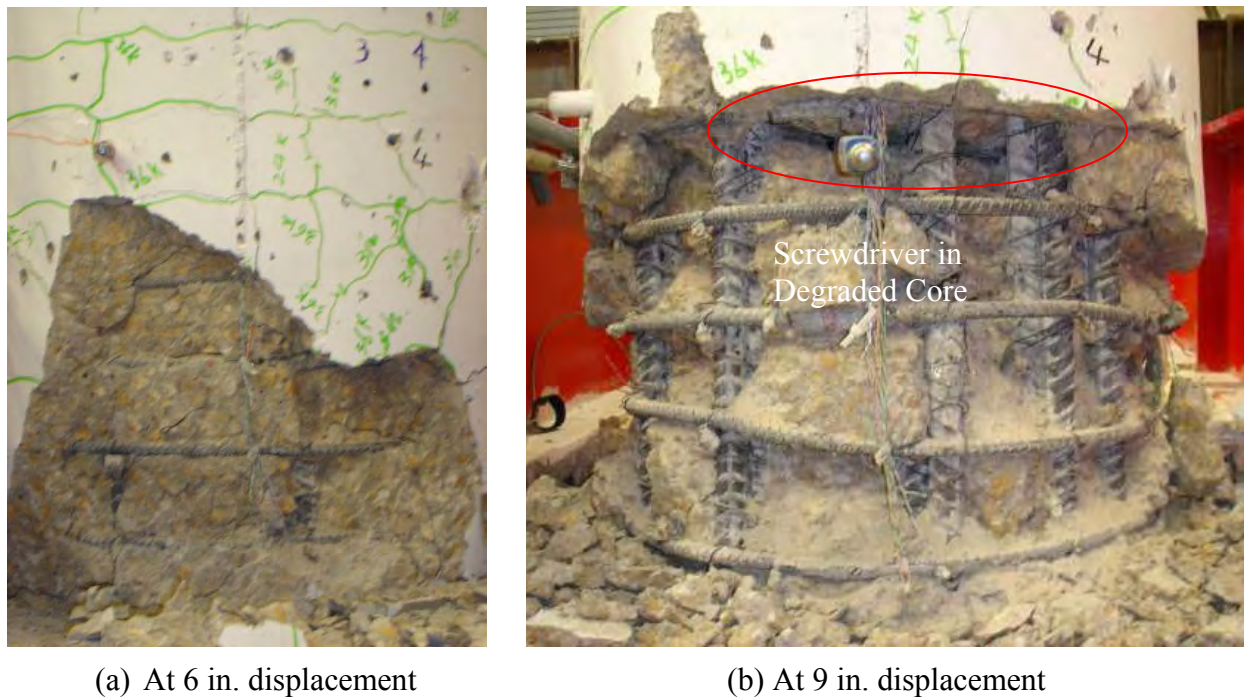
Figure 5.48 Concrete cover spalling and concrete core degradation of Column #1
