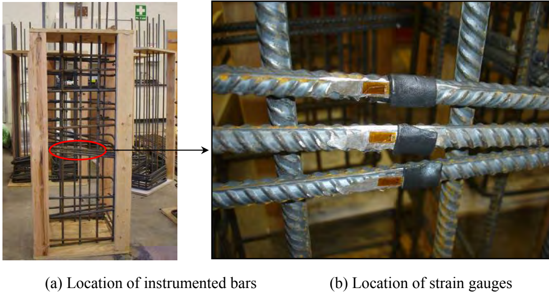
Figure 5.25 Strain gauges on stirrups.
