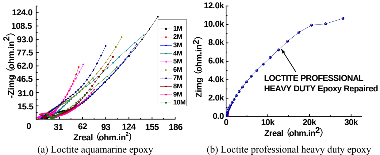
Figure 6.62 Nyquist plots of enamel-coated steel discs strengthened with different epoxies.
