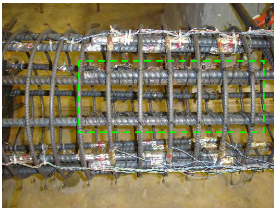
(a) Detail of lap splices
