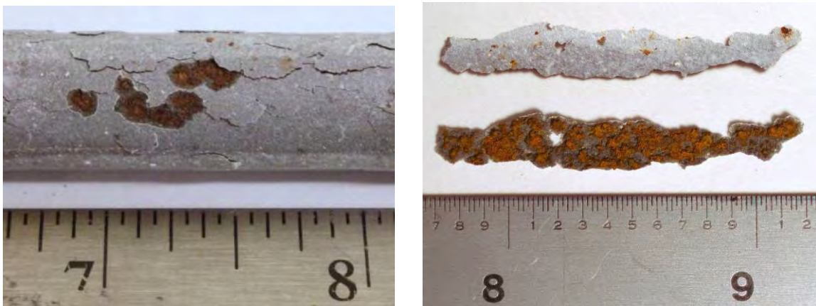
(a) Spalling of enamel coating
