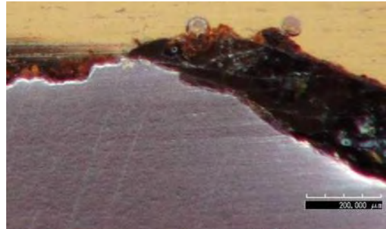
(c) No undercutting of coating even after significantly damaged on a deformed bar
