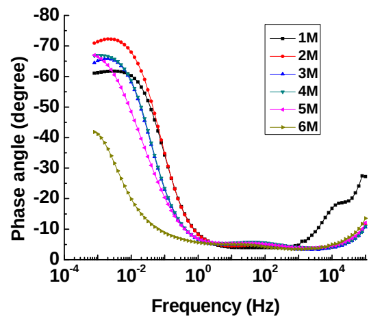
(c) Impedance phase angle
