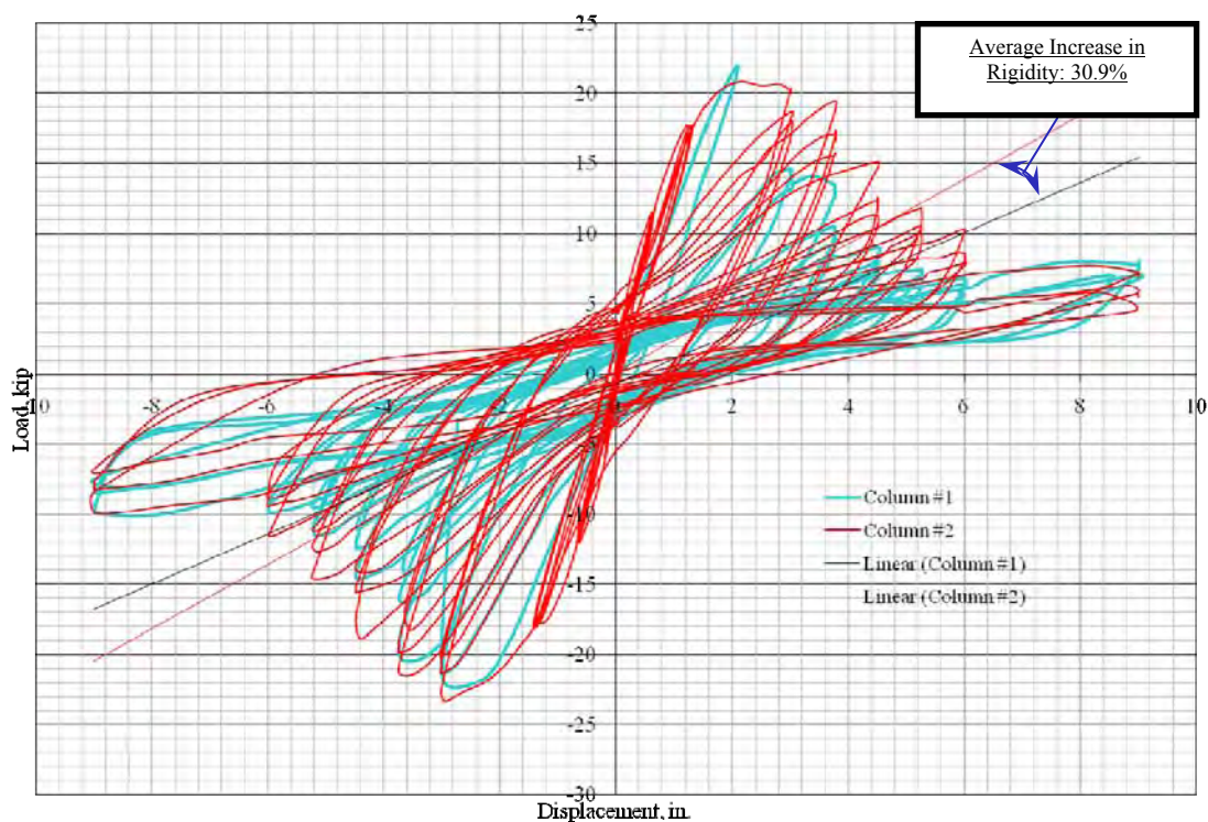
Figure 5.51 Load-displacement curves of two columns.
