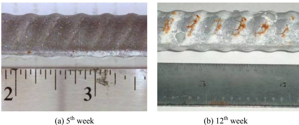
Figure 6.5 A typical condition of a deformed 50/50 enamel-coated specimen after testing.
