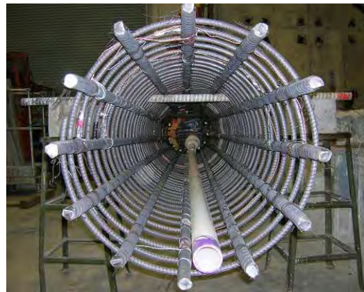
(b) Cross-sectional view of column cage
