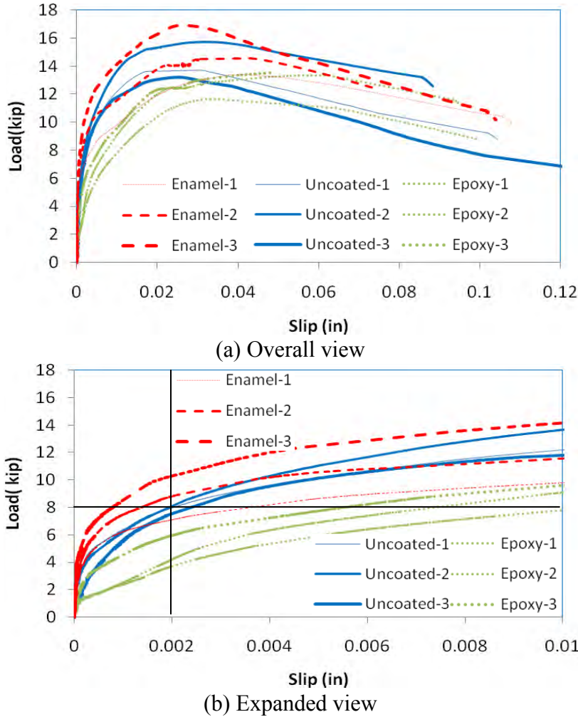
Figure 4.12 Load-slip curves of specimens with various coatings.
