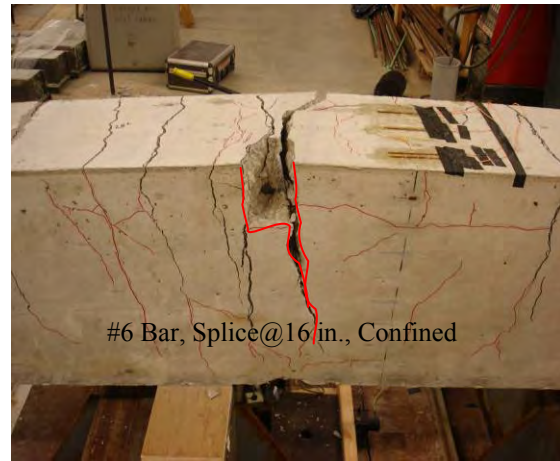
(b) Flexural failure of B-6-2
