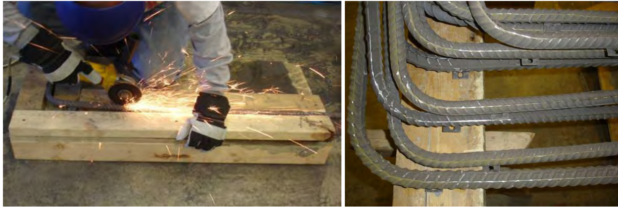
(a) Groove cutting
