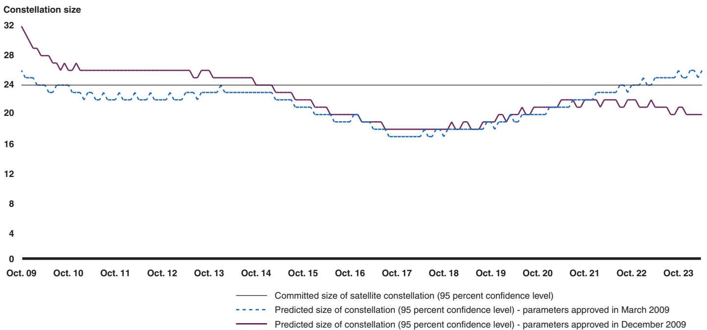
Figure 4: Predicted Size of GPS Constellation (at the 95 Percent Confidence Level) Based on a 2-Year GPS III Launch Delay and Reliability Data and Launch Schedules as of March 2009 and December 2009
