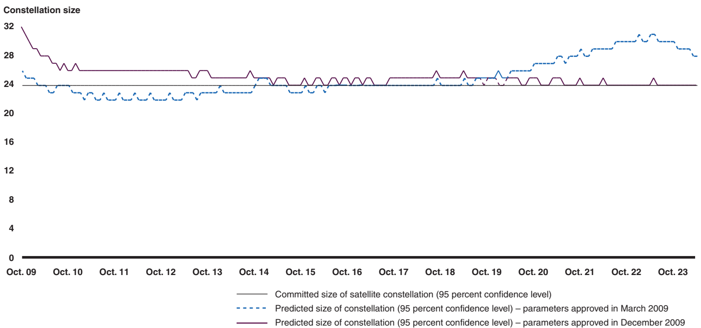
Figure 3: Comparison of Predicted Size of GPS Constellation (at the 95 Percent Confidence Level) Based on Reliability Data and Launch Schedules as of March 2009 and December 2009
