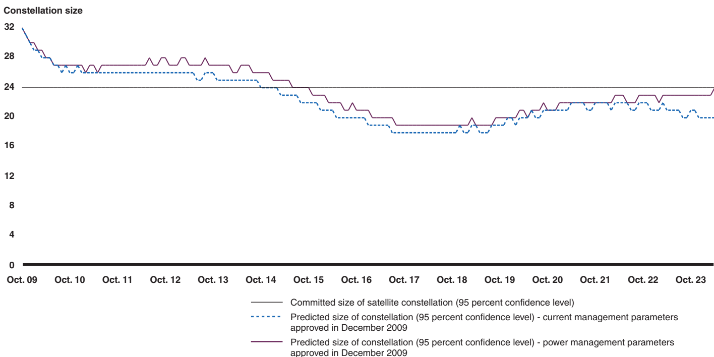
Figure 6: Predicted Size of GPS Constellation (at the 95 Percent Confidence Level) Based on a 2-Year GPS III Launch Delay and Current Management and Power Management Reliability Data and Launch Schedules as of December 2009
