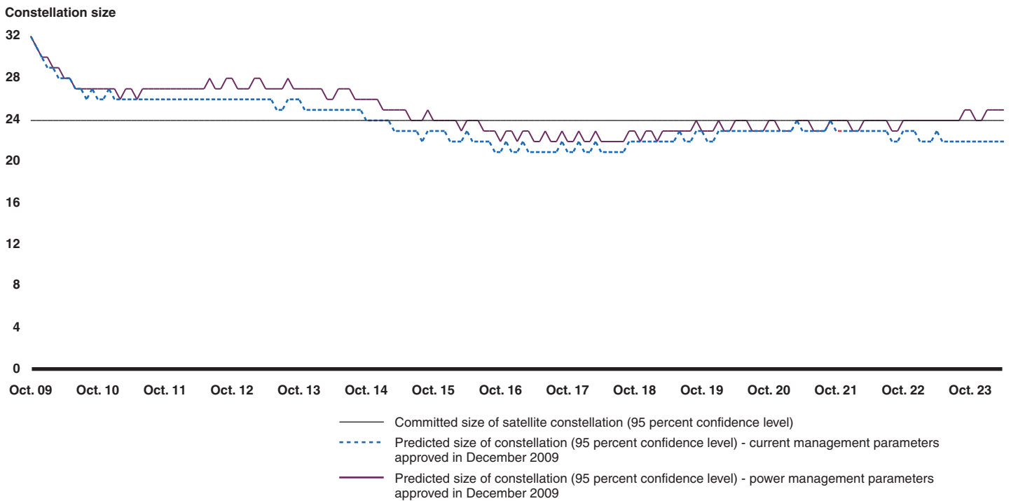
Figure 5: Predicted Size of GPS Constellation (at the 95 Percent Confidence Level) Based on a 1-Year GPS III Launch Delay and Current Management and Power Management Reliability Data and Launch Schedules as of December 2009
