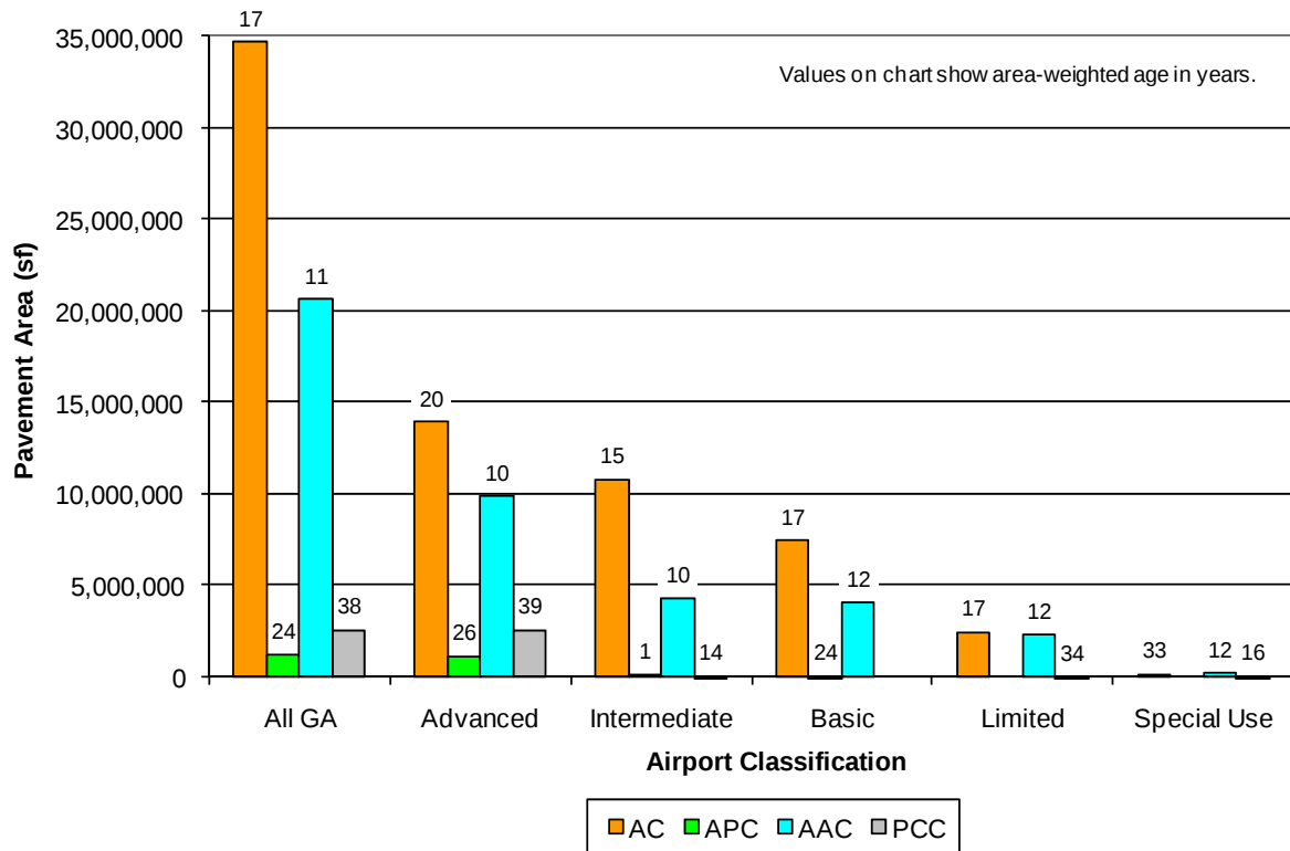
Figure 2. GA airports' pavement areas distributed by surface type.
