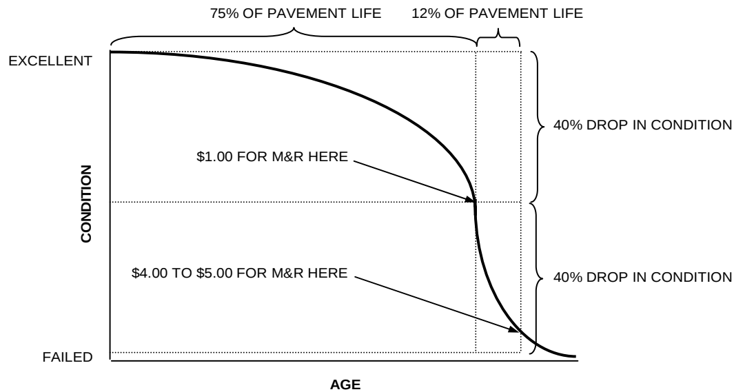
Figure 1. Pavement condition versus cost of repair.
