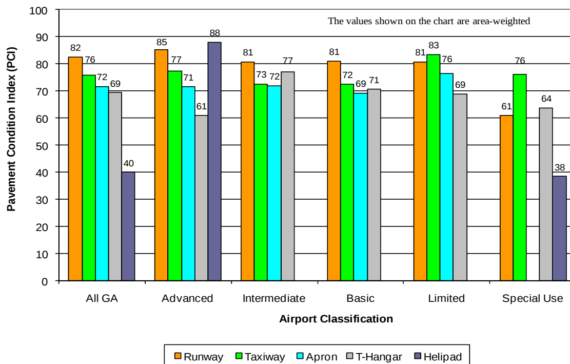
Figure 9. 2008 PCI by facility type for GA.
