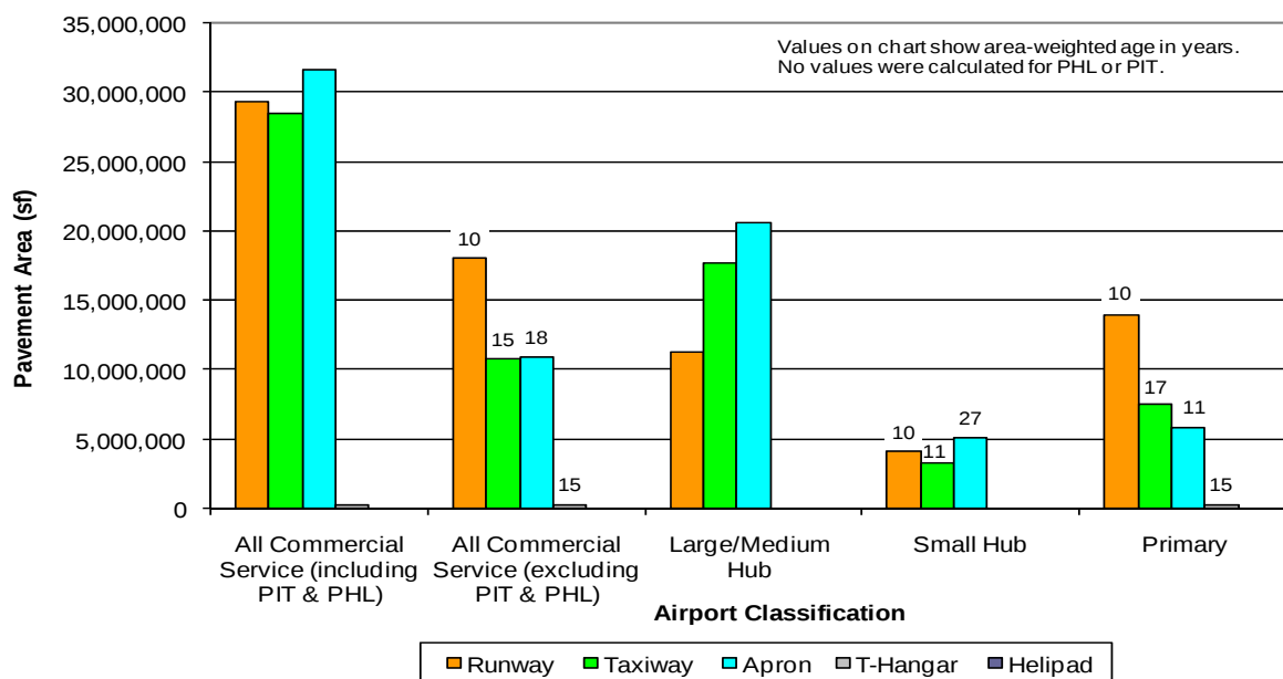
Figure 5. Commercial service airports' pavement areas distributed by facility type.
