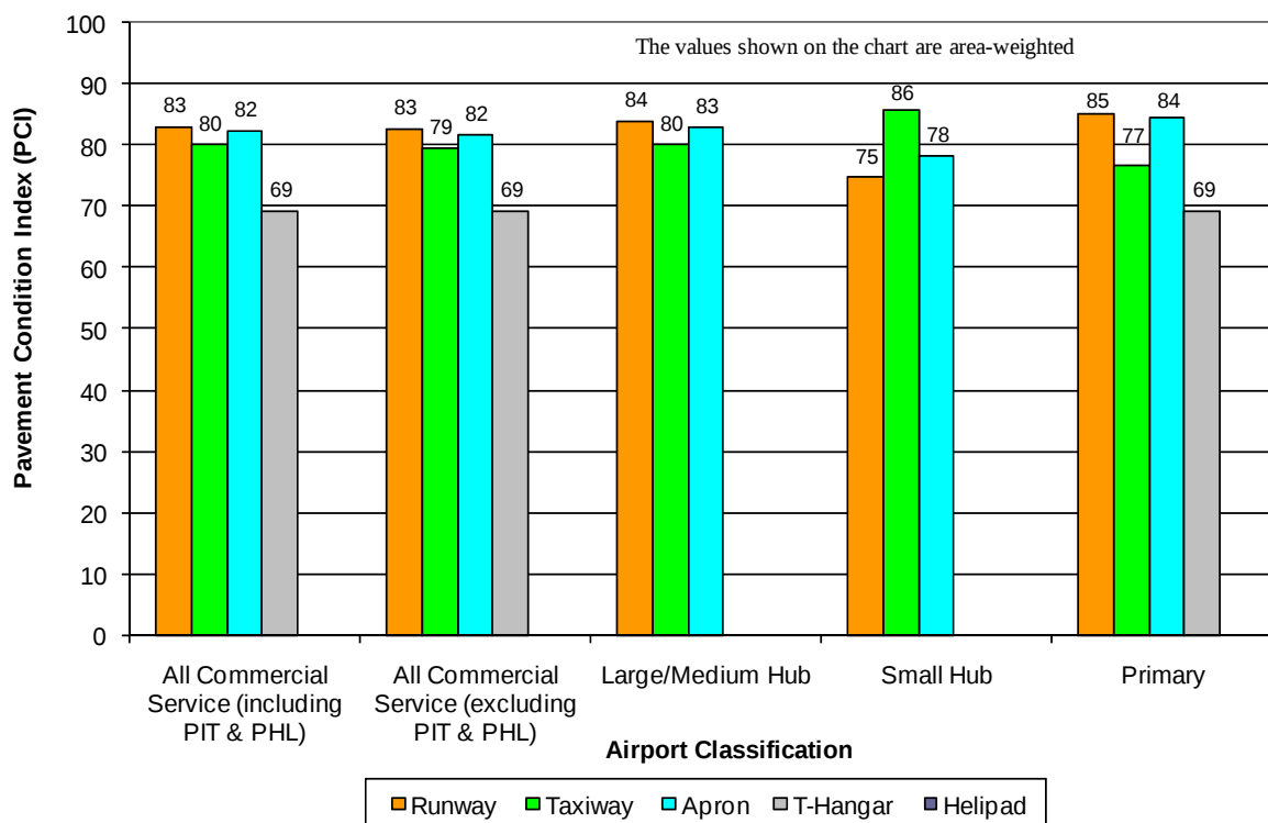
Figure 13. 2008 PCI by facility type for commercial service airports.
