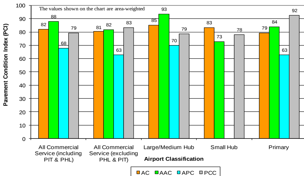
Figure 15. 2008 PCI by surface type for commercial service airports.
