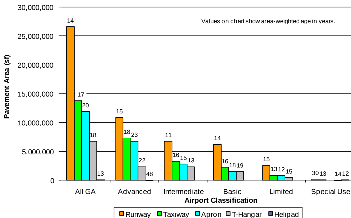
Figure 4. GA airports' pavement areas distributed by facility type.
