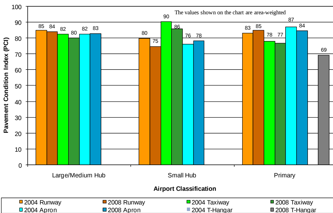
Figure 14. 2004 PCI versus 2008 PCI by facility type for commercial service airports.
