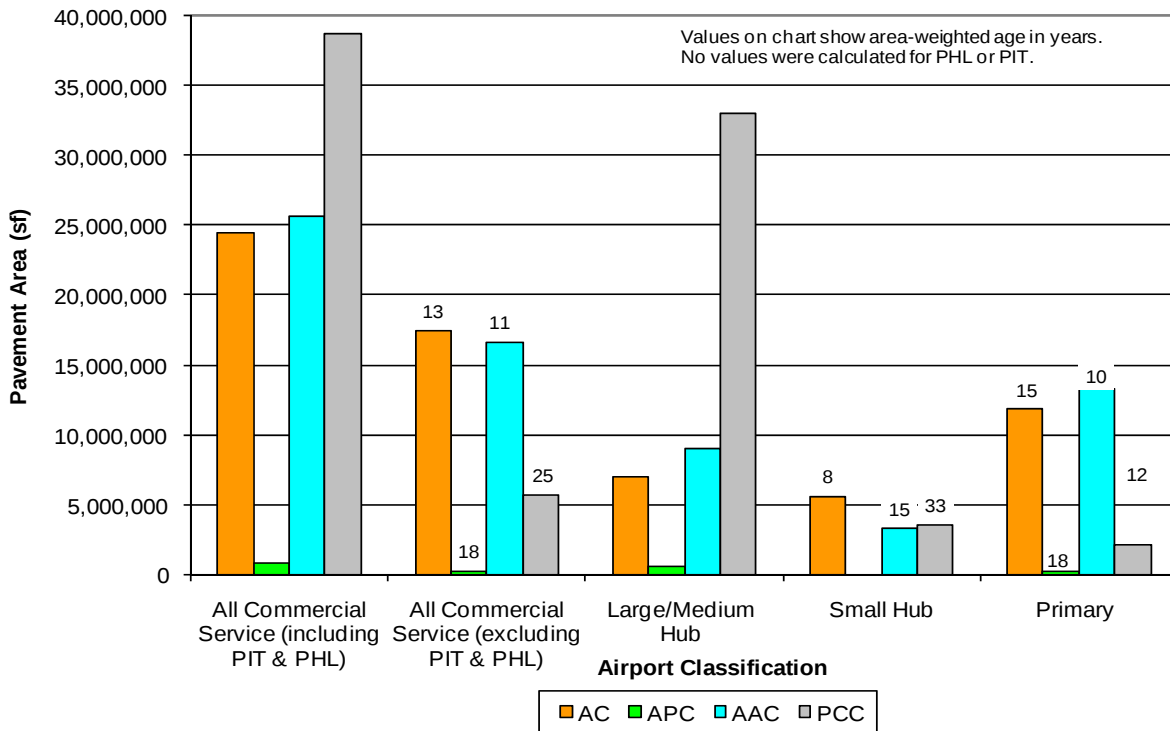
Figure 3. Commercial service airports' pavement areas distributed by surface type.
