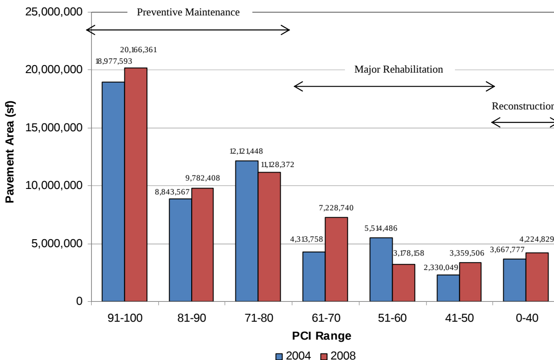
Figure 17. Condition distribution for GA airports.
