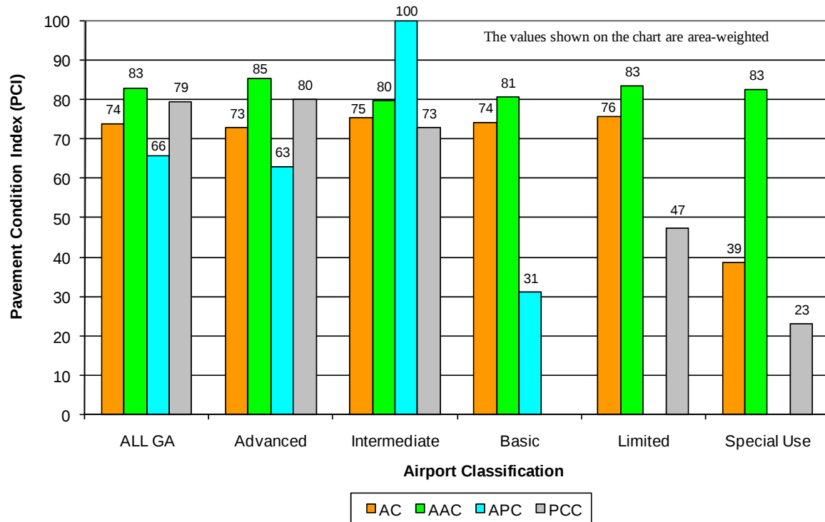
Figure 11. 2008 PCI by surface type for GA airports.
