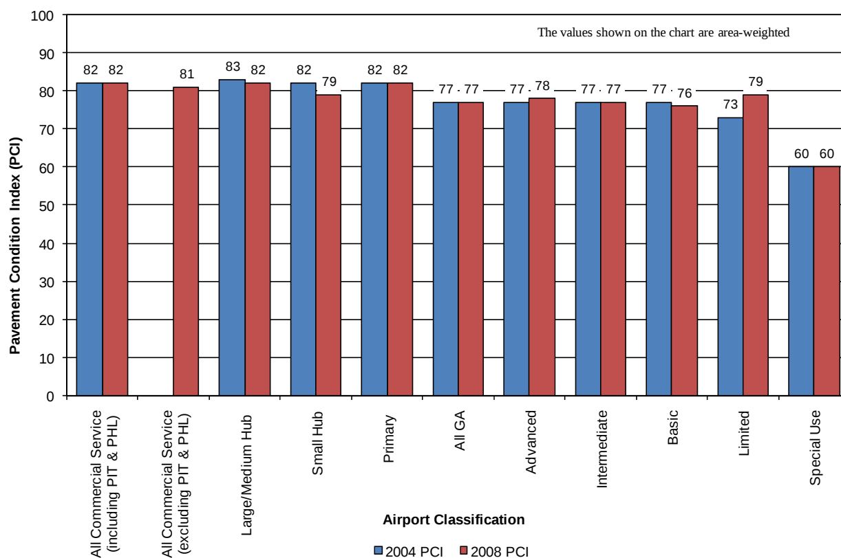
Figure 8. PCI by airport classification.
