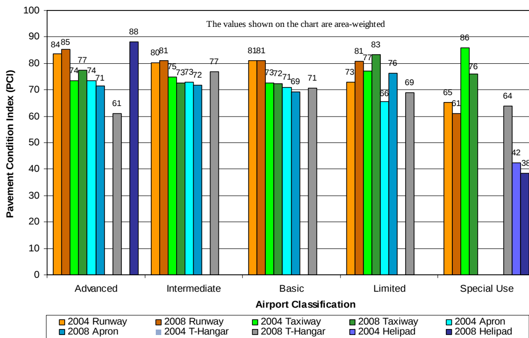
Figure 10. 2004 PCI versus 2008 PCI by facility type for GA airports.
