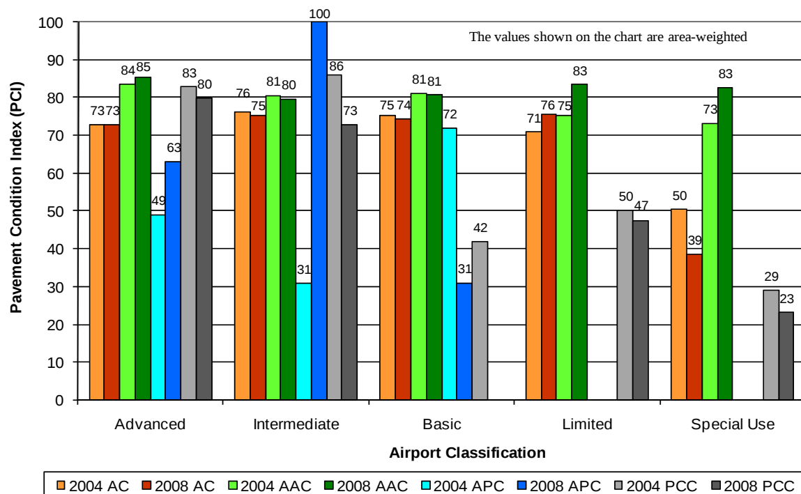
Figure 12. 2004 PCI versus 2008 PCI by surface type for GA airports.
