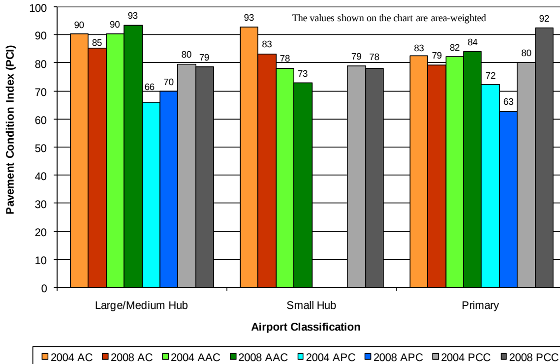
Figure 16. 2004 PCI versus 2008 PCI by surface type for commercial service airports.
