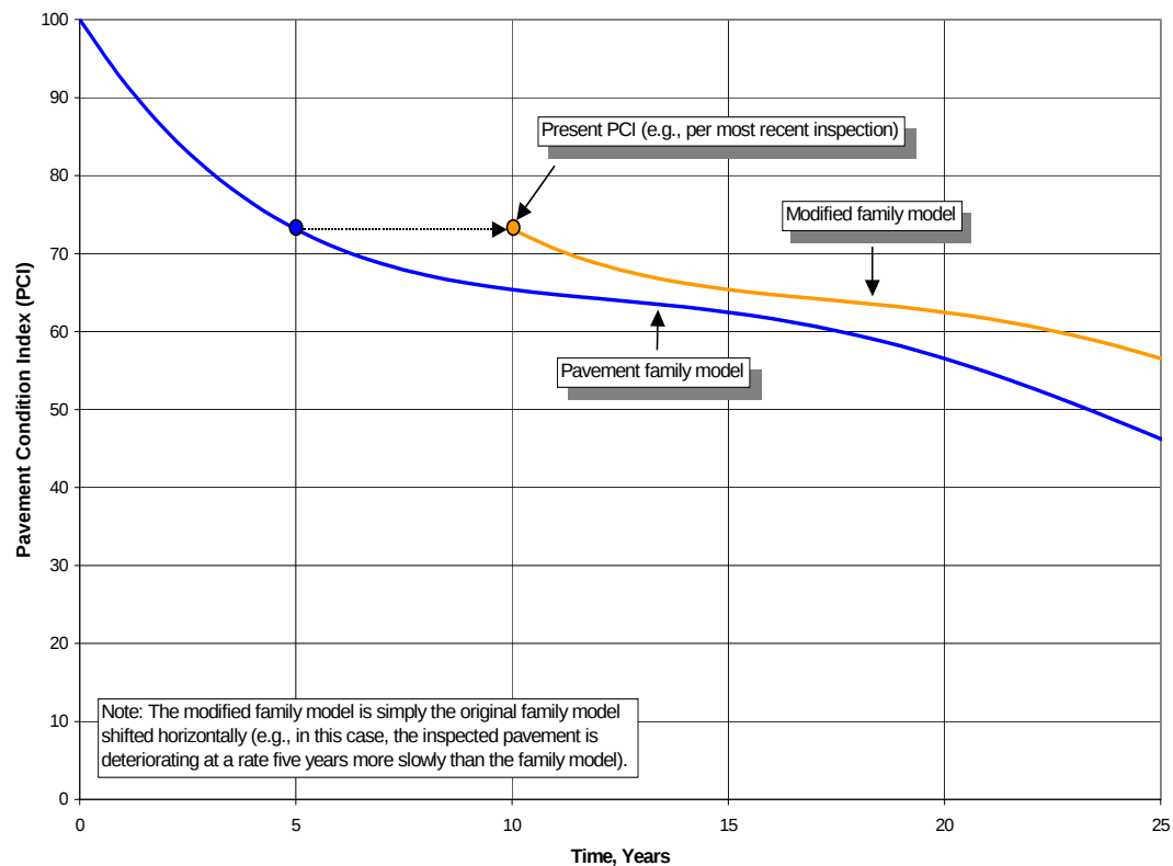
Figure 19. Performance model application.
