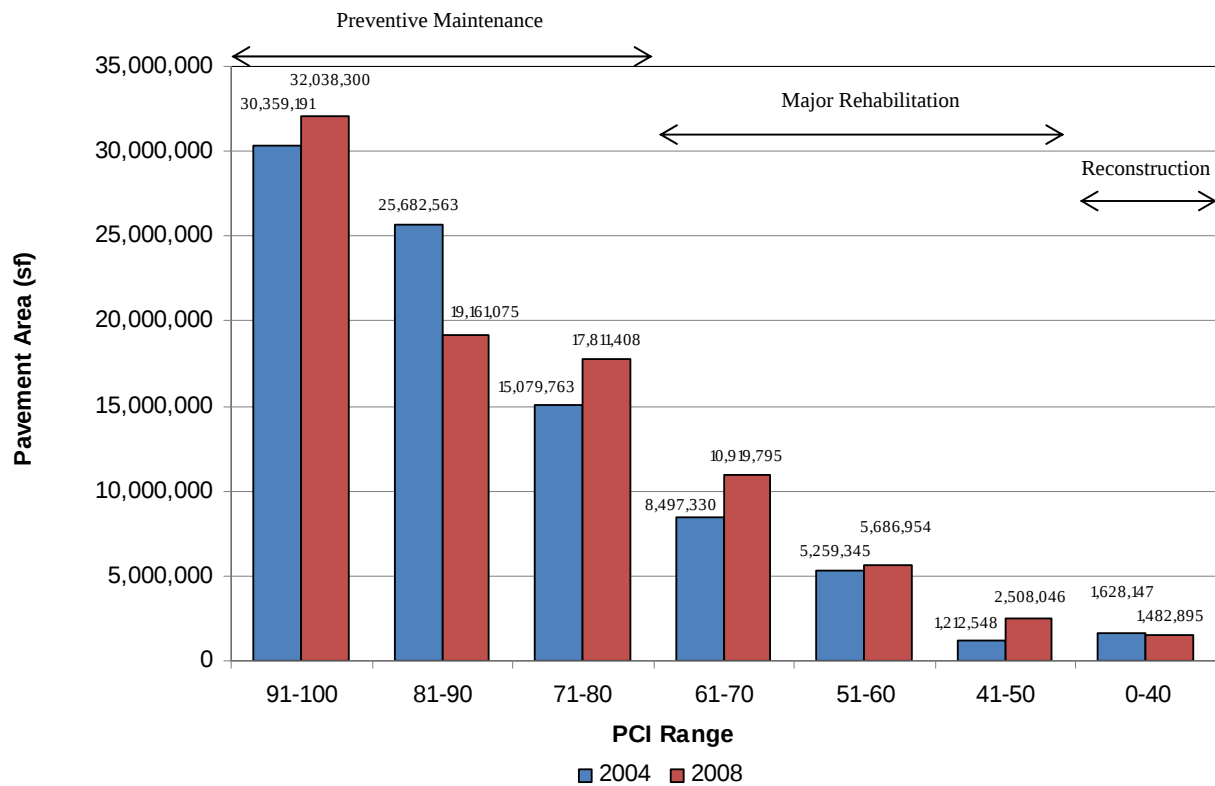
Figure 18. Condition distribution for commercial service airports.
