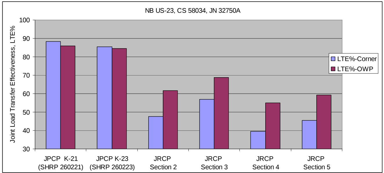
Figure 4.1 (a, b). Joint load transfer effectiveness.
