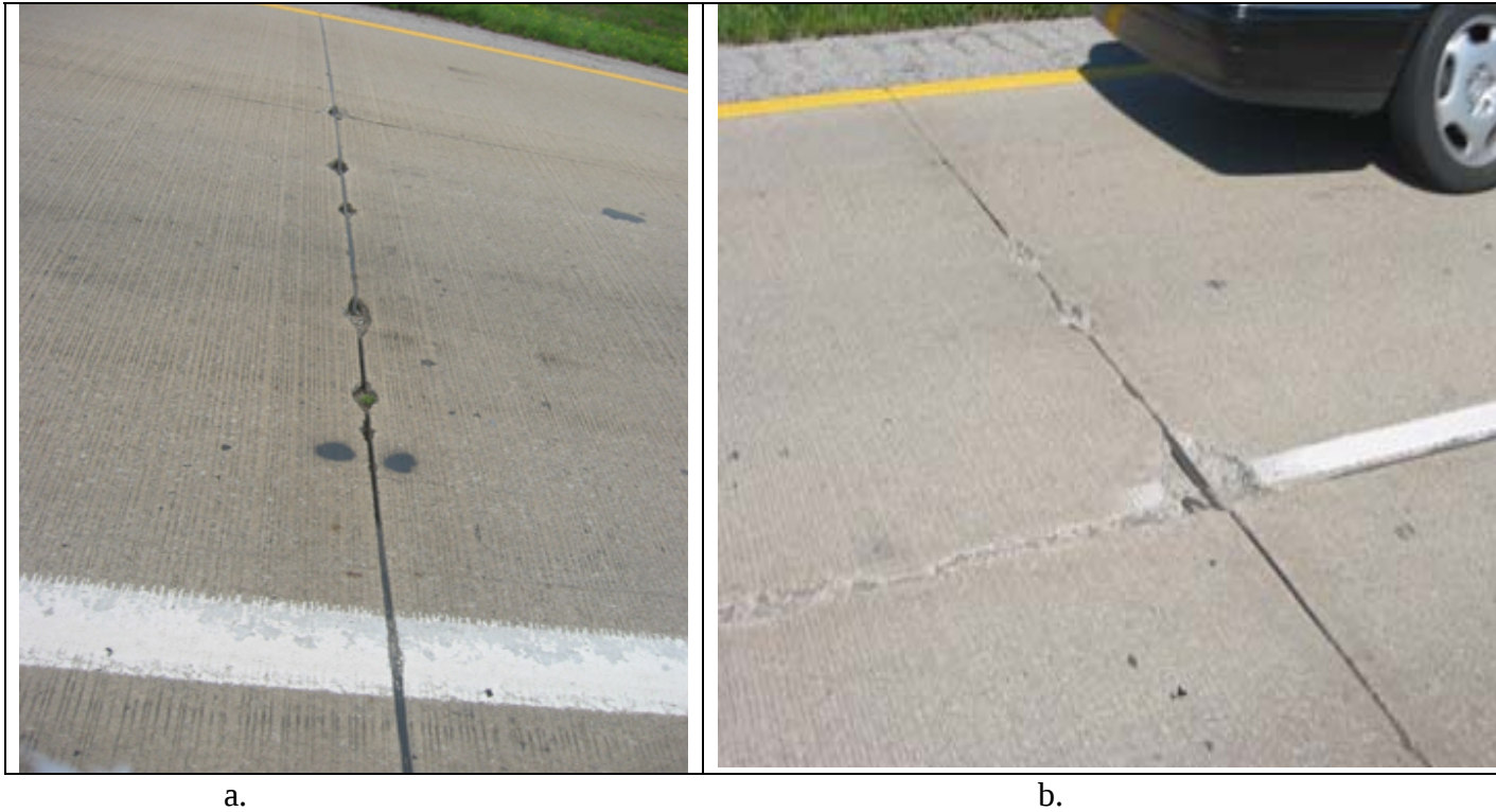
Figure 4.8 Joint spalling for test sections SHRP 260221 (a) and 260223 (b).
