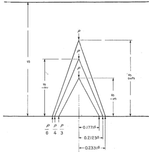
FIGURE 20.—POSITIONS OF RESULTANTS, EACH REPRESENTING LEFT HALF OR RIGHT HALF OF THE DIAGRAM OF REACTIONS, IN CASES SHOWN IN FIGURE 19 (FROM EQUATION 116). POISSON'S RATIO, \mu=0.15
