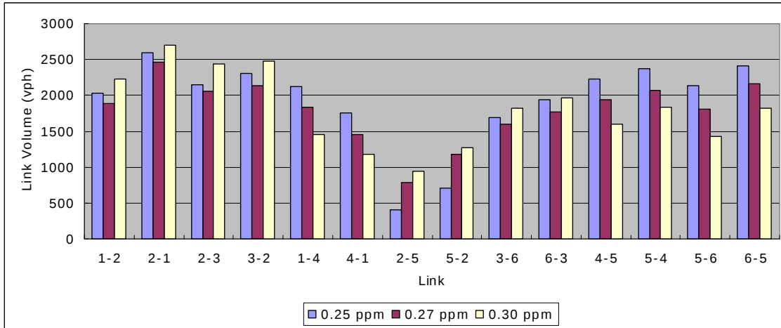
Figure 25. Link volumes under different CE s (0.25, 0.27, and 0.30 ppm)
