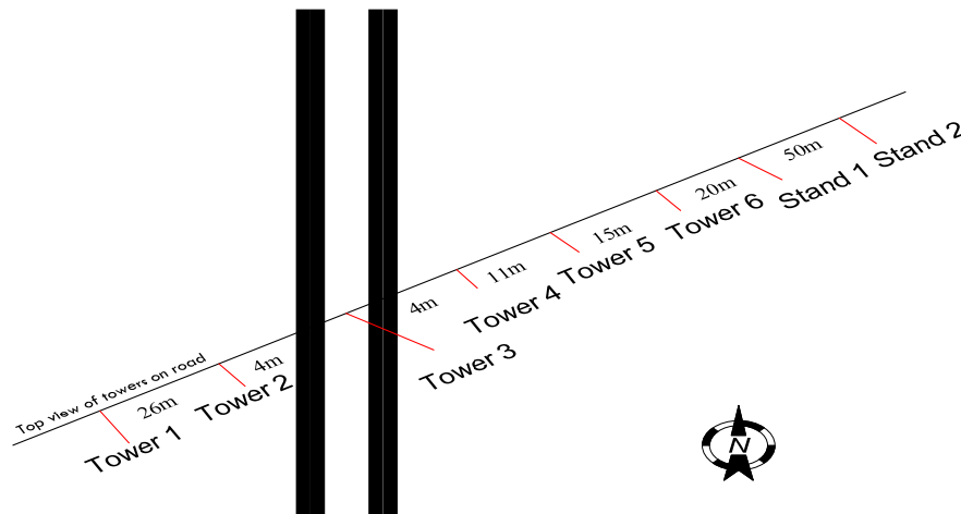
Figure 3. The alignment of six towers and two stands
