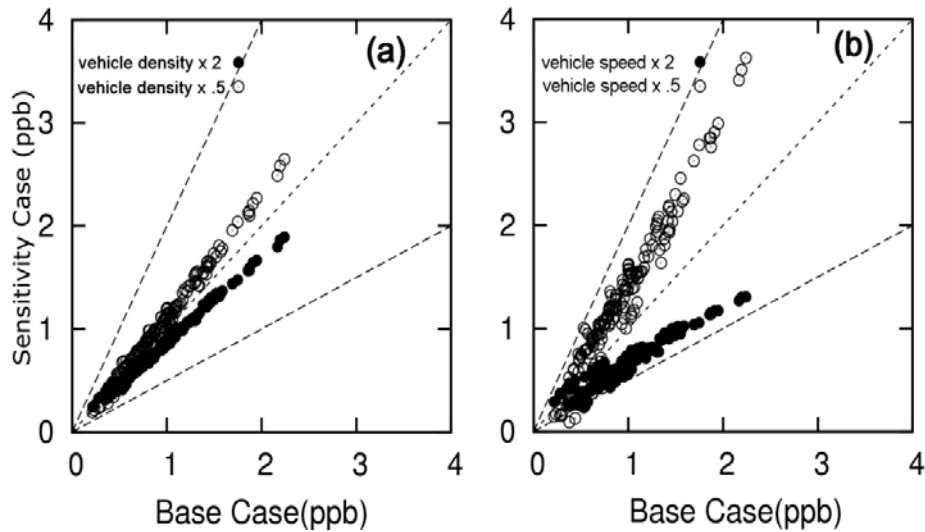
Figure 10. Sensitivity of the predicted \text{SF}_6 concentrations to the change in vehicle density and speed
