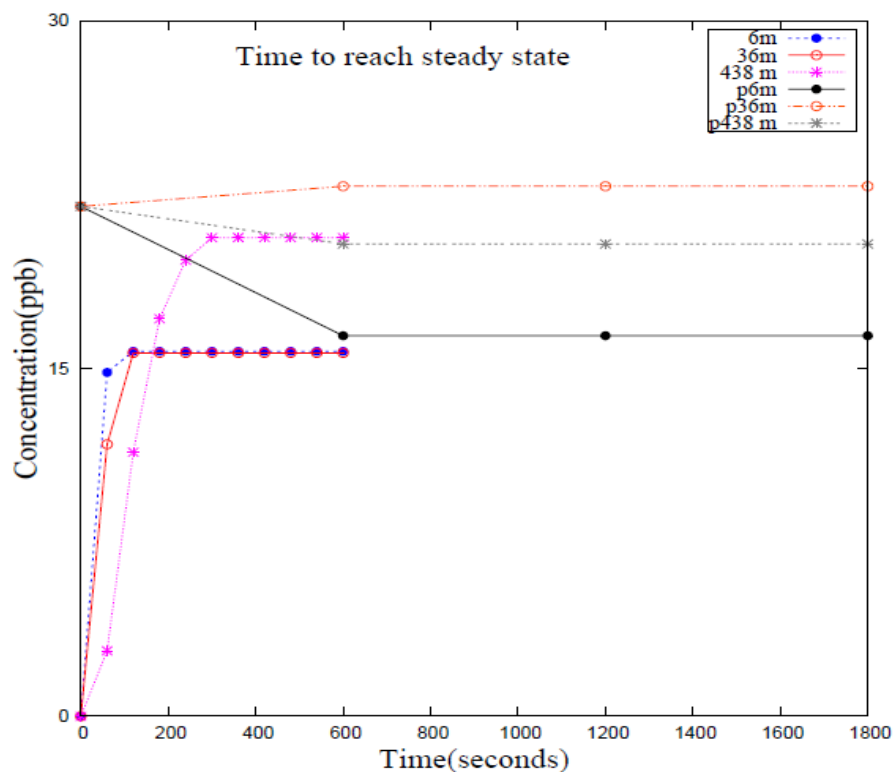
Figure 13. Change in ozone concentration with time at the heights of 6, 36, and 438 m
