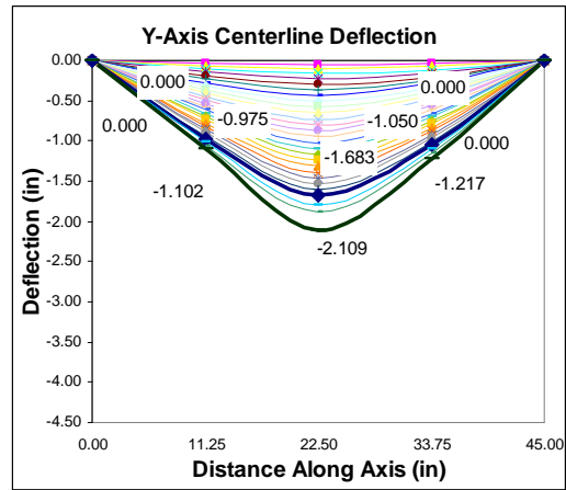
Figure 3.34 Y-Axis Deflection
