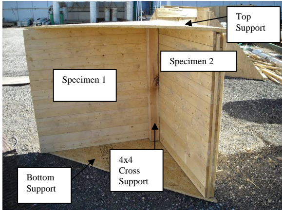
Figure 2.7 Wall Self-Supporting Structure
