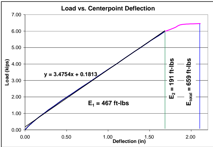
Figure 3.32 Static Test #3 Load vs. Centerpoint Deflection
