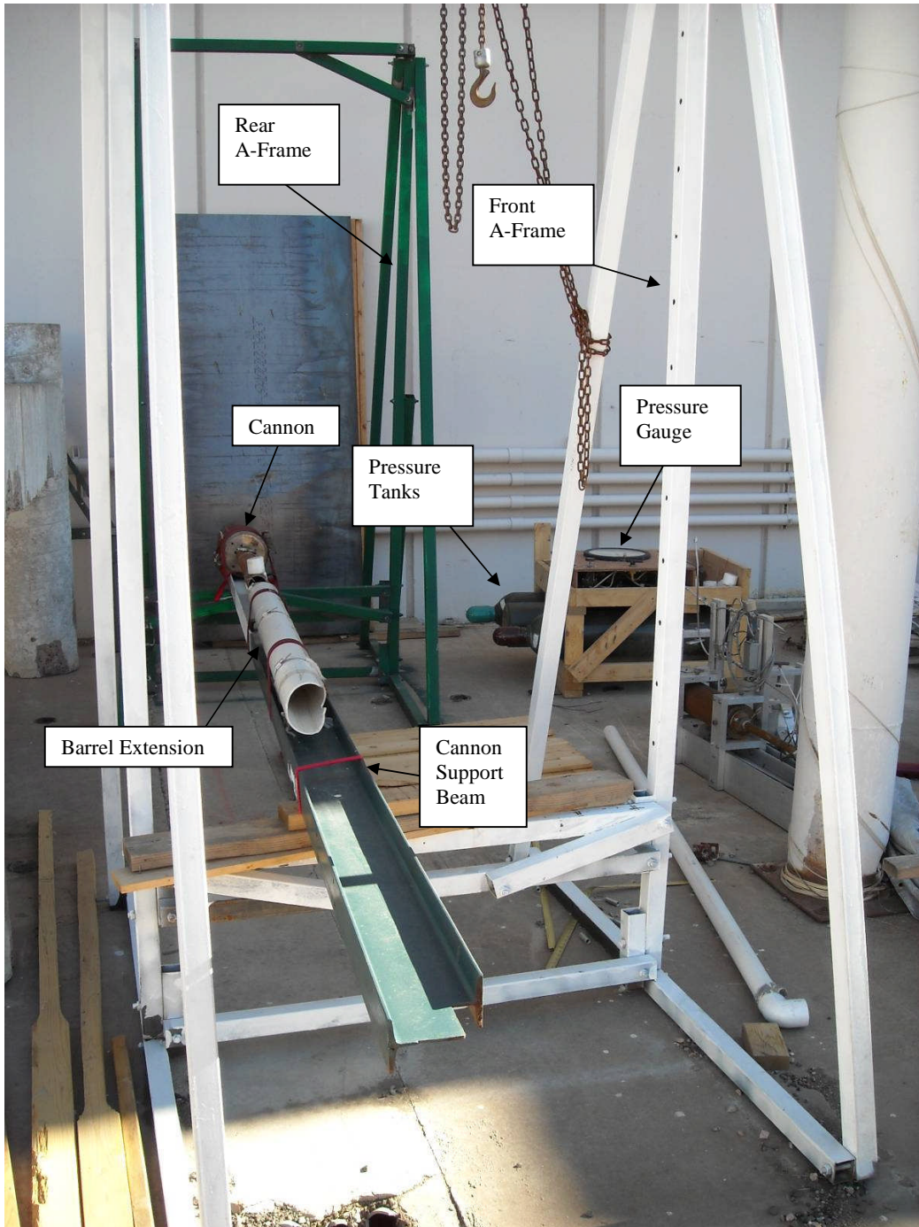
Figure 2.2 Cannon Experimental Test Setup
