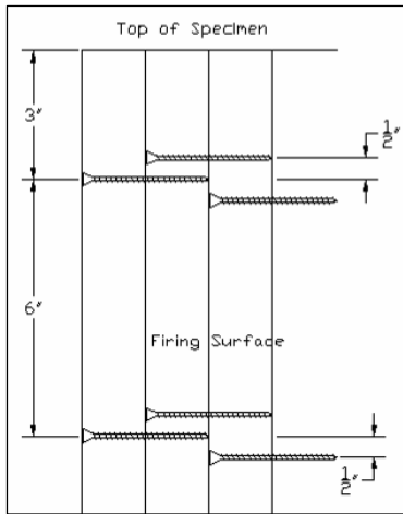
Figure 2.17 Front View of Strong Axis Fastener Distribution
