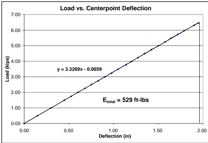
Figure 3.29 Static Test #2 Load vs. Centerpoint Deflection
