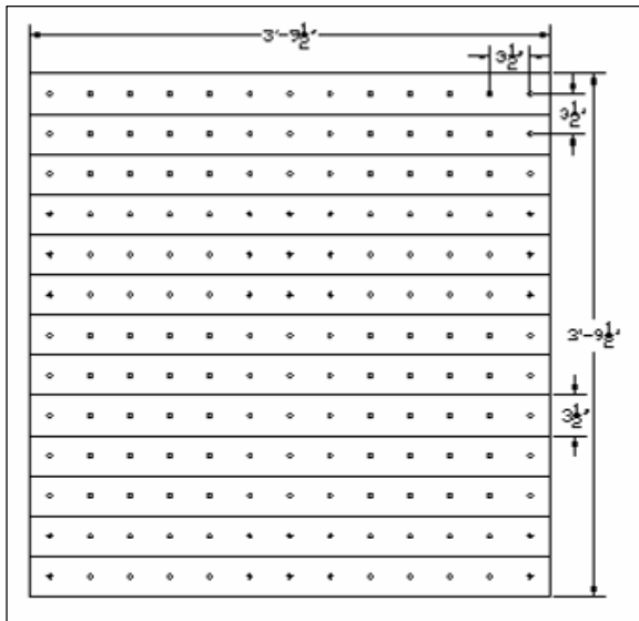
Figure 2.18 “Every Intersection” Fastener Distribution
