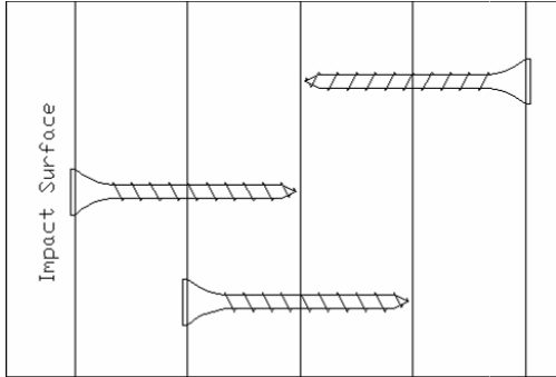
Figure 2.21 "Method 1" Fastener Directions
