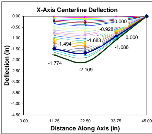
Figure 3.33 X-Axis Deflection
