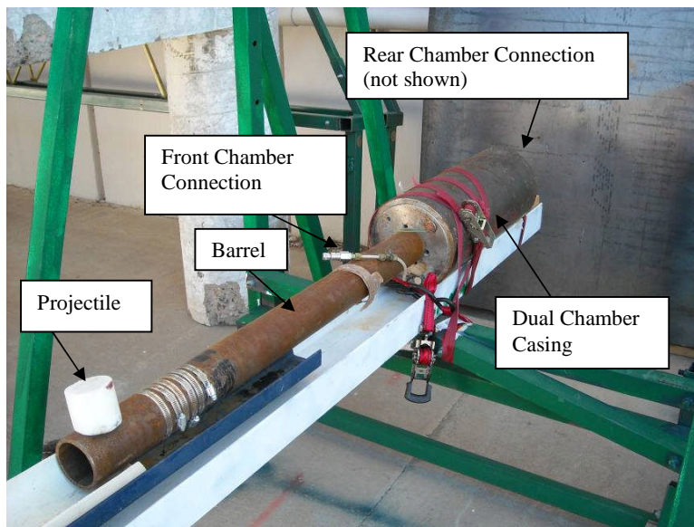
Figure 2.1 Cannon with Projectile
