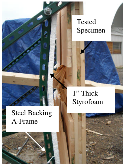
Figure 2.6 Flexible Backing
