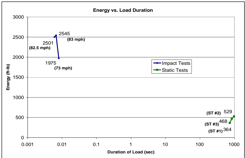
Figure 4.3 Energy vs. Load Duration for Passing Specimens
