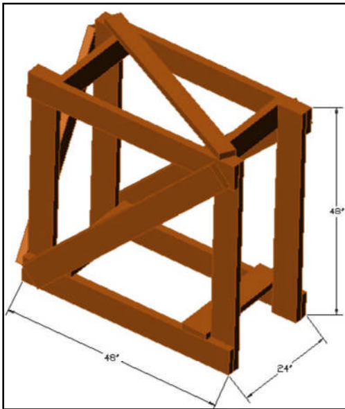
Figure 2.3 Wood Backing Frame
