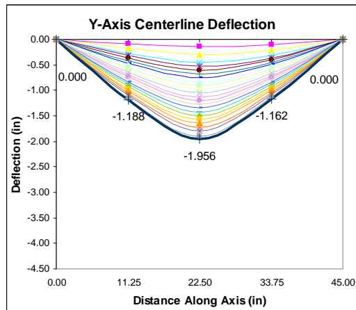
Figure 3.31 Y-Axis Deflection
