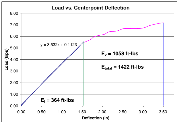
Figure 3.25 Static Test #1 Load vs. Centerpoint Deflection
