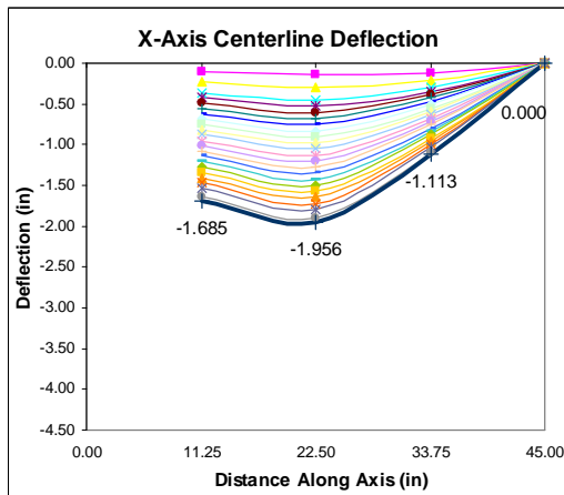
Figure 3.30 X-Axis Deflection
