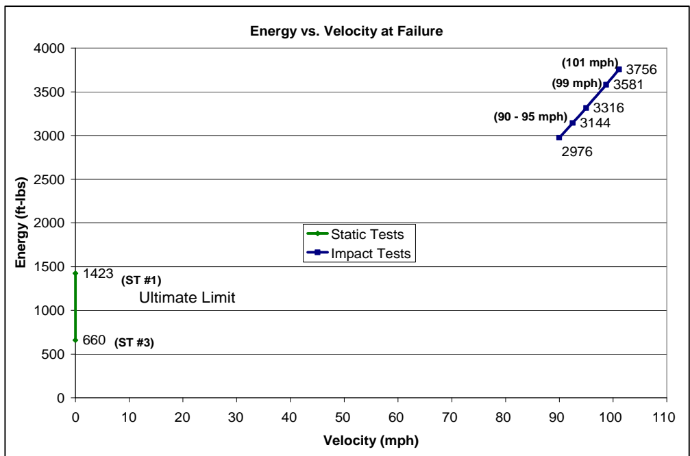
Figure 4.4 Energy vs. Velocity for Specimens at Failure
