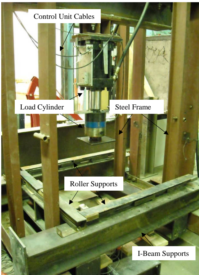
Figure 2.8 Static Loading Specimen Support
