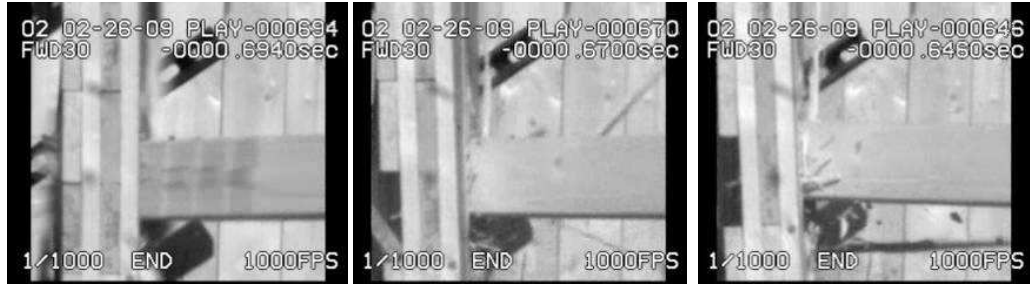
Figure 3.8a Test #39 (Impact)
