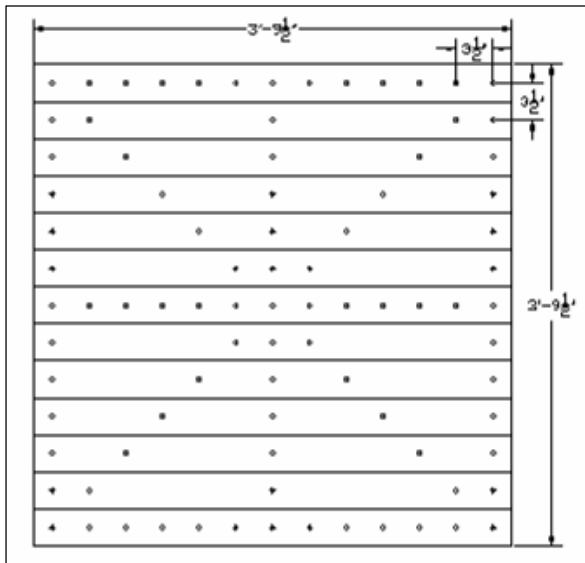
Figure 2.20 “Edge/Star” Fastener Distribution
