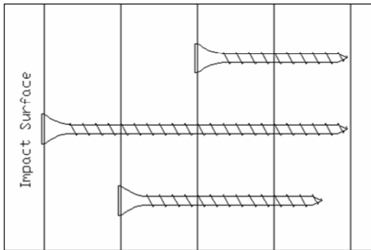
Figure 2.22 "Method 2" Fastener Directions
