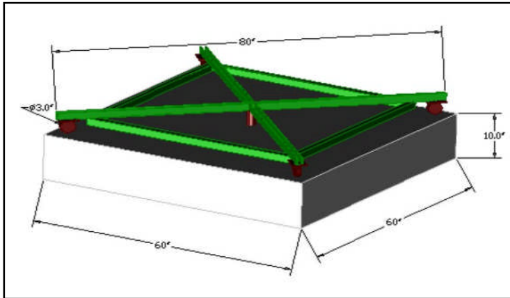
Figure 2.4 Turntable and Concrete Base
