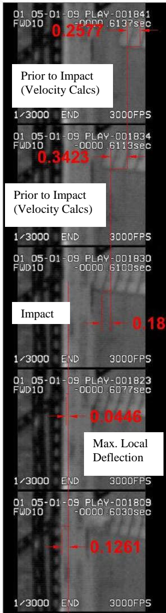
Figure 2.12 Impact Load Deflection Measurement
