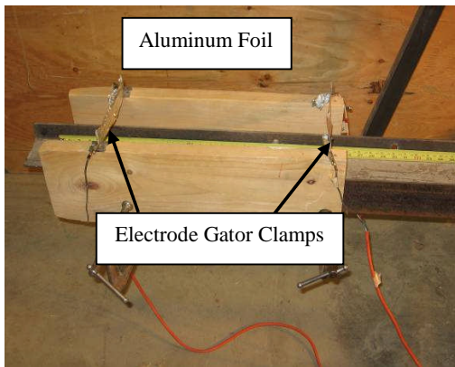
Figure 2.9 Time Measurement Setup
