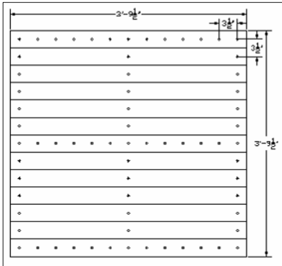
Figure 2.19 “Edge/Cross” Fastener Distribution
