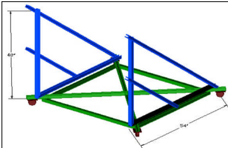
Figure 2.5 Steel Backing Frame Support
