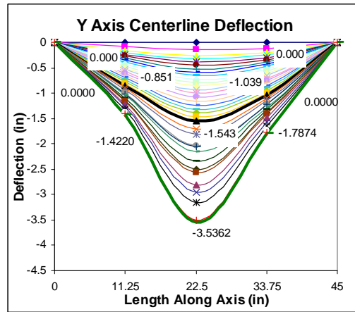
Figure 3.27 Y-Axis Deflection
