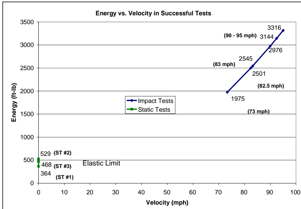
Figure 4.2 Energy vs. Velocity for Passing Specimens
