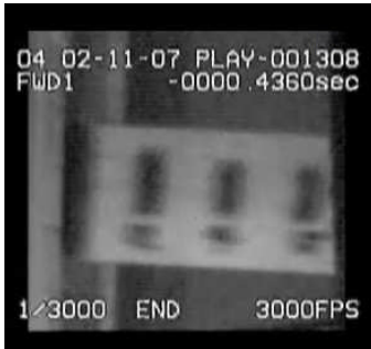
Figure 3.1a Test #19 (Impact)
