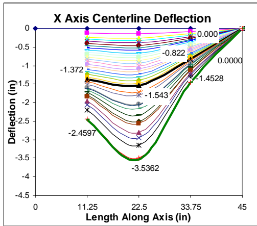
Figure 3.26 X-Axis Deflection
