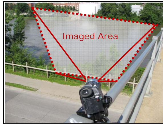
Figure 3-23 LSPIV measurements during the Iowa River flood of 2008: location of the measurement site (left and right)
