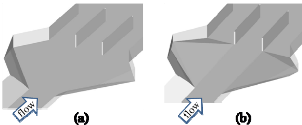
Figure 3-3. Illustration of the computational domains: a) 3-box I culvert design, and b) self-cleaning culvert design for a)
