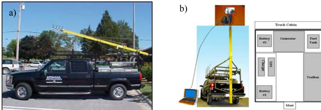
Figure 3-4 MLSPIV unit: a) general view; b) mast deployed and ancillary equipment
