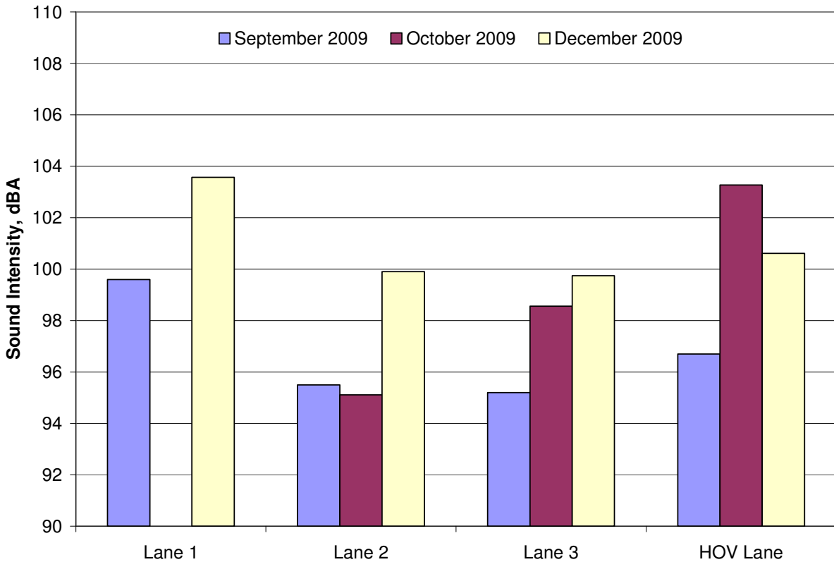
Figure 23. Sound intensity level (dBA) measurements for the OGFC-SBS sections.
