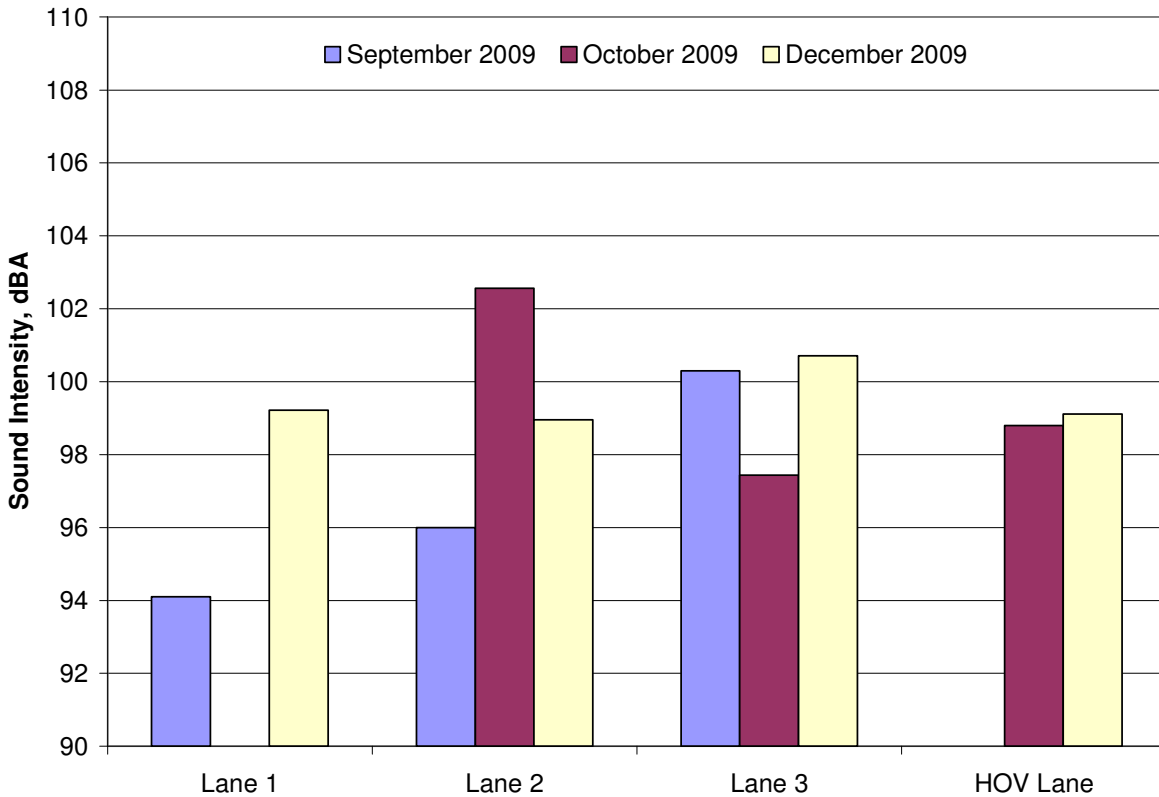
Figure 22. Sound intensity level (dBA) measurements for the OGFC-AR sections.
