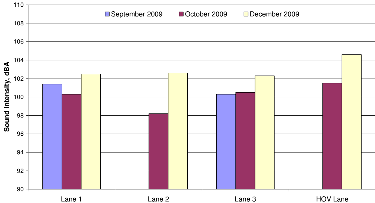
Figure 24. Sound intensity level (dBA) measurements for 1/2 inch HMA control section.
