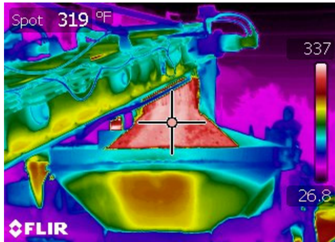
Image of temperature from MTD to paver hopper
