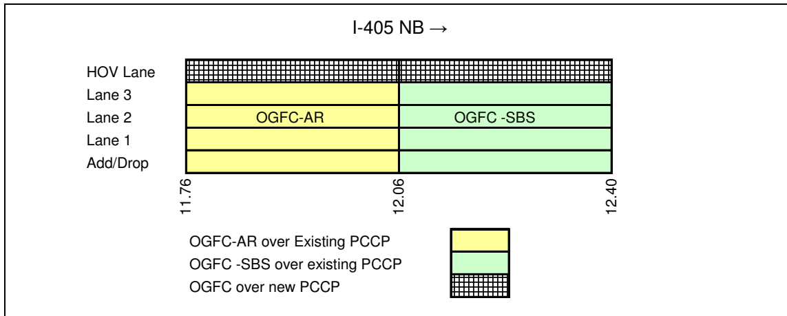
Figure 3. Schematic of paving limits for test sections north of I-90 (north section).
