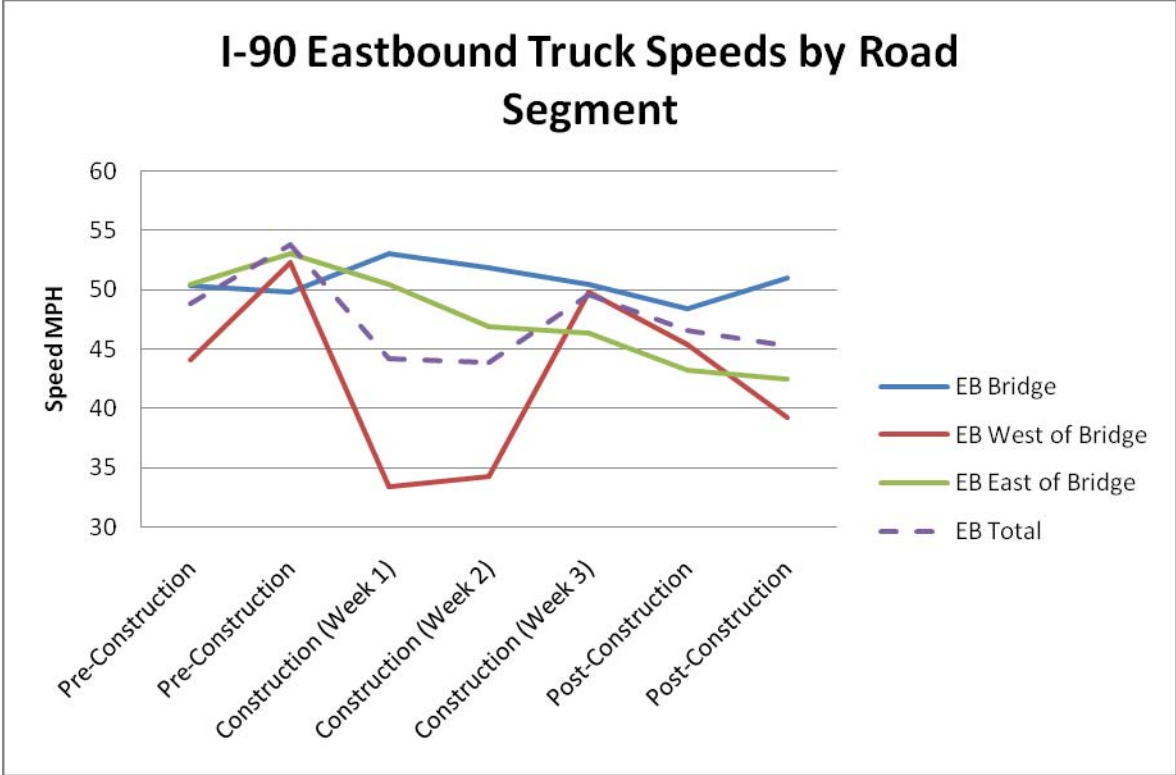
Figure A3-4: Eastbound truck speed comparison by road segment
