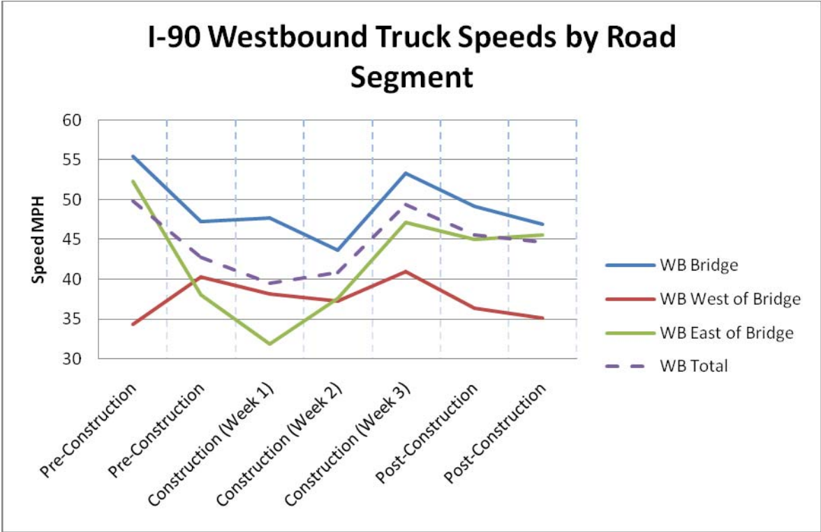
Figure A3-3: Westbound truck speed comparison by road segment
