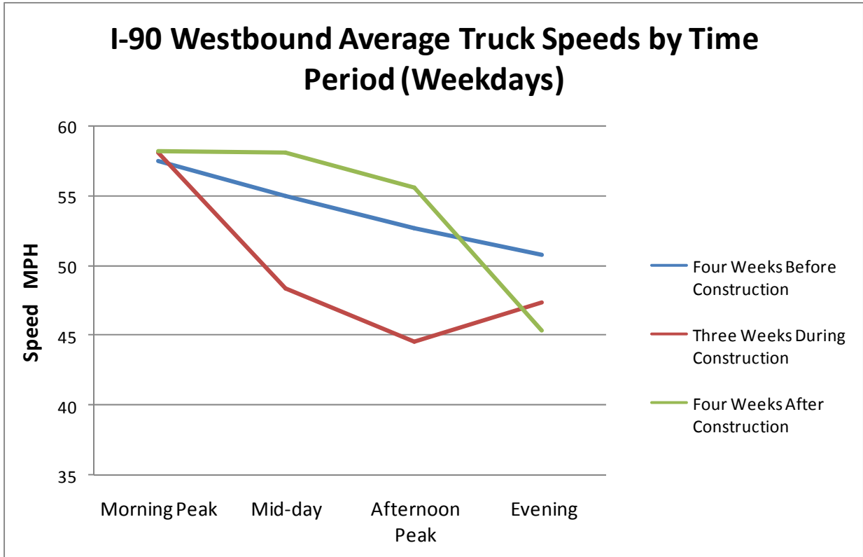
Figure A3-1: Westbound truck speed comparisons by time period
