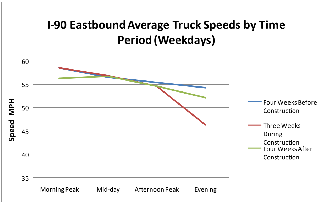
Figure A3-2: Eastbound truck speed comparisons by time period
