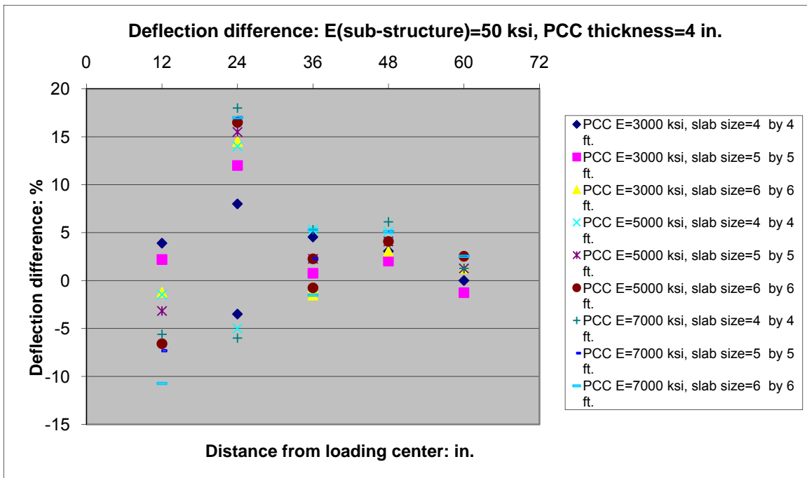
Figure 35. Plots of Deflection Differences for Sub-structure Modulus=50 ksi, PCC thickness=4 in.
