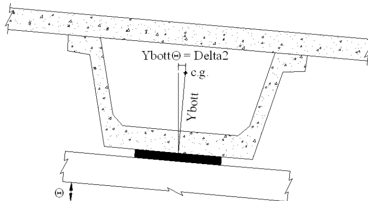
Figure 3.2 - Geometric Displacement Delta2 caused by Y_{\text{bott}}\Theta = \text{Delta2}
