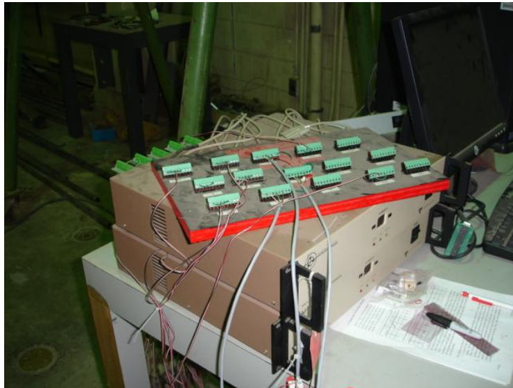
Figure 4.22 – Vishay Model 5000
