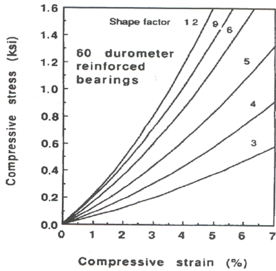
Figure C14.7.5.3.3-1 Stress-Strain Curves.
