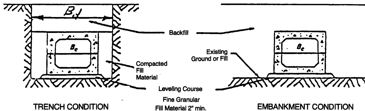
CONCRETE BOX SECTIONS FIGURE 16.6A
