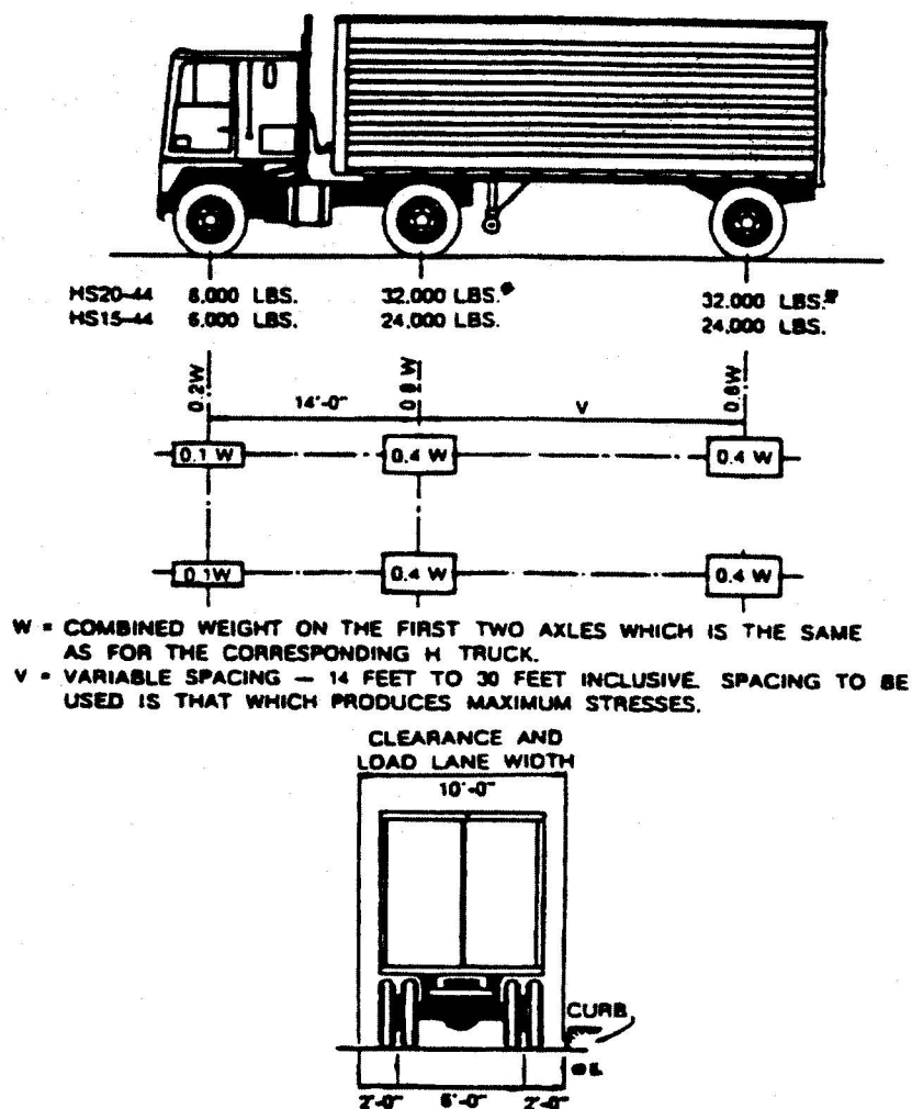
Figure 6.7.2.1 Standard HS Truck
