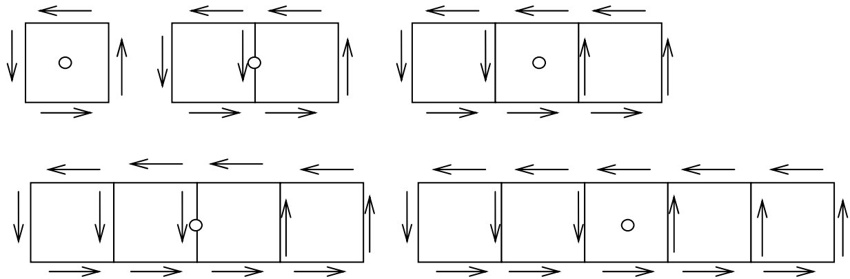
FIGURE VI.15. RISAs-2D BEAM ELEMENT LAYOUT PATTERN FOR 1, 2, 3, 4 AND 5-SPAN CULVERTS
