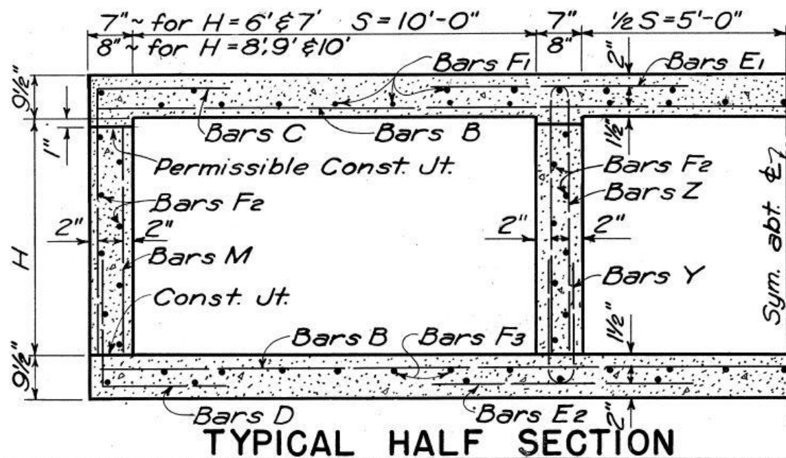
FIGURE IX.3. EXAMPLE CULVERT, DIMENSIONS FROM PLAN SHEET.
