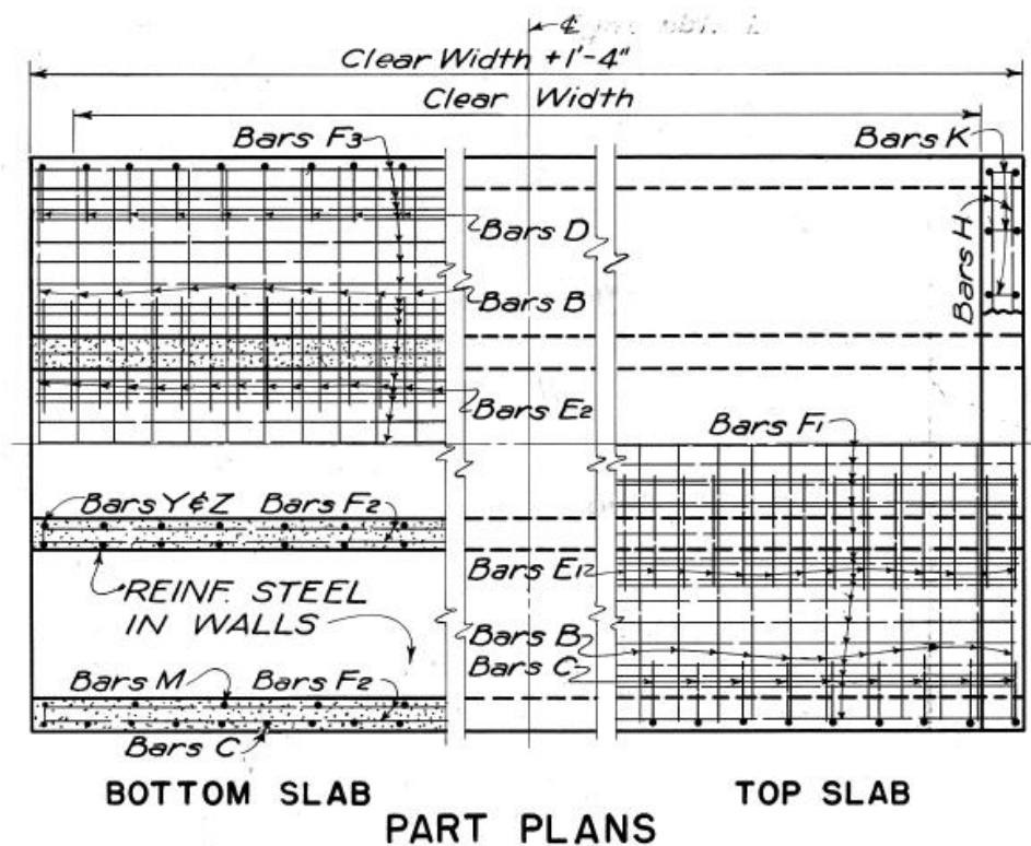
FIGURE IX.6. EXAMPLE CULVERT, DESIGNATION OF REINFORCING STEEL AS PER PLAN SHEET.
