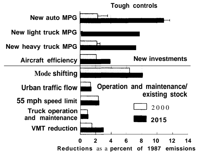
Figure 5-6--CO 2 Emissions Reductions in 2000 and 2015 Expressed as a Percentage of 1987 Transport Sector Emissions, By Control Method, Under the Tough Scenario
