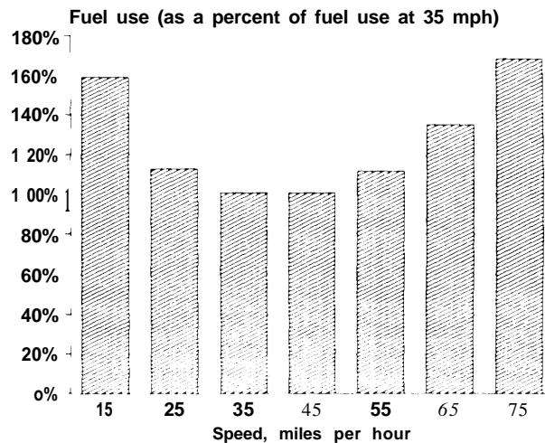
Figure 5-4—The Effect of Vehicle Speed on Fuel Consumption
