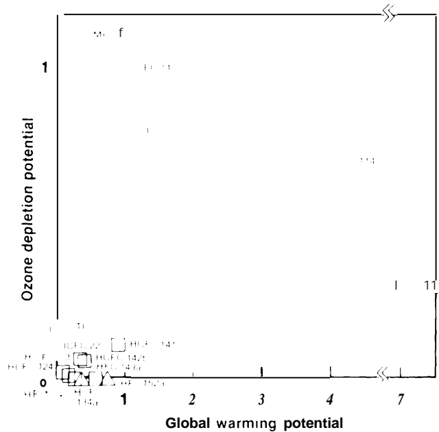
Figure 2-14—Ozone Depletion Potential and Global Warming Potential of CFCs and Replacement Compounds (HFCs and HCFCs)
