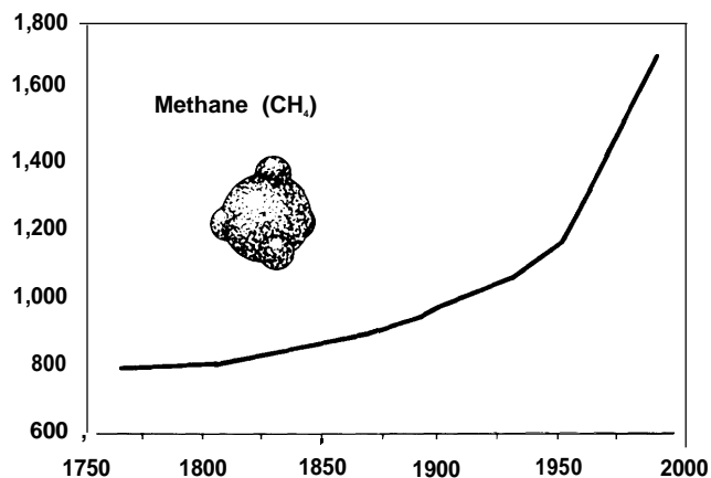
Figure 2-10-Atmospheric: Methane Concentration (parts per billion by volume)
