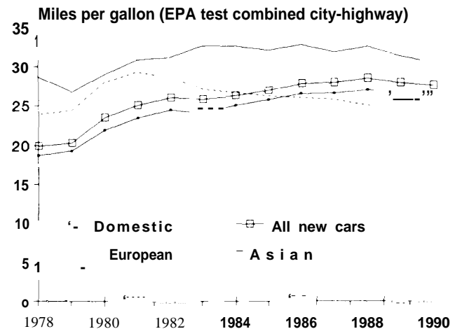
Figure 5-3-Trends in New Passenger Car Fuel Economy, 1978-90
