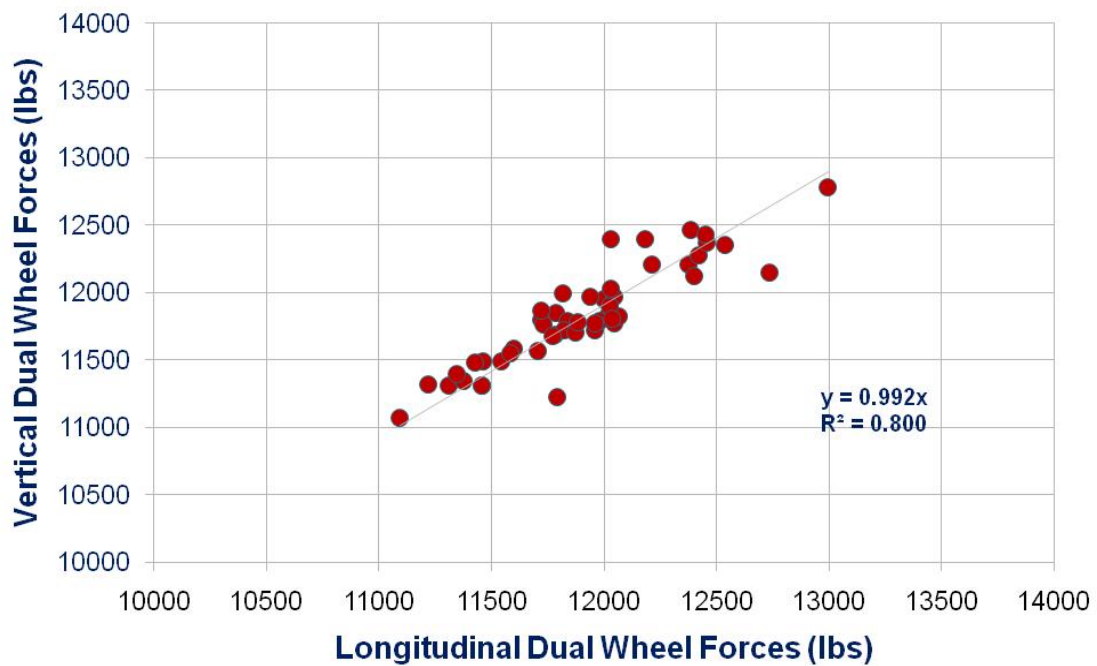
Figure 41. Relationship between Vertical and Longitudinal Wheel Forces.
