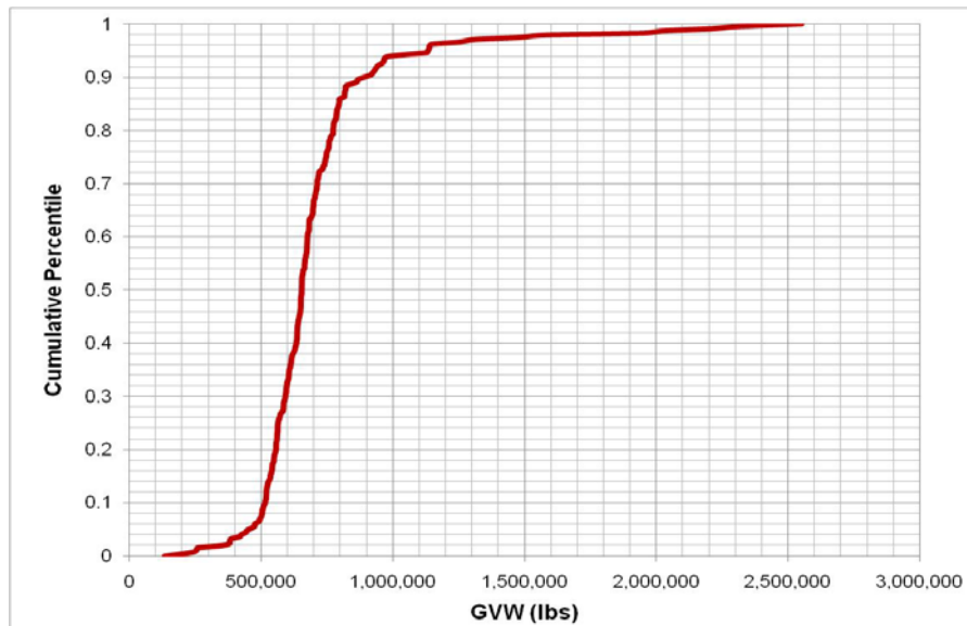
Figure 43. Cumulative Percentile of GVW.
