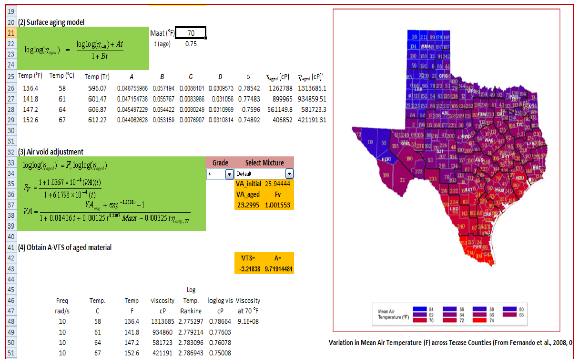
Figure C2. Select Binder Type for A-VTS Coefficient Calculation and MAAT.
