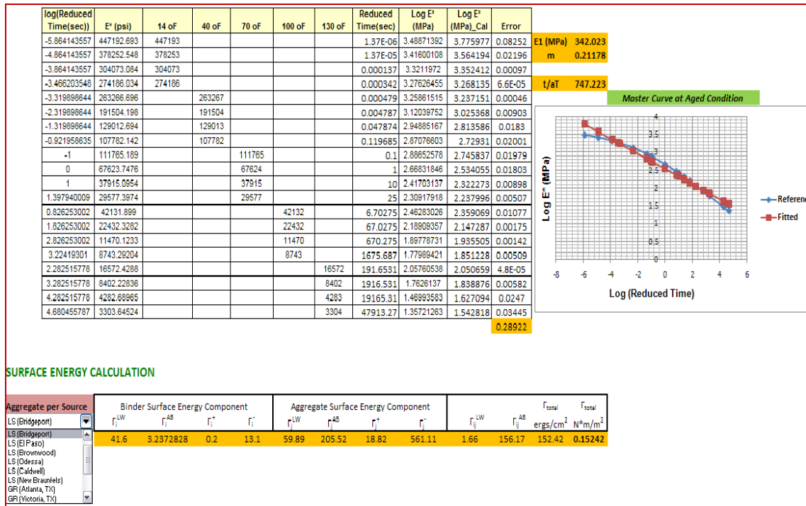
Figure C5. Select Aggregate Sources for Surface Energy Calculation.
