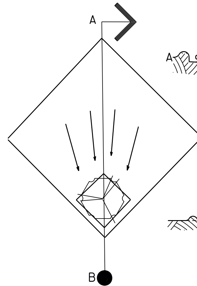
MICRO-CATCHMENT PLAN VIEW NOT TO SCALE
