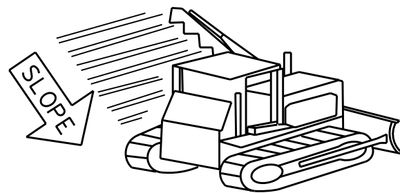
DOZER EQUIPPED WITH SPECIAL BLADE CREATES GROOVES PERPENDICULAR TO SLOPE
