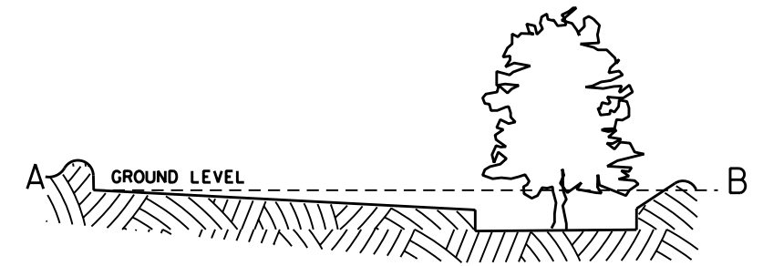
MICRO-CATCHMENT CROSS SECTION WITH TREE PLANTING NOT TO SCALE
