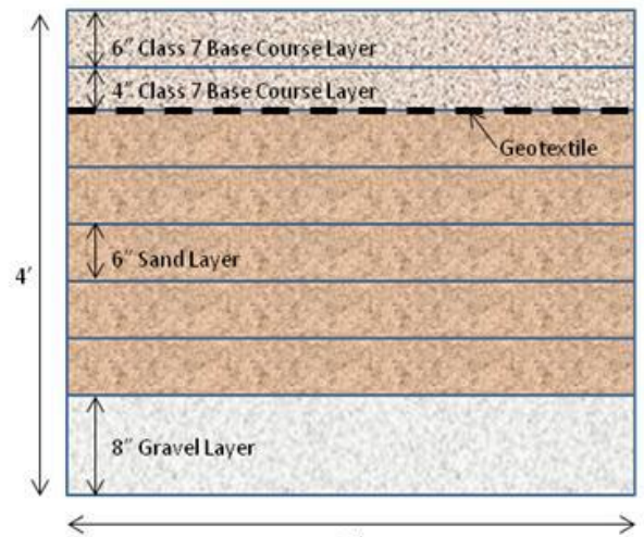
Figure 4.8: Location of geotextile reinforcement.
