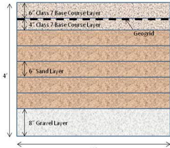
Figure 4.7: Location of geogrid reinforcement.
