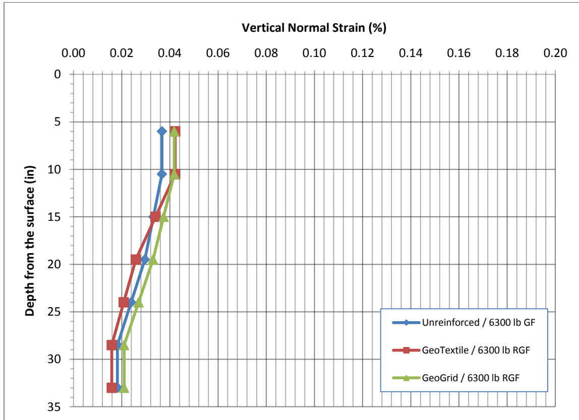
Figure 3.41: Comparison of vertical normal stain versus depth in each test section after adjusting all strains to a reference ground force (RGF) of 6300 lbs.
