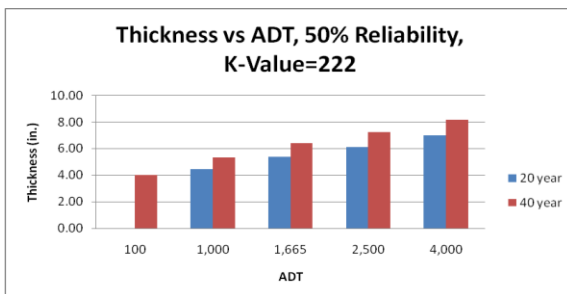
(e) k-value=222 (Reliability: 50%)
