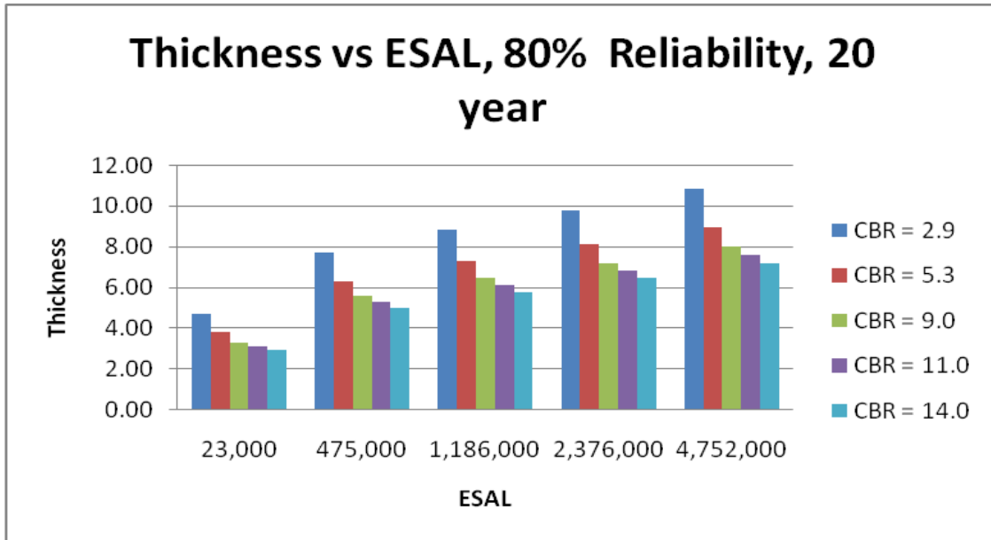
Figure 4-14. Impact of traffic level and subgrade strength on asphalt pavement thickness given reliability of 80% and design life of 20 years
