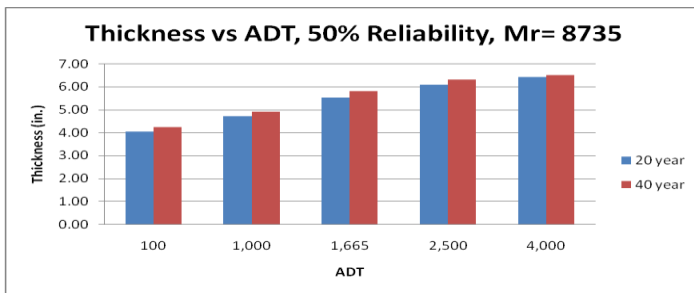
(c) Mr=8735 (Reliability: 50%)
