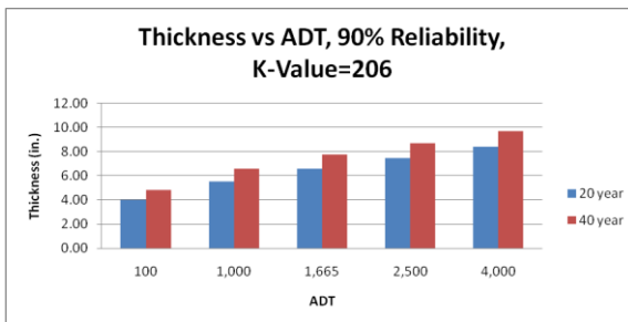
(m) k-value=206 (Reliability: 90%)
