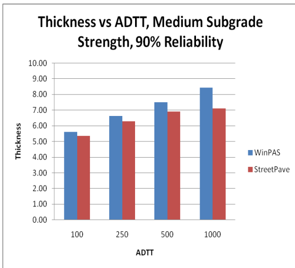
(h) Medium subgrade (Reliability=90%)
