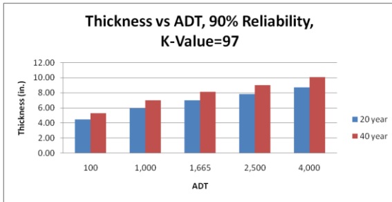
(k) k-value=97 (Reliability: 90%)
