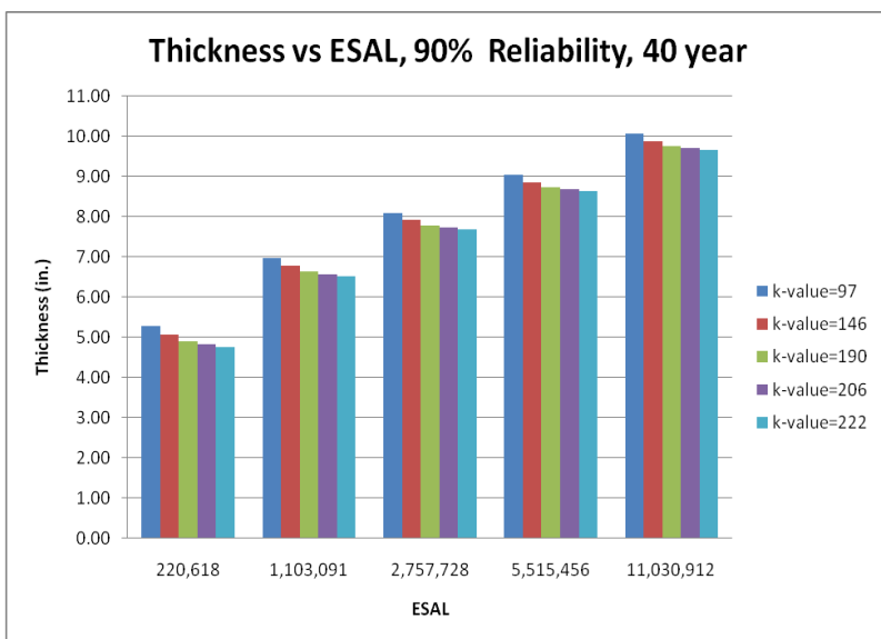
(h) Reliability: 90%
