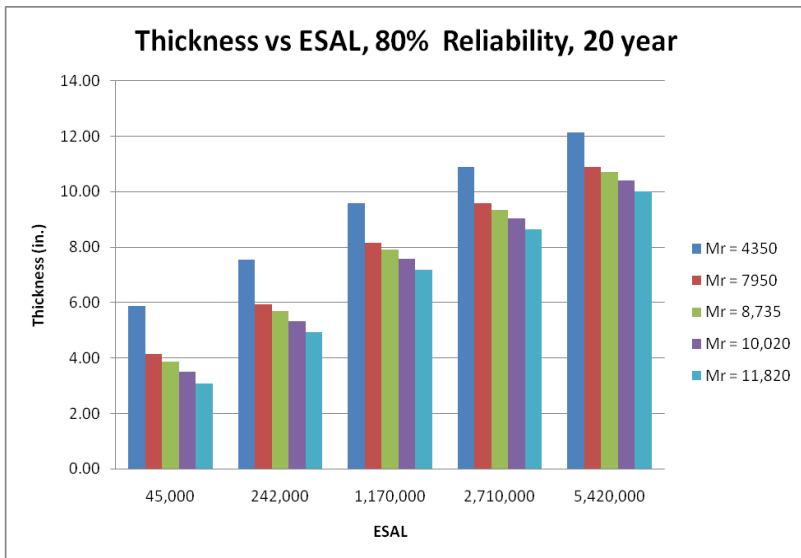
(g) Reliability: 80%
