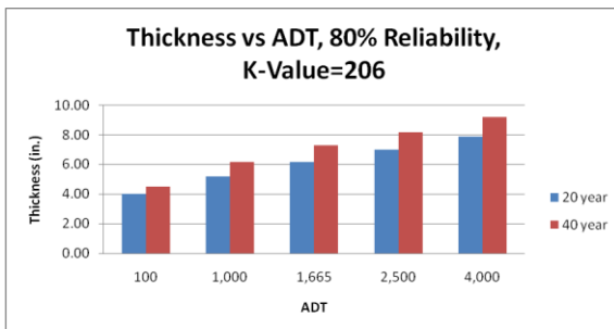
(i) k-value=206 (Reliability: 80%)
