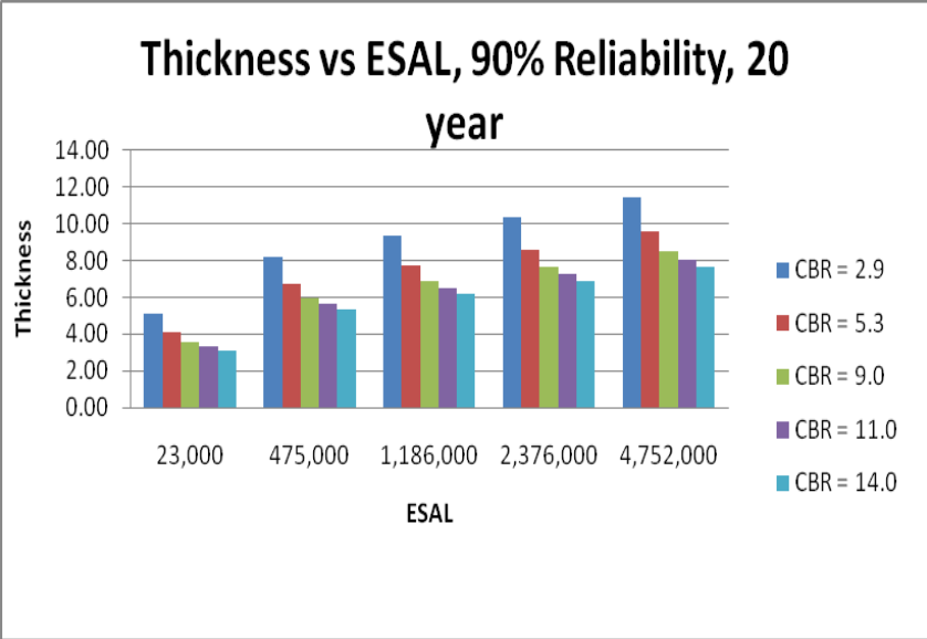
(g) Reliability: 90%
