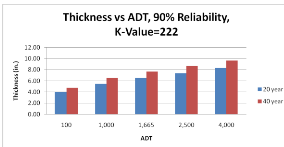
(o) k-value=222 (Reliability: 90%)
