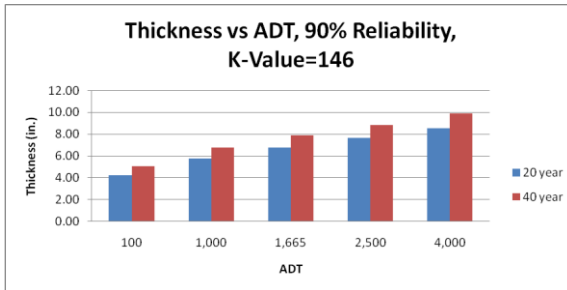
(l) k-value=146 (Reliability: 90%)
