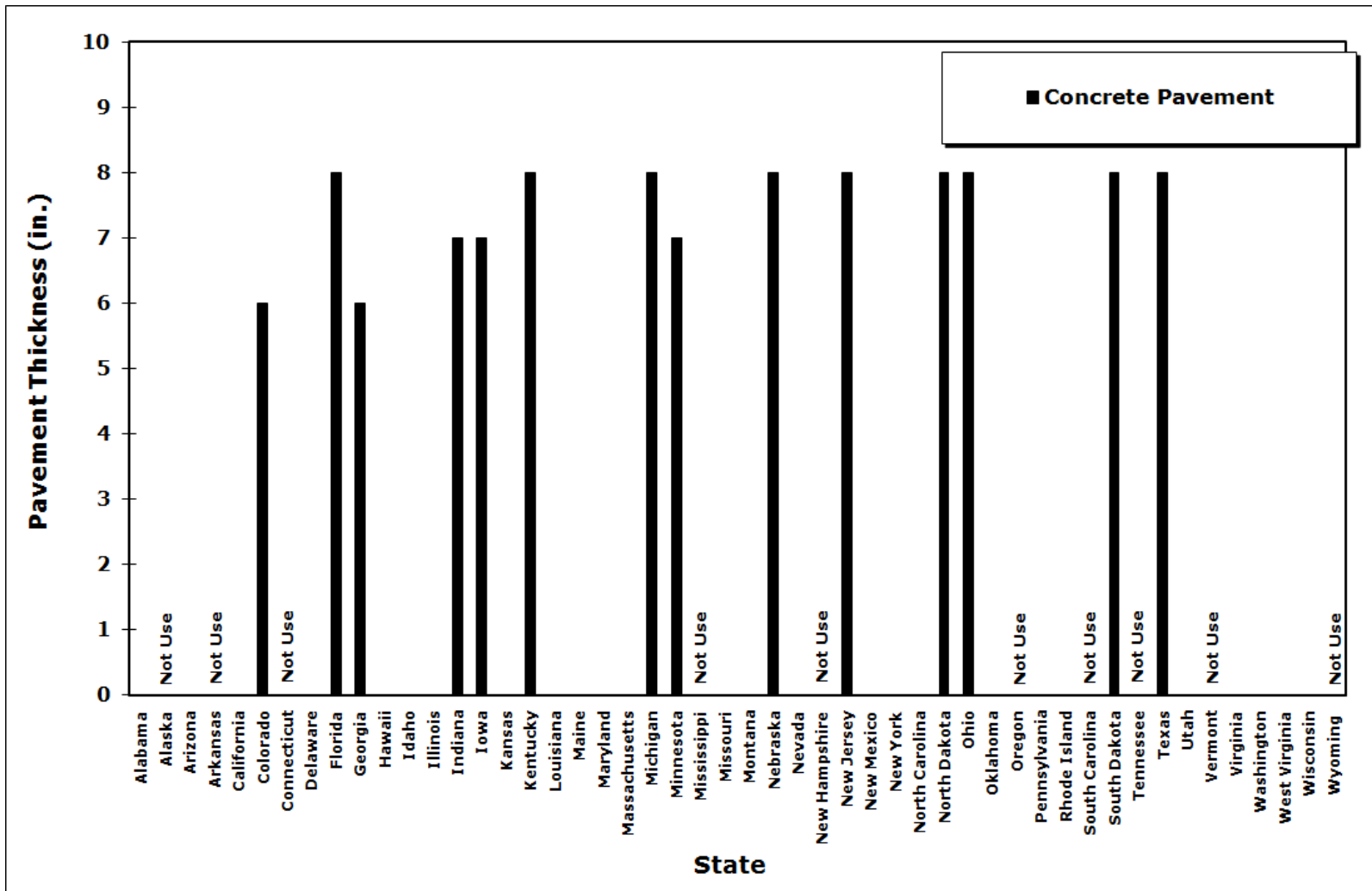
Figure A-3. Comparisons of minimum thickness for concrete pavement from 24 states
