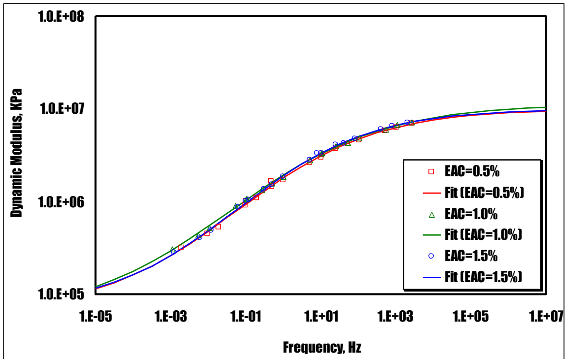
Figure 8-9. Mater curves for CIR- HFMS-2p from Story County at three EACs
