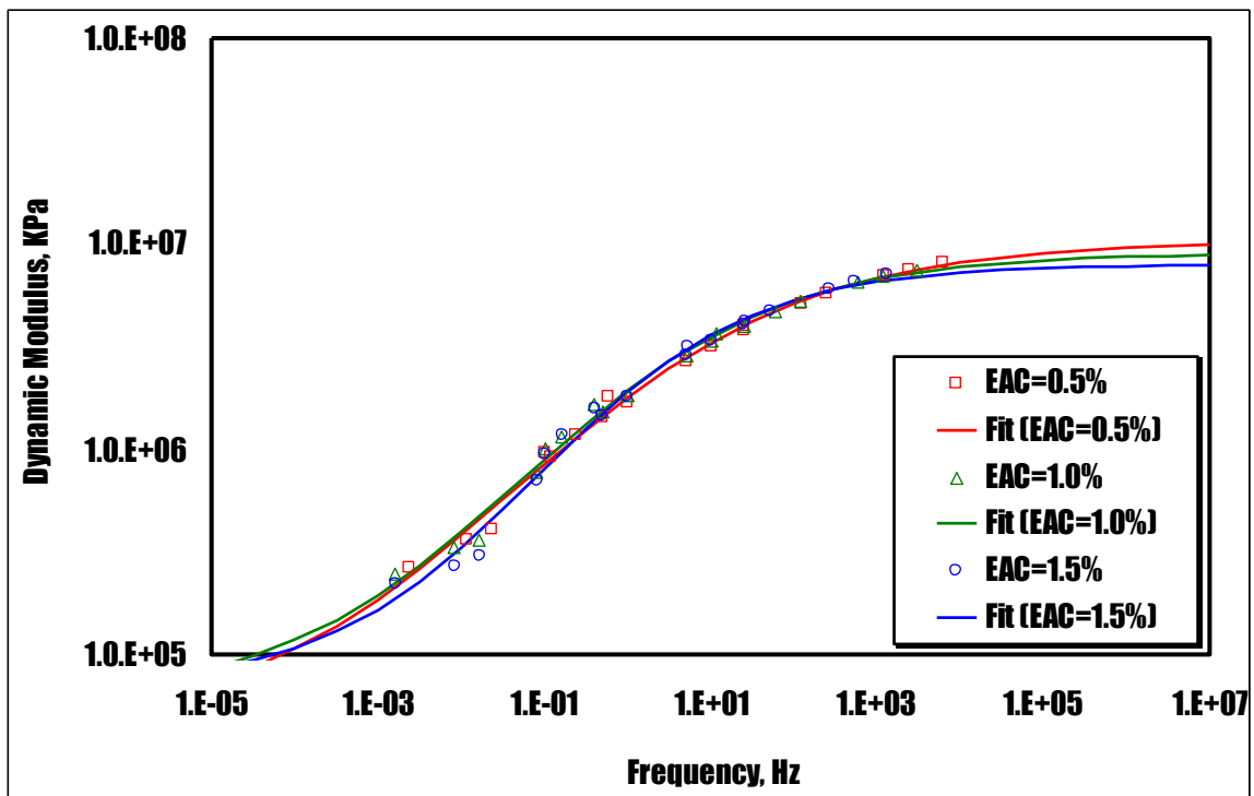
Figure 8-7. Mater curves for CIR-CSS-1h from Story County at three EACs
