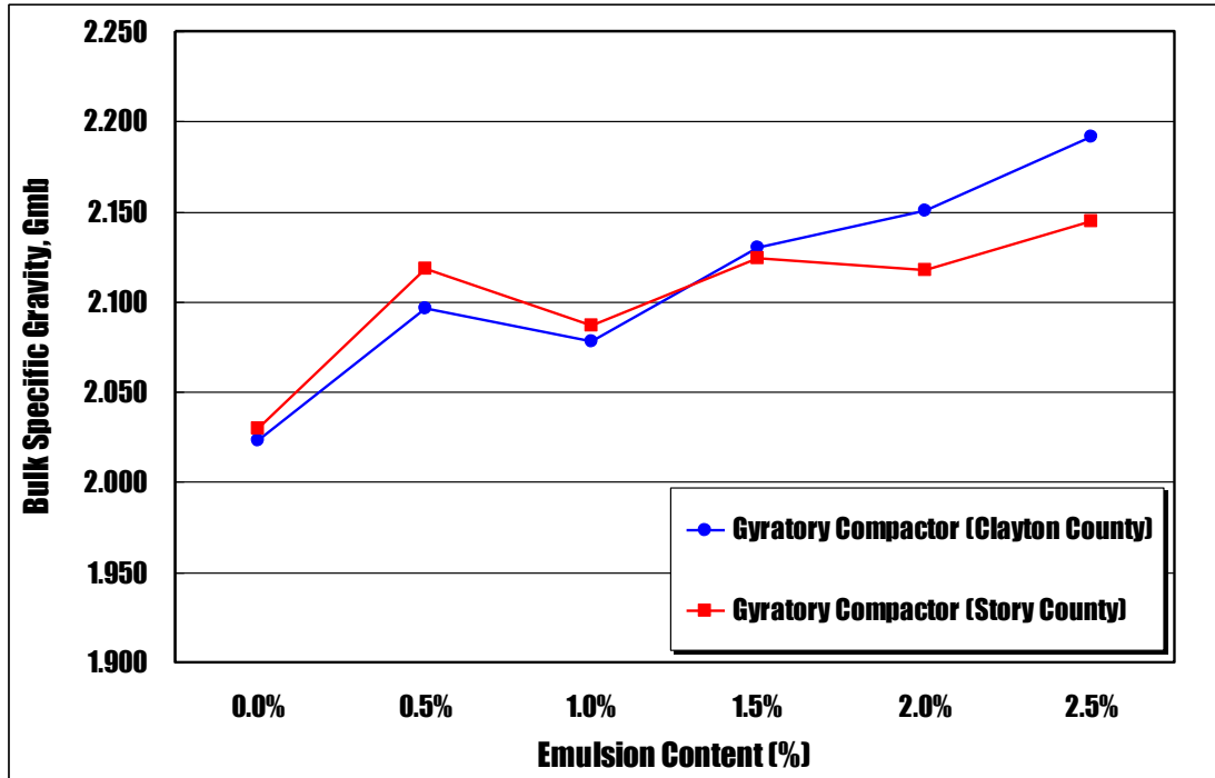
Figure 7-3. Plots of bulk specific gravity against emulsified asphalt content for gyratory compacted CIR-HEMS-2p specimens using different RAP materials
