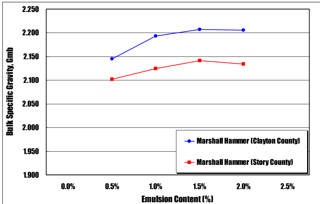
Figure 7-4. Plots of bulk specific gravity against emulsified asphalt content for Marshall compacted CIR-HFMS-2p specimens using different RAP materials
