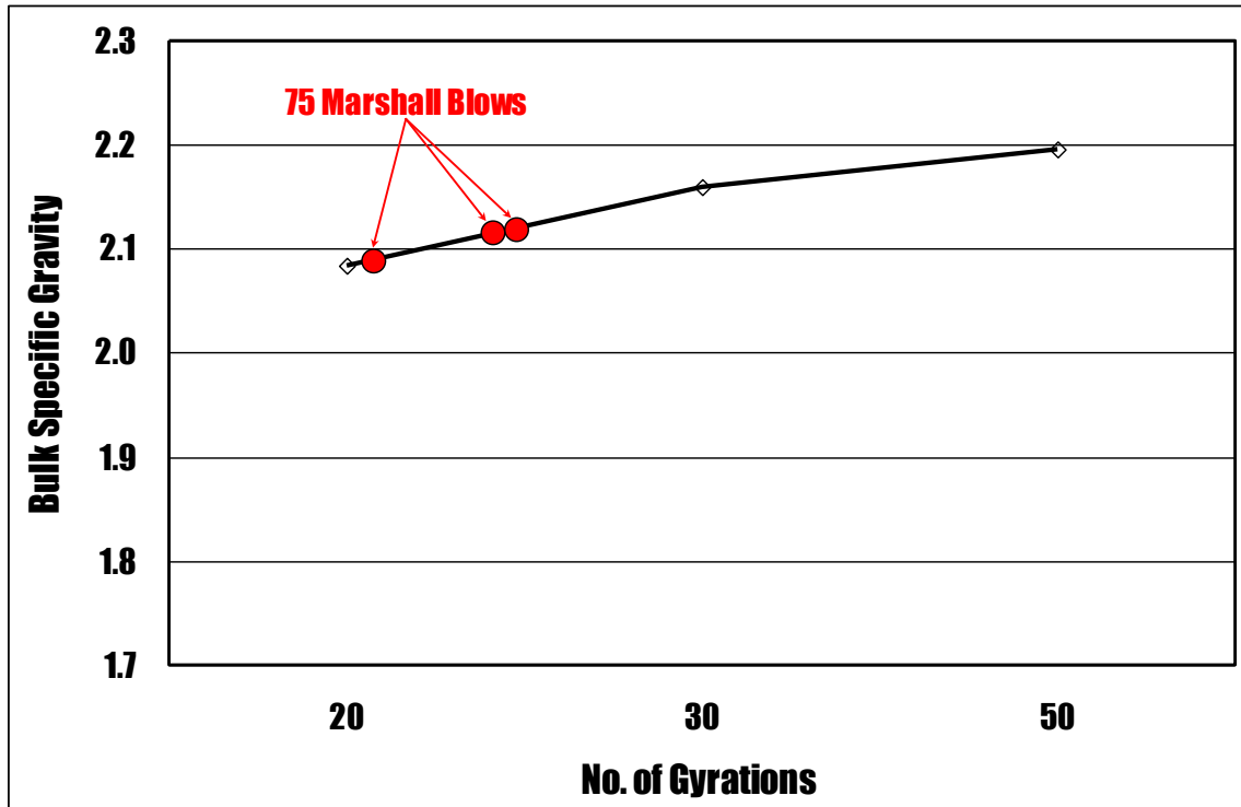
Figure 6-1. Plots of average bulk specific gravities against different number of gyrations
