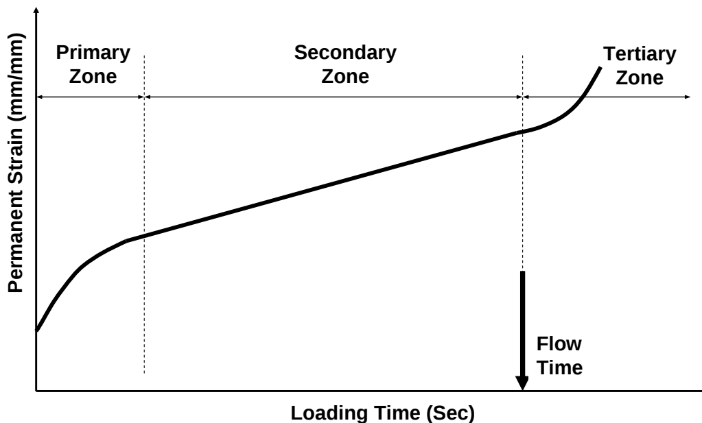
Figure 8-15. Permanent deformation behavior against loading time
