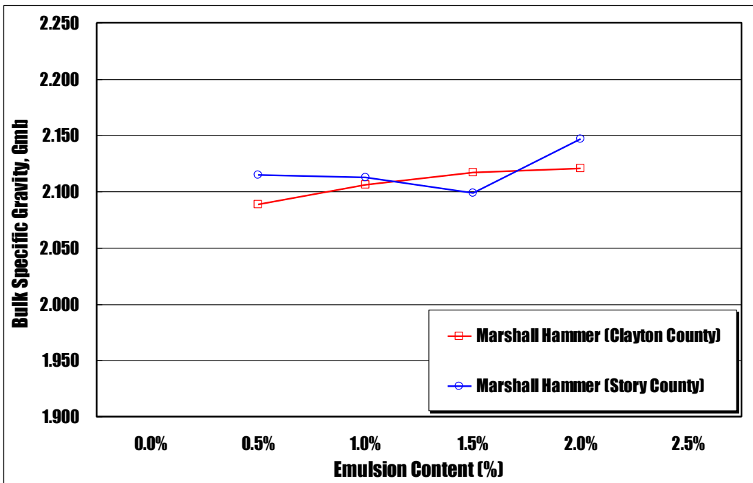
Figure 7-2. Plots of bulk specific gravity against emulsified asphalt content for Marshall compacted CIR-CSS-1h specimens using different RAP materials
