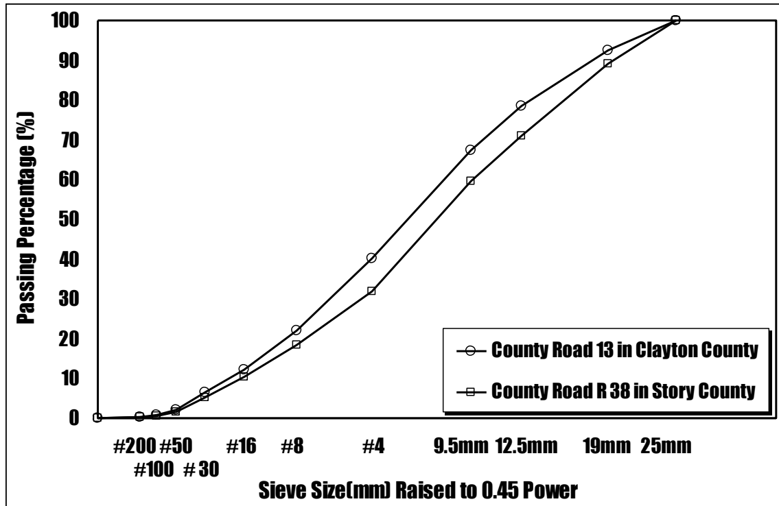
Figure 5-3. Gradation plots of two RAP materials passing 25mm sieve
