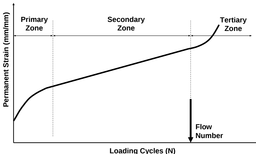
Figure 8-11. Permanent deformation behavior against loading cycles
