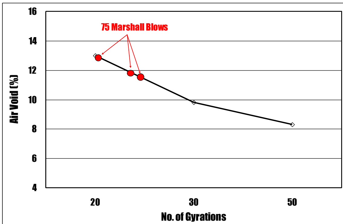
Figure 6-2. Plots of average air voids against different number of gyrations
