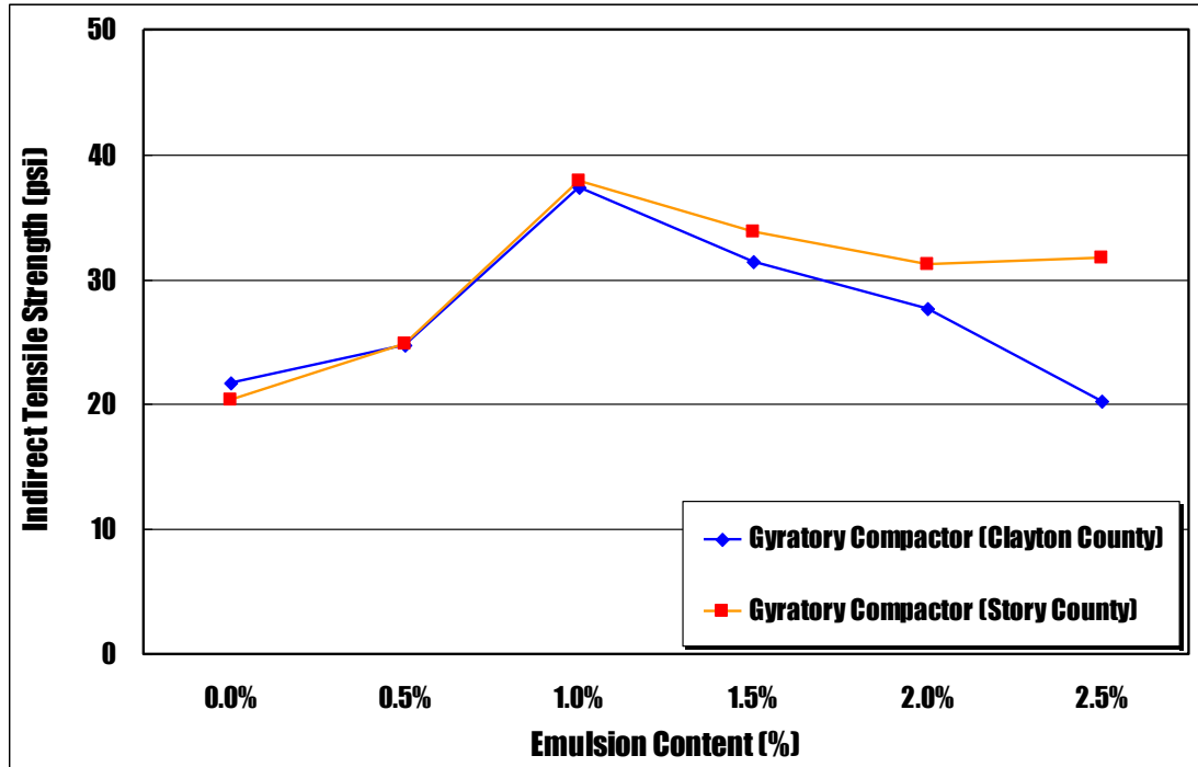
Figure 7-13. Plots of indirect tensile strength against emulsified asphalt content for gyrotory compacted CIR- HFMS-2p specimens using two different RAP materials
