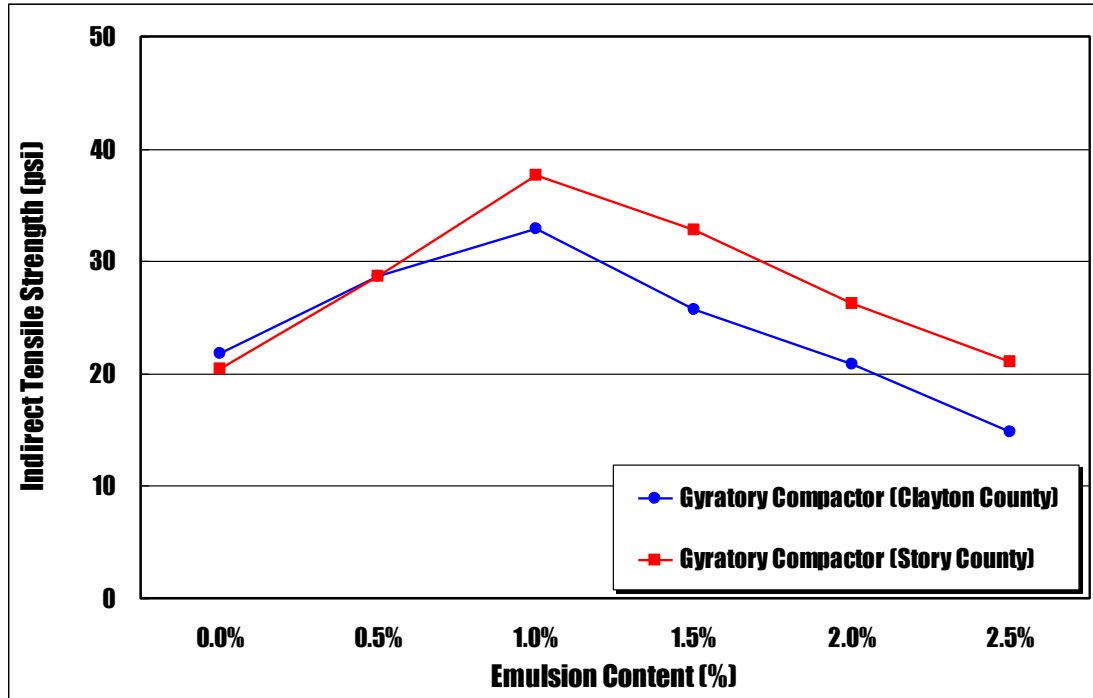
Figure 7-11. Plots of indirect tensile strength against emulsified asphalt content for Gyratory compacted CIR-CSS-1 specimens using two different RAP materials
