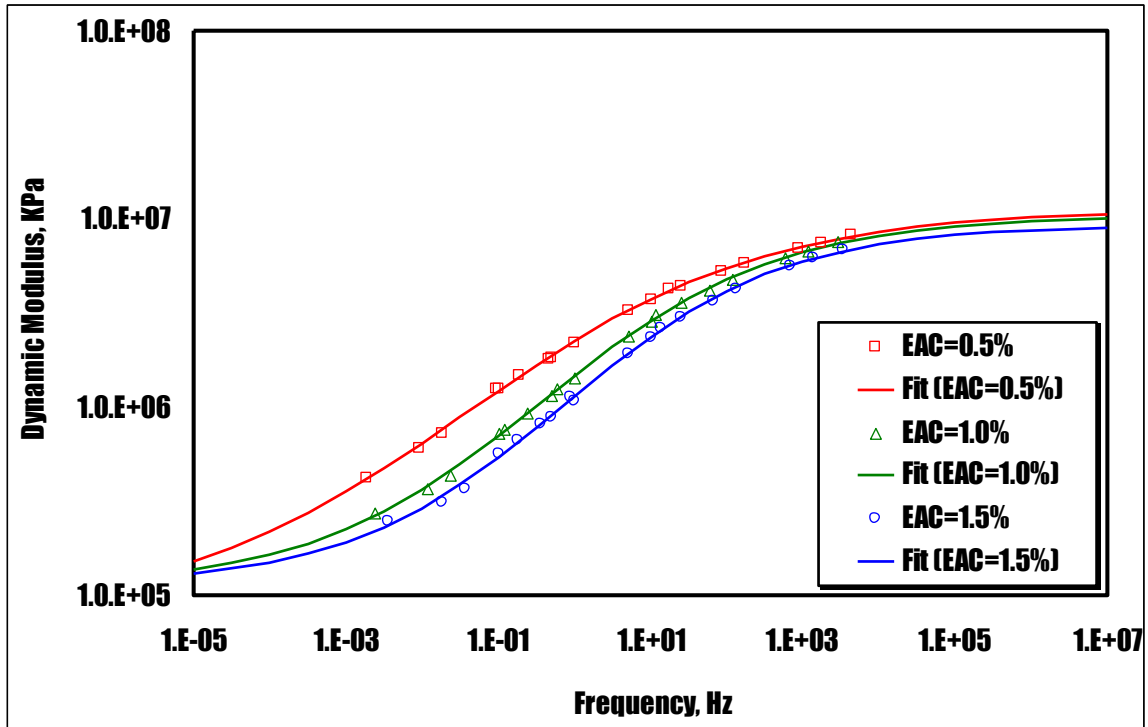
Figure 8-8. Mater curves for CIR-HFMS-2p from Clayton County at three EACs
