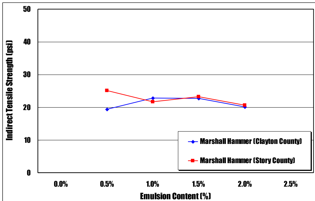
Figure 7-14. Plots of indirect tensile strength against emulsified asphalt content for Marshall compacted CIR- HFMS-2p specimens using two different RAP materials
