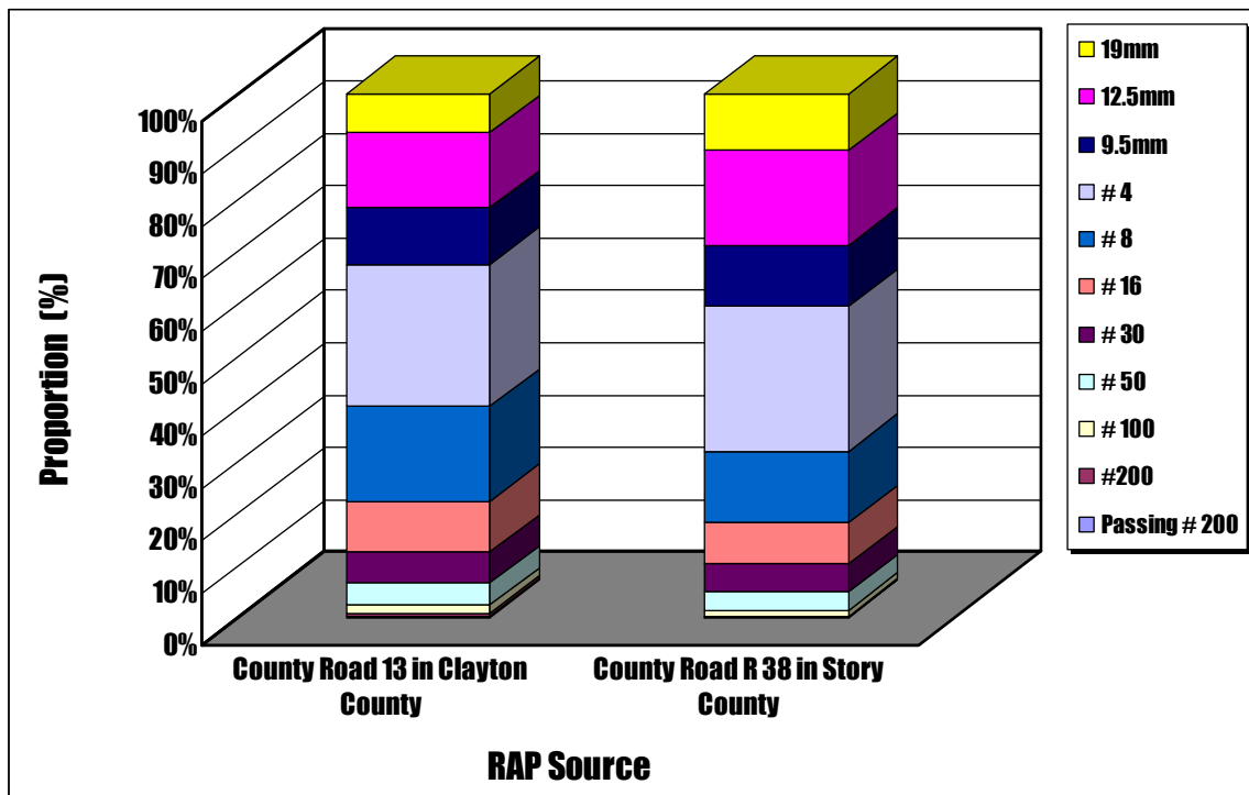
Figure 5-4. Cumulated gradation bar charts of seven different RAP materials passing 25mm sieve
