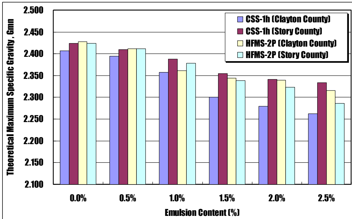
Figure 7-5. Bar charts of theoretical maximum specific gravities against emulsified asphalt content for two emulsion types and two RAP sources
