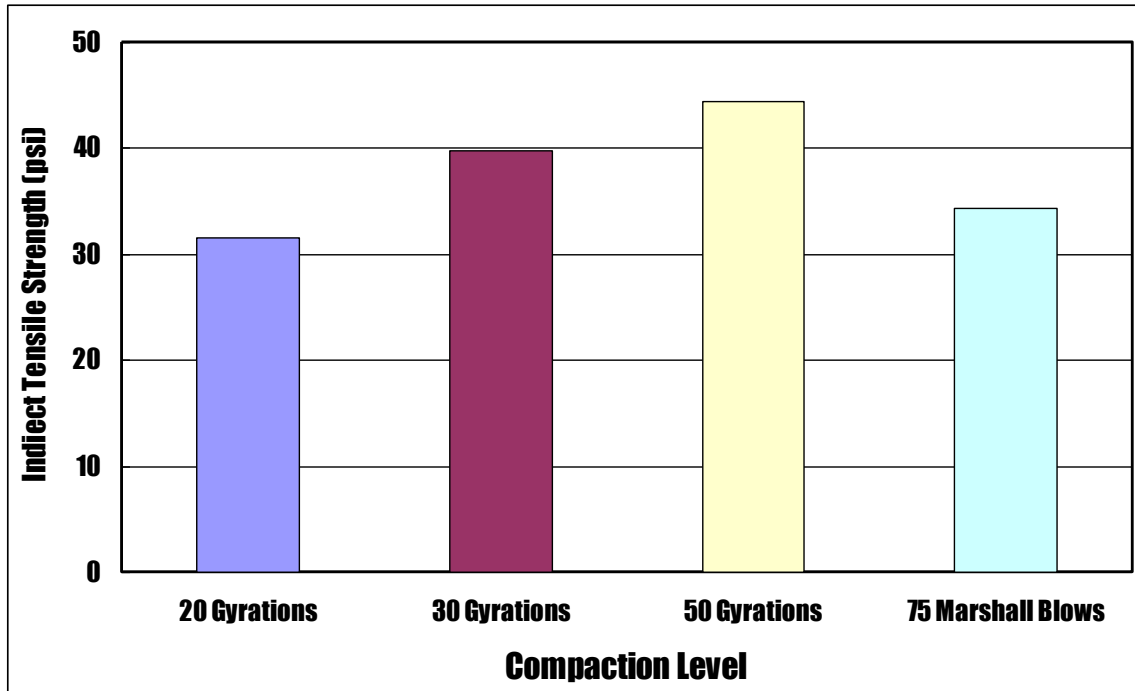
Figure 6-3. Comparison of average indirect tensile strength at four different compaction levels
