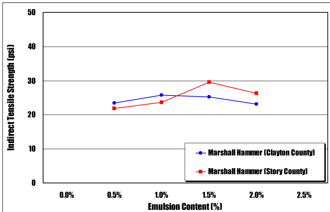
Figure 7-12. Plots of indirect tensile strength against emulsified asphalt content for Marshall compacted CIR-CSS-1 specimens using two different RAP materials
