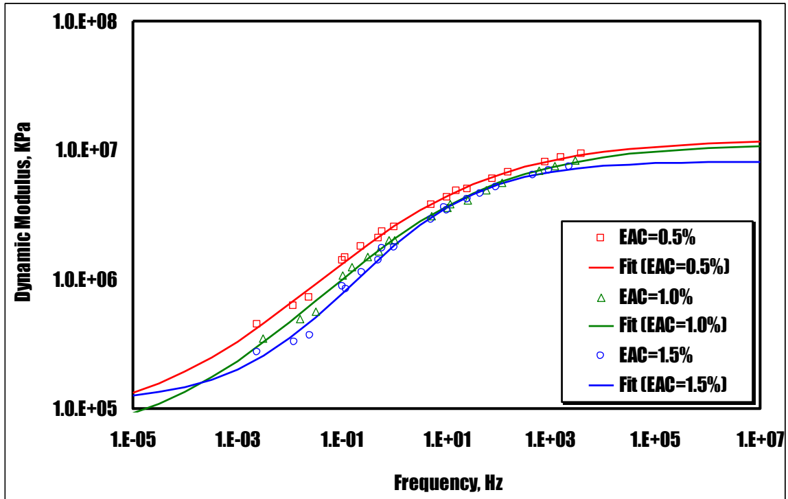
Figure 8-6. Mater curves for CIR-CSS-1h from Clayton County at three EACs
