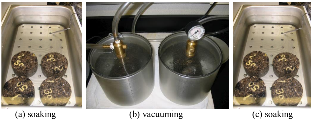
Figure 7-10. Vacuum saturation procedure for making wet specimens
