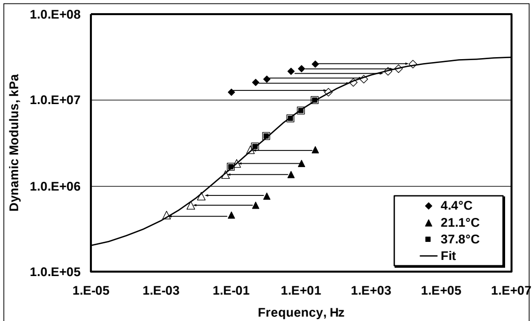
Figure 8-1. Construction of master curve
