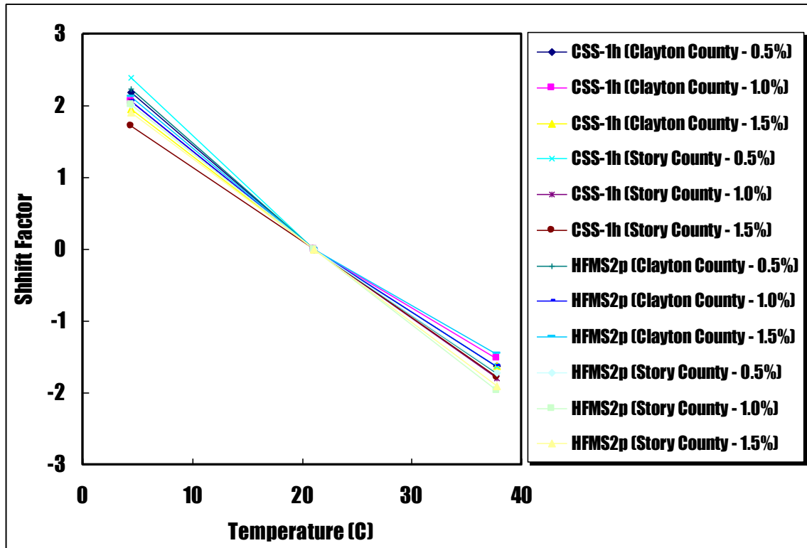
Figure 8-10. Shift factors against three temperatures
