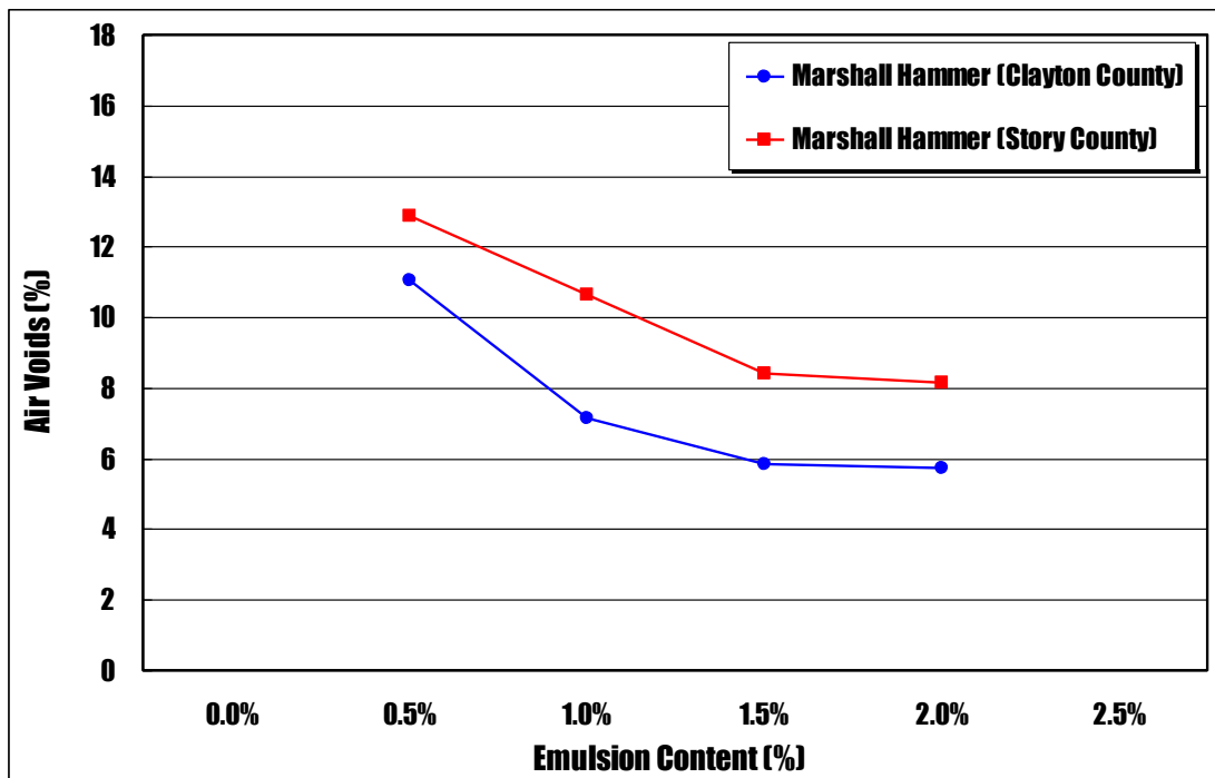
Figure 7-9. Plots of air void against emulsified asphalt content for Marshall compacted HFMS-2p specimens using two different RAP materials
