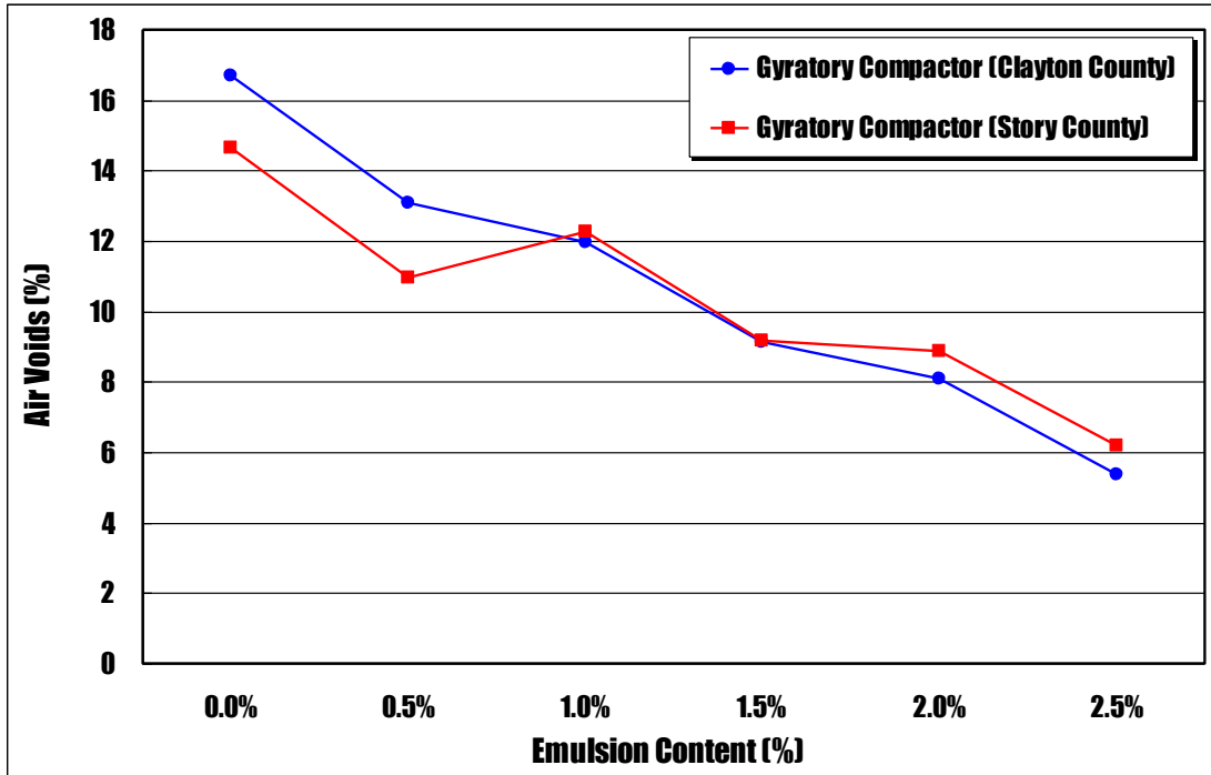
Figure 7-8. Plots of air void against emulsified asphalt content for gyratory compacted CIR-HFMS-2p specimens using two different RAP materials
