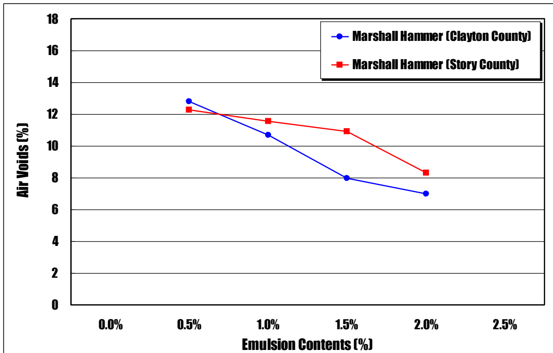
Figure 7-7. Plots of air void against emulsified asphalt content for Marshall compacted CIR-CSS-1h specimens using two different RAP materials
