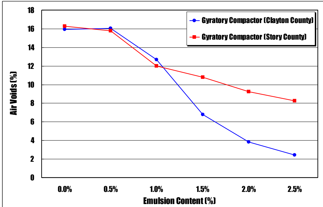
Figure 7-6. Plots of air void against emulsified asphalt content for gyratory compacted CIR-CSS-1h specimens using two different RAP materials
