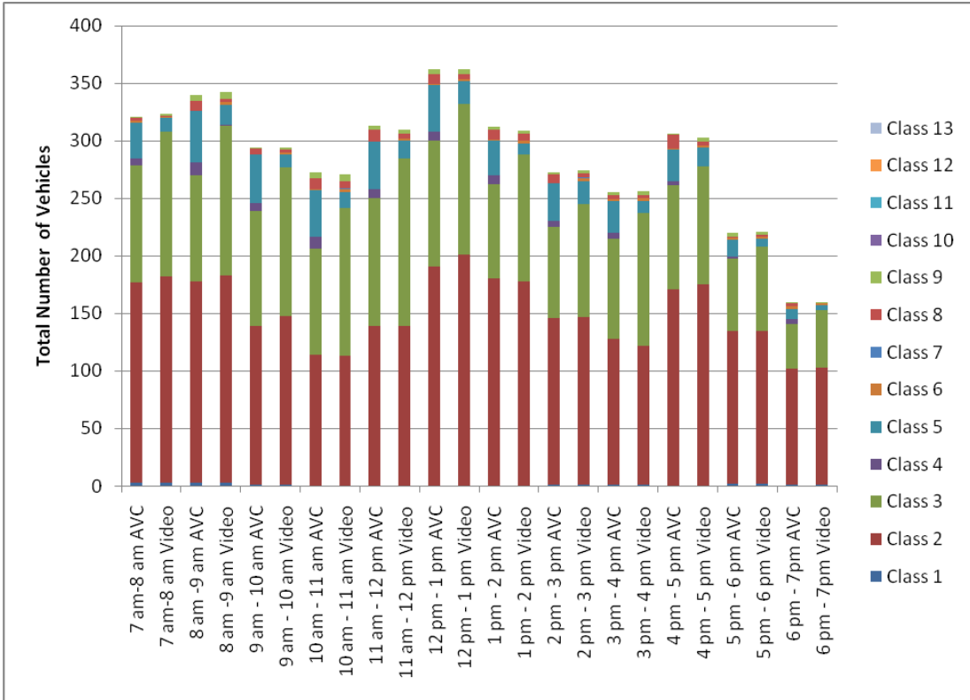
Figure 53. Site 2 Westbound – AVC vs Video Classification Counts by 1-Hour Interval.
