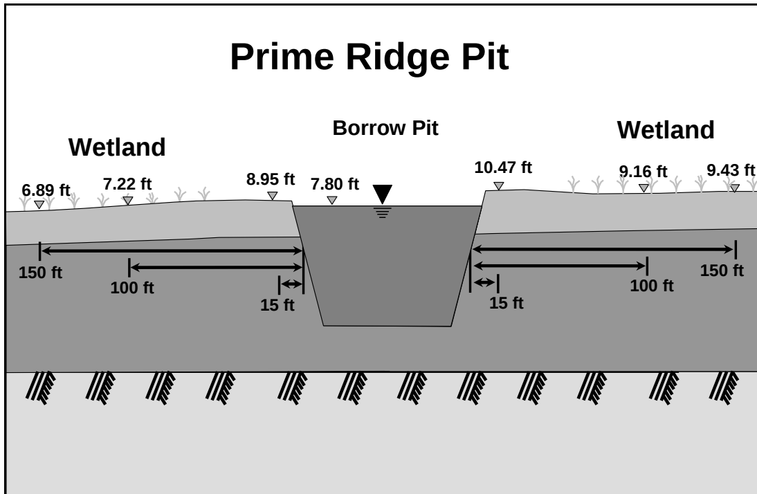
Figure 24. Type 3 – Wetlands both upslope and down slope of pit. Vann Pit. Prime Ridge Pit. Ground surface elevation of one wetland is lower than pit water level, and ground surface elevation of other wetland is higher than pit water level.
