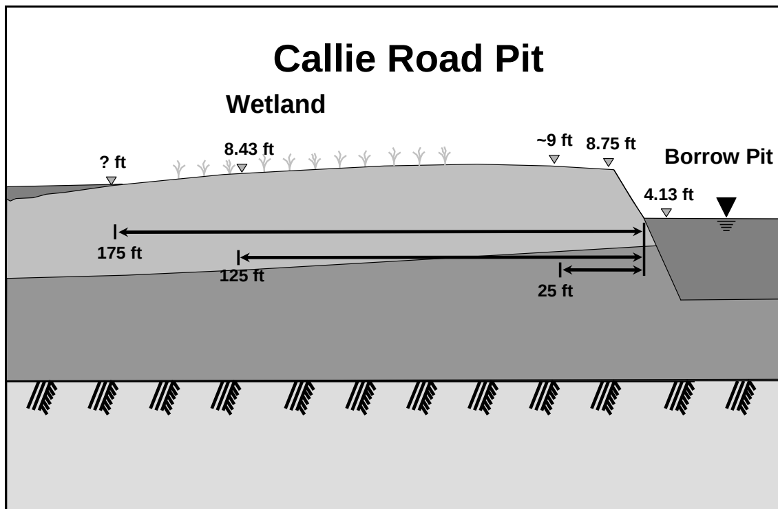
Figure 15. Type 1 - Wetland upslope of pit. Callie Road Pit. Ground surface of wetland at higher elevation than pit water level. Limit of pit water level not determined.
