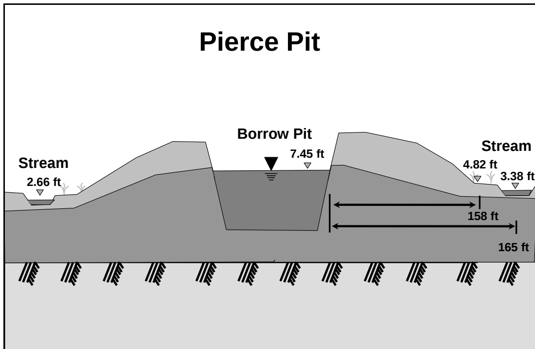
Figure 13. Type 2 - Wetland down slope of pit. Pierce Pit. Ground surface of wetland at lower elevation than pit water level. Wetland on the floodplain of the streams. Pit is located on a ridge between streams.
