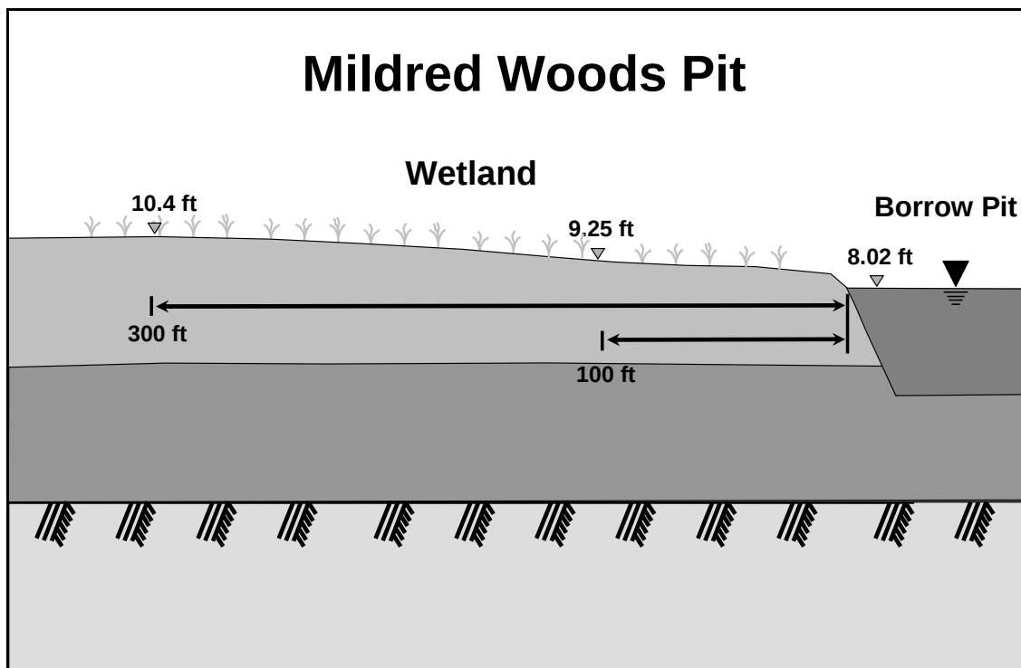
Figure 9. Type 1a – Wetland upslope of pit. Mildred Woods Pit. Ground surface of wetland at higher elevation than pit water level. Water level of pit controlled by elevation of outlet.
