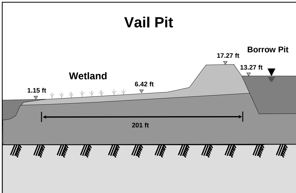
Figure 10. Type 2 - Wetland down slope of pit. Vail Pit. Ground surface of wetland at lower elevation than pit water level. Wetland on the floodplain of the stream.
