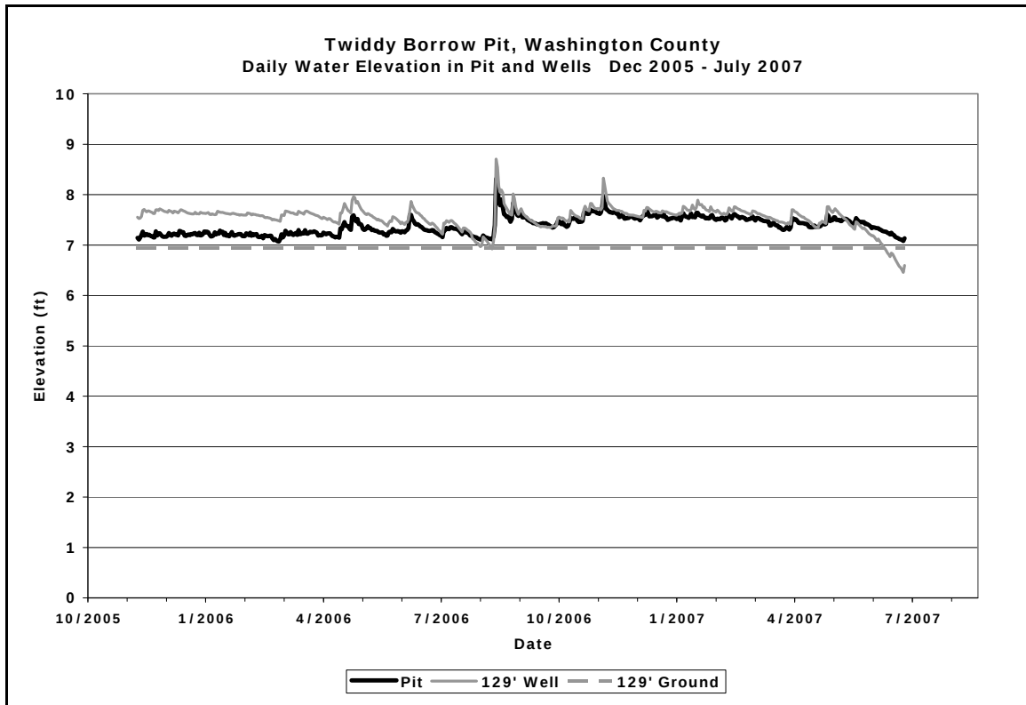
Figure 34. Water table and pond elevations (referenced to 6.5 ft below the base of the pond staff) for December 2005 to July 2007 at the Twiddy borrow pit. Well at 129' refer to wells located 129 ft. from the edge of pit.
