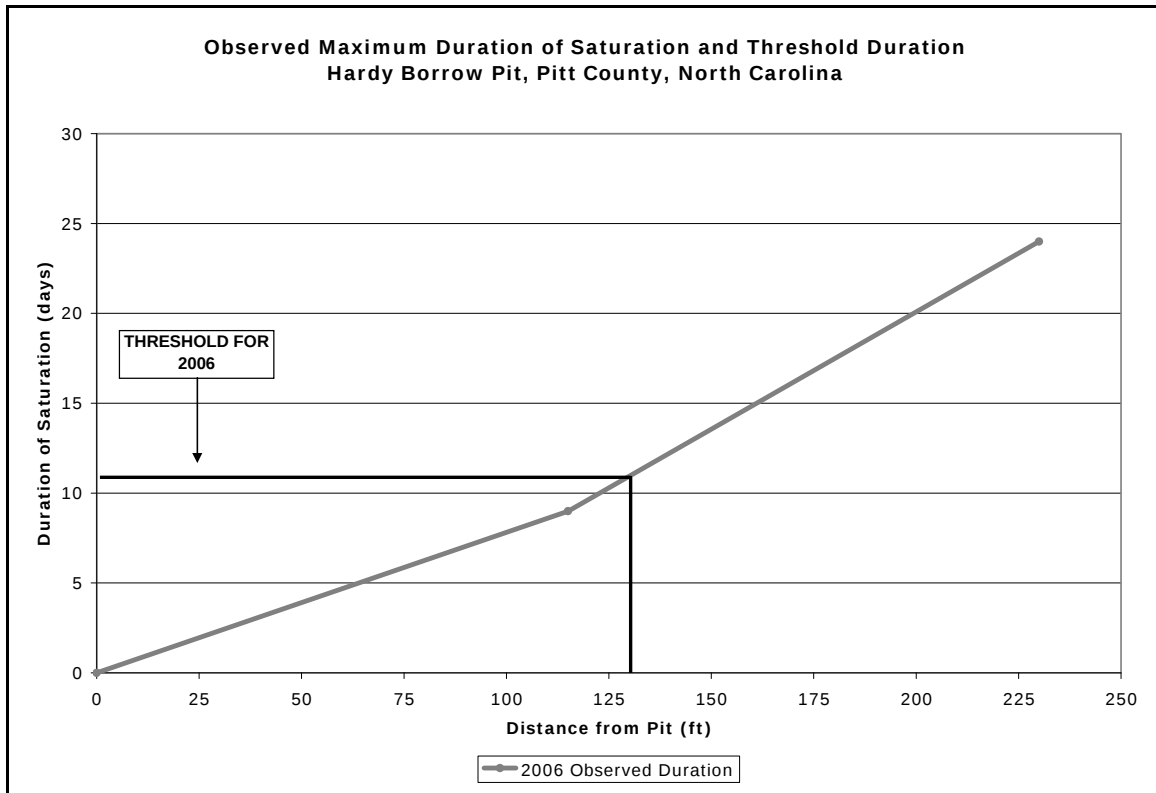
Figure 36. Observed consecutive number of days with water table within 1 ft of surface as a function of distance from ditch. Threshold values are the number of consecutive days that a site that barely satisfies the criterion would have in each year.
