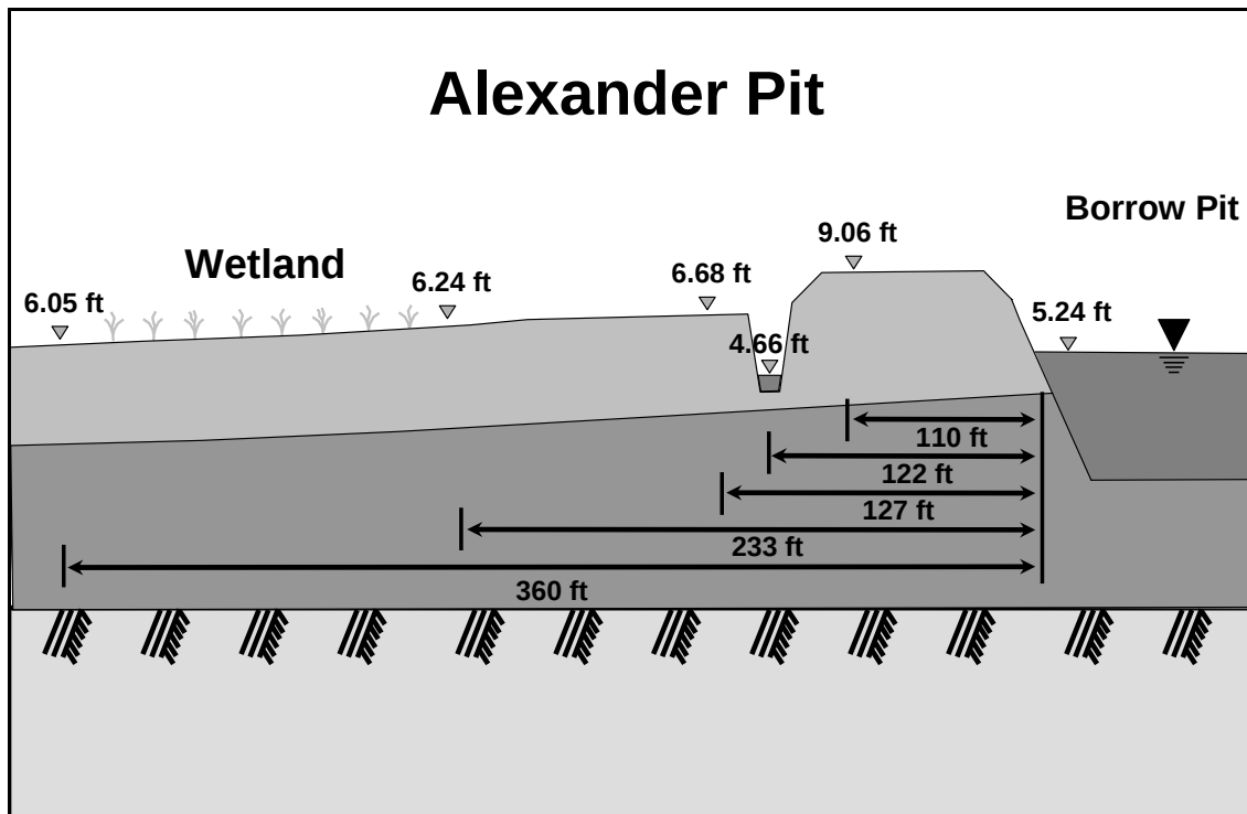
Figure 5. Type 1b - Wetland upslope of pit. Alexander Pit. Ground surface of wetland at higher elevation than pit water level. Water level of pit limited by seepage to ditch. Note that the ditch between the wetland and the pit.
