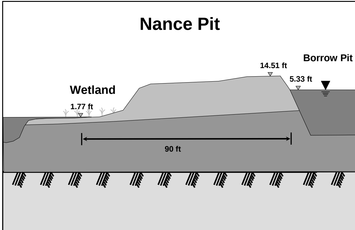
Figure 19. Type 2 - Wetland down slope of pit. Nance Pit. Ground surface of wetland at lower elevation than pit water level. Wetland on the floodplain of the stream.
