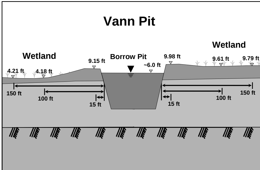
Figure 15. Type 3 – Wetlands both upslope and down slope of pit. Vann Pit. Ground surface elevation of one wetland is lower than pit water level, and ground surface elevation of other wetland is higher than pit water level.
