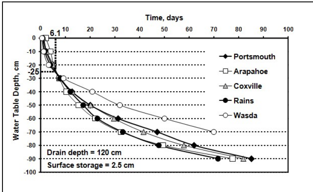
Figure 3. Predicted midpoint water table drawdown for threshold ditch spacings of 5 North Carolina soils. Results are for a ditch depth of 120 cm and surface storage of S = 2.5 cm. Time for water table drawdown of 25 cm ( T_{25} ) is approximately 6.1 days for all soils.
