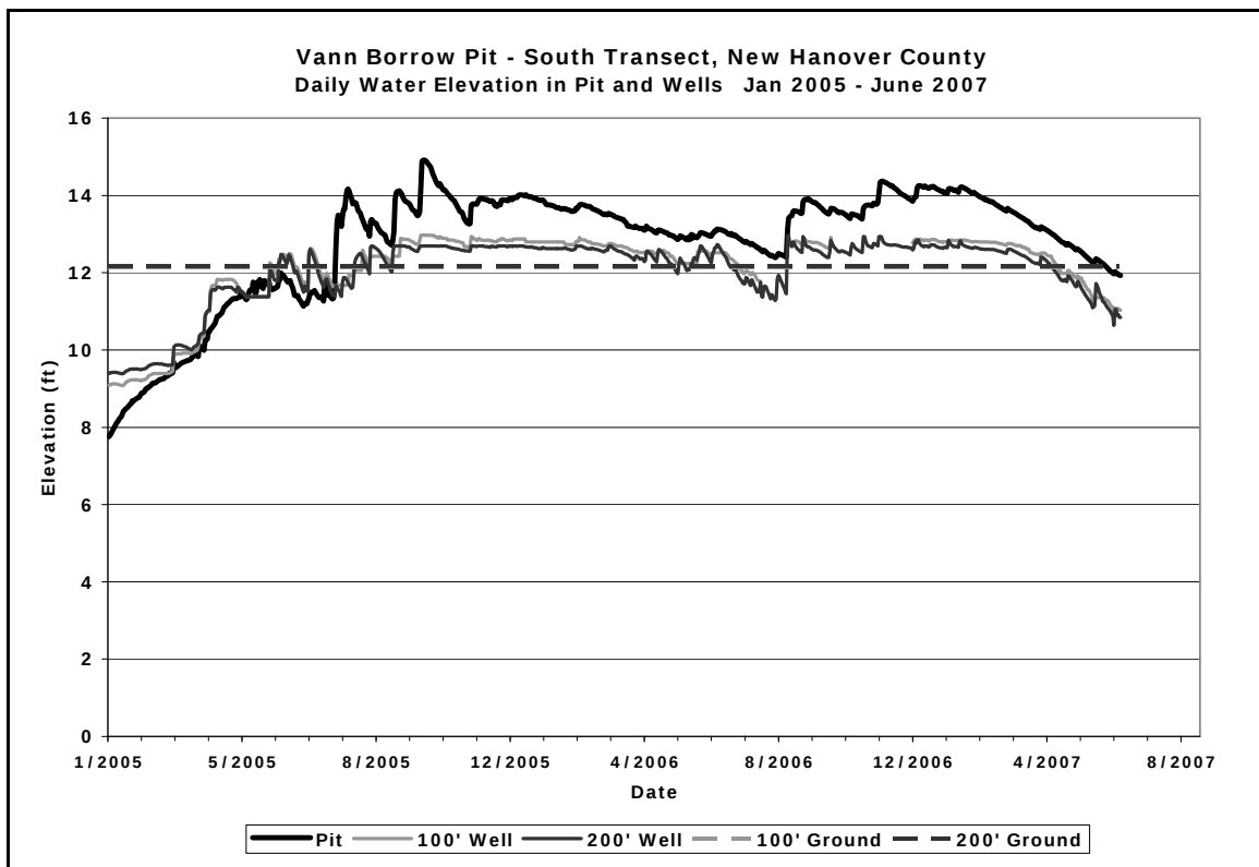
Figure 29. Water table and pond elevations (referenced to 6.5 ft below the base of the pond staff) for Jan 2005 to June 2007 at the Vann borrow pit south transect. The water table data were measured along a line south of the pit where land is downslope from the pit. This pit closed in October, 2004. The increase in stage at the end of July was caused by water (approx 1,728,000 gallons) being pumped into the pit.
