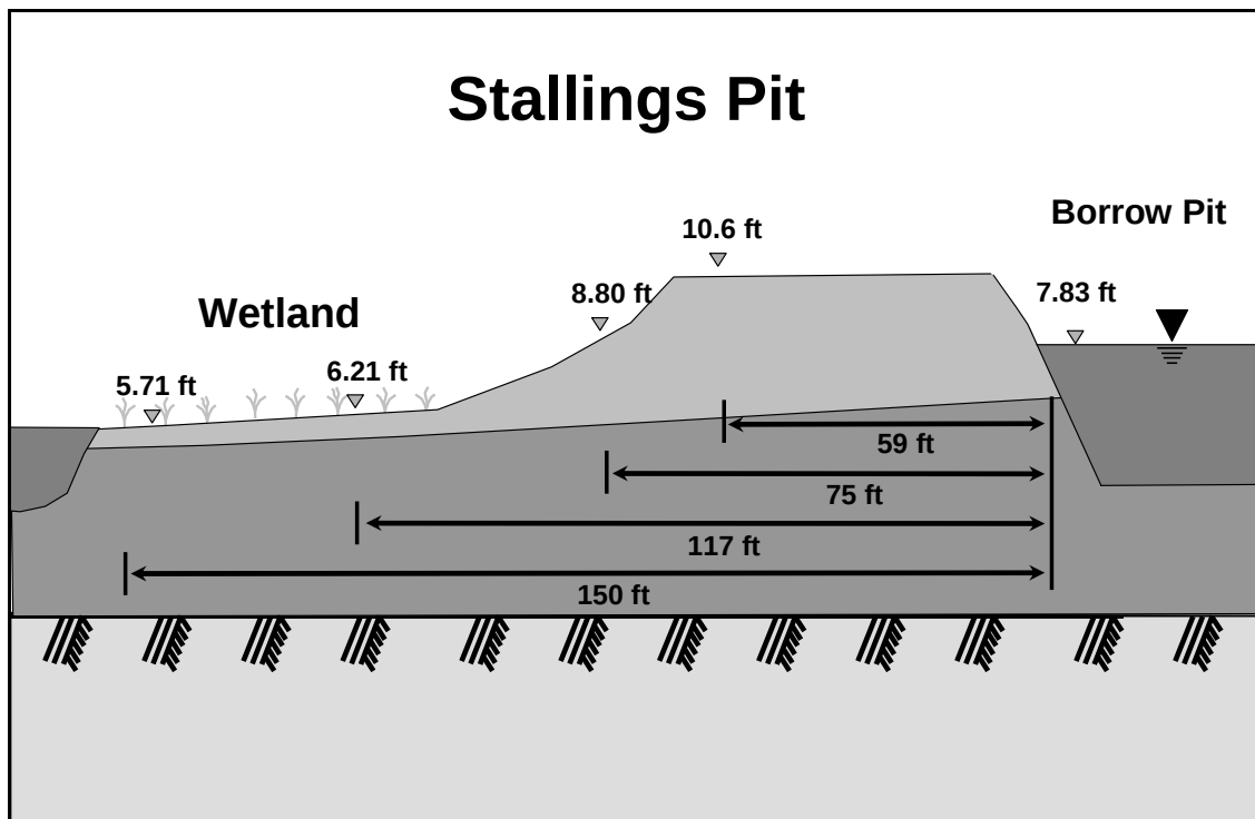
Figure 9. Type 2 Stallings Pit. Wetland down slope of pit. Ground surface of wetland at lower elevation than pit water level. Wetland on the floodplain of the stream.
