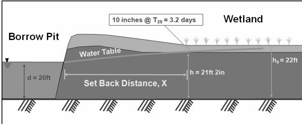
Figure 5. Schematic of borrow pit showing the required set back distance of the pit.
