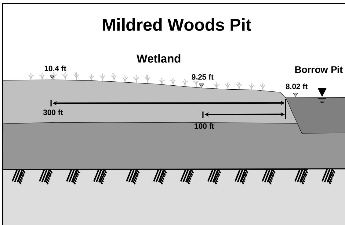
Figure 1. Type 1a – Wetland upslope of pit. Mildred Woods Pit. Ground surface of wetland at higher elevation than pit water level. Water level of pit controlled by elevation of outlet.
