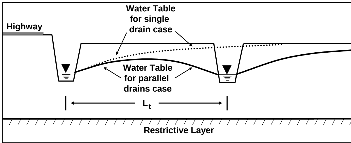
Figure 2. Schematic of parallel ditches showing the effect of a second ditch on the water table depth.
