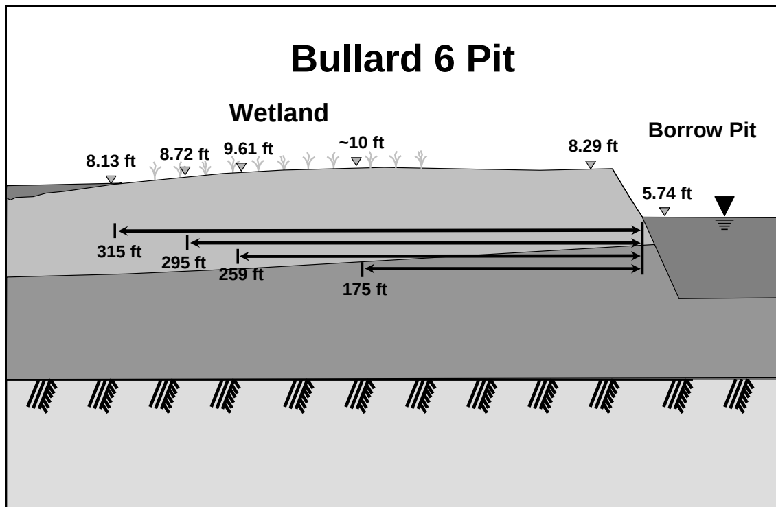
Figure 16. Type 1 - Water level limit unknown. Bullard 6 Pit. Ground surface of wetland at higher elevation than pit water level. Limit of pit water level not determined.
