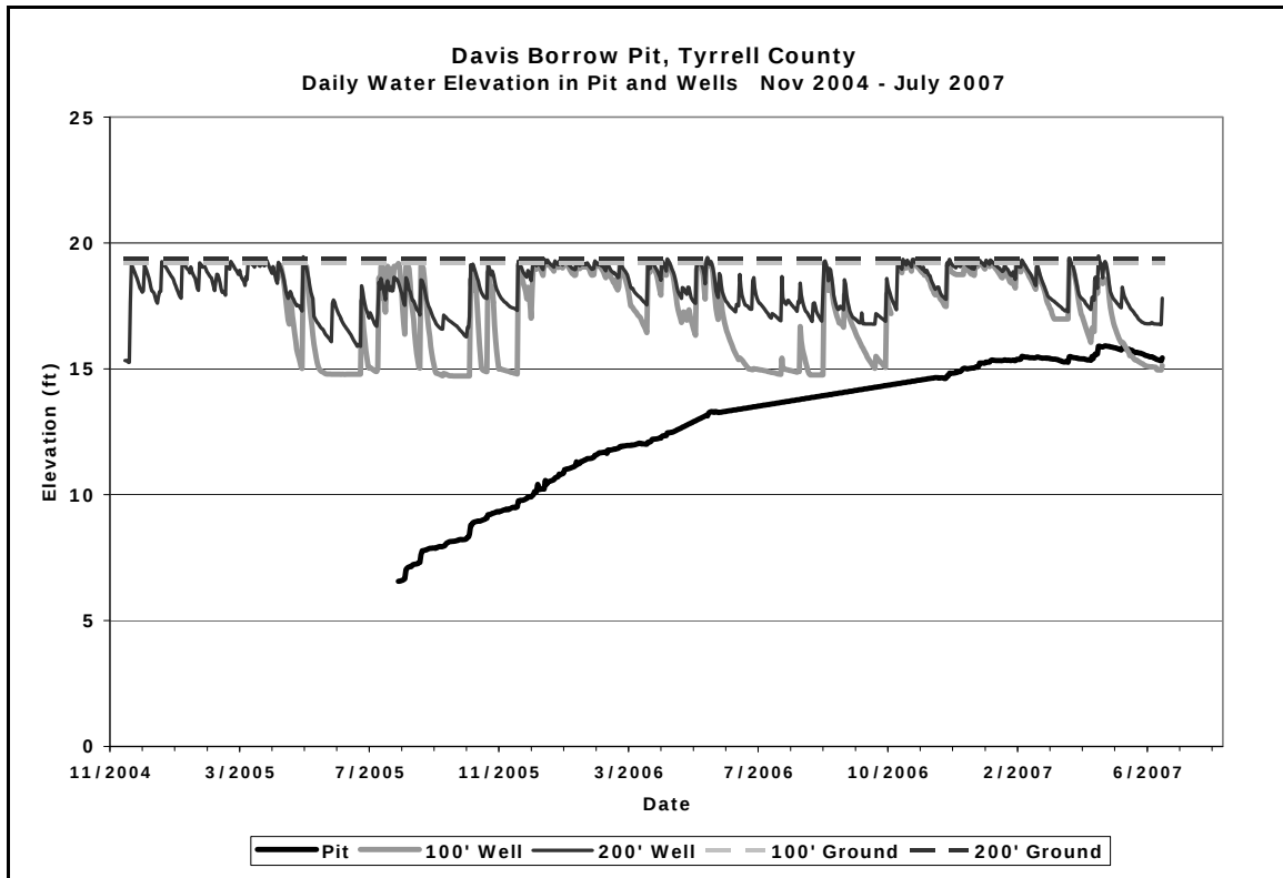
Figure 26. Water table and pond elevations (referenced to 6.5 ft below the base of the pond staff) Nov. 2004 to July 2007 at Davis borrow pit. This pit closed in late July, 2005. Well at 100' and Well at 200' refer to wells located 100 ft. and 200 ft. from the edge of pit.
