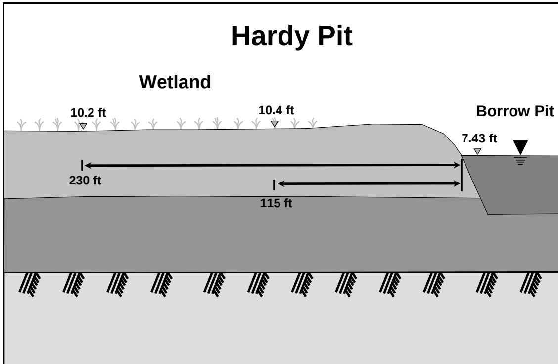
Figure 2. Type 1a – Hardy Pit. Ground surface of wetland at higher elevation than pit water level, which is controlled by weir elevation in outlet control structure.
