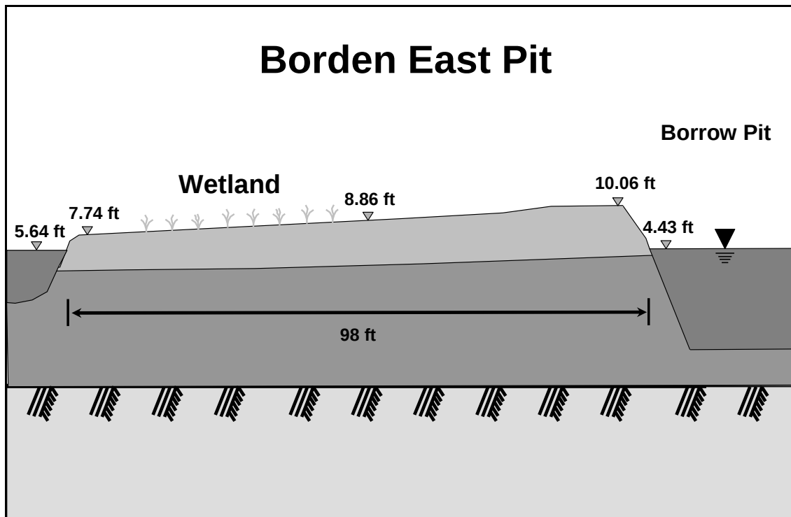
Figure 6. Type 1b - Water level of pit limited by seepage to sink. Borden East Pit. Ground surface of wetland at higher elevation than pit water level. Water level of pit limited by seepage to stream. The stream level was high during this measurement.
