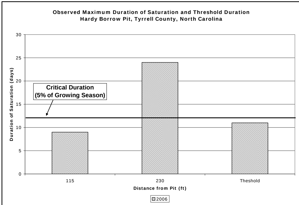
Figure 35. Observed and predicted number of consecutive days when water table was within 1 ft of the surface during the growing season plotted for 2006 for the Hardy site. Threshold conditions represent the number of days in each year for a site that barely satisfies the wetland hydrologic criterion.
