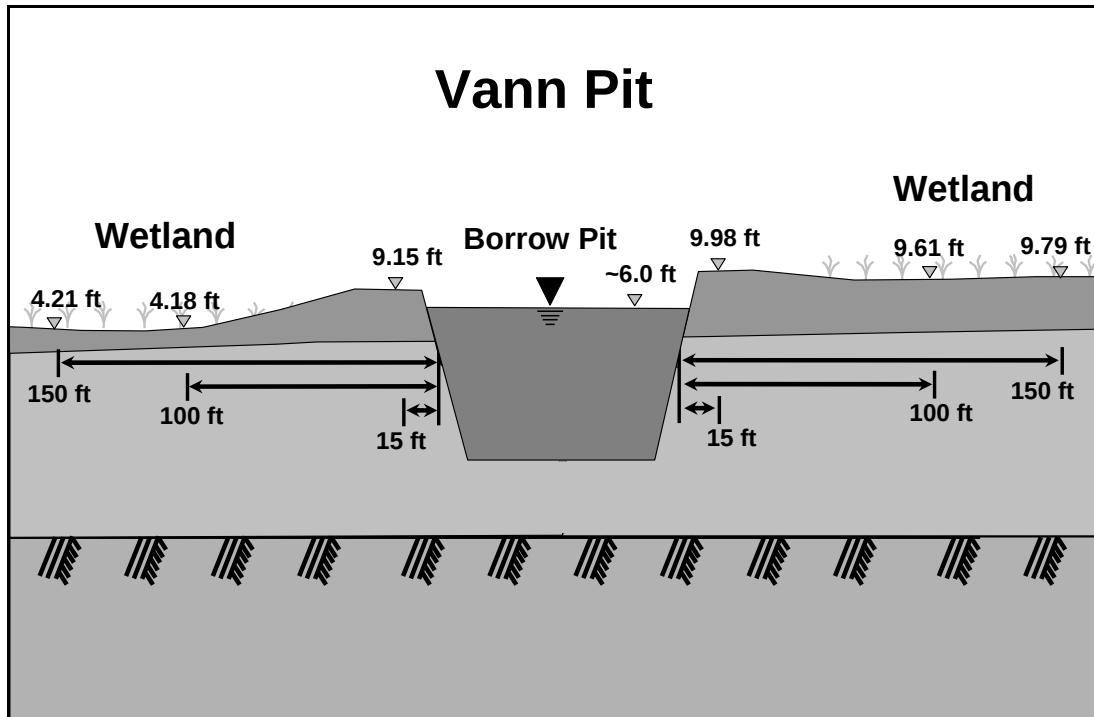
Figure 23. Type 3 – Wetlands both upslope and down slope of pit. Vann Pit. Ground surface elevation of one wetland is lower than pit water level, and ground surface elevation of other wetland is higher than pit water level.
