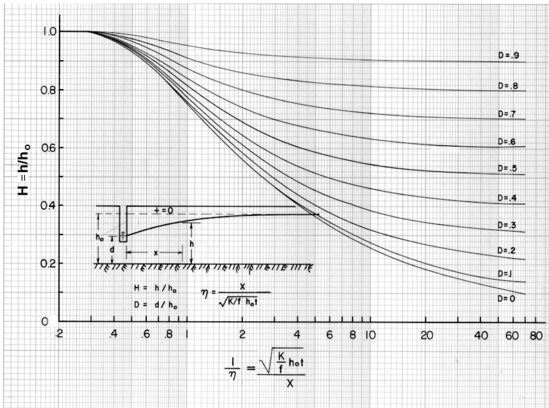
Figure 4. Nondimensional solutions to the Boussinesq equation for water table drawdown due to drainage to a single ditch (after Skaggs, 1976).
