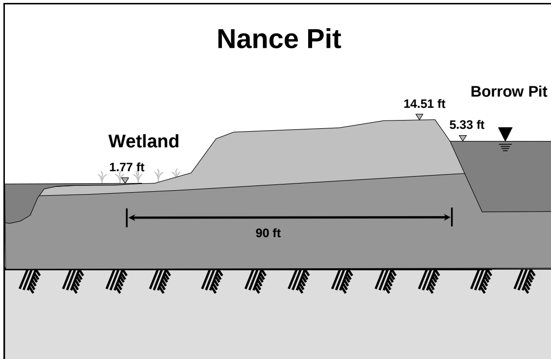
Figure 11. Type 2 - Wetland down slope of pit. Nance Pit. Ground surface of wetland at lower elevation than pit water level. Wetland on the floodplain of the stream.
