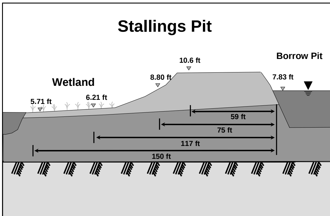
Figure 17. Type 2 Stallings Pit. Wetland down slope of pit. Ground surface of wetland at lower elevation than pit water level. Wetland on the floodplain of the stream.
