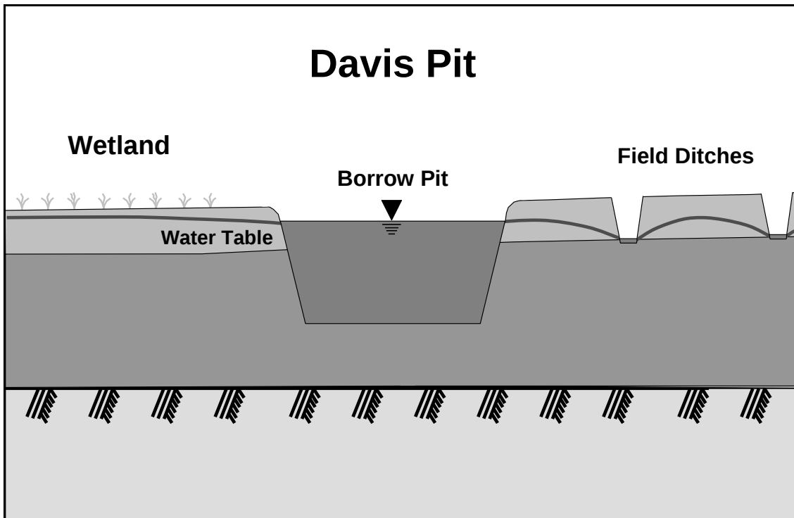
Figure 3. Type 1b. Davis Pit. Wetland upslope of pit. Ground surface of wetland at higher elevation than pit water level. Water level of pit controlled by seepage to field ditches.
