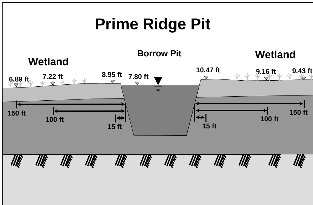
Figure 16. Type 3 – Wetlands both upslope and down slope of pit. Vann Pit. Prime Ridge Pit. Ground surface elevation of one wetland is lower than pit water level, and ground surface elevation of other wetland is higher than pit water level.
