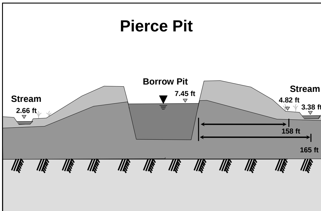
Figure 21. Type 2 - Wetland down slope of pit. Pierce Pit. Ground surface of wetland at lower elevation than pit water level. Wetland on the floodplain of the streams. Pit is located on a ridge between streams.
