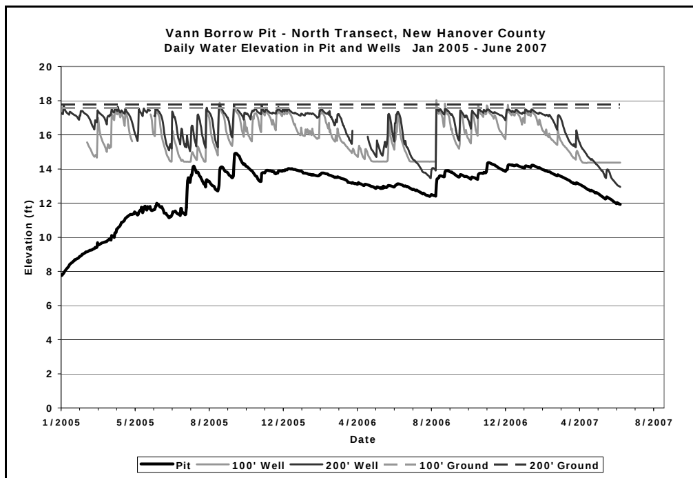
Figure 28. Water table and pond elevations (referenced to 6.5 ft below the base of the pond staff) for Jan 2005 to June 2007 at the Vann borrow pit north transect. The water table data were measured along a line north of the pit where land is upslope from the pit. This pit closed in October, 2004. The increase in stage at the end of July 2005 was caused by water (approx 1,728,000 gallons) being pumped into the pit.
