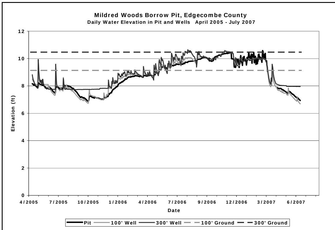
Figure 31. Water table and pond elevations (referenced to 6.5 ft below the base of the pond staff) for April 2005 to July 2007 at the Mildred Woods borrow pit. 100' Well and 300' Well refer to wells located 100 ft. and 300 ft. from the edge of pit.
