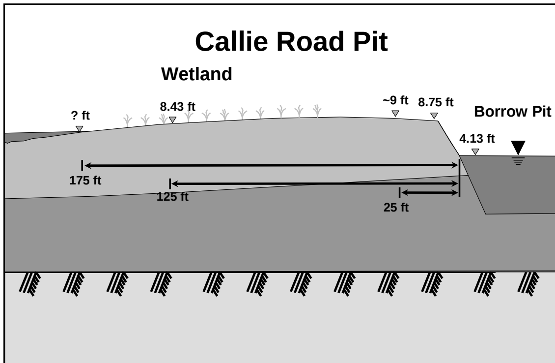
Figure 7. Type 1 - Wetland upslope of pit. Callie Road Pit. Ground surface of wetland at higher elevation than pit water level. Limit of pit water level not determined.
