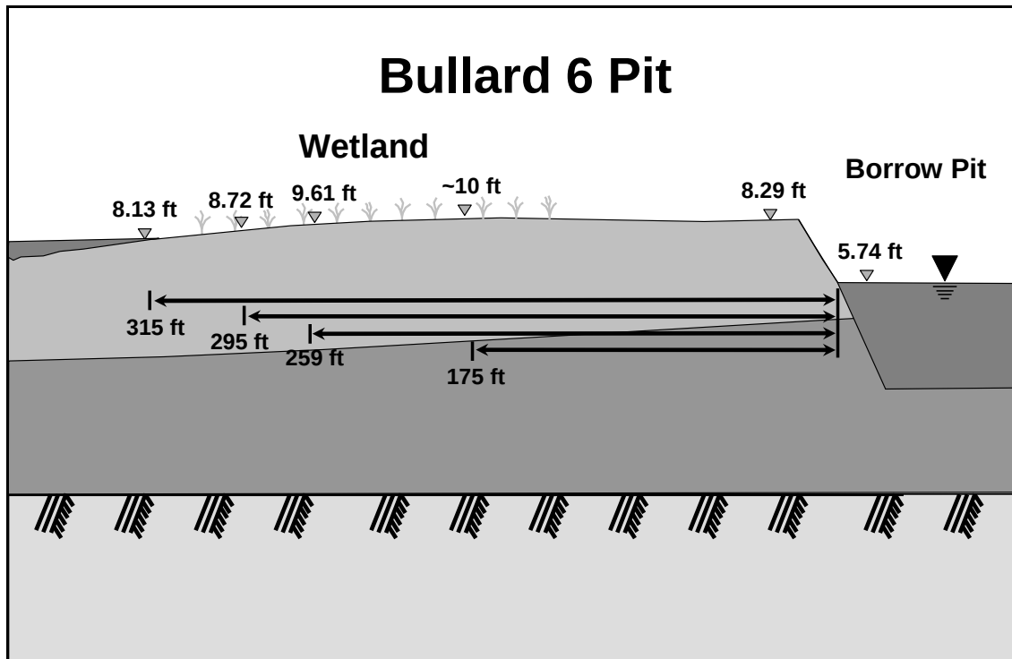
Figure 8. Type 1 - Water level limit unknown. Bullard 6 Pit. Ground surface of wetland at higher elevation than pit water level. Limit of pit water level not determined.
