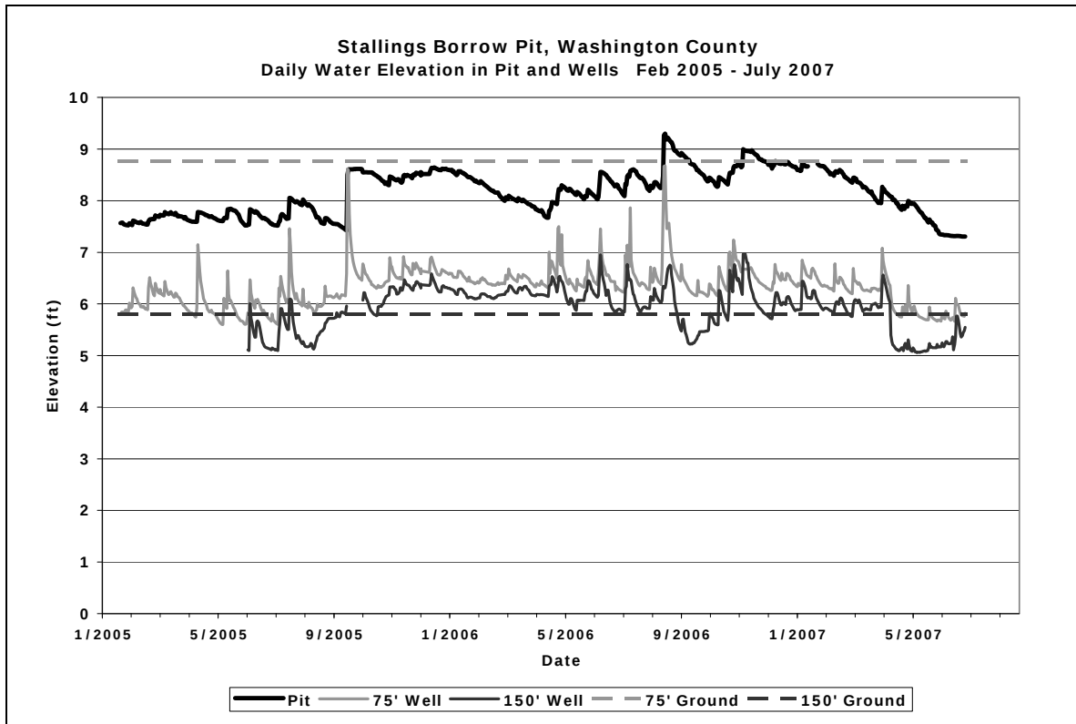
Figure 33. Water table and pond elevations (referenced to 6.5 ft below the base of the pond staff) for February 2005 to July 2007 at the Stallings borrow pit. This pit has been closed since 2003. Well at 75' and Well at 150' refer to wells located 75 ft. and 150 ft. from the edge of pit.
