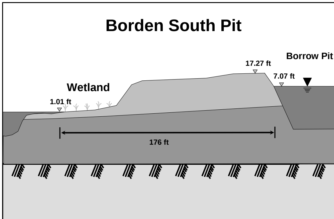
Figure 20. Type 2 - Wetland down slope of pit. Borden South Pit. Ground surface of wetland at lower elevation than pit water level. Wetland on the floodplain of the stream.
