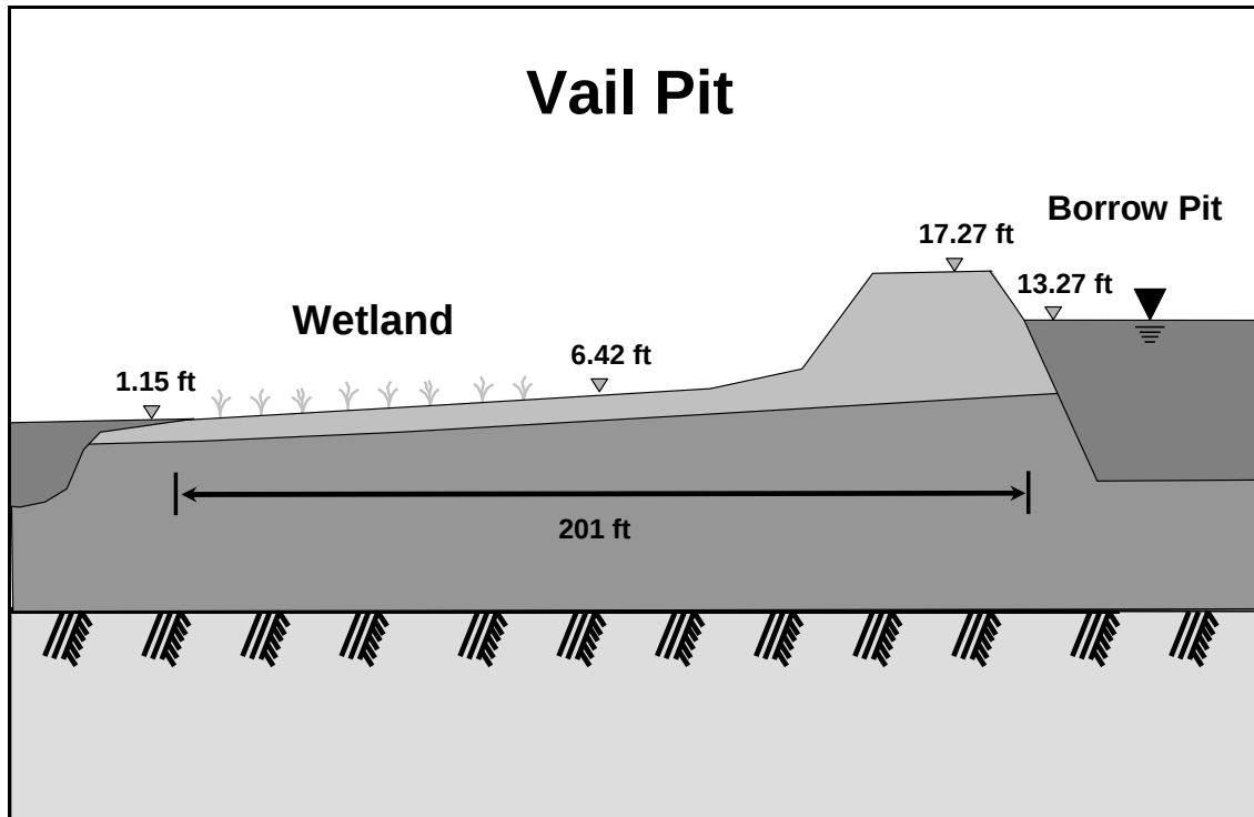
Figure 18. Type 2 - Wetland down slope of pit. Vail Pit. Ground surface of wetland at lower elevation than pit water level. Wetland on the floodplain of the stream.
