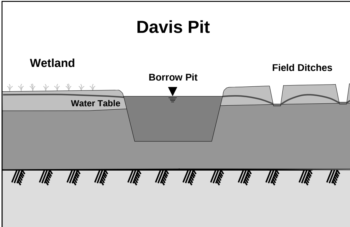
Figure 11. Type 1b. Davis Pit. Wetland upslope of pit. Ground surface of wetland at higher elevation than pit water level. Water level of pit controlled by seepage to field ditches.
