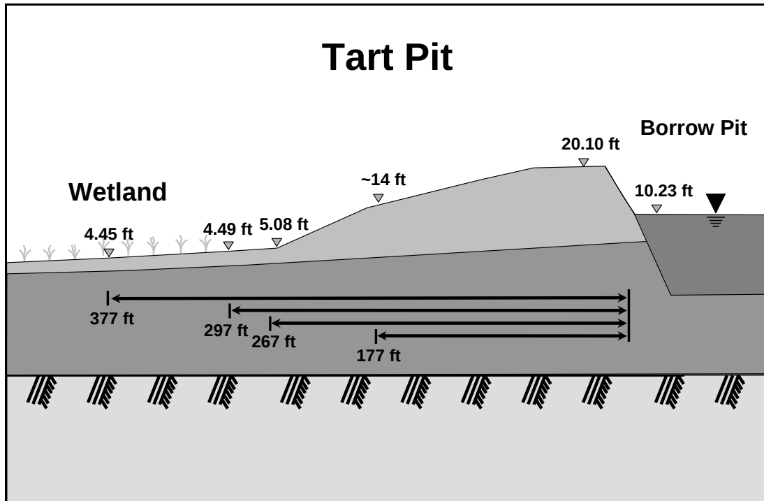
Figure 14. Type 2 - Wetland down slope of pit. Tart Pit. Ground surface of wetland at lower elevation than pit water level. Wetland on a slope away from the pit.
