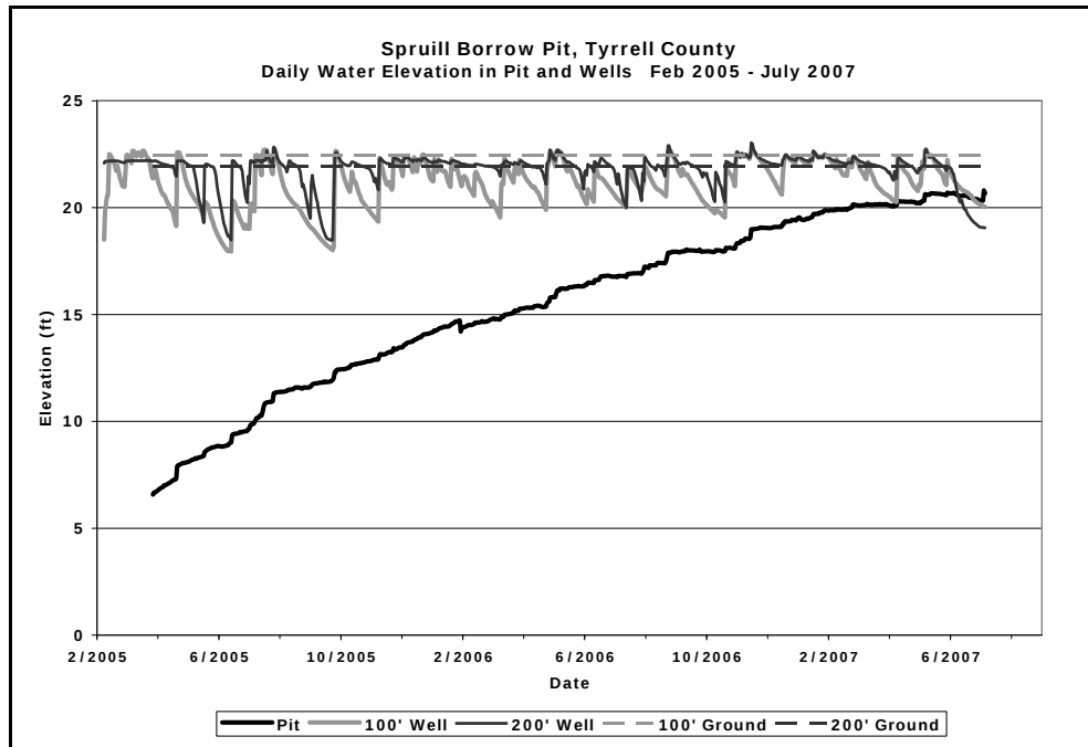
Figure 27. Water table and pond elevations (referenced to 6.5 ft below the base of the pond staff) for Feb 2005 to July 2007 at the Spruill borrow pit. This pit closed in April, 2005. Well at 100' and Well at 200' refer to wells located 100 ft. and 200 ft. from the edge of pit
