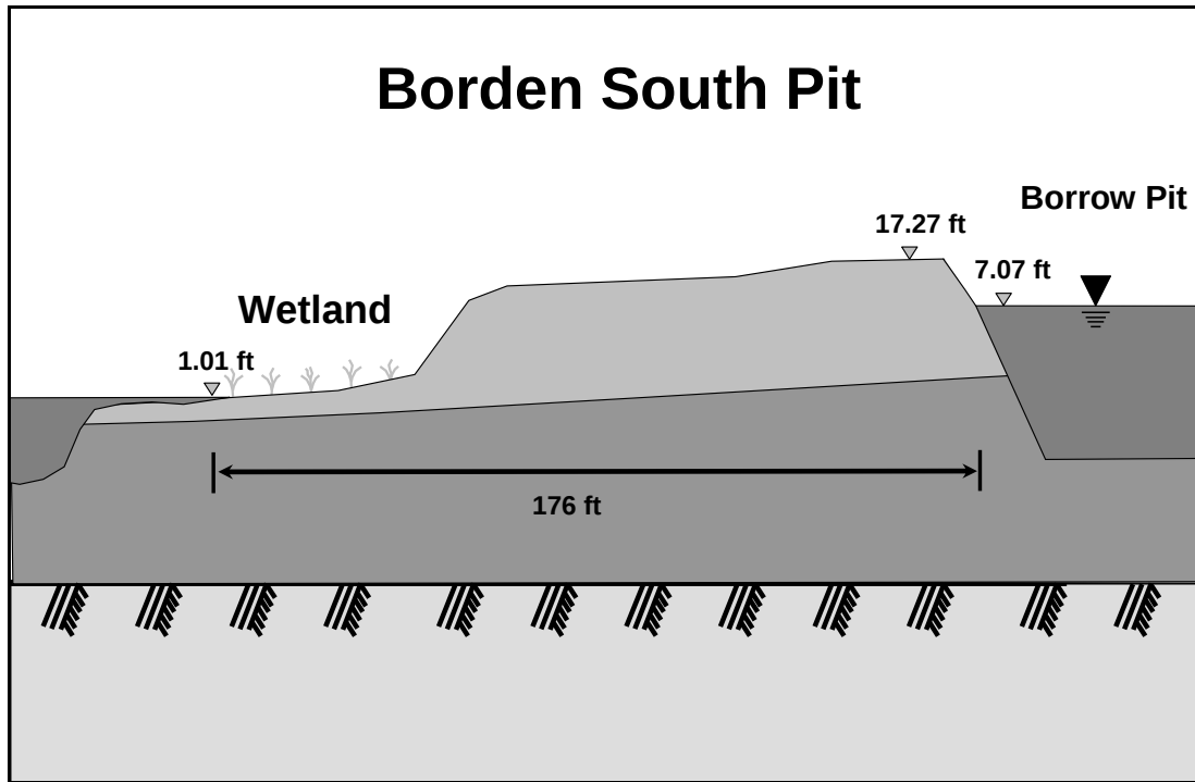
Figure 12. Type 2 - Wetland down slope of pit. Borden South Pit. Ground surface of wetland at lower elevation than pit water level. Wetland on the floodplain of the stream.
