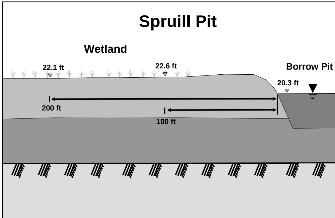
Figure 4. Type 1b. Spruill Pit. Water level of pit limited by seepage to sink. Ground surface of wetland at higher elevation than pit water level. Water level of pit limited by seepage to field ditches (not shown).
