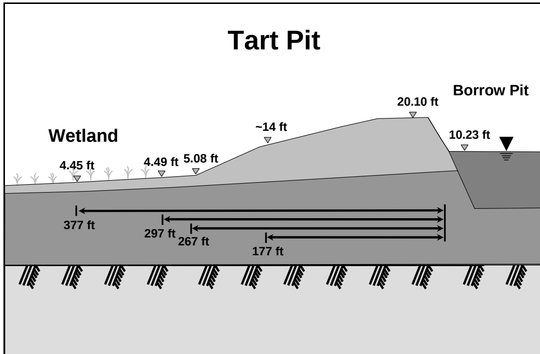
Figure 22. Type 2 - Wetland down slope of pit. Tart Pit. Ground surface of wetland at lower elevation than pit water level. Wetland on a slope away from the pit.
