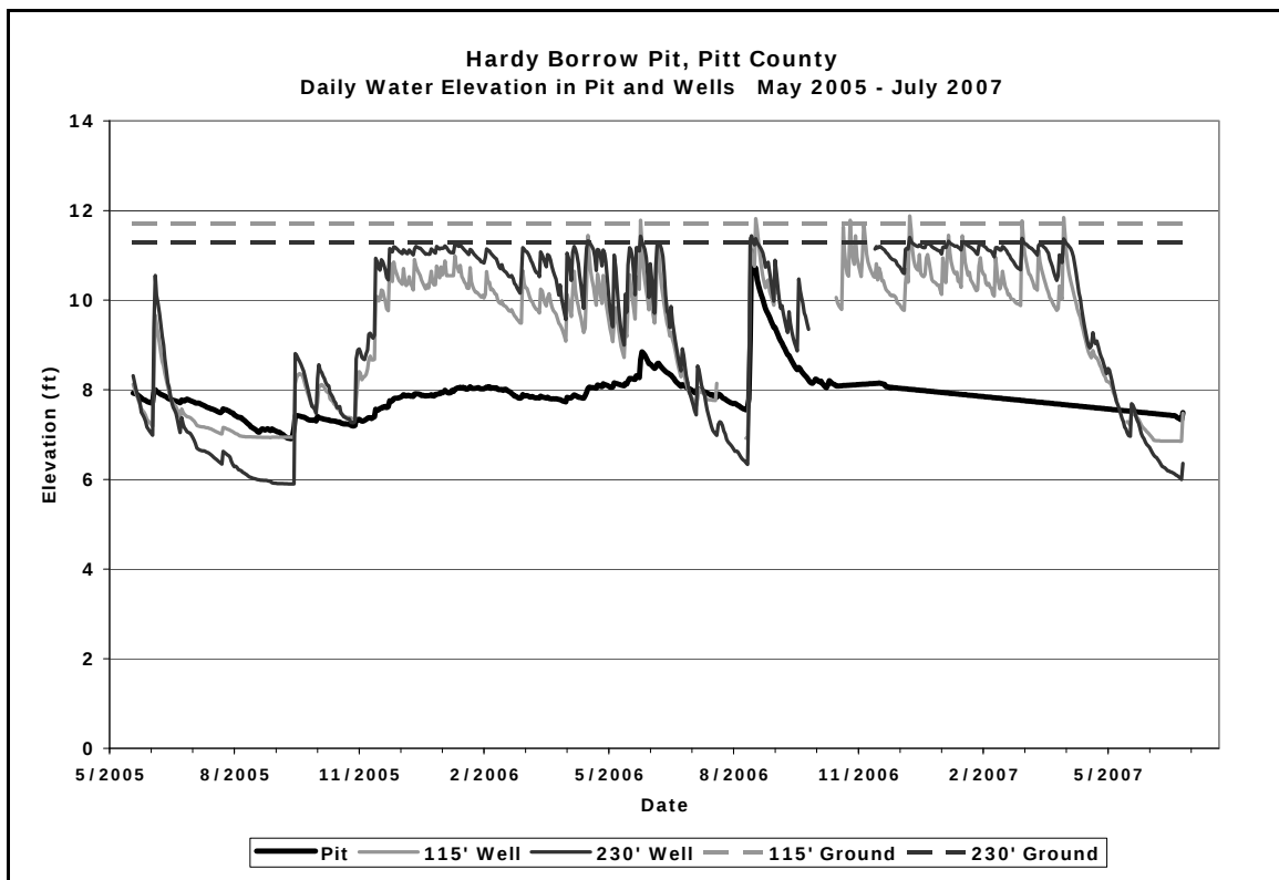
Figure 32. Water table and pond elevations (referenced to 6.5 ft below the base of the pond staff) for May 2005 to July 2007 at the Hardy borrow pit. Well at 115' and Well at 230' refer to wells located 115 ft. and 230 ft. from the edge of pit.
