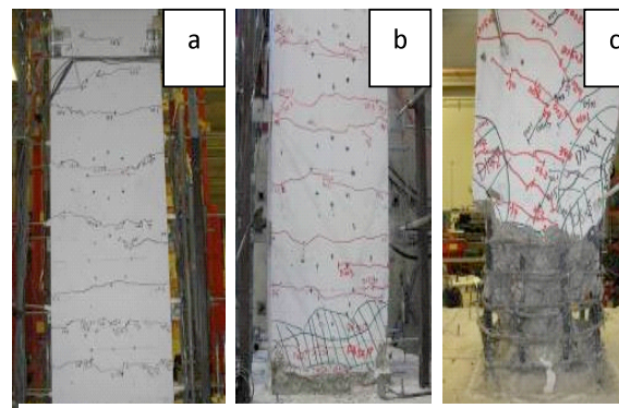
Figure 4 - Failure Modes under Flexure at (a) Longitudinal Bar Yield, (b) Ultimate, and (c) Final failure
