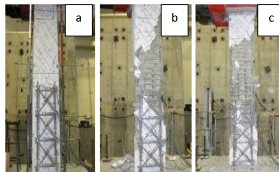
Figure 6 - Failure Modes under Pure Torsion at (a) Transverse Yield, (b) Ultimate, and (c) Final failure
