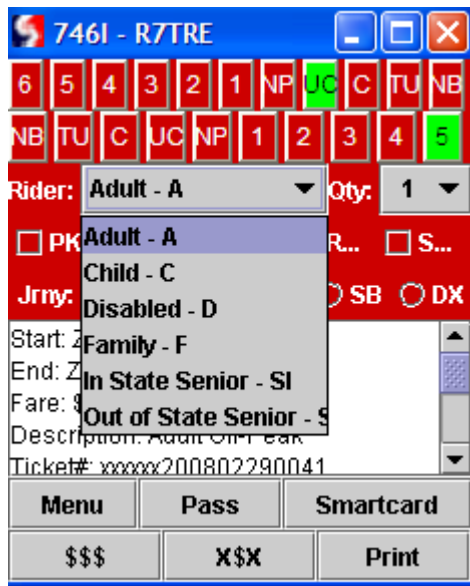
Figure 7: Ticket Processing GUI.
