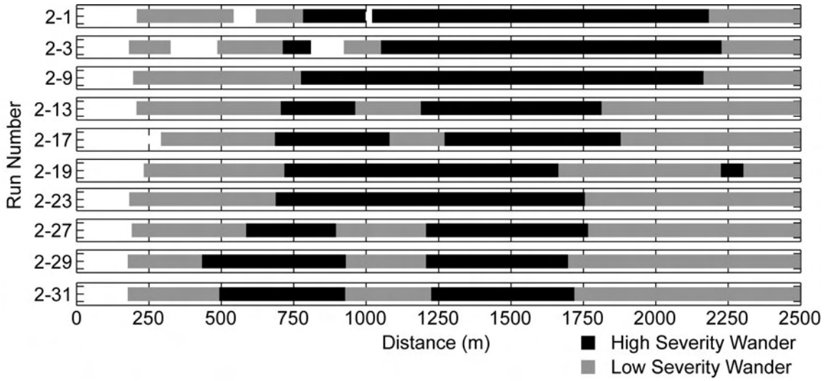
Figure 4-17. Trigger signals for 113km/h (70mph) day two east-bound runs
