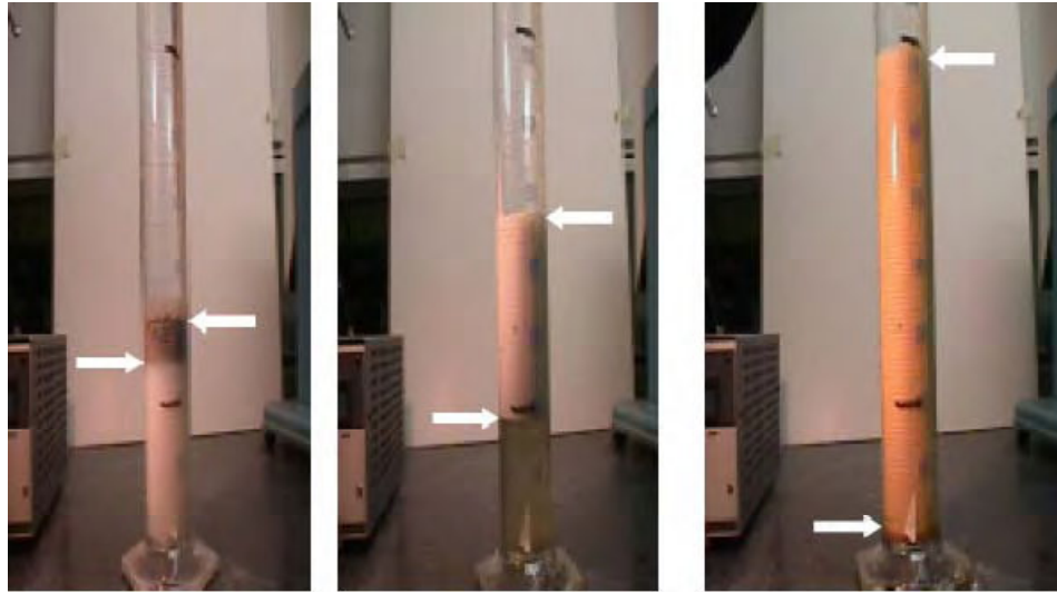
Figure 5. Foam drainage testing of three different AEAs (Cross et al., 2000).
