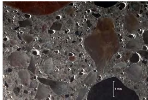
Magnification: 10x Description: Hardened air void system.
