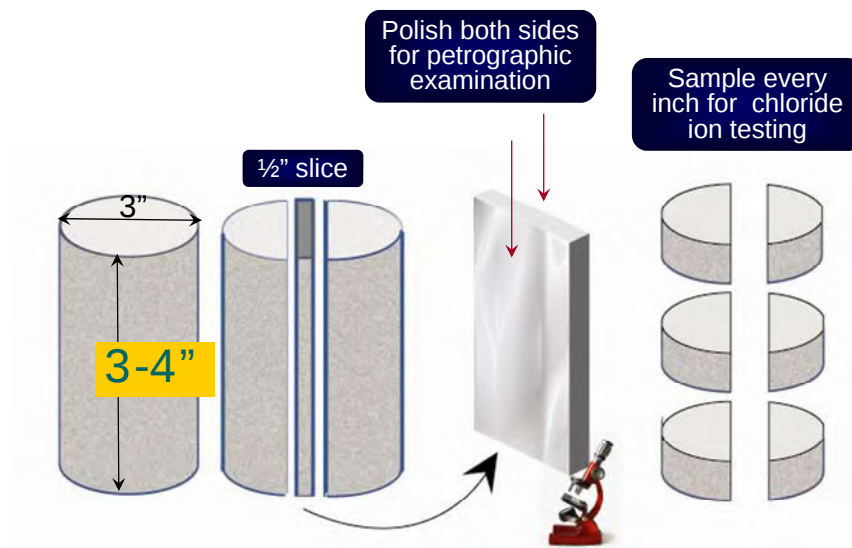
Figure 21. Samples obtained from each core for petrographic and chloride testing
