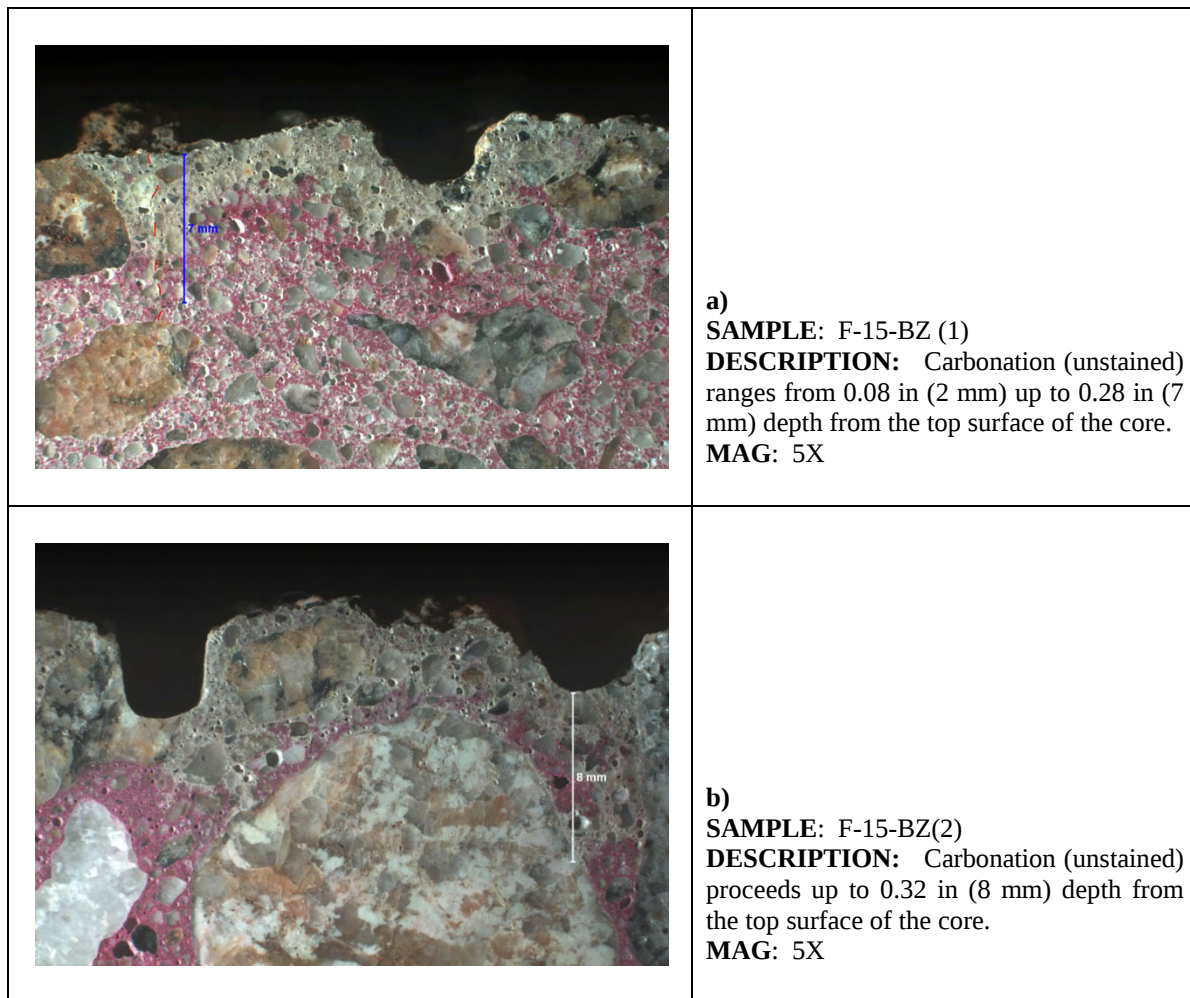
Figure 33. Magnified images of structure F-15-BZ under petrographic examination
