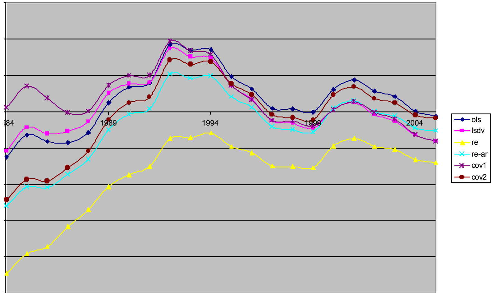
Figure G2: Percent Deviation of the Six Models from Actual Container Counts (1984-2005)
