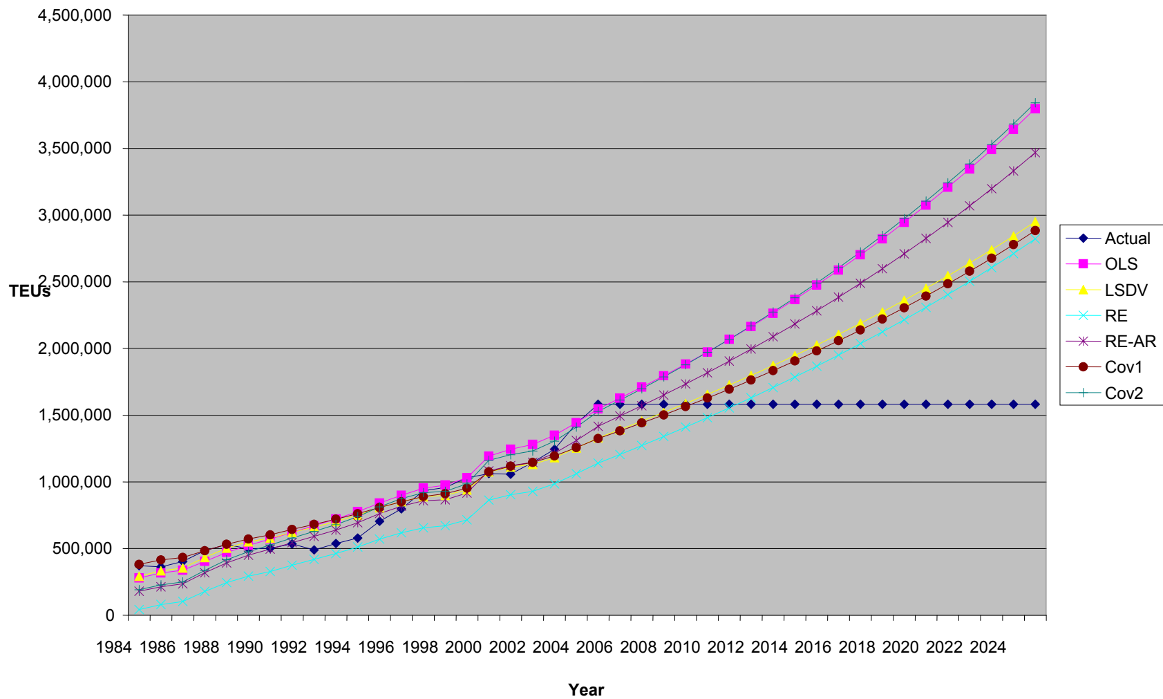
Figure G3: Predicted Container Counts by the Six Models (1984-2025)
