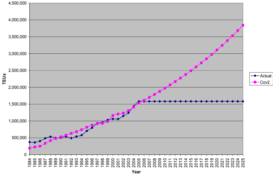
Figure 6.1: Houston Container Count Predictions Using the Cov2 Model (1984-2025)
