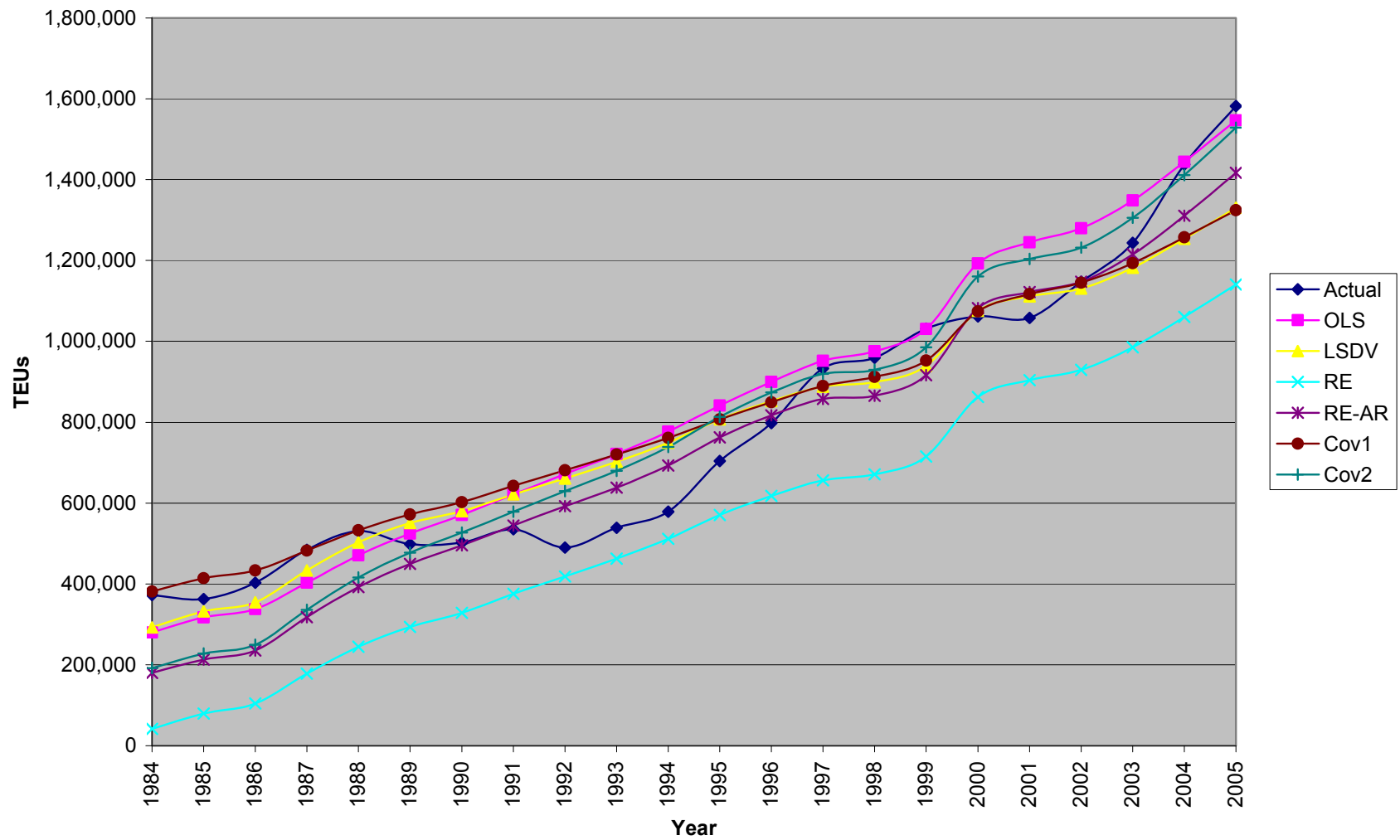
Figure G1: Houston Container Count Predictions of the Six Models (1984-2005)
