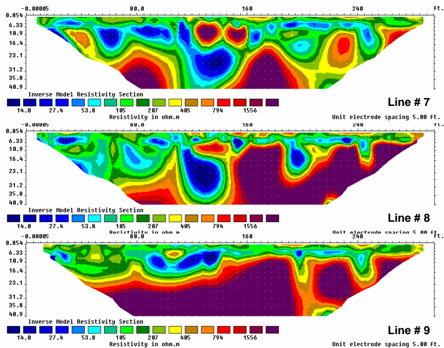
Figure 7: Grid "1A" electrical resistivity profiles 7, 8 and 9 (Figure 4).
