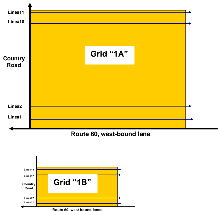
Figure 4: Two grids of electrical resistivity profiles were acquired at the Greene County site. Grid “1A” data, consisting of 11 profiles spaced at 25 ft intervals, were acquired using 68 electrodes spaced at 5 ft intervals. Grid “1B” data, consisting of 8 profiles spaced at 10 ft intervals were acquired using 40 electrodes spaced at 3 ft intervals.
