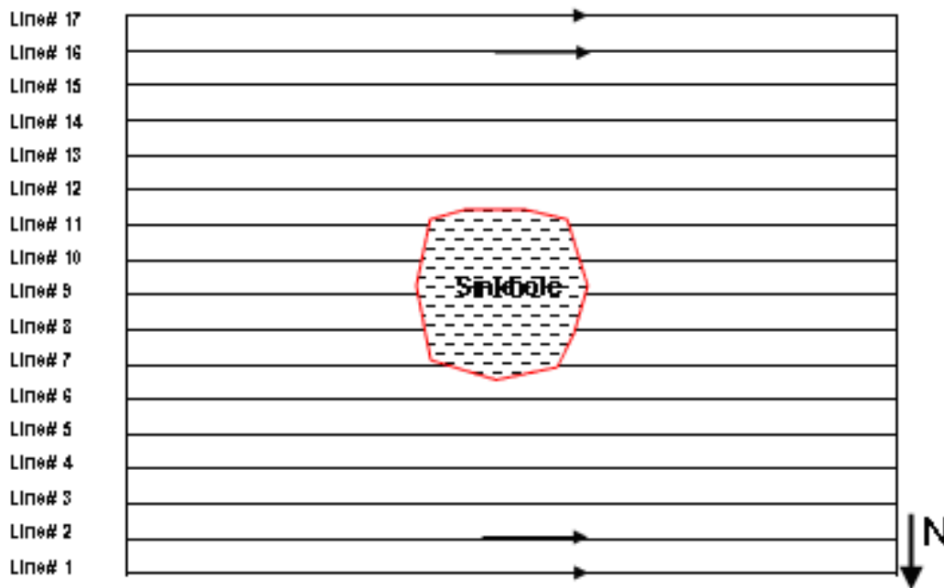
Figure 16: A single grid of electrical resistivity profiles was acquired at the Jefferson County site. The grid consisting of 17 profiles spaced at 25 ft intervals, were acquired using an electrode spacing of 12 ft.
