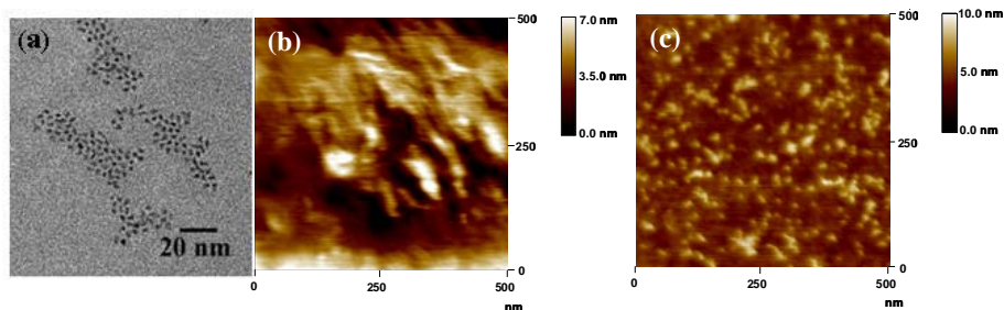
Fig. 27. The bright field TEM image of the 11-HUDA functionalized CdSe QDs after washing; The AFM images of the isocyanate-bearing glass substrate (b), a monolayer of CdSe QDs on a glass (c).
