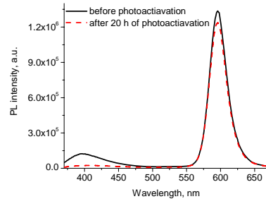
Fig. 22 PL changes before and after of 20 hours of photoactivation at 350 nm irradiation of QDs in C 12
