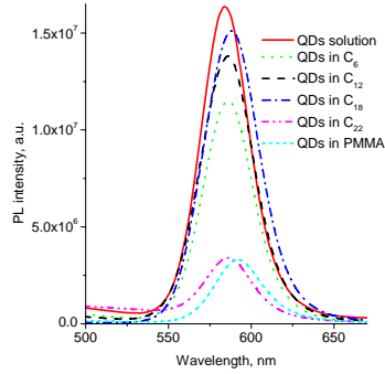
Fig. 20: Photoluminescence spectra of QDs in polymers
