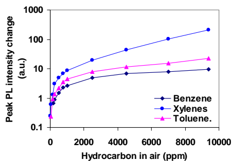
Fig.50 Benzene, toluene, and xylenes sensing characteristics of a Si/AAO/QD
