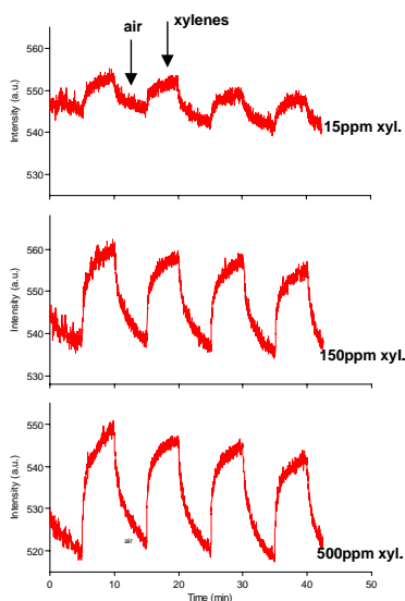
Fig. 13 Peak PL intensity change of QD-NA/PMMA film with chemical exposure time, with the exposure cycled between air and xylenes at different concentration levels
