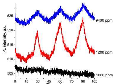
Fig. 23 PL intensity changes of QDs-NA 10wt% in C 12 while exposure to xylenes
