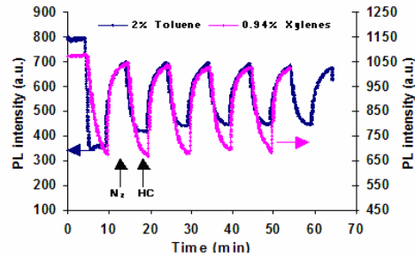
Fig. 6 PL intensity response of a QD-SA film toward exposure to 2 % toluene and 0.94 % xylens in nitrogen.
