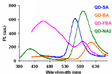
Fig.10 Fluorescence spectra of PMMA films with imbedded CdSe QDs with different surface groups: unmodified QD-SA, BA, FBA and NA surface modified CdSe QDs
