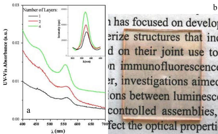
Fig. 28 (a) Optical absorbance spectra of the multilayered films fabricated using the 16-HHDA functionalized QDs with the inset showing the PL spectra of these films. (b) Photo of the 10 layered film fabricated on a glass slide.
