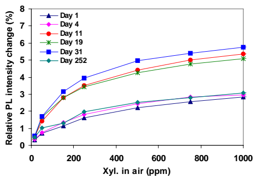
Fig. 53 Xylenes sensing performances of an AAO/QD (core/shell) sample over a time period of 252 days
