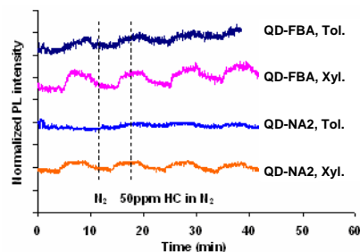
Fig. 12 Comparison of the selectivity of the QD films towards a 50ppm xylenes or 50ppm toluene in nitrogen
