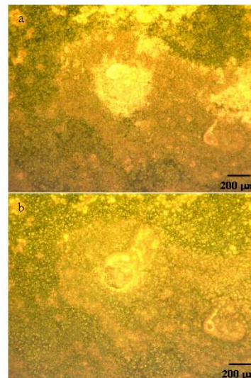
Fig.38 Reversible change of Fluorescence Optical Microscope images of a CdSe-NA QD/PMMA film exposed to (a) dry air and (b) 9400 ppm xylenes mixed with air. The CCD exposure time is 4 times shorter for image (a) than that for image (b).
