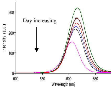
Fig. 52 (a) PL stability of an AAO/QD (core/shell) sample
