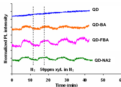
Fig. 11 Comparison of the sensitivity of the QD films towards a 50ppm xylenes in nitrogen exposure
