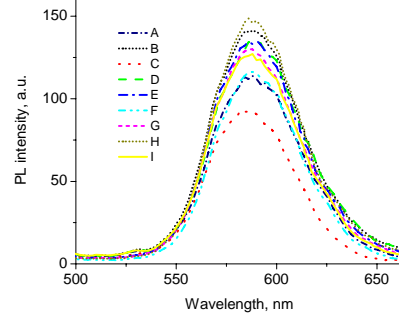
Fig. 21: PL spectra of 9 different points of the same CdSe/C 12 film
