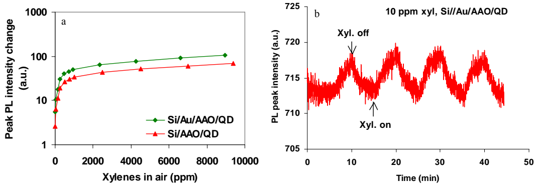
Fig. 51 (a) Comparison of xylenes sensing characteristics of QD samples with/without Au presence, (b) 10 ppm xylenes sensing trace of the Si//Au/AAO/Qd sample
