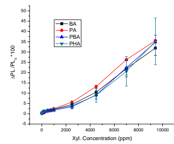
Fig.44 Normalized change in PL upon QD films exposure to Xylenes vs. HC concentration.
