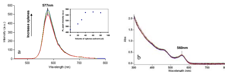
Fig. 35 (a) Photoluminescence and (b) absorbance of solution samples of CdSe-NA QDs in \text{CHCl}_3 mixed with different volumes of liquid xylenes, where the inset in (a) shows peak PL intensity as a function of xylenes volume.
