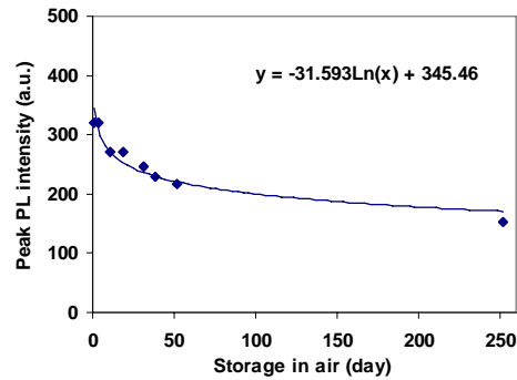
Fig. 52 (b) PL stability of an AAO/QD (core/shell) sample over a time period of 252 days
