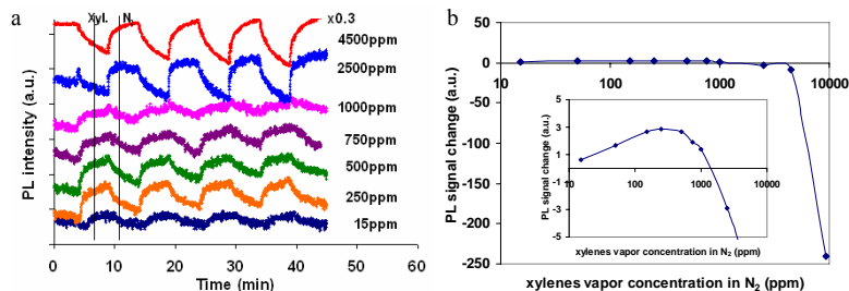
Fig.33 (a) PL peak intensity responses to exposures of xylenes at different concentrations and (b) the sensing characteristics as a function of xylenes concentration, from a CdSe quantum dot/PMMA thin film prepared with method A described in the text, where the inset in (b) shows the detail at low hydrocarbon level exposures.
