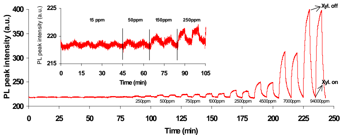
Fig. 49 Xylenes sensing trace of an AAO/QD (core) sample placed on Si
