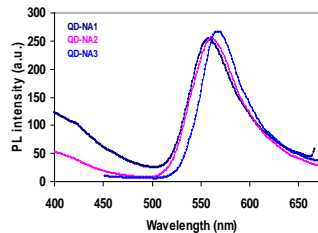
Fig. 14 PL comparison of QD-NA films made from QD-NA solutions with three different NA surface coverages
