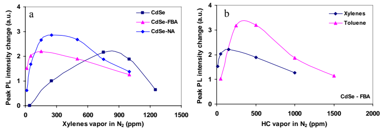
Fig.36 Sensing signal of peak PL intensity change of QD/PMMA films as a function of HC vapor concentration in N 2 for (a) different surface modifying groups bound to CdSe QDs, (b) different types of targeted hydrocarbon species exposed to the same CdSe-FBA QDs
