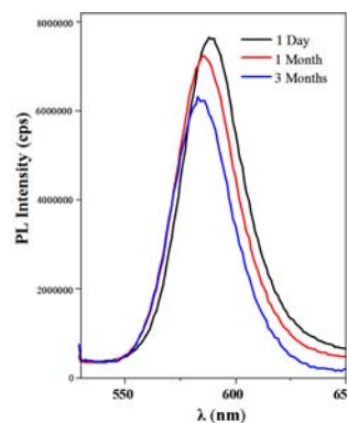
Fig. 31. PL intensity of the 10 layered CdSe-film on glass at different time
