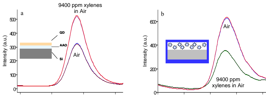
Fig. 28 (a) PL enhancement from Si/AAO/QD in contrast to (b) PL quenching from Si/QD embedded PMMA exposed to 9400 ppm xylenes
