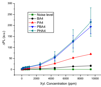
Fig.43 Absolute change in PL upon QD films exposure to Xylenes vs. HC concentration.
