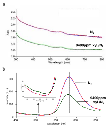
Fig.37 Two-cycle reversible change in (a) absorbance of CdSe-NA substrate and (b) photoluminescence of CdSe-NA QD/PMMA film on a silicon substrate, QD/PMMA film on a glass under exposures switched between N 2 and 9400 ppm xylenes mixed with N 2 , where the inset in (b) shows a background signal change
