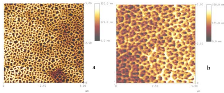
Fig. 45 Atomic Force Microscopy (AFM) images of (a) a blank anodic aluminum oxide (AAO) and (b) QD drop-cast AAO
