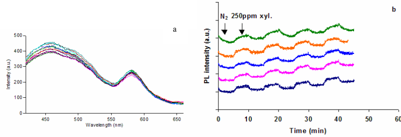
Fig. 4 (a) PL spectra of 15 drop coated QD-FBA films and (b) peak PL intensity responses of five of these films towards 250 ppm xylenes exposure
