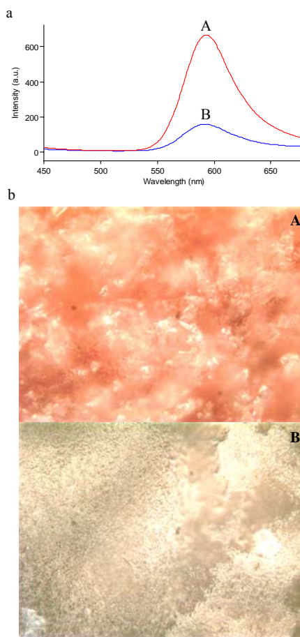
Fig.32 Comparison of (a) photoluminescence and (b) Optical Microscope images of CdSe quantum dot/PMMA thin films having different surface roughness, sample A and B
