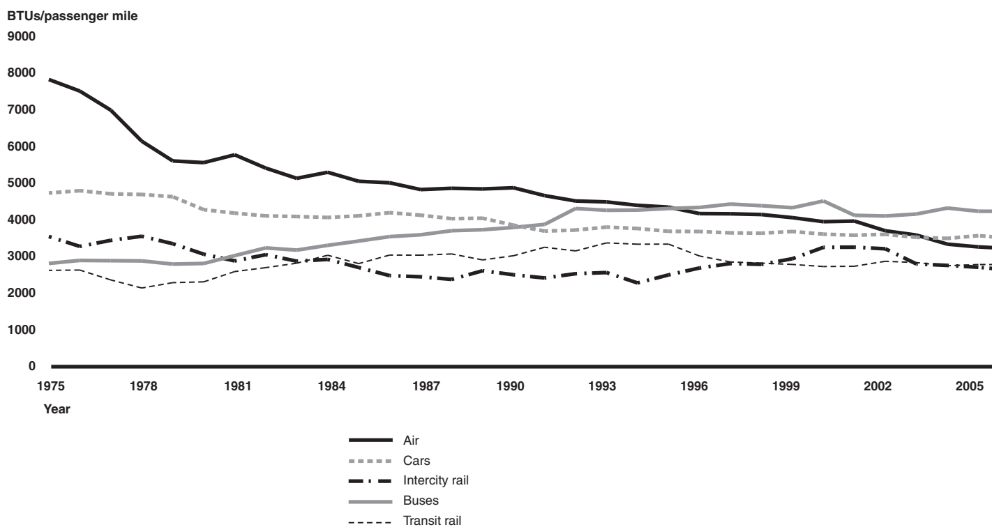
Figure 3: Energy use per Passenger-mile, by Mode of Transportation
