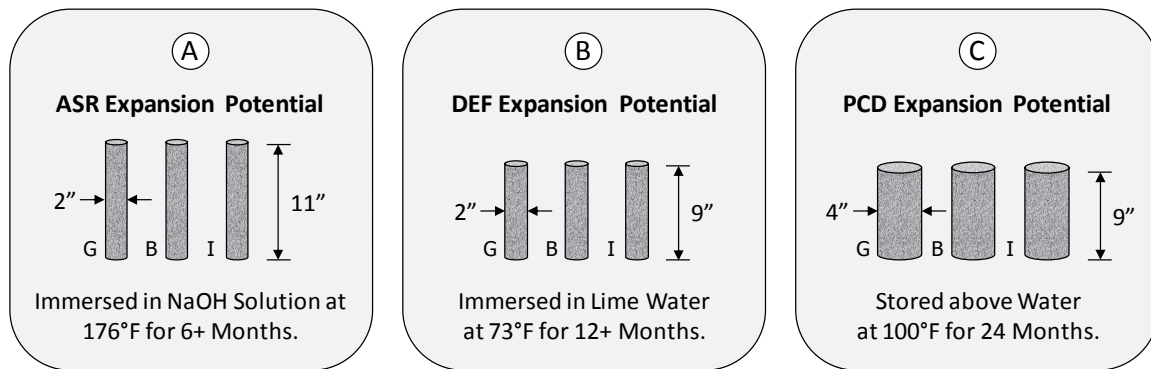
Figure 4-34: Residual Expansion Testing Per Specimen
