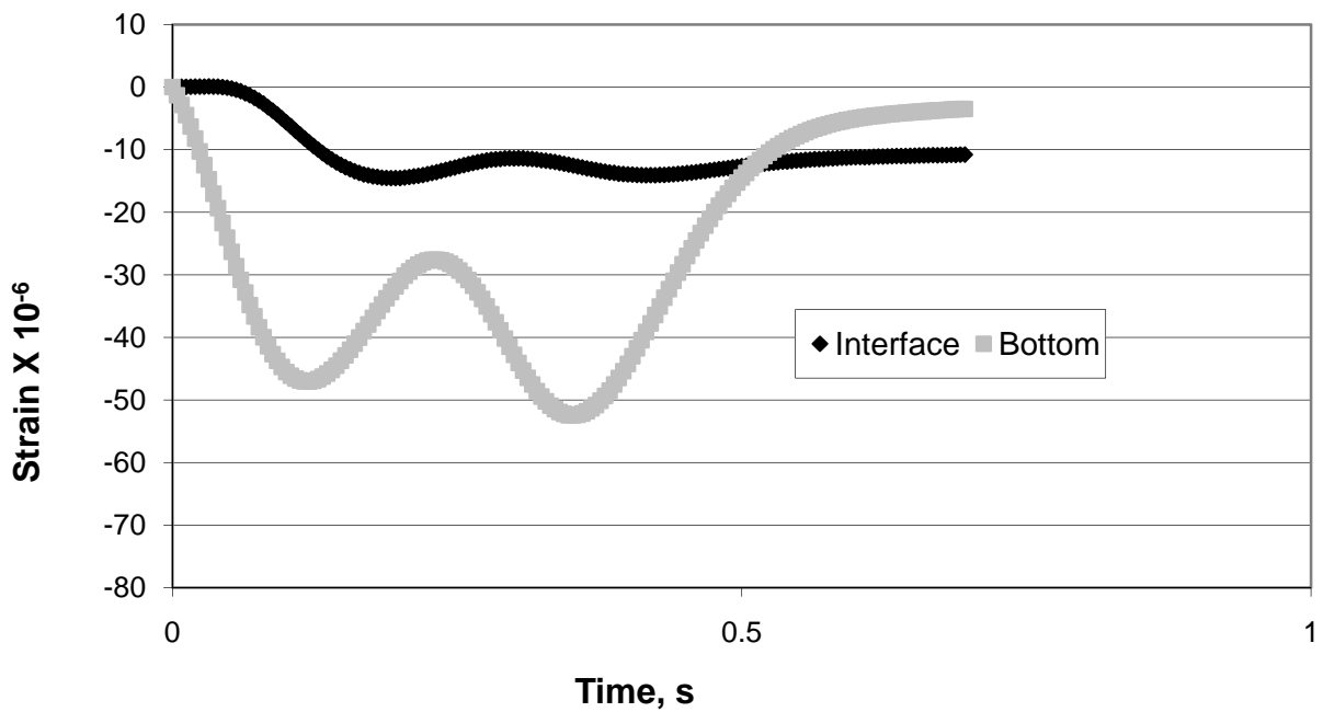
Figure 18: Strain Measurement from Truck Run 8 – July 2005
