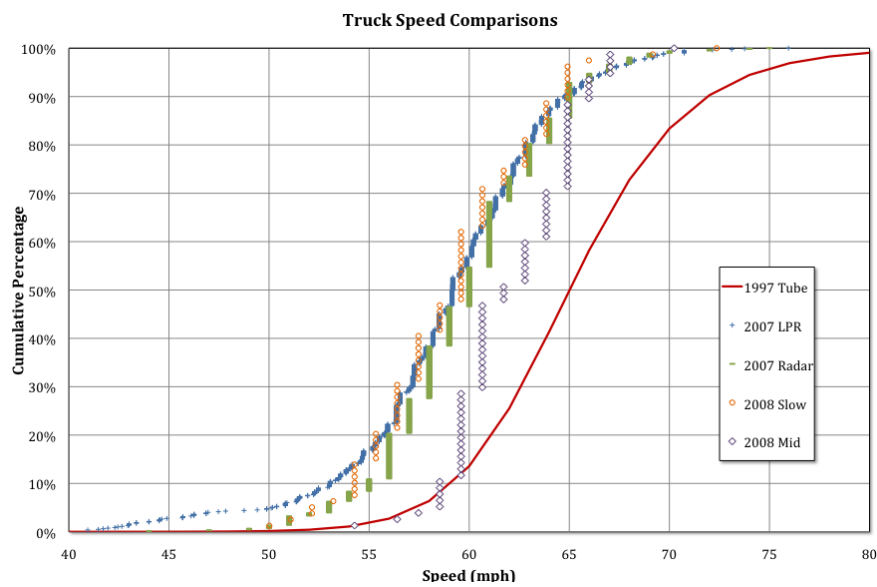
Figure 19. Graph. Truck Speed Comparisons.
