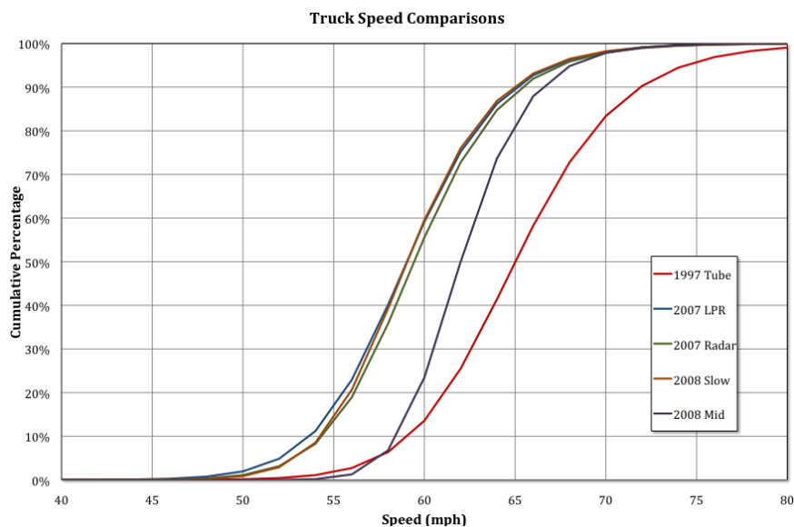
Figure 20. Graph. Truck Speed Comparisons.
