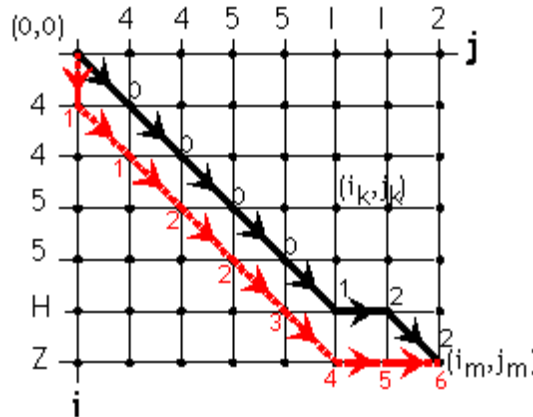
Figure 18. Graph. An Illustration of Alternative Matching Paths with Different Levenshtein Distances.
