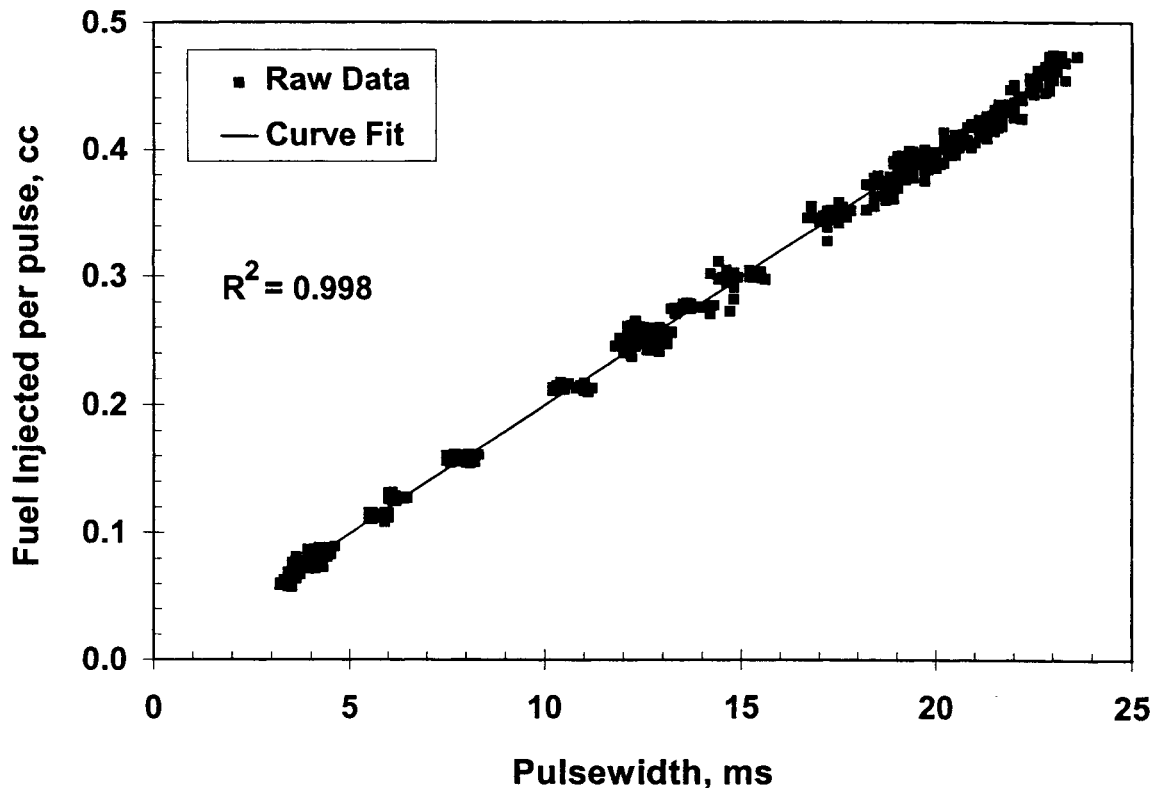
Figure 3. Fuel calibration curve for Oldsmobile Eighty-Eight.
