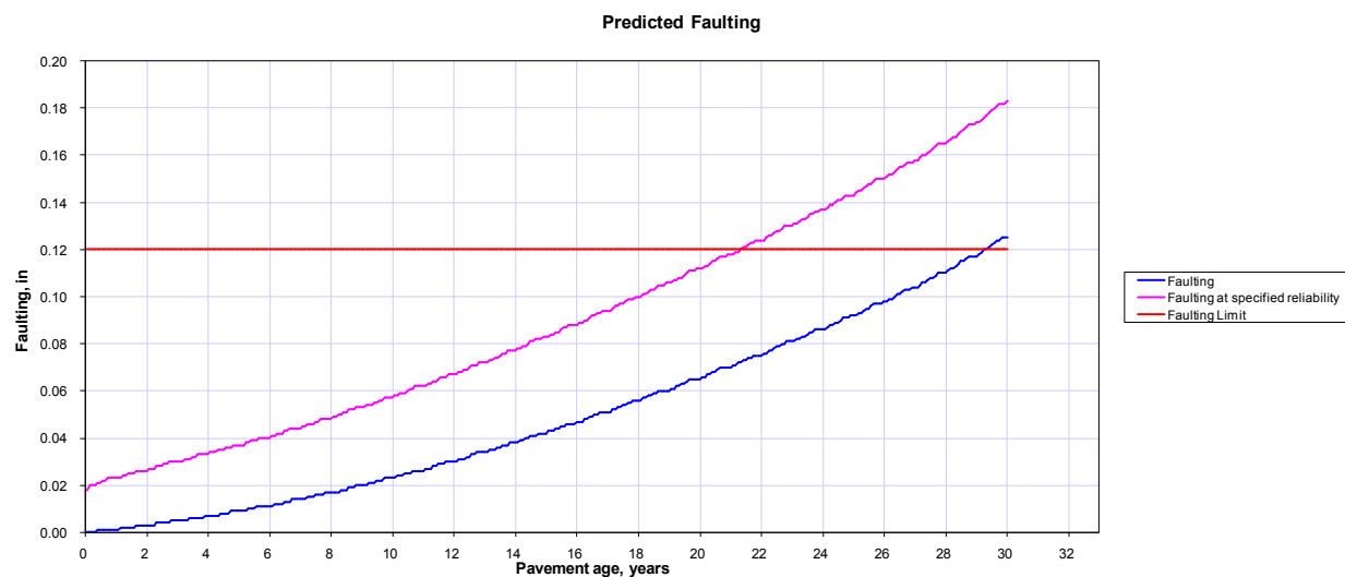
Figure 43. Plot of faulting over analysis period for new JPCP.
