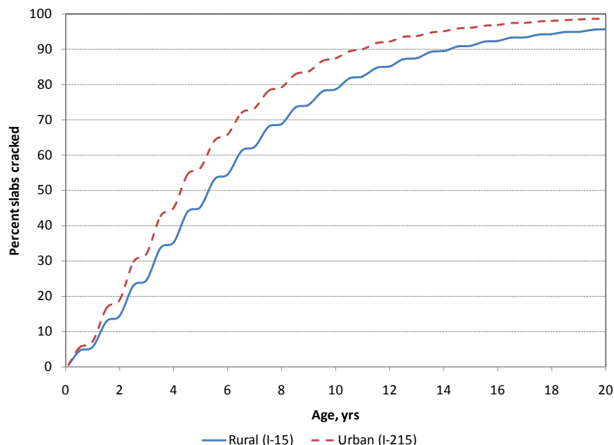
Figure 14. Effect of axle load distribution (urban & rural) on JPCP transverse “fatigue” cracking.
