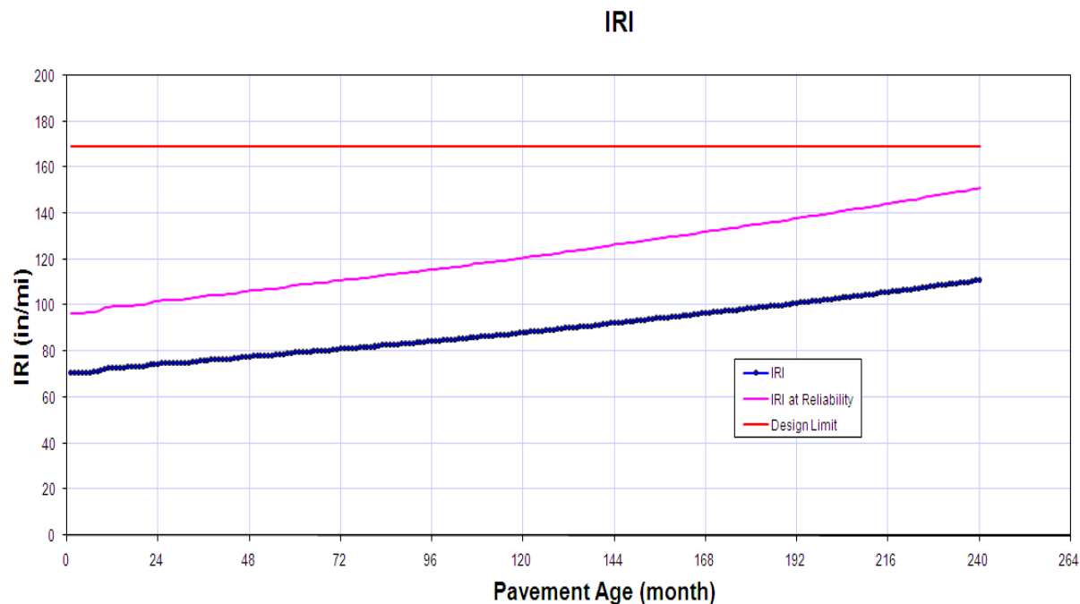
Figure A-21. Plot showing predicted IRI over the design life of the 8-in HMA pavement. The design criterion of 169 in/miles is met by the top curve at 90 percent reliability. Note that top curve is the 90 percentile and the lowest curve is the mean 50 percentile prediction curve.
