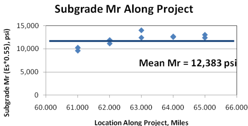
Figure A-16. Profile of subgrade Mr along the project as determined by backcalculation and then multiplying by the 0.55 (A-4 fine grained soil) to obtain the mean input for the MEPDG of 12,383 psi.
