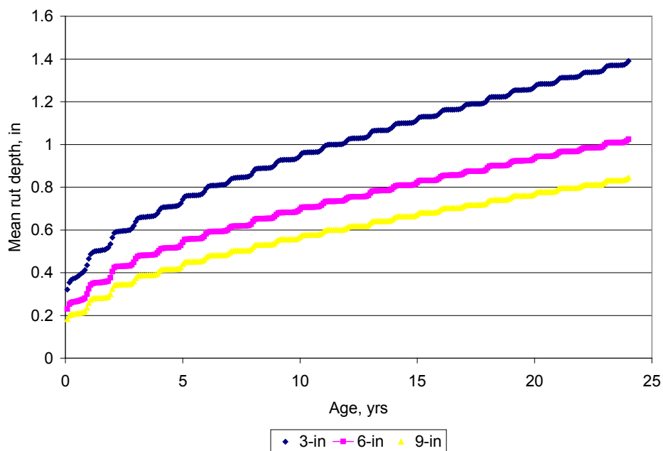
Figure 22. Large Effect of HMA thickness on rutting.
