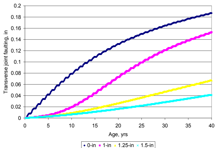
Figure 29. Large effect of JPCP transverse joint load transfer efficiency (LTE) on joint faulting.
