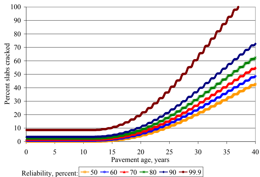
Figure 7. Illustration of the effect of design reliability on JPCP fatigue cracking. (Note the very large effect when reliability approaches 99.9 percent)
