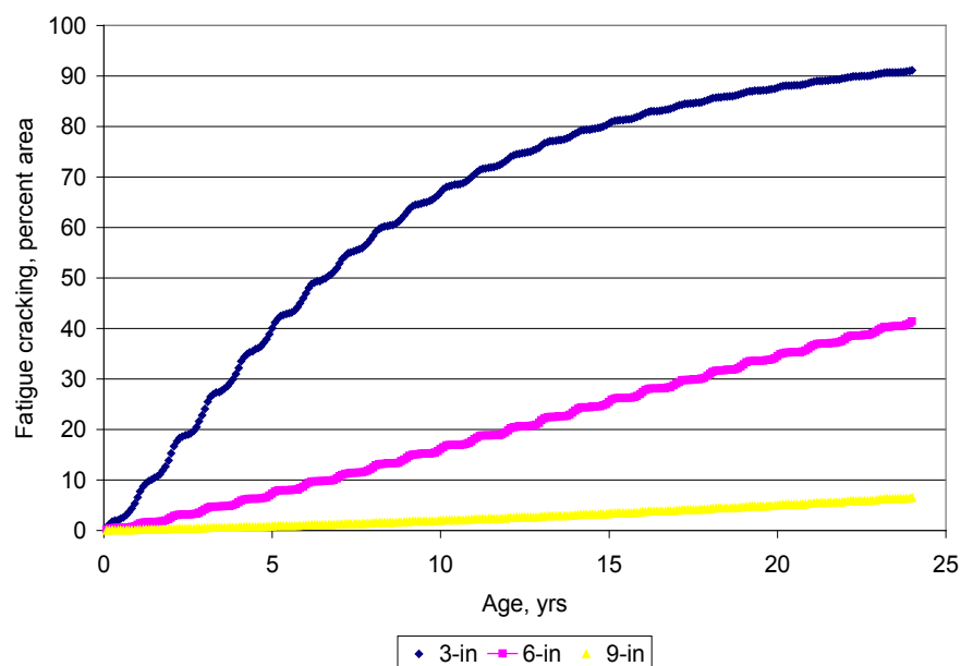
Figure 21. Large Effect of HMA thickness on HMA bottom up alligator fatigue cracking.
