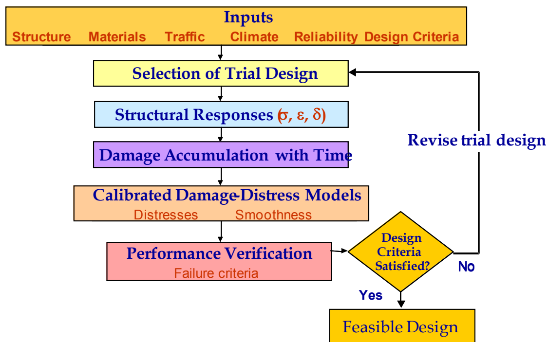
Figure 1. MEPDG overall trial &amp; error process.
