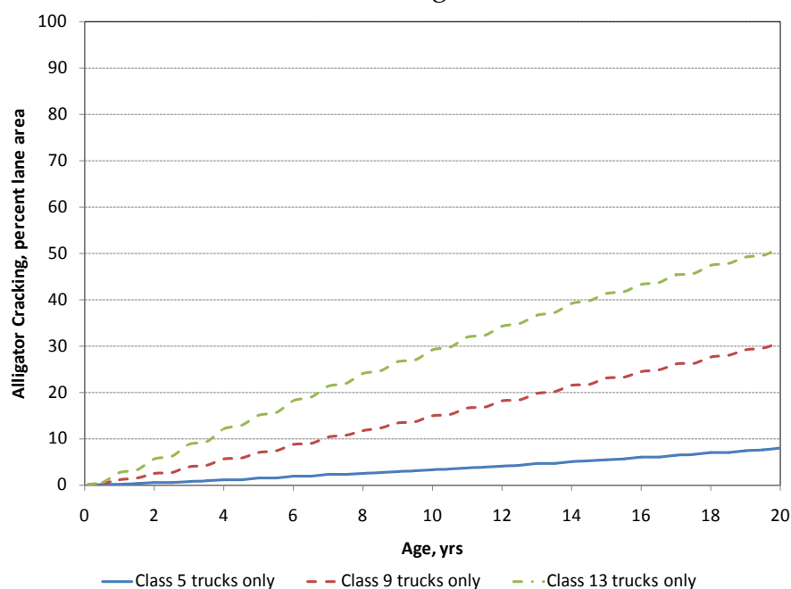
Figure 15. Effect of vehicle class distribution (same number of class 5, class 9, & class 13 trucks) HMA fatigue cracking.
