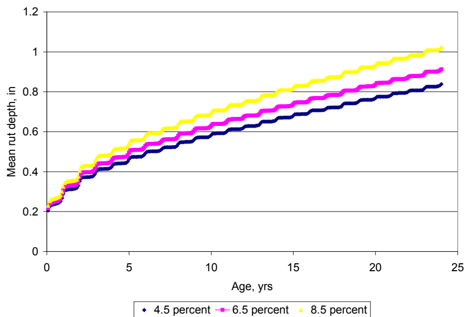
Figure 24. Significant Effect of HMA in situ air void content on rutting.
