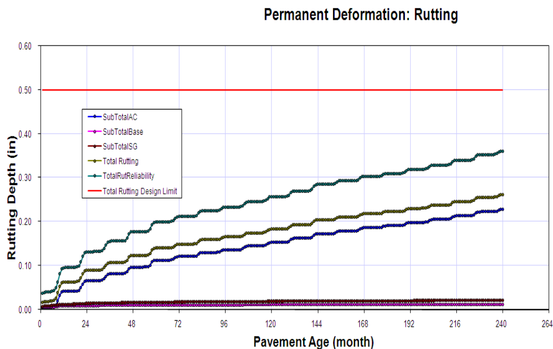
Figure A-20. Permanent deformation or rutting over time. The horizontal red line is the design criteria of 0.50-in, top curve is the 90 percent reliability level, second curve down is mean 50 percent total rutting prediction, third curve down is the HMA rutting, and lower two curves are unbound base/subbase and subgrade.
