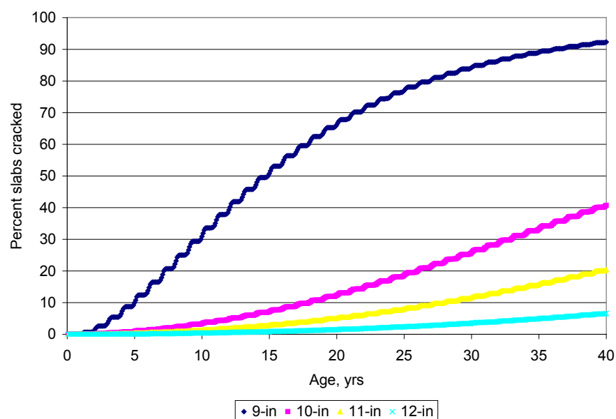
Figure 30. Large effect of PCC slab thickness on transverse cracking of JPCP.
