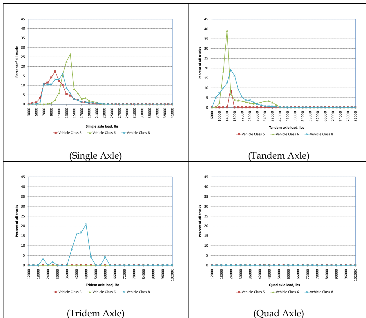
Figure 10. Example of axle load distributions for site HMA_R1 01 (local route).
