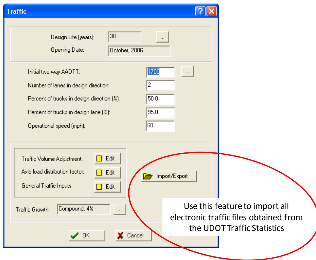
Figure 35. MEPDG features used for directly importing traffic inputs in electronic format.
