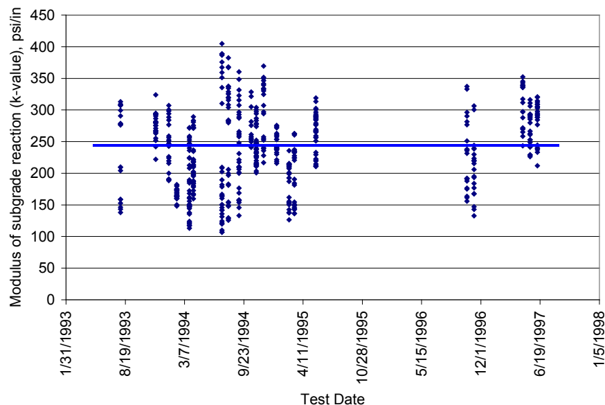
Figure B-14. Backcalculated dynamic k-value using data from FWD center slab loading.
