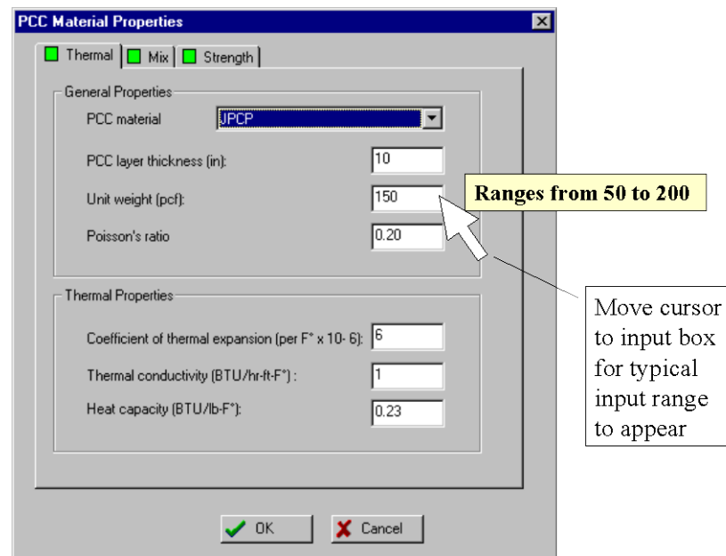
Figure 6. Tool tip help.
