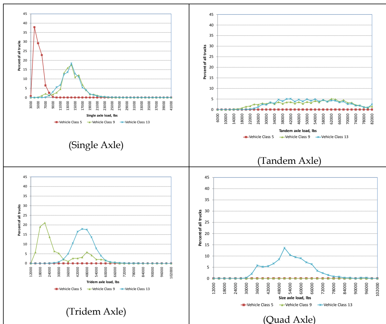
Figure 12. Example of axle load distributions for site CPR7 (urban Interstate).
