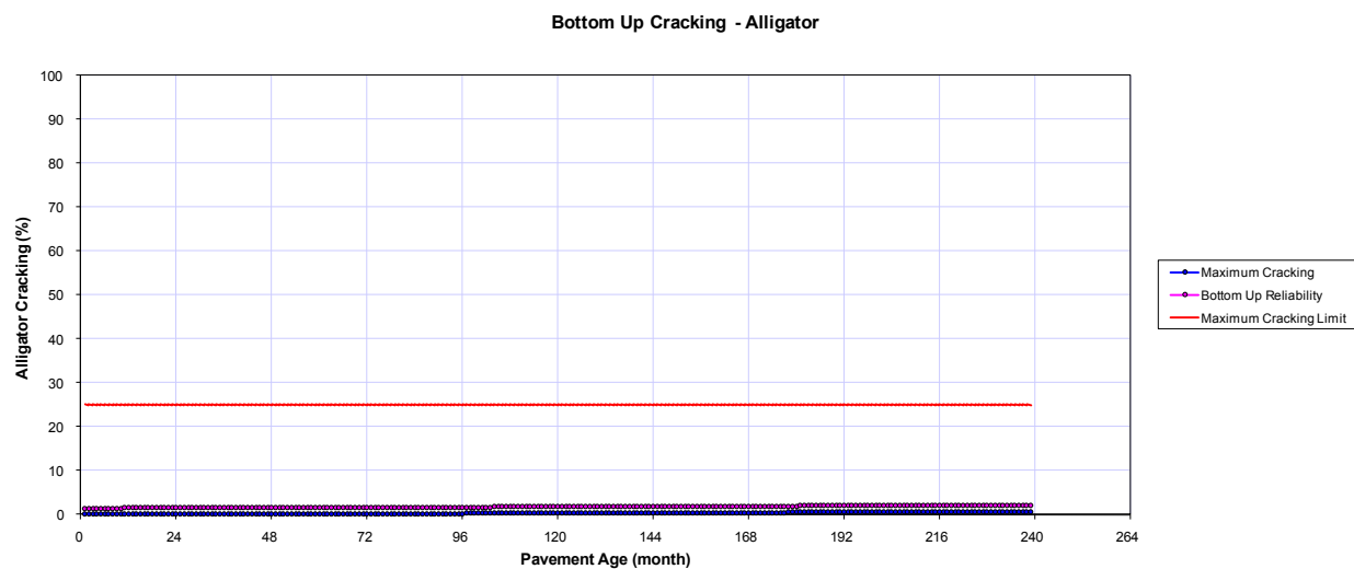
Figure 39. Plot of bottom-up cracking over analysis period for new HMA.
