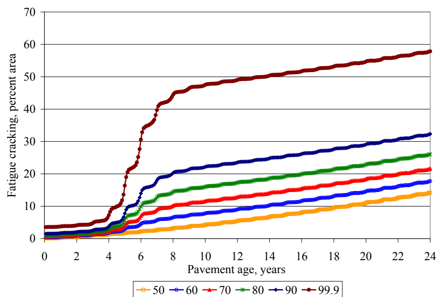
Figure 8. Illustration of the effect of design reliability on HMA fatigue cracking. (Note the very large effect when reliability approaches 99.9 percent)
