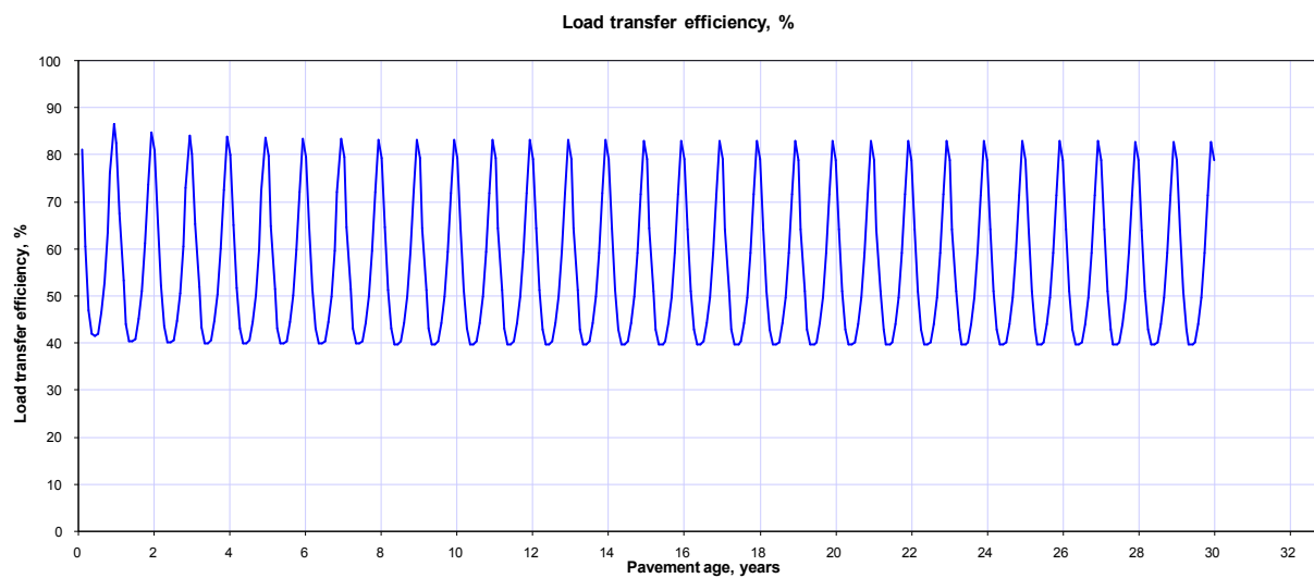
Figure 44. Plot of LTE over analysis period for new JPCP without dowels.
