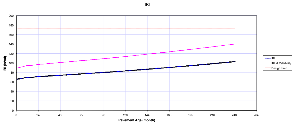
Figure 42. Plot of IRI over analysis period for new HMA.
