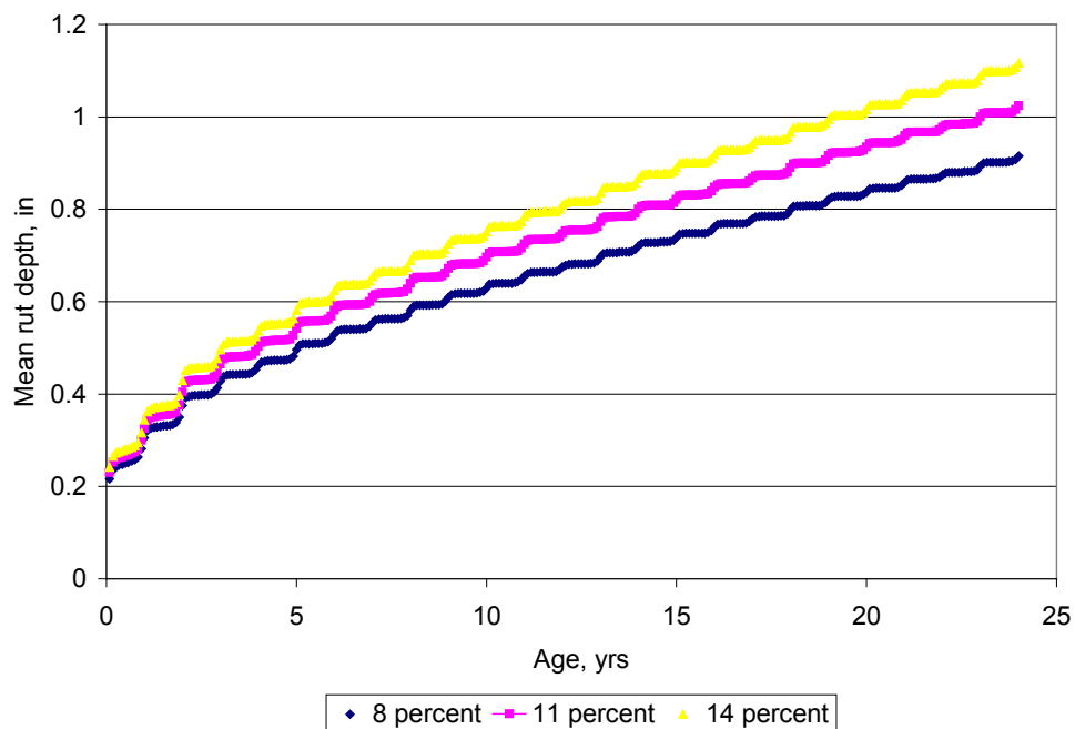
Figure 26. Significant Effect of HMA volumetric binder content on rutting.
