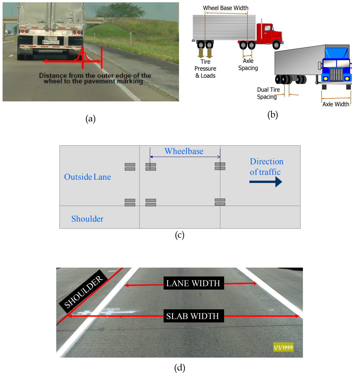
Figure 13. Schematic illustration of mean wheel location (a), axle configuration and wheelbase (b and c), and lane width (d).
