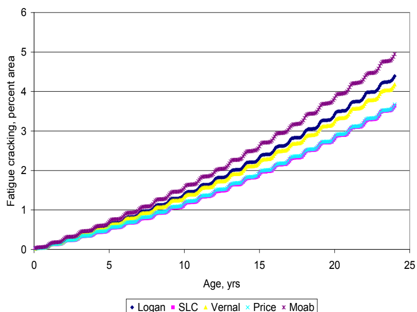
Figure 18. Significant Effect of Utah climates on HMA fatigue (alligator) cracking.
