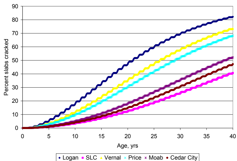
Figure 17. Significant Effect of Utah Climates on JPCP transverse cracking.
