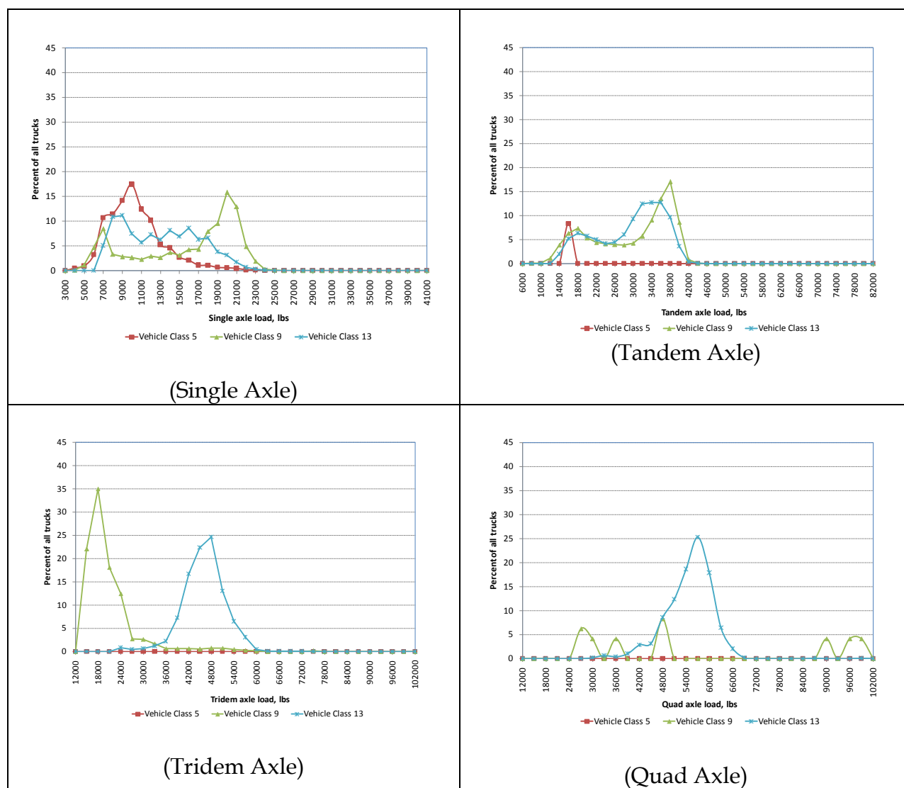
Figure 11. Example of axle load distributions for site JPCP16 (rural Interstate).
