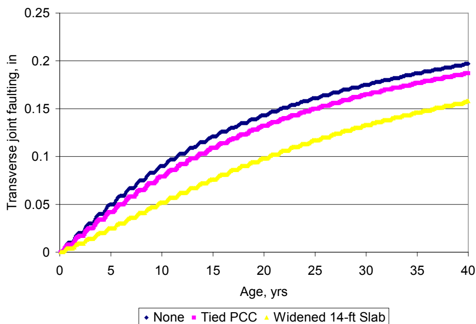
Figure 32. Effect of shoulder or widening edge support on transverse joint faulting of JPCP.
