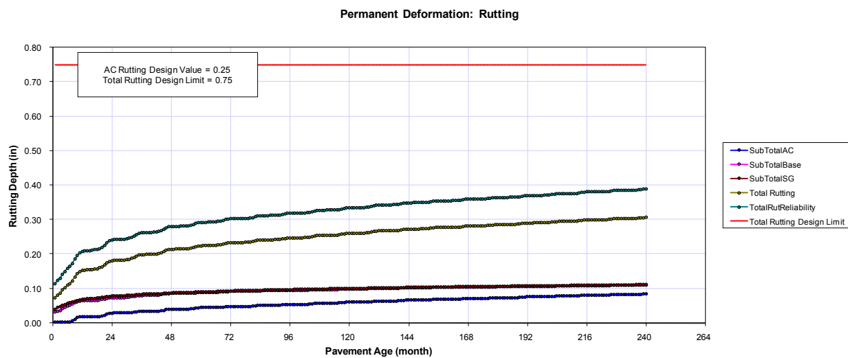
Figure 41. Plot of rutting over analysis period for new HMA.
