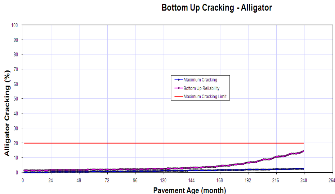
Figure A-19. Plot showing alligator cracking, percent lane area over time. The horizontal red line is the design criteria of 20 percent, the dark blue lower curve is mean 50 percent prediction, and the darker red curve is 90 percent reliability level.
