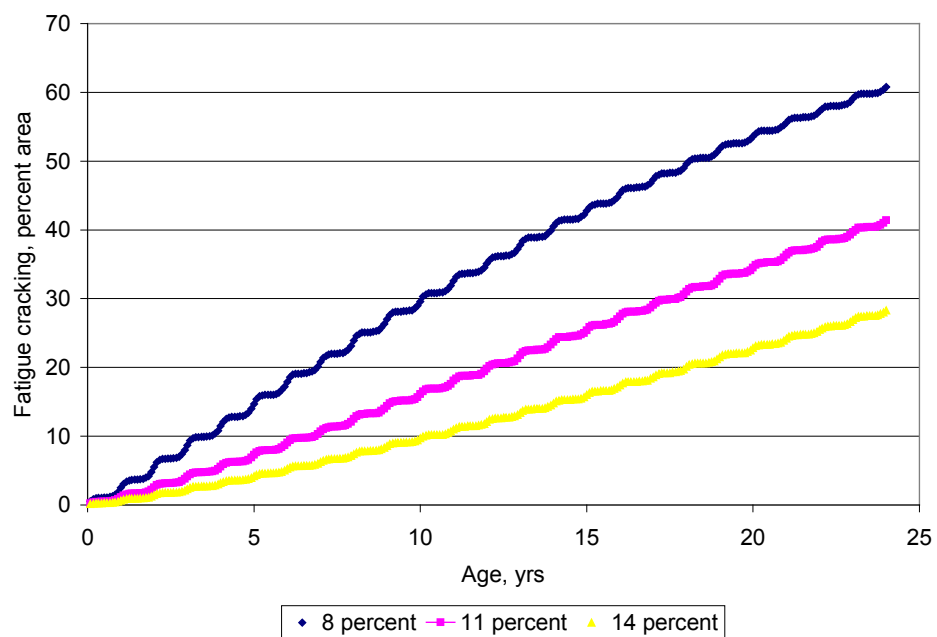
Figure 25. Large Effect of HMA volumetric binder content on fatigue (alligator) cracking.
