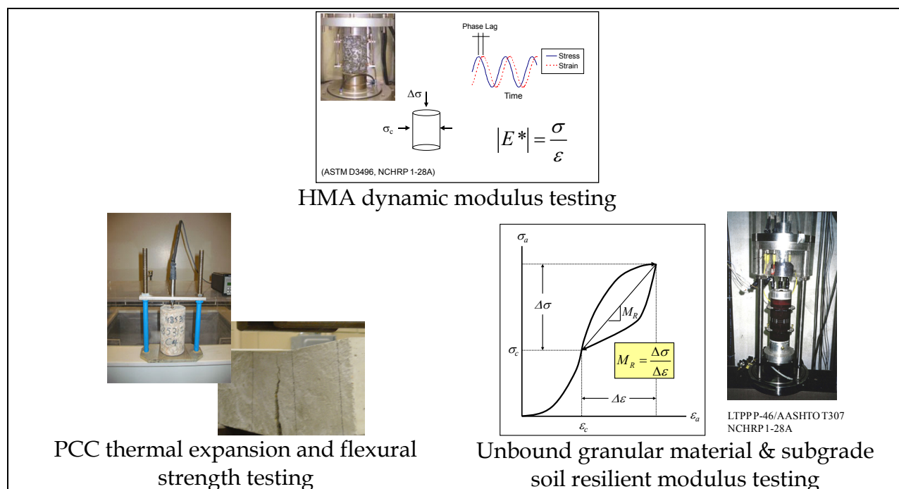
Figure 20. Level 1 material testing program.
