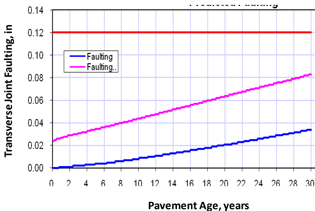
Figure B-17. Plot of predicted faulting versus pavement age.
