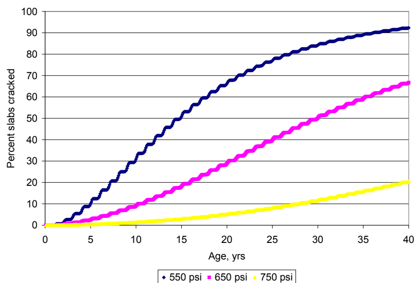
Figure 34. Large effect of PCC flexural strength on slab transverse cracking for JPCP.
