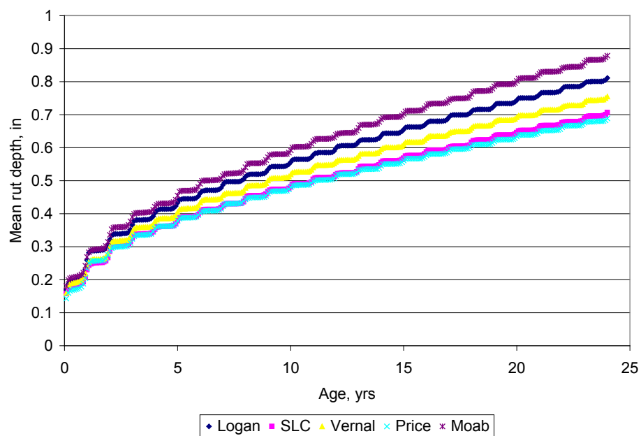
Figure 19. Significant Effect of Utah climates on HMA rutting.
