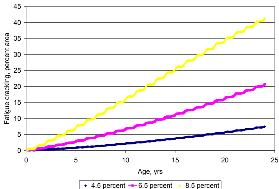
Figure 23. Large Effect of HMA in situ air void content on fatigue (alligator) cracking.
