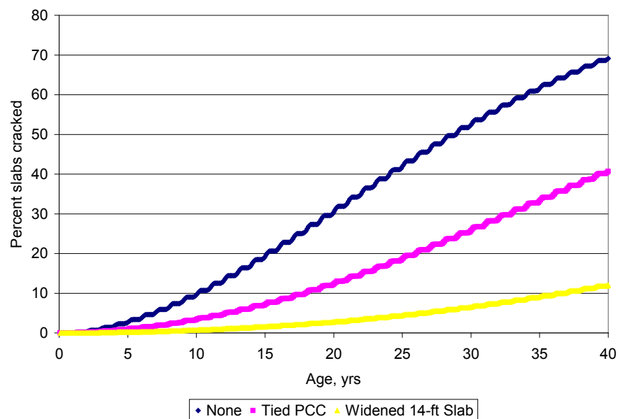
Figure 33. Large effect of edge support on slab transverse cracking for JPCP.
