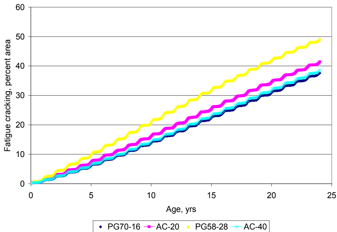
Figure 27. Effect of HMA binder type on fatigue (alligator) cracking.
