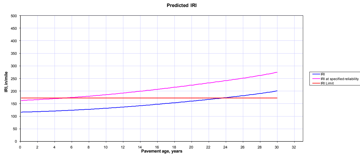
Figure 47. Plot of IRI over analysis period for new JPCP.
