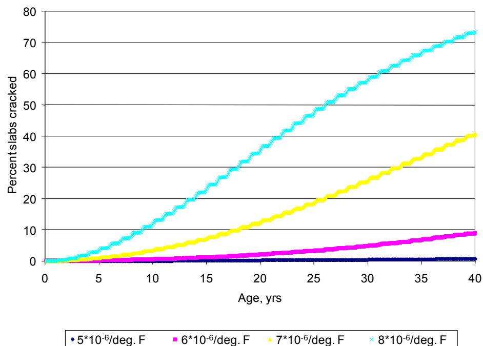
Figure 31. Large effect of PCC coefficient of thermal expansion on transverse cracking of JPCP.
