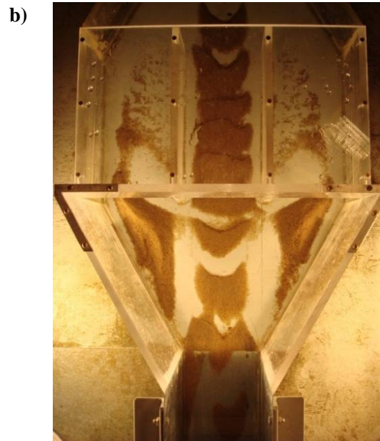
Figure 4-3-1 Sedimentation pattern compare to the baseline test result
