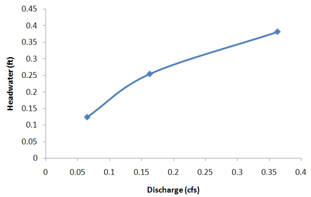
Figure 4-2-11 Flow condition in baseline test 3
