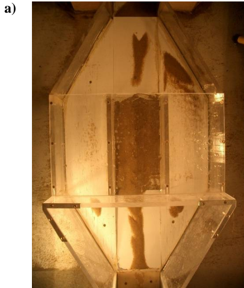
Figure 4-3-3 Sedimentation pattern compare to the baseline test result
