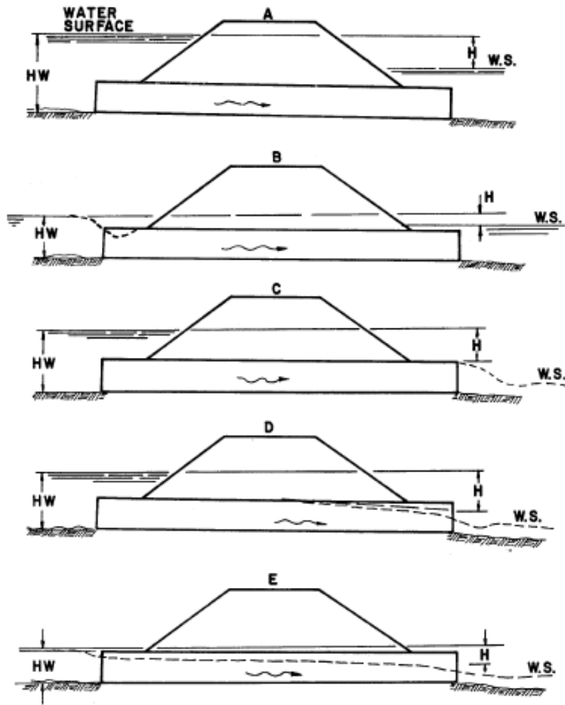
Figure 2-3-5 Types of outlet control (Normann, 1985)
