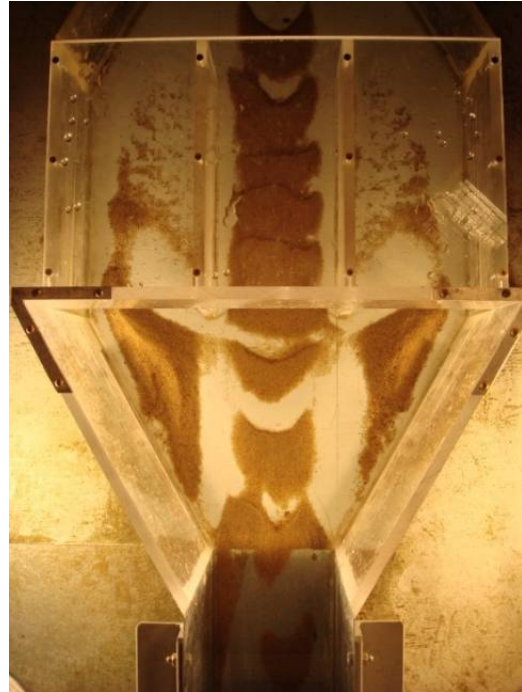
Figure 4-3-5 Sedimentation pattern compare to the baseline test result
