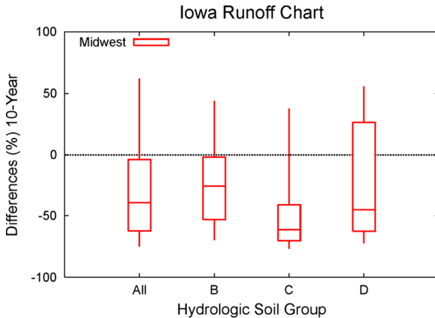
Figure 4.19: Range of 10-year return period flood frequency estimates for the Iowa Runoff Chart by hydrologic soil group. Differences (%) from the streamgauge estimates are shown for the 46 Midwest sites. The boxes contain 50% of the estimates; 90% of the estimates fall within the range shown by the bars. The median is indicated by the horizontal line within the boxes.
