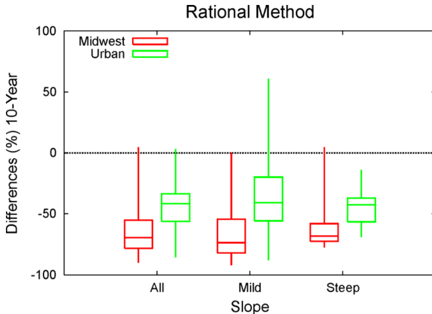
Figure 4.20: Range of 10-year return period flood frequency estimates for the Rational Method by average watershed slope. Differences (%) from the streamgauge estimates are shown for the 46 Midwest sites and the 21 Urban sites. The boxes contain 50% of the estimates; 90% of the estimates fall within the range shown by the bars. The median is indicated by the horizontal line within the boxes.
