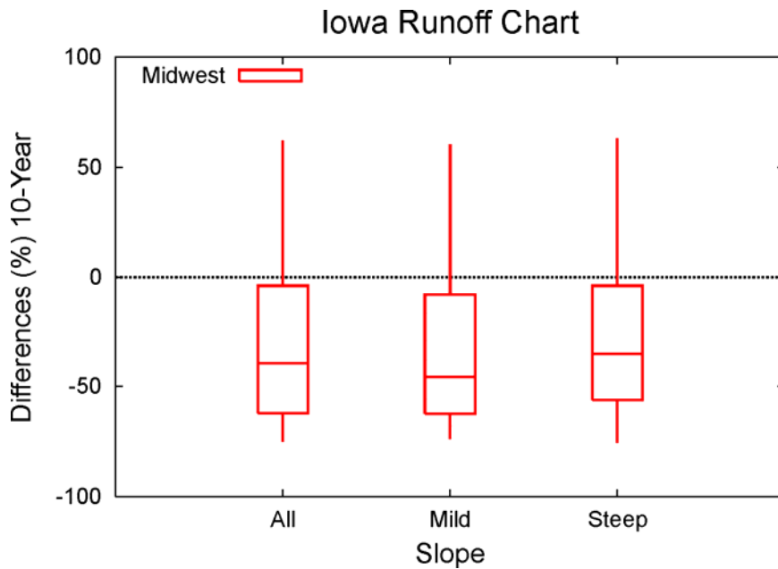
Figure 4.22: Range of 10-year return period flood frequency estimates for the Iowa Runoff Chart by average watershed slope. Differences (%) from the streamgauge estimates are shown for the 46 Midwest sites. The boxes contain 50% of the estimates; 90% of the estimates fall within the range shown by the bars. The median is indicated by the horizontal line within the boxes.
