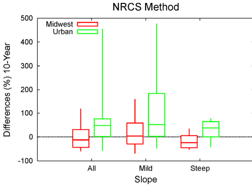
Figure 4.21: Range of 10-year return period flood frequency estimates for the NRCS method by average watershed slope. Differences (%) from the streamgauge estimates are shown for the 46 Midwest sites and the 21 Urban sites. The boxes contain 50% of the estimates; 90% of the estimates fall within the range shown by the bars. The median is indicated by the horizontal line within the boxes.
