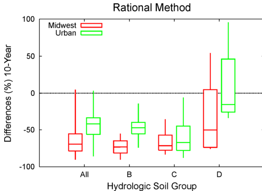
Figure 4.17: Range of 10-year return period flood frequency estimates for the Rational Method by hydrologic soil group. Differences (%) from the streamgauge estimates are shown for the 46 Midwest sites and the 21 Urban sites. The boxes contain 50% of the estimates; 90% of the estimates fall within the range shown by the bars. The median is indicated by the horizontal line within the boxes.
