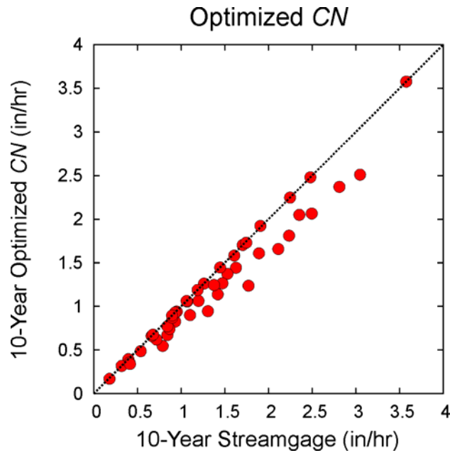
Figure 4.29: Estimates of the 10-year return period peak discharge based on the optimized NRCS runoff curve number and streamgauge data for the 46 Midwest sites. The peak discharge per unit area (in/hr) is shown to facilitate comparison.
