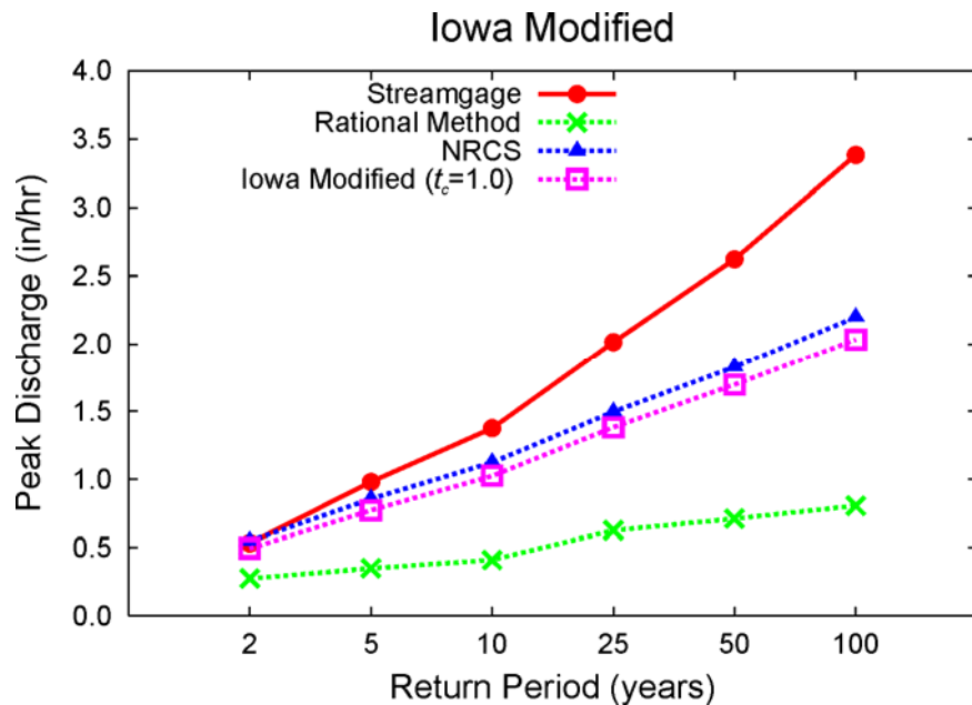
Figure 4.27: Average flood frequency estimates for the 46 Midwest sites based on streamgauge data, the Rational Method, the NRCS curve number method, and the Iowa-modified Rational Method. The peak discharge per unit area (in/hr) is shown to facilitate comparison.
