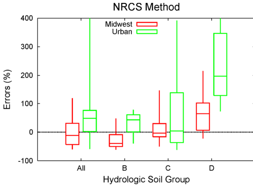
Figure 4.18: Range of 10-year return period flood frequency estimates for the NRCS Method by hydrologic soil group. Differences (%) from the streamgauge estimates are shown for the 46 Midwest sites and the 21 Urban sites. The boxes contain 50% of the estimates; 90% of the estimates fall within the range shown by the bars. The median is indicated by the horizontal line within the boxes.
