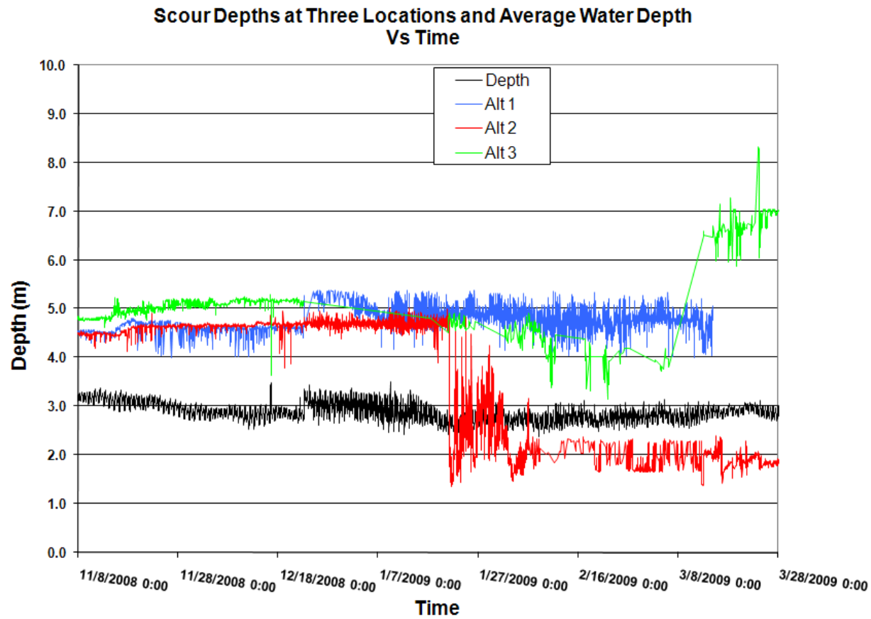
Figure 8 Scour depth at three locations and water depth seaward of the pier versus time.
