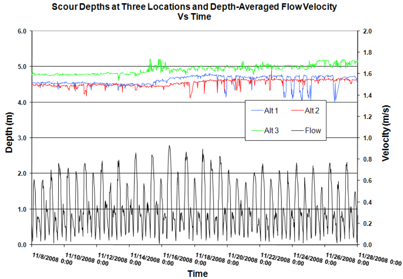
Figure 7 Scour depth and depth averaged flow velocity versus time for a 20 day interval.
