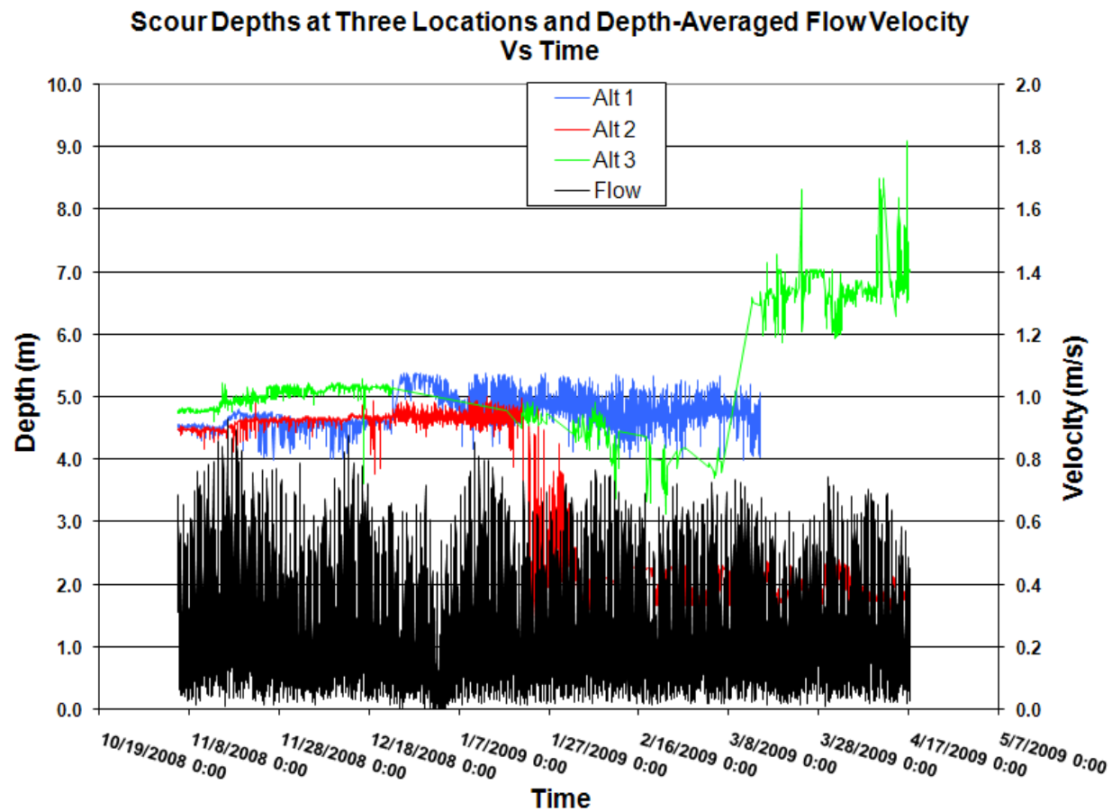
Figure 6 Scour depth and depth-averaged flow velocity versus time.
