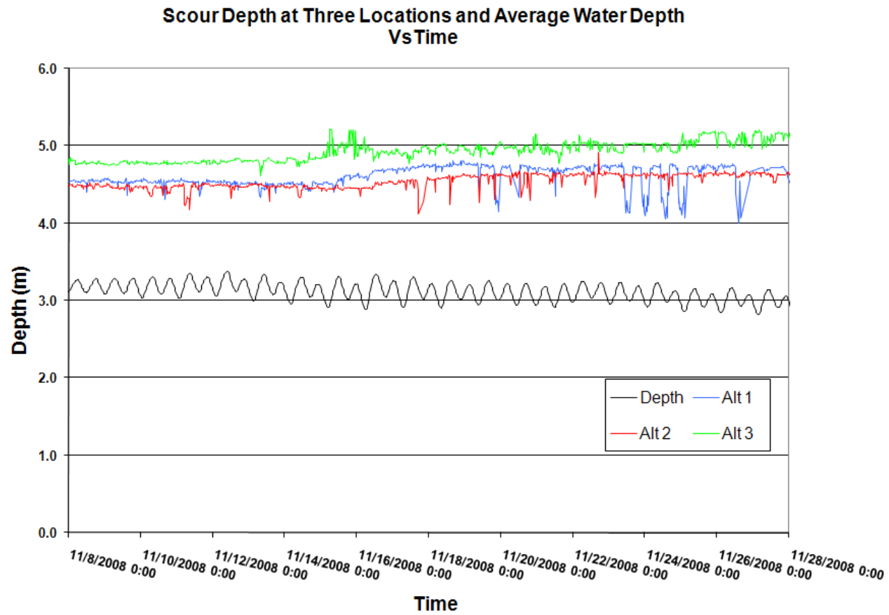
Figure 9 Scour depth at three locations and water depth seaward of the pier versus time for a 20 day time interval.
