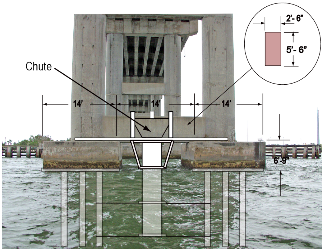
Figure 3 Drawing showing sand chute used in placing sediment in local scour hole.
