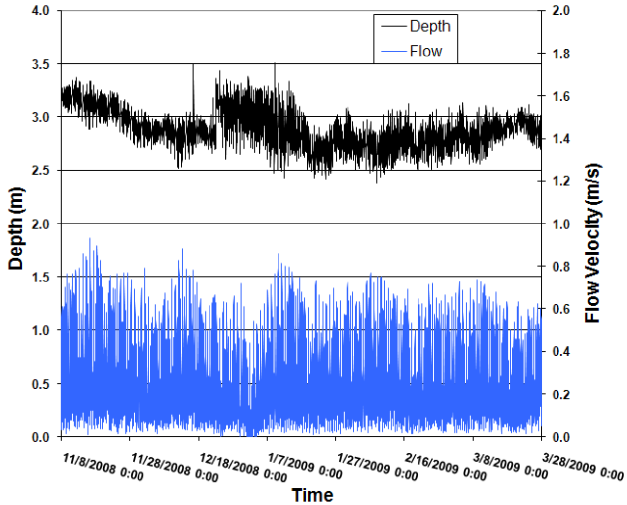
Average Water Depth and Depth-Average Flow Velocity Vs Time
