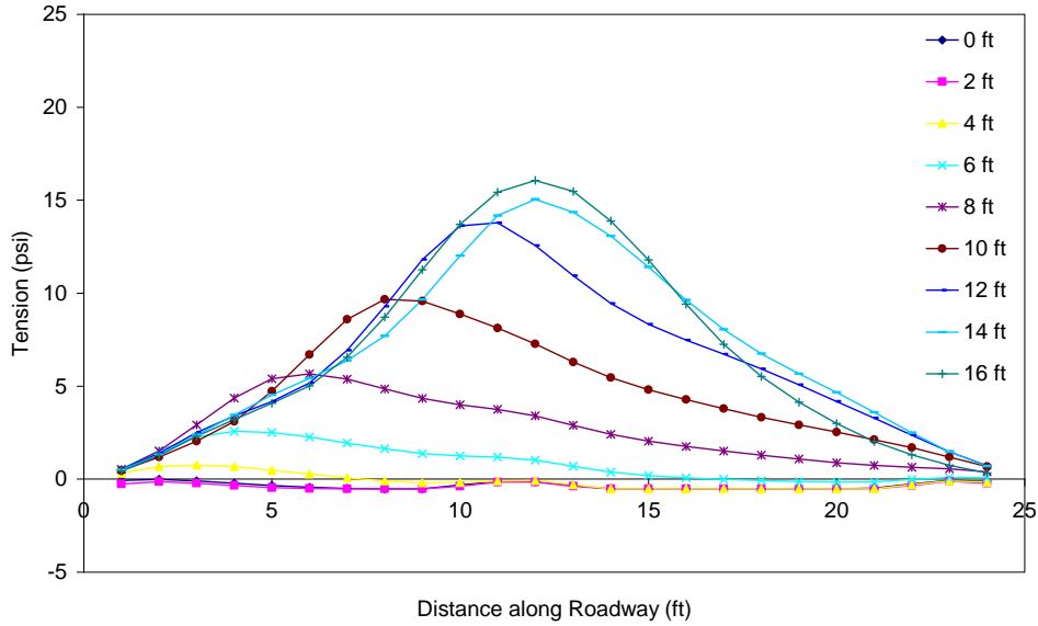
Figure C.38 Tension in the asphalt throughout excavation (PZ-40 wall in stronger soil with lane load) 2 ft from wall.
