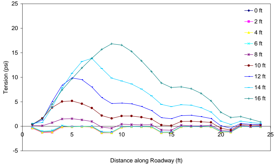
Figure C.48 Tension in the asphalt throughout excavation (PZ-40 wall in stronger soil with truck load) 10 ft from wall.
