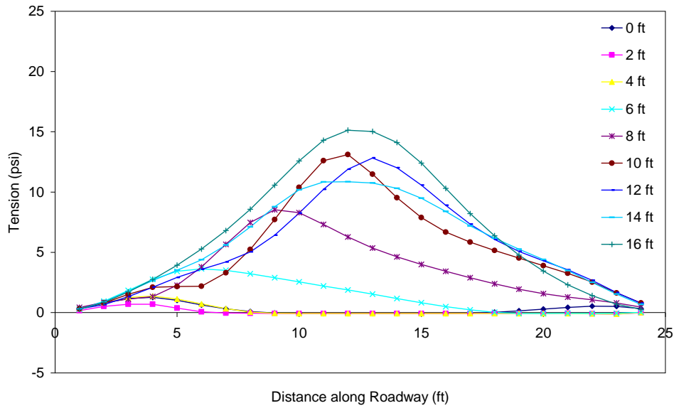
Figure C.5 Tension in the asphalt throughout excavation (PZ-27 wall in weaker soil with no load) 0 ft from wall.
