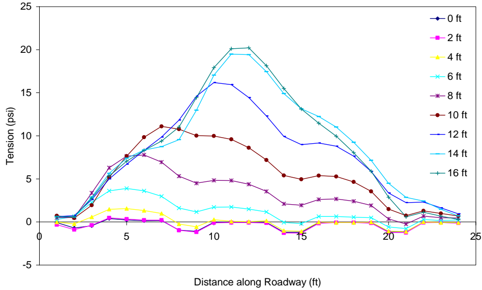
Figure C.46 Tension in the asphalt throughout excavation (PZ-40 wall in stronger soil with truck load) 2 ft from wall.
