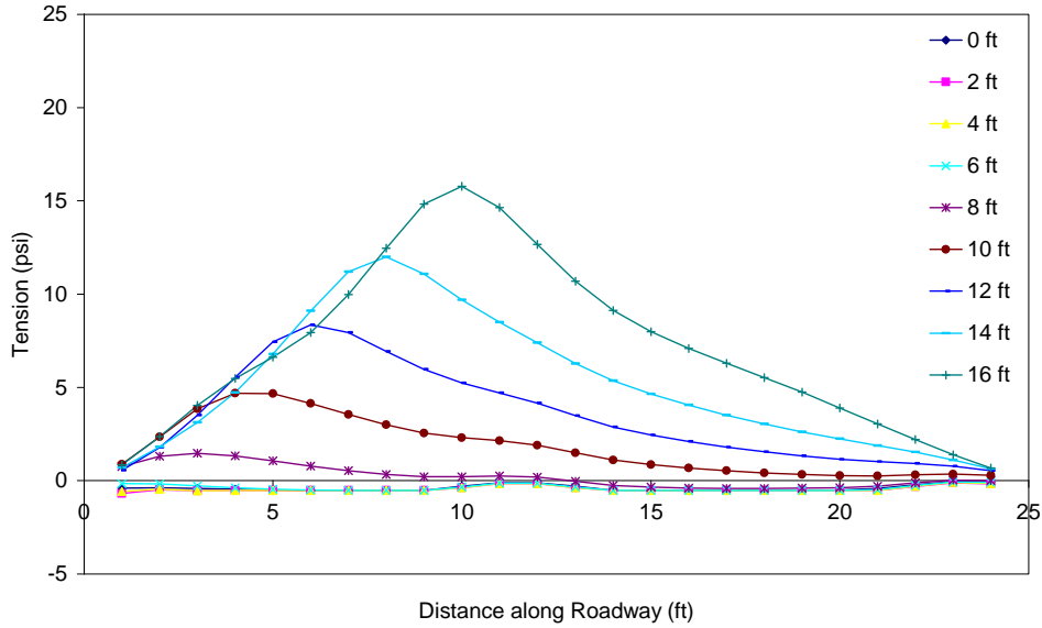
Figure C.40 Tension in the asphalt throughout excavation (PZ-40 wall in stronger soil with lane load) 10 ft from wall.
