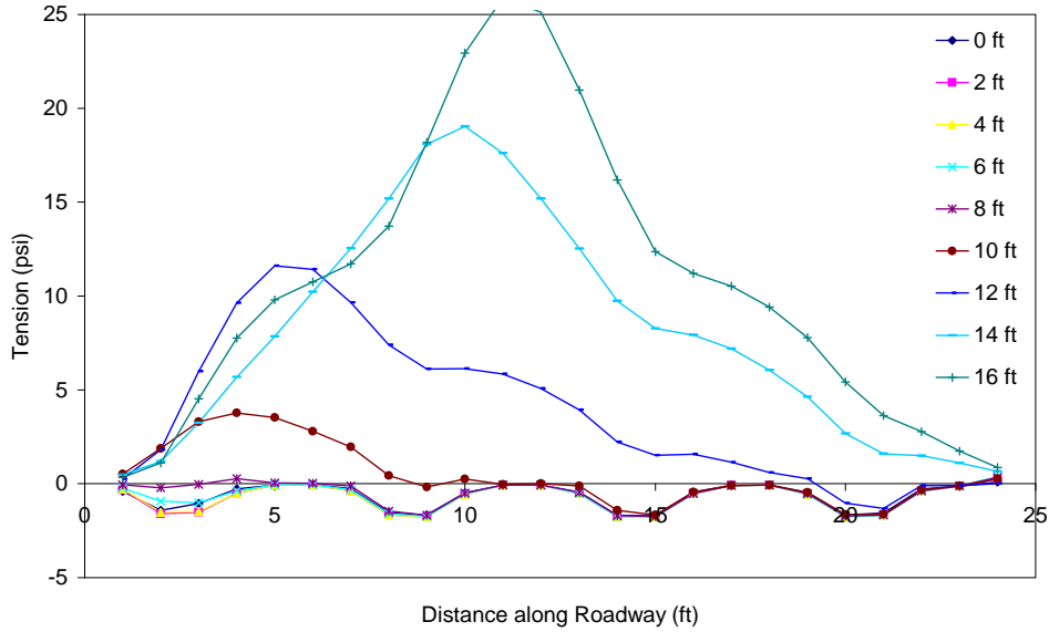
Figure C.12 Tension in the asphalt throughout excavation (PZ-27 wall in weaker soil with truck load) 10 ft from wall.
