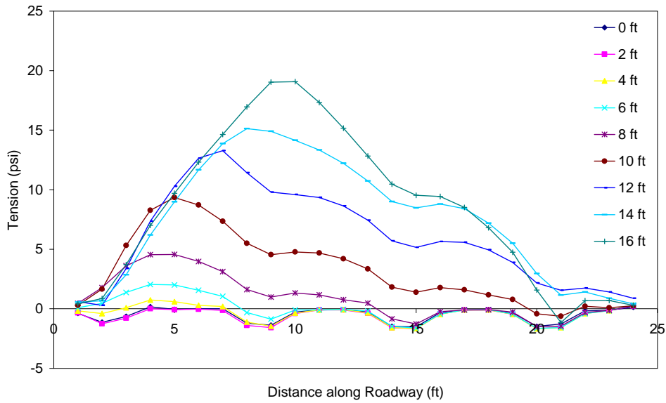
Figure C.23 Tension in the asphalt throughout excavation (PZ-40 wall in weaker soil with truck load) 5 ft from wall.
