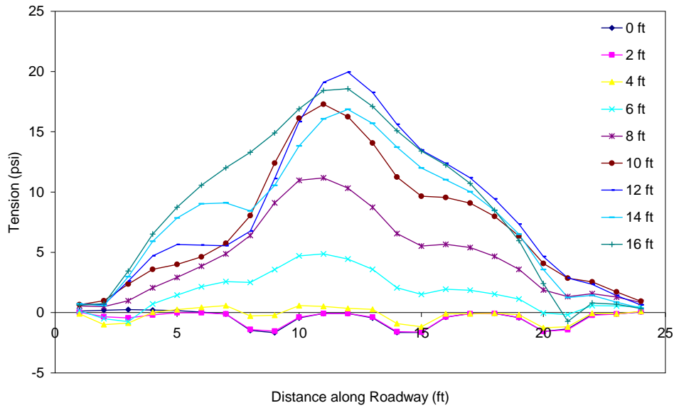
Figure C.21 Tension in the asphalt throughout excavation (PZ-40 wall in weaker soil with truck load) 0 ft from wall.
