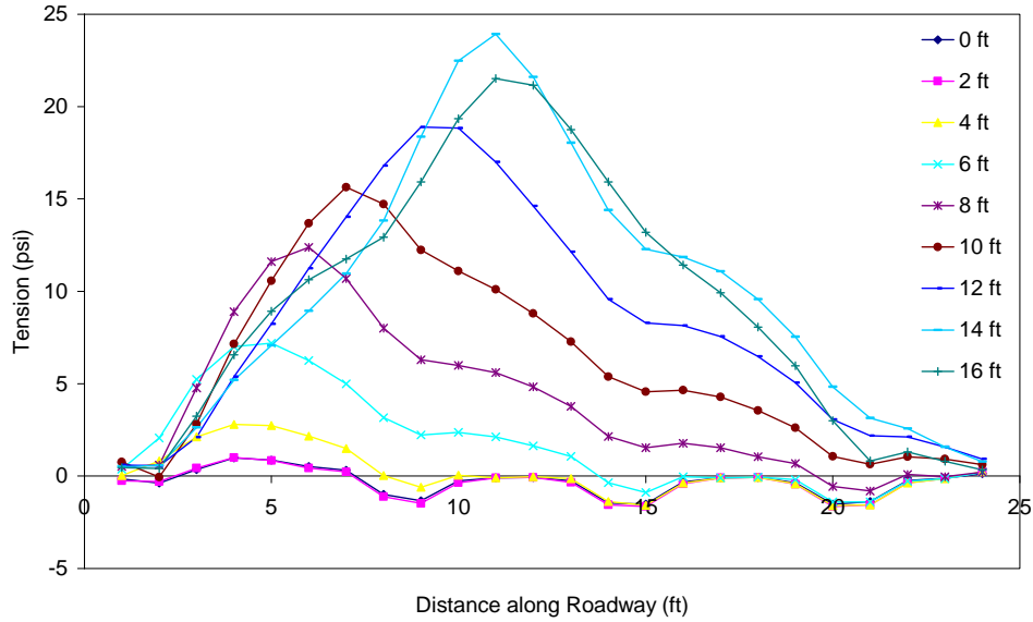
Figure C.22 Tension in the asphalt throughout excavation (PZ-40 wall in weaker soil with truck load) 2 ft from wall.
