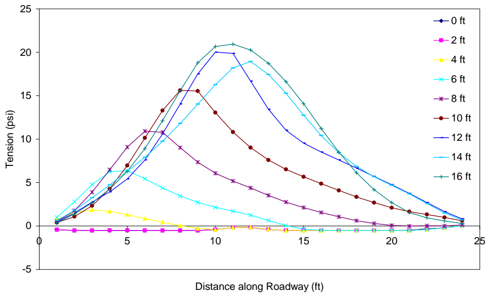
Figure C.2 Tension in the asphalt throughout excavation (PZ-27 wall in weaker soil with lane load) 2 ft from wall.
