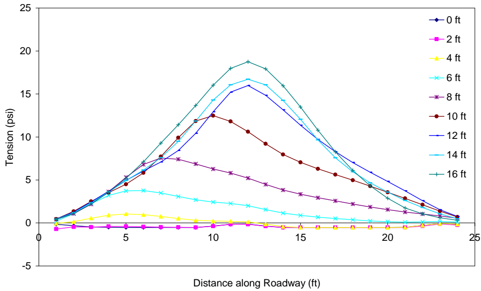
Figure C.25 Tension in the asphalt throughout excavation (PZ-27 wall in stronger soil with lane load) 0 ft from wall.
