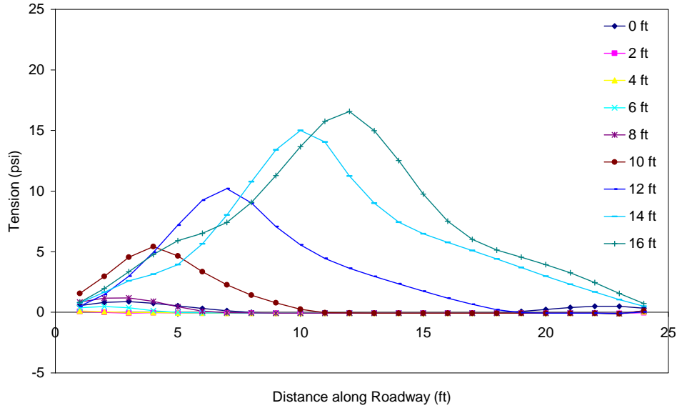
Figure C.8 Tension in the asphalt throughout excavation (PZ-27 wall in weaker soil with no load) 10 ft from wall.
