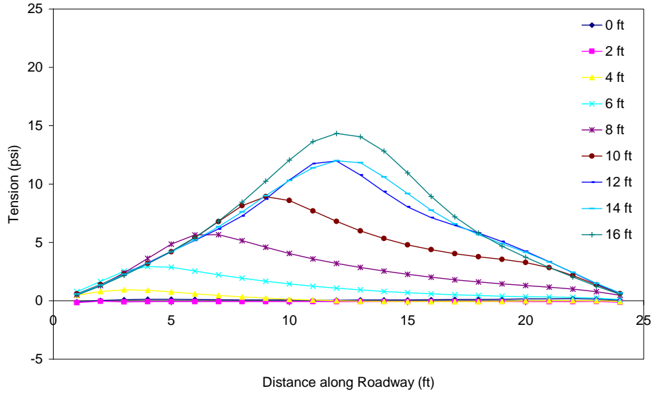
Figure C.30 Tension in the asphalt throughout excavation (PZ-27 wall in stronger soil with no load) 2 ft from wall.
