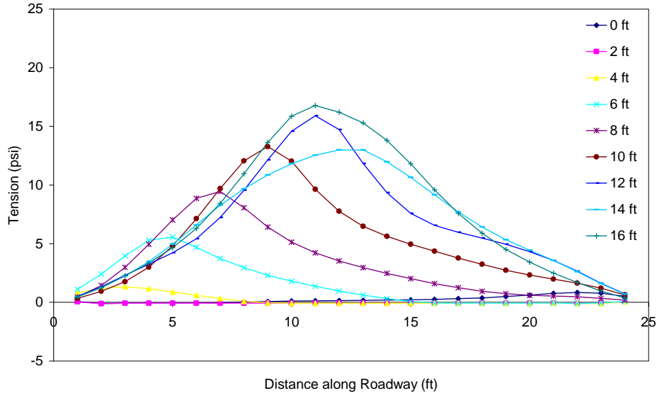
Figure C.6 Tension in the asphalt throughout excavation (PZ-27 wall in weaker soil with no load) 2 ft from wall.
