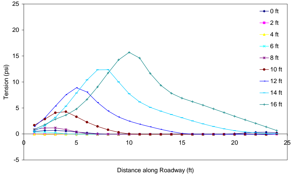
Figure C.20 Tension in the asphalt throughout excavation (PZ-40 wall in weaker soil with no load) 10 ft from wall.
