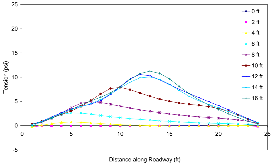
Figure C.41 Tension in the asphalt throughout excavation (PZ-40 wall in stronger soil with no load) 0 ft from wall.
