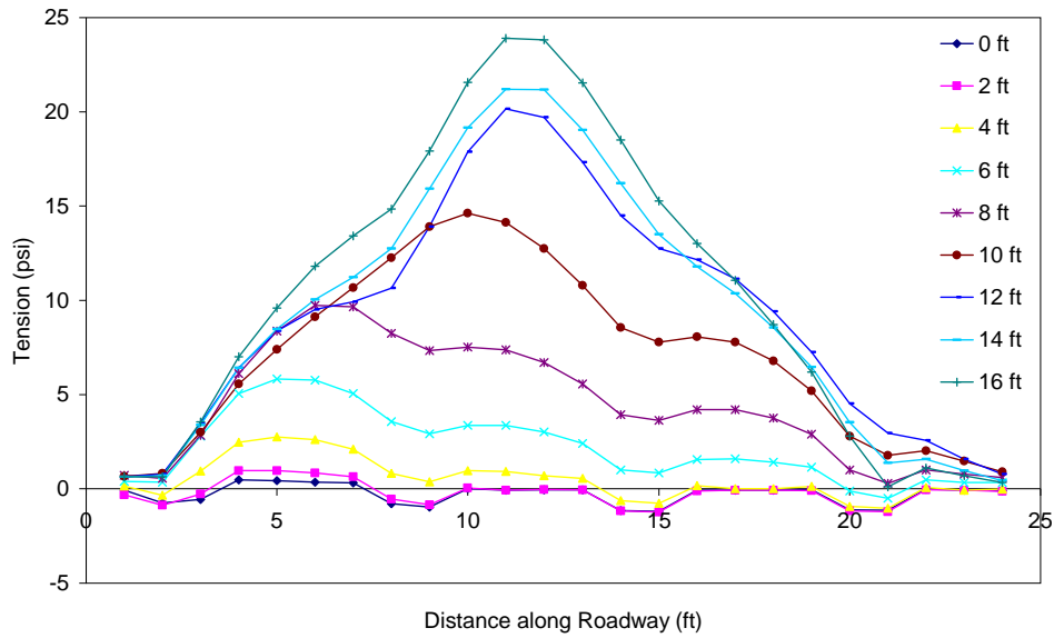
Figure C.33 Tension in the asphalt throughout excavation (PZ-27 wall in stronger soil with truck load) 0 ft from wall.
