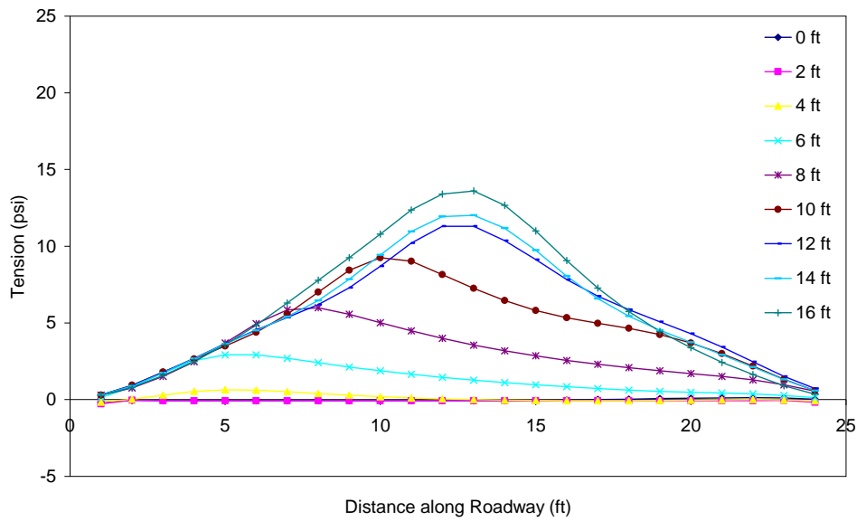
Figure C.29 Tension in the asphalt throughout excavation (PZ-27 wall in stronger soil with no load) 0 ft from wall.
