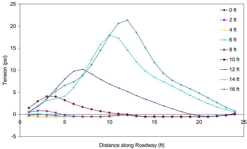
Figure C.4 Tension in the asphalt throughout excavation (PZ-27 wall in weaker soil with lane load) 10 ft from wall.
