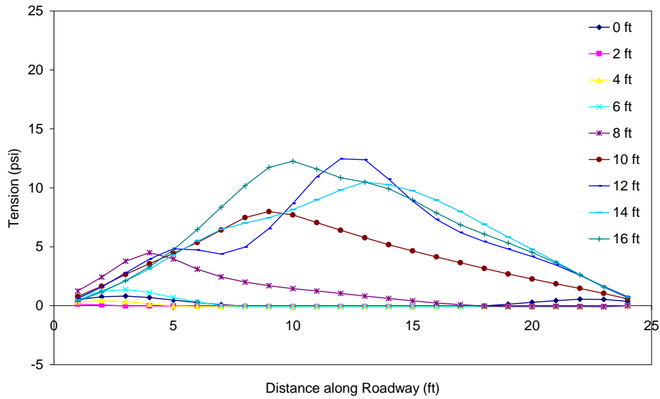
Figure C.7 Tension in the asphalt throughout excavation (PZ-27 wall in weaker soil with no load) 5 ft from wall.
