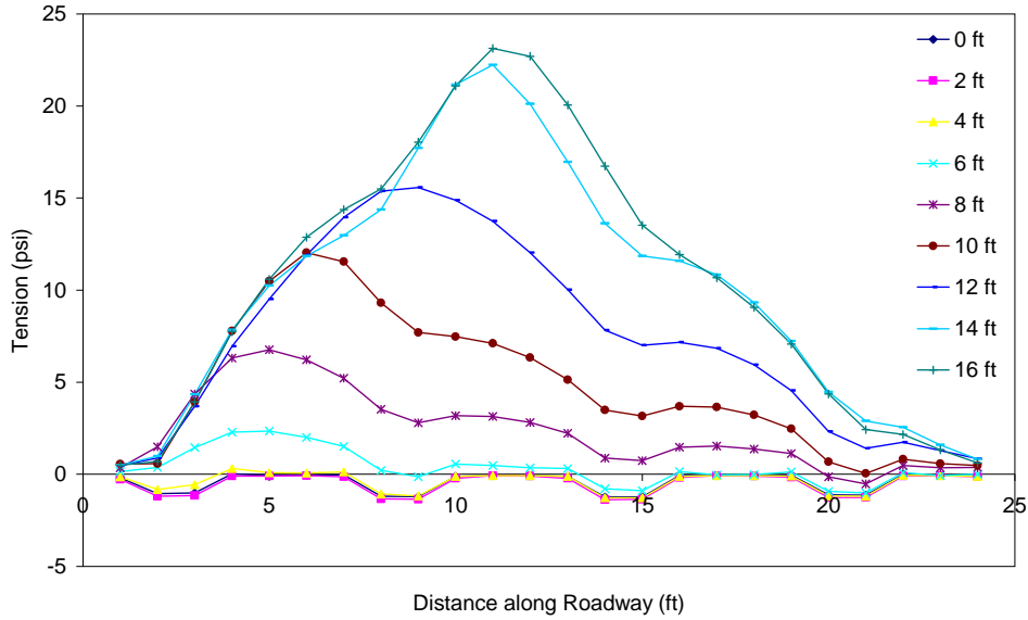
Figure C.35 Tension in the asphalt throughout excavation (PZ-27 wall in stronger soil with truck load) 5 ft from wall.
