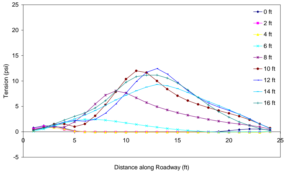
Figure C.17 Tension in the asphalt throughout excavation (PZ-40 wall in weaker soil with no load) 0 ft from wall.
