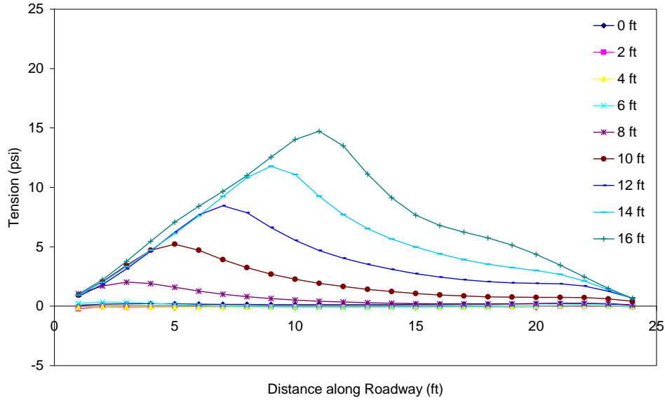
Figure C.32 Tension in the asphalt throughout excavation (PZ-27 wall in stronger soil with no load) 10 ft from wall.
