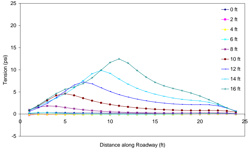
Figure C.44 Tension in the asphalt throughout excavation (PZ-40 wall in stronger soil with no load) 10 ft from wall.
