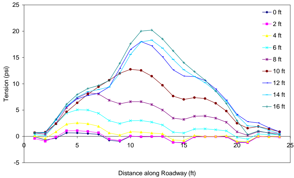
Figure C.45 Tension in the asphalt throughout excavation (PZ-40 wall in stronger soil with truck load) 0 ft from wall.
