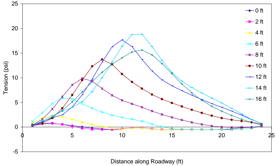
Figure C.14 Tension in the asphalt throughout excavation (PZ-40 wall in weaker soil with lane load) 2 ft from wall.
