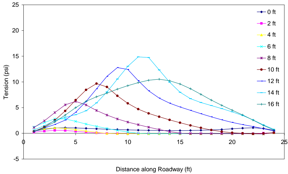
Figure C.19 Tension in the asphalt throughout excavation (PZ-40 wall in weaker soil with no load) 5 ft from wall.
