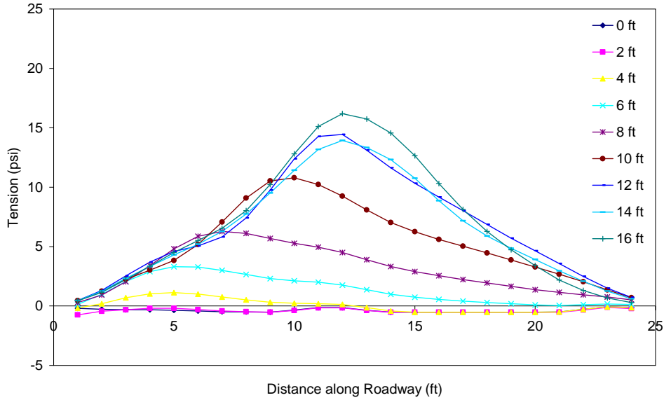
Figure C.37 Tension in the asphalt throughout excavation (PZ-40 wall in stronger soil with lane load) 0 ft from wall.
