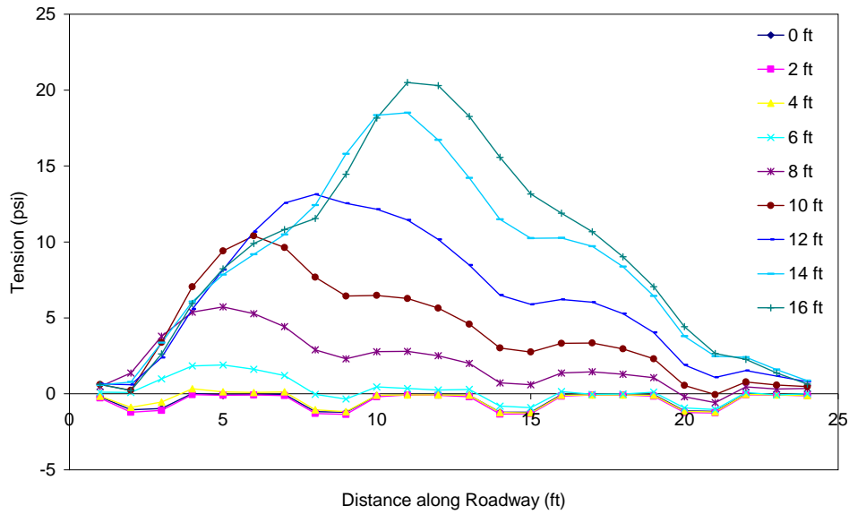
Figure C.47 Tension in the asphalt throughout excavation (PZ-40 wall in stronger soil with truck load) 5 ft from wall.
