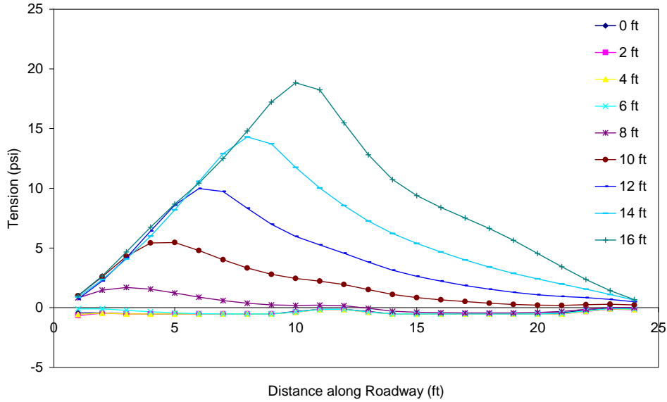
Figure C.28 Tension in the asphalt throughout excavation (PZ-27 wall in stronger soil with lane load) 10 ft from wall.
