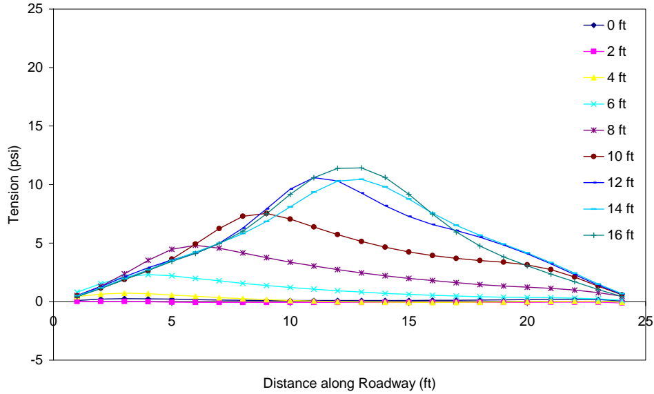
Figure C.42 Tension in the asphalt throughout excavation (PZ-40 wall in stronger soil with no load) 2 ft from wall.
