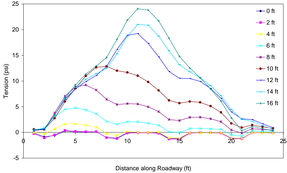
Figure C.34 Tension in the asphalt throughout excavation (PZ-27 wall in stronger soil with truck load) 2 ft from wall.
