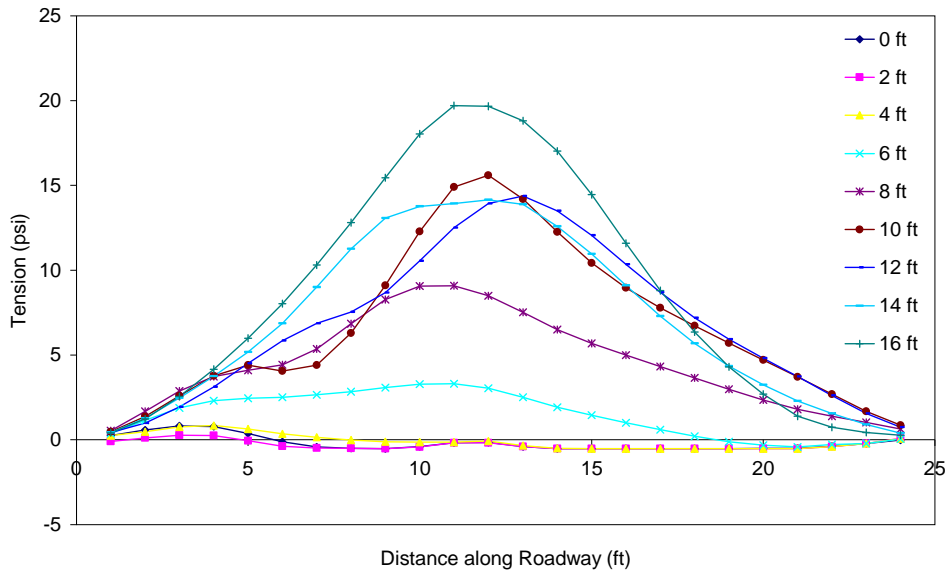
Figure C.1 Tension in the asphalt throughout excavation (PZ-27 wall in weaker soil with lane load) 0 ft from wall.
