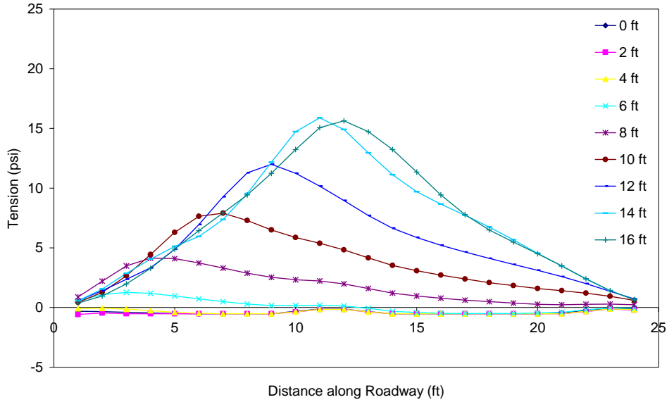
Figure C.39 Tension in the asphalt throughout excavation (PZ-40 wall in stronger soil with lane load) 5 ft from wall.
