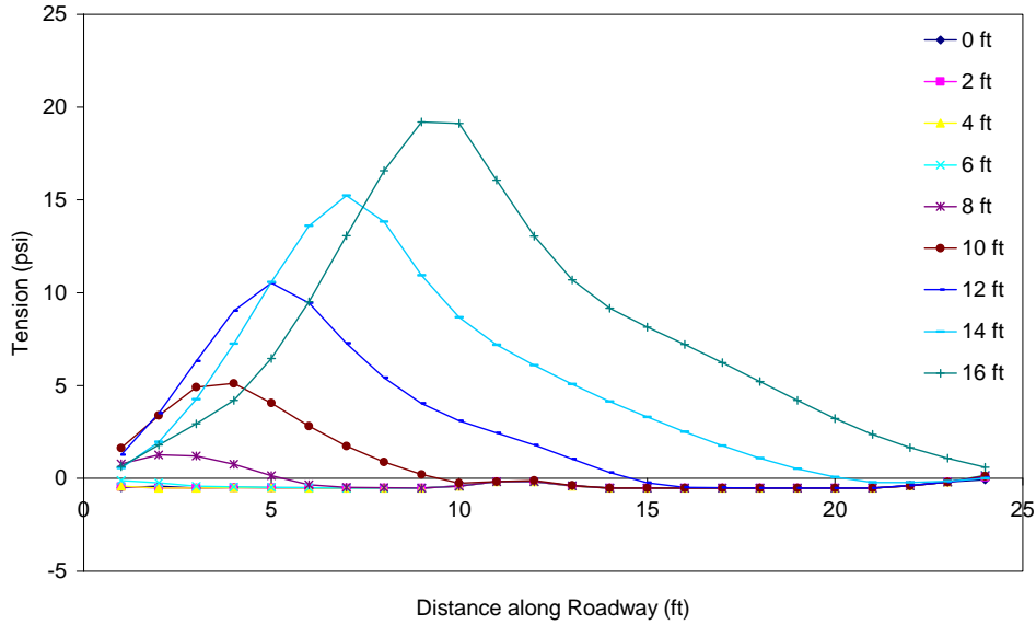
Figure C.16 Tension in the asphalt throughout excavation (PZ-40 wall in weaker soil with lane load) 10 ft from wall.
