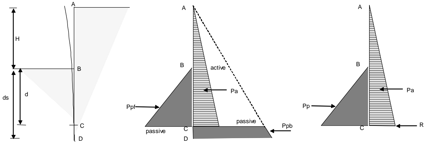
Figure 2.2 Simplified pressure diagram adapted from Whitlow (1990).
