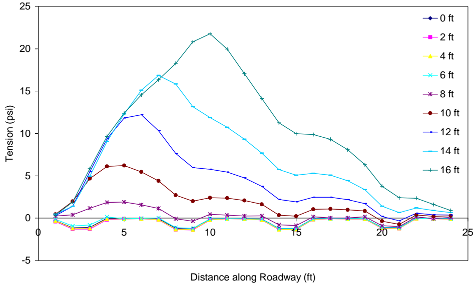
Figure C.36 Tension in the asphalt throughout excavation (PZ-27 wall in stronger soil with truck load) 10 ft from wall.
