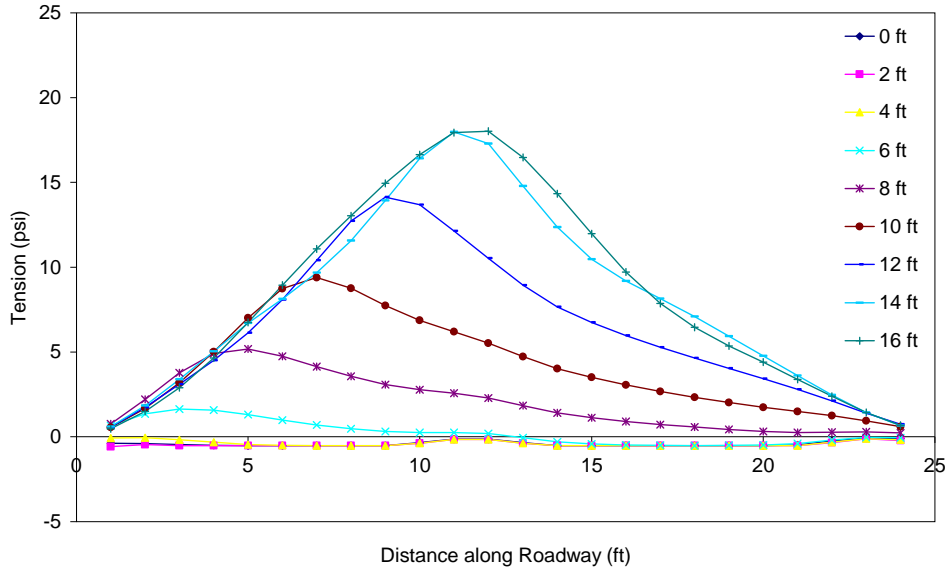
Figure C.27 Tension in the asphalt throughout excavation (PZ-27 wall in stronger soil with lane load) 5 ft from wall.
