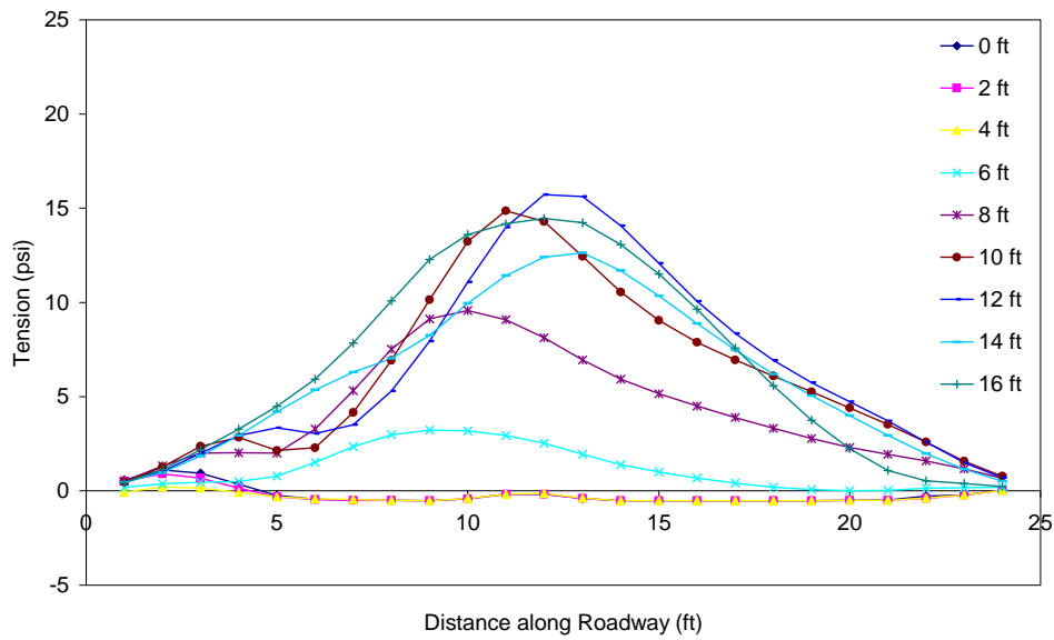
Figure C.13 Tension in the asphalt throughout excavation (PZ-40 wall in weaker soil with lane load) 0 ft from wall.
