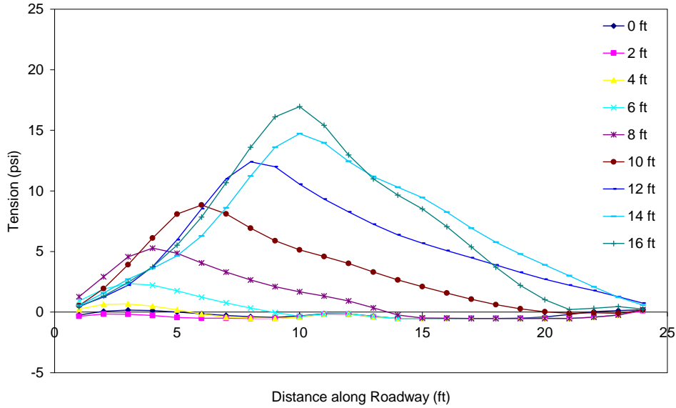
Figure C.15 Tension in the asphalt throughout excavation (PZ-40 wall in weaker soil with lane load) 5 ft from wall.
