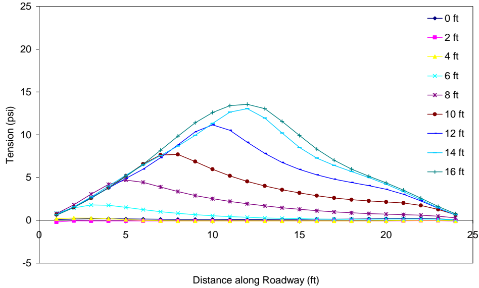
Figure C.31 Tension in the asphalt throughout excavation (PZ-27 wall in stronger soil with no load) 5 ft from wall.
