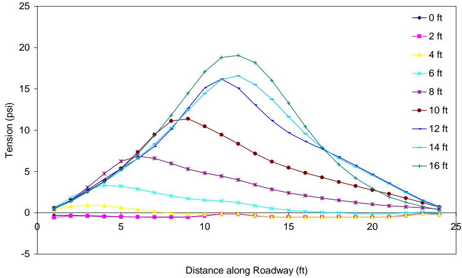
Figure C.26 Tension in the asphalt throughout excavation (PZ-27 wall in stronger soil with lane load) 2 ft from wall.
