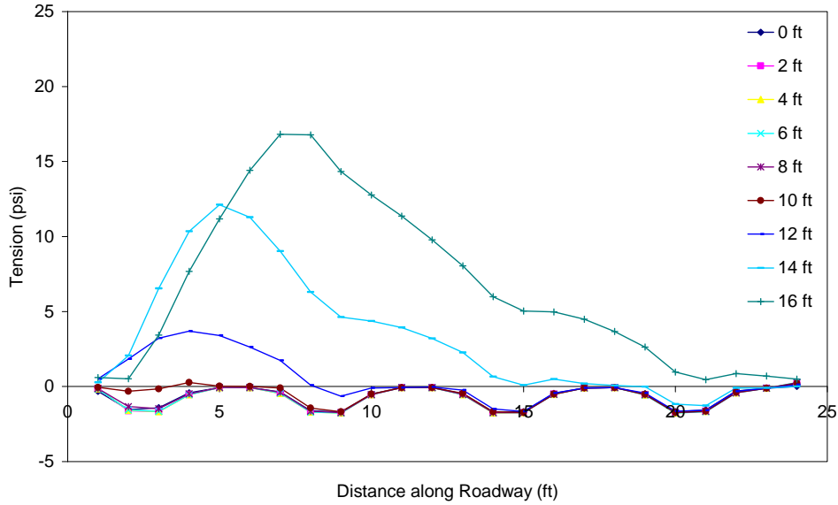
Figure C.24 Tension in the asphalt throughout excavation (PZ-40 wall in weaker soil with truck load) 10 ft from wall.
