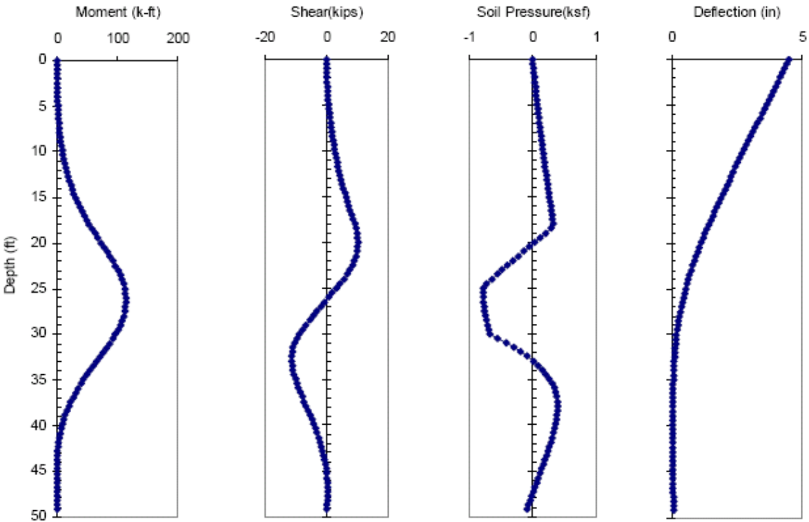
Figure 2.7 Output data from SPW2006 for same conditions shown in Figure 2.5 (top).
