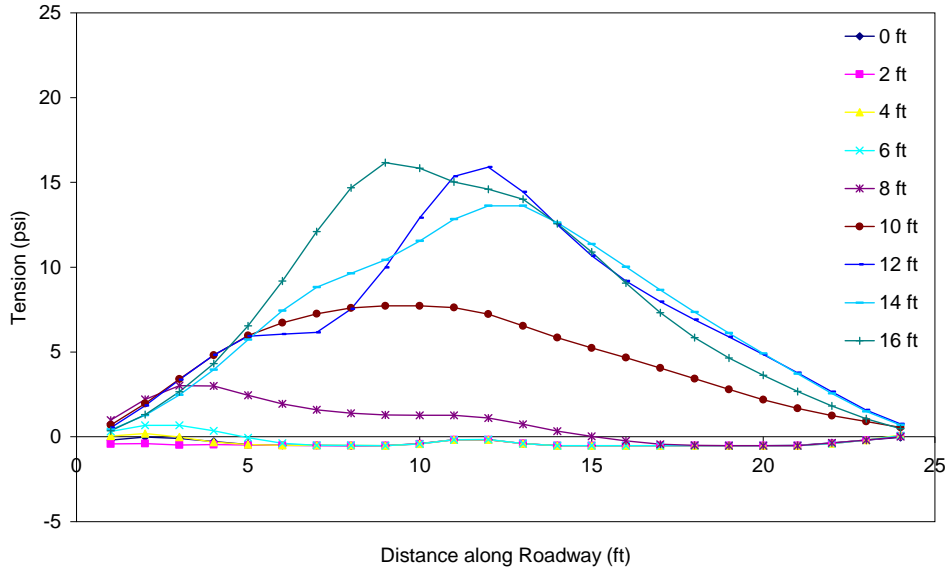
Figure C.3 Tension in the asphalt throughout excavation (PZ-27 wall in weaker soil with lane load) 5 ft from wall.
