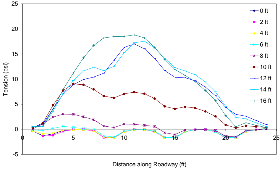
Figure C.11 Tension in the asphalt throughout excavation (PZ-27 wall in weaker soil with truck load) 5 ft from wall.
