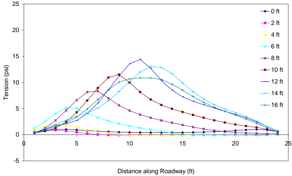
Figure C.18 Tension in the asphalt throughout excavation (PZ-40 wall in weaker soil with no load) 2 ft from wall.
