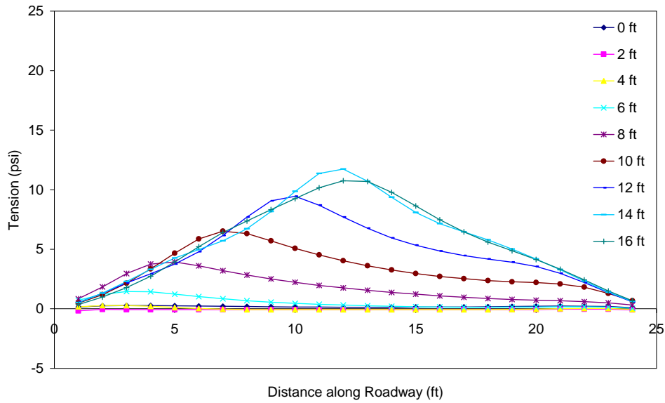
Figure C.43 Tension in the asphalt throughout excavation (PZ-40 wall in stronger soil with no load) 5 ft from wall.
