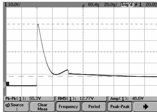
Figure 10. CITEL DS210-12VDC at 300A
