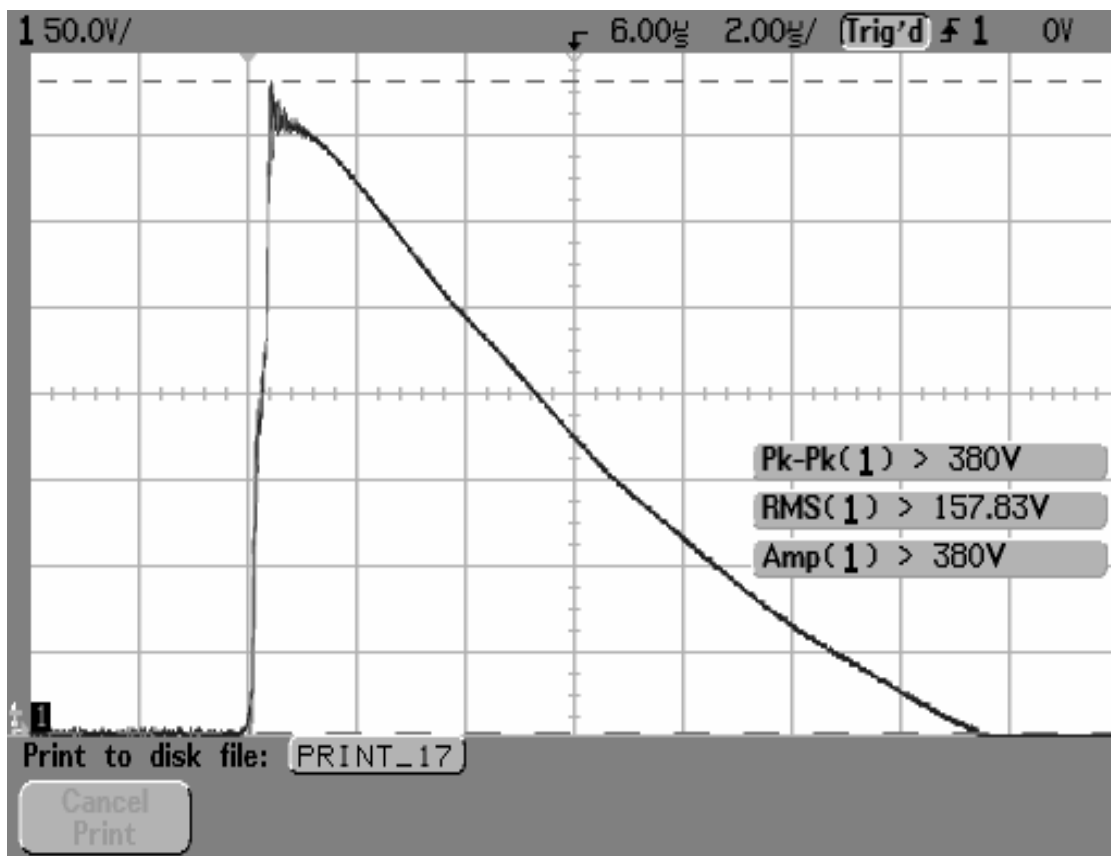
Figure 7. CITELE BP1-06 at 4000A
