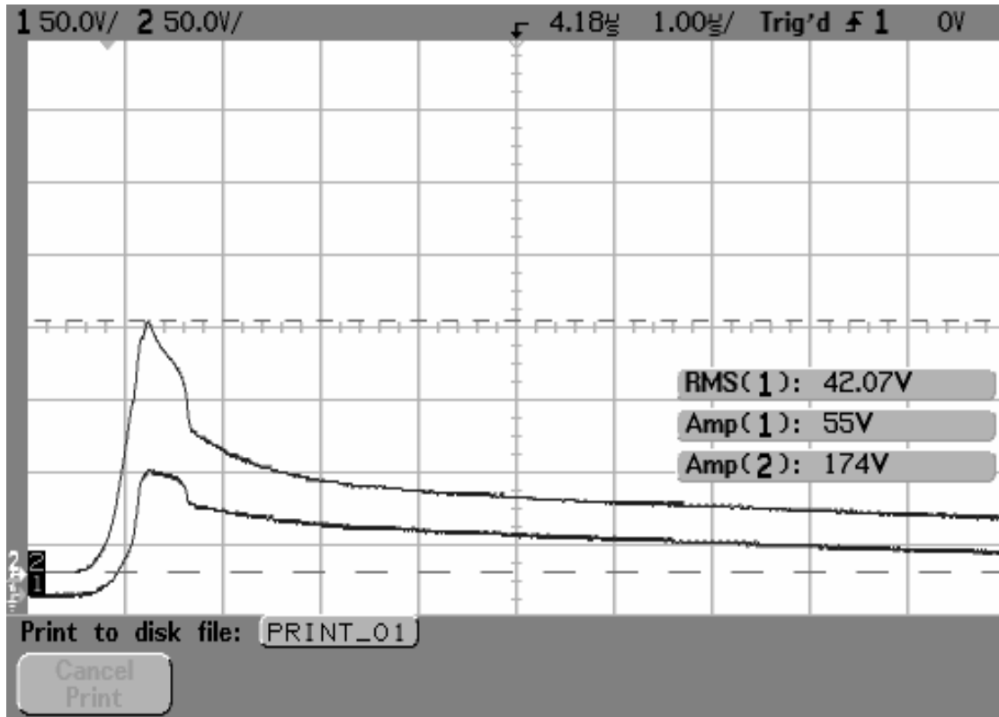
Figure 5: EDCO SRA6CLA-916 at 500A
