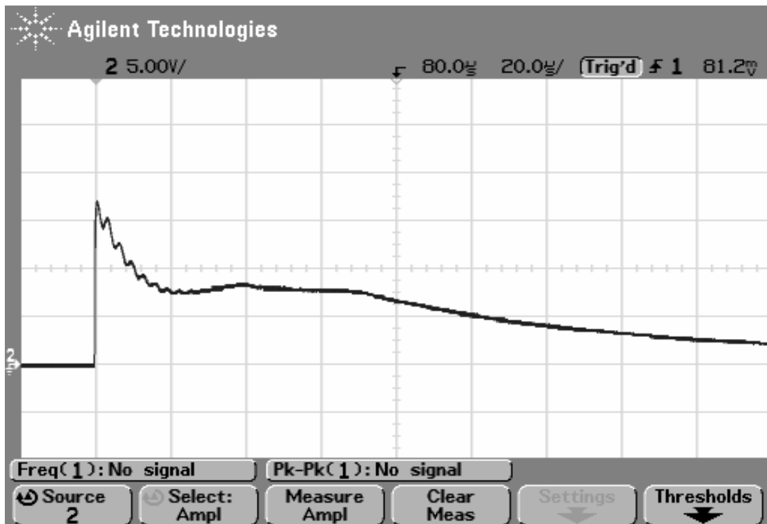
Figure 13. Atlantic Scientific 24516 output for 2000A input current
