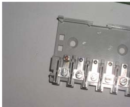
Figure 9. CITELE BP1-06 Endurance
