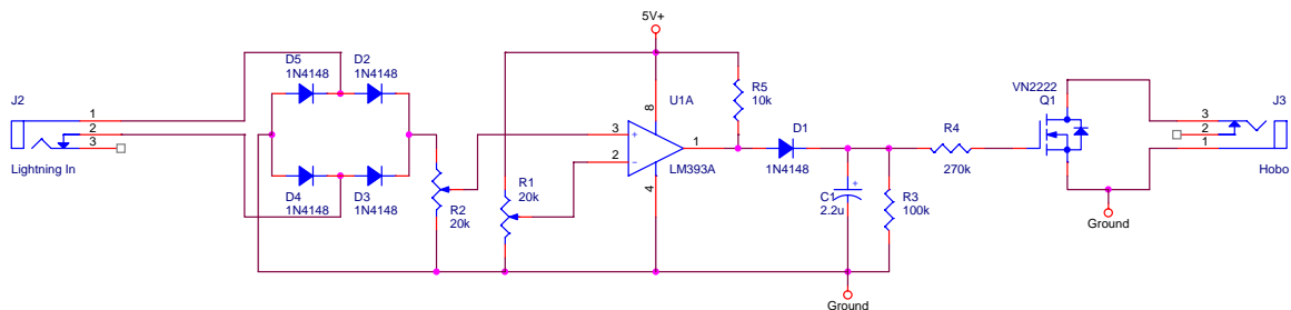
Figure 6. Interface Electronics for Low-Voltage Surge Counter
