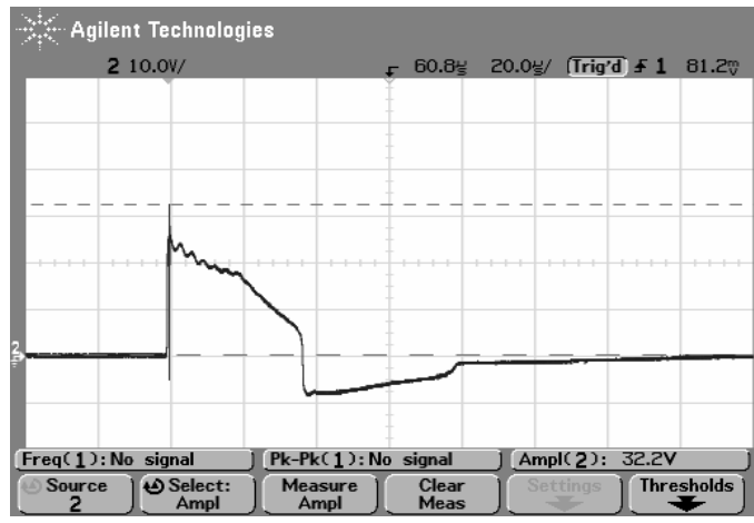
Atlantic Scientific 24538 Output for 2000A input current
