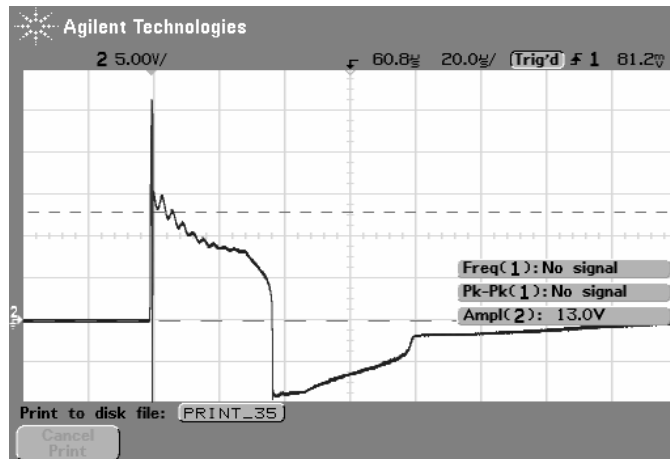
Atlantic Scientific 24528 Output for 2000A input current
