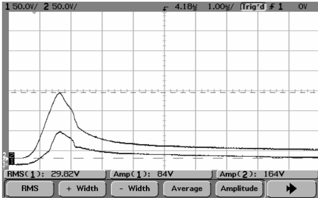
Figure 4. EDCO SRA6LCA-916 at 250A
