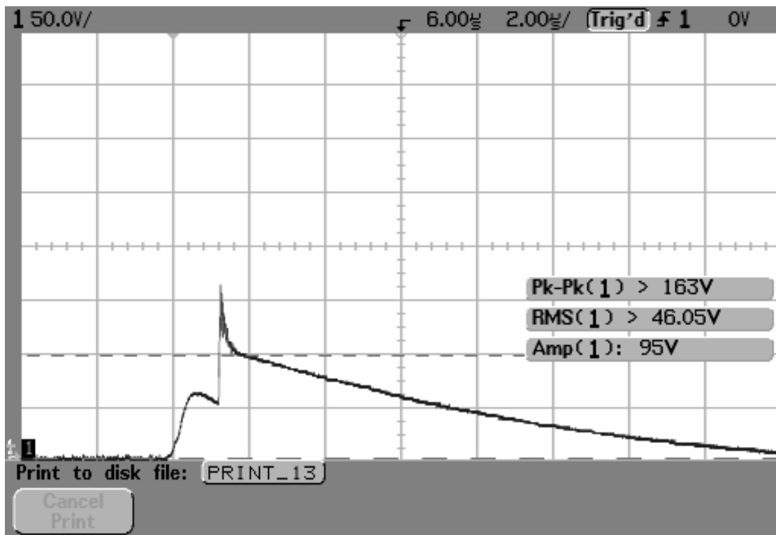
Figure 6. CITEL BP1-06 at 1000A
