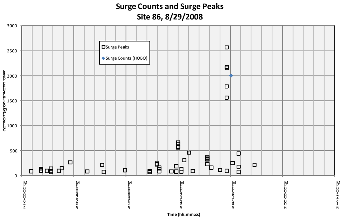
Figure 16. Comparison of Surge Peaks and Surge Counts for an Intense or Close Lightning Strike
