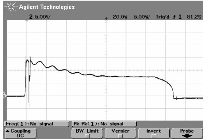
Atlantic Scientific 90489 Output for 2000A input current
