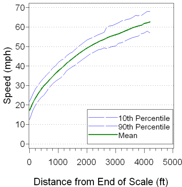
Figure 5-17: Average Speed Profile for Combined “Level” Data Set
