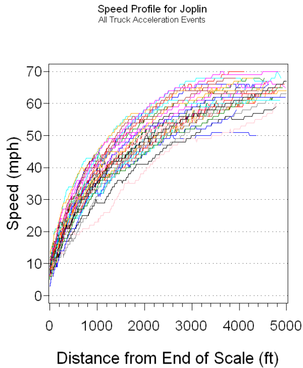
Figure 5-9: Initial Speed Profile for Joplin Data Collection Site
