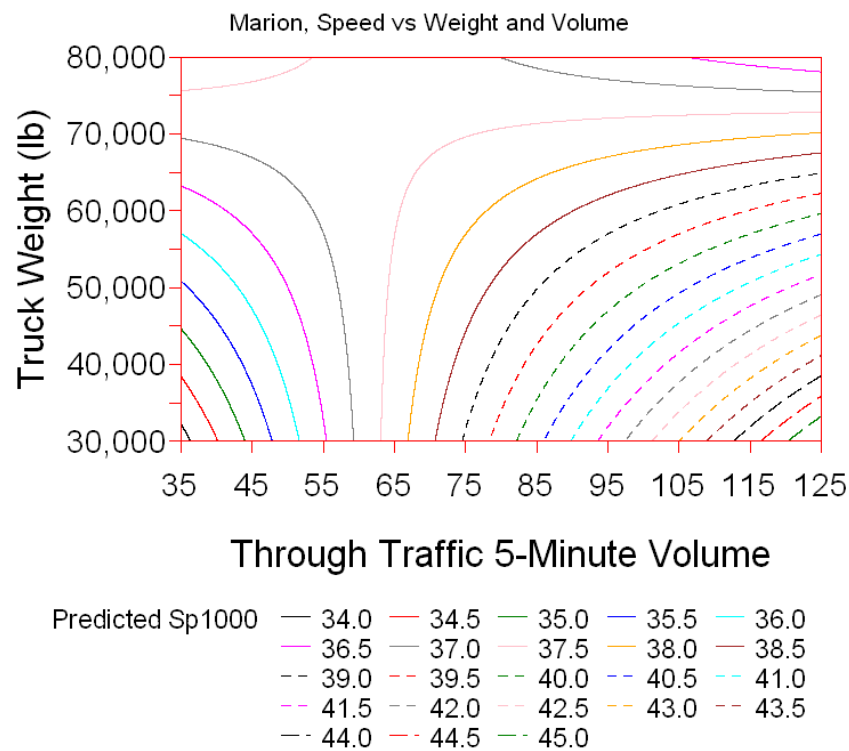
Figure 5-6: Contour Plot for Truck Speed at 1000 Feet at Marion Data Collection Site
