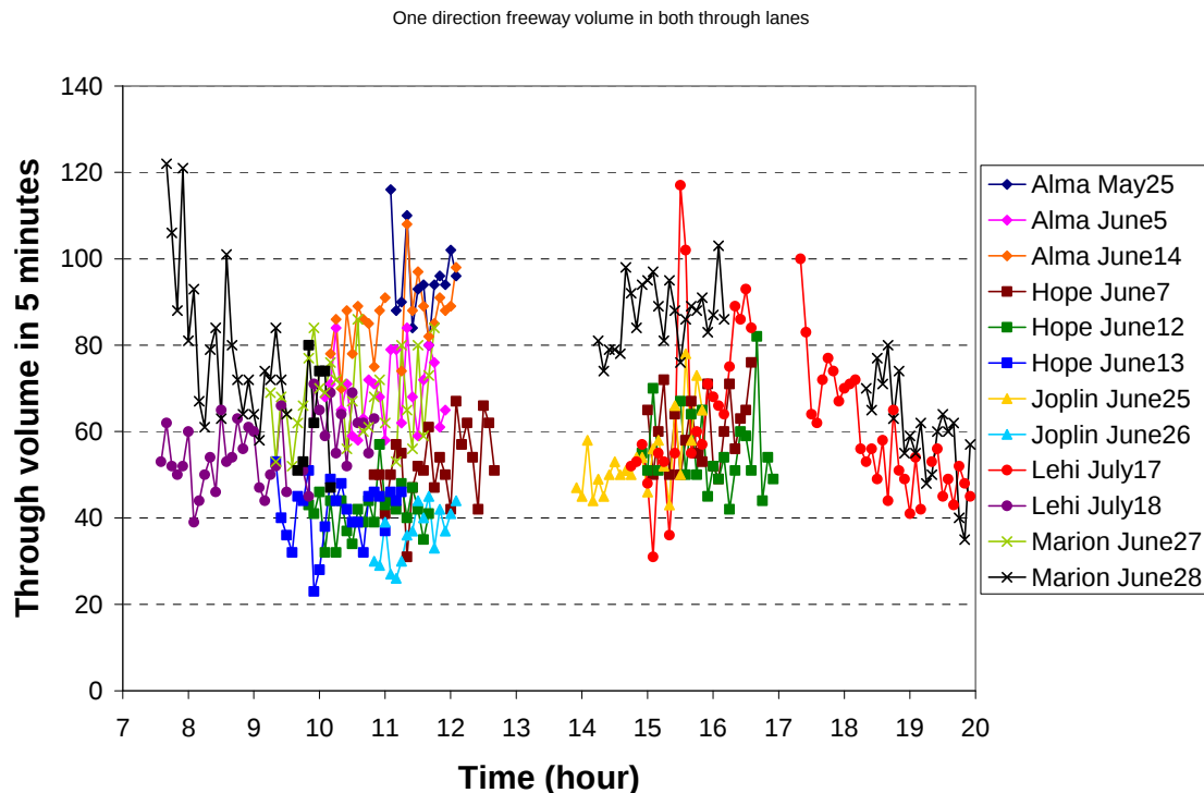
Figure 5-3: Five Minute Freeway Volumes during Data Collection
