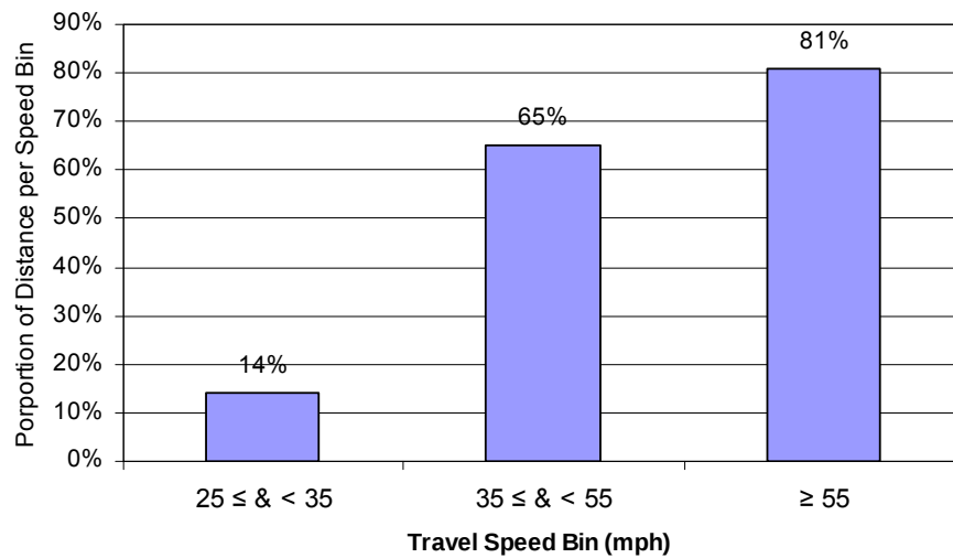
Figure 9. LDW availability by travel speed
