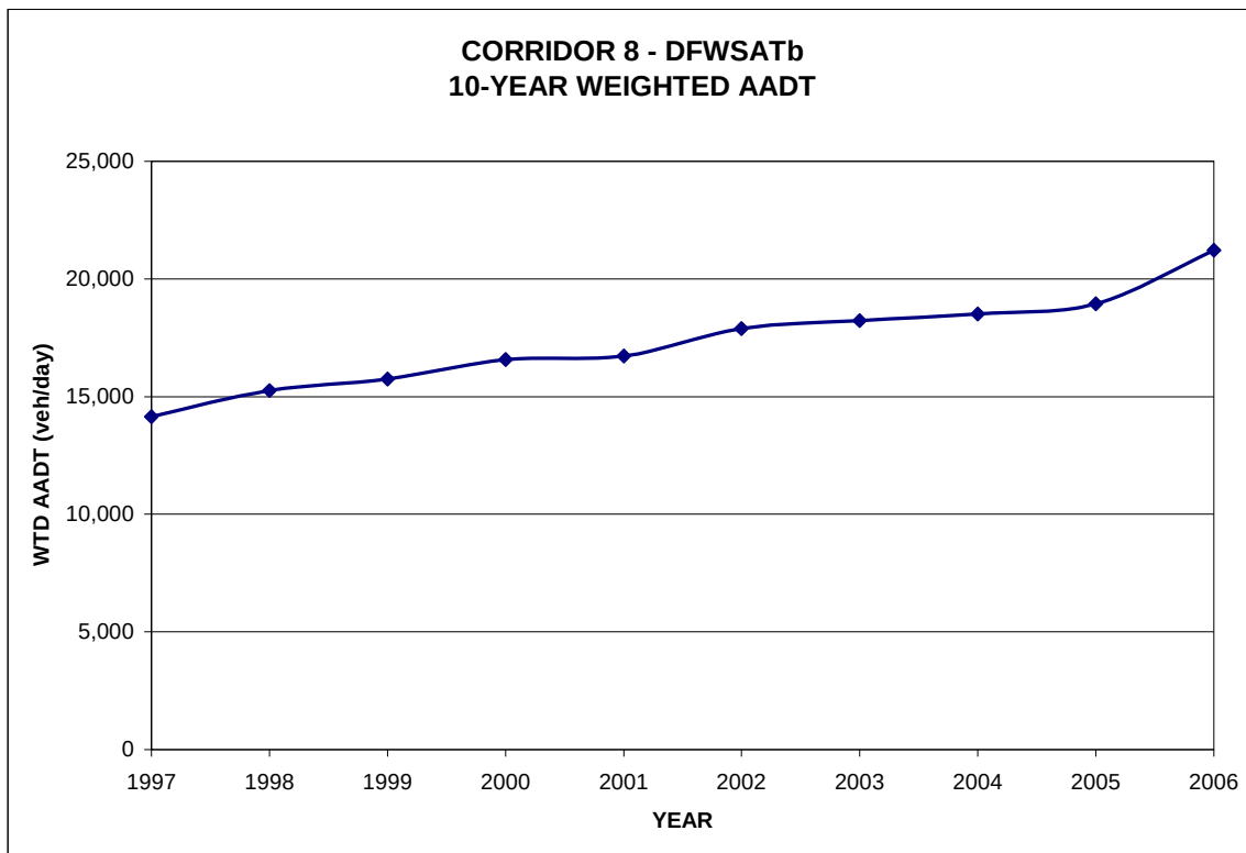
Figure 2-10. Corridor 8 – DFWSATb – 10-Year AADT.
