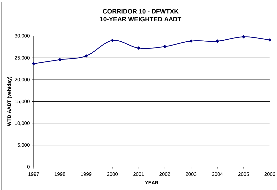
Figure 2-12. Corridor 10 – DFWTXK – 10-Year AADT.
