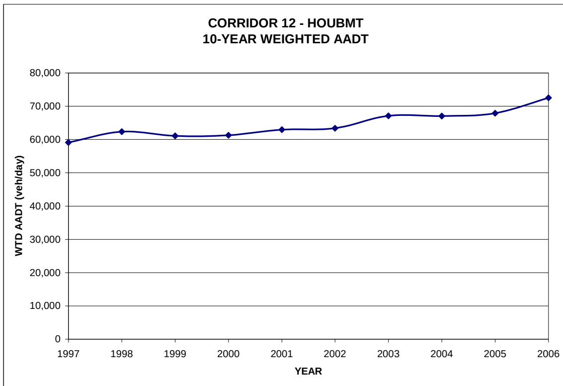
Figure 2-14. Corridor 12 – HOUBMT – 10-Year AADT.
