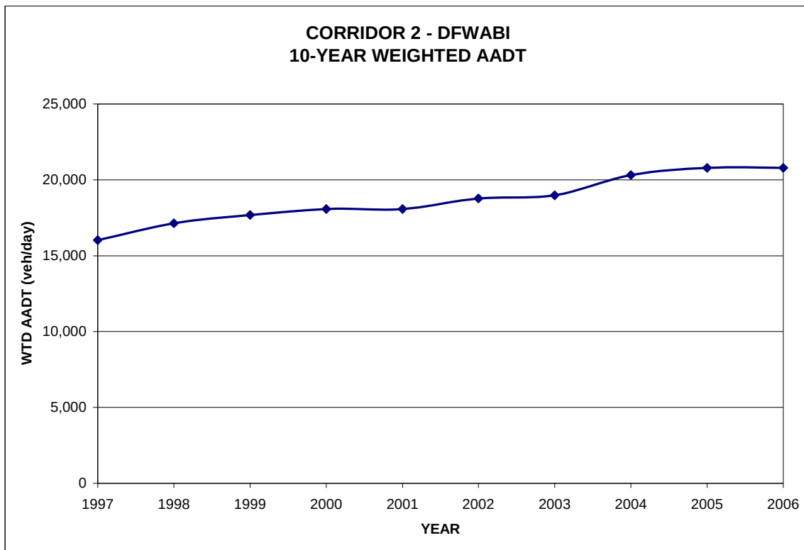
Figure 2-4. Corridor 2 – DFWABI – 10-Year AADT.
