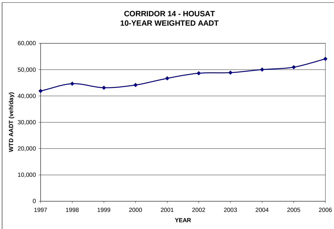
Figure 2-16. Corridor 14 – HOUSAT – 10-Year AADT.
