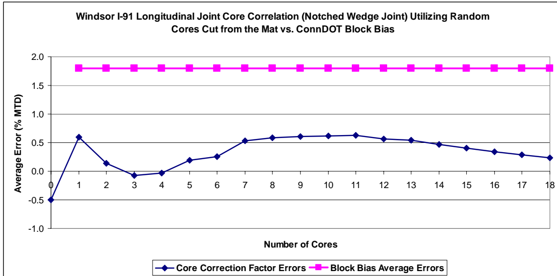
Figure 10 Comparison of Correction Factors for Use on Notched Wedge Joints
