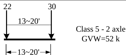
Fig. 4.8 Representative vehicle for Class 5 vehicles
