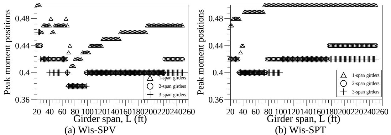
Fig. 6.7 Relative locations of peak moments in simply supported girders
