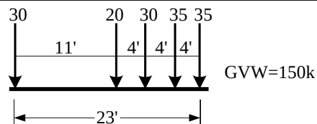
Fig. 6.3 The proposed 5-axle vehicle to supplement the Wis-SPV
