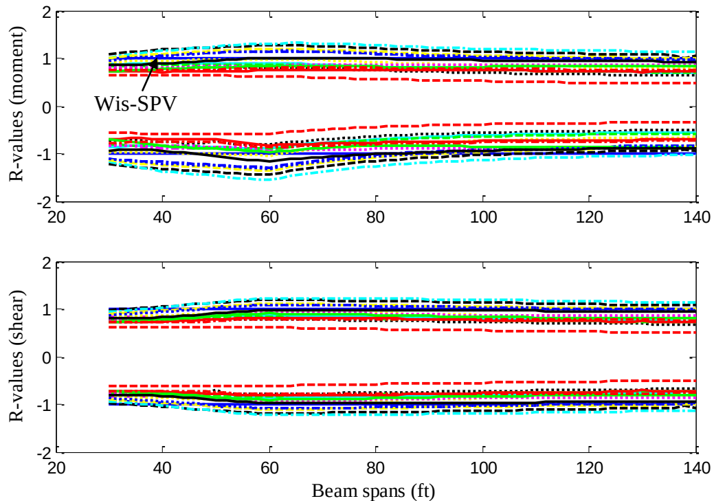
Fig. 5.21 R-values for representative permit vehicles on two-span girders
