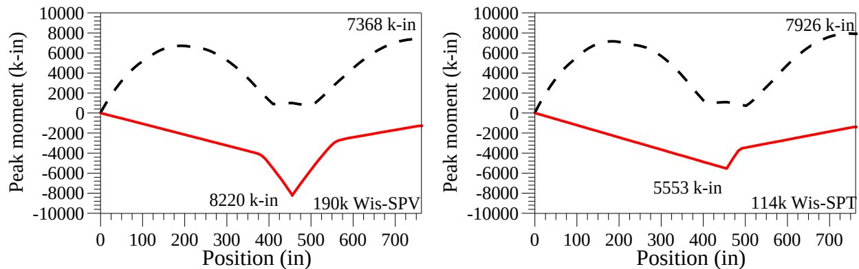
Fig. 6.23 Moment envelops of a 3-span slab bridge under permit vehicles
