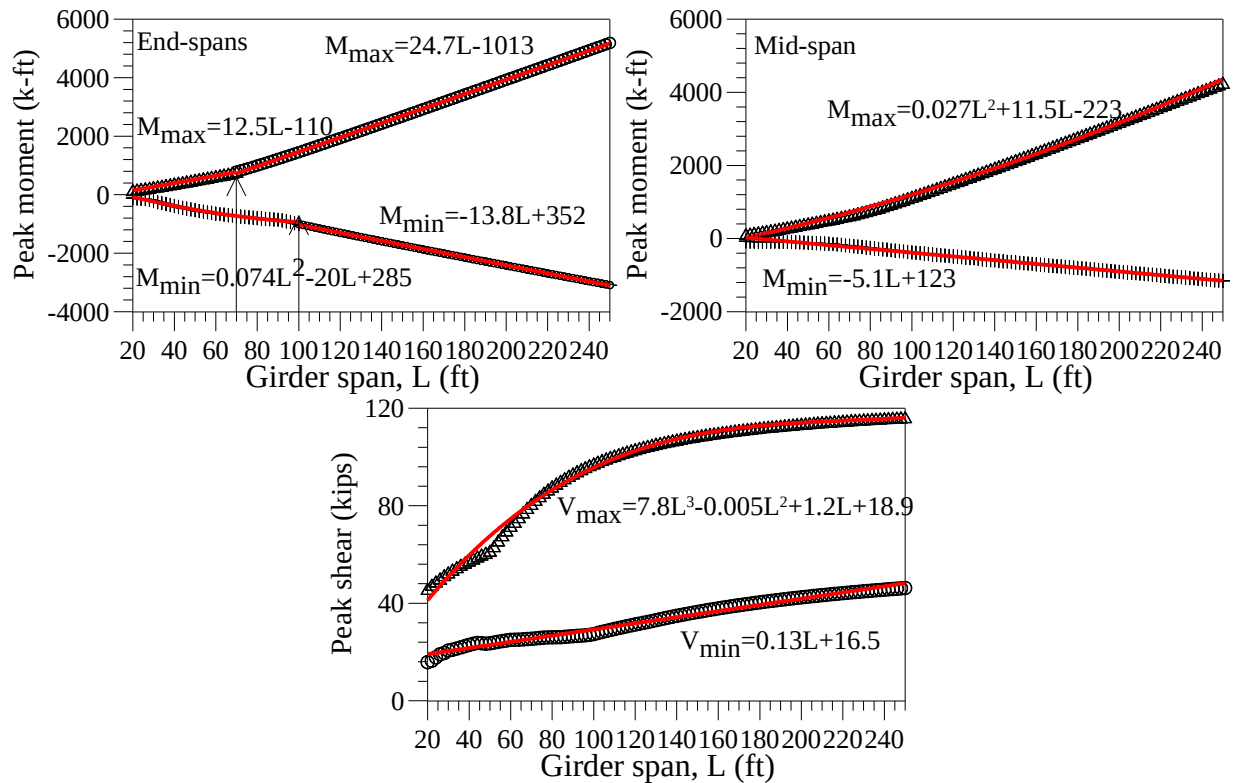
Fig. 6.19 Regression analysis of the peak responses under Wis-SPV in 3-span girders
