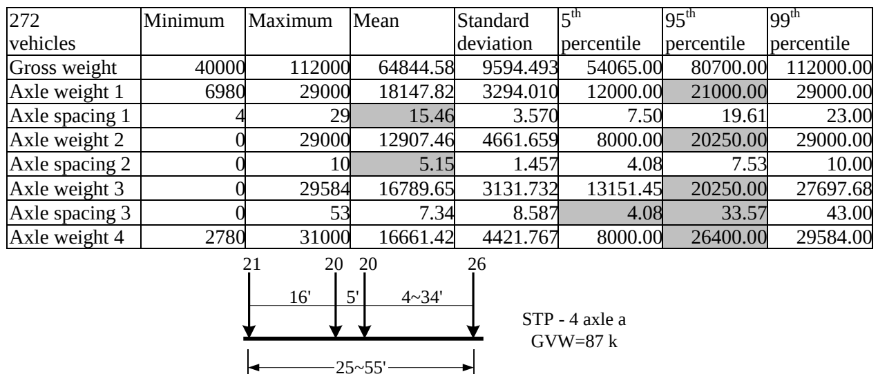
Fig. 5.3 Representative vehicle for 4-axle permit vehicles (Type 3S1)
