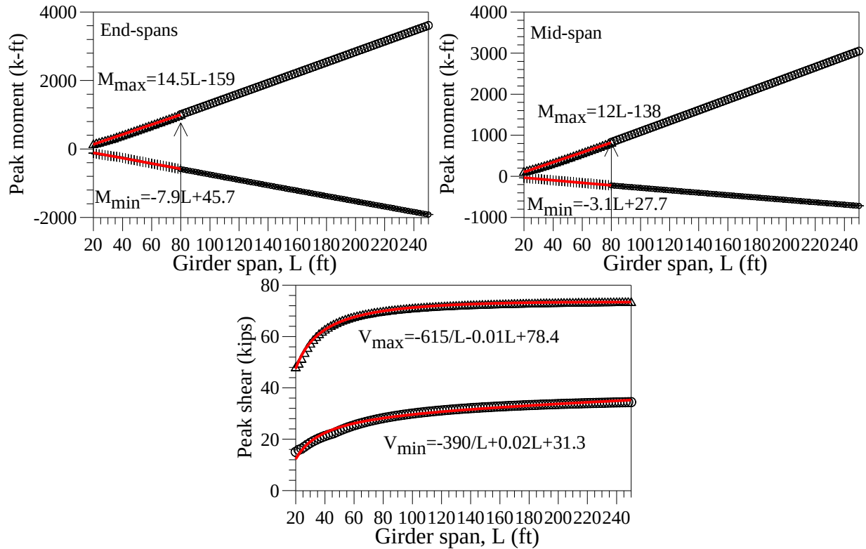
Fig. 6.21 Regression analysis of the peak responses under Wis-SPT in 3-span girders
