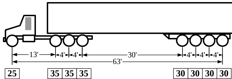
Fig. 1.2 Wisconsin Standard Permit Vehicle
