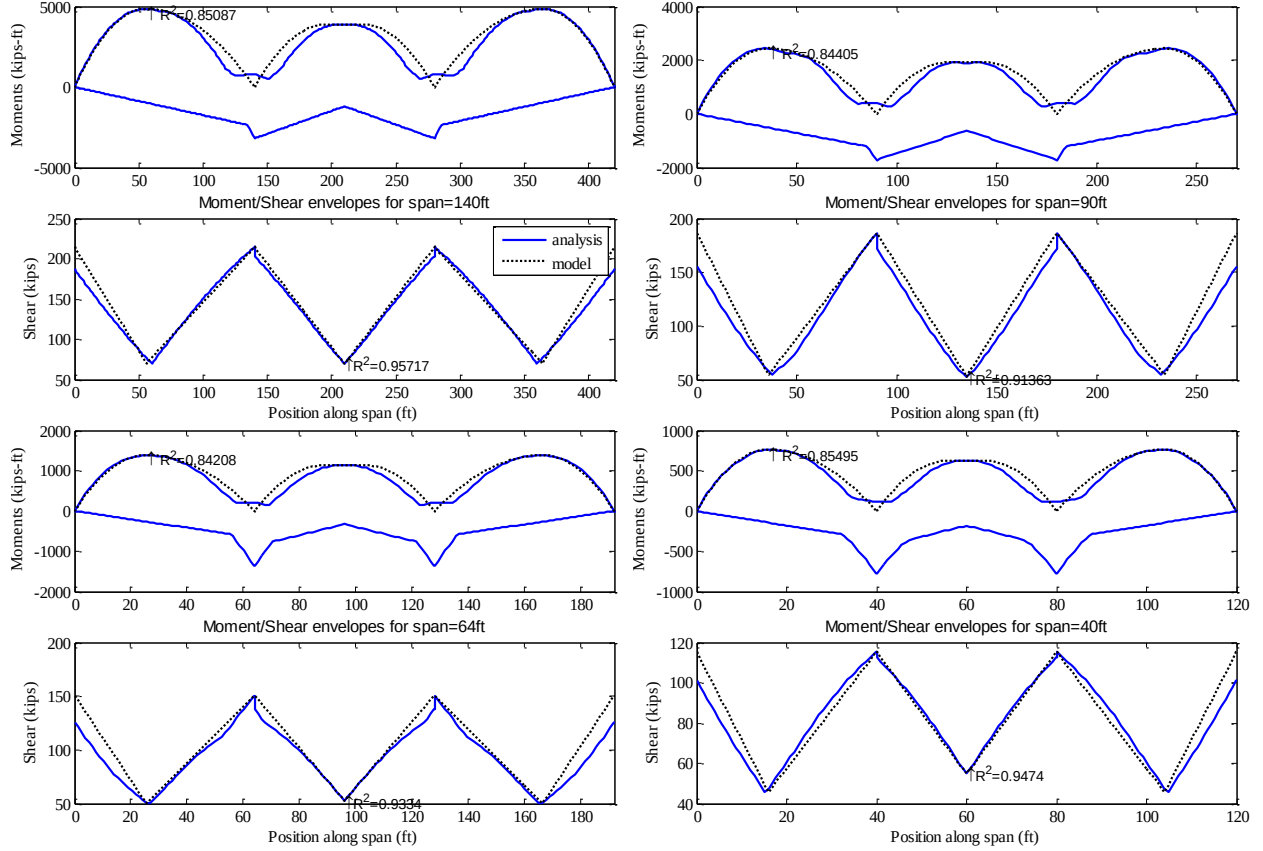
Fig. 6.20 Models of the peak responses under Wis-SPV in 3-span girders
