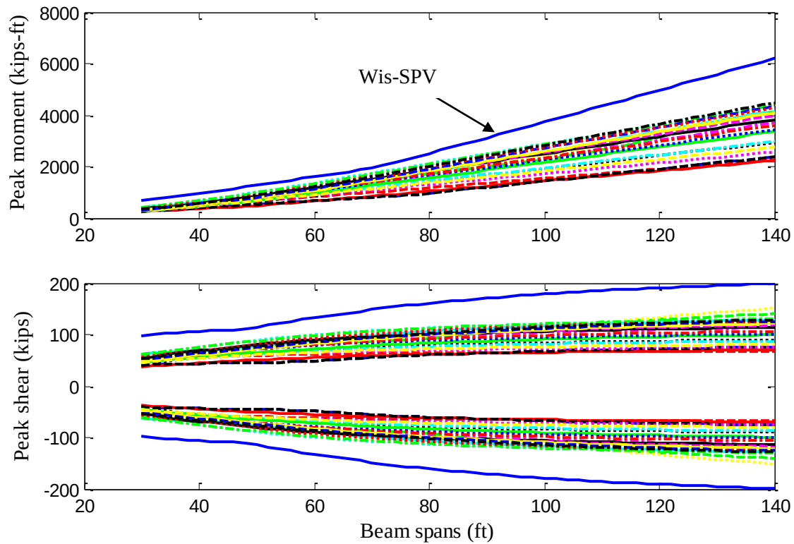
Fig. 3.4 Comparison of the maximum moments in simply-supported girders
