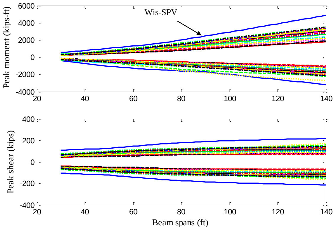
Fig. 3.8 Comparison of the peak moments in 3-span simply-supported girders
