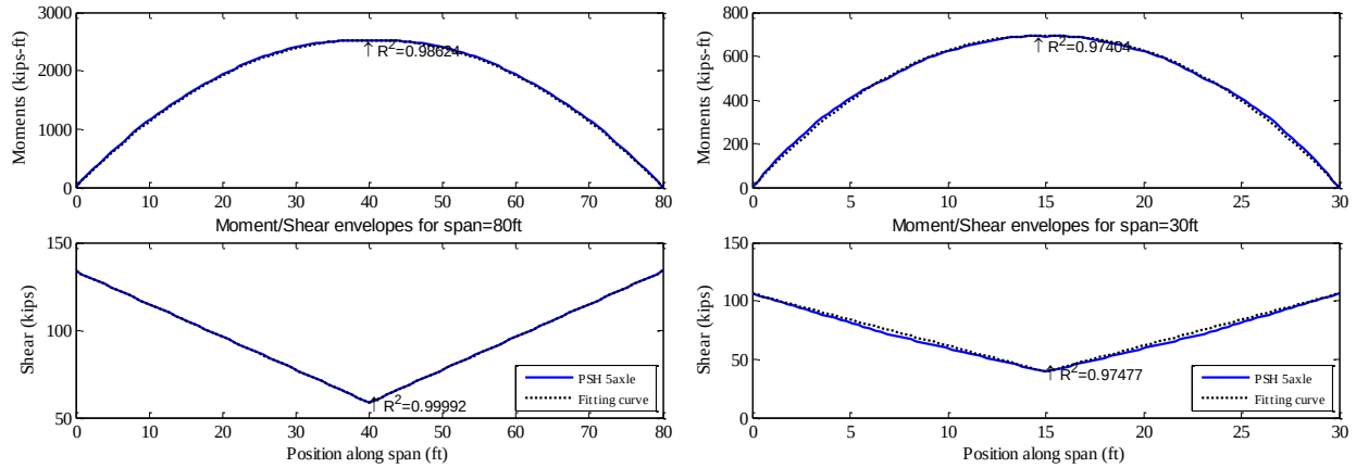
Fig. 6.12 Models of the peak responses under Wis-SPT in 1-span girders
