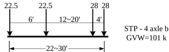
Fig. 5.4 Representative vehicle for 4-axle permit vehicles (Type 2S2)
