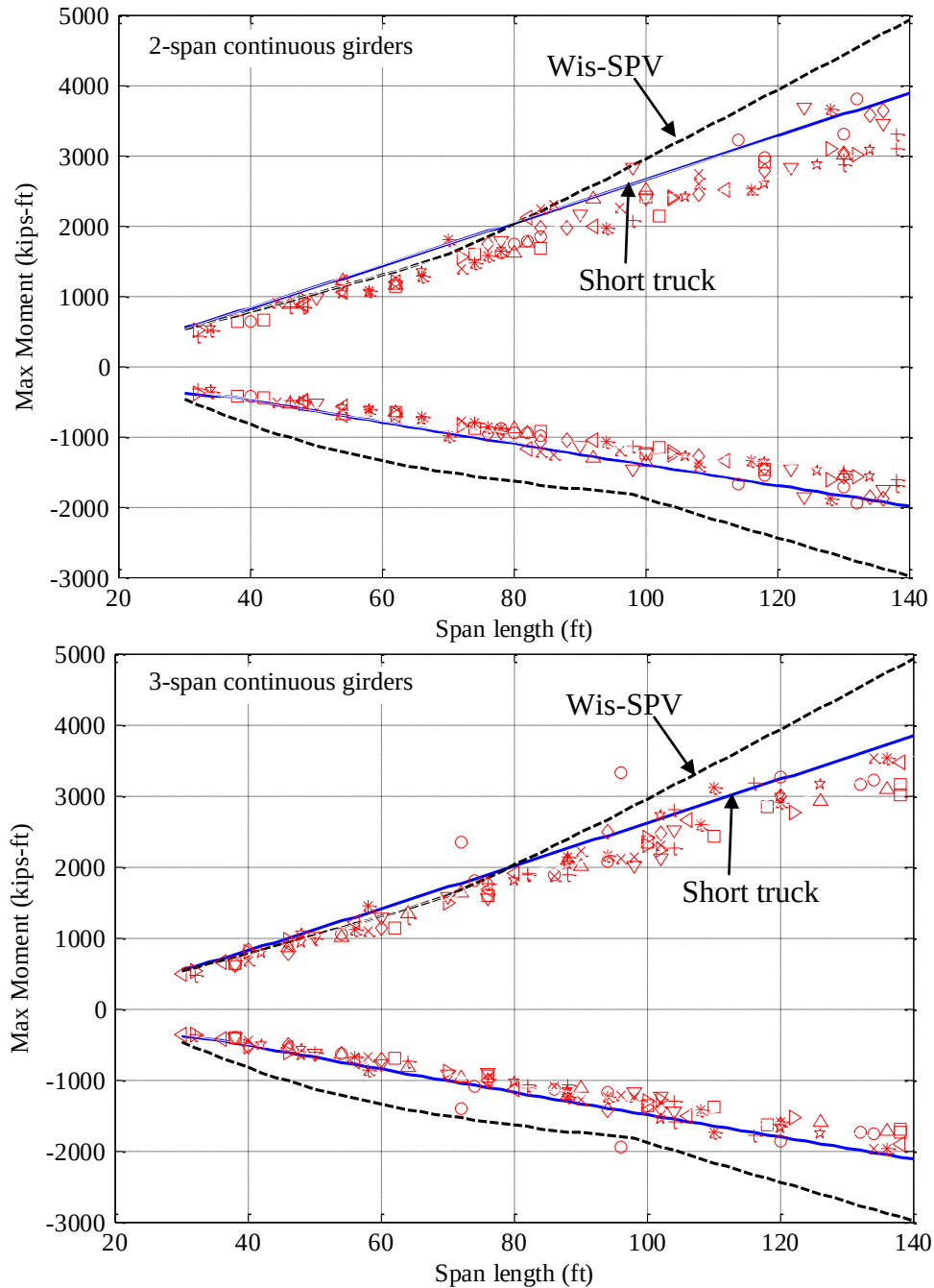
Fig. 6.5 Comparison of the proposed short truck with randomly selected 5-axle trucks
