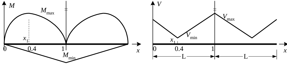
Fig. 6.13 Moment/shear envelope for one-span simply supported girders
