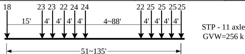
Fig. 5.15 Representative vehicle for 11-axle permit vehicles
