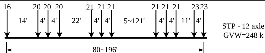
Fig. 5.16 Representative vehicle for 12-axle permit vehicles
