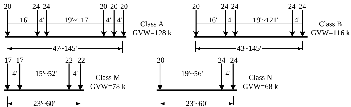
Fig. 2.6 Truck configurations for multi-trip permits in Illinois
