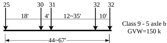
Fig. 4.14 Representative vehicle for Class 9 vehicles (Type 3S2 split)
