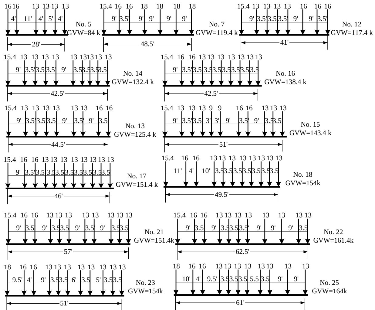
Fig. 2.4 Michigan Legal Vehicles with GVW larger than federal limit
