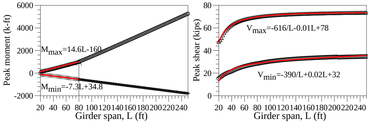
Fig. 6.16 Regression analysis of the peak responses under Wis-SPV in 2-span girders
