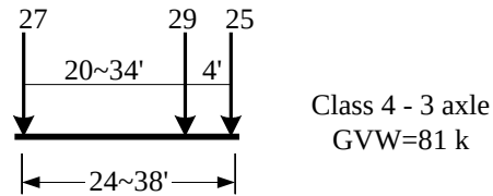
Fig. 4.5 Representative vehicle for Class 4 vehicles (3-axle)
