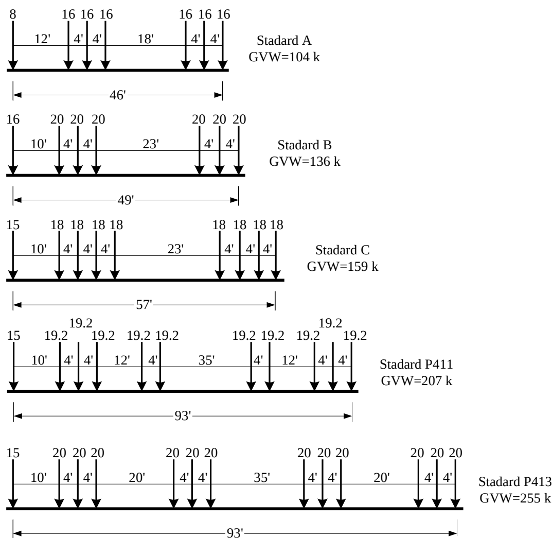
Fig. 2.2 Standard MnDOT Overload Permit Trucks
