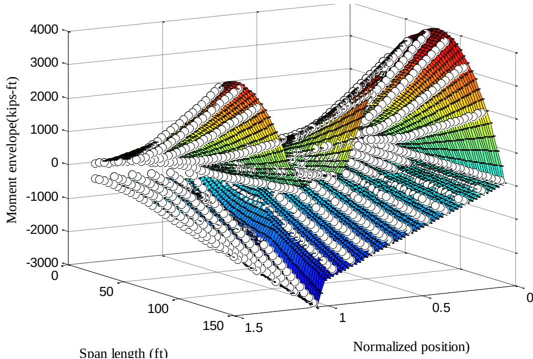
Fig. 3.3 Comparison of SAP2000 analysis results with WisDOT Bridge Manual (three-span)
