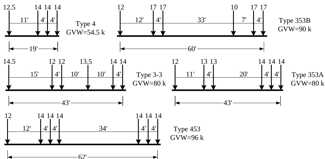
Fig. 2.3 Iowa rating vehicles
