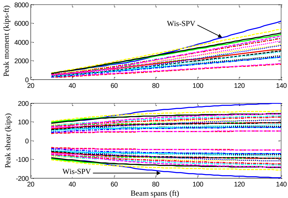
Fig. 4.24 Peak moment/shear values for overweight vehicles on one-span girders
