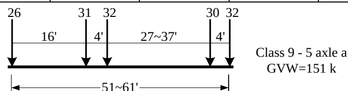
Fig. 4.15 Representative vehicle for Class 9 vehicles (Type 3S2)
