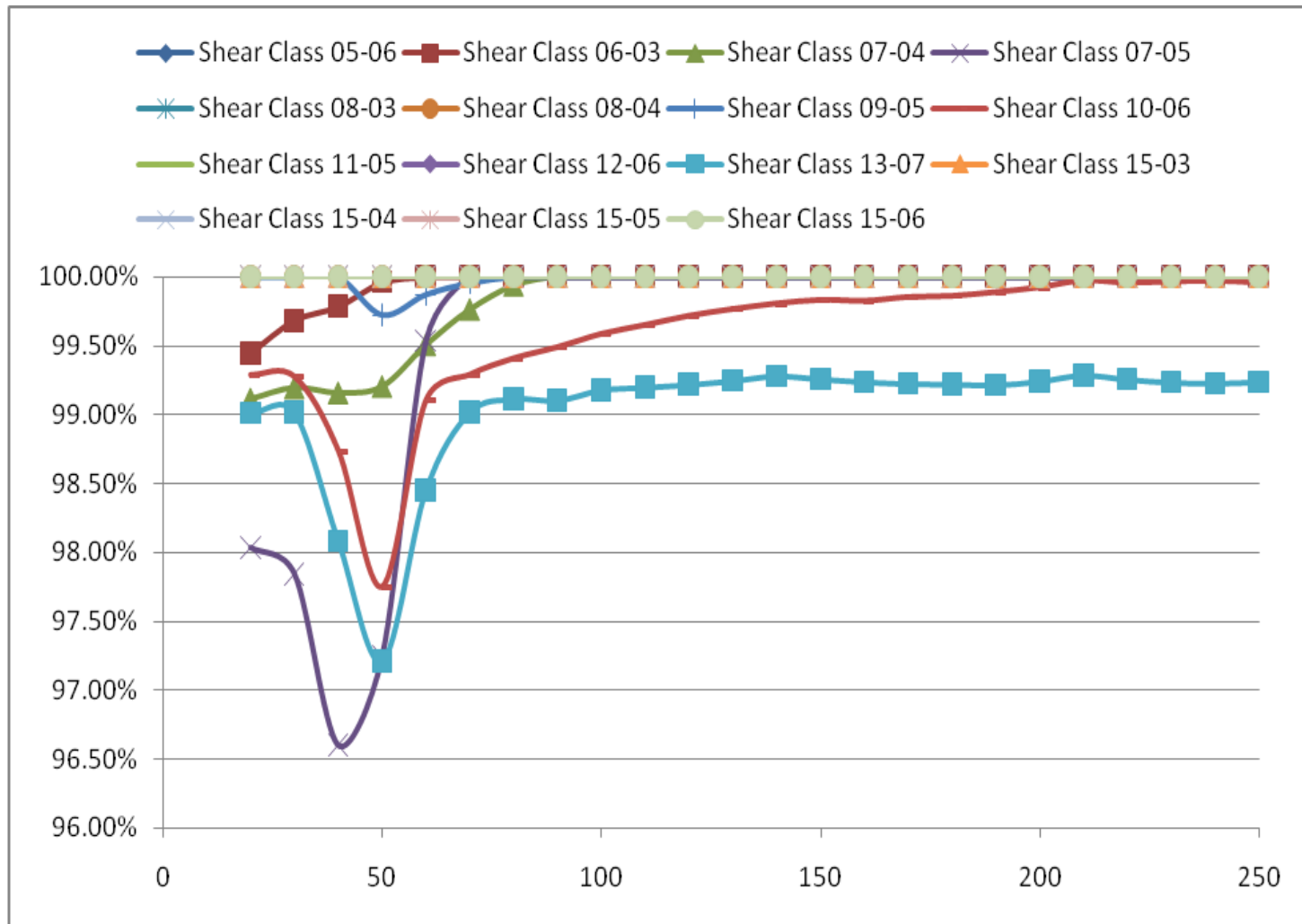
Fig. A4.7. Plot of 250-WPV shear as percentile of H5P data versus span length (ft) for each truck class-axle group.
