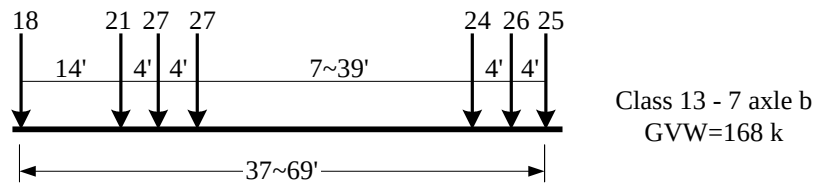
Fig. 4.22 Representative vehicle for Class 13 vehicles
