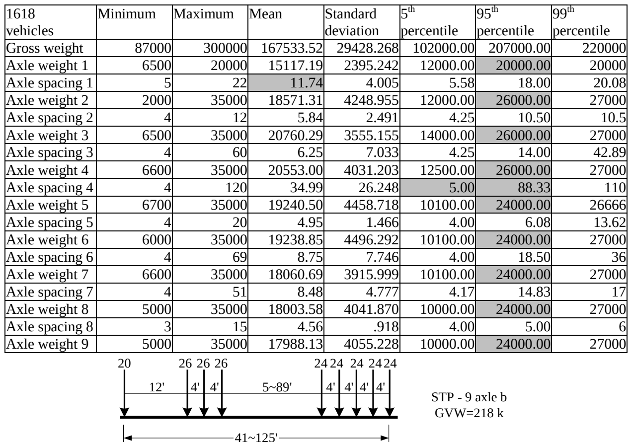
Fig. 5.12 Representative vehicle for 9-axle permit vehicles (Type b)
