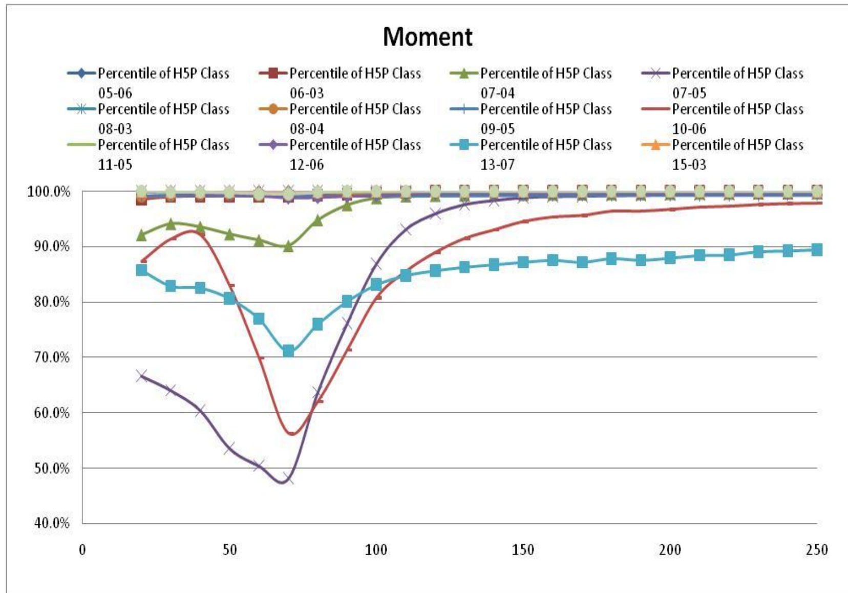
Fig. A4.8. Plot of 190-WPV moments as percentile of H5P data versus span length (ft) for each truck class-axle group.
