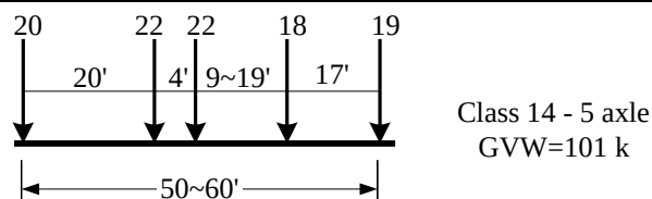
Fig. 4.23 Representative vehicle for Class 14 vehicles
