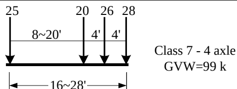
Fig. 4.10 Representative vehicle for Class 7 vehicles (4-axle)
