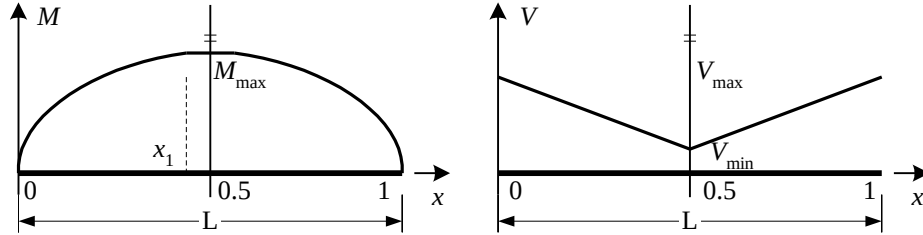
Fig. 6.8 Moment/shear envelope for one-span simply supported girders
