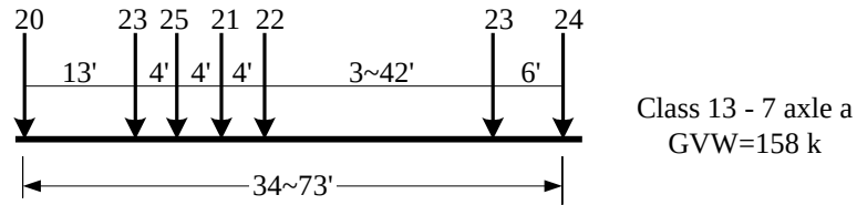
Fig. 4.21 Representative vehicle for Class 13 vehicles
