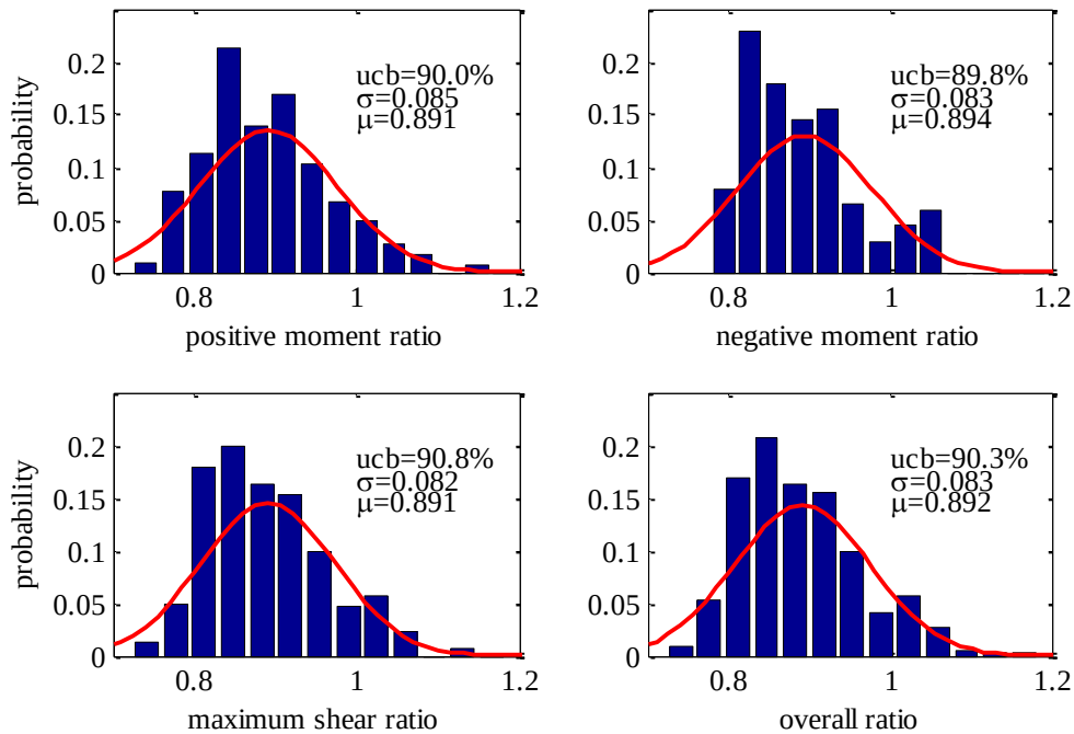
Fig. 6.6 Statistical analysis of randomly selected 5-axle trucks
