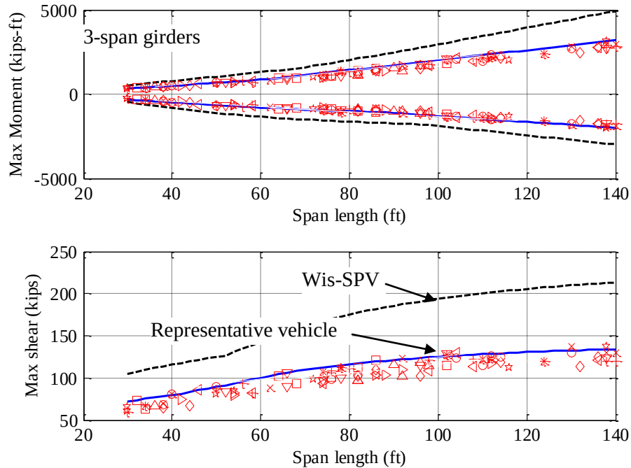
Fig. 4.29 Comparison of randomly selected vehicles with the representative vehicle (Type 3S2)
