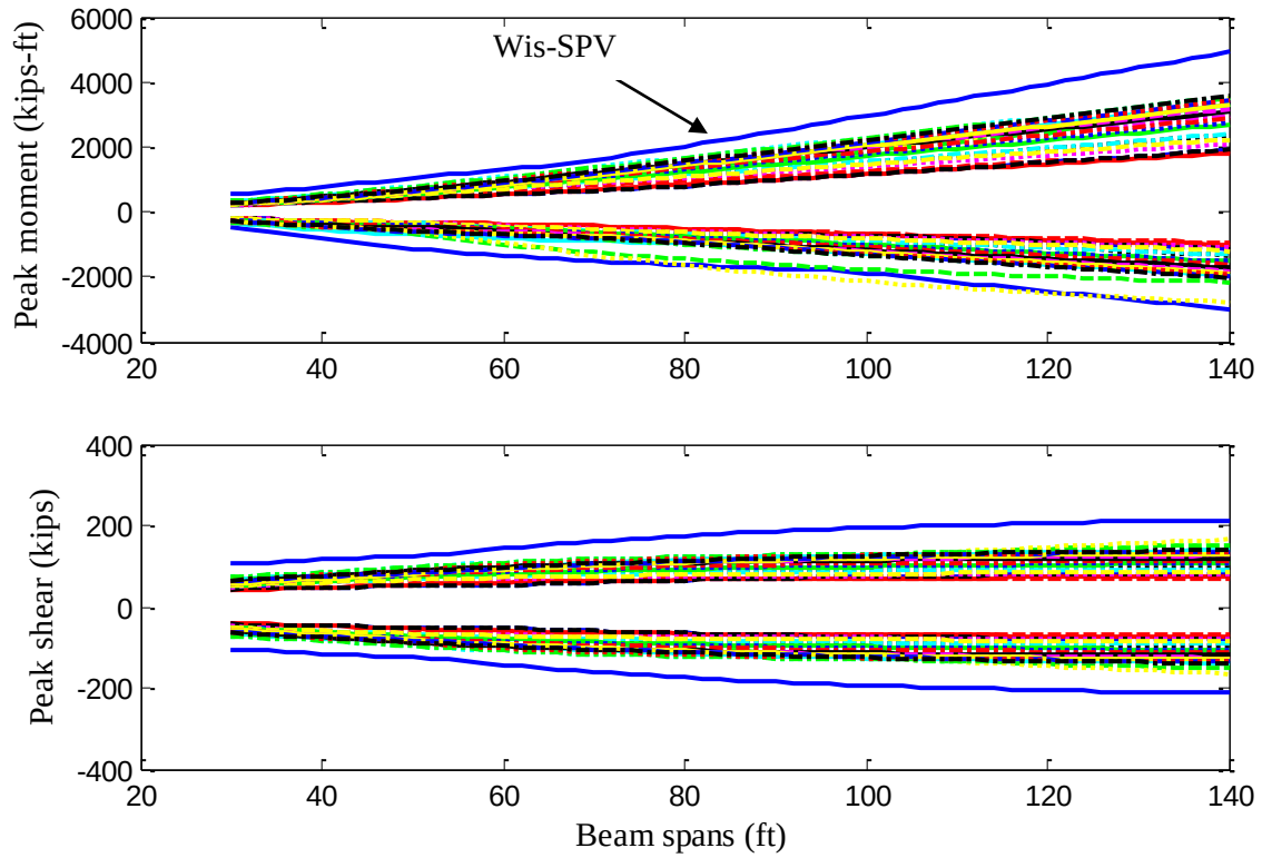
Fig. 3.6 Comparison of the peak moments in 2-span simply-supported girders
