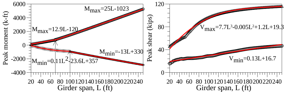
Fig. 6.14 Regression analysis of the peak responses under Wis-SPV in 2-span girders
