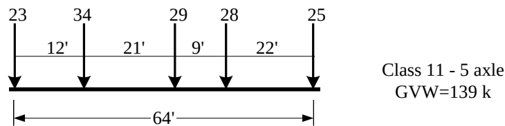
Fig. 4.19 Representative vehicle for Class 11 vehicles
