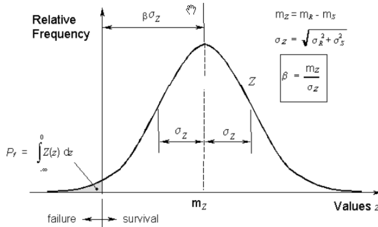
Fig. A3.2 Structural safety in LRFD structural design
