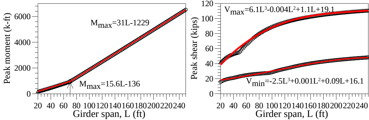
Fig. 6.9 Regression analysis of the peak responses under Wis-SPV in 1-span girders
