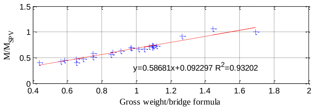
Fig. 3.13 Maximum moment distribution in 3-span girders
