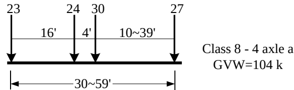
Fig. 4.13 Representative vehicle for Class 8 vehicles (Type 3S1)
