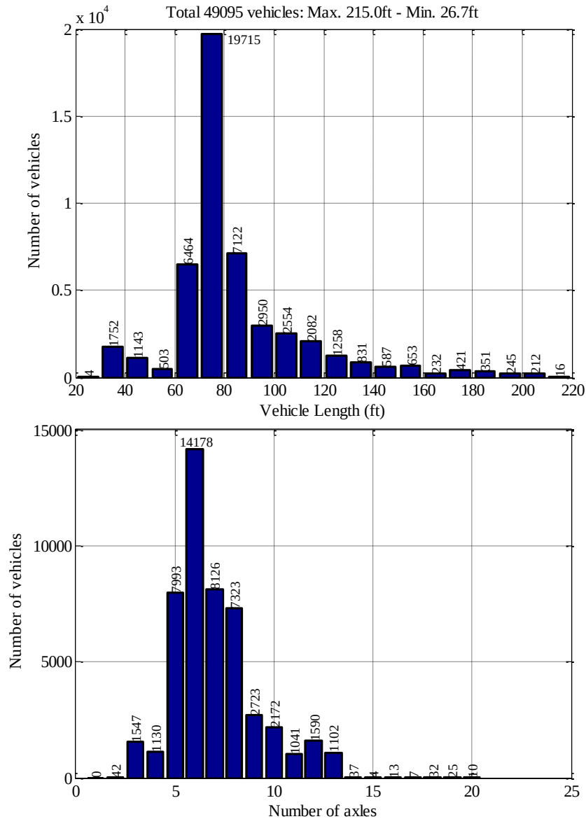
Fig. 5.1 Overview of vehicles with single-trip permits
