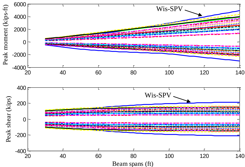
Fig. 4.26 Peak moment/shear values for overweight vehicles on two-span girders
