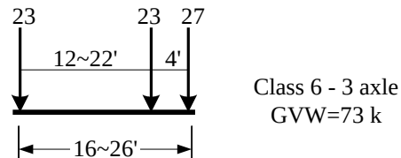
Fig. 4.9 Representative vehicle for Class 6 vehicles
