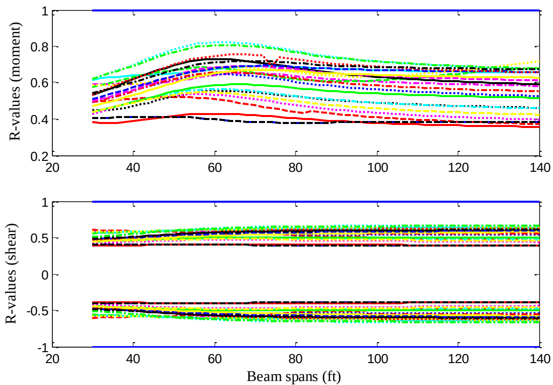
Fig. 3.5 R-values for the moment/shear envelopes in simply-supported girders
