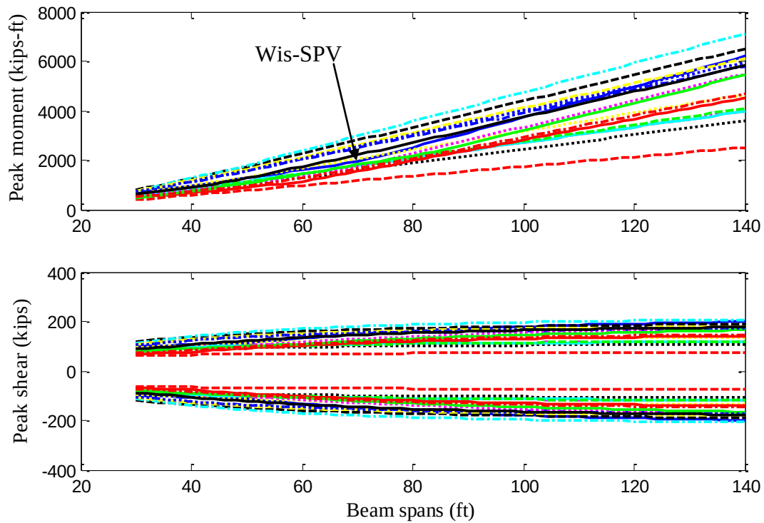
Fig. 5.18 Peak moment/shear values for representative permit vehicles on one-span girders
