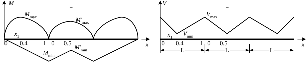
Fig. 6.18 Moment/shear envelope for one-span simply supported girders
