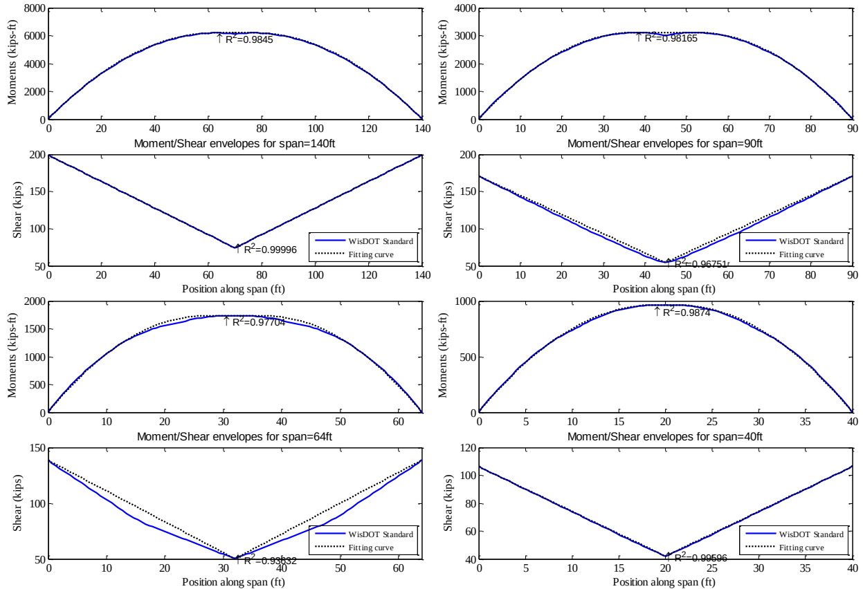
Fig. 6.10 Models of the peak responses under Wis-SPV in 1-span girders
