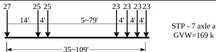
Fig. 5.8 Representative vehicle for 7-axle permit vehicles
