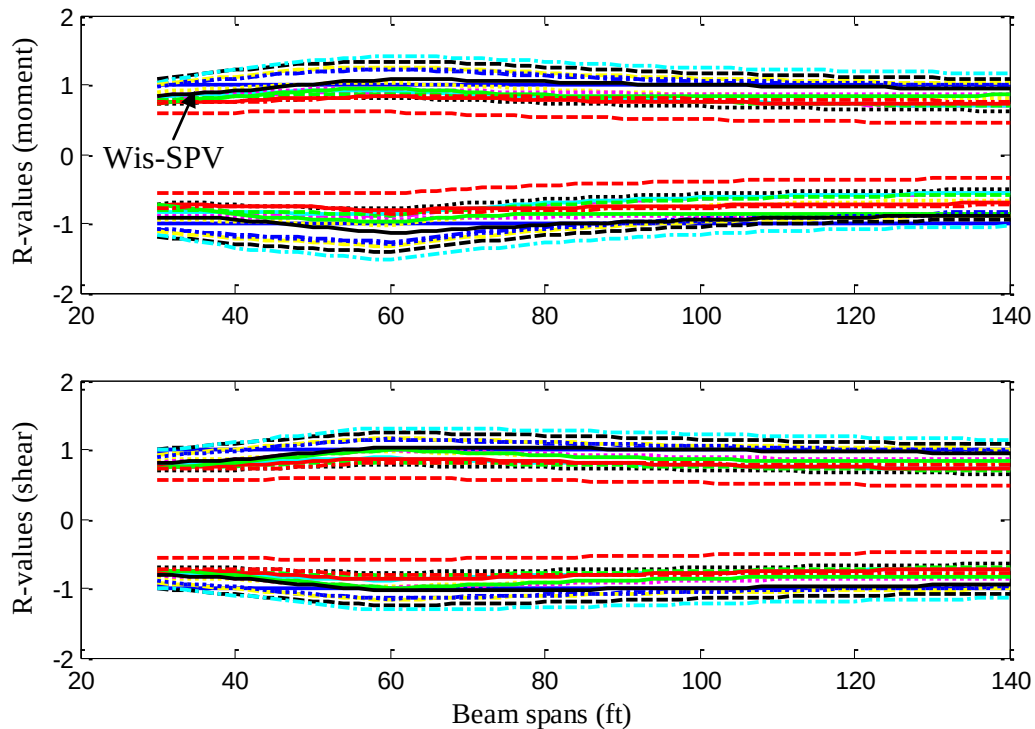
Fig. 5.23 R-values for representative permit vehicles on three-span girders
