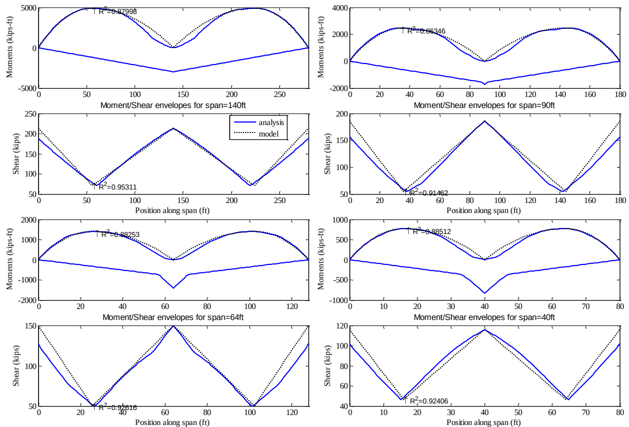
Fig. 6.15 Models of the peak responses under Wis-SPV in 2-span girders
