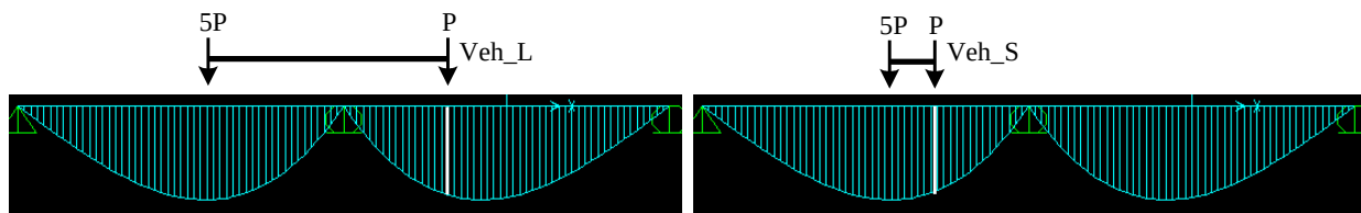
Fig. 6.1 Demonstration of short vehicles causing the worst negative moments
