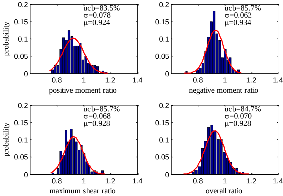
Fig. 4.30 Statistical evaluation of the representative vehicle for Class 9 (Type 3S2)
