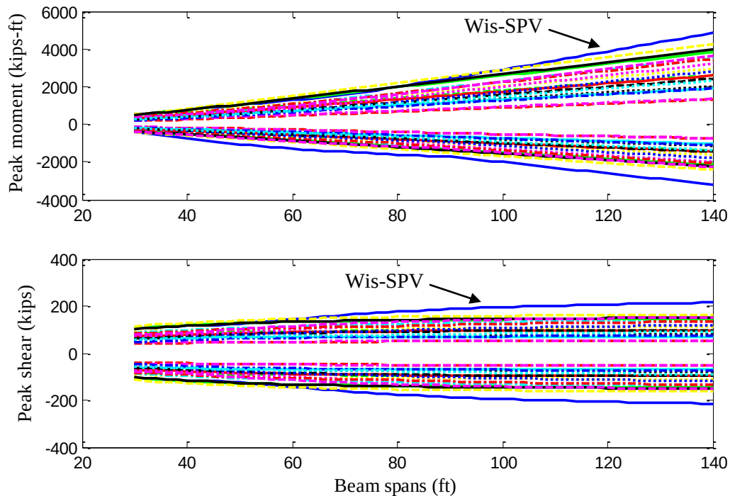
Fig. 4.27 Peak moment/shear values for overweight vehicles on three-span girders
