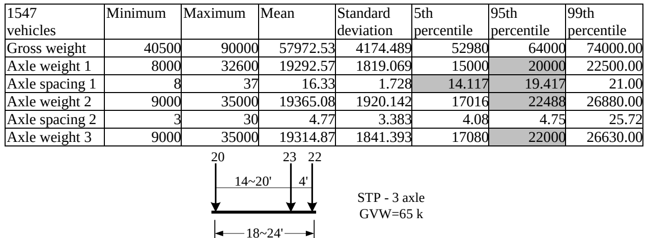
Fig. 5.2 Representative vehicle for 3-axle permit vehicles
