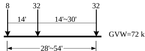
Fig. 2.1 Design truck in AASHTO LRFD and WisDOT Bridge Manual
