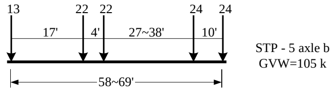
Fig. 5.6 Representative vehicle for 5-axle permit vehicles (Type 3S2 split)
