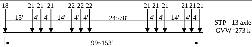
Fig. 5.17 Representative vehicle for 13-axle permit vehicles
