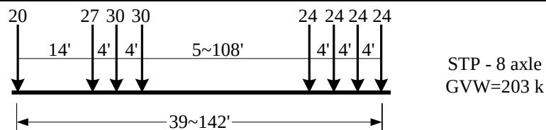
Fig. 5.10 Representative vehicle for 8-axle permit vehicles
