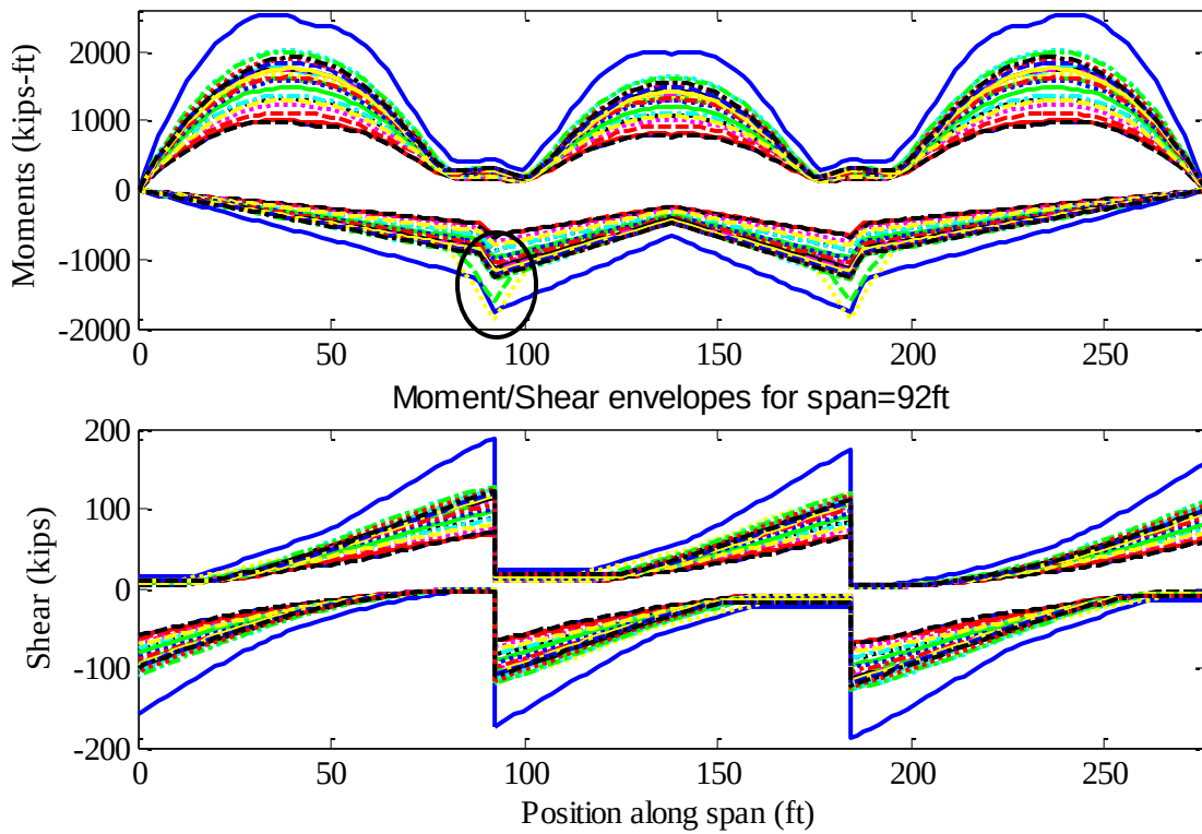
Fig. 3.10 Demonstration of breaching peak negative moment of Wis-SPV
