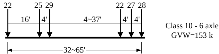
Fig. 4.17 Representative vehicle for Class 10 vehicles (Type 3S3)
