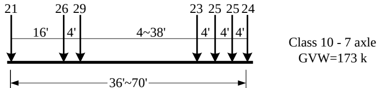
Fig. 4.18 Representative vehicle for Class 10 vehicles (Type 3S4)
