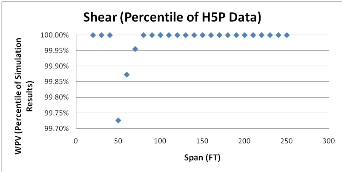
Fig. A4.5. Wisconsin 250-WPV Shear Results Compared to H5P Class 9 Truck Simulations
