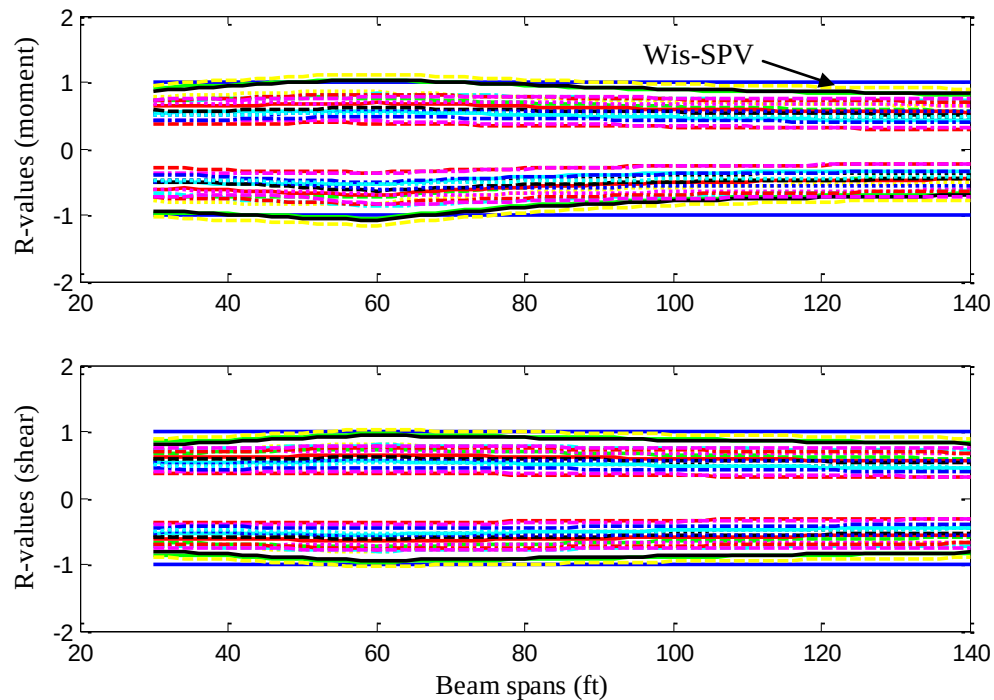
Fig. 4.28 R-values for overweight vehicles on three-span girders
