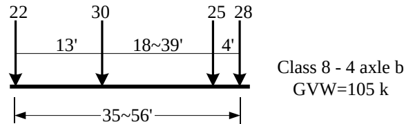
Fig. 4.14 Representative vehicle for Class 8 vehicles (Type 2S2)
