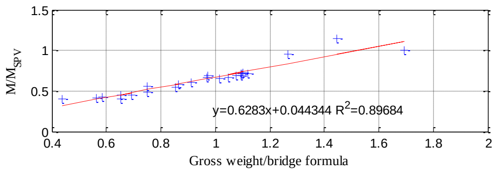
Fig. 3.12 Maximum moment distribution in 2-span girders
