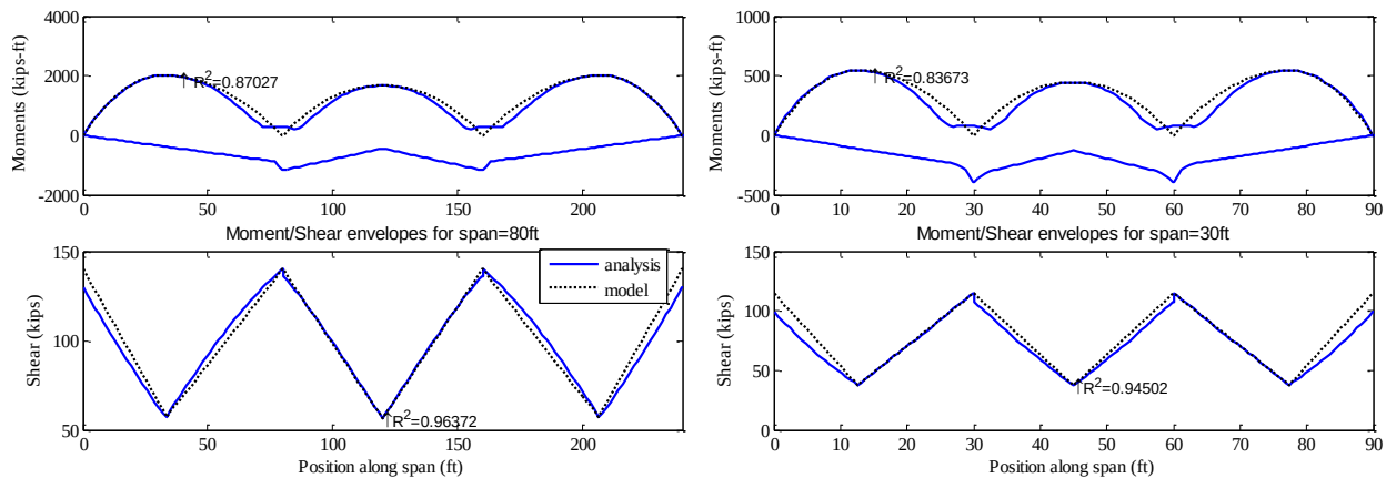
Fig. 6.22 Models of the peak responses under Wis-SPT in 3-span girders
