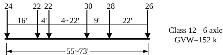
Fig. 4.20 Representative vehicle for Class 12 vehicles
