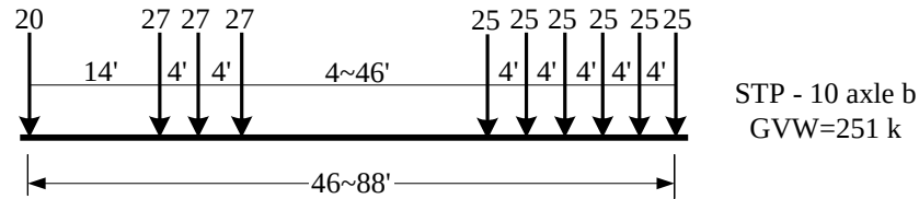
Fig. 5.14 Representative vehicle for 10-axle permit vehicles
