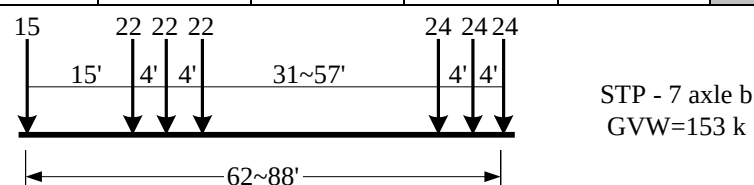
Fig. 5.9 Representative vehicle for 7-axle permit vehicles
