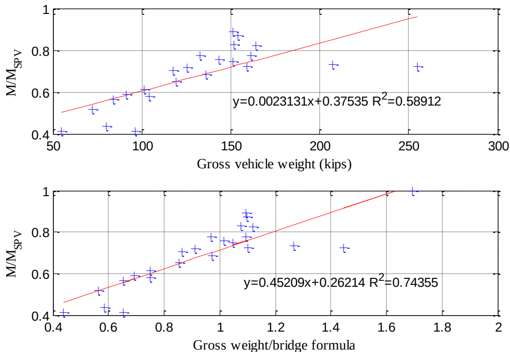
Fig. 3.11 Maximum moment distribution in 1-span girders
