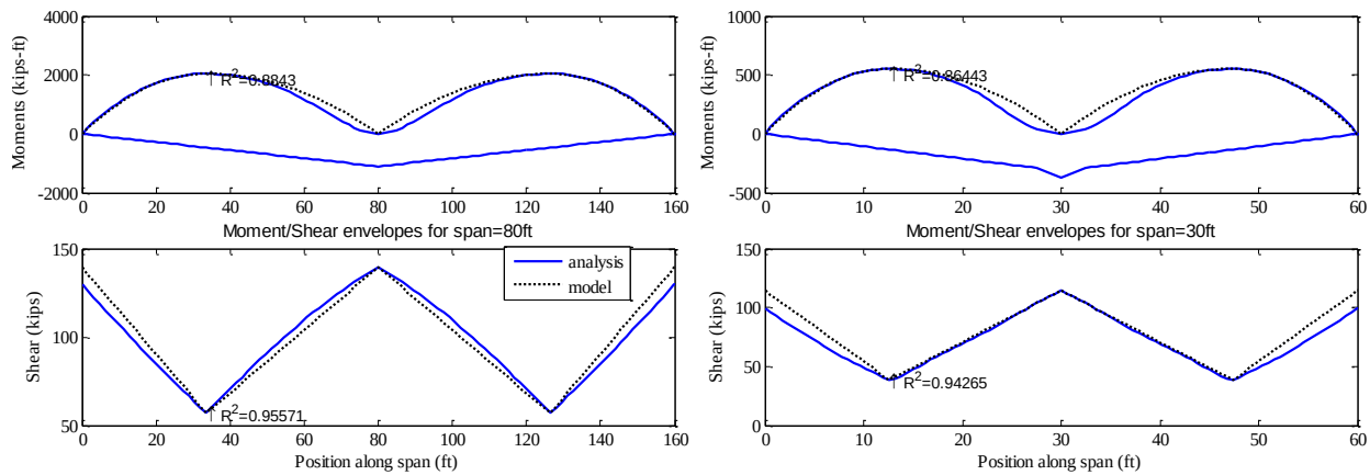
Fig. 6.17 Models of the peak responses under Wis-SPT in 2-span girders
