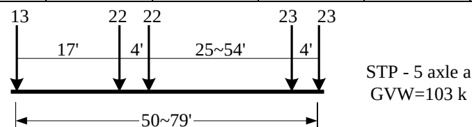
Fig. 5.5 Representative vehicle for 5-axle permit vehicles (Type 3S2)
