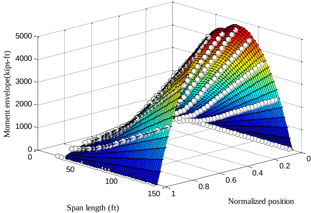
Fig. 3.1 Comparison of SAP2000 analysis results with WisDOT Bridge Manual (one-span)
