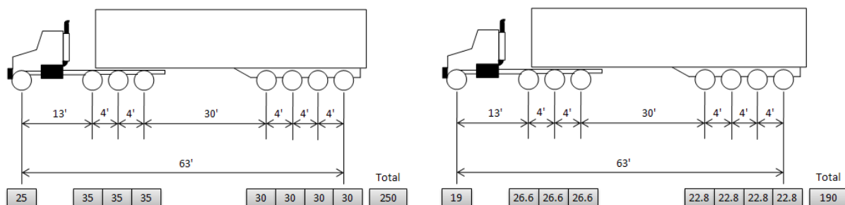
Fig. A4.2. The 250-kip and 190-kip Wisconsin Permit Vehicles.
