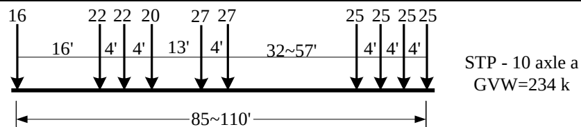
Fig. 5.13 Representative vehicle for 10-axle permit vehicles (Type a)
