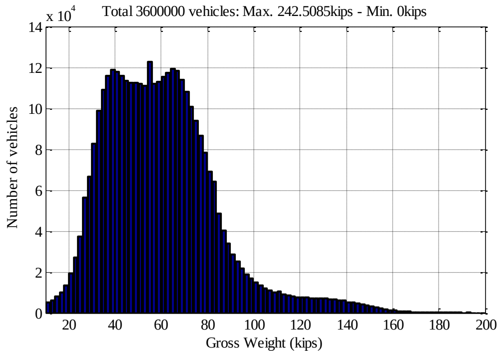
Fig. 4.2 Weight distribution of Class 9 semi-trailers
