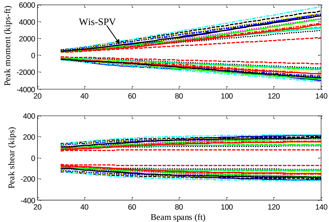
Fig. 5.20 Peak moment/shear values for representative permit vehicles on two-span girders
