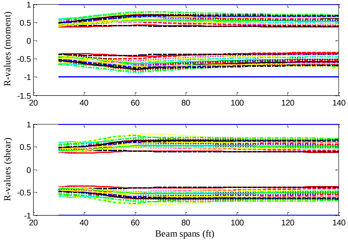
Fig. 3.9 R-values for the moment/shear envelopes in three-span girders
