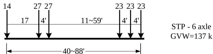
Fig. 5.7 Representative vehicle for 6-axle permit vehicles (Type 3S3)
