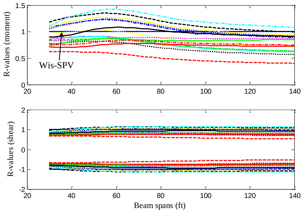
Fig. 5.19 R-values for representative permit vehicles on one-span girders
