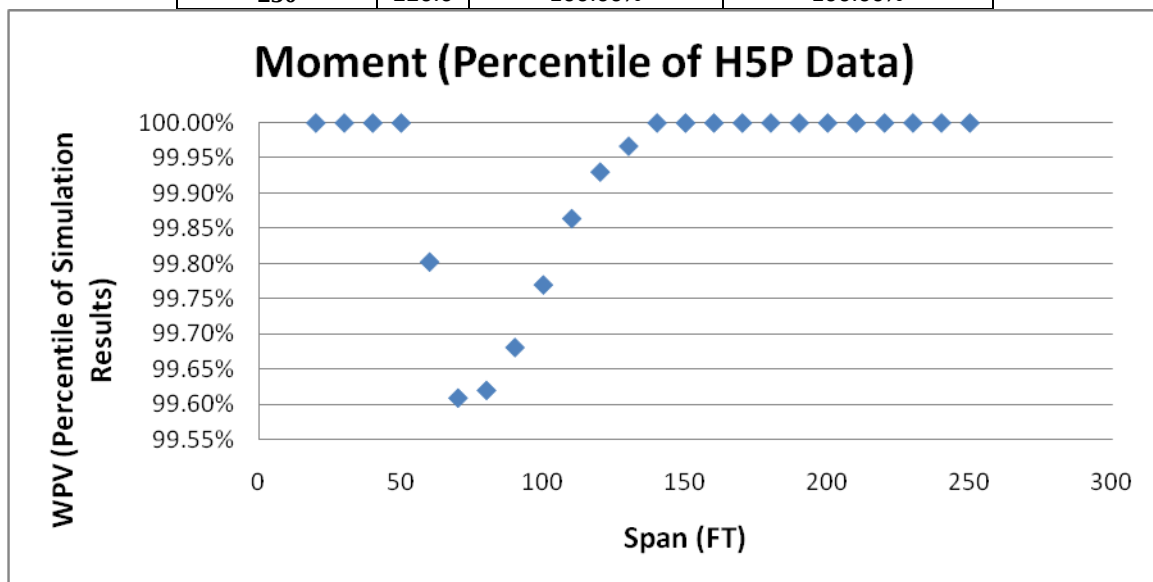
Fig. A4.4. Wisconsin 250-WPV Moment Results Compared to H5P Class 9 Truck Simulations
