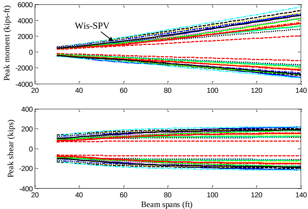
Fig. 5.22 Peak moment/shear values for representative permit vehicles on three-span girders
