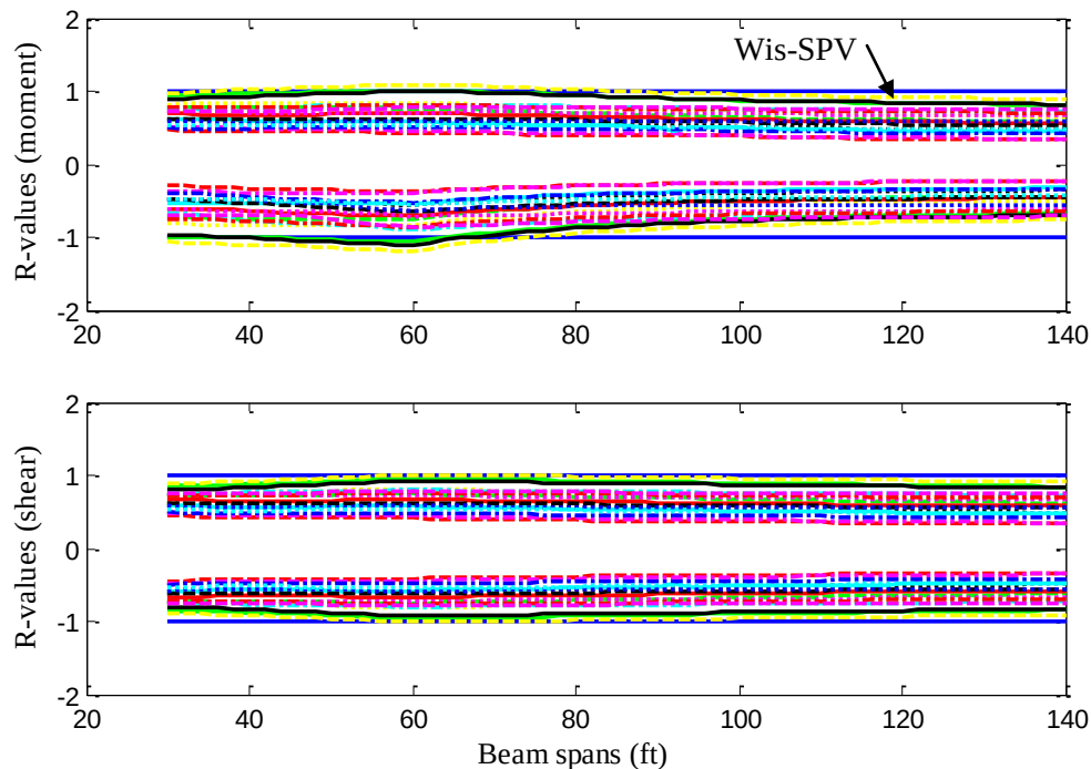
Fig. 4.27 R-values for overweight vehicles on two-span girders
