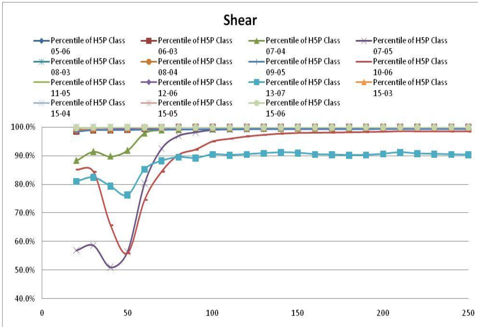
Fig. A4.9. Plot of 190-WPV shear as percentile of H5P data versus span length (ft) for each truck class-axle group.
