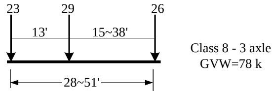
Fig. 4.12 Representative vehicle for Class 8 vehicles (Type 2S1)
