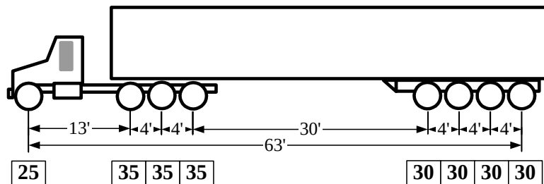
Fig. A3.1 Wisconsin Standard Permit Vehicle
