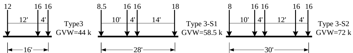
Fig. 2.5 Illinois load rating and posting trucks
