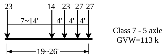
Fig. 4.11 Representative vehicle for Class 7 vehicles (5-axle)
