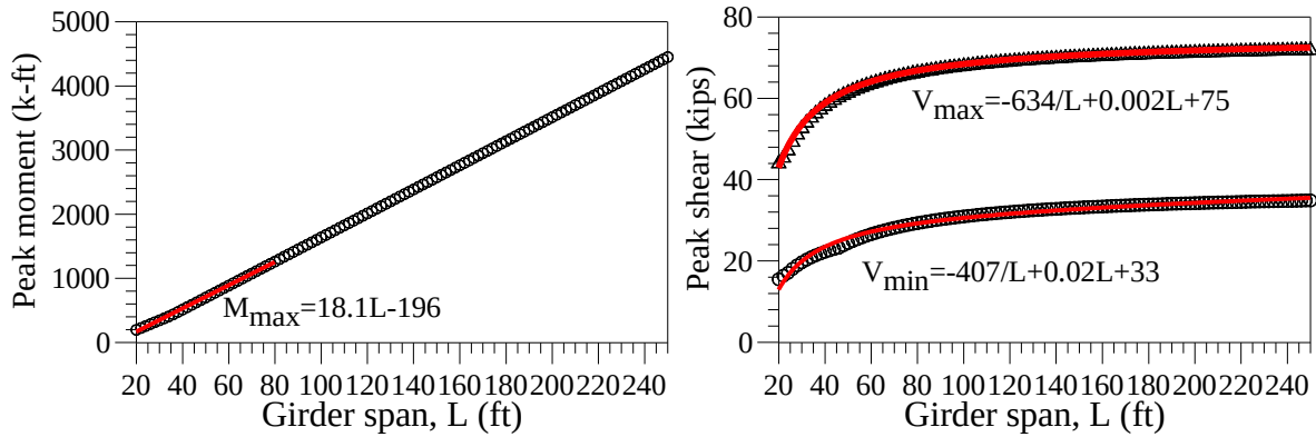
Fig. 6.11 Regression analysis of the peak responses under Wis-SPV in 1-span girders
