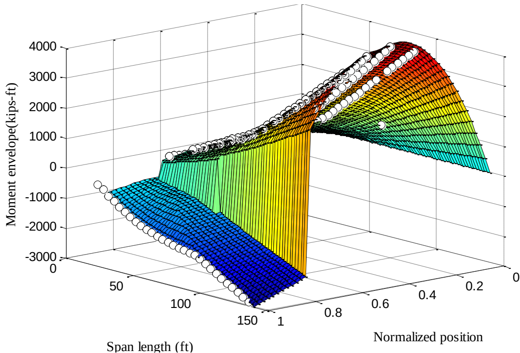
Fig. 3.2 Comparison of SAP2000 analysis results with WisDOT Bridge Manual (two-span)
