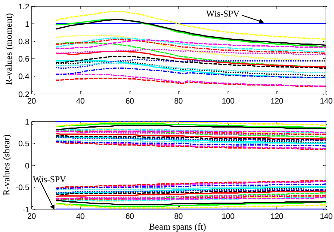
Fig. 4.25 R-values for overweight vehicles on one-span girders
