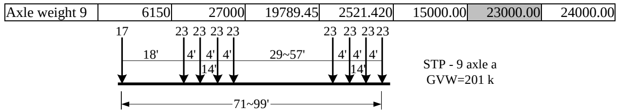
Fig. 5.11 Representative vehicle for 9-axle permit vehicles (Type a)
