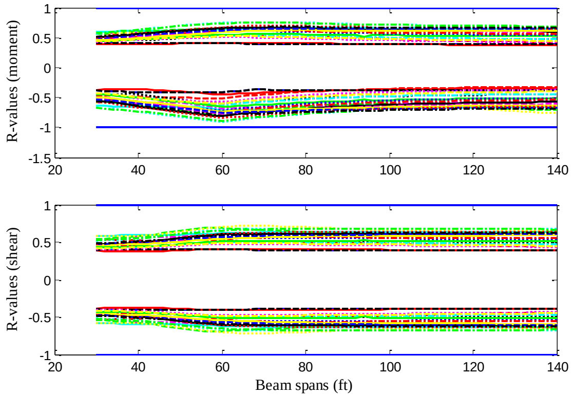
Fig. 3.7 R-values for the moment/shear envelopes in two-span girders
