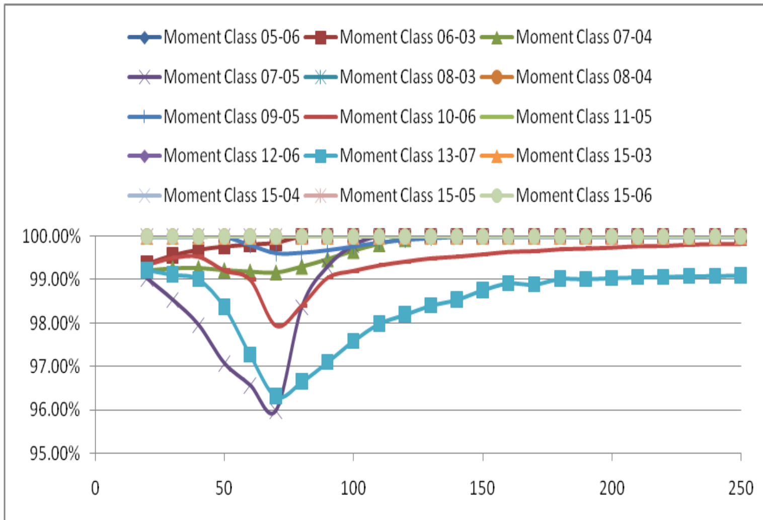
Fig. A4.6. Plot of 250-WPV moments as percentile of H5P data versus span length (ft) for each truck class-axle group.
