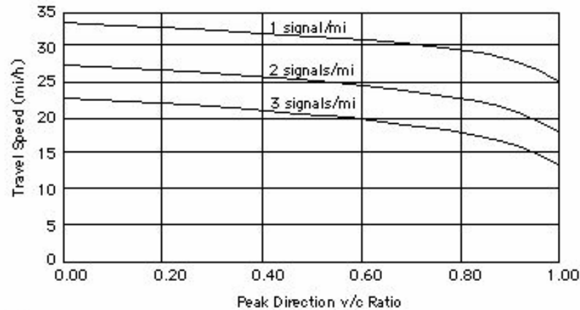
EXHIBIT 15-9. SPEED-FLOW CURVES FOR CLASS II URBAN STREETS (SEE FOOTNOTE FOR ASSUMED VALUES)
