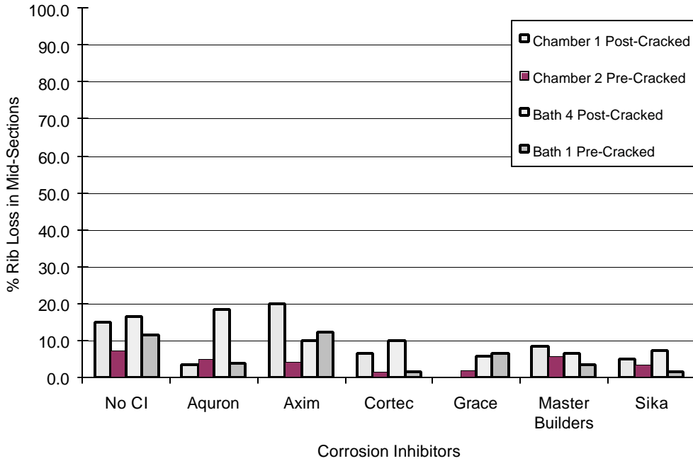
Figure 4.28 - % Rib Loss in Midsections for 0.0% Chloride (Set #1)
