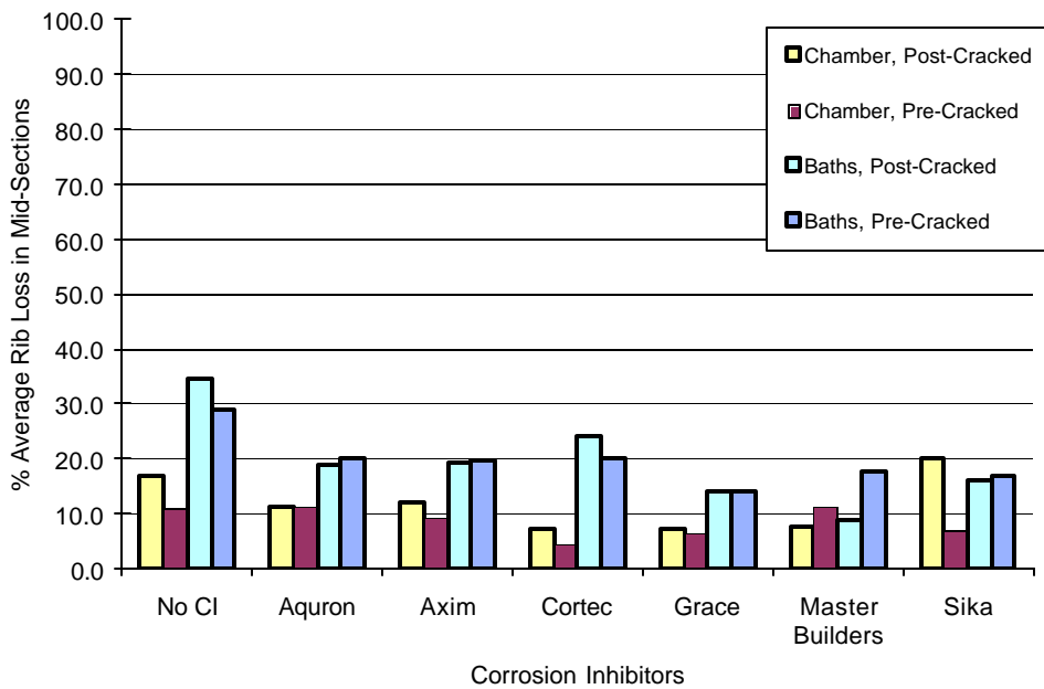
Figure E.14 Rib Loss at Mid Section for Average of all Chloride Contaminants (Set#1)
