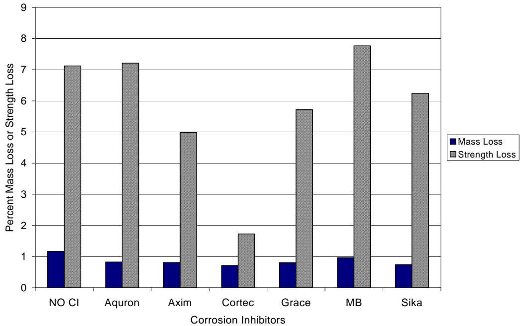
Figure G.62 – Mass Loss and Strength Loss for Chamber Shelf 2, 0.0% Chloride, Pre-Cracked
