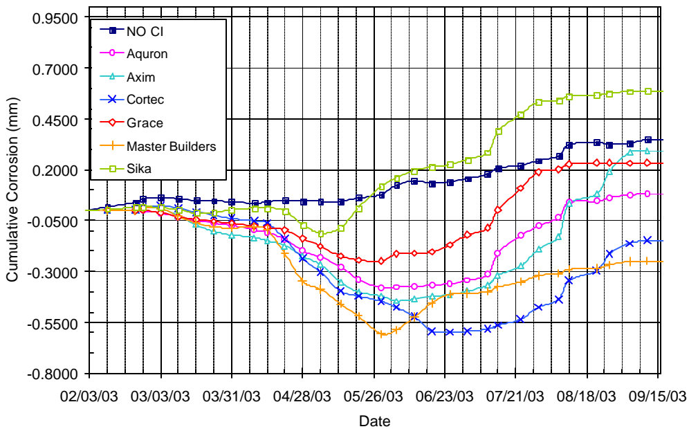
Figure B.24 – Cumulative Corrosion Over Time for Bath 4, 1.5% Chloride, Post-Cracked
