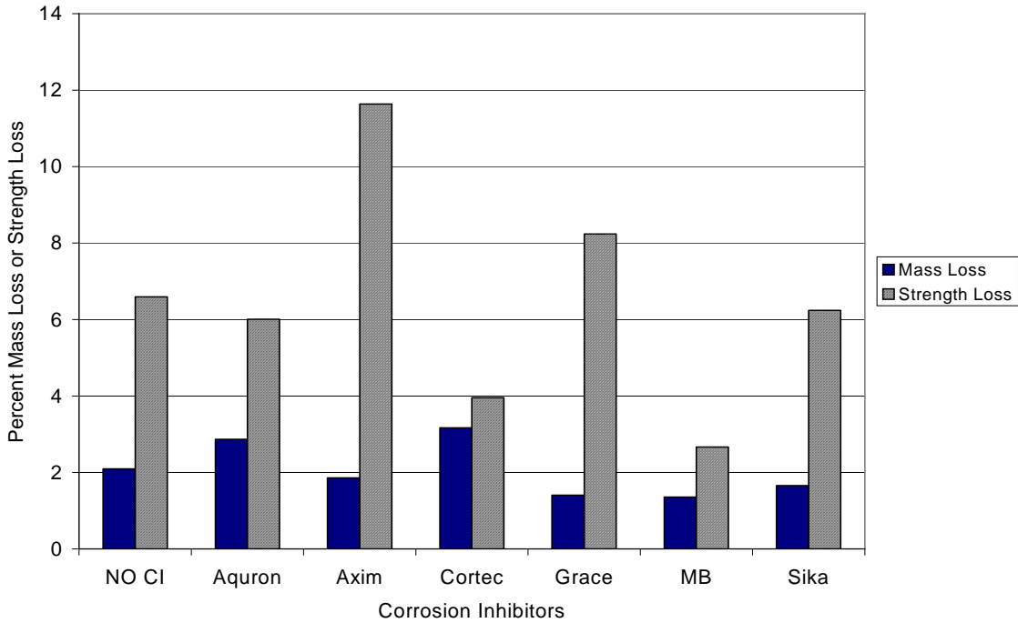
Figure G.46 – Mass Loss and Strength Loss for Bath 4, 2.0% Chloride, Post-Cracked
