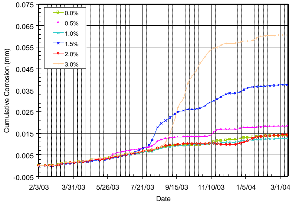
Figure 4.4 - Cumulative Corrosion Over Time for Control Specimens (Set #2)
