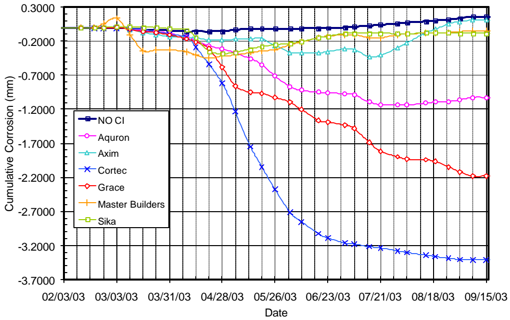
Figure B.5 – Cumulative Corrosion Over Time for Bath 1, 1.0% Chloride, Pre-Cracked
