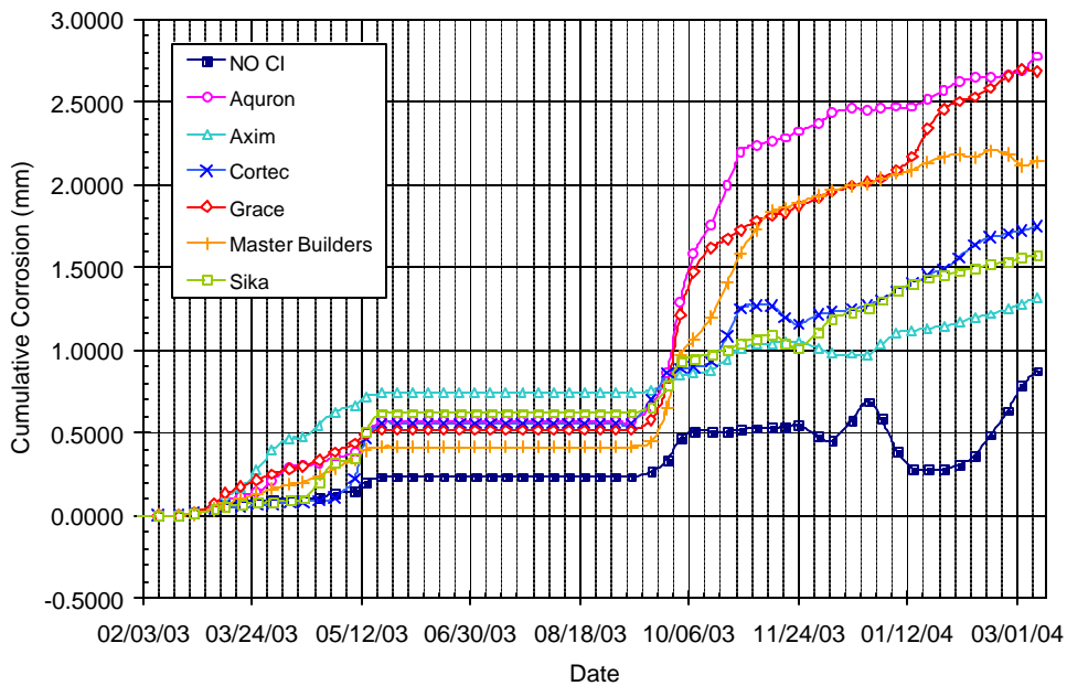
Figure B.50 – Cumulative Corrosion Over Time for Chamber Shelf 4, 3.0% Chloride, Pre-Cracked
