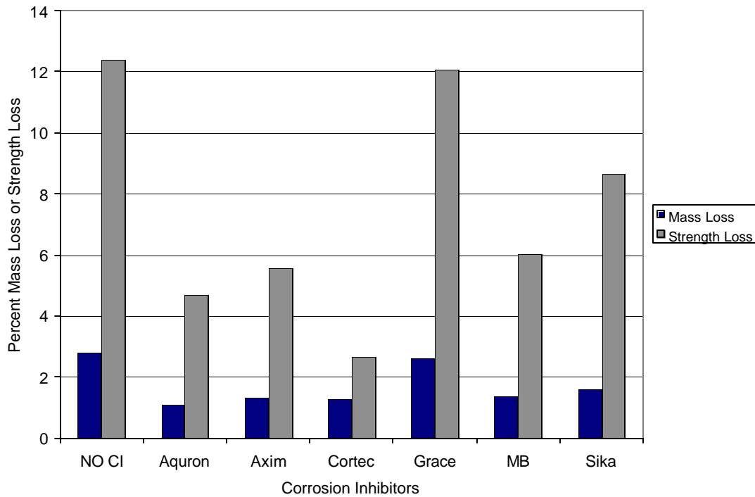
Figure 4.42 – Mass Loss and Strength Loss for Bath 2, 0.0% Chloride, Pre-Cracked Specimens
