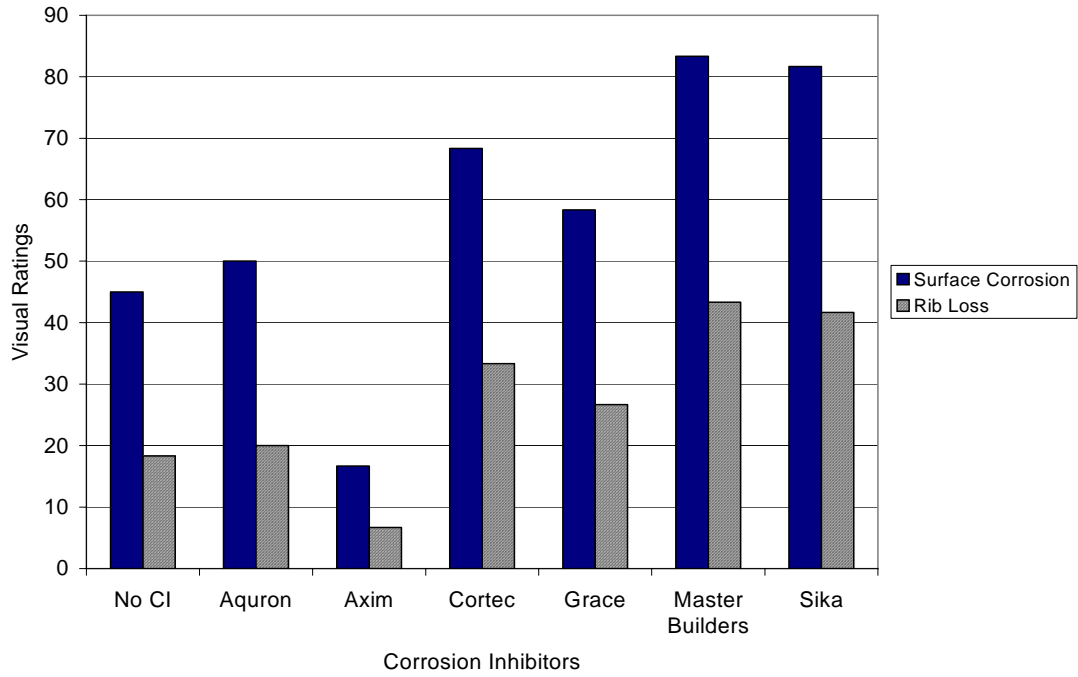
Figure G.17 – Visual Ratings for Bath 2, 1.0% Chloride, Pre-Cracked
