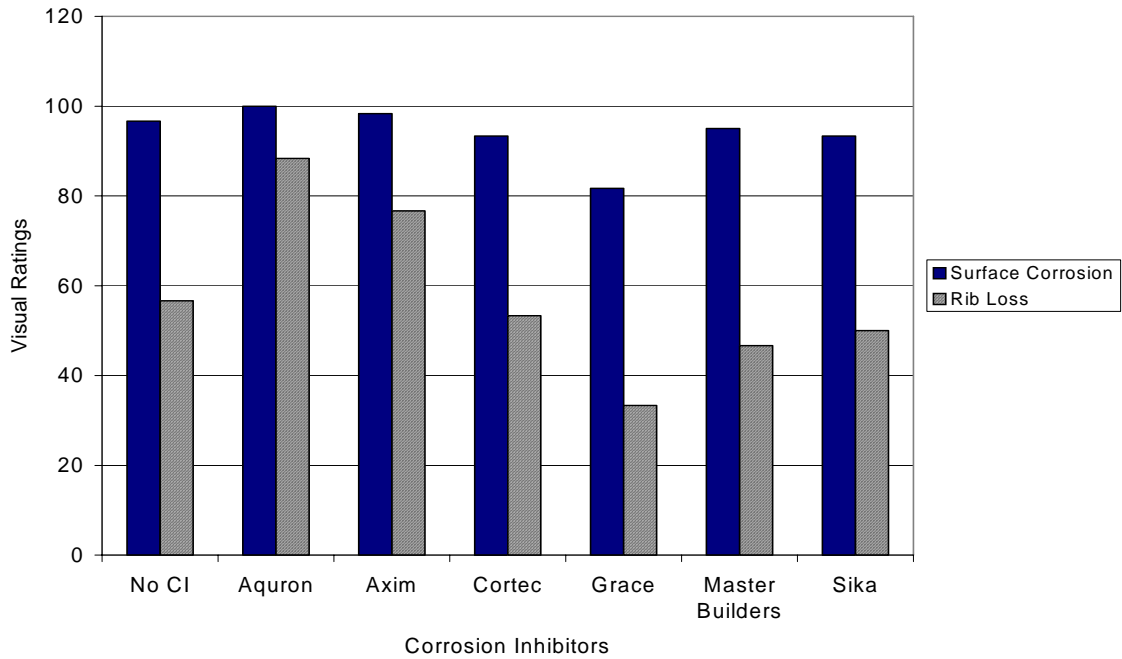
Figure G.31 – Visual Ratings for Bath 3, 1.5% Chloride, Post-Cracked
