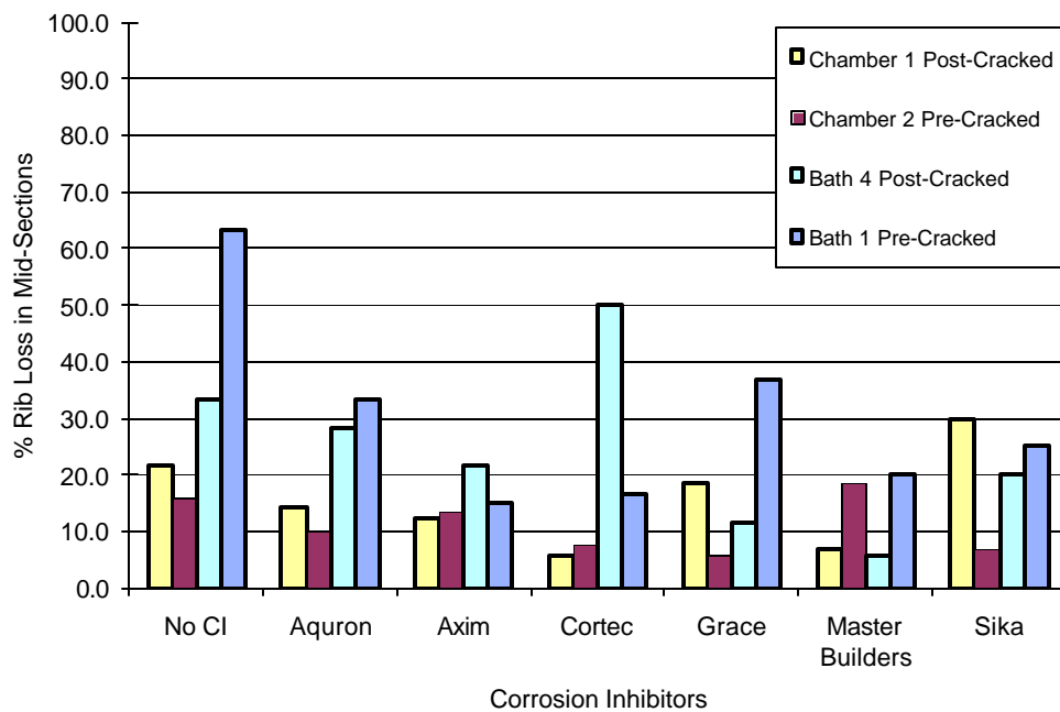
Figure E.10 Rib Loss at Mid Section for 2.0% Chloride (Set #1)
