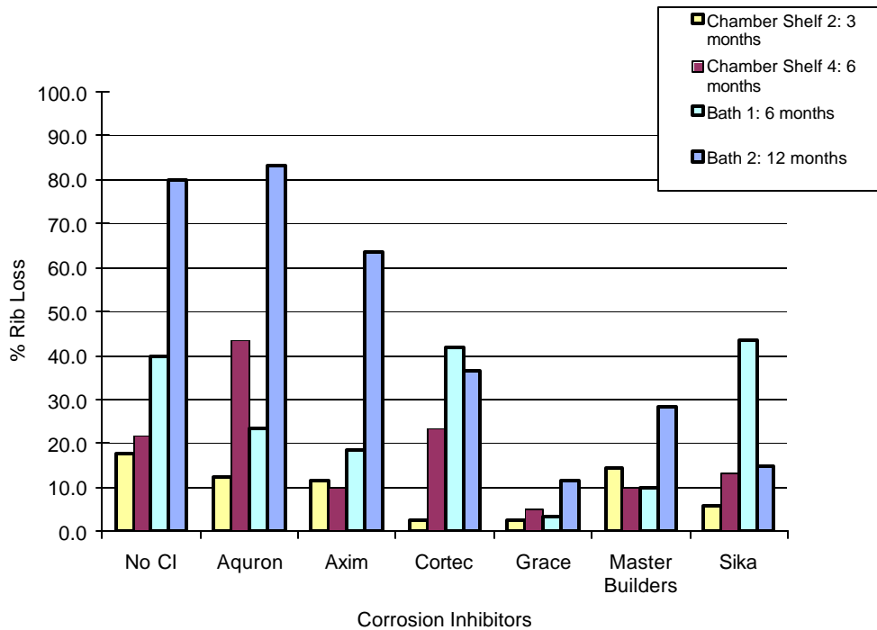
Figure E.36 Time Step of Rib Loss for 1.5% Chloride Pre-Cracked Specimens
