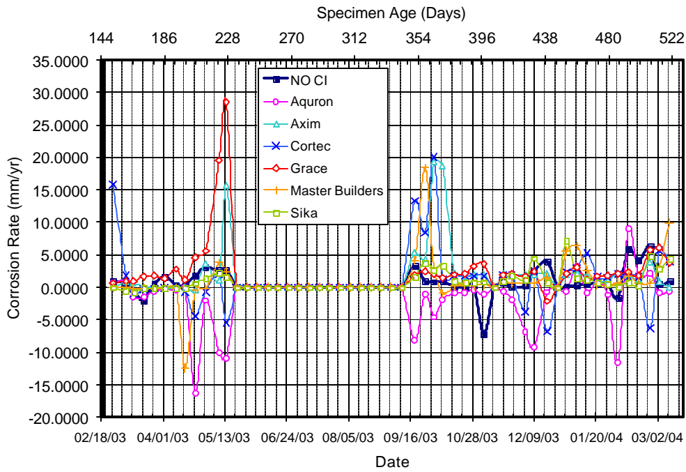
Figure A.47 – Corrosion Rate for Chamber Shelf 4, 1.0% Chloride, Pre-Cracked
