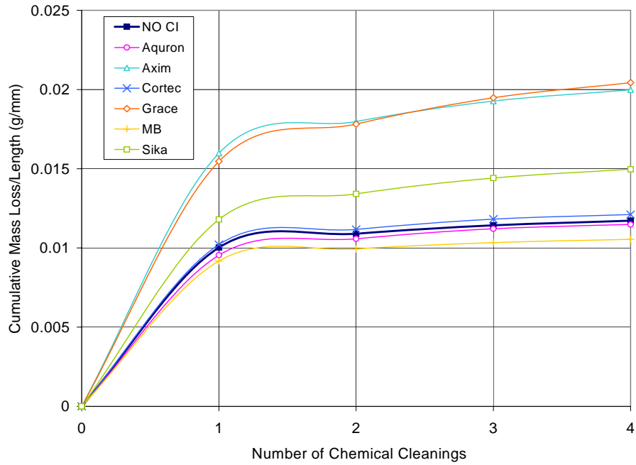
Figure F.25 – Cumulative Mass Loss/Length for Bath 4, 3.0% Chloride Post-Cracked Specimens
