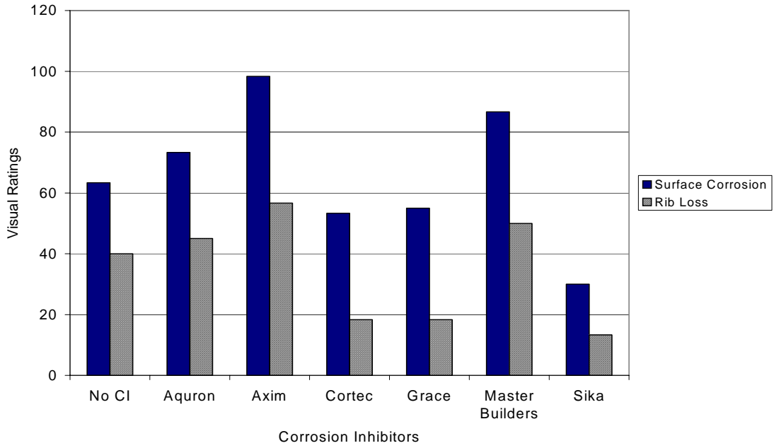
Figure G.23 – Visual Ratings for Bath 2, 3.0% Chloride, Pre-Cracked
