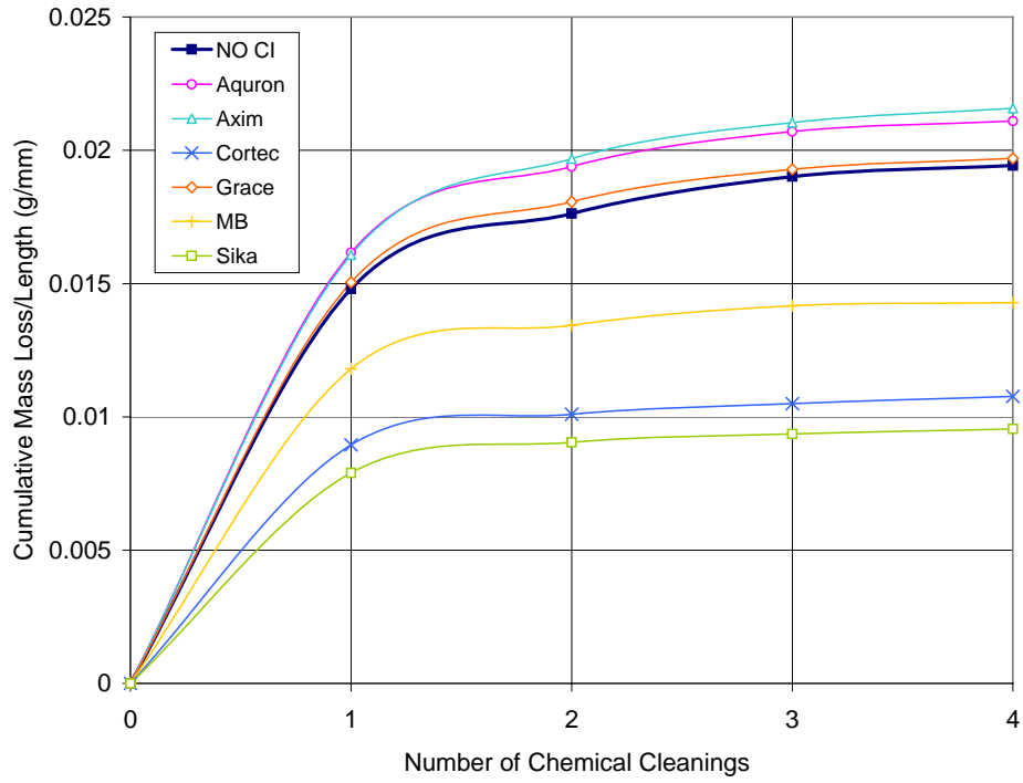
Figure F.49 – Cumulative Mass Loss/Length for Chamber Shelf 4 3.0% Chloride, Pre-Cracked Specimens
