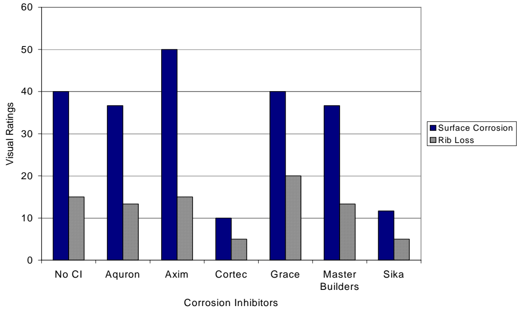
Figure G.95 – Visual Ratings for Chamber Shelf 4, 3.0% Chloride, Pre-Cracked
