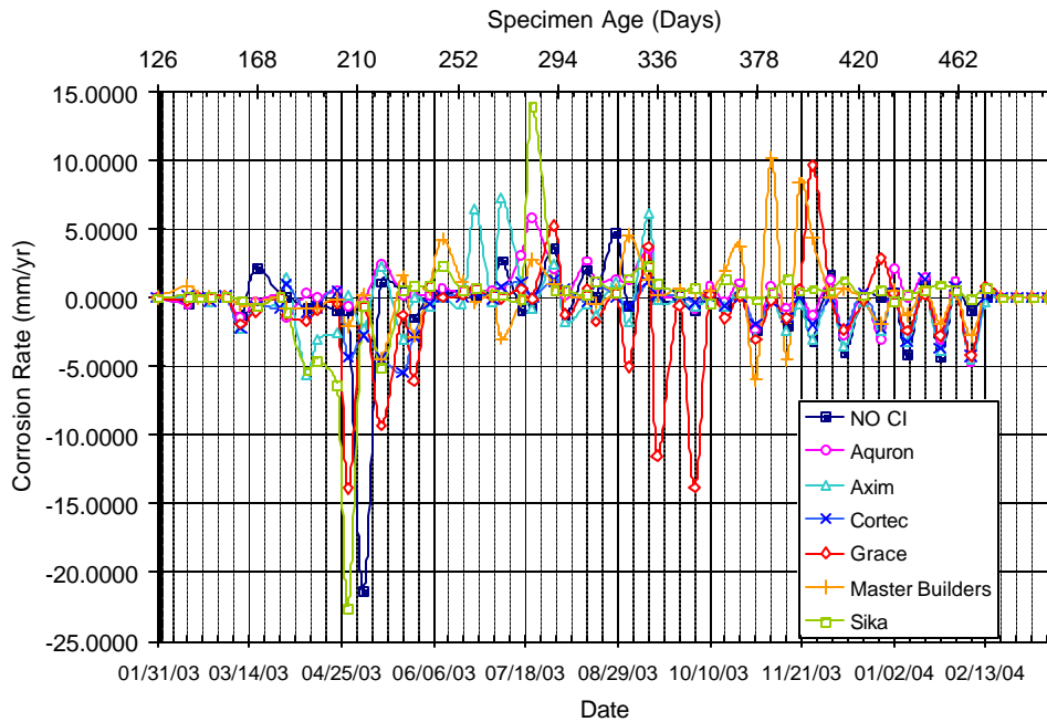
Figure A.16 – Corrosion Rate for Bath 3, 0.5% Chloride, Post-Cracked
