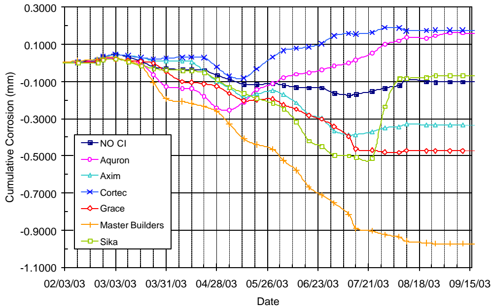
Figure B.25 – Cumulative Corrosion Over Time for Bath 4, 2.0% Chloride, Post-Cracked
