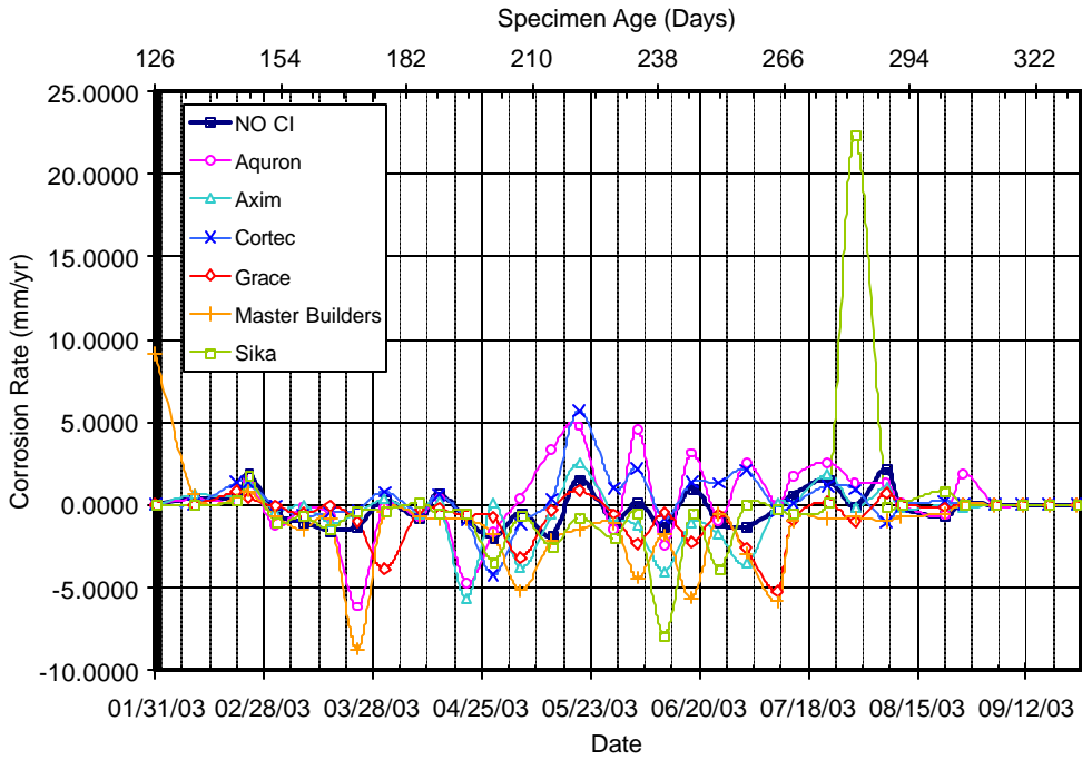
Figure A.25 – Corrosion Rate for Bath 4, 2.0% Chloride, Post-Cracked
