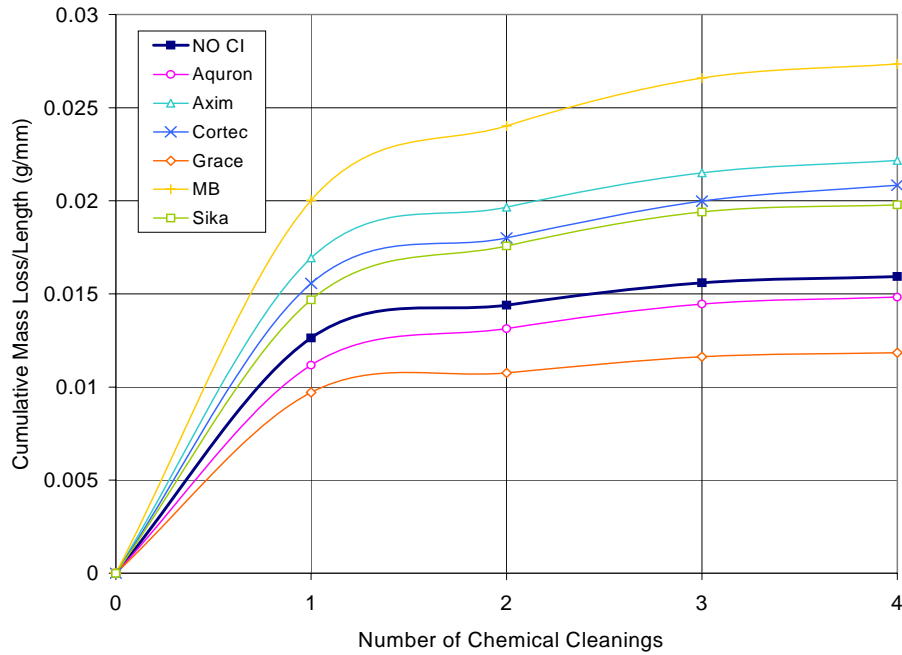
Figure F.43 – Cumulative Mass Loss/Length for Chamber Shelf 3 3.0% Chloride, Post-Cracked Specimens
