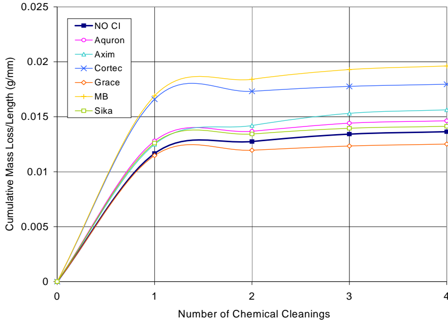
Figure F.3 – Cumulative Mass Loss/Length for Bath 1, 0.5% Chloride Pre-Cracked Specimens
