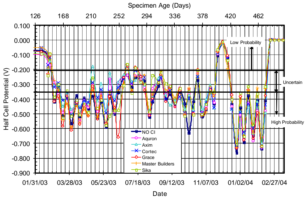
Figure C.11 – Half Cell Potential Readings for Bath 2, 1.0% Chloride, Pre-Cracked
