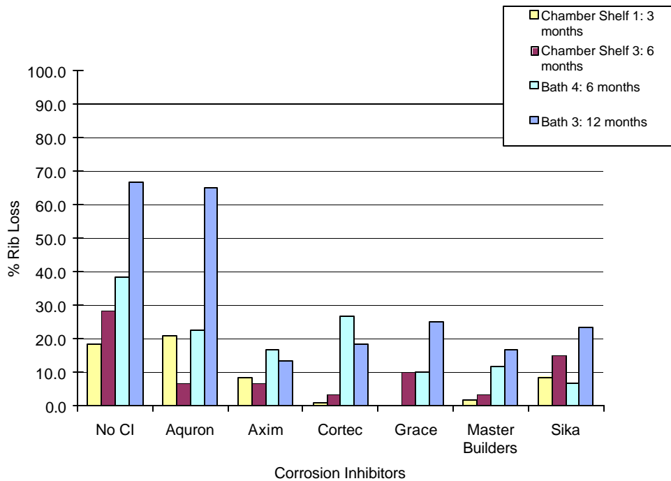
Figure E.44 Time Step of Rib Loss for 0.5% Chloride Post-Cracked Specimens
