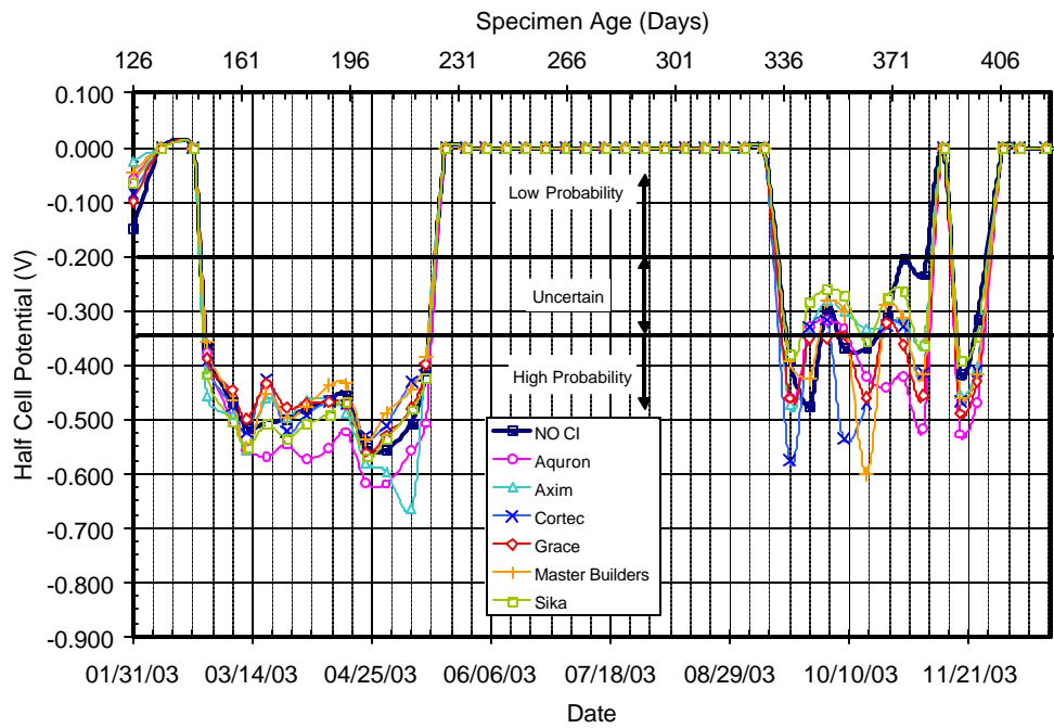
Figure C.32 – Half Cell Potential Readings for Chamber Shelf 1, 3.0% Chloride, Post-Cracked
