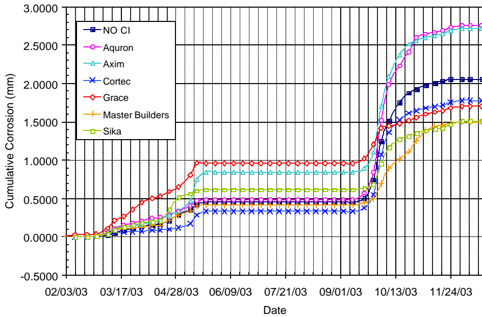
Figure B.31 – Cumulative Corrosion Over Time for Chamber Shelf 1, 2.0% Chloride, Post-Cracked
