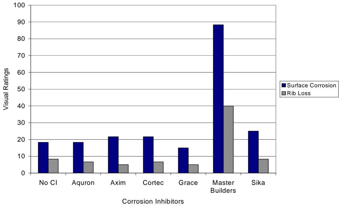
Figure G.35 – Visual Ratings for Bath 3, 3.0% Chloride, Post-Cracked
