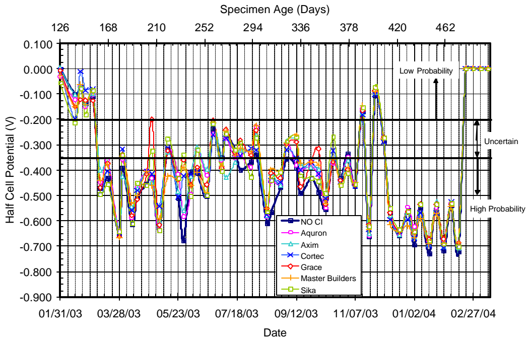
Figure C.15 – Half Cell Potential Readings for Bath 3, 0.0% Chloride, Post-Cracked
