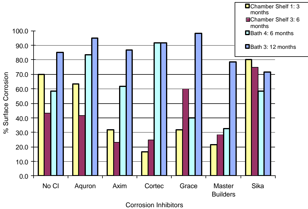
Figure E.49 Time Step of Surface Corrosion for 2.0% Chloride Post-Cracked Specimens
