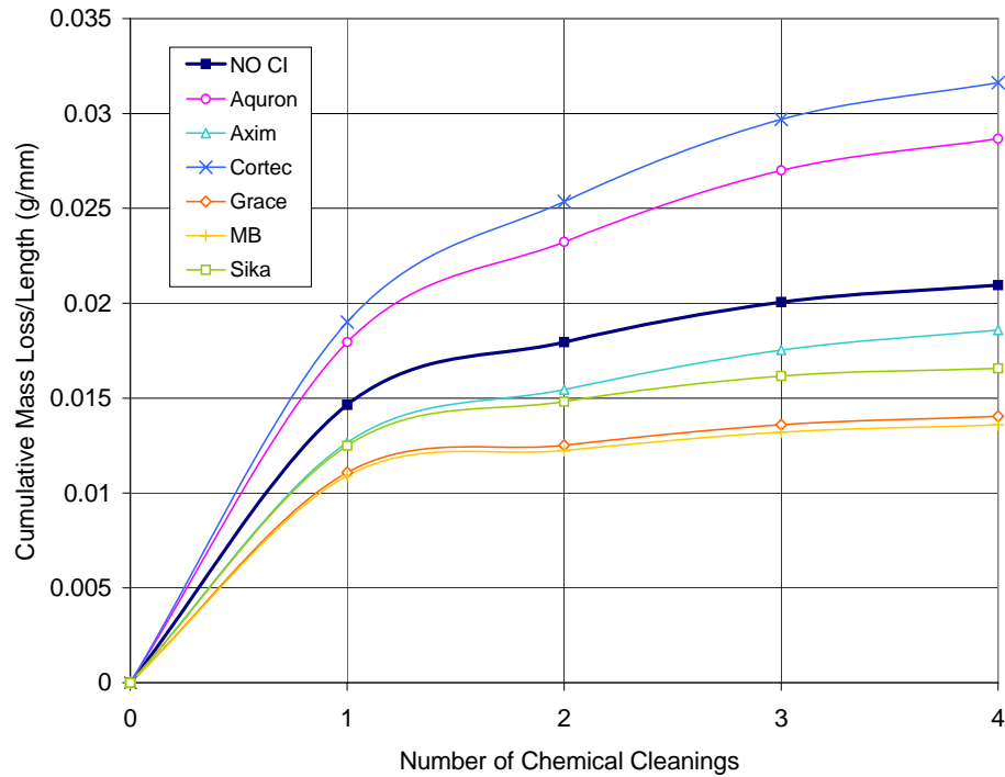
Figure F.23 – Cumulative Mass Loss/Length for Bath 4, 1.5% Chloride Post-Cracked Specimens
