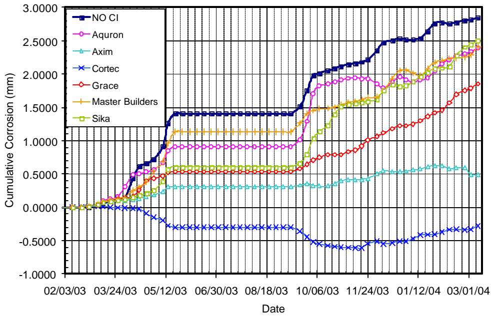
Figure B.43 – Cumulative Corrosion Over Time for Chamber Shelf 3, 2.0% Chloride, Post-Cracked
