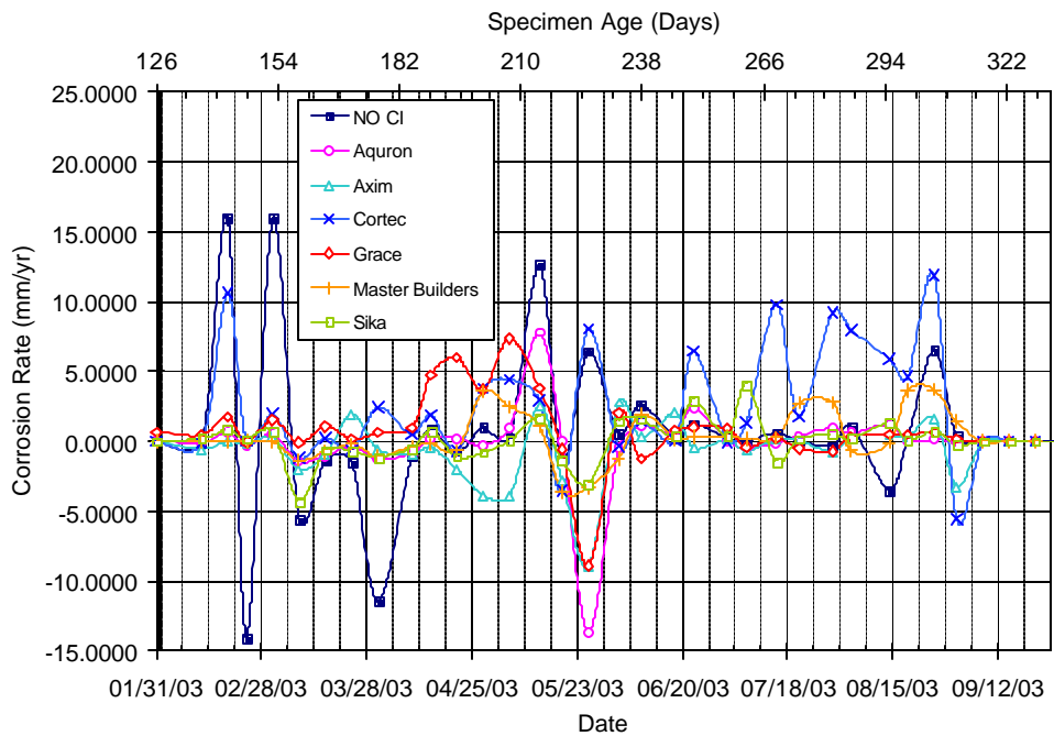
Figure A.8 – Corrosion Rate for Bath 1, 3.0% Chloride, Pre-Cracked
