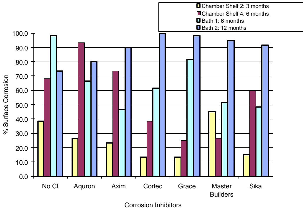
Figure E.37 Time Step of Surface Corrosion for 2.0% Chloride Pre-Cracked Specimens
