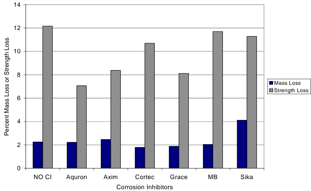
Figure G.60 – Mass Loss and Strength Loss for Chamber Shelf 1, 3.0% Chloride, Post-Cracked
