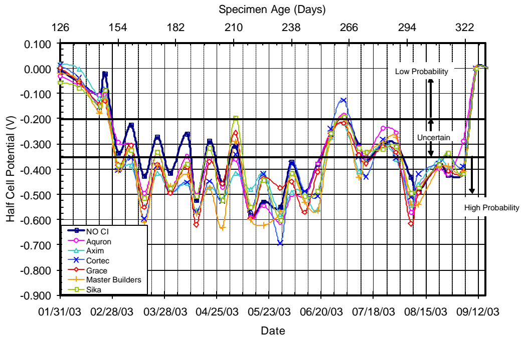
Figure C.21 – Half Cell Potential Readings for Bath 4, 0.0% Chloride, Post-Cracked
