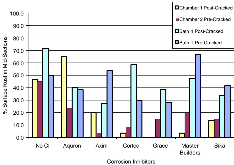
Figure E.3 Surface Corrosion at Mid Section for 0.5% Chloride (Set#1)
