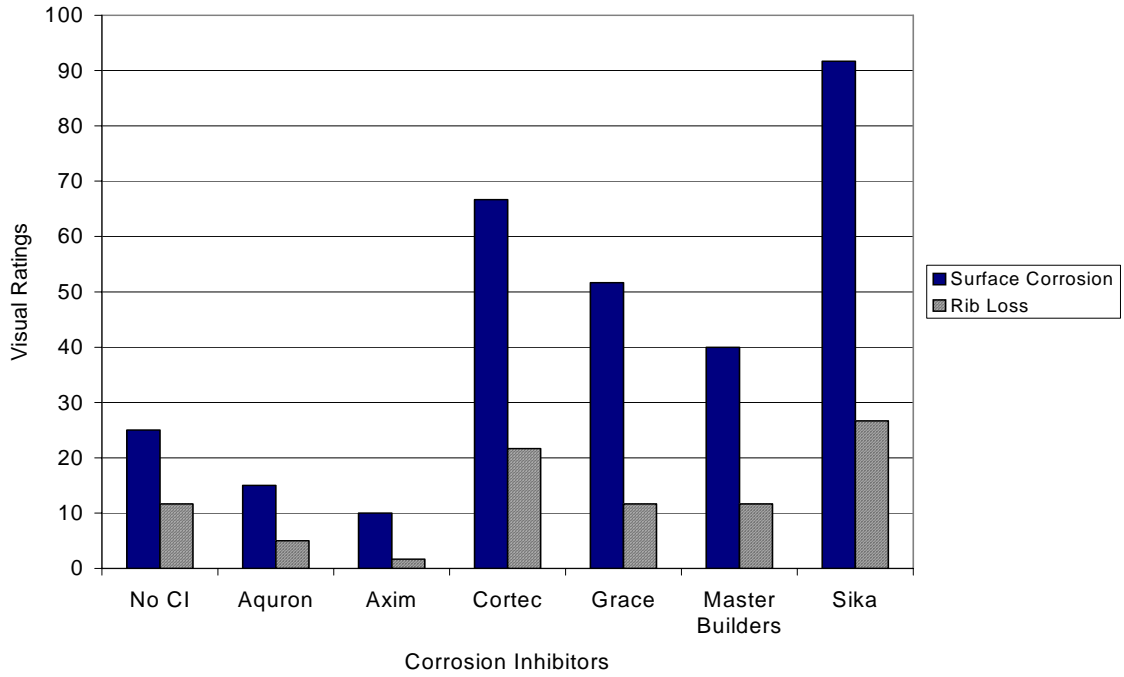
Figure G.29 – Visual Ratings for Bath 3, 1.0% Chloride, Post-Cracked
