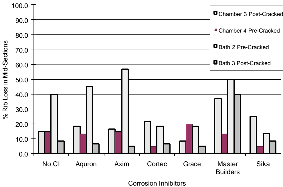
Figure 4.33 - % Rib Loss in Midsections for 3.0% Chloride (Set #2)
