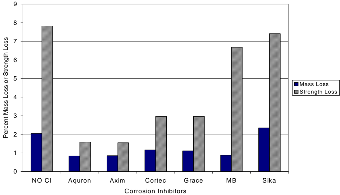
Figure G.42 – Mass Loss and Strength Loss for Bath 4, 1.0% Chloride, Post-Cracked
