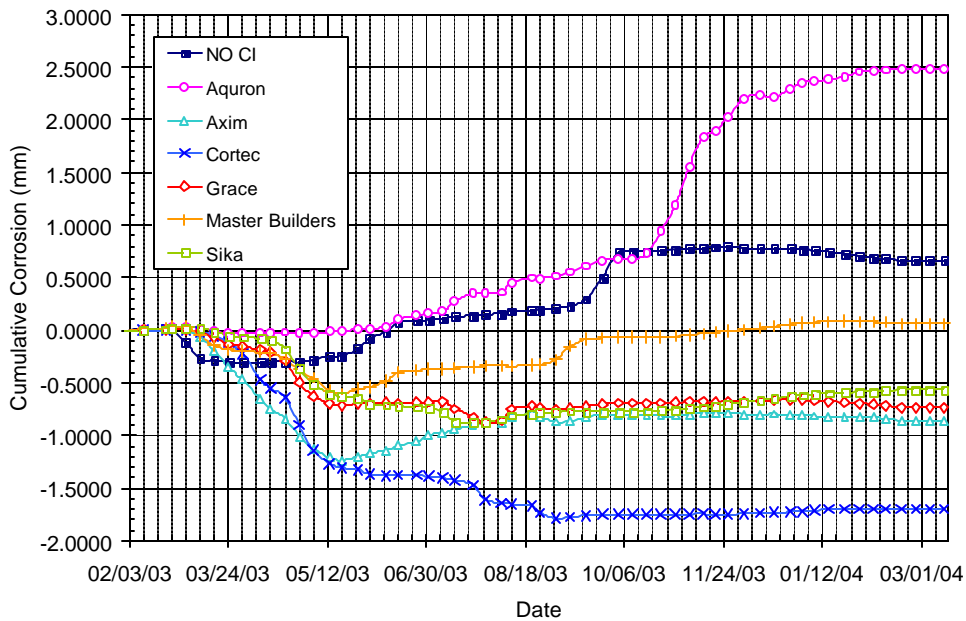
Figure B.14 – Cumulative Corrosion Over Time for Bath 2, 3.0% Chloride, Pre-Cracked
