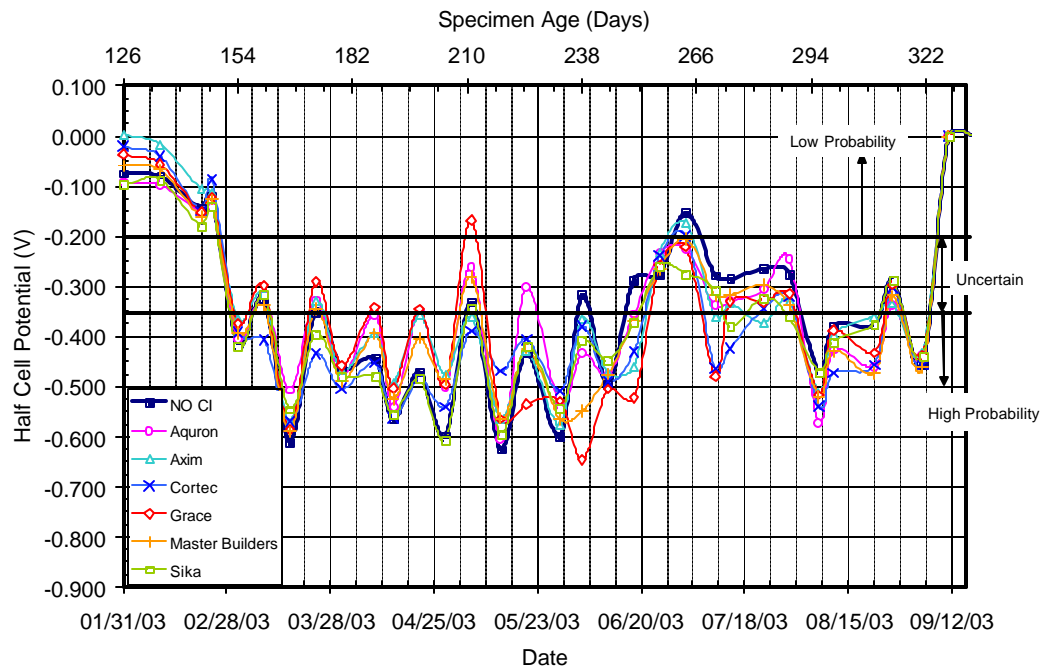
Figure C.22 – Half Cell Potential Readings for Bath 4, 0.5% Chloride, Post-Cracked
