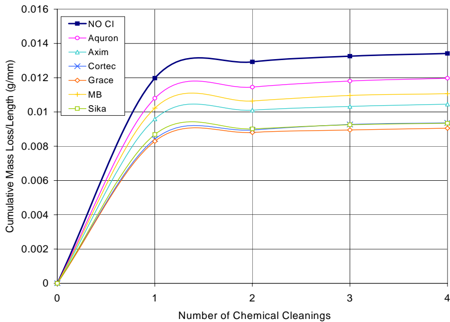
Figure F.19 – Cumulative Mass Loss/Length for Bath 3, 3.0% Chloride Post-Cracked Specimens
