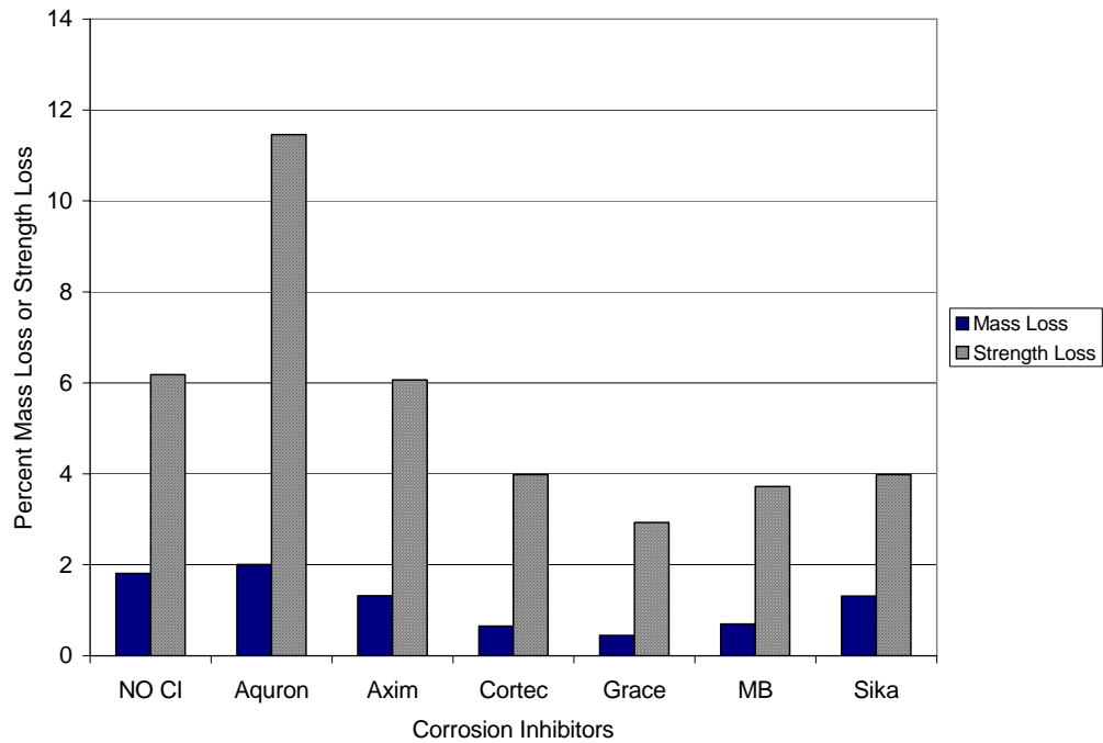
Figure G.52 – Mass Loss and Strength Loss for Chamber Shelf 1, 0.5% Chloride, Post-Cracked
