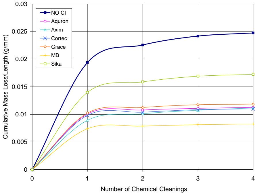
Figure F.39 – Cumulative Mass Loss/Length for Chamber Shelf 3 0.5% Chloride, Post-Cracked Specimens
