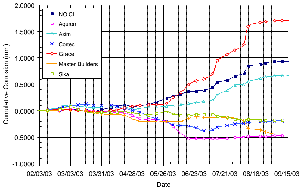
Figure B.26 – Cumulative Corrosion Over Time for Bath 4, 3.0% Chloride, Post-Cracked
