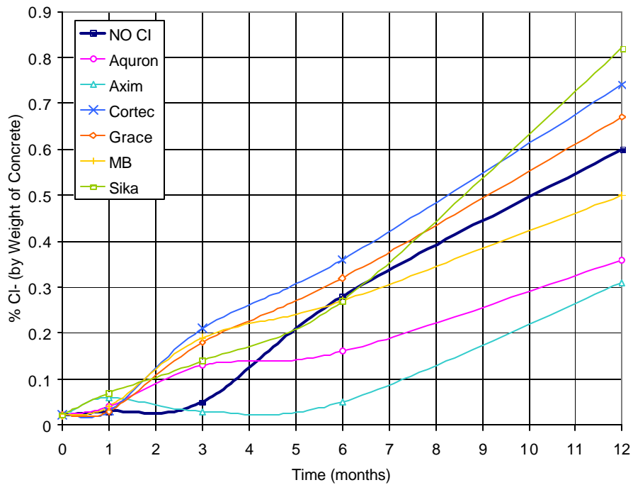
Figure D.2 – Chloride Content for Bath Specimens – 0.0% Chloride
