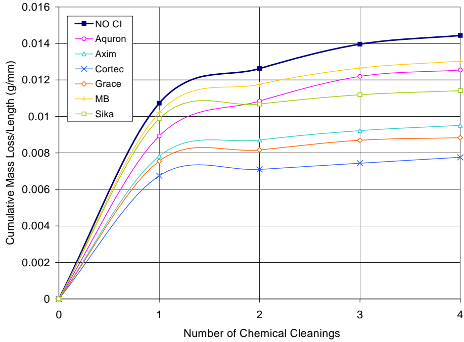
Figure F.35 – Cumulative Mass Loss/Length for Chamber Shelf 2 1.5% Chloride, Pre-Cracked Specimens
