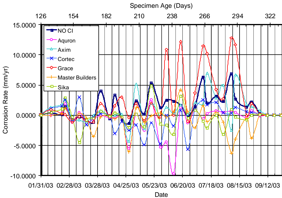
Figure A.26 – Corrosion Rate for Bath 4, 3.0% Chloride, Post-Cracked
