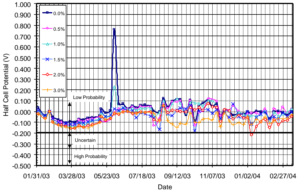
Figure 4.7 - Half Cell Readings for Control Specimens (Set #2)
