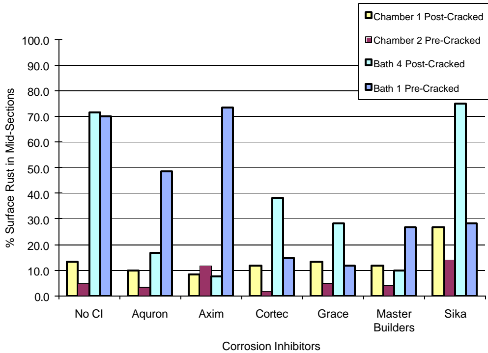
Figure E.5 Surface Corrosion at Mid Section for 1.0% Chloride (Set#1)
