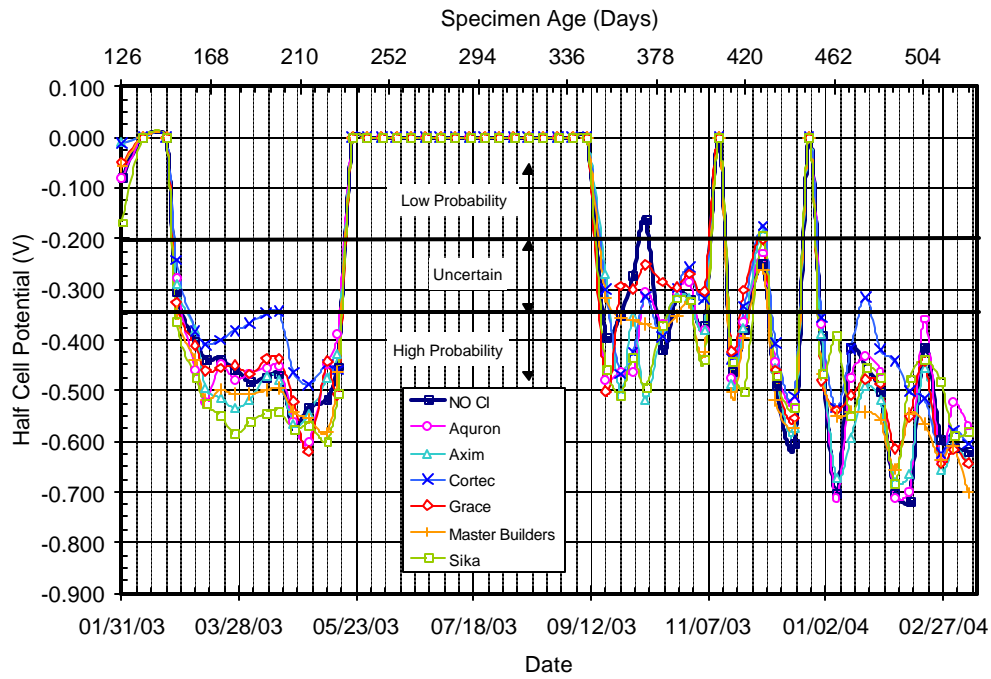
Figure C.49 – Half Cell Potential Readings for Chamber Shelf 4, 2.0% Chloride, Pre-Cracked
