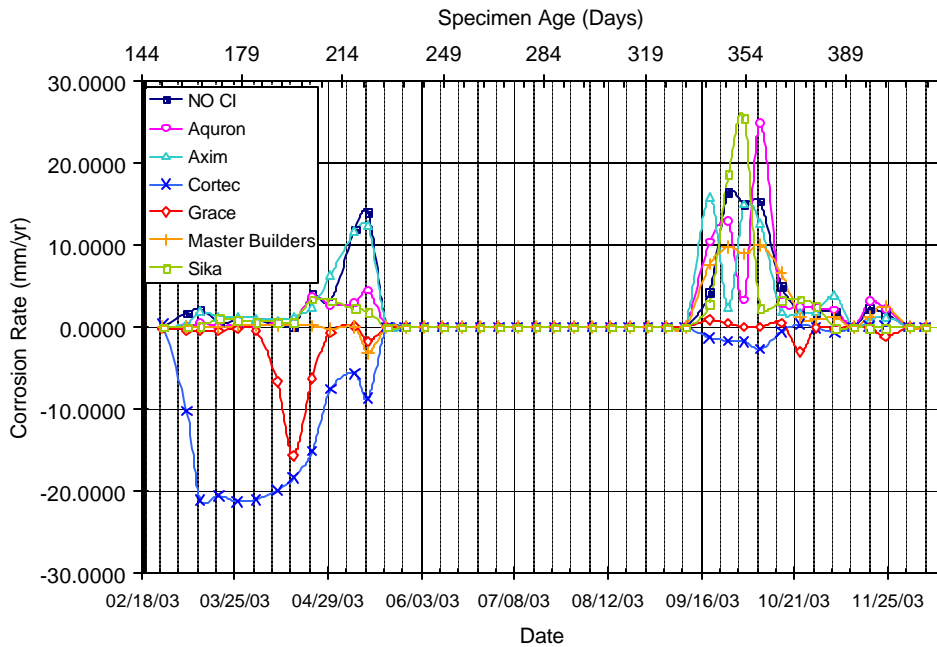
Figure A.28 – Corrosion Rate for Chamber Shelf 1, 0.5% Chloride, Post-Cracked
