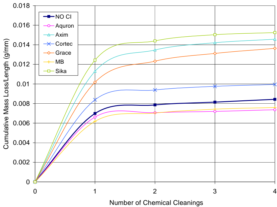
Figure F.45 – Cumulative Mass Loss/Length for Chamber Shelf 4 0.5% Chloride, Pre-Cracked Specimens
