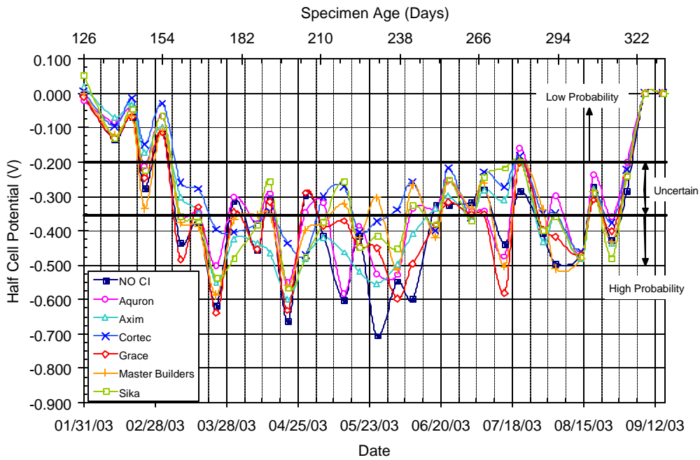
Figure C.3 – Half Cell Potential Readings for Bath 1, 0.0% Chloride, Pre-Cracked
