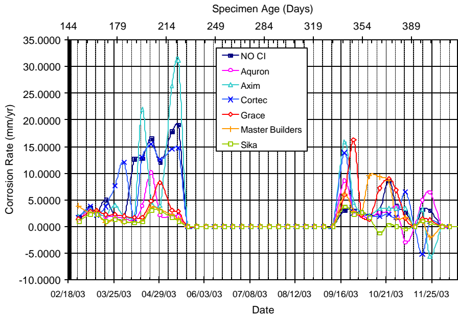
Figure A.38 – Corrosion Rate for Chamber Shelf 2, 3.0% Chloride, Pre-Cracked
