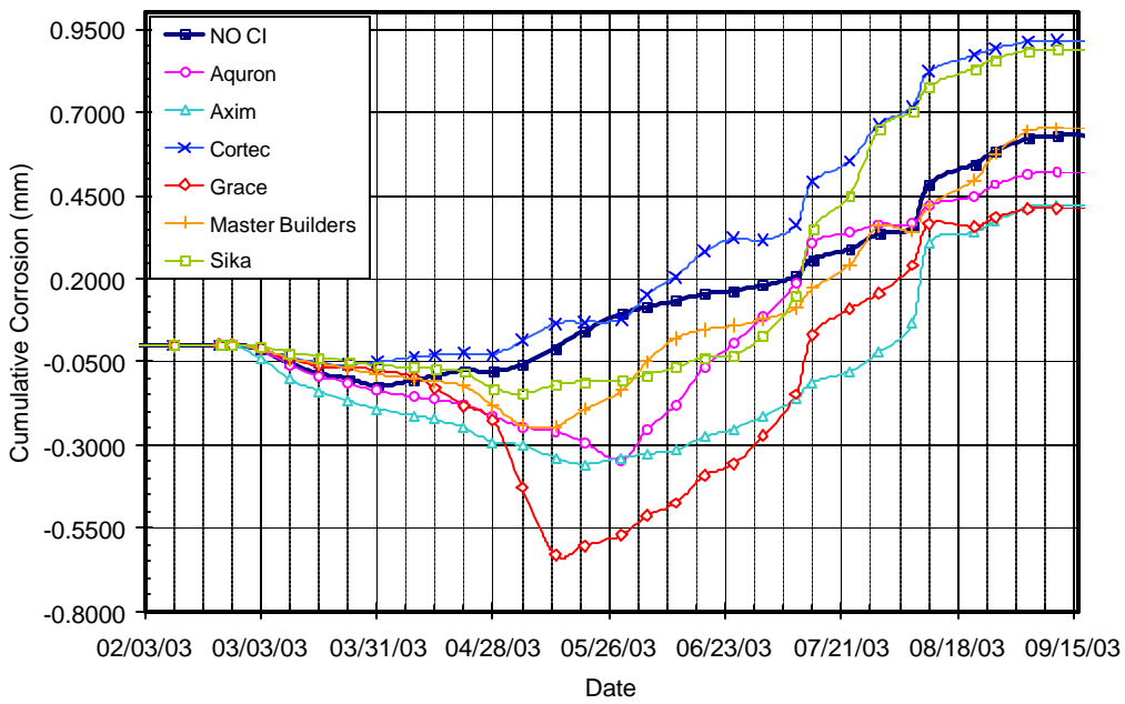
Figure B.22 – Cumulative Corrosion Over Time for Bath 4, 0.5% Chloride, Post-Cracked
