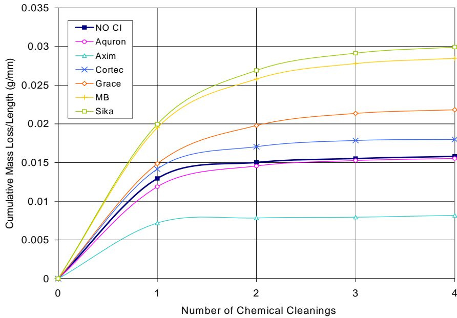
Figure F.9 – Cumulative Mass Loss/Length for Bath 2, 0.5% Chloride Pre-Cracked Specimens
