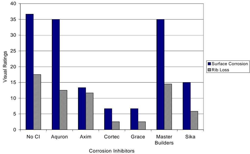
Figure G.67 – Visual Ratings for Chamber Shelf 2, 1.5% Chloride, Pre-Cracked
