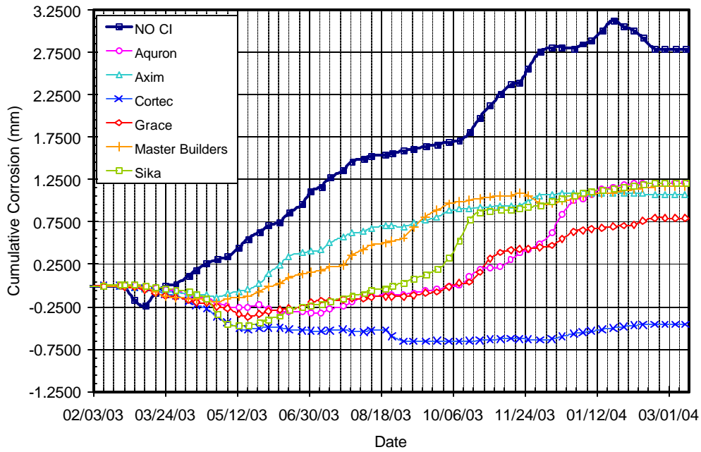
Figure B.9 – Cumulative Corrosion Over Time for Bath 2, 0.0% Chloride, Pre-Cracked
