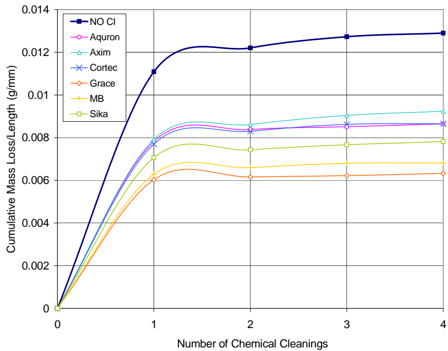
Figure F.37 – Cumulative Mass Loss/Length for Chamber Shelf 2 3.0% Chloride, Pre-Cracked Specimens
