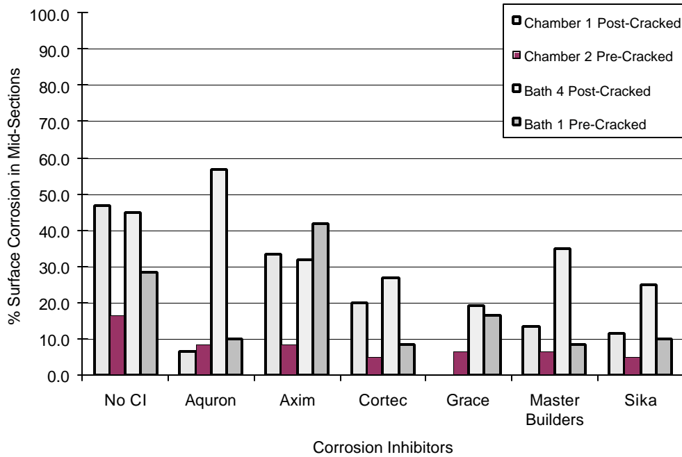
Figure 4.21 - % Surface Corrosion at Midsection for 0.0% Chloride (Set #1)
