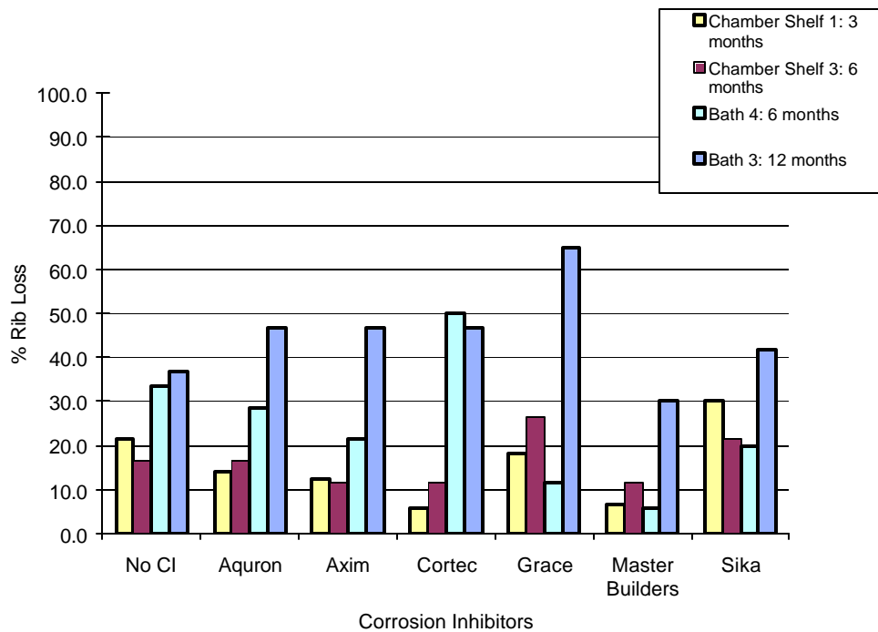
Figure E.50 Time Step of Rib Loss for 2.0% Chloride Post-Cracked Specimens
