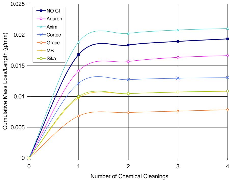
Figure F.3 – Cumulative Mass Loss/Length for Bath 1, 0.5% Chloride Pre-Cracked Specimens
