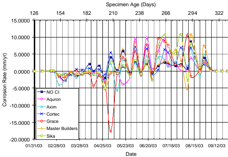
Figure A.22 – Corrosion Rate for Bath 4, 0.5% Chloride, Post-Cracked
