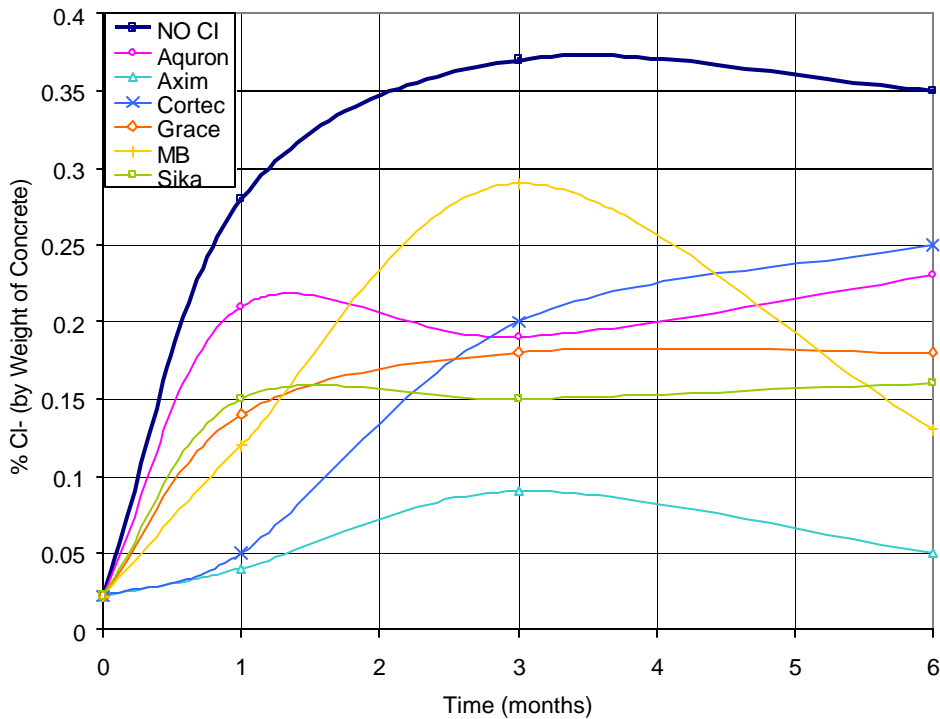
Figure 4.16 - Chloride Content for Chamber Specimens – 0.0% Chloride
