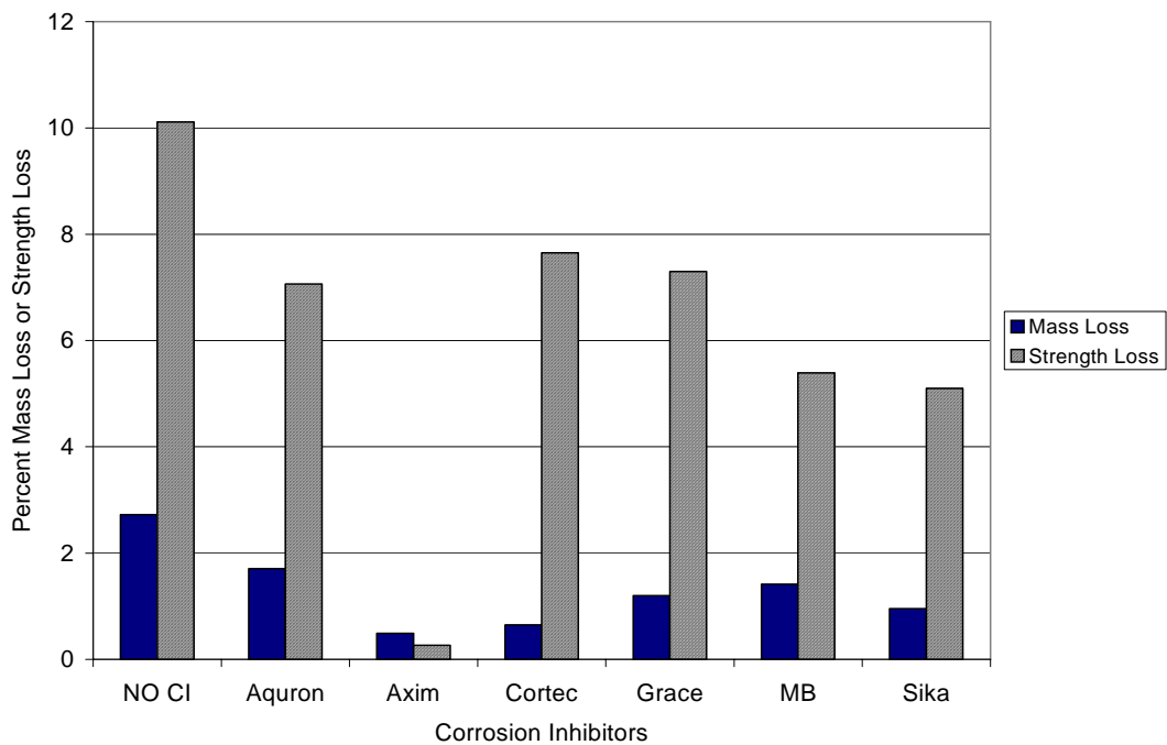
Figure G.64 – Mass Loss and Strength Loss for Chamber Shelf 2, 0.5% Chloride, Pre-Cracked
