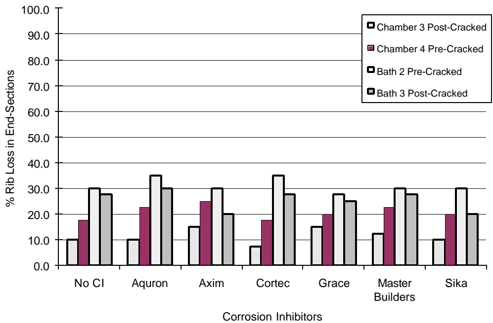
Figure 4.20 - % Rib Loss at End Sections for 1.0% Chloride (Set #2)
