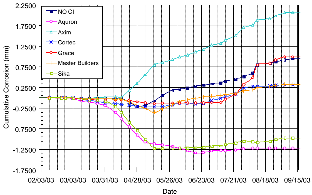
Figure B.21 – Cumulative Corrosion Over Time for Bath 4, 0.0% Chloride, Post-Cracked
