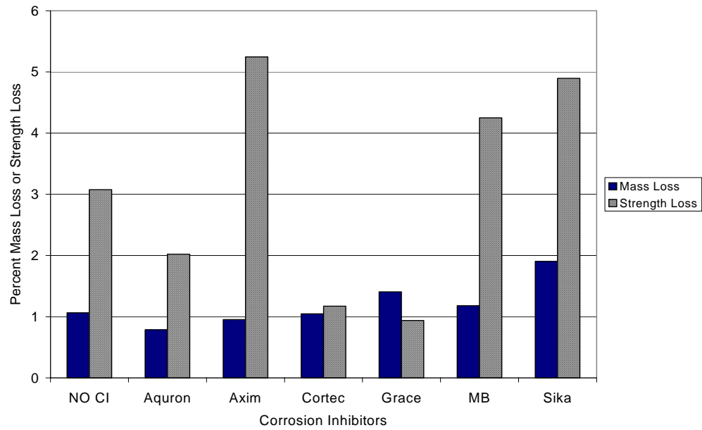
Figure G.54 – Mass Loss and Strength Loss for Chamber Shelf 1, 1.0% Chloride, Post-Cracked
