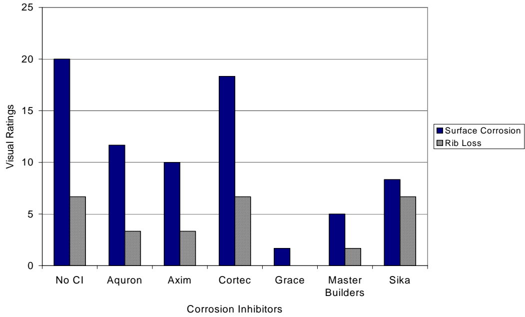
Figure G.73 – Visual Ratings for Chamber Shelf 3, 0.0% Chloride, Post-Cracked
