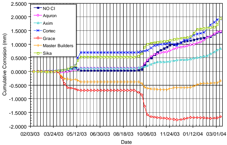
Figure B.39 – Cumulative Corrosion Over Time for Chamber Shelf 3, 0.0% Chloride, Post-Cracked
