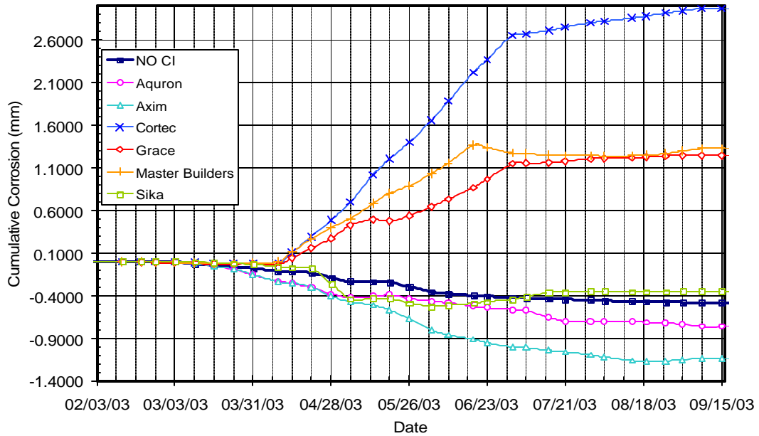
Figure B.4 – Cumulative Corrosion Over Time for Bath 1, 0.5% Chloride, Pre-Cracked
