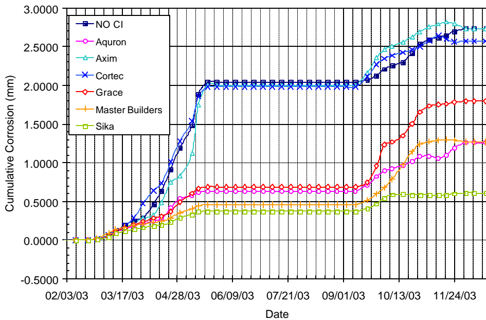
Figure B.38 – Cumulative Corrosion Over Time for Chamber Shelf 2, 3.0% Chloride, Pre-Cracked
