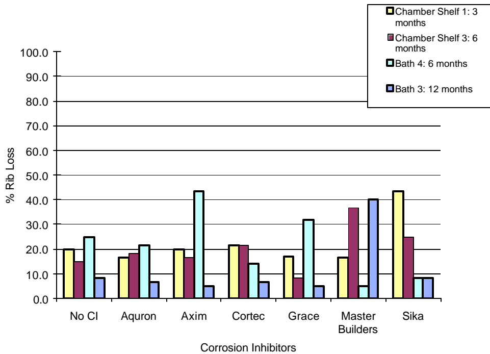
Figure E.52 Time Step of Rib Loss for 3.0% Chloride Post-Cracked Specimens
