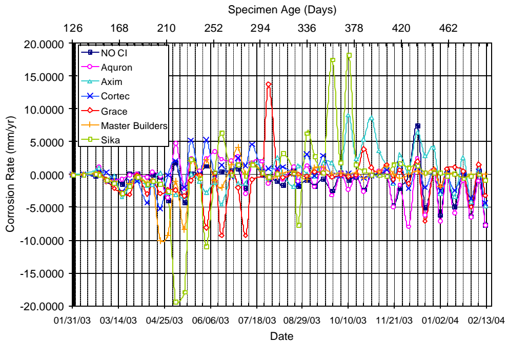
Figure A.12 – Corrosion Rate for Bath 2, 1.5% Chloride, Pre-Cracked
