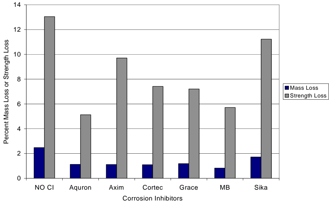
Figure G.76 – Mass Loss and Strength Loss for Chamber Shelf 3, 0.5% Chloride, Post-Cracked
