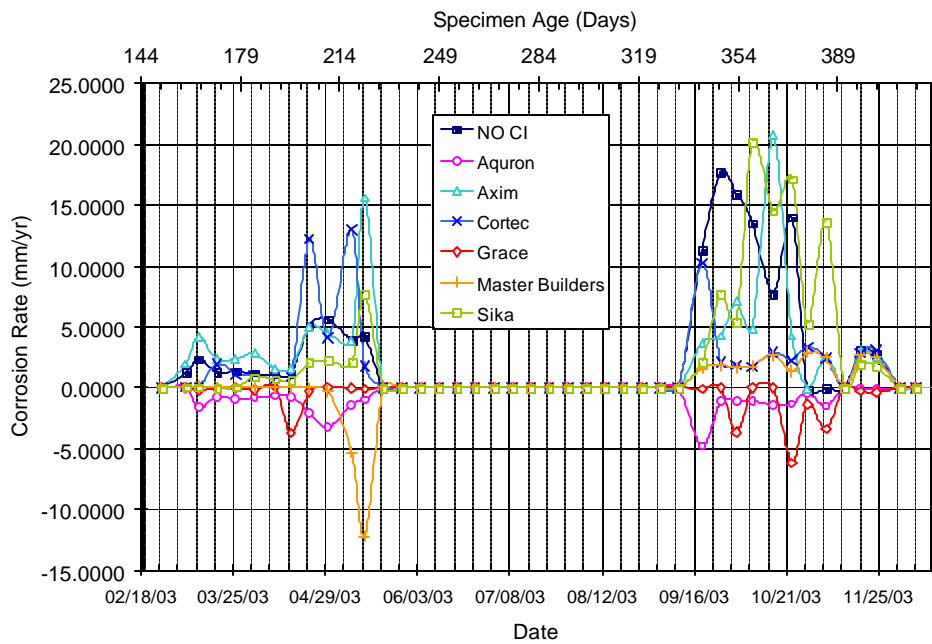
Figure A.27 – Corrosion Rate for Chamber Shelf 1, 0.0% Chloride, Post-Cracked
