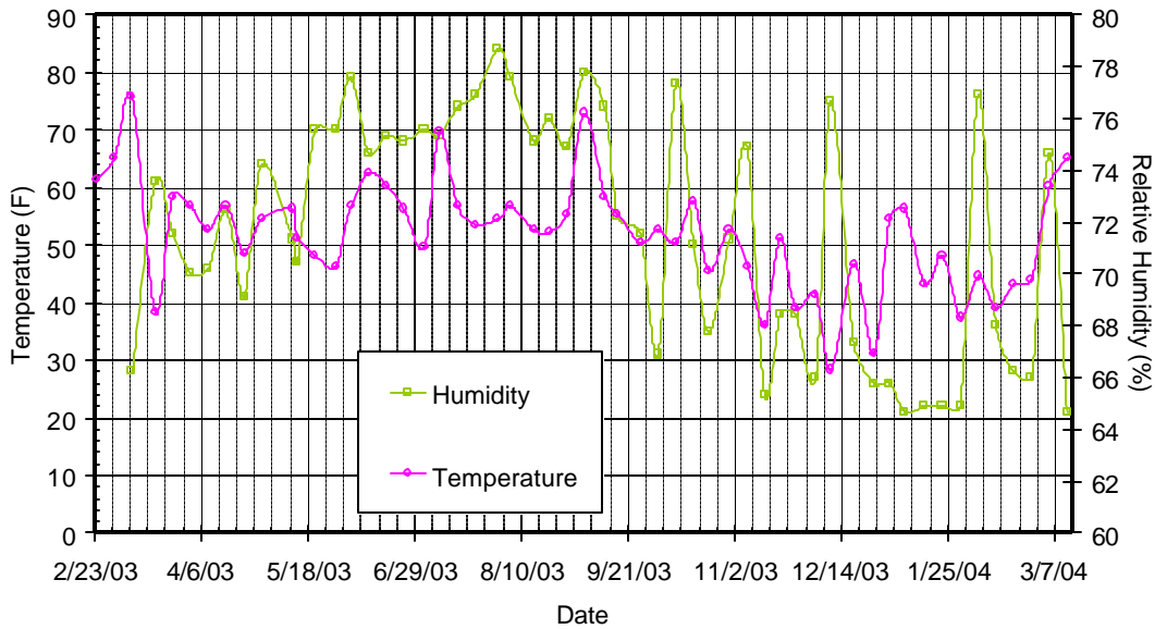
Figure 4.13 - Humidity and Temperature Over Time for Control Environment
