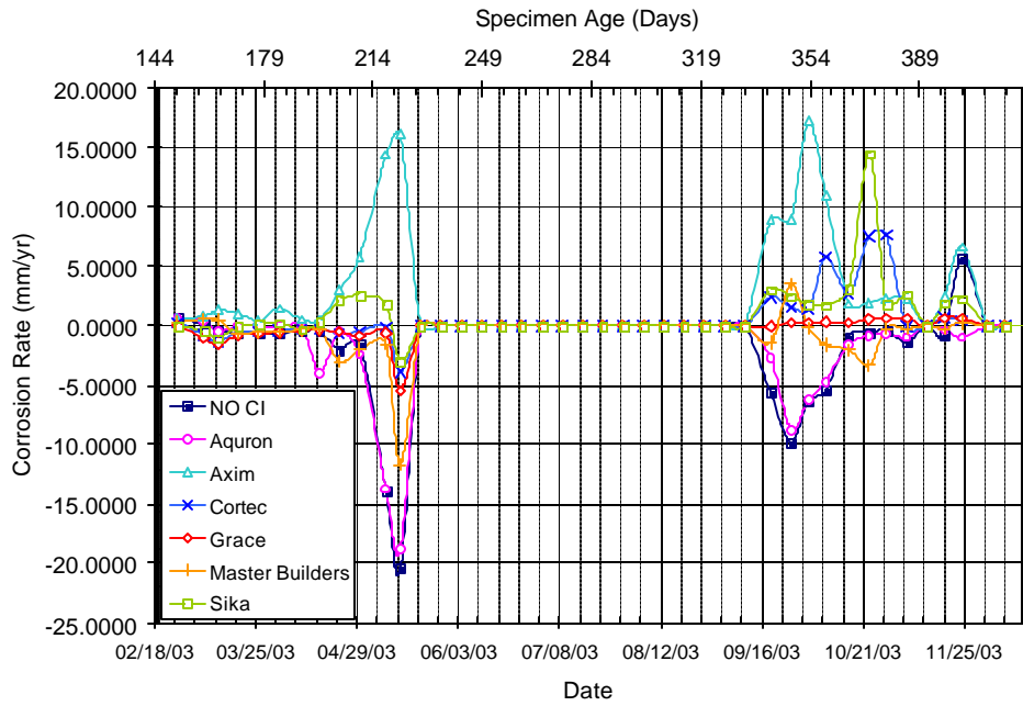
Figure A.35 – Corrosion Rate for Chamber Shelf 2, 1.0% Chloride, Pre-Cracked
