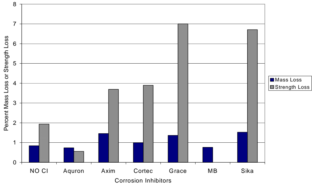
Figure G.90 – Mass Loss and Strength Loss for Chamber Shelf 4, 1.0% Chloride, Pre-Cracked
