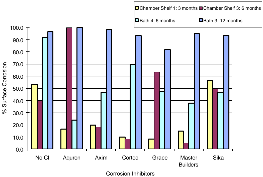
Figure E.47 Time Step of Surface Corrosion for 1.5% Chloride Post-Cracked Specimens
