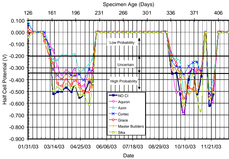
Figure C.33 – Half Cell Potential Readings for Chamber Shelf 2, 0.0% Chloride, Pre-Cracked
