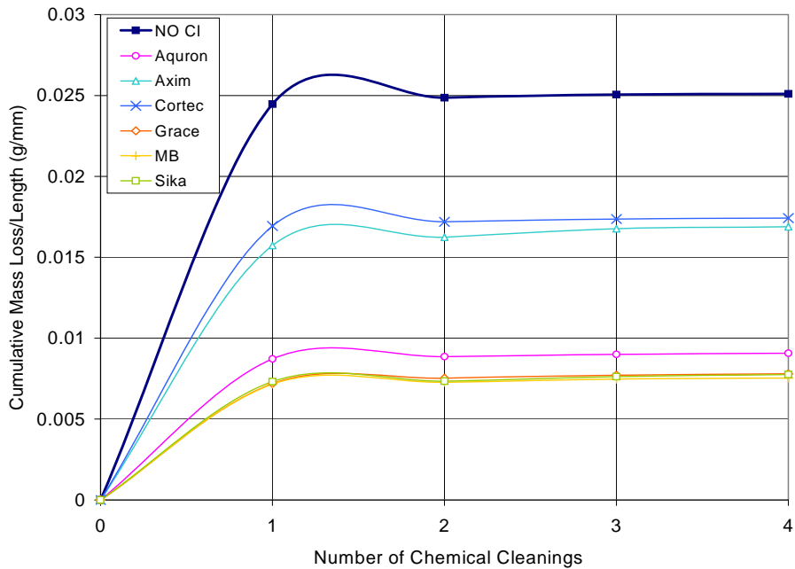
Figure F.2 – Cumulative Mass Loss/Length for Bath 1, 0.0% Chloride Pre-Cracked Specimens
