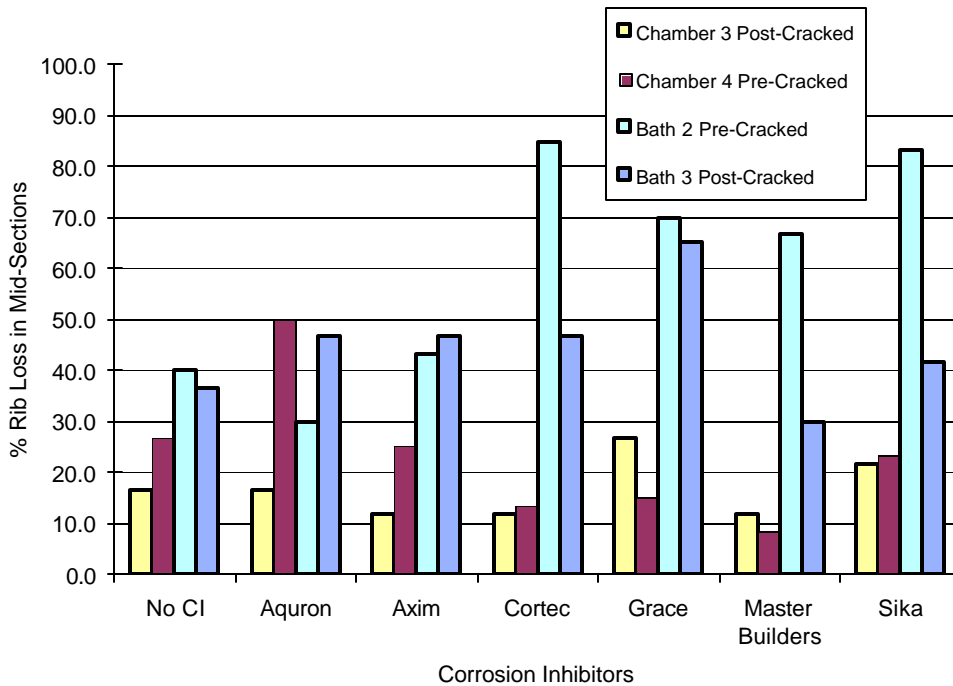
Figure E.24 Rib Loss at Mid Section for 2.0% Chloride (Set #2)
