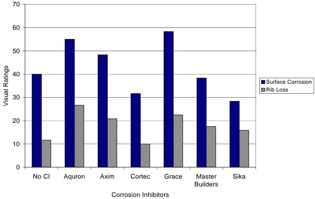
Figure G.71 – Visual Ratings for Chamber Shelf 2, 3.0% Chloride, Pre-Cracked
