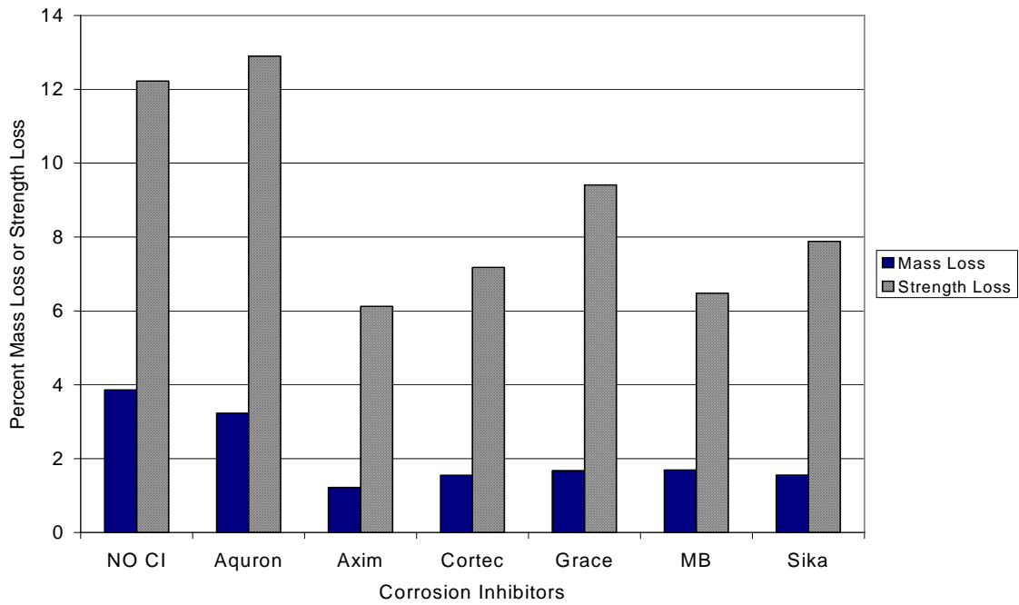
Figure G.28 – Mass Loss and Strength Loss for Bath 3, 0.5% Chloride, Post-Cracked
