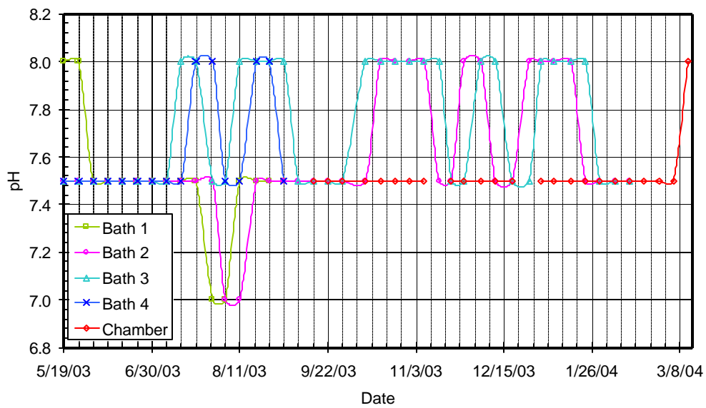
Figure 4.11 - pH Over Time for Bath and Chamber Environments
