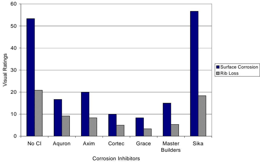
Figure G.55 – Visual Ratings for Chamber Shelf 1, 1.5% Chloride, Post-Cracked
