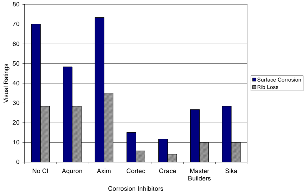
Figure G.5 – Visual Ratings for Bath 1, 1.0% Chloride, Pre-Cracked
