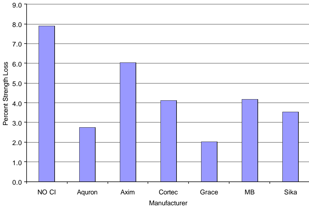
Figure 4.40 – Percent Strength Loss Based on Tension Tests for Chamber 0.5% Chloride, Shelf 4, Pre-Cracked
