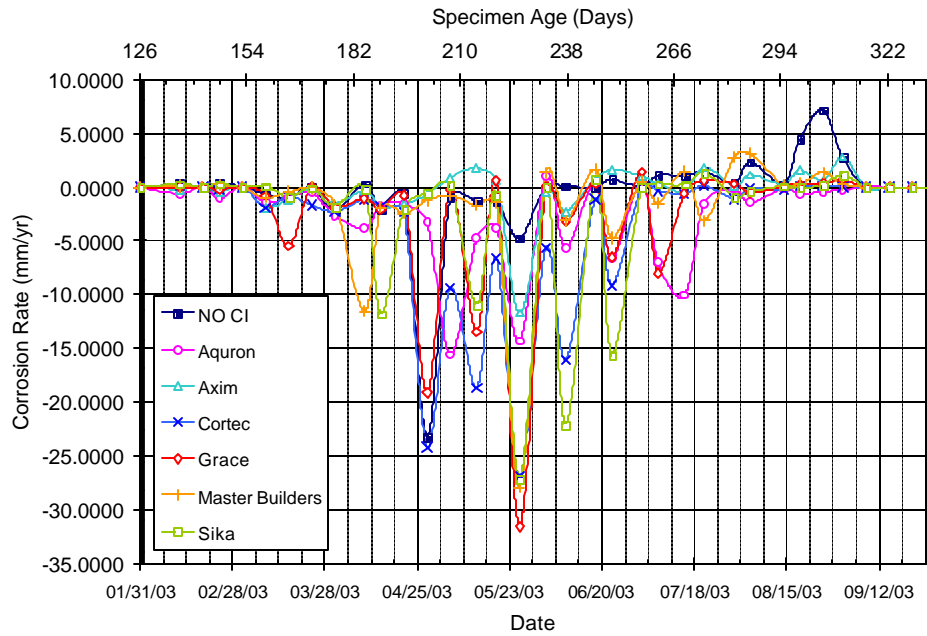
Figure A.3 – Corrosion Rate for Bath 1, 0.0% Chloride, Pre-Cracked
