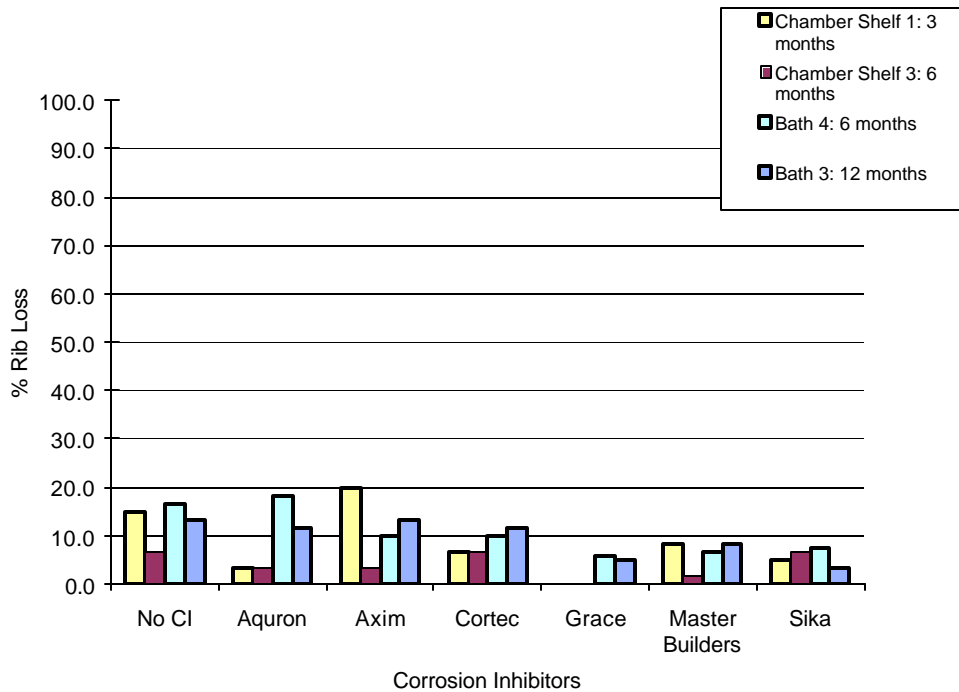
Figure E.42 Time Step of Rib Loss for 0.0% Chloride Post-Cracked Specimens
