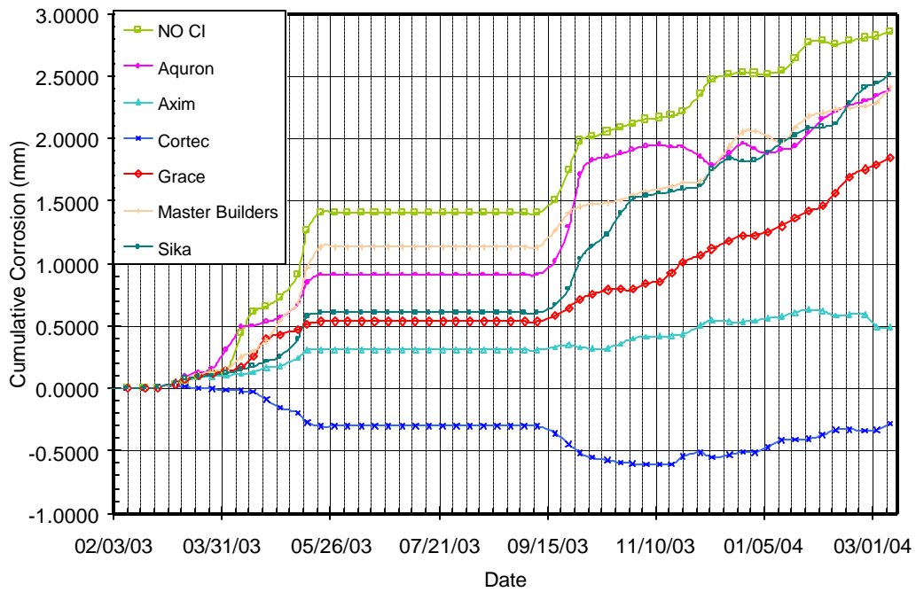
Figure 4.6 - Cumulative Corrosion Over Time for Chamber Shelf 3, 2.0% Chloride, Post-Cracked
