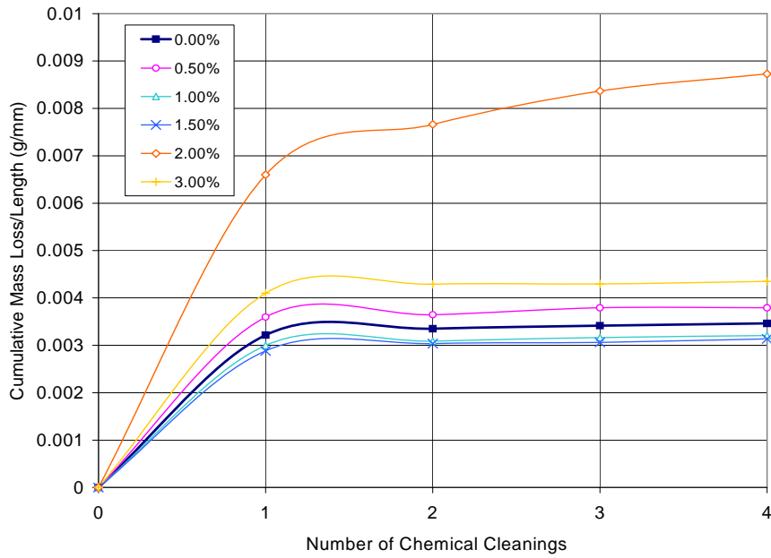
Figure F.1 – Cumulative Mass Loss/Length for Control Specimens
