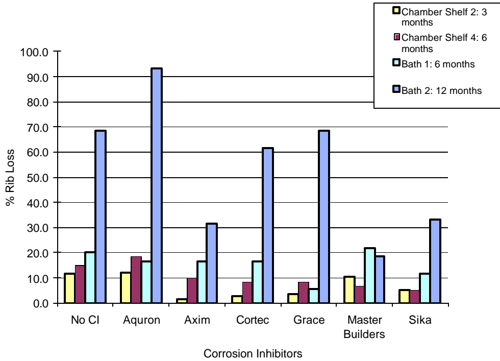
Figure E.32 Time Step of Rib Loss for 0.5% Chloride Pre-Cracked Specimens
