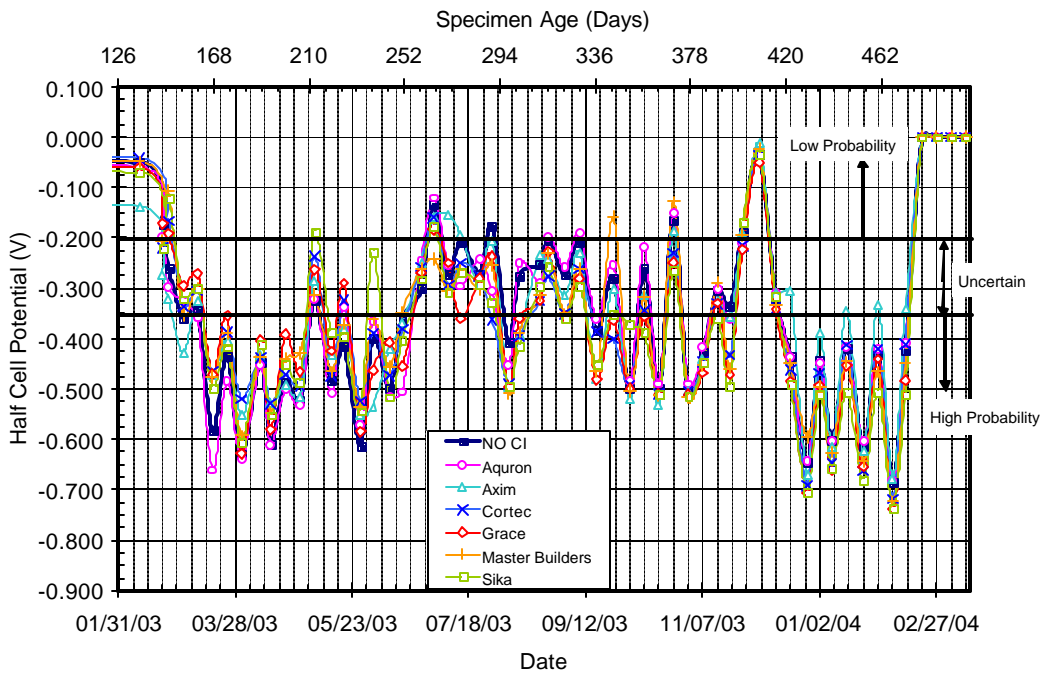
Figure C.12 – Half Cell Potential Readings for Bath 2, 1.5% Chloride, Pre-Cracked
