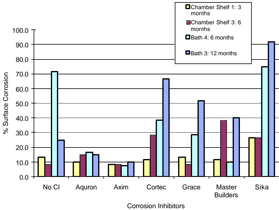
Figure E.45 Time Step of Surface Corrosion for 1.0% Chloride Post-Cracked Specimens
