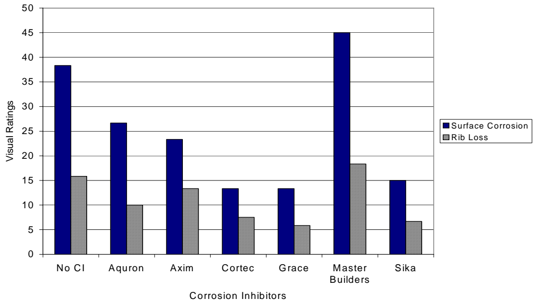
Figure G.69– Visual Ratings for Chamber Shelf 2, 2.0% Chloride, Pre-Cracked
