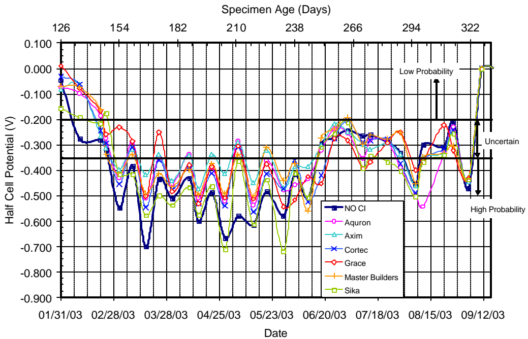
Figure C.24 – Half Cell Potential Readings for Bath 4, 1.5% Chloride, Post-Cracked
