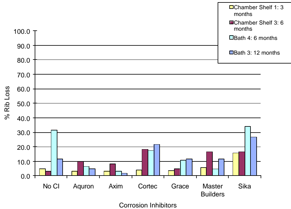
Figure E.46 Time Step of Rib Loss for 1.0% Chloride Post-Cracked Specimens
