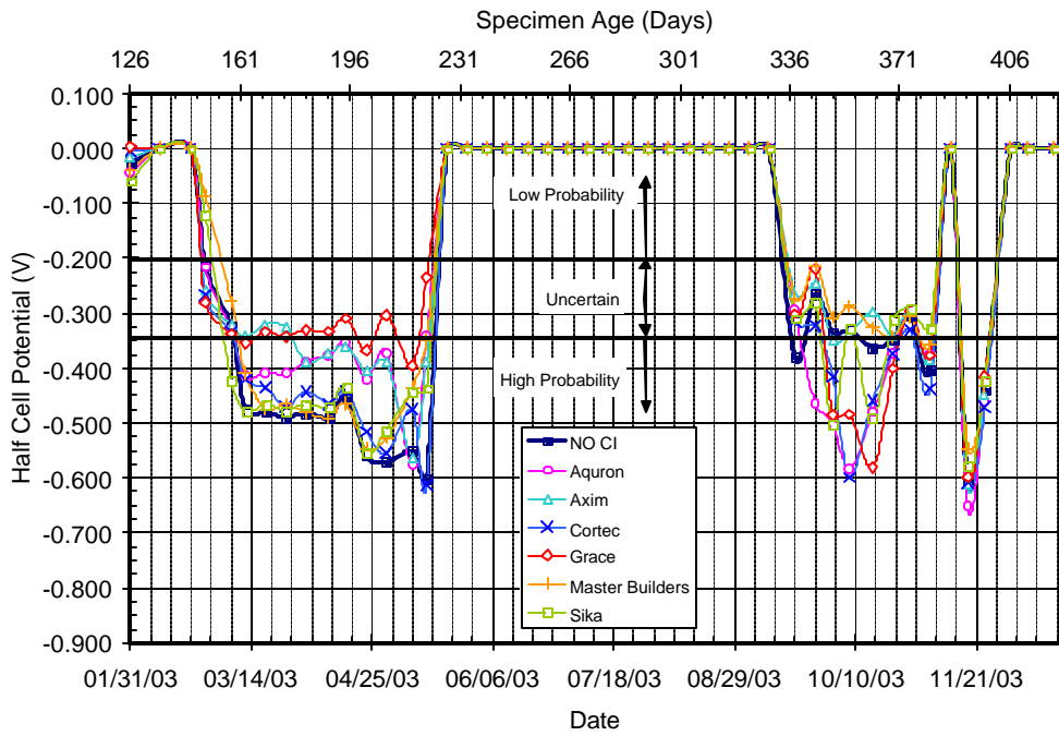
Figure C.29 – Half Cell Potential Readings for Chamber Shelf 1, 1.0% Chloride, Post-Cracked
