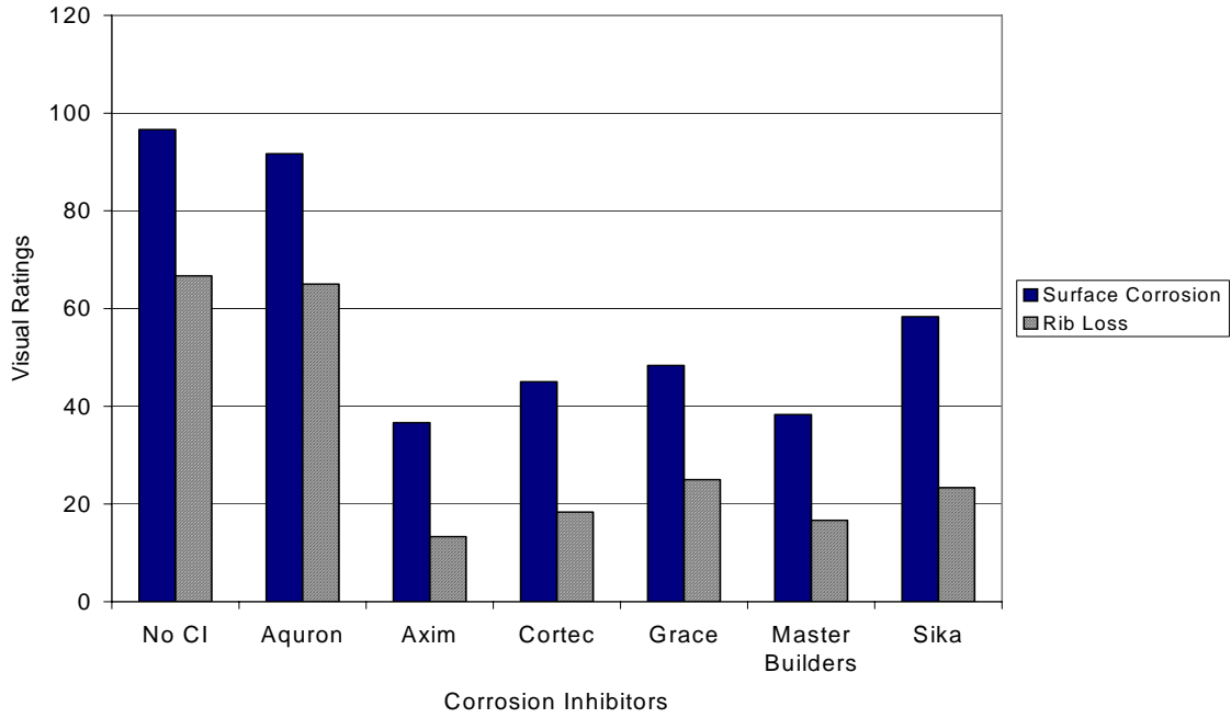
Figure G.27 – Visual Ratings for Bath 3, 0.5% Chloride, Post-Cracked
