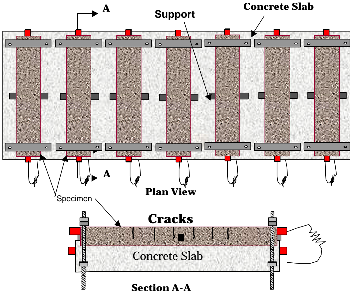
Figure 3.7 – Test Setup
