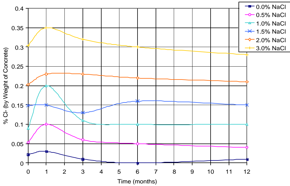
Figure D.1 – Chloride Content for Control Specimens
