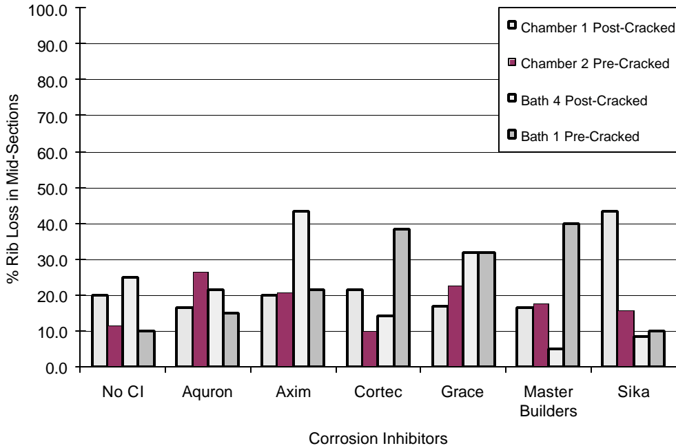
Figure 4.30 - % Rib Loss in Midsections for 3.0% Chloride (Set #1)
