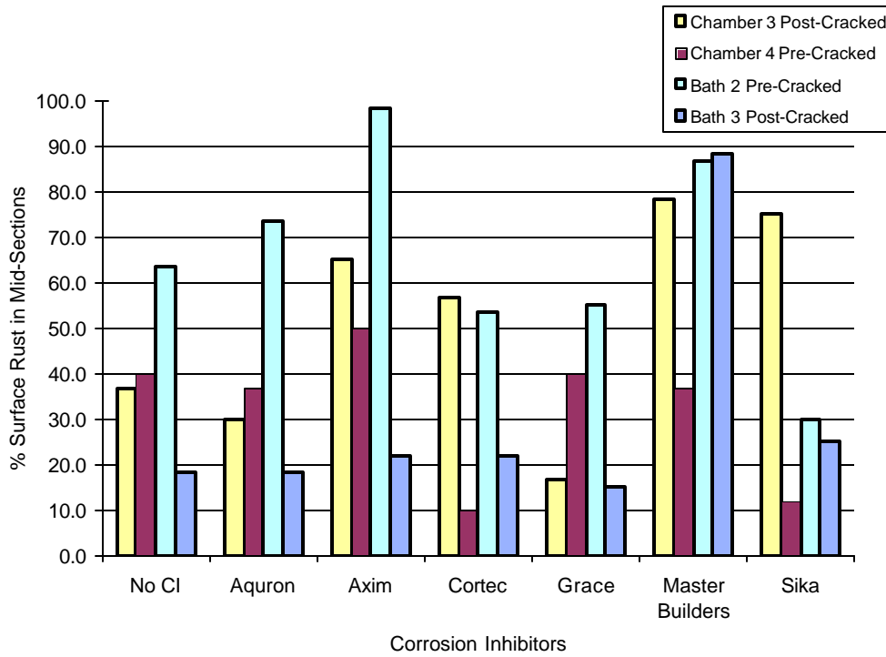
Figure E.25 Surface Corrosion at Mid Section for 3.0% Chloride (Set#2)
