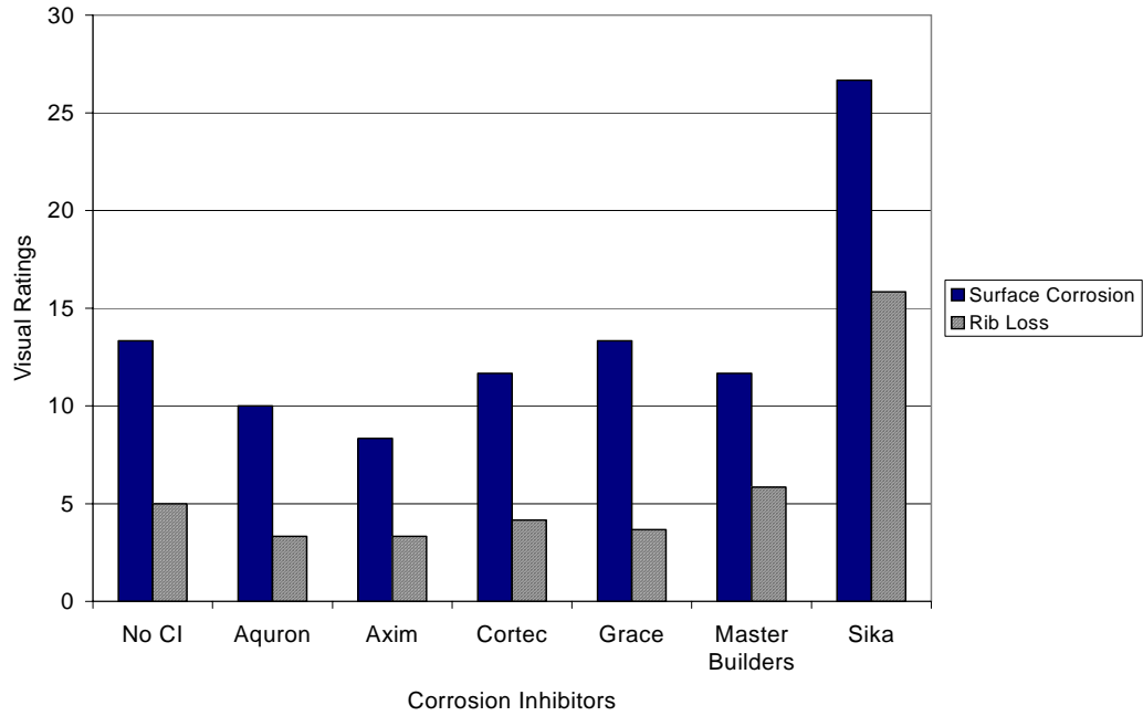
Figure G.53 – Visual Ratings for Chamber Shelf 1, 1.0% Chloride, Post-Cracked
