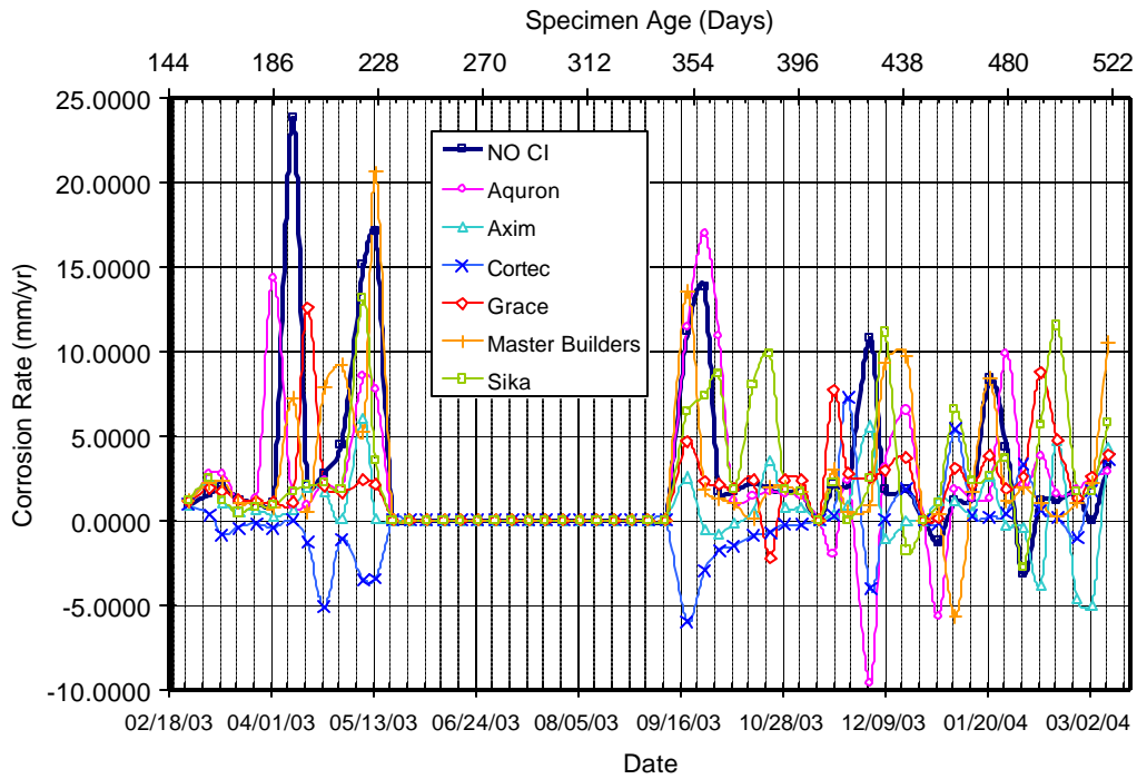
Figure 4.3 - Corrosion Rate for Chamber Shelf 3, 2.0% Chloride, Post-Cracked
