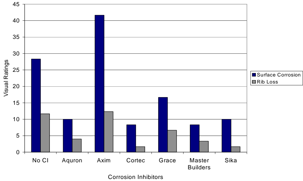
Figure G.1 – Visual Ratings for Bath 1, 0.0% Chloride, Pre-Cracked
