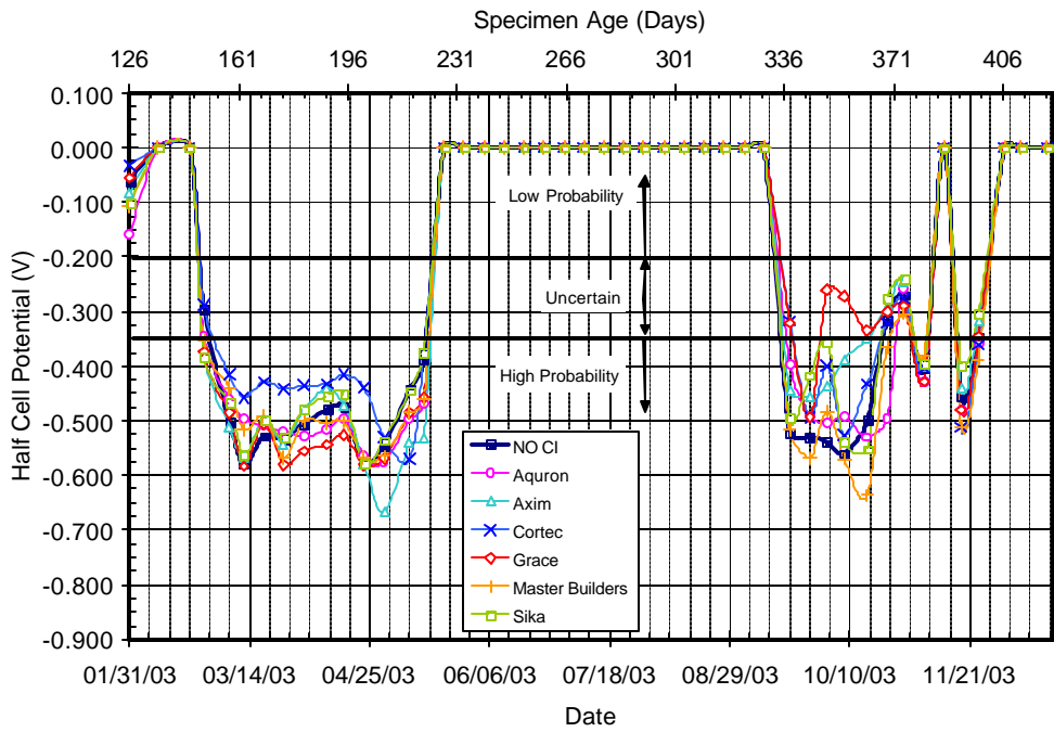
Figure C.31 – Half Cell Potential Readings for Chamber Shelf 1, 2.0% Chloride, Post-Cracked
