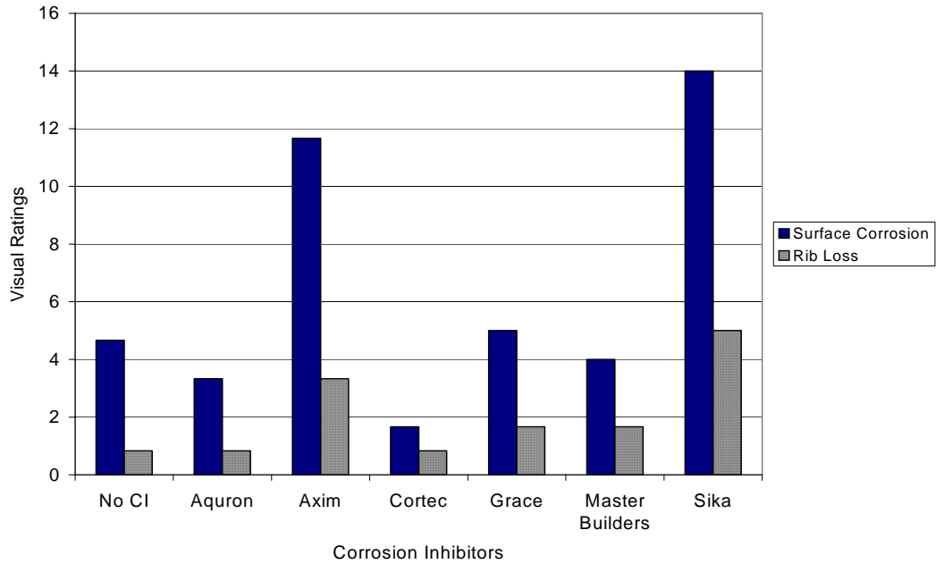
Figure G.65– Visual Ratings for Chamber Shelf 2, 1.0% Chloride, Pre-Cracked
