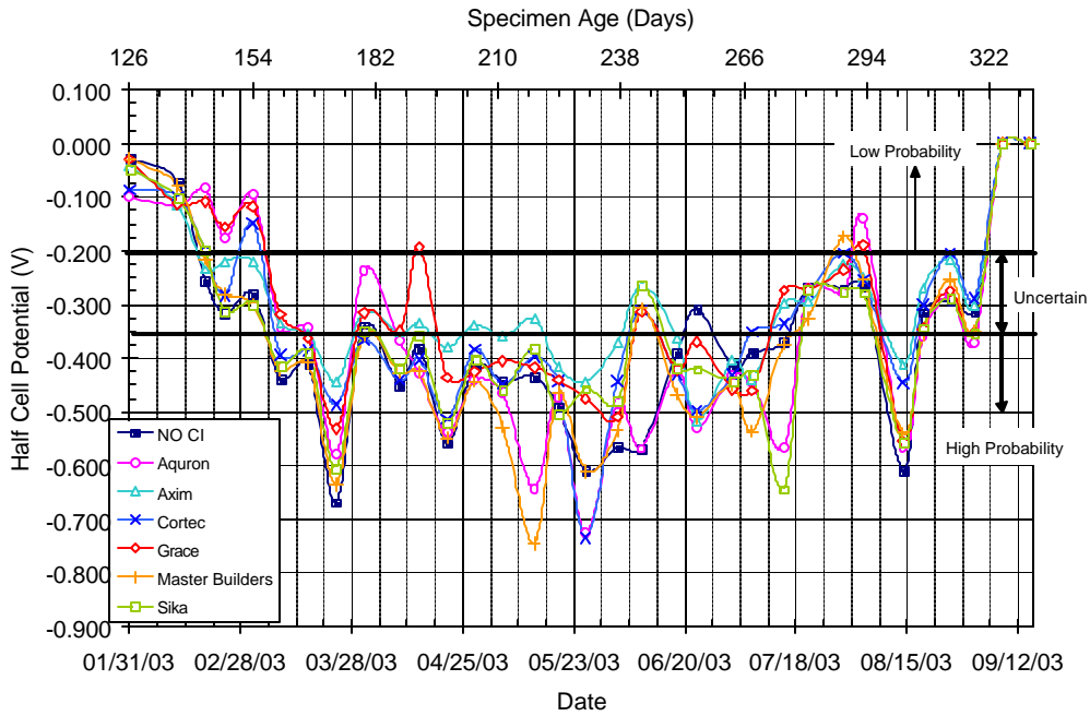
Figure C.7 – Half Cell Potential Readings for Bath 1, 2.0% Chloride, Pre-Cracked
