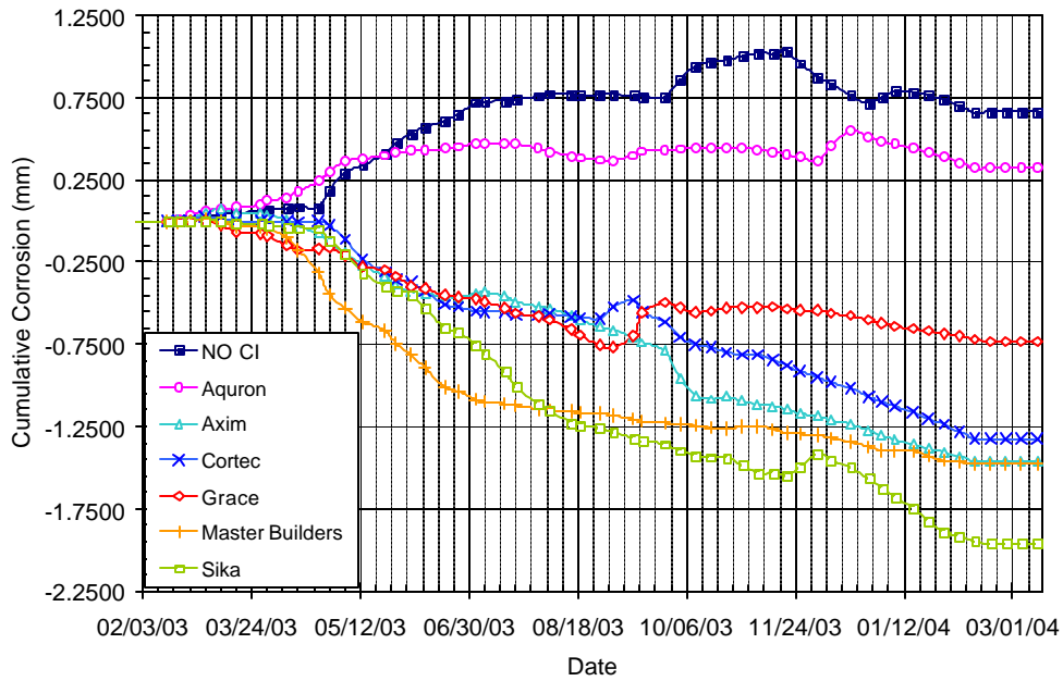
Figure B.19 – Cumulative Corrosion Over Time for Bath 3, 2.0% Chloride, Post-Cracked
