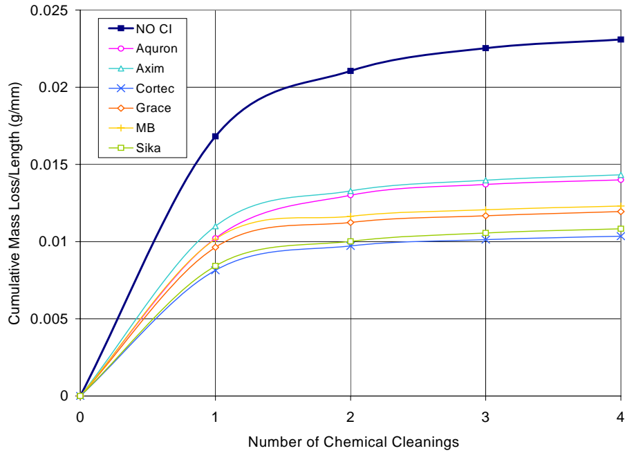
Figure F.21 – Cumulative Mass Loss/Length for Bath 4, 0.5% Chloride Post-Cracked Specimens
