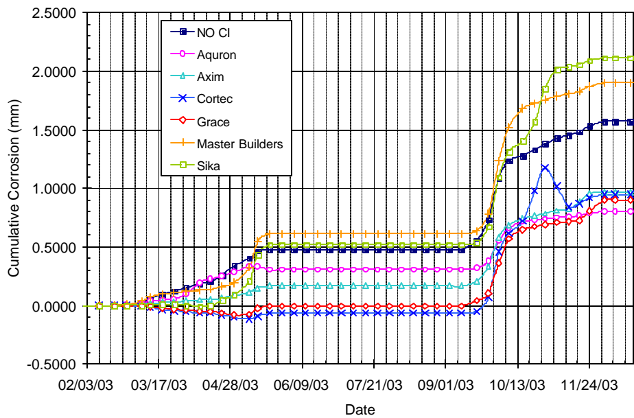
Figure B.36 – Cumulative Corrosion Over Time for Chamber Shelf 2, 1.5% Chloride, Pre-Cracked
