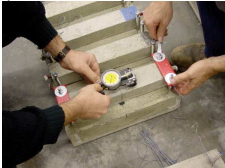
Figure 3.12 – Pilot Test 2: Using DEMEC Points and Dial Gauge
