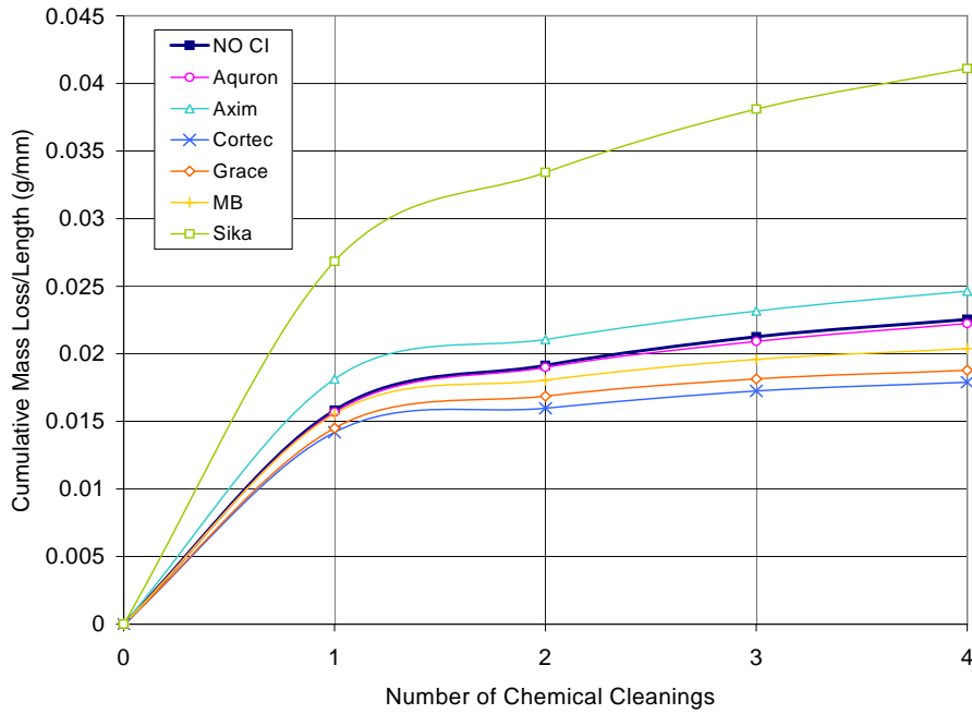
Figure F.31 – Cumulative Mass Loss/Length for Chamber Shelf 1 3.0% Chloride, Post-Cracked Specimens
