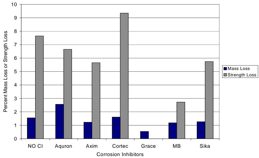
Figure G.92 – Mass Loss and Strength Loss for Chamber Shelf 4, 1.5% Chloride, Pre-Cracked
