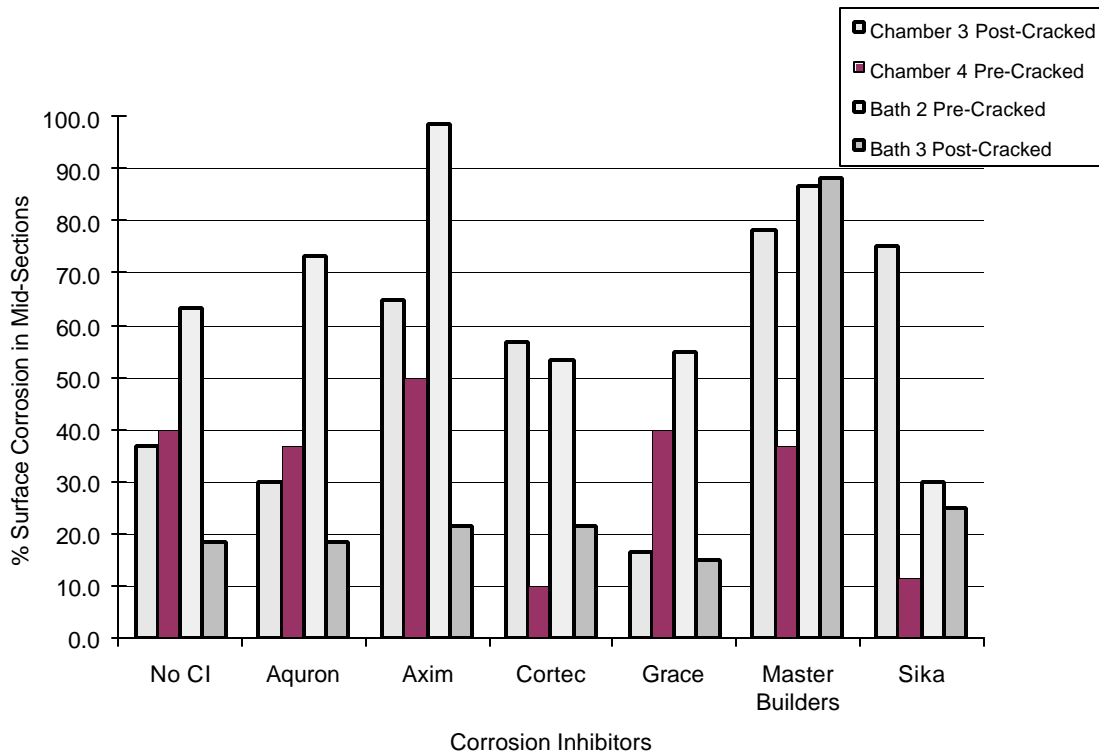
Figure 4.26 - % Surface Corrosion at Midsection for 3.0% Chloride (Set #2)
