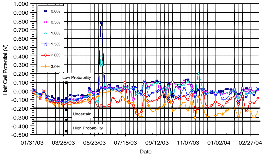
Figure C.1 – Half Cell Potential Readings for Control Set #1
