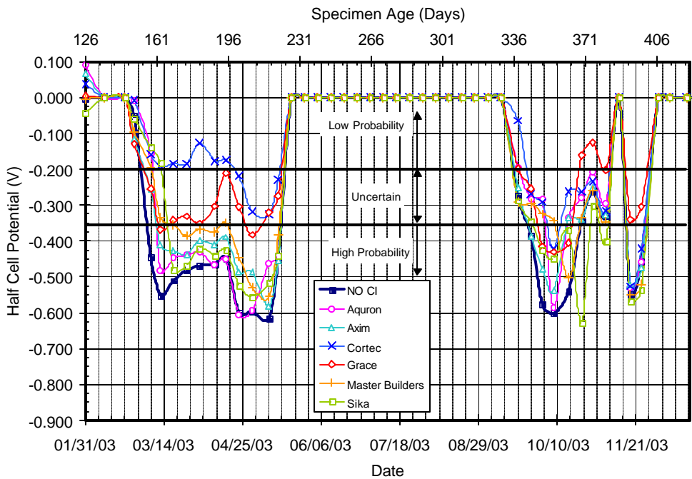
Figure C.28 – Half Cell Potential Readings for Chamber Shelf 1, 0.5% Chloride, Post-Cracked
