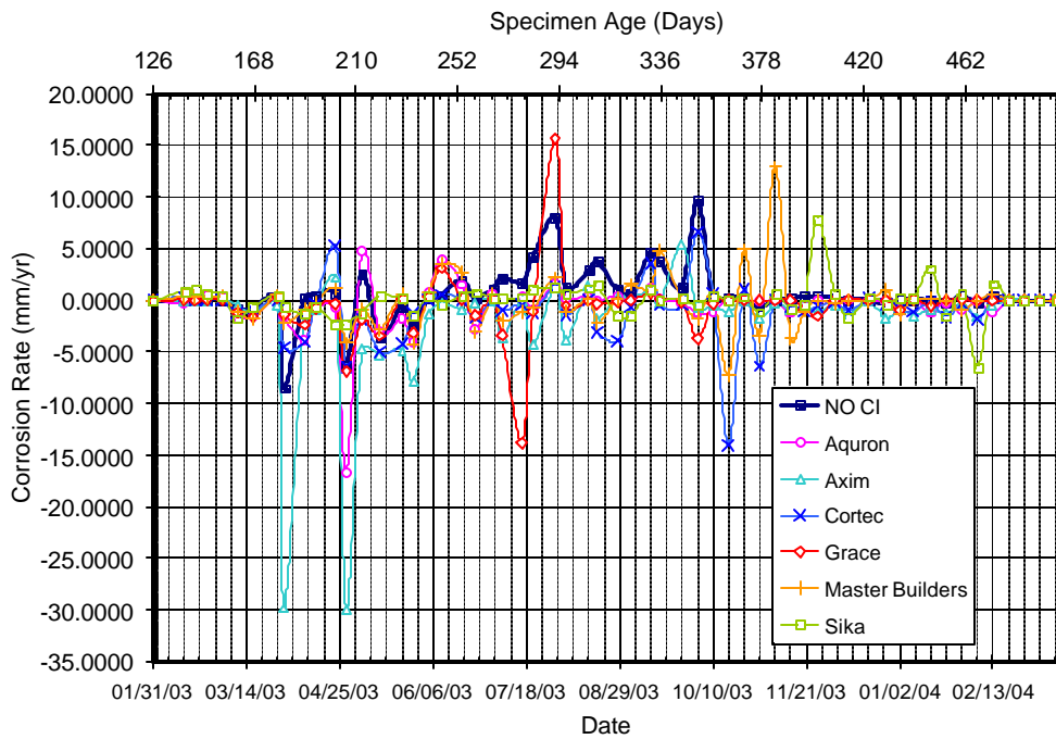
Figure A.17 – Corrosion Rate for Bath 3, 1.0% Chloride, Post-Cracked
