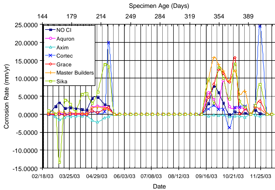
Figure A.34 – Corrosion Rate for Chamber Shelf 2, 0.5% Chloride, Pre-Cracked
