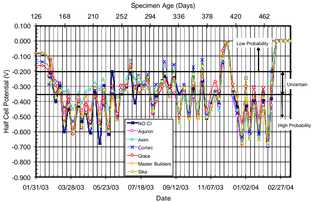
Figure C.13 – Half Cell Potential Readings for Bath 2, 2.0% Chloride, Pre-Cracked
