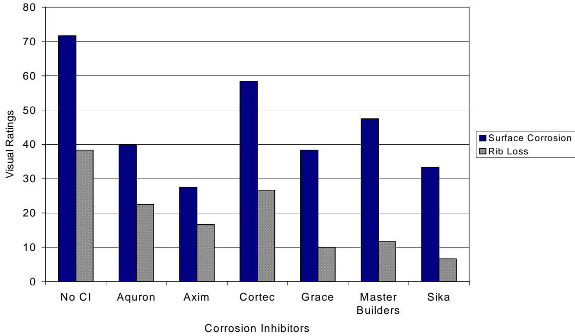
Figure G.39 – Visual Ratings for Bath 4, 0.5% Chloride, Post-Cracked
