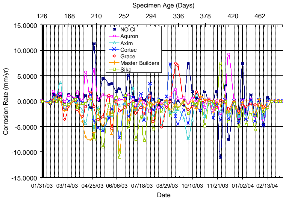
Figure A.19 – Corrosion Rate for Bath 3, 2.0% Chloride, Post-Cracked
