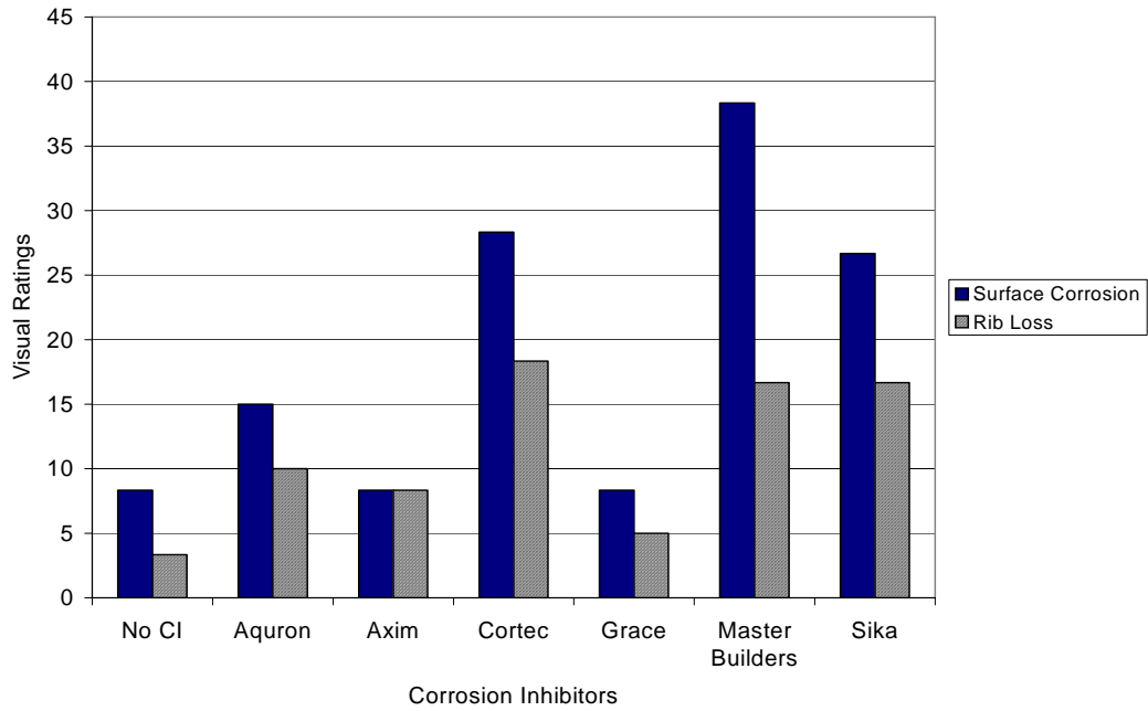
Figure G.77 – Visual Ratings for Chamber Shelf 3, 1.0% Chloride, Post-Cracked
