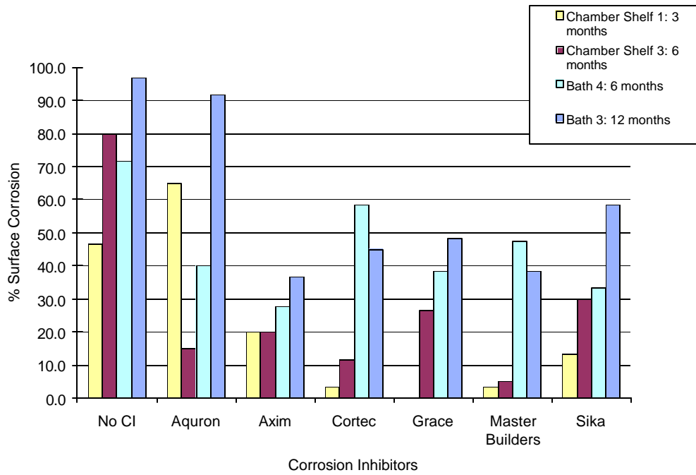
Figure E.43 Time Step of Surface Corrosion for 0.5% Chloride Post-Cracked Specimens
