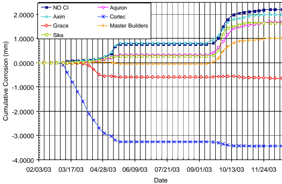
Figure B.28 – Cumulative Corrosion Over Time for Chamber Shelf 1, 0.5% Chloride, Post-Cracked
