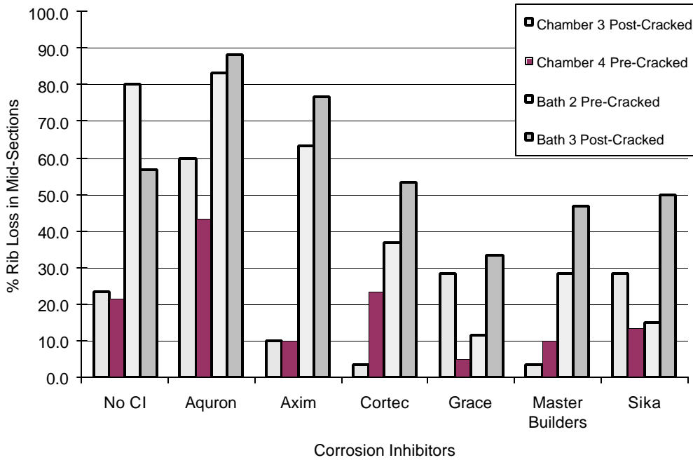
Figure 4.32 - % Rib Loss in Midsections for 1.5% Chloride (Set #2)
