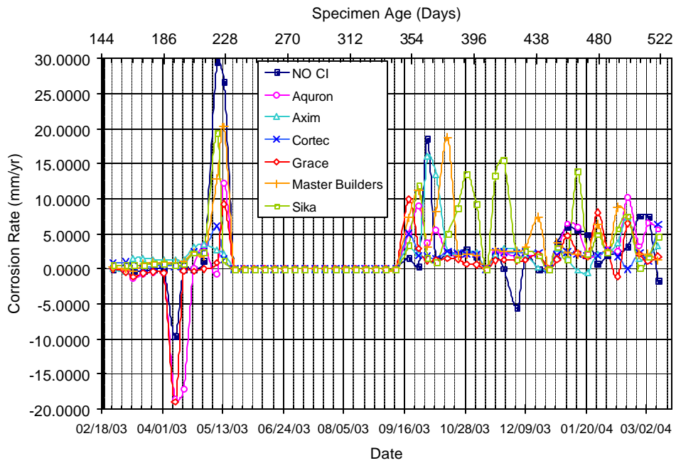
Figure A.41 – Corrosion Rate for Chamber Shelf 3, 1.0% Chloride, Post-Cracked
