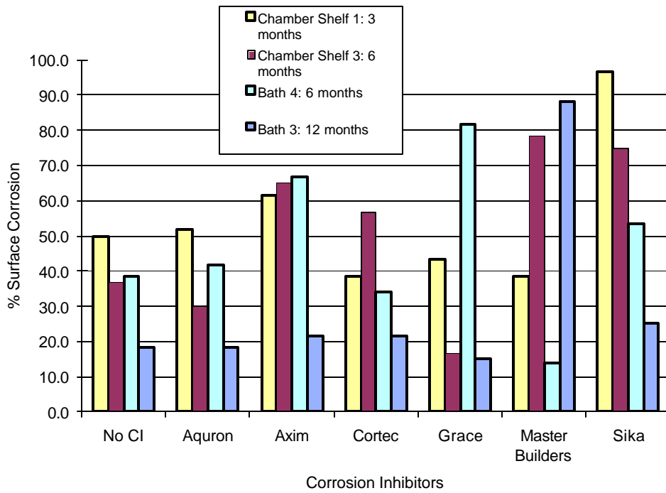
Figure E.51 Time Step of Surface Corrosion for 3.0% Chloride Post-Cracked Specimens
