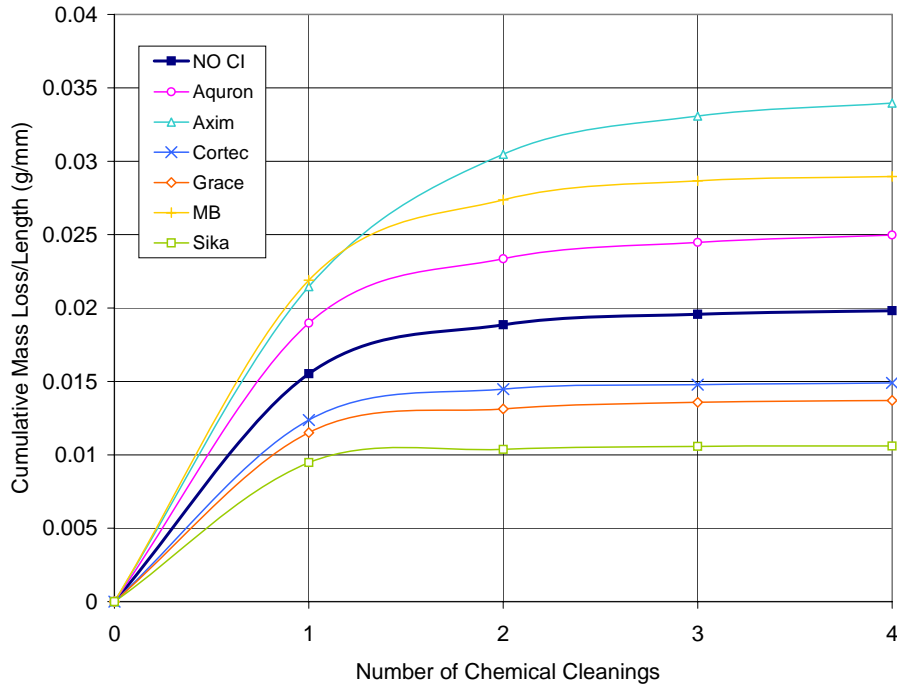
Figure F.13 – Cumulative Mass Loss/Length for Bath 2, 3.0% Chloride Pre-Cracked Specimens
