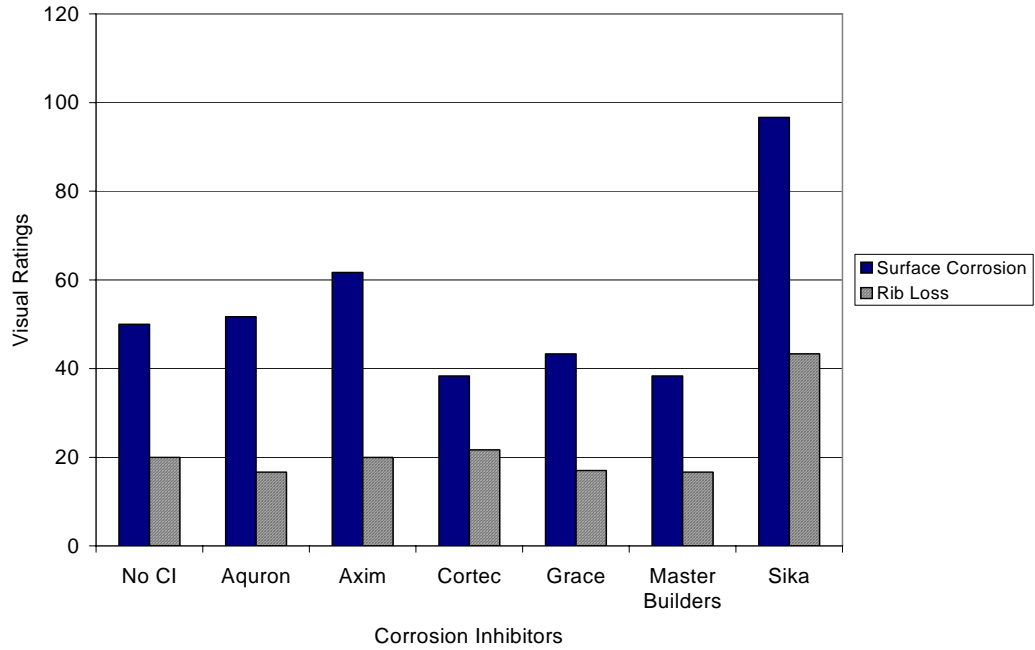
Figure G.59 – Visual Ratings for Chamber Shelf 1, 3.0% Chloride, Post-Cracked
