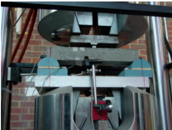
Figure 3.9 – Pilot Test Setup
