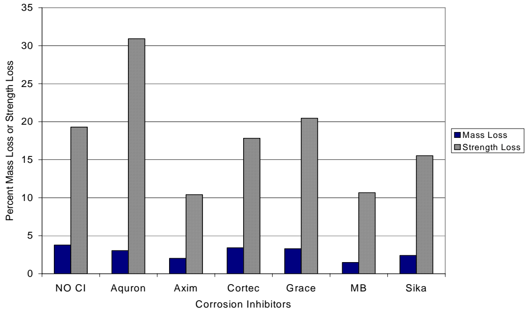
Figure G.16 – Mass Loss and Strength Loss for Bath 2, 0.5% Chloride, Pre-Cracked
