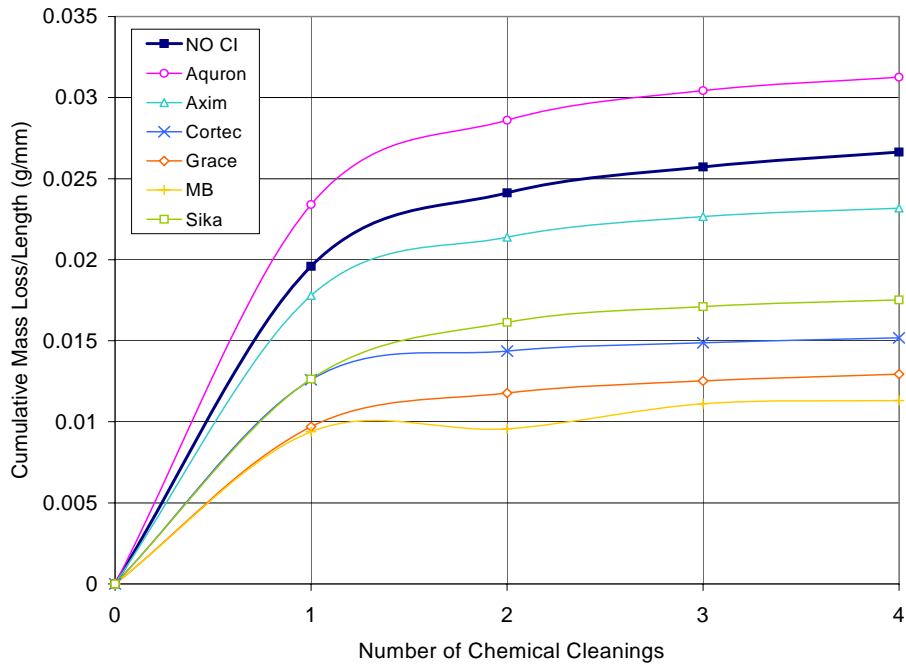
Figure F.47 – Cumulative Mass Loss/Length for Chamber Shelf 4 1.5% Chloride, Pre-Cracked Specimens
