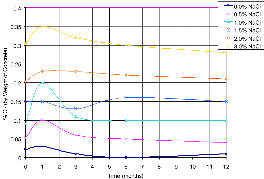
Figure 4.14 - Chloride Content for Control Specimens
