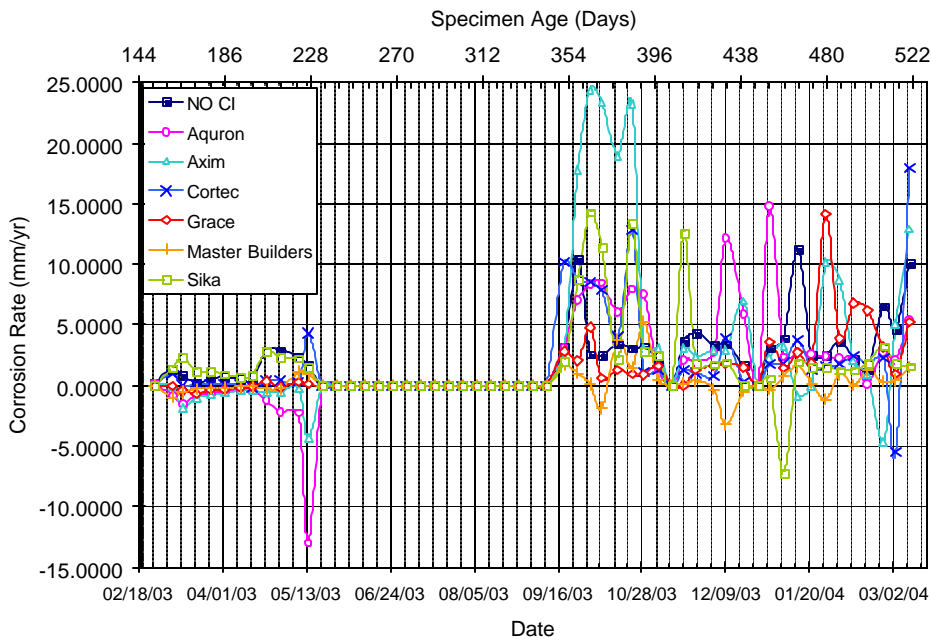
Figure A.40 – Corrosion Rate for Chamber Shelf 3, 0.5% Chloride, Post-Cracked
