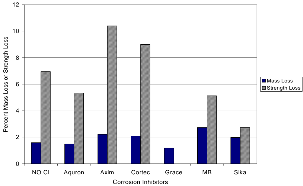
Figure G.84 – Mass Loss and Strength Loss for Chamber Shelf 3, 3.0% Chloride, Post-Cracked
