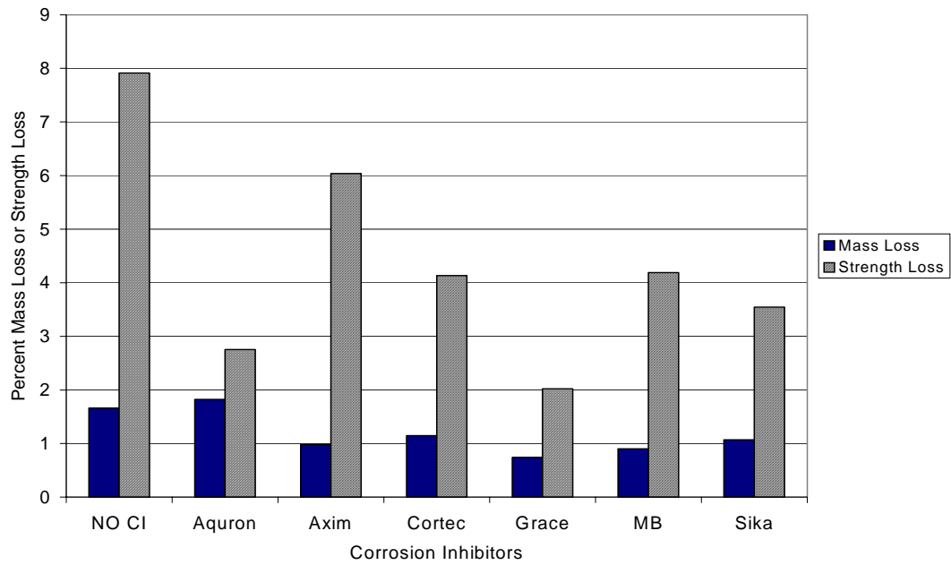
Figure G.88 – Mass Loss and Strength Loss for Chamber Shelf 4, 0.5% Chloride, Pre-Cracked
