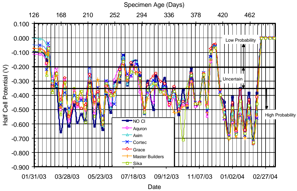
Figure C.9 – Half Cell Potential Readings for Bath 2, 0.0% Chloride, Pre-Cracked
