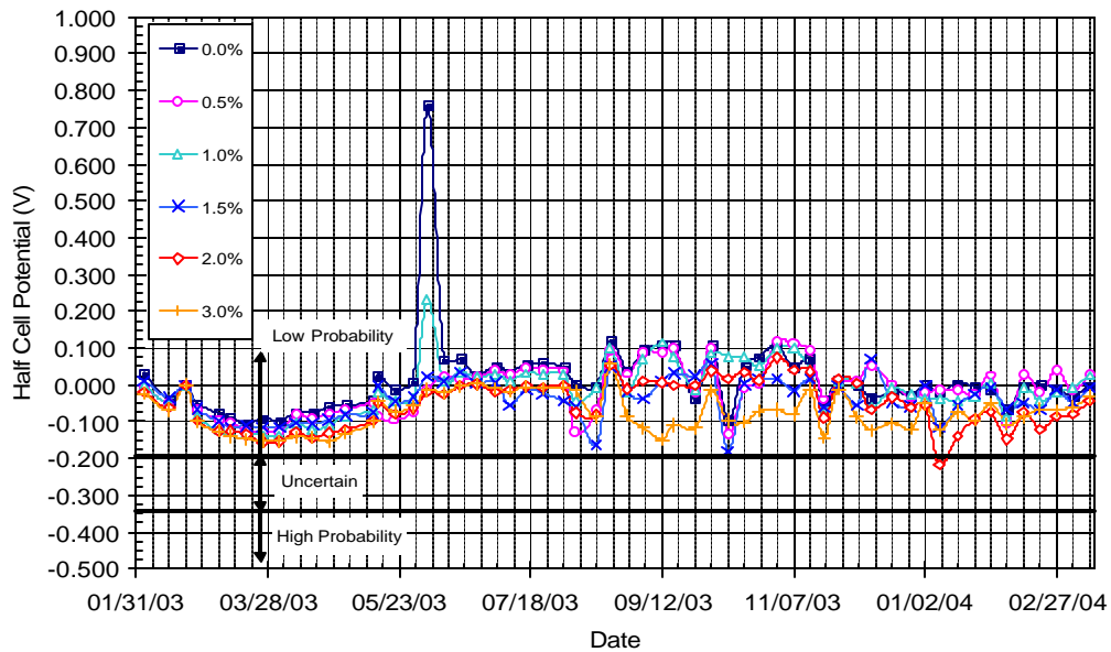
Figure C.2 – Half Cell Potential Readings for Control Set #2
