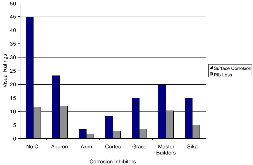
Figure 4.43 – Visual Ratings for Chamber 0.5% Chloride, Shelf 2, Pre-Cracked Specimens
