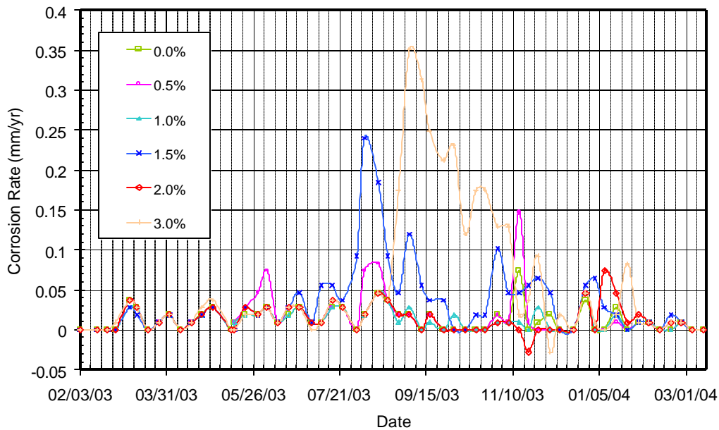
Figure 4.1 - Corrosion Rate for Control Specimens (Set #2)
