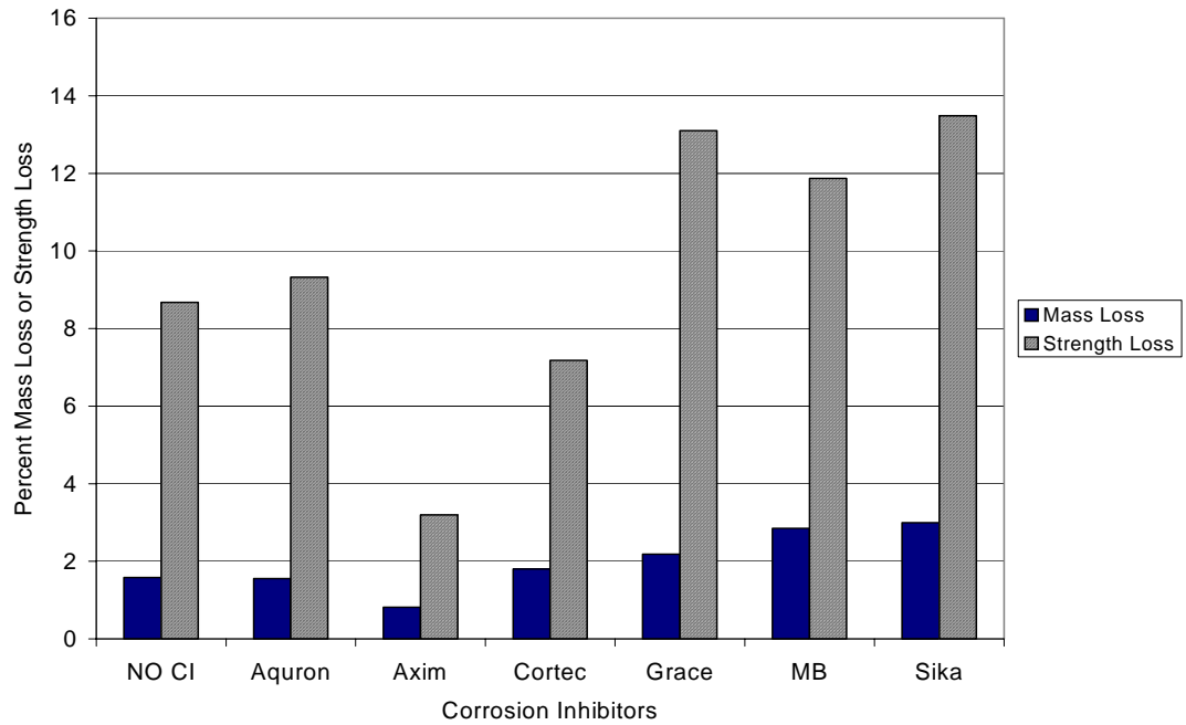
Figure G.18 – Mass Loss and Strength Loss for Bath 2, 1.0% Chloride, Pre-Cracked
