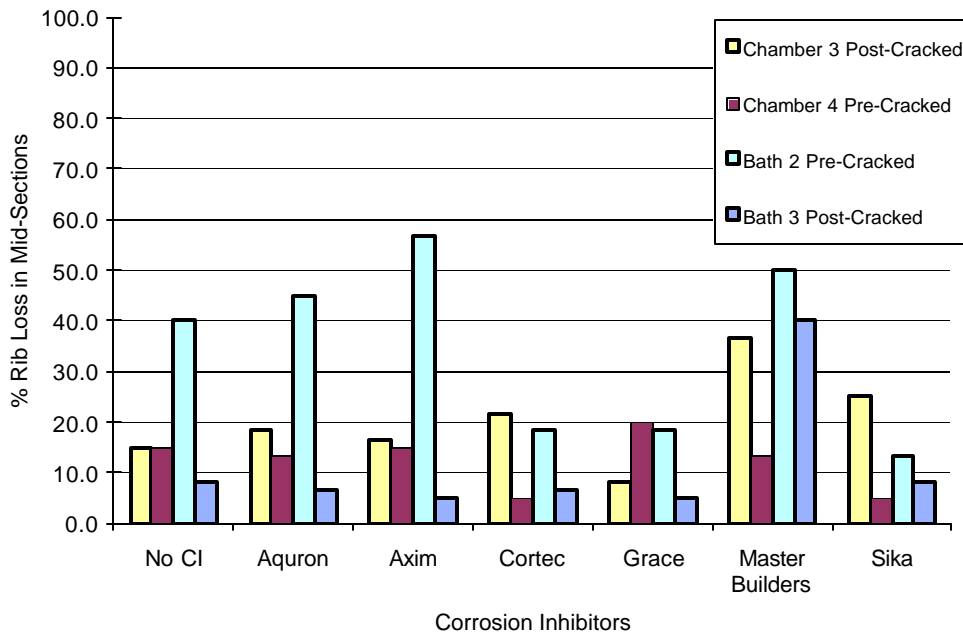
Figure E.26 Rib Loss at Mid Section for 3.0% Chloride (Set #2)
