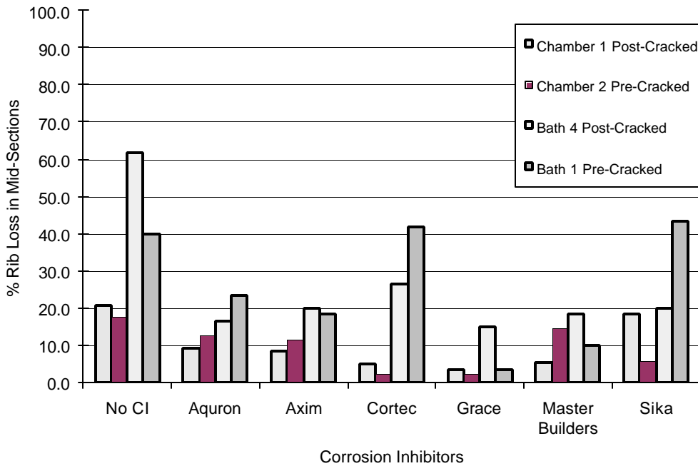
Figure 4.29 - % Rib Loss in Midsections for 1.5% Chloride (Set #1)
