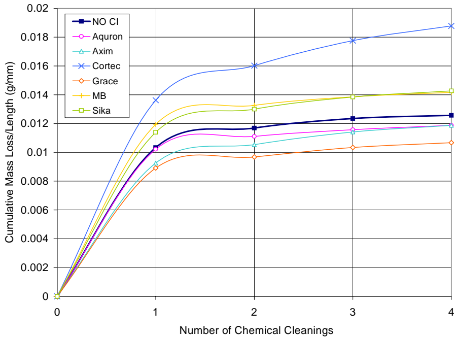
Figure F.39 – Cumulative Mass Loss/Length for Chamber Shelf 3 0.5% Chloride, Post-Cracked Specimens
