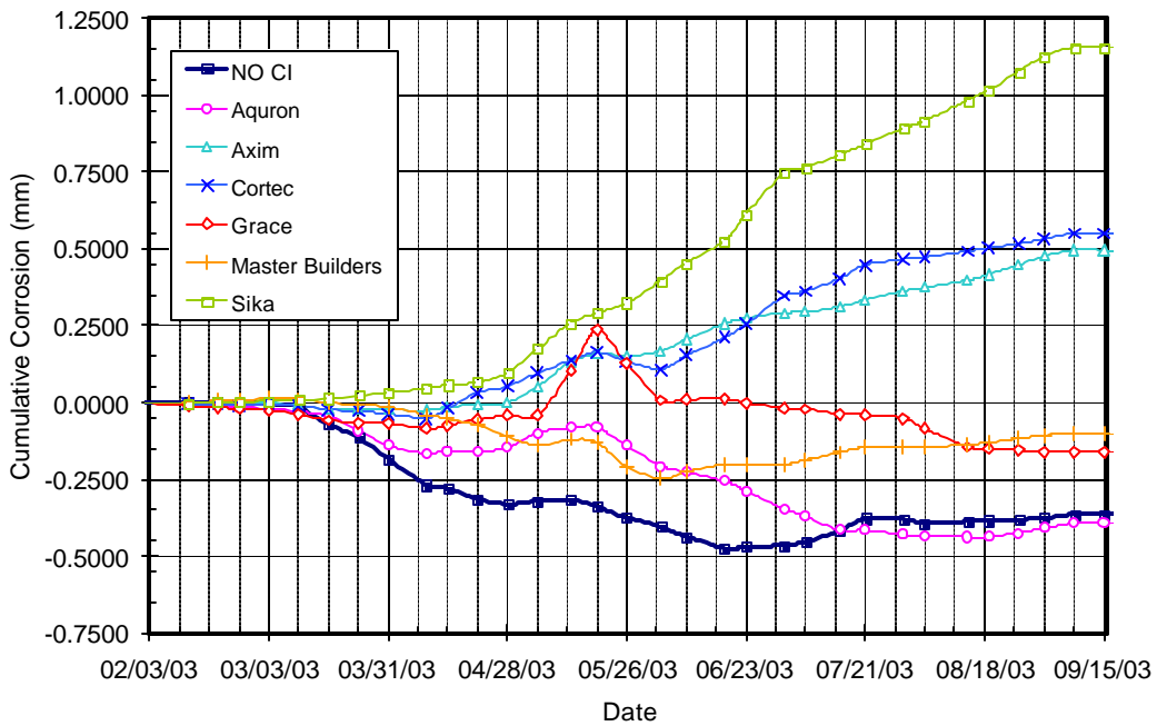
Figure B.6 – Cumulative Corrosion Over Time for Bath 1, 1.5% Chloride, Pre-Cracked
