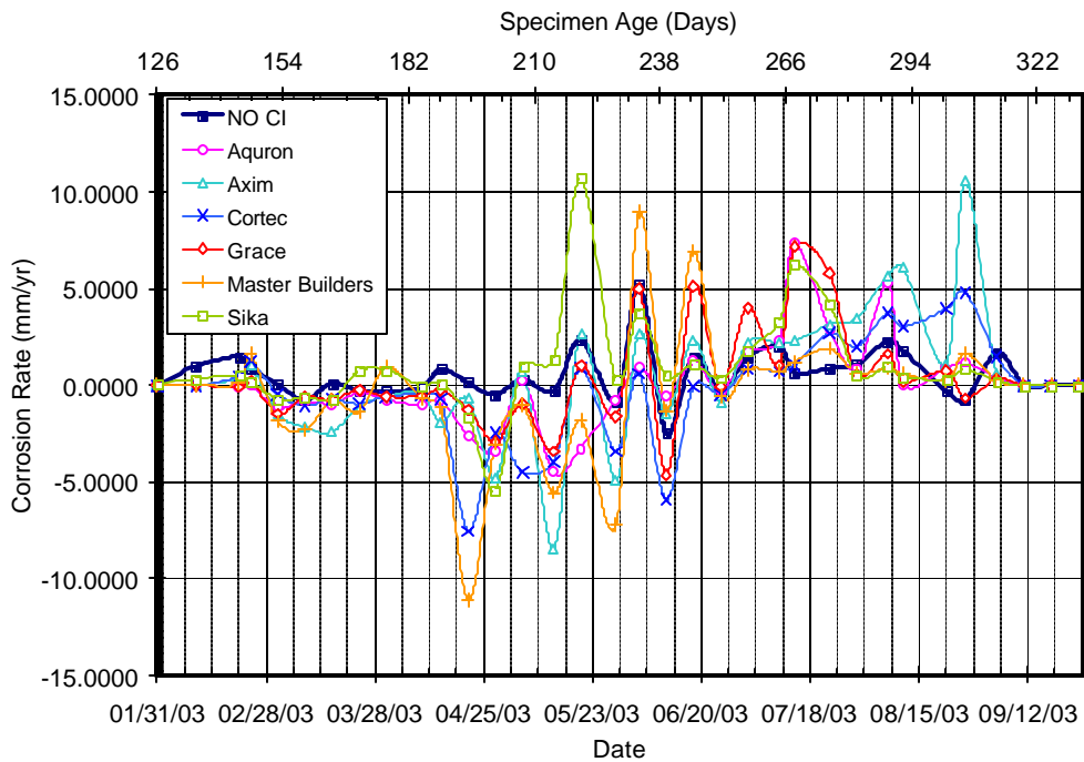
Figure A.24 – Corrosion Rate for Bath 4, 1.5% Chloride, Post-Cracked
