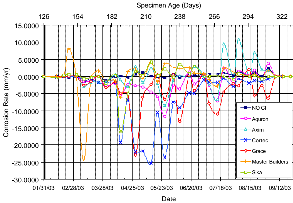
Figure A.5 – Corrosion Rate for Bath 1, 1.0% Chloride, Pre-Cracked
