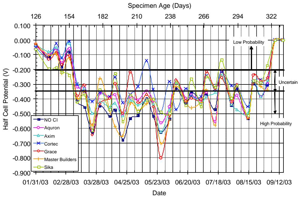
Figure C.5 – Half Cell Potential Readings for Bath 1, 1.0% Chloride, Pre-Cracked
