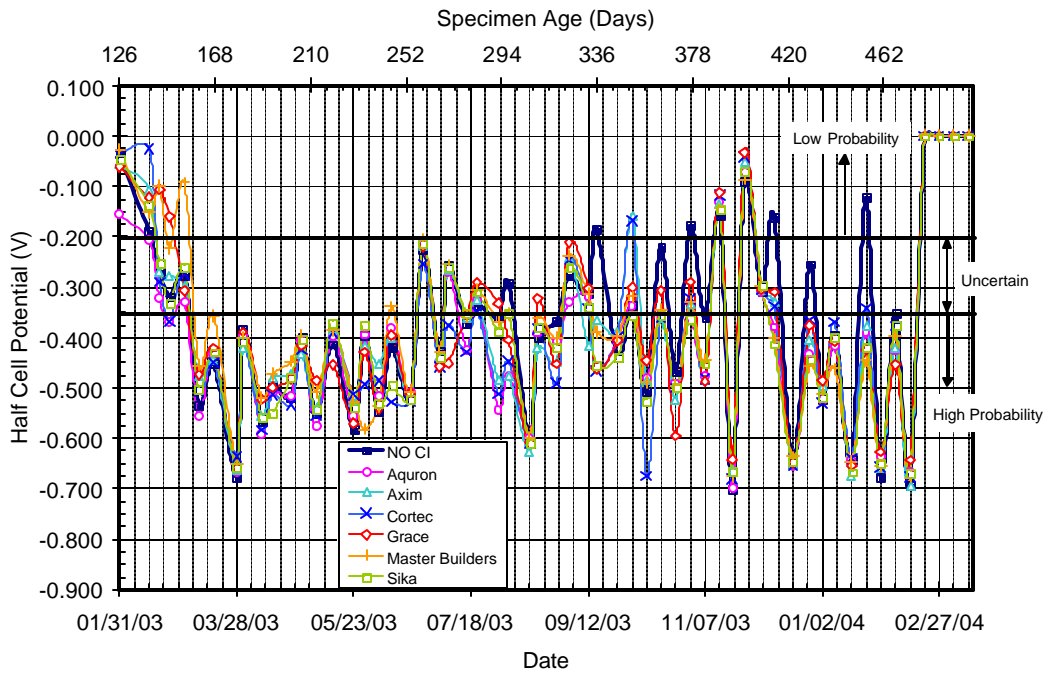
Figure C.19 – Half Cell Potential Readings for Bath 3, 2.0% Chloride, Post-Cracked
