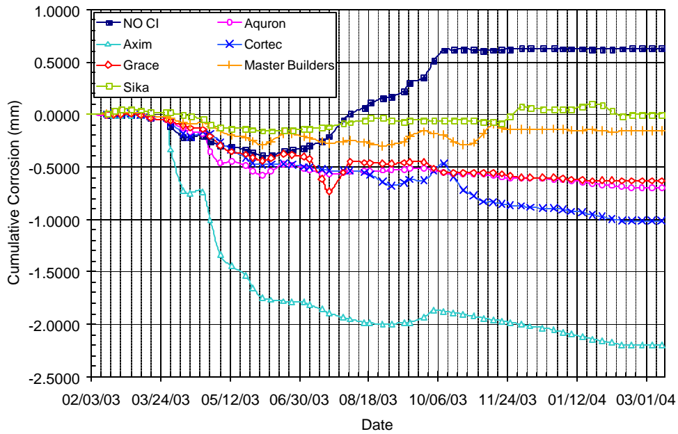
Figure B.17 – Cumulative Corrosion Over Time for Bath 3, 1.0% Chloride, Post-Cracked
