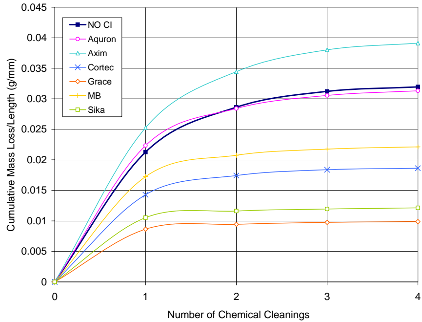
Figure F.11 – Cumulative Mass Loss/Length for Bath 2, 1.5% Chloride Pre-Cracked Specimens
