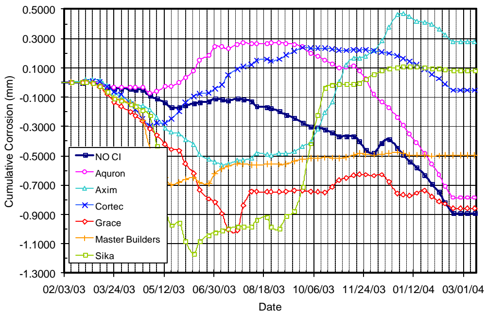
Figure B.12 – Cumulative Corrosion Over Time for Bath 2, 1.5% Chloride, Pre-Cracked
