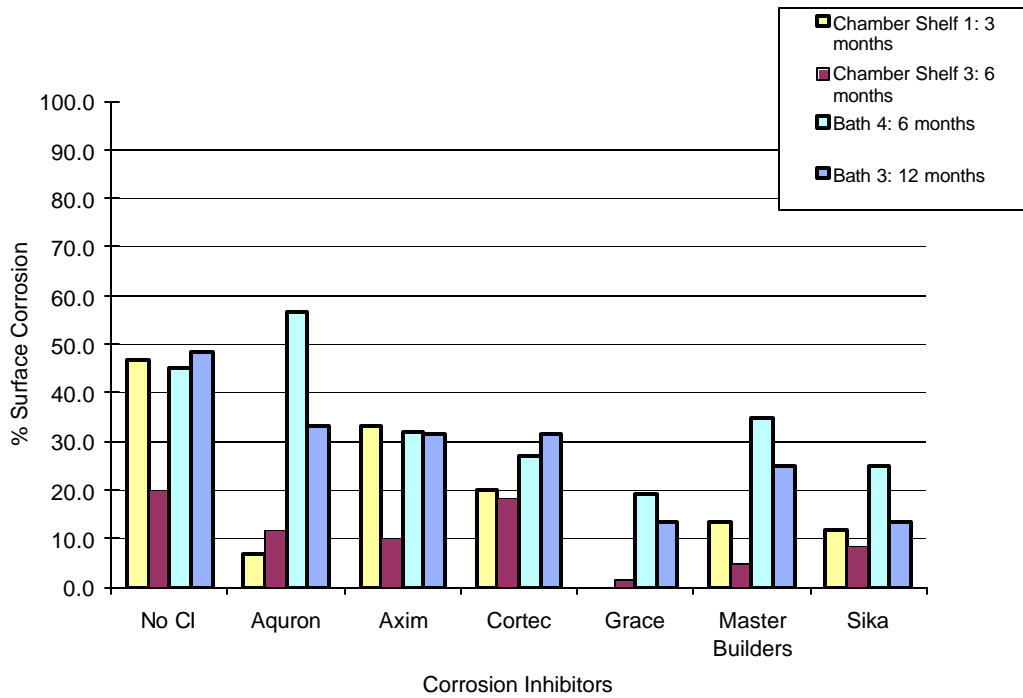
Figure E.41 Time Step of Surface Corrosion for 0.0% Chloride Post-Cracked Specimens
