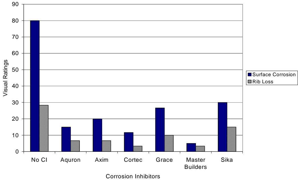
Figure G.75 – Visual Ratings for Chamber Shelf 3, 0.5% Chloride, Post-Cracked
