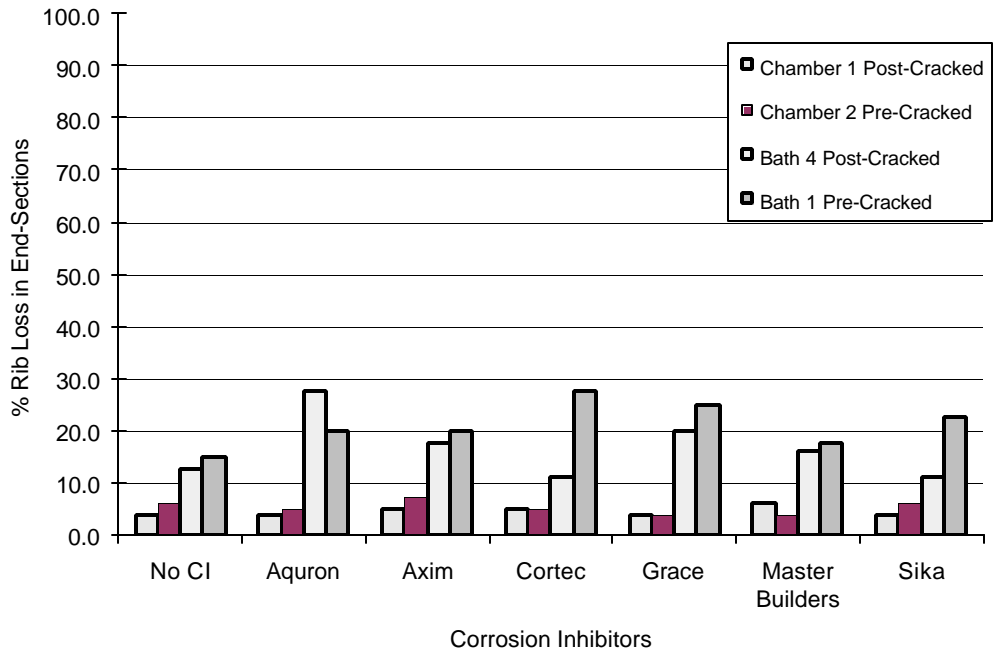
Figure 4.19 - % Rib Loss at End Sections for 1.0% Chloride (Set #1)
