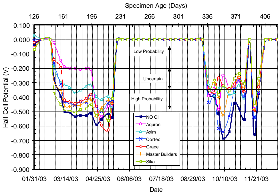
Figure C.30 – Half Cell Potential Readings for Chamber Shelf 1, 1.5% Chloride, Post-Cracked
