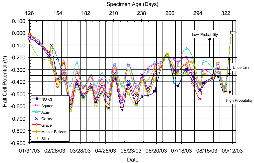
Figure C.23 – Half Cell Potential Readings for Bath 4, 1.0% Chloride, Post-Cracked
