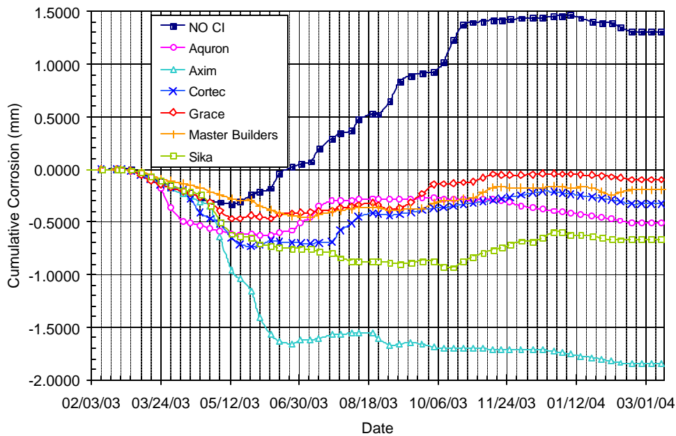
Figure B.11 – Cumulative Corrosion Over Time for Bath 2, 1.0% Chloride, Pre-Cracked
