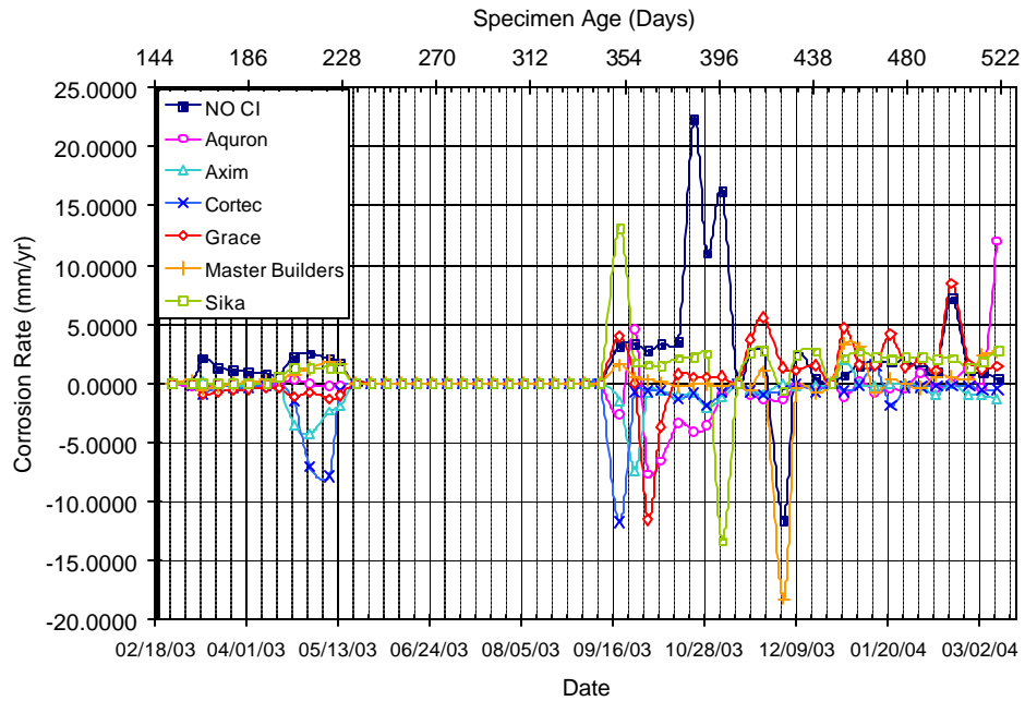
Figure A.45 – Corrosion Rate for Chamber Shelf 4, 0.0% Chloride, Pre-Cracked
