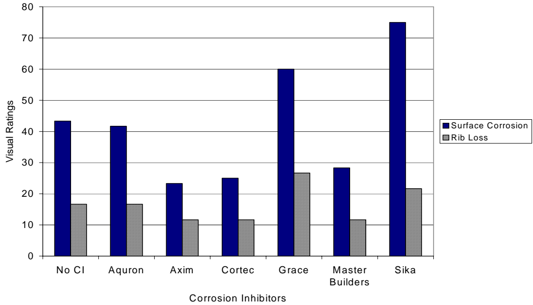
Figure G.81 – Visual Ratings for Chamber Shelf 3, 2.0% Chloride, Post-Cracked
