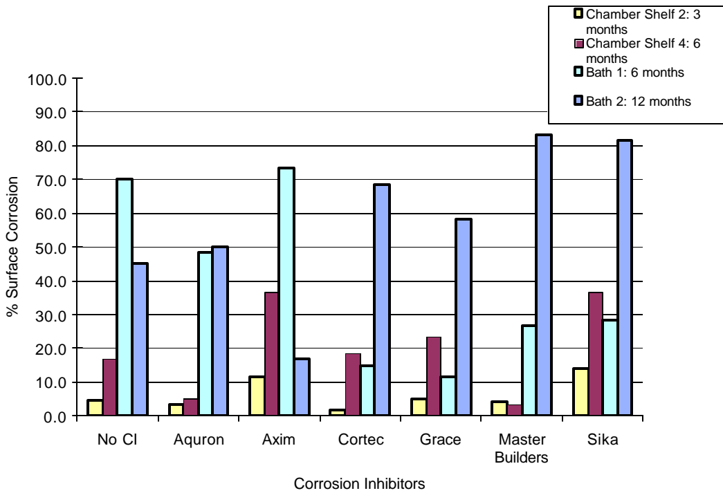
Figure E.33 Time Step of Surface Corrosion for 1.0% Chloride Pre-Cracked Specimens
