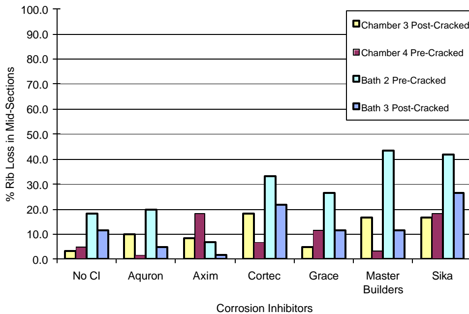
Figure E.20 Rib Loss at Mid Section for 1.0% Chloride (Set #2)
