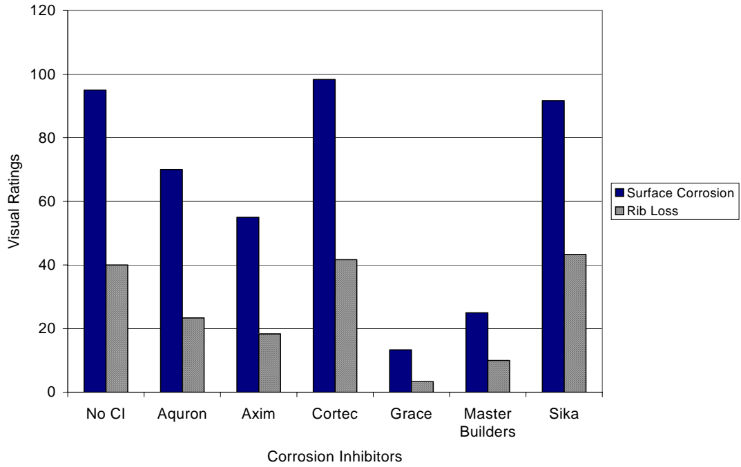
Figure G.7 – Visual Ratings for Bath 1, 1.5% Chloride, Pre-Cracked
