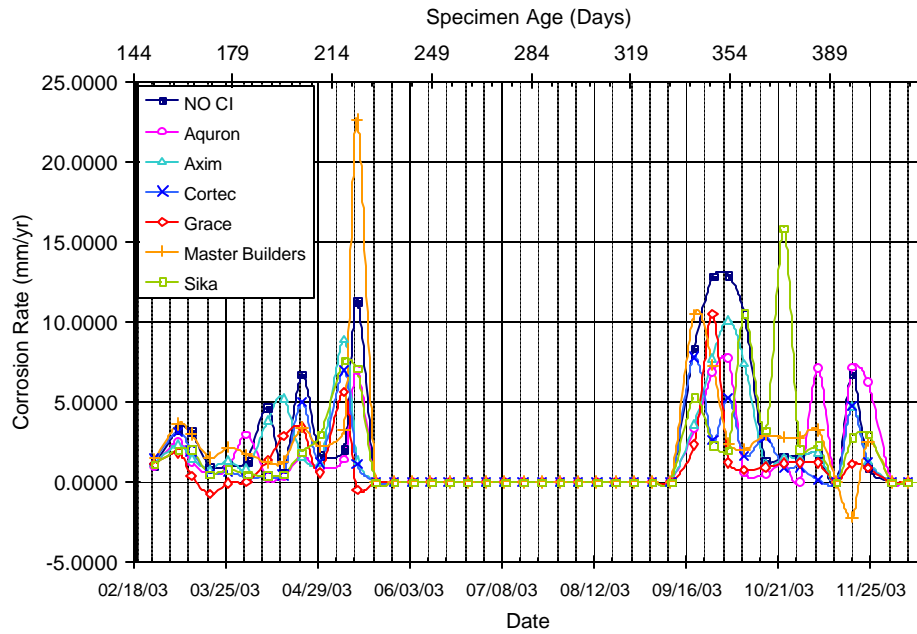
Figure A.37 – Corrosion Rate for Chamber Shelf 2, 2.0% Chloride, Pre-Cracked
