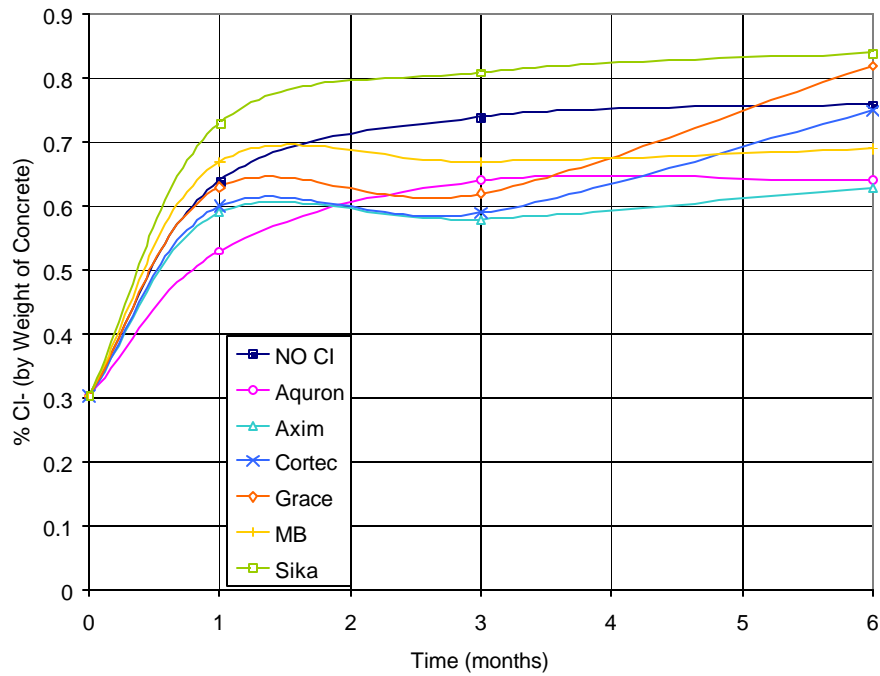
Figure D.12 – Chloride Content for Chamber Specimens – 3.0% Chloride
