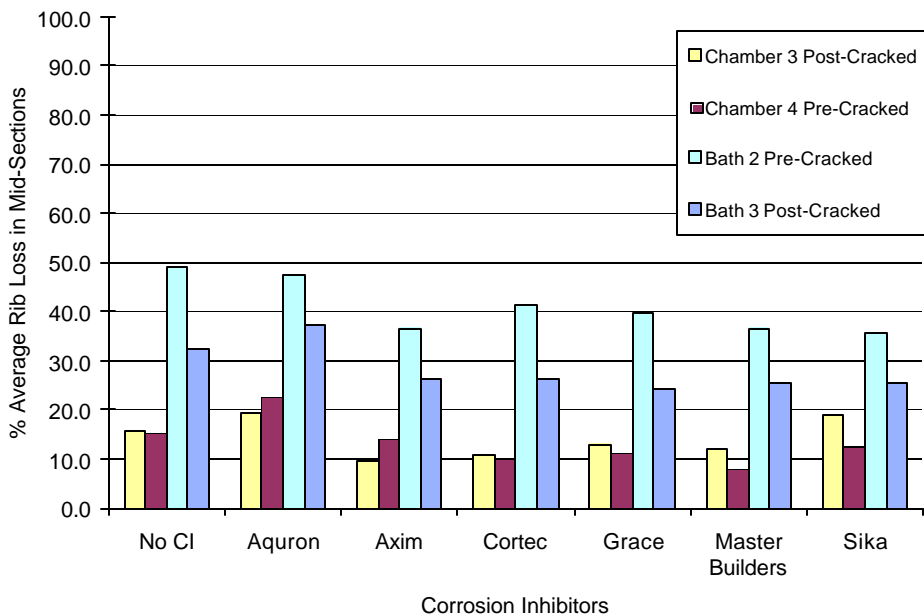
Figure E.28 Rib Loss at Mid Section for Average of all Chloride Contaminants (Set#2)
