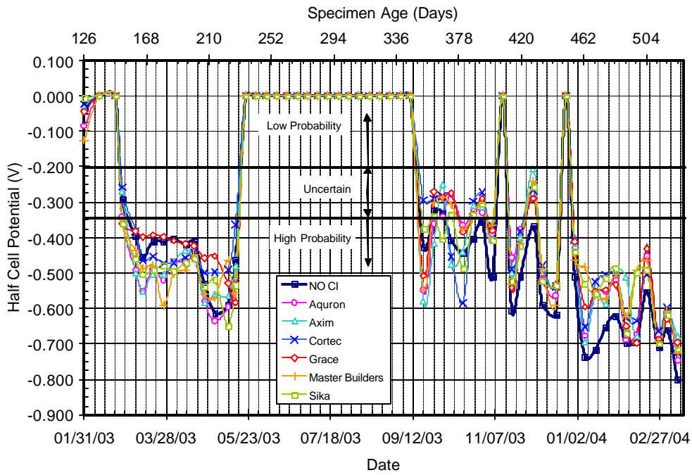
Figure C.43 – Half Cell Potential Readings for Chamber Shelf 3, 2.0% Chloride, Post-Cracked
