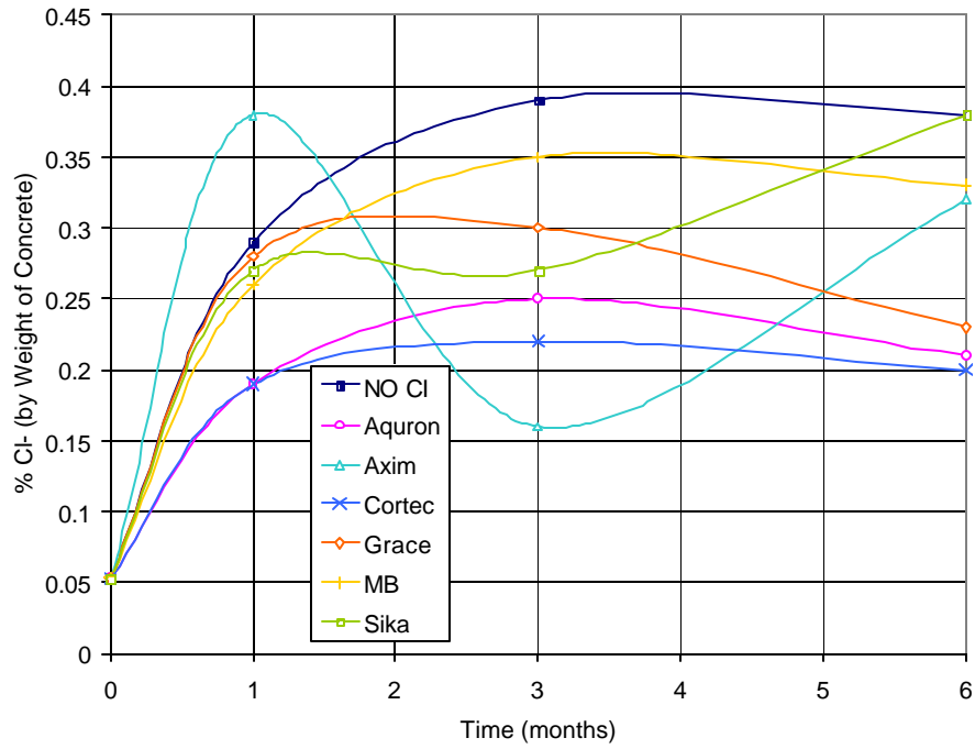
Figure D.9 – Chloride Content for Chamber Specimens – 0.5% Chloride
