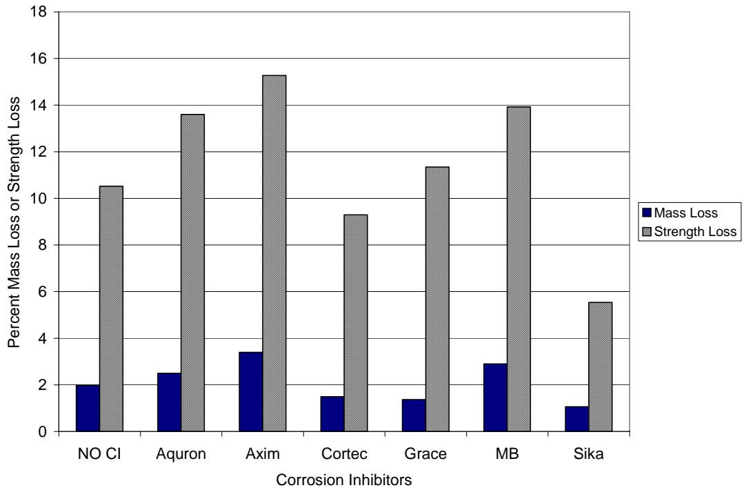
Figure G.24 – Mass Loss and Strength Loss for Bath 2, 3.0% Chloride, Pre-Cracked
