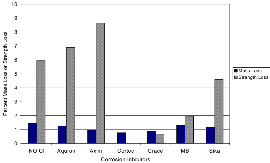
Figure G.56 – Mass Loss and Strength Loss for Chamber Shelf 1, 1.5% Chloride, Post-Cracked
