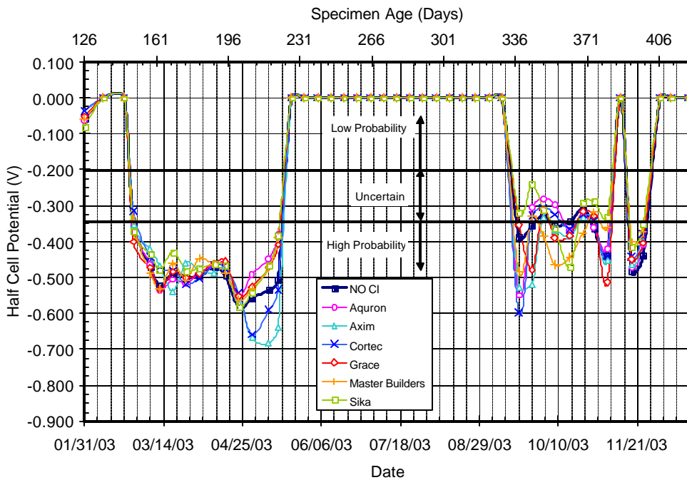
Figure C.38 – Half Cell Potential Readings for Chamber Shelf 2, 3.0% Pre-Cracked
