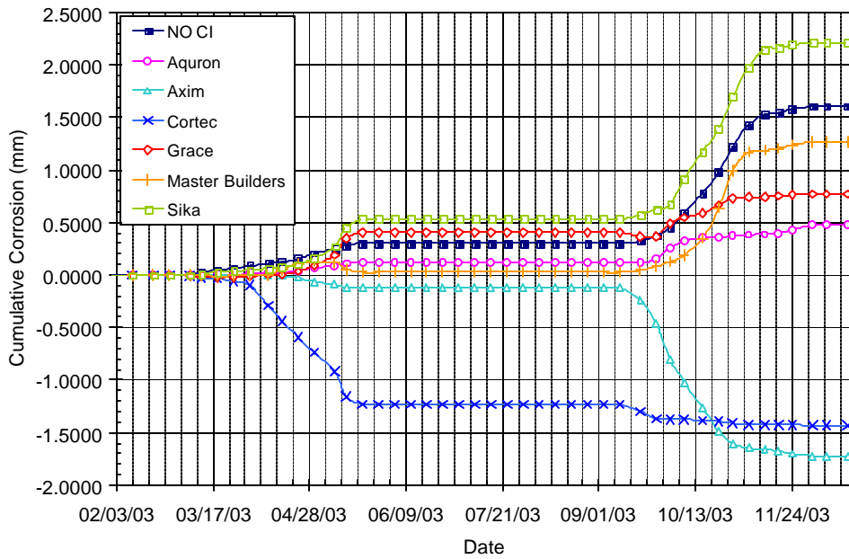
Figure B.33 – Cumulative Corrosion Over Time for Chamber Shelf 2, 0.0% Chloride, Pre-Cracked
