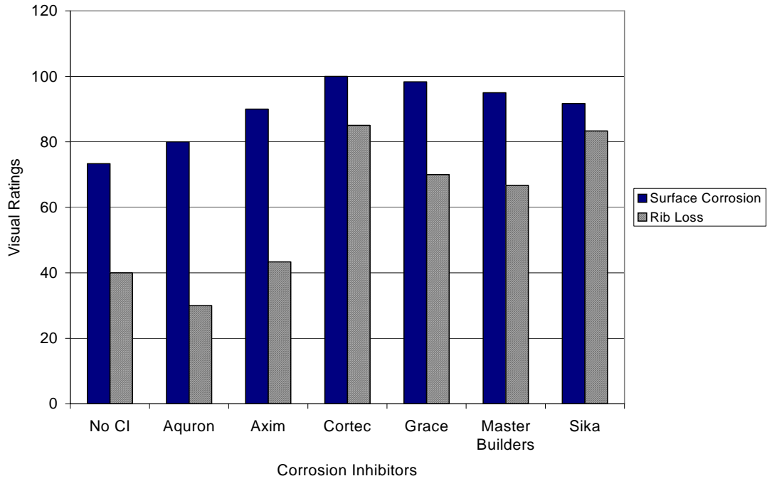
Figure G.21 – Visual Ratings for Bath 2, 2.0% Chloride, Pre-Cracked
