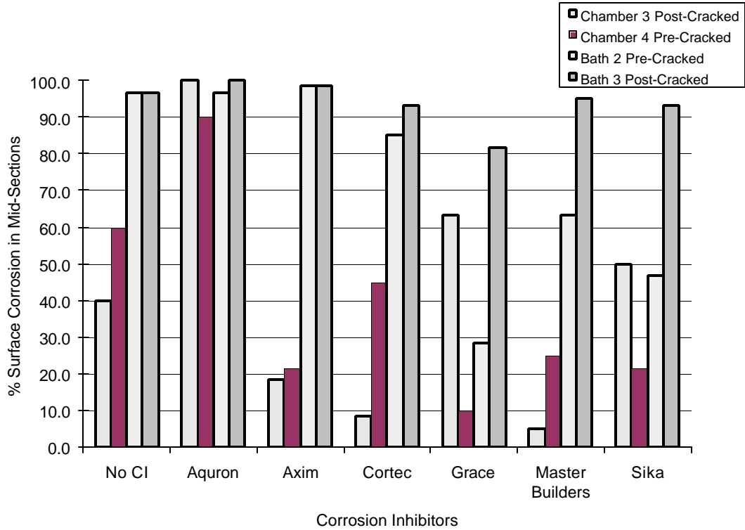
Figure 4.25 - % Surface Corrosion at Midsection for 1.5% Chloride (Set #2)
