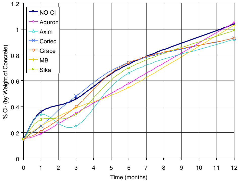
Figure 4.15 - Chloride Content for Bath Specimens – 1.5% Chloride
