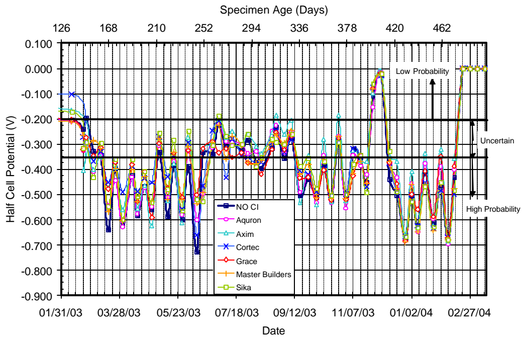
Figure C.14 – Half Cell Potential Readings for Bath 2, 3.0% Chloride, Pre-Cracked
