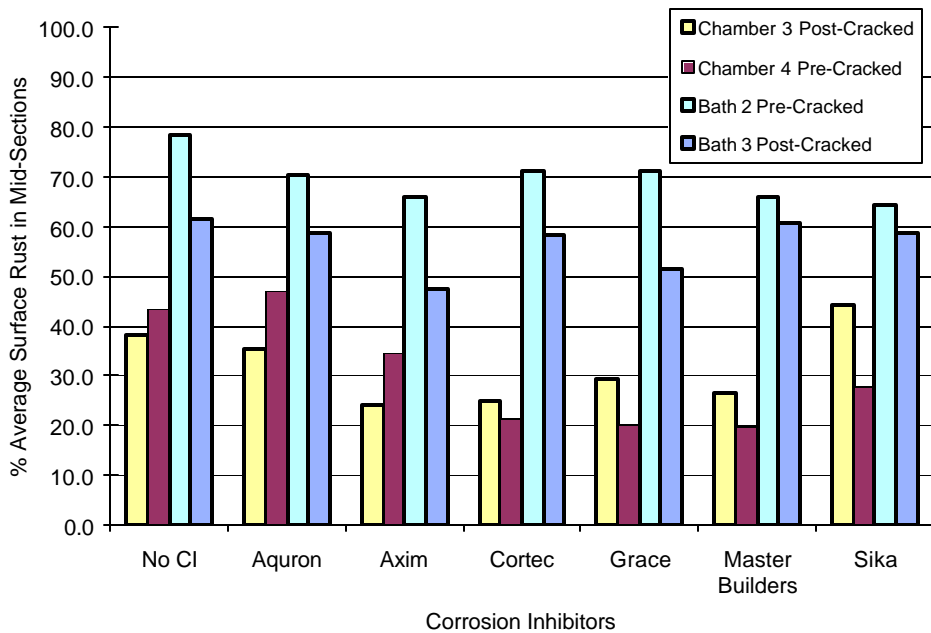
Figure E.27 Surface Corrosion at Mid Section for Average of all Chloride Contaminants (Set#2)
