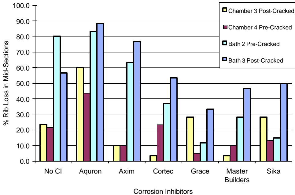
Figure E.22 Rib Loss at Mid Section for 1.5% Chloride (Set #2)
