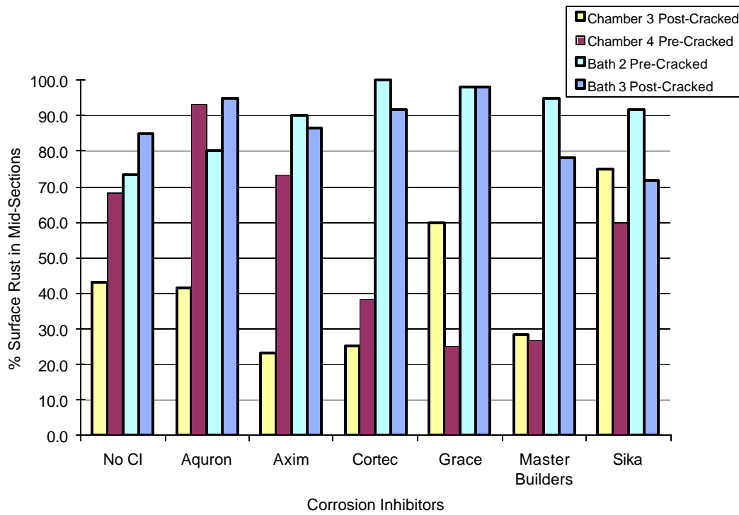
Figure E.23 Surface Corrosion at Mid Section for 2.0% Chloride (Set#2)
