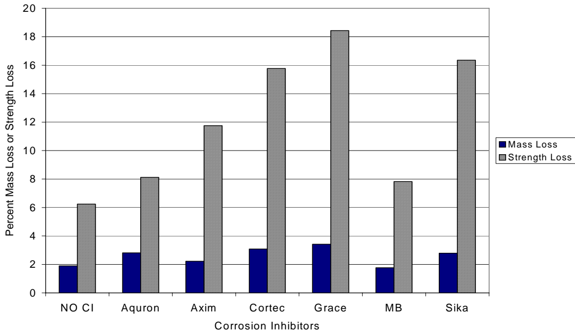
Figure G.34 – Mass Loss and Strength Loss for Bath 3, 2.0% Chloride, Post-Cracked
