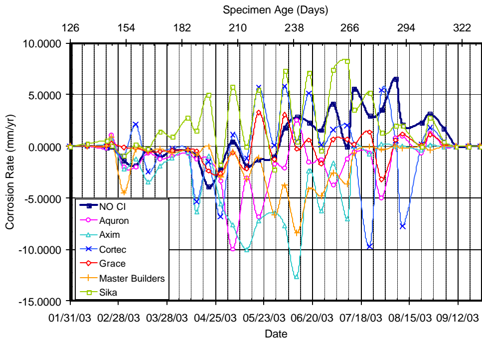
Figure A.23 – Corrosion Rate for Bath 4, 1.0% Chloride, Post-Cracked
