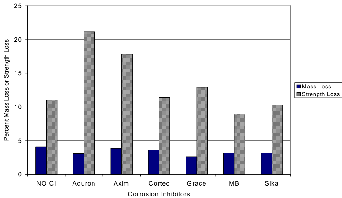
Figure G.32 – Mass Loss and Strength Loss for Bath 3, 1.5% Chloride, Post-Cracked
