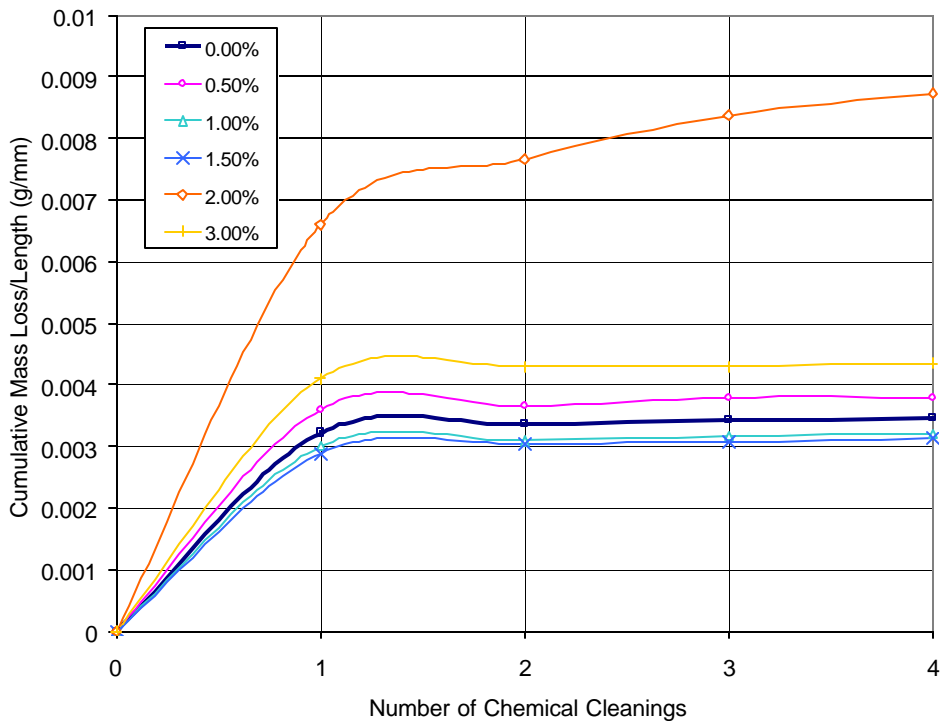
Figure 4.35 – Cumulative Mass Loss/Length for Control Specimens
