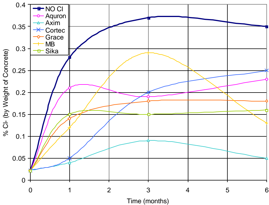
Figure D.8 – Chloride Content for Chamber Specimens – 0.0% Chloride
