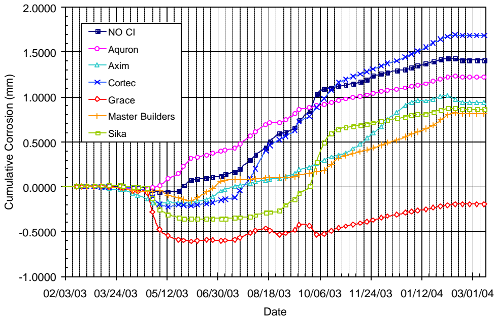
Figure B.15 – Cumulative Corrosion Over Time for Bath 3, 0.0% Chloride, Post-Cracked
