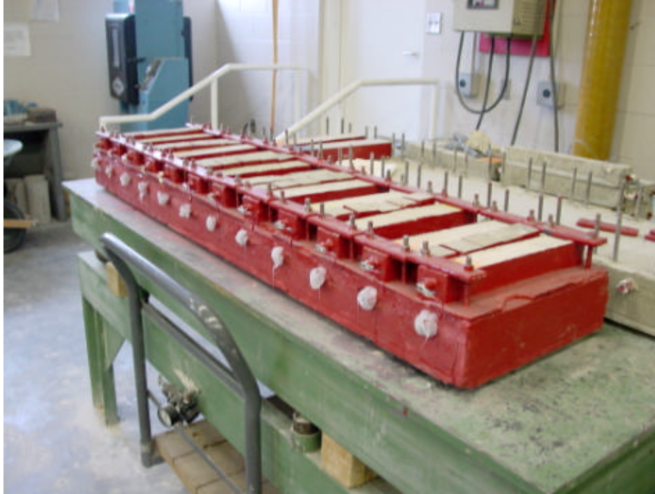
Figure 3.20 – Control Environment Specimens
