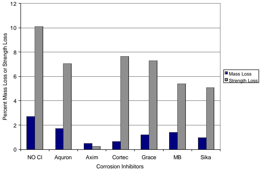
Figure 4.44 – Mass Loss and Strength Loss for Chamber 0.5% Chloride, Shelf 2, Pre-Cracked Specimens
