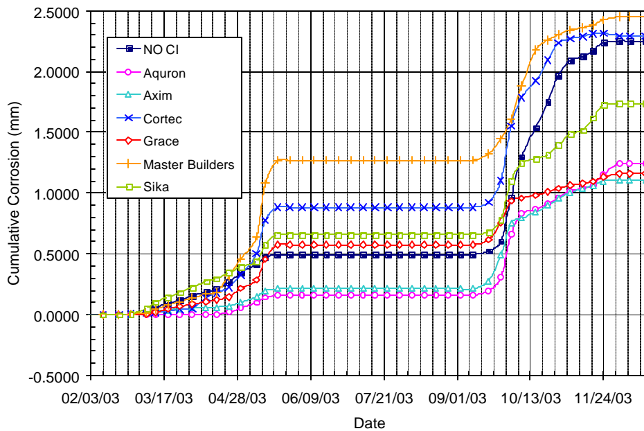
Figure B.30 – Cumulative Corrosion Over Time for Chamber Shelf 1, 1.5% Chloride, Post-Cracked
