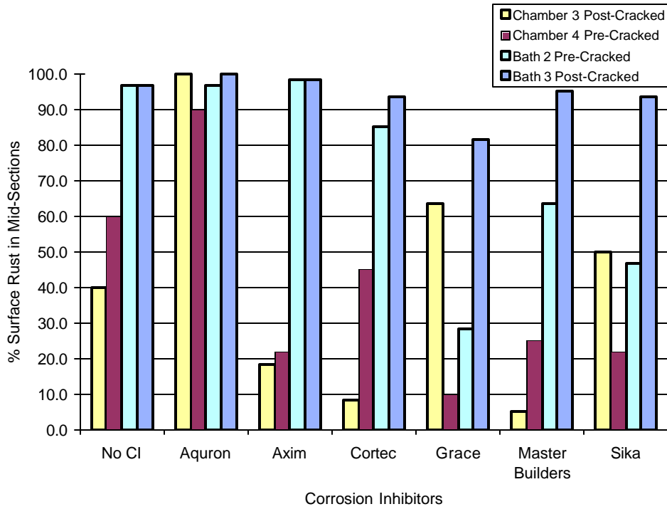
Figure E.21 Surface Corrosion at Mid Section for 1.5% Chloride (Set#2)
