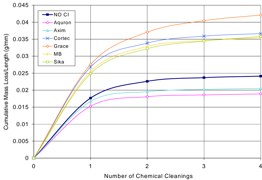
Figure F.11 – Cumulative Mass Loss/Length for Bath 2, 1.5% Chloride Pre-Cracked Specimens
