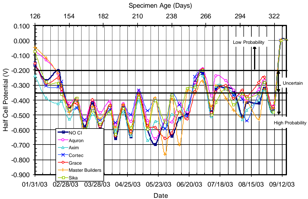
Figure C.26 – Half Cell Potential Readings for Bath 4, 3.0% Chloride, Post-Cracked
