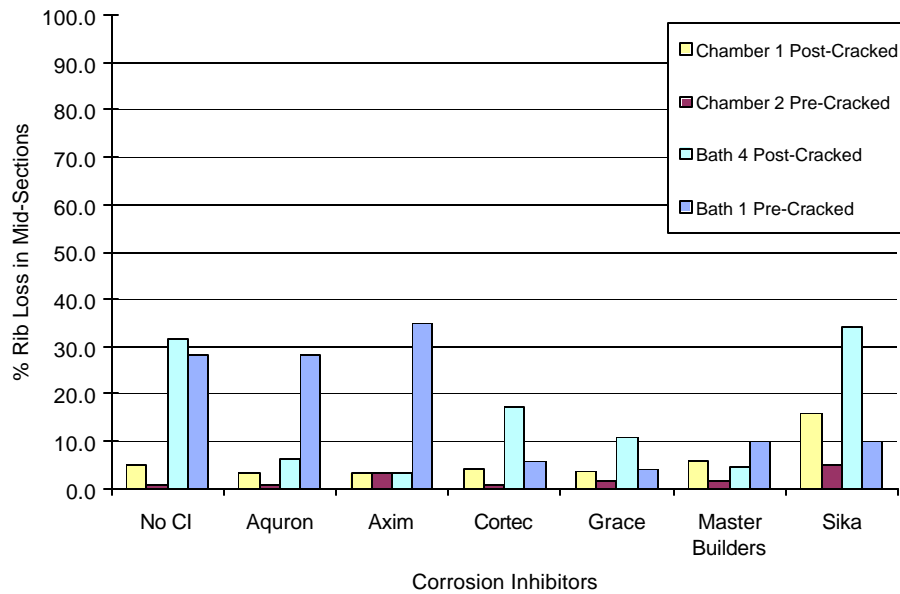
Figure E.6 Rib Loss at Mid Section for 1.0% Chloride (Set #1)
