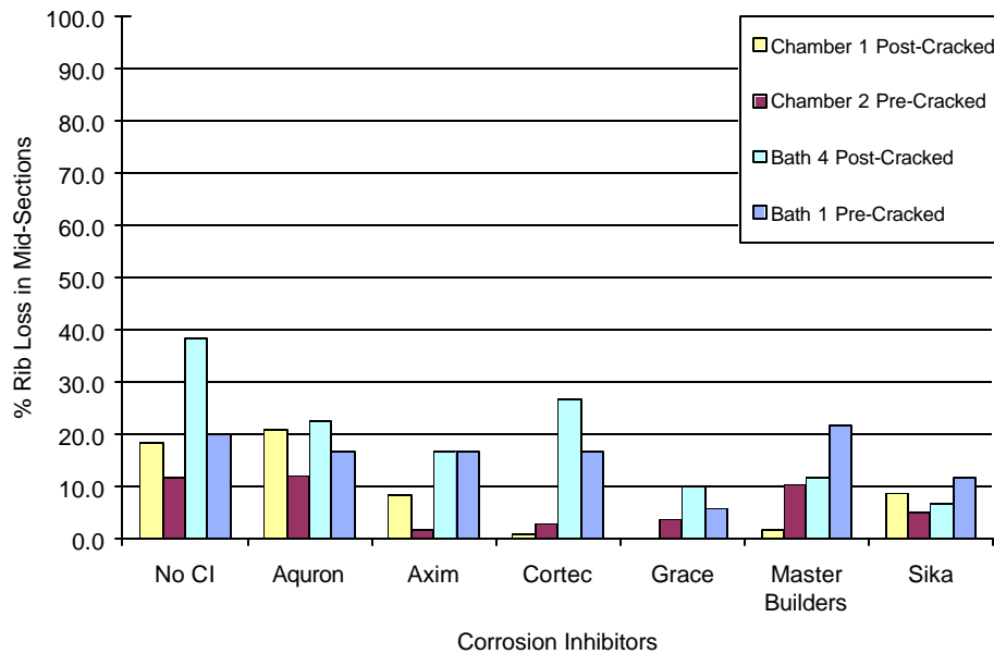
Figure E.4 Rib Loss at Mid Section for 0.5% Chloride (Set #1)
