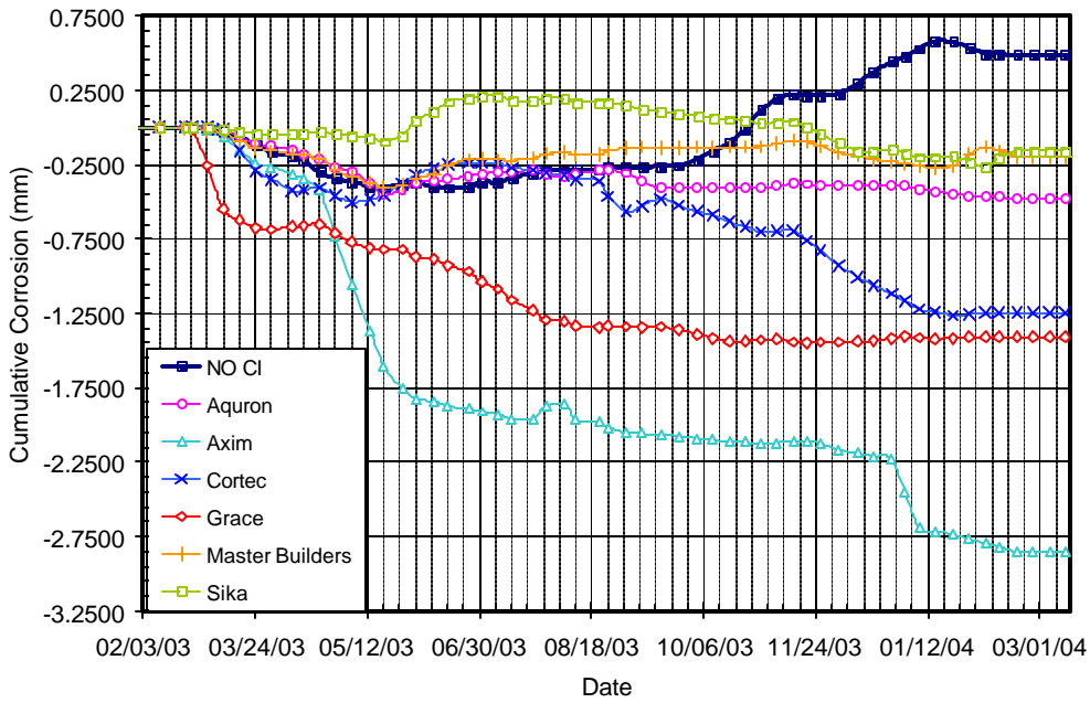
Figure B.13 – Cumulative Corrosion Over Time for Bath 2, 2.0% Chloride, Pre-Cracked
