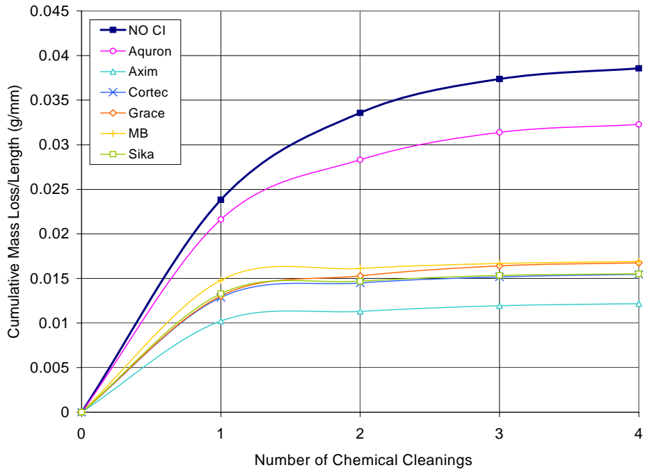
Figure F.15 – Cumulative Mass Loss/Length for Bath 3, 0.5% Chloride Post-Cracked Specimens
