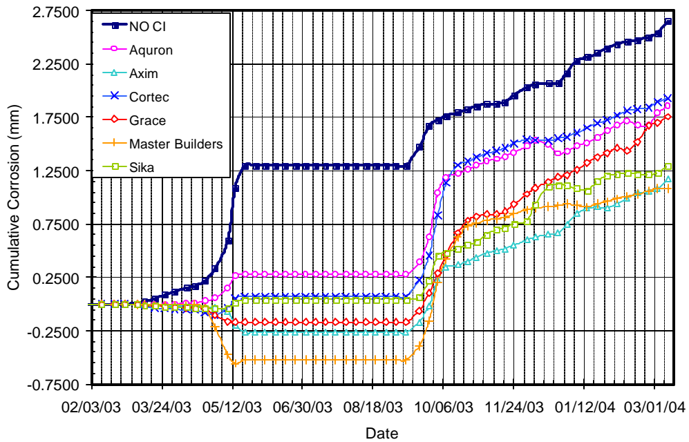
Figure B.46 – Cumulative Corrosion Over Time for Chamber Shelf 4, 0.5% Chloride, Pre-Cracked
