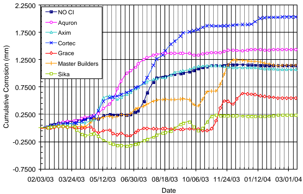
Figure B.20 – Cumulative Corrosion Over Time for Bath 3, 3.0% Chloride, Post-Cracked
