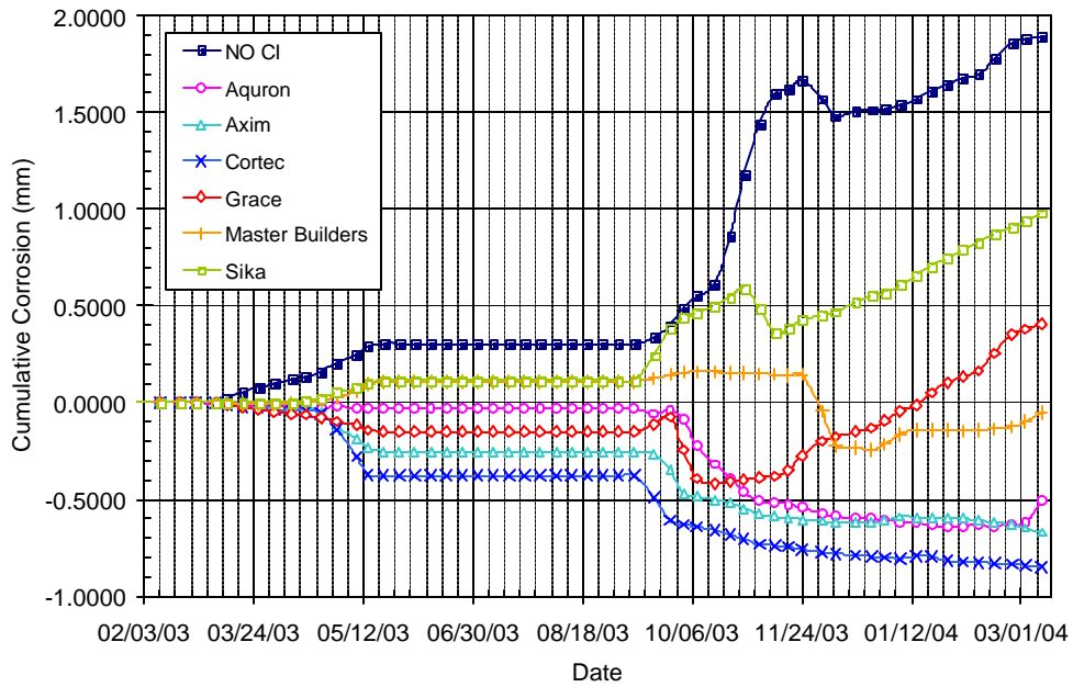
Figure B.45 – Cumulative Corrosion Over Time for Chamber Shelf 4, 0.0% Chloride, Pre-Cracked
