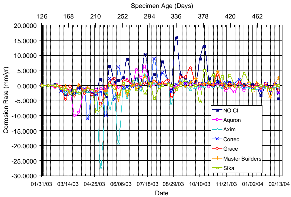
Figure A.11 – Corrosion Rate for Bath 2, 1.0% Chloride, Pre-Cracked
