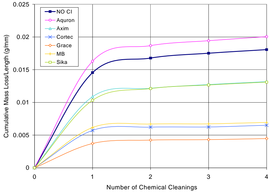
Figure F.27 – Cumulative Mass Loss/Length for Chamber Shelf 1 0.5% Chloride, Post-Cracked Specimens
