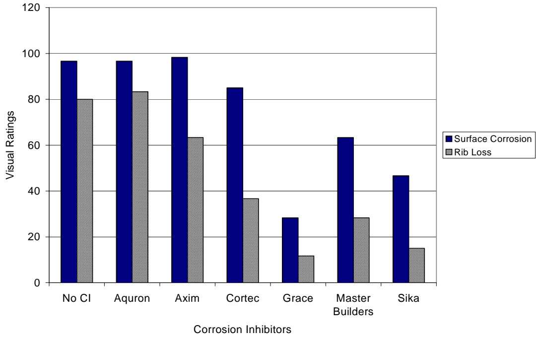
Figure G.19 – Visual Ratings for Bath 2, 1.5% Chloride, Pre-Cracked
