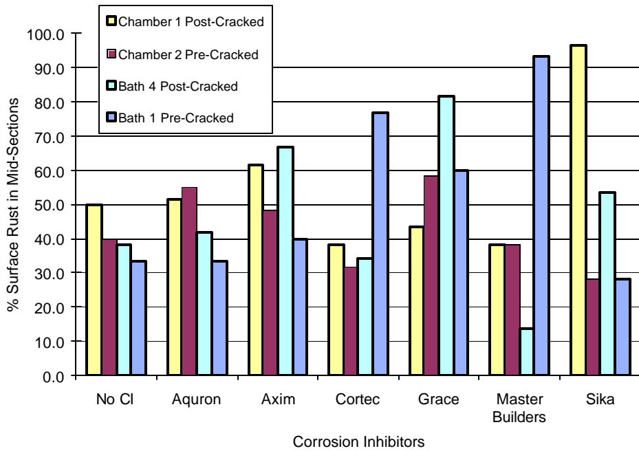
Figure E.11 Surface Corrosion at Mid Section for 3.0% Chloride (Set#1)
