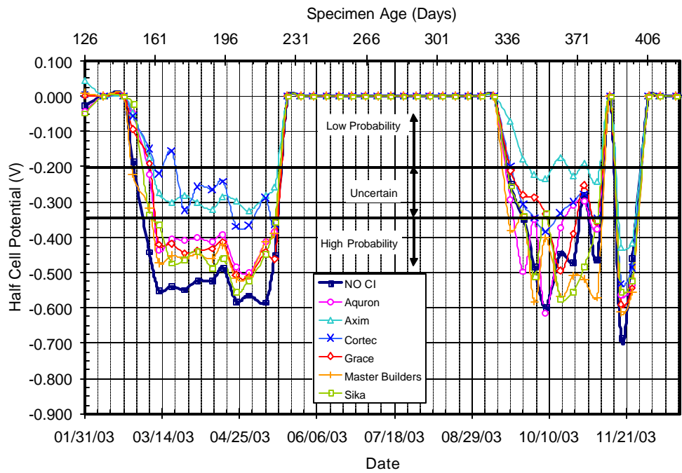
Figure C.34 – Half Cell Potential Readings for Chamber Shelf 2, 0.5% Chloride, Pre-Cracked
