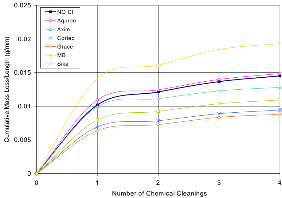
Figure F.35 – Cumulative Mass Loss/Length for Chamber Shelf 2 1.5% Chloride, Pre-Cracked Specimens
