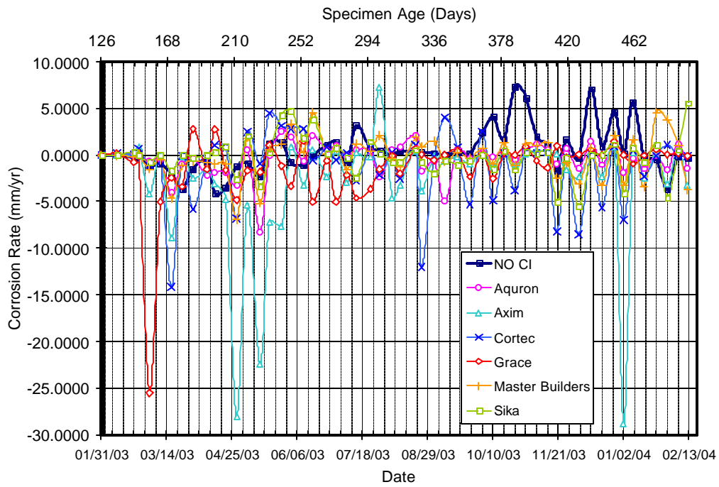
Figure A.13 – Corrosion Rate for Bath 2, 2.0% Chloride, Pre-Cracked
