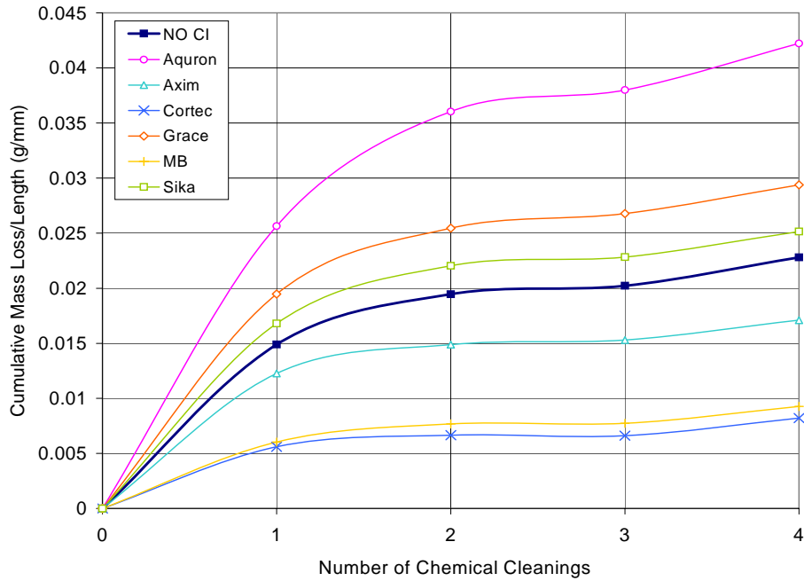
Figure F.41 – Cumulative Mass Loss/Length for Chamber Shelf 3 1.5% Chloride, Post-Cracked Specimens
