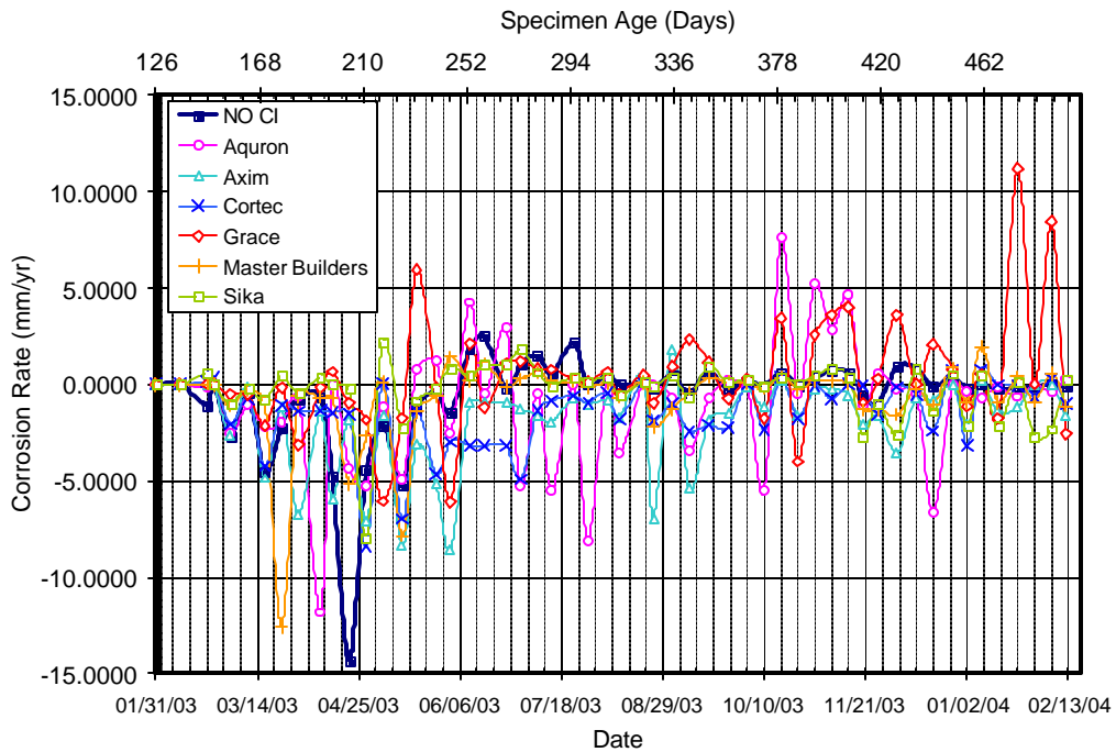
Figure A.10 – Corrosion Rate for Bath 2, 0.5% Chloride, Pre-Cracked
