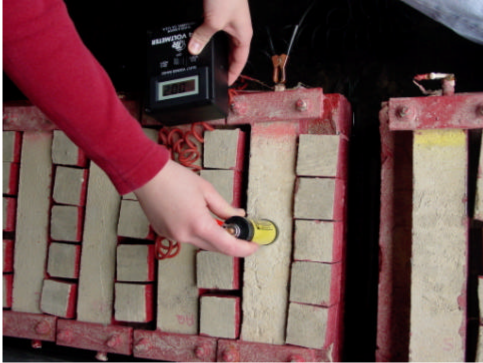
Figure 3.22 – Typical Half Cell Potential Reading Procedure
