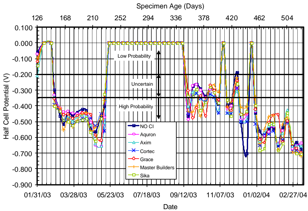
Figure C.44 – Half Cell Potential Readings for Chamber Shelf 3, 3.0% Chloride, Post-Cracked
