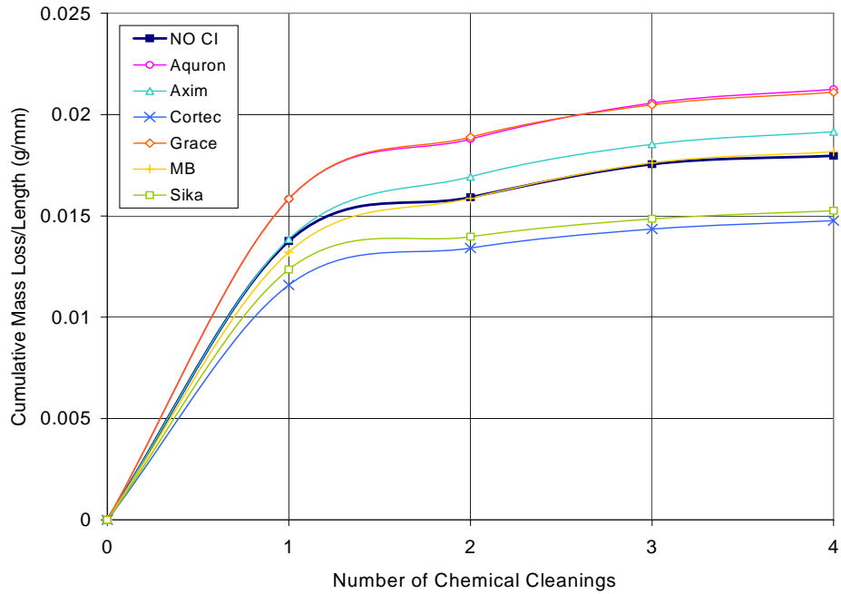
Figure F.37 – Cumulative Mass Loss/Length for Chamber Shelf 2 3.0% Chloride, Pre-Cracked Specimens
