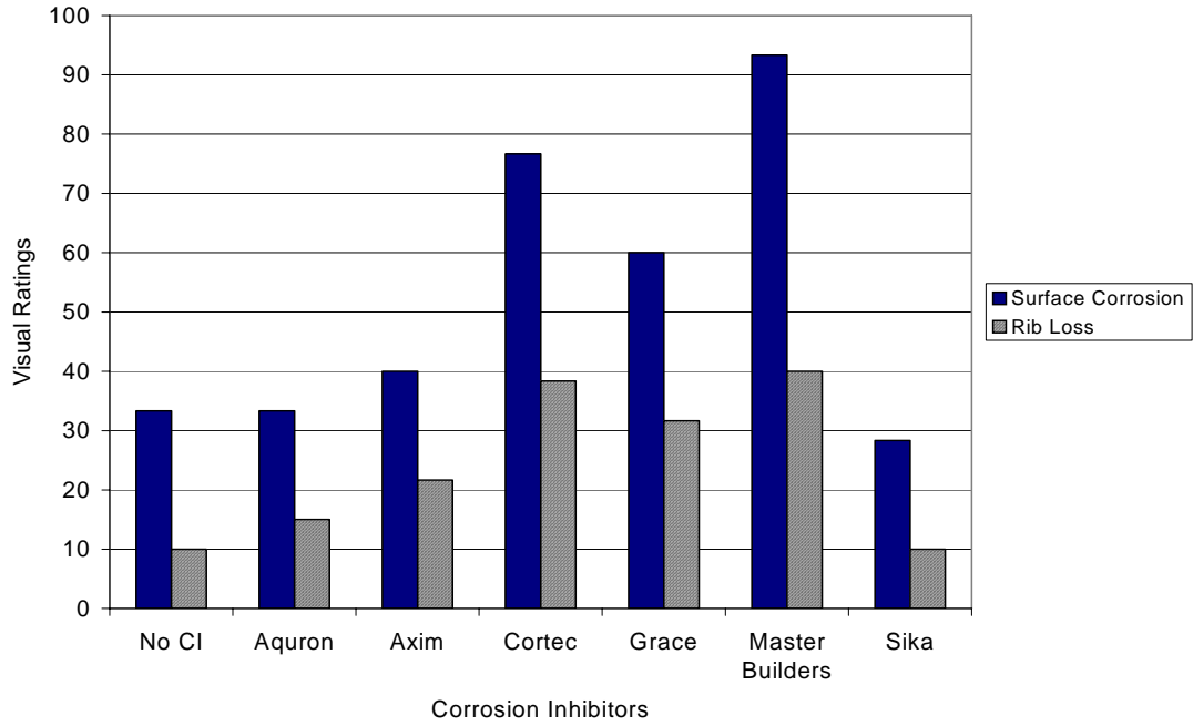
Figure G.11 – Visual Ratings for Bath 1, 3.0% Chloride, Pre-Cracked
