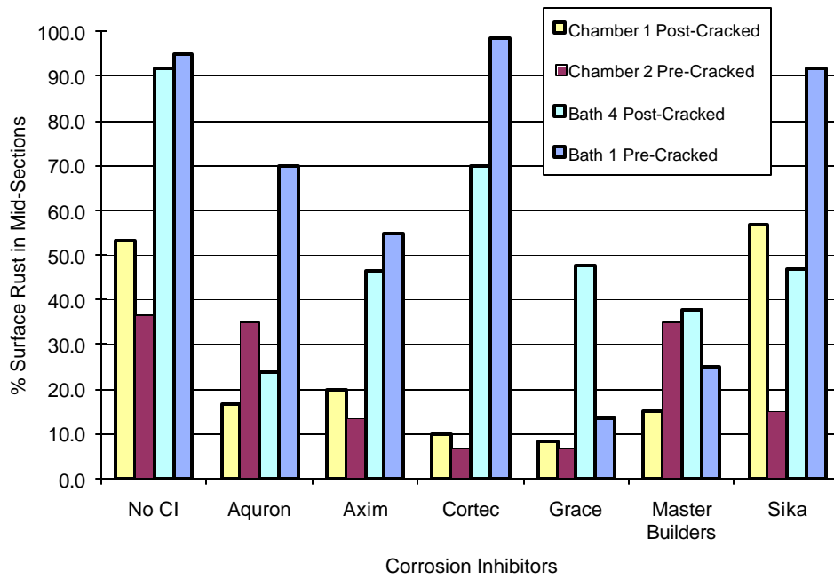
Figure E.7 Surface Corrosion at Mid Section for 1.5% Chloride (Set#1)
