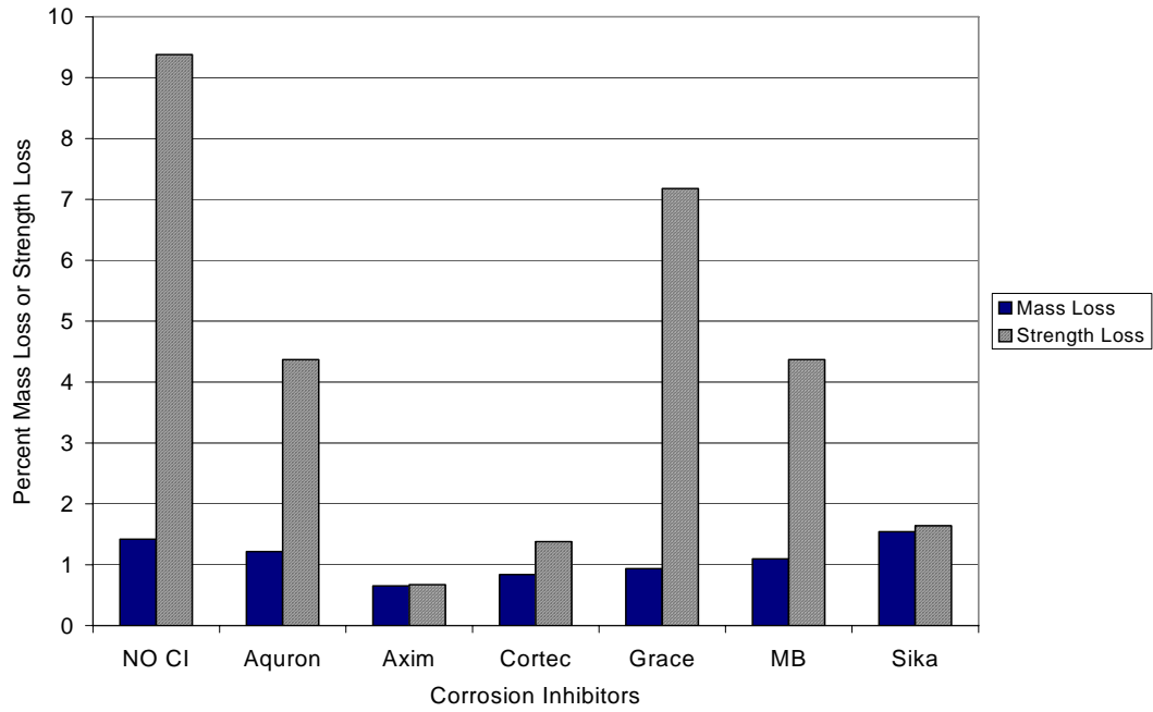
Figure G.86 – Mass Loss and Strength Loss for Chamber Shelf 4, 0.0% Chloride, Pre-Cracked
