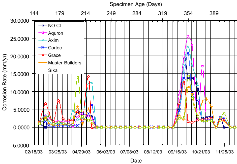
Figure A.31 – Corrosion Rate for Chamber Shelf 1, 2.0% Chloride, Post-Cracked
