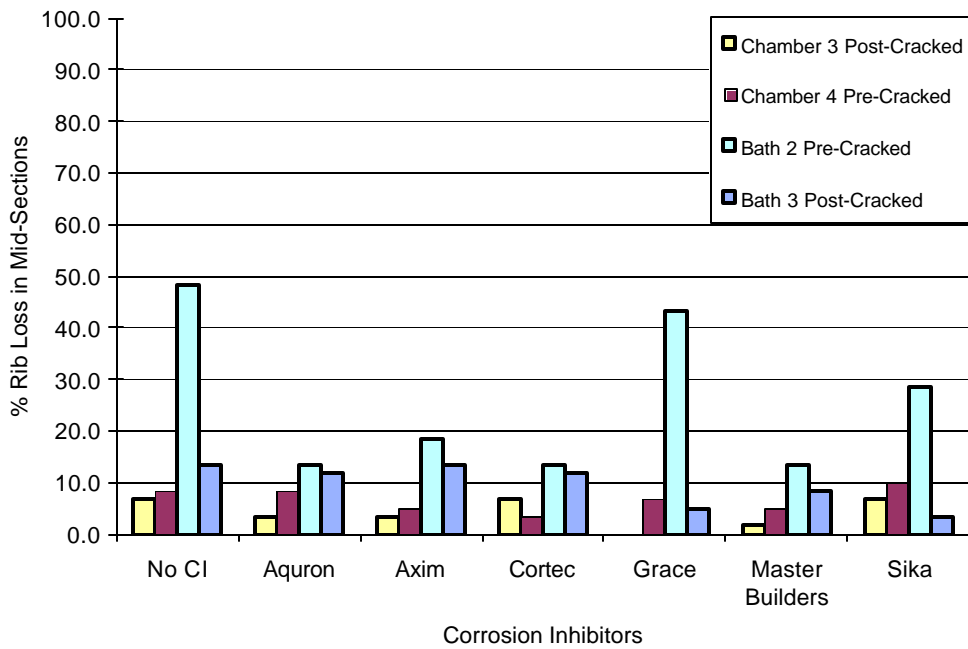
Figure E.16 Rib Loss at Mid Section for 0.0% Chloride (Set #2)
