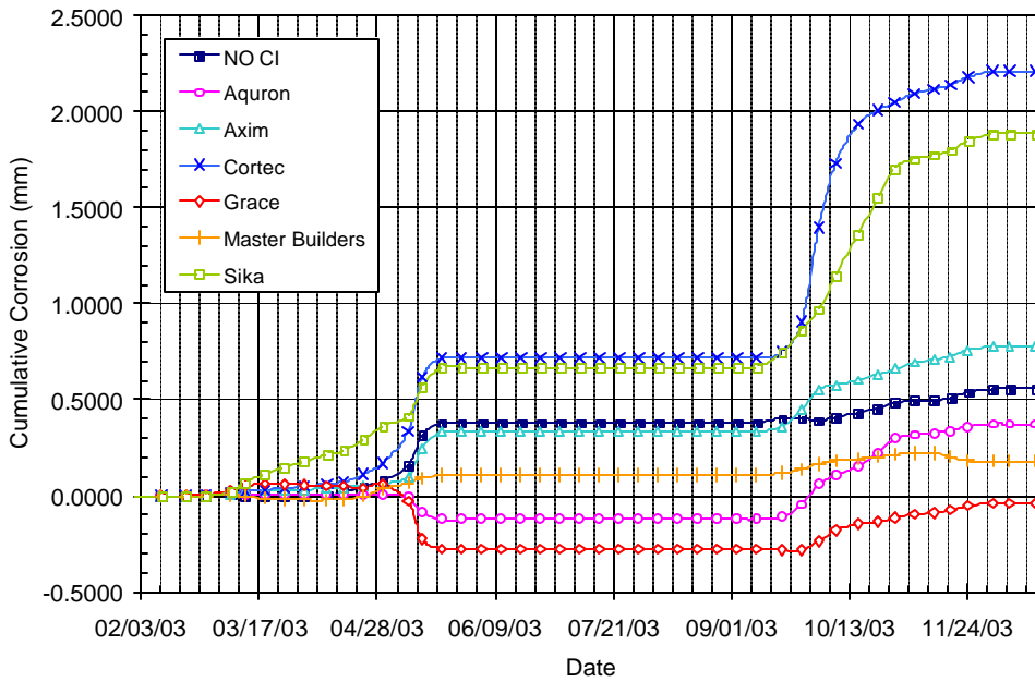
Figure B.29 – Cumulative Corrosion Over Time for Chamber Shelf 1, 1.0% Chloride, Post-Cracked
