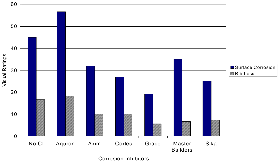
Figure G.37 – Visual Ratings for Bath 4, 0.0% Chloride, Post-Cracked
