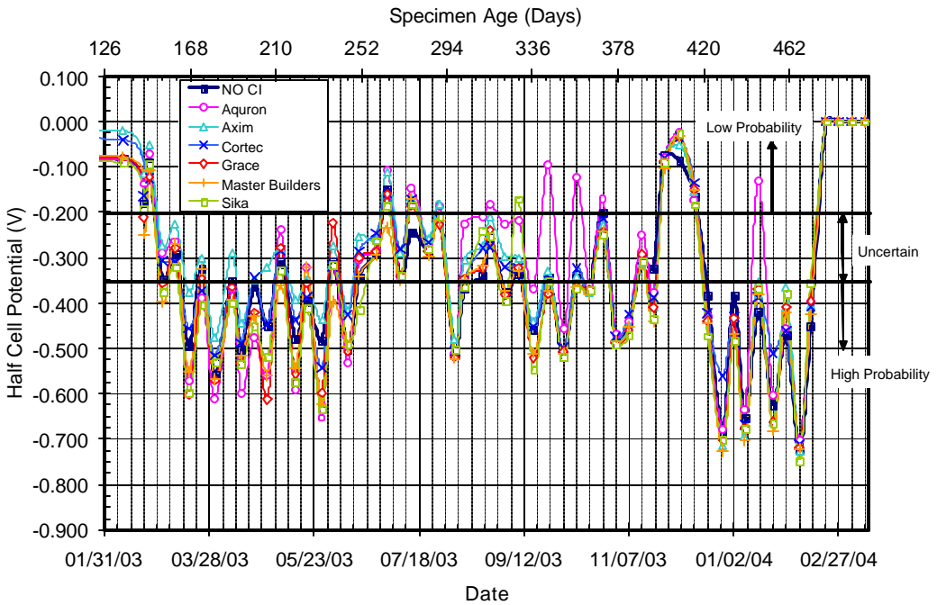
Figure C.10 – Half Cell Potential Readings for Bath 2, 0.5% Chloride, Pre-Cracked
