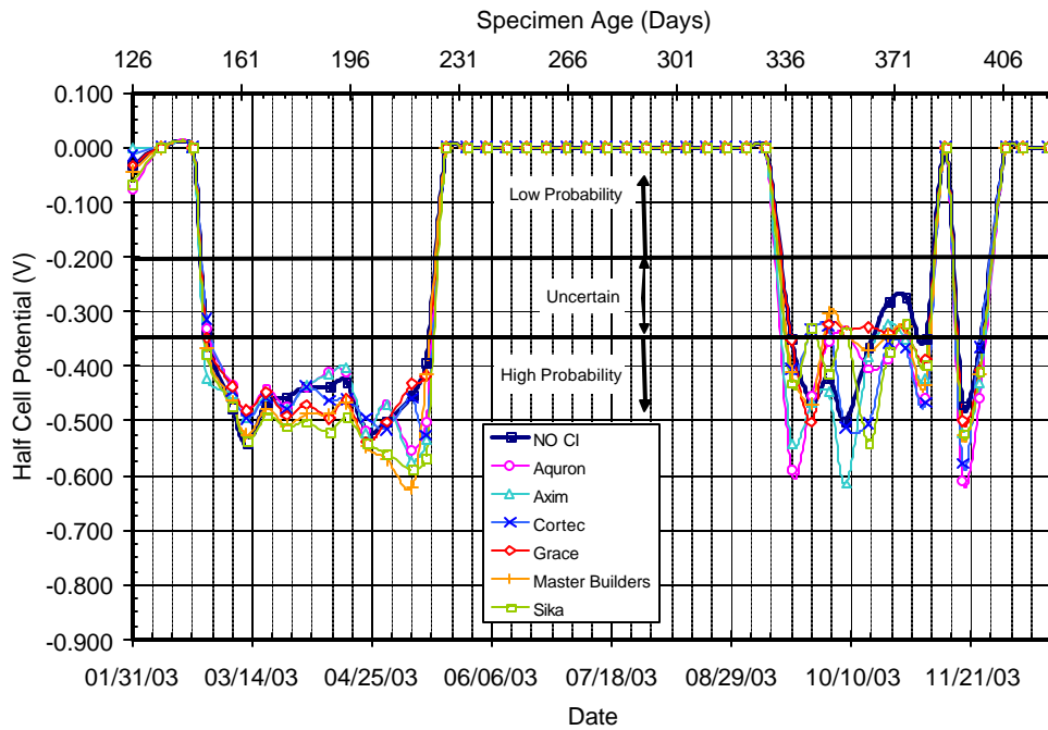
Figure C.37 – Half Cell Potential Readings for Chamber Shelf 2, 2.0% Chloride, Pre-Cracked
