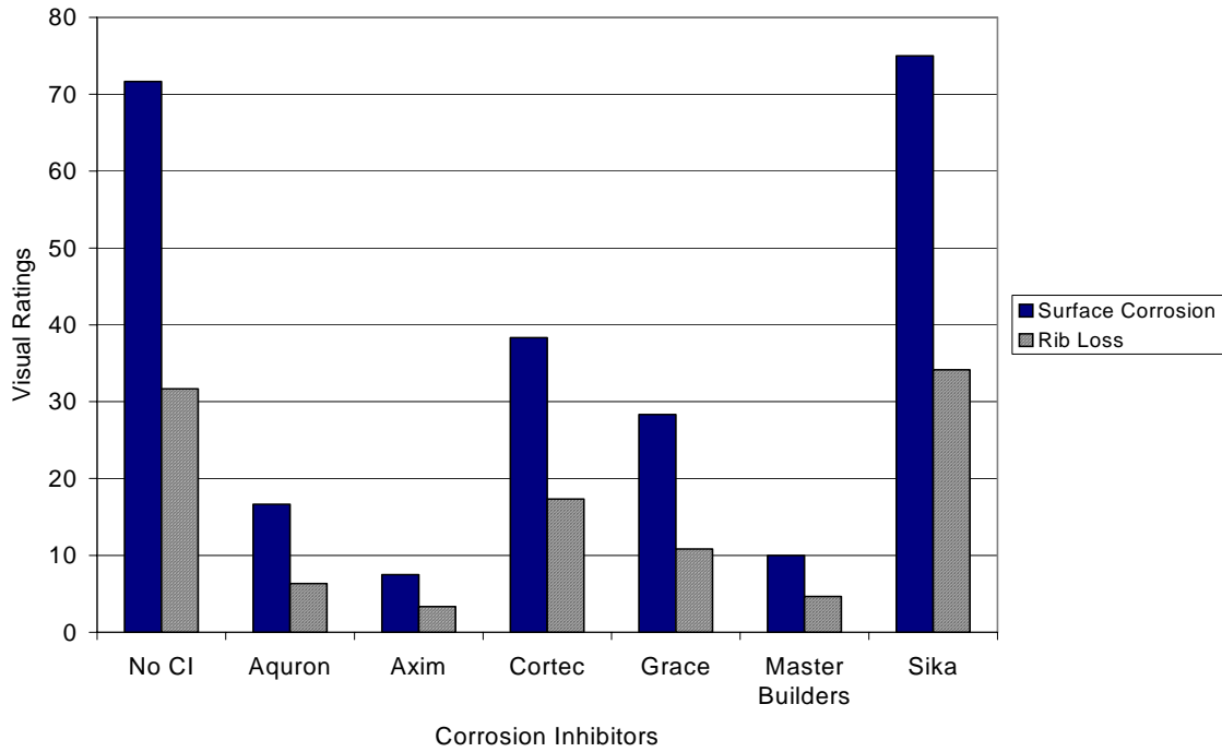
Figure G.41 – Visual Ratings for Bath 4, 1.0% Chloride, Post-Cracked
