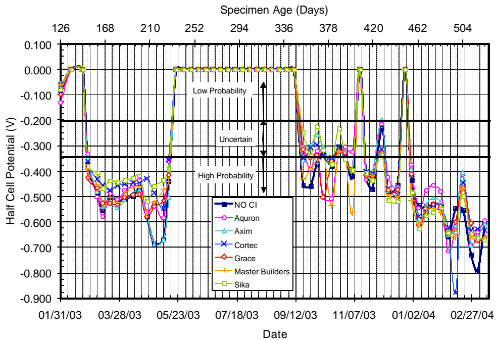
Figure C.50 – Half Cell Potential Readings for Chamber Shelf 4, 3.0% Chloride, Pre-Cracked
