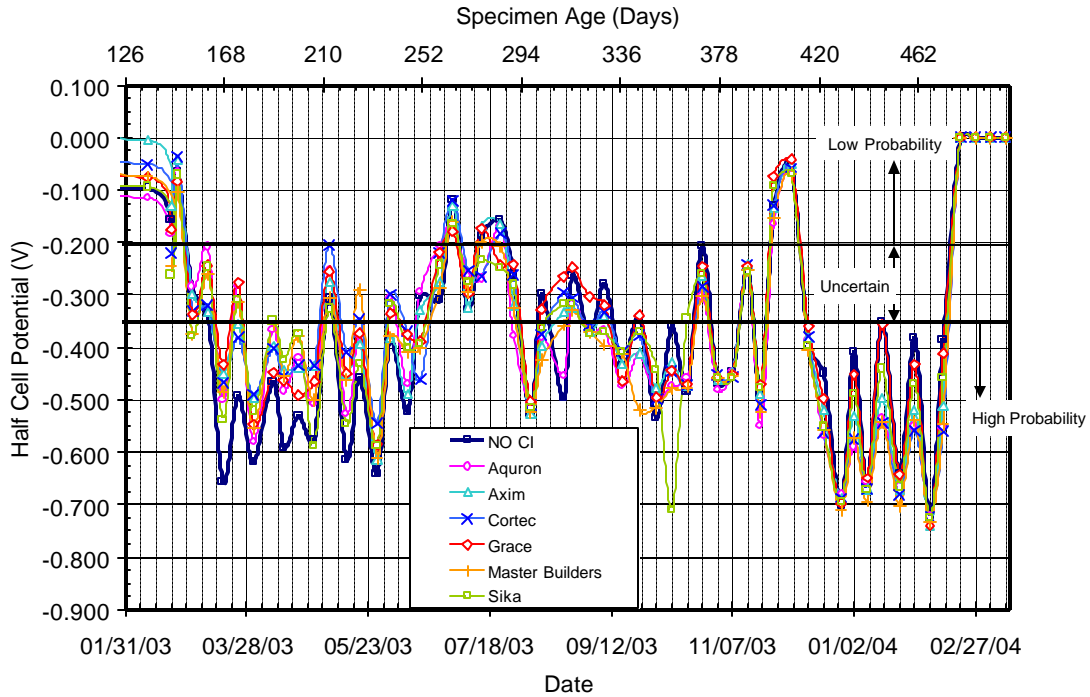
Figure 4.8 - Half Cell Readings for Bath 2, 0.0% Chloride, Pre-Cracked
