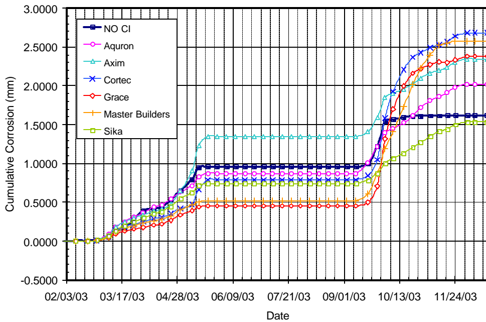
Figure B.32 – Cumulative Corrosion Over Time for Chamber Shelf 1, 3.0% Chloride, Post-Cracked
