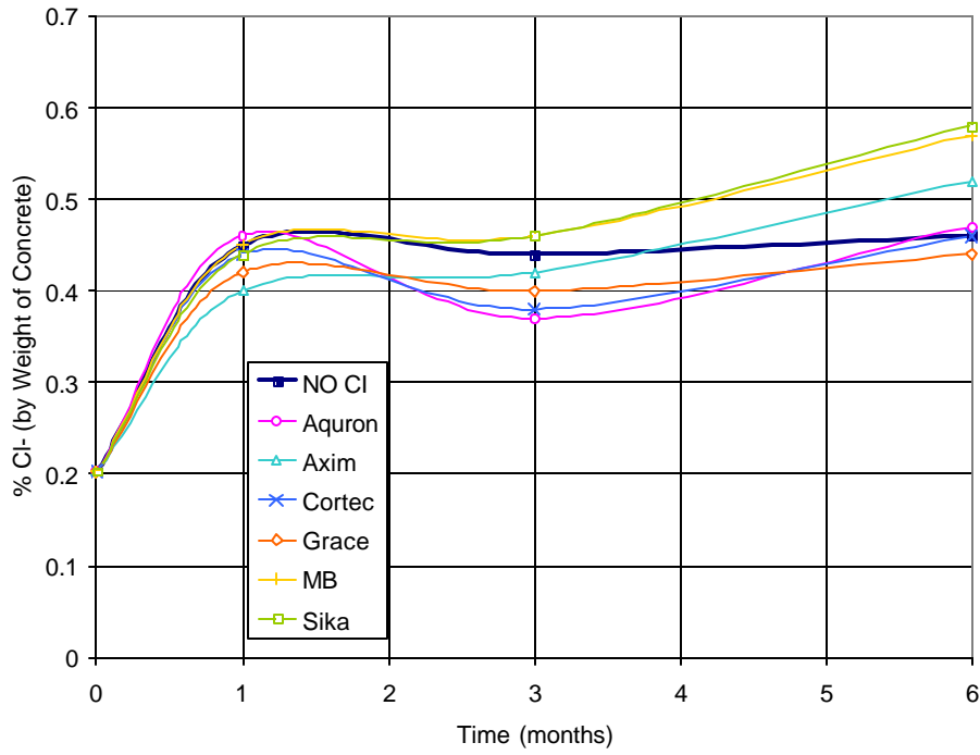
Figure D.11 – Chloride Content for Chamber Specimens 2.0% Chloride
