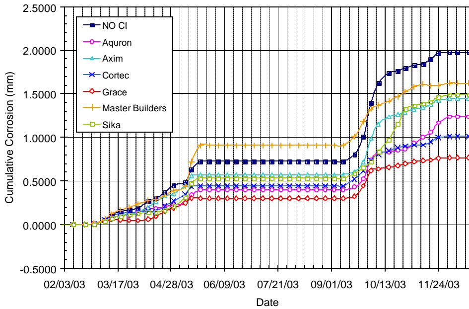
Figure B.37 – Cumulative Corrosion Over Time for Chamber Shelf 2, 2.0% Chloride, Pre-Cracked
