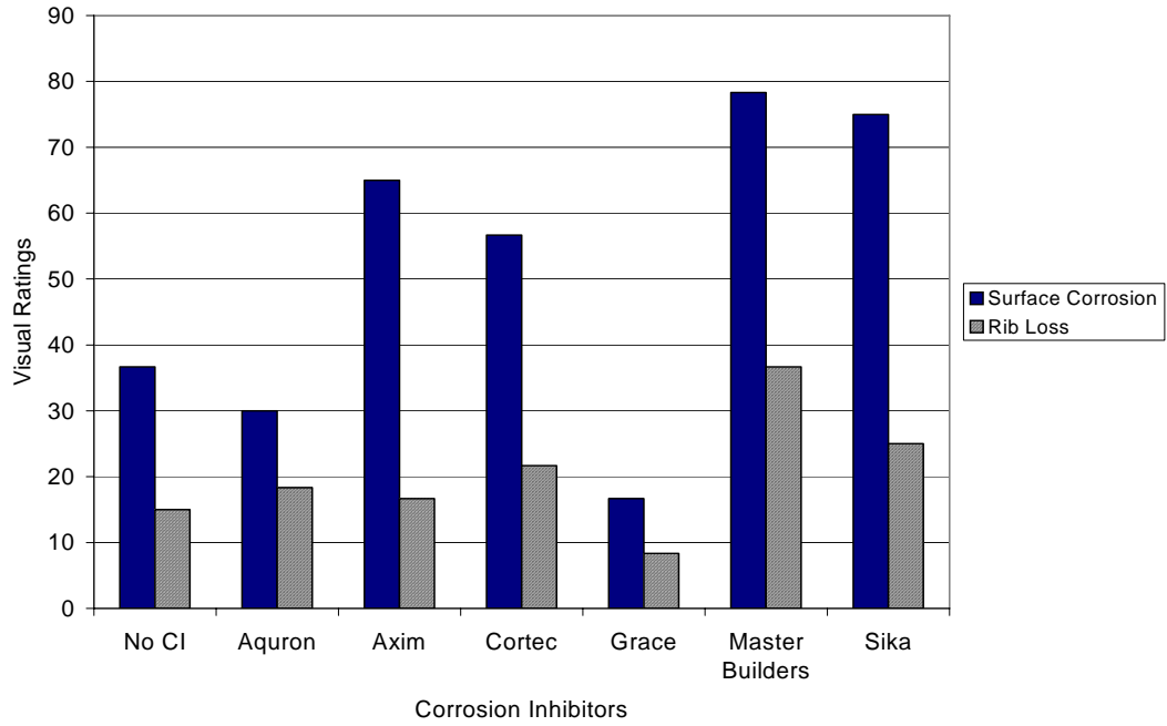
Figure G.83 – Visual Ratings for Chamber Shelf 3, 3.0% Chloride, Post-Cracked
