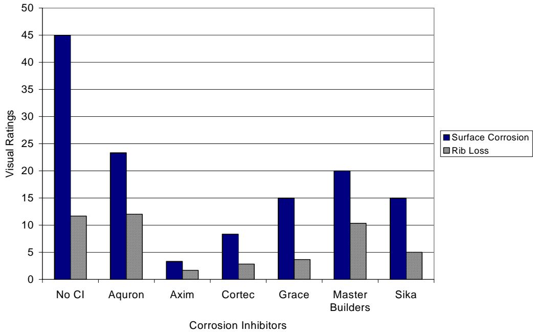
Figure G.63 – Visual Ratings for Chamber Shelf 2, 0.5% Chloride, Pre-Cracked
