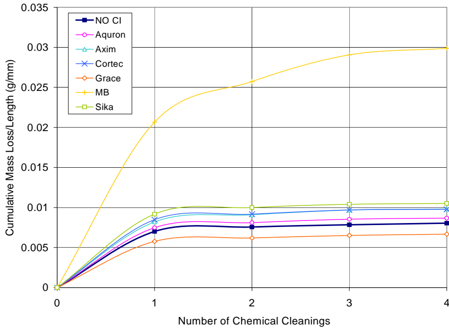
Figure F.19 – Cumulative Mass Loss/Length for Bath 3, 3.0% Chloride Post-Cracked Specimens
