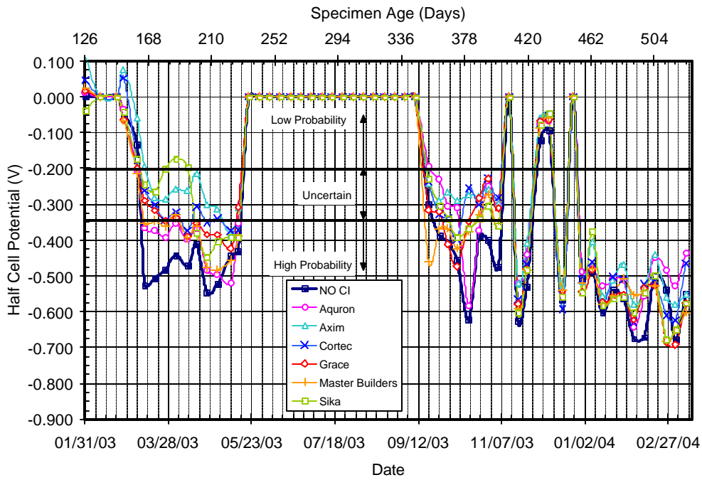
Figure C.45 – Half Cell Potential Readings for Chamber Shelf 4, 0.0% Chloride, Pre-Cracked
