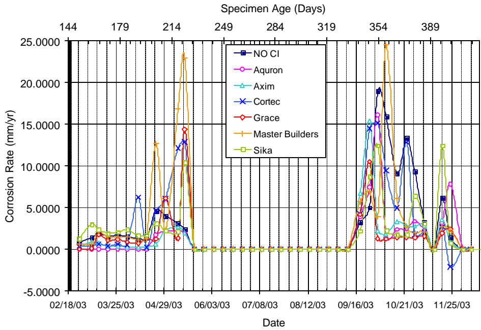
Figure A.30 – Corrosion Rate for Chamber Shelf 1, 1.5% Chloride, Post-Cracked
