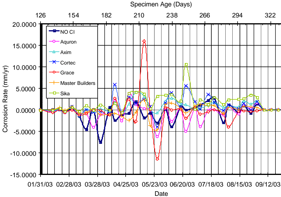
Figure A.6 – Corrosion Rate for Bath 1, 1.5% Chloride, Pre-Cracked
