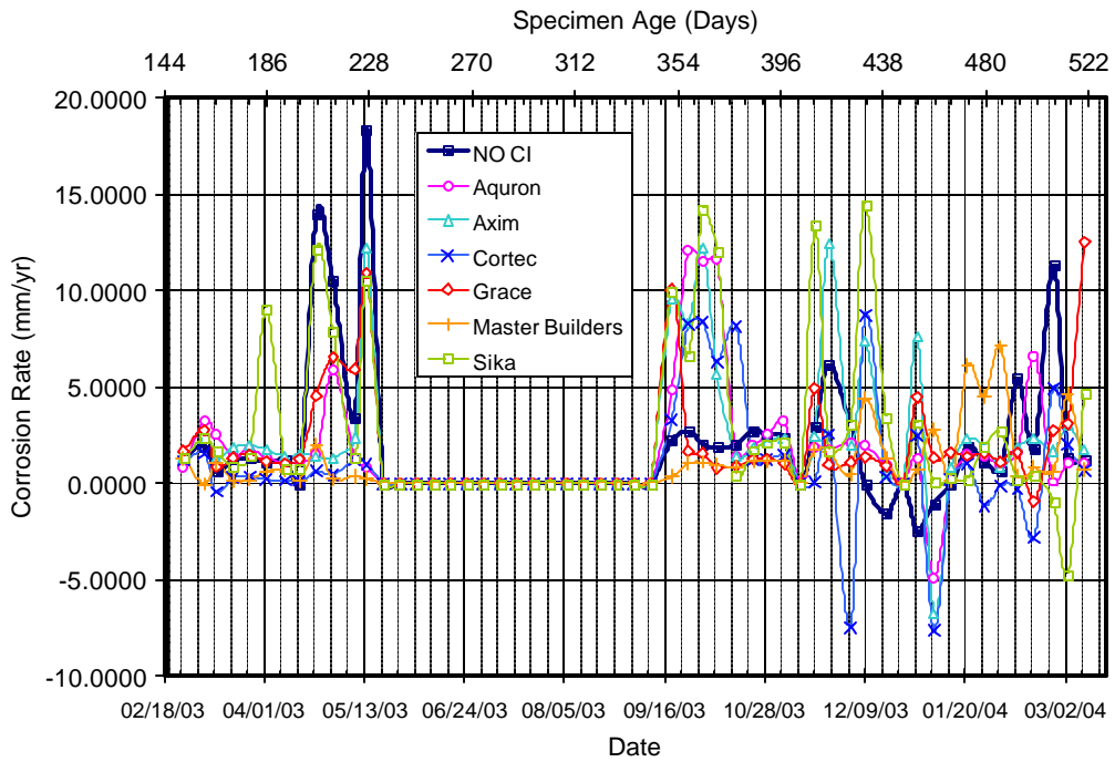
Figure A.49 – Corrosion Rate for Chamber Shelf 4, 2.0% Chloride, Pre-Cracked
