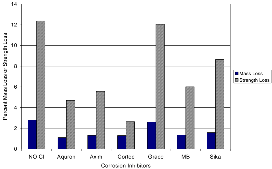
Figure G.14 – Mass Loss and Strength Loss for Bath 2, 0.0% Chloride, Pre-Cracked
