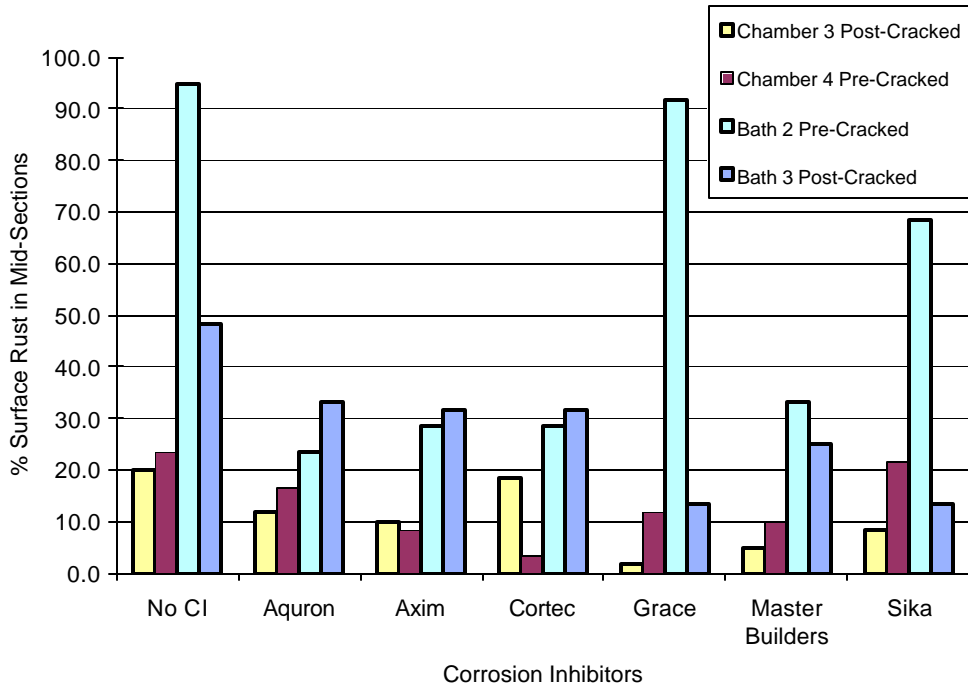
Figure E.15 Surface Corrosion at Mid Section for 0.0% Chloride (Set#2)
