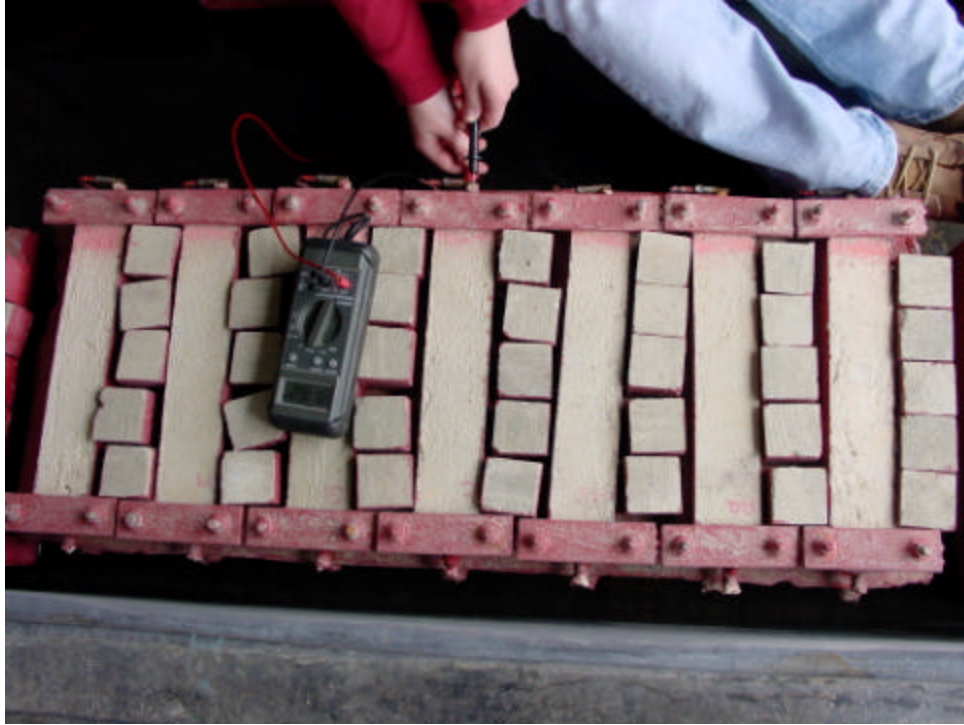
Figure 3.21 – Typical Voltmeter Reading Procedure
