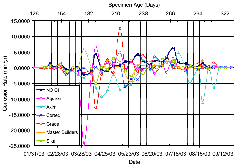
Figure A.7 – Corrosion Rate for Bath 1, 2.0% Chloride, Pre-Cracked
