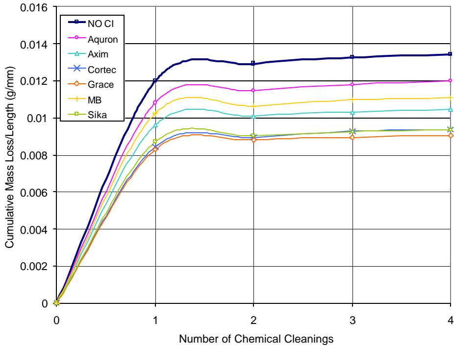
Figure 4.36 – Cumulative Mass Loss/Length for Bath 4, 0.0% Chloride, Post-Cracked Specimens
