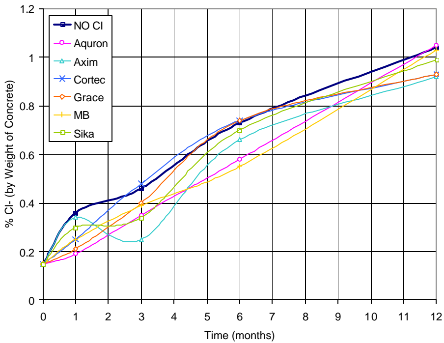
Figure D.5 – Chloride Content for Bath Specimens – 1.5% Chloride
