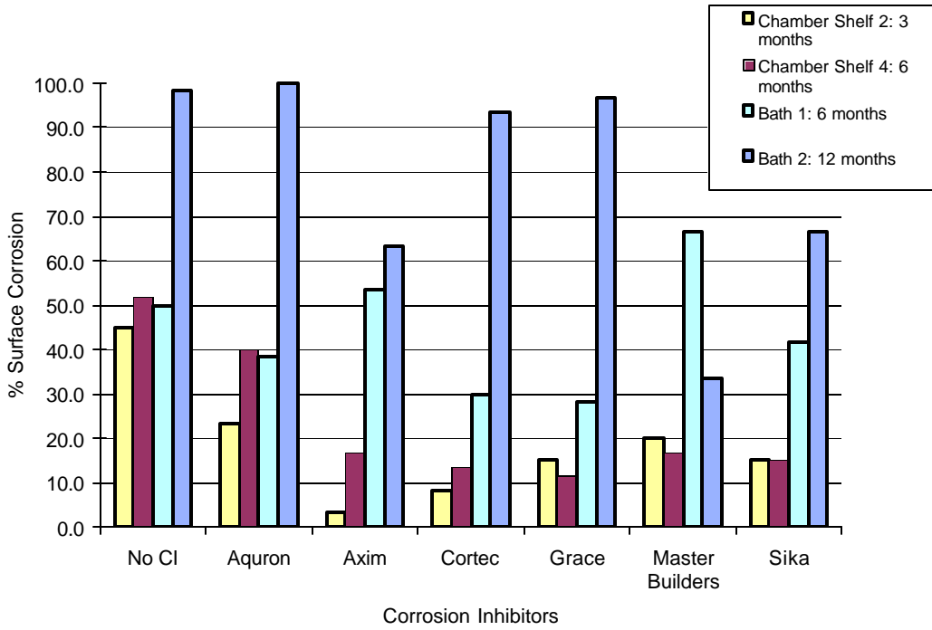
Figure E.31 Time Step of Surface Corrosion for 0.5% Chloride Pre-Cracked Specimens
