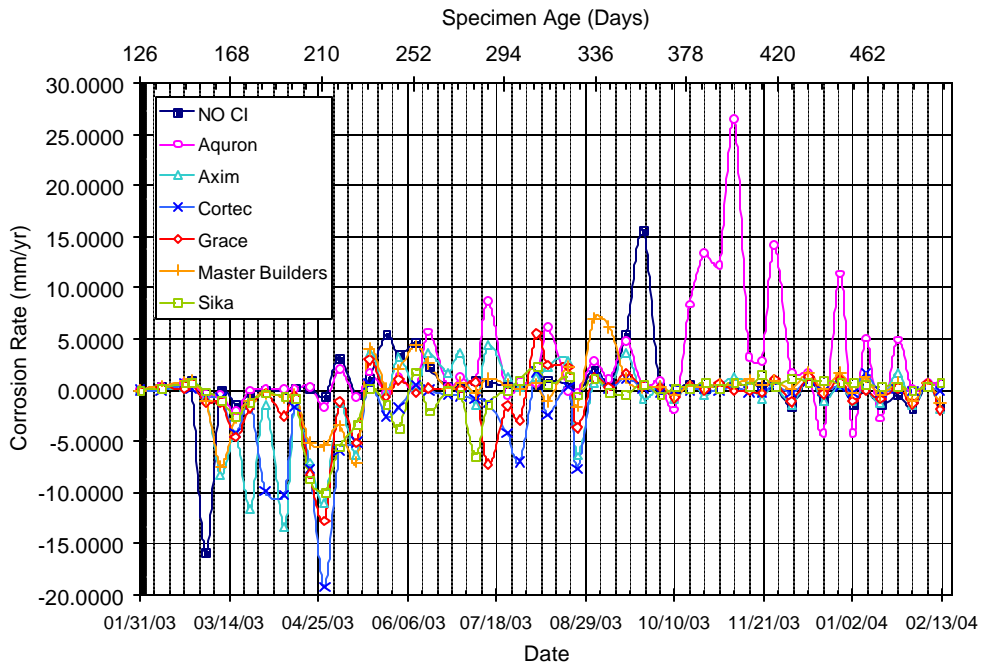
Figure A.14 – Corrosion Rate for Bath 2, 3.0% Chloride, Pre-Cracked
