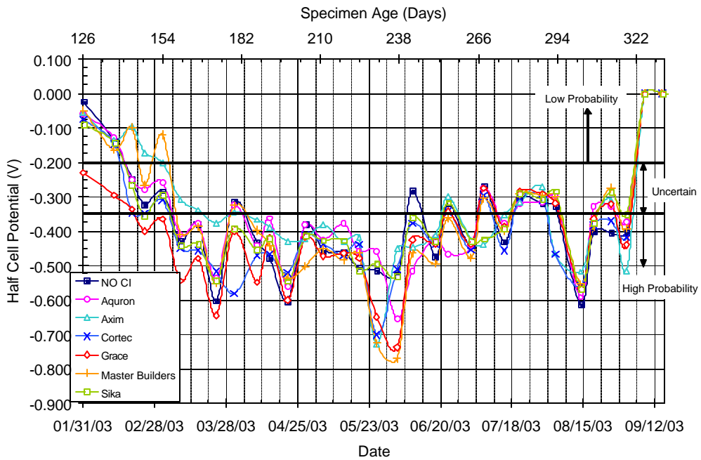
Figure C.8 – Half Cell Potential Readings for Bath 1, 3.0% Chloride, Pre-Cracked
