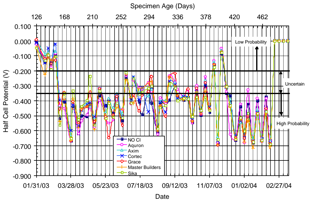
Figure C.16 – Half Cell Potential Readings for Bath 3, 0.5% Chloride, Post-Cracked
