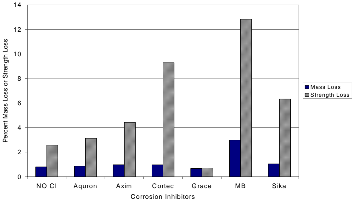
Figure G.36 – Mass Loss and Strength Loss for Bath 3, 3.0% Chloride, Post-Cracked
