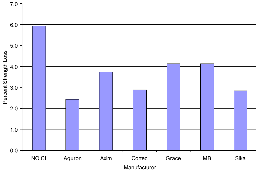
Figure 4.39 – Percent Strength Loss Based on Tension Tests for Bath 3, 0.0% Chloride, Post-Cracked
