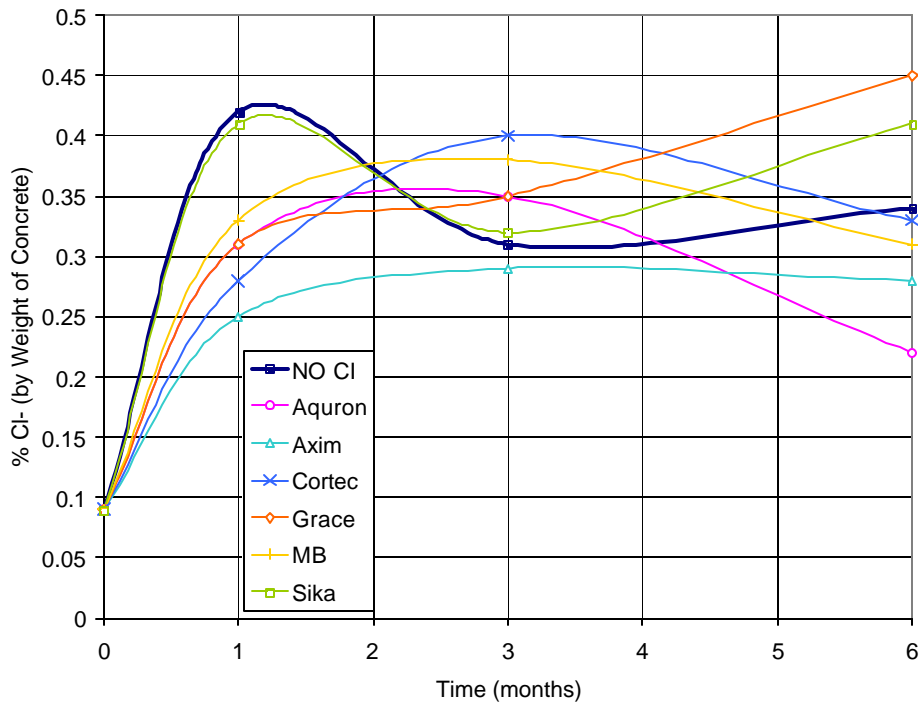
Figure D.10 – Chloride Content for Chamber Specimens – 1.0% Chloride
