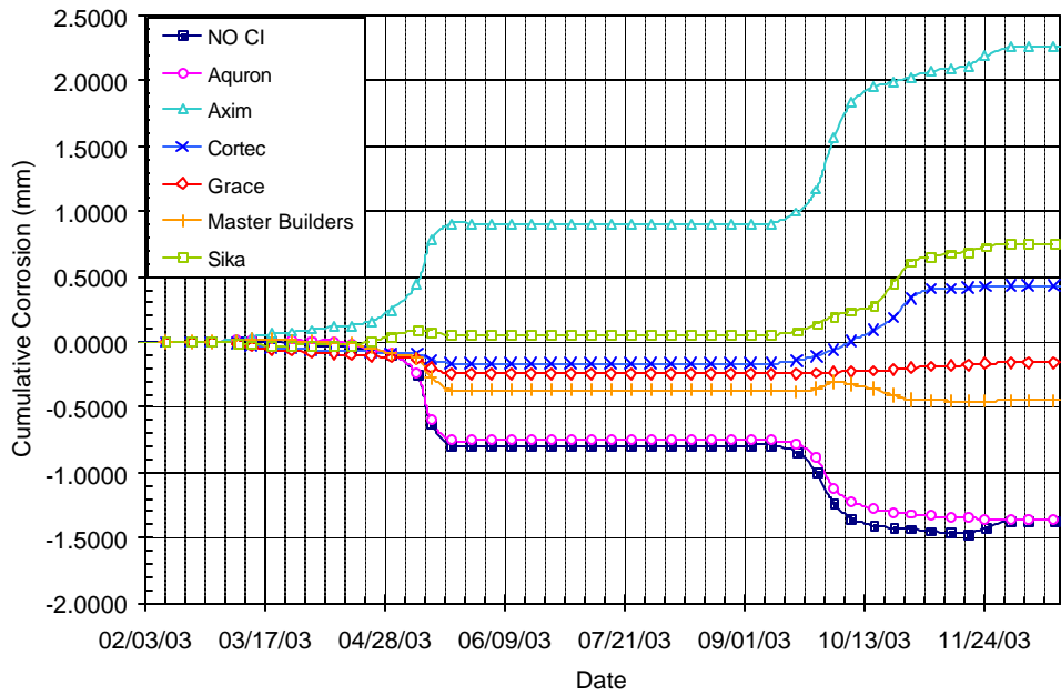
Figure B.35 – Cumulative Corrosion Over Time for Chamber Shelf 2, 1.0% Chloride, Pre-Cracked
