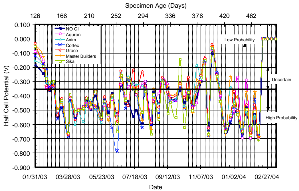
Figure C.20 – Half Cell Potential Readings for Bath 3, 3.0% Chloride, Post-Cracked
