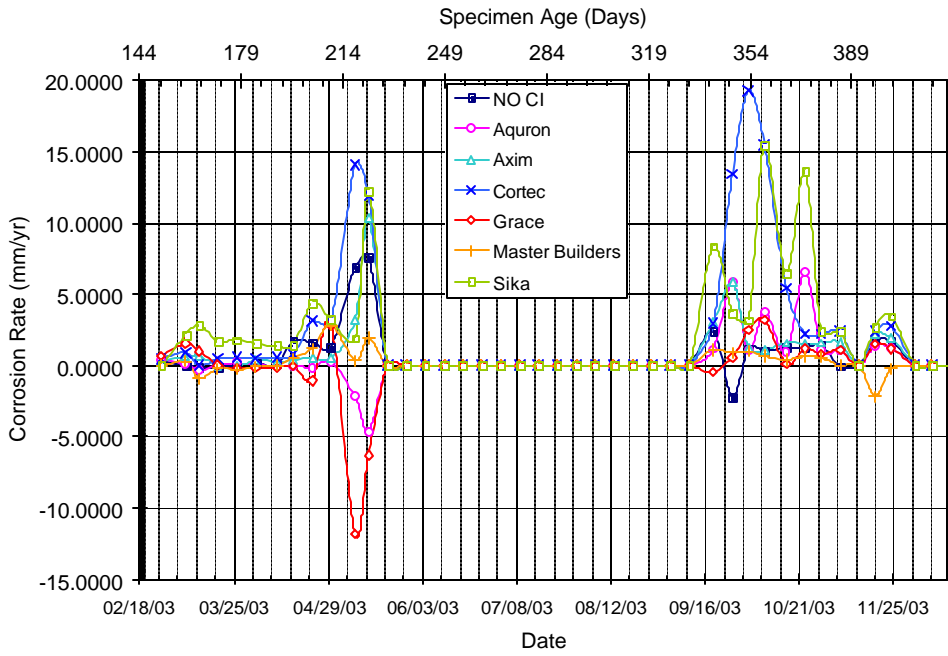
Figure A.29 – Corrosion Rate for Chamber Shelf 1, 1.0% Chloride, Post-Cracked
