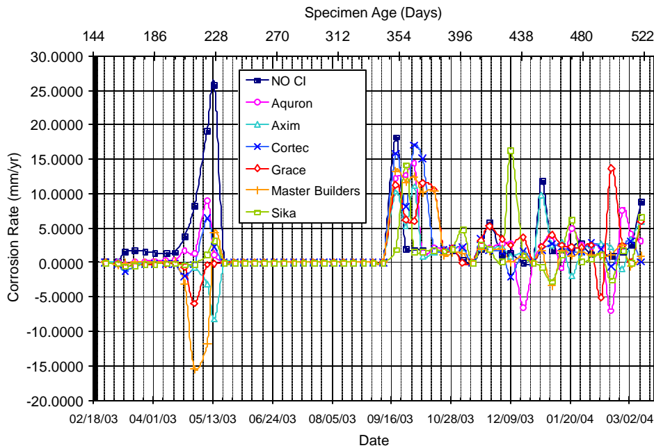
Figure A.46 – Corrosion Rate for Chamber Shelf 4, 0.5% Chloride, Pre-Cracked
