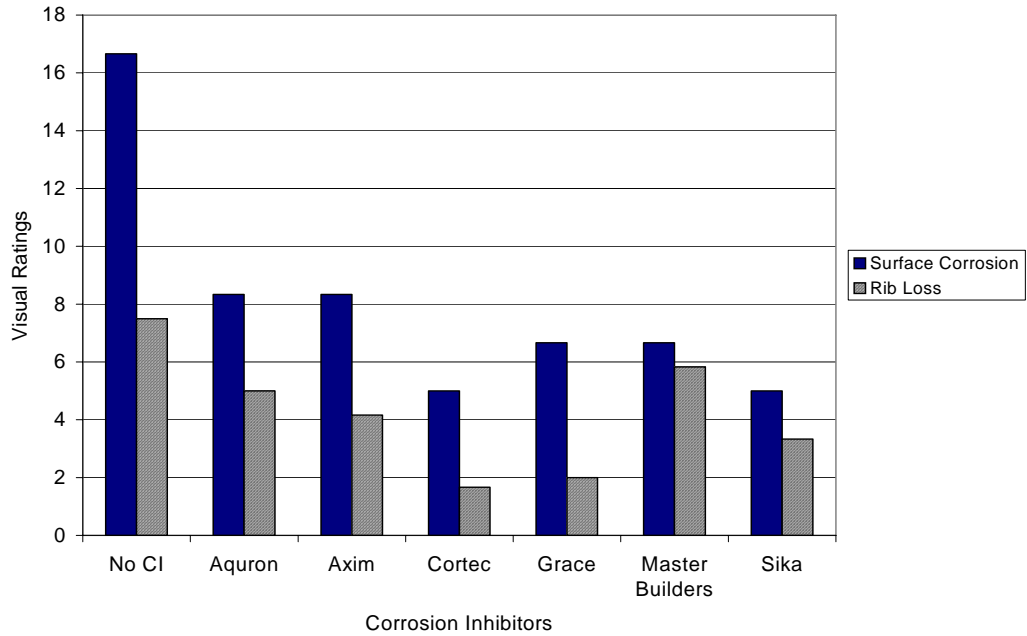
Figure G.61 – Visual Ratings for Chamber Shelf 2, 0.0% Chloride, Pre-Cracked
