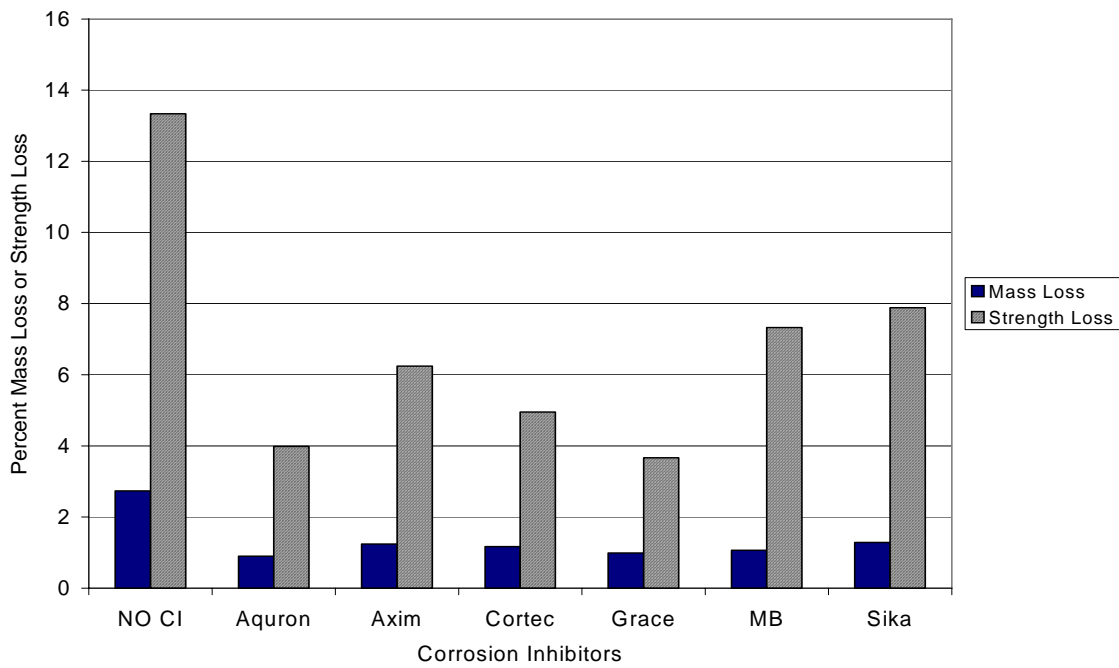
Figure G.44 – Mass Loss and Strength Loss for Bath 4, 1.5% Chloride, Post-Cracked
