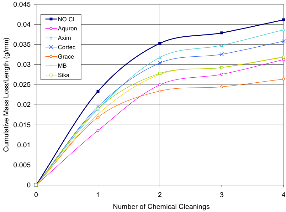
Figure F.17 – Cumulative Mass Loss/Length for Bath 3, 1.5% Chloride Post-Cracked Specimens
