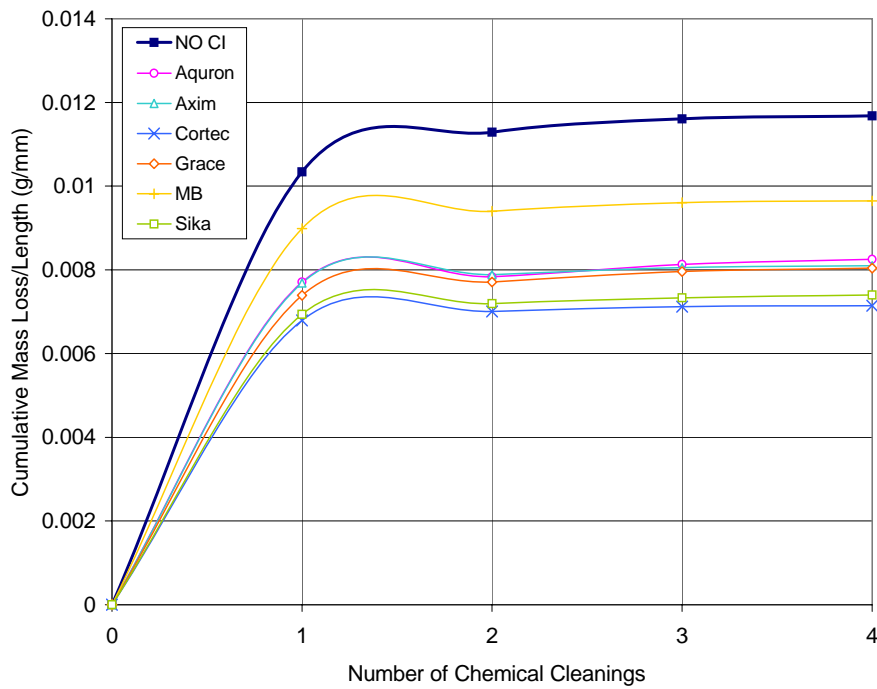
Figure F.31 – Cumulative Mass Loss/Length for Chamber Shelf 1 3.0% Chloride, Post-Cracked Specimens
