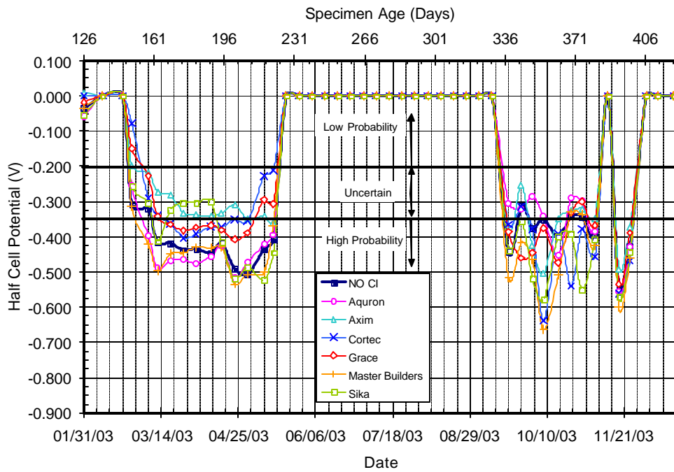
Figure C.36 – Half Cell Potential Readings for Chamber Shelf 2, 1.5% Chloride, Pre-Cracked
