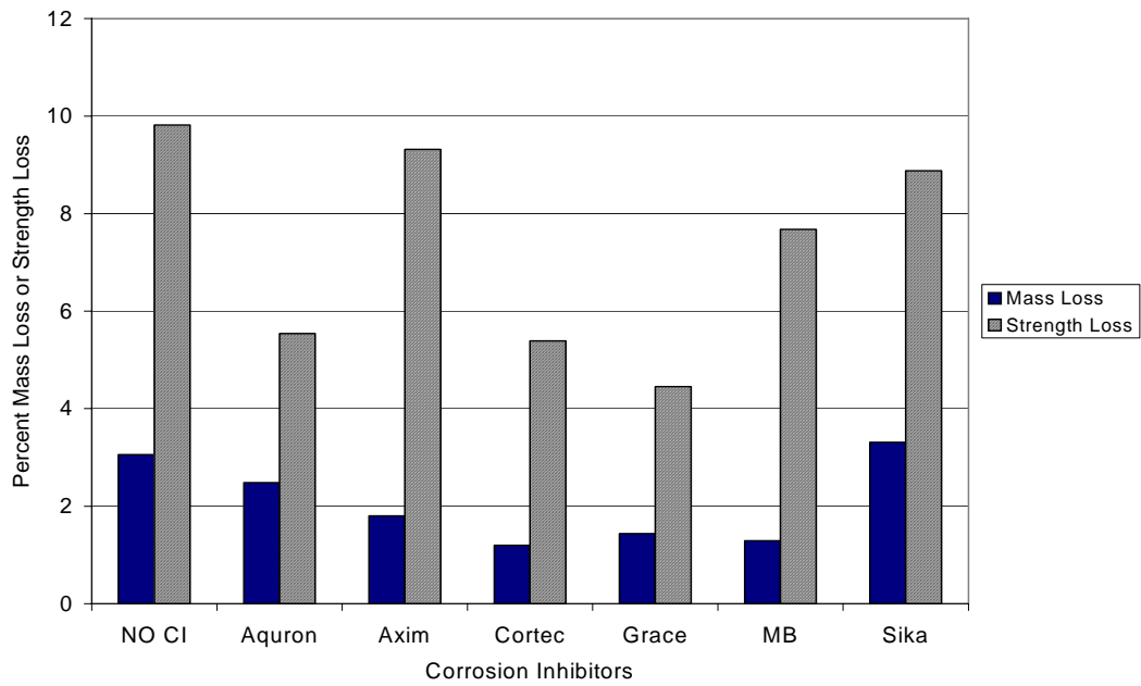
Figure G.58 – Mass Loss and Strength Loss for Chamber Shelf 1, 2.0% Chloride, Post-Cracked
