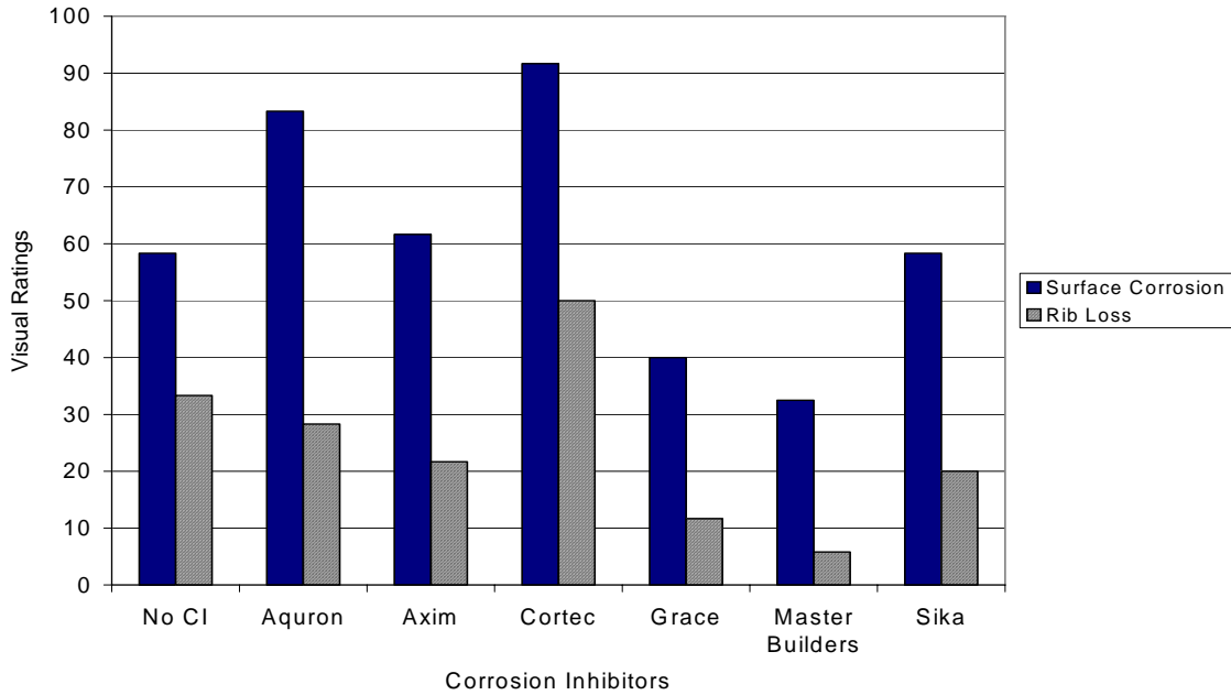
Figure G.45 – Visual Ratings for Bath 4, 2.0% Chloride, Post-Cracked
