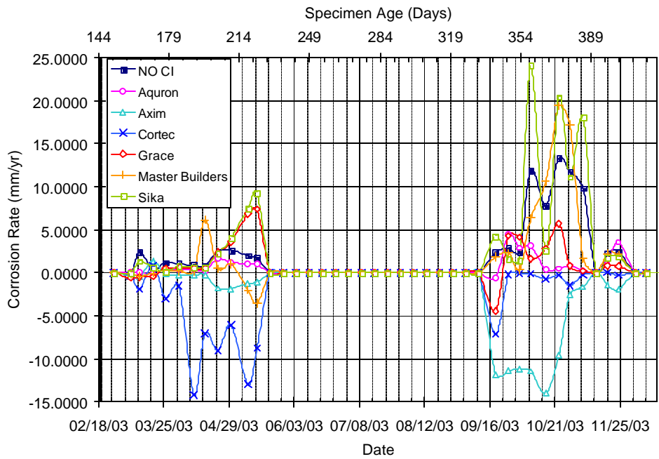
Figure A.33 – Corrosion Rate for Chamber Shelf 2, 0.0% Chloride, Pre-Cracked
