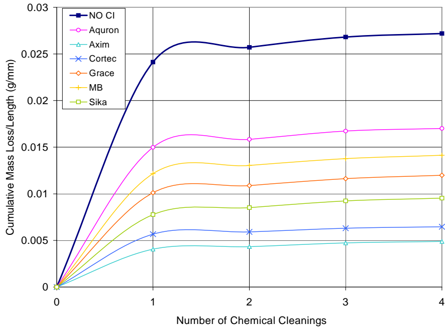
Figure F.33 – Cumulative Mass Loss/Length for Chamber Shelf 2 0.5% Chloride, Pre-Cracked Specimens
