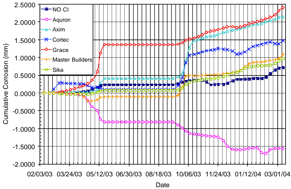
Figure B.47 – Cumulative Corrosion Over Time for Chamber Shelf 4, 1.0% Chloride, Pre-Cracked
