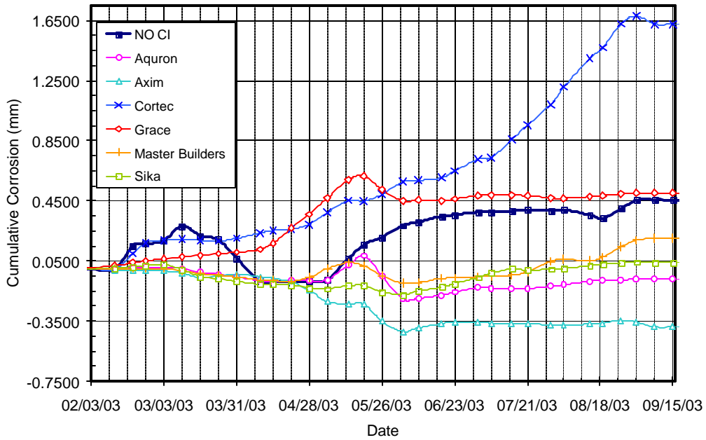
Figure B.8 – Cumulative Corrosion Over Time for Bath 1, 3.0% Chloride, Pre-Cracked
