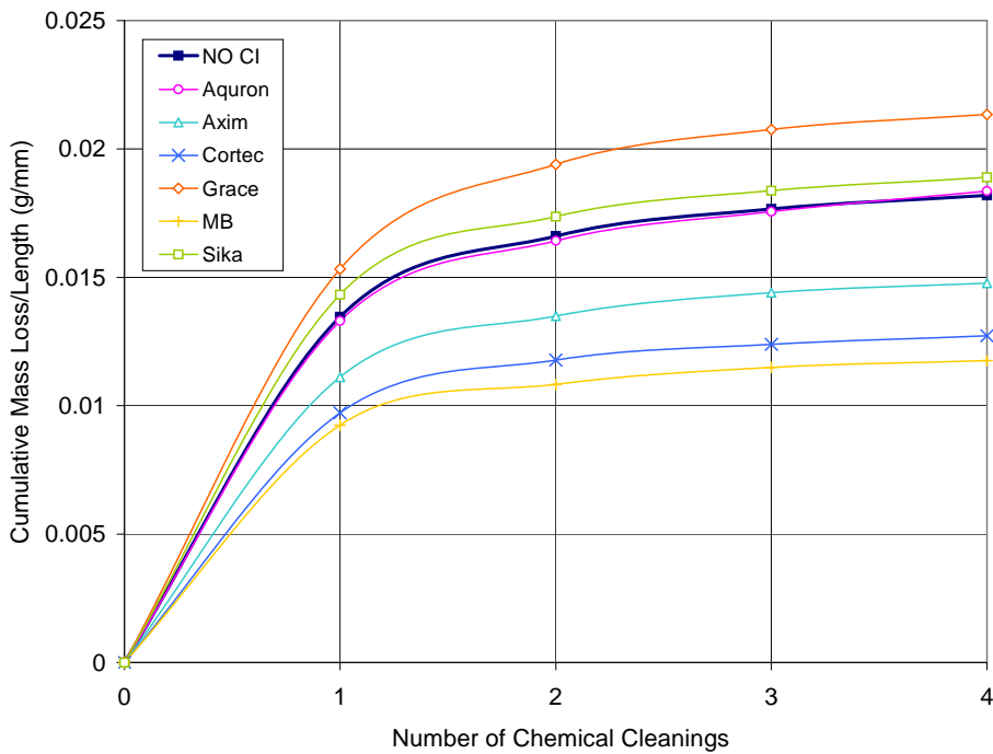
Figure F.41 – Cumulative Mass Loss/Length for Chamber Shelf 3 1.5% Chloride, Post-Cracked Specimens
