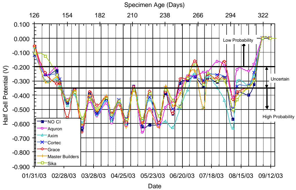
Figure C.25 – Half Cell Potential Readings for Bath 4, 2.0% Chloride, Post-Cracked
