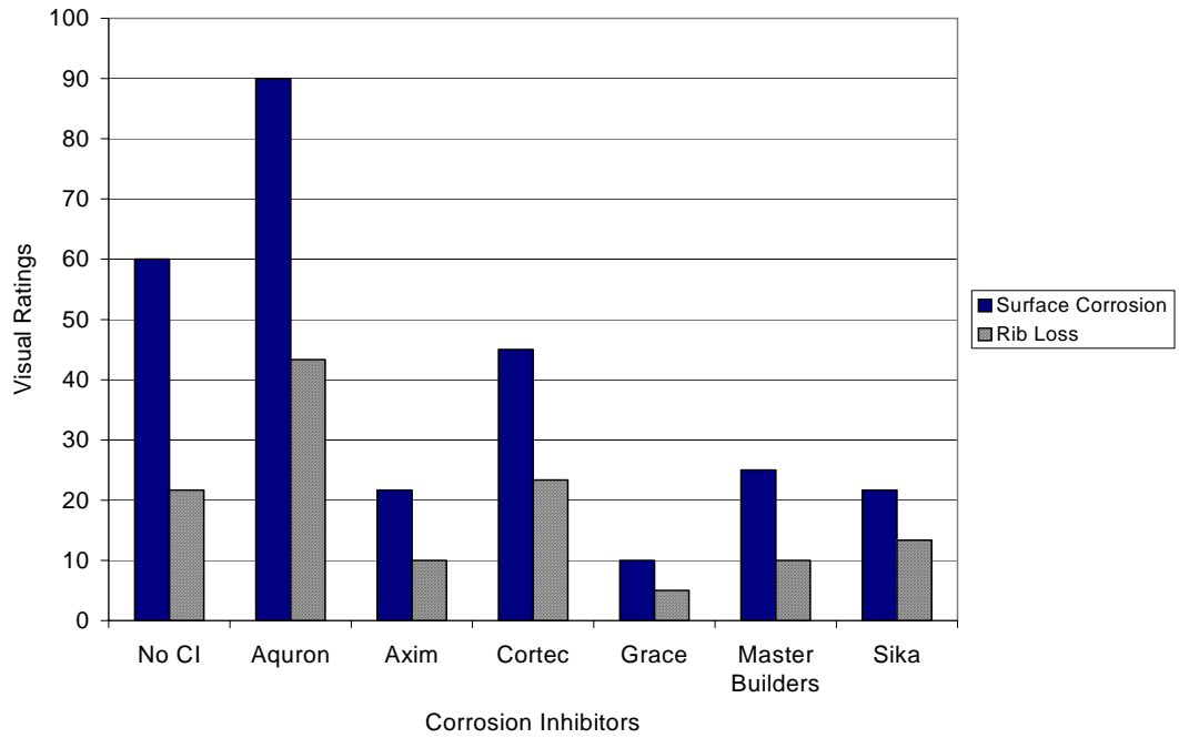
Figure G.91 – Visual Ratings for Chamber Shelf 4, 1.5% Chloride, Pre-Cracked
