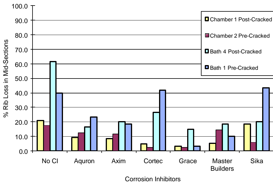
Figure E.8 Rib Loss at Mid Section for 1.5% Chloride (Set #1)
