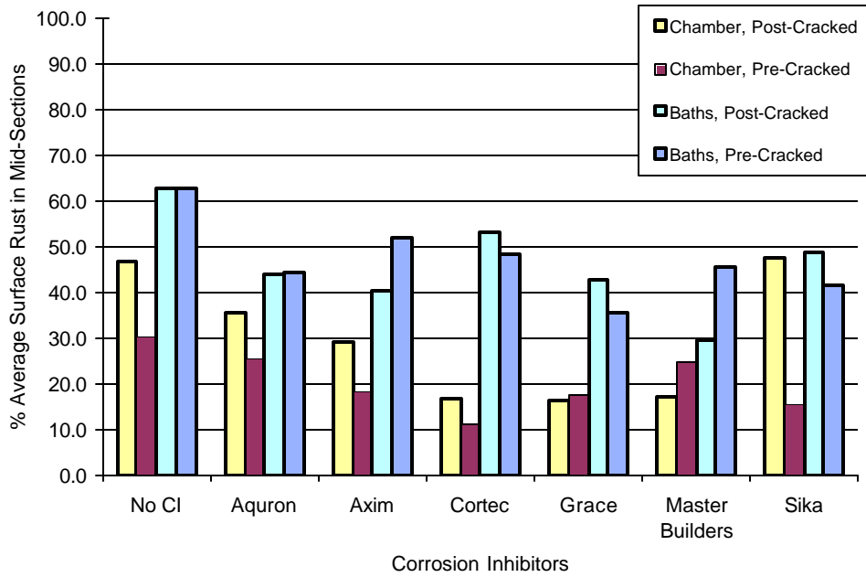
Figure E.13 Surface Corrosion at Mid Section for Average of all Chloride Contaminants (Set#1)
