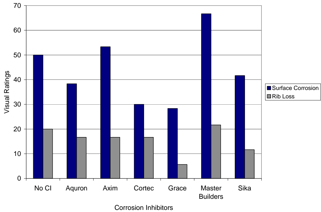
Figure G.3 – Visual Ratings for Bath 1, 0.5% Chloride, Pre-Cracked
