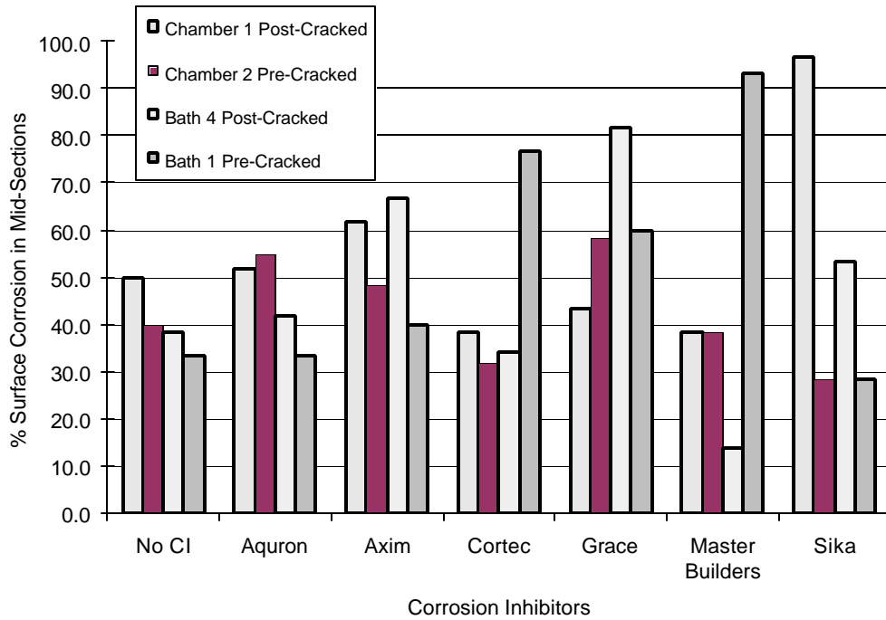
Figure 4.23 - % Surface Corrosion at Midsection for 3.0% Chloride (Set #1)
