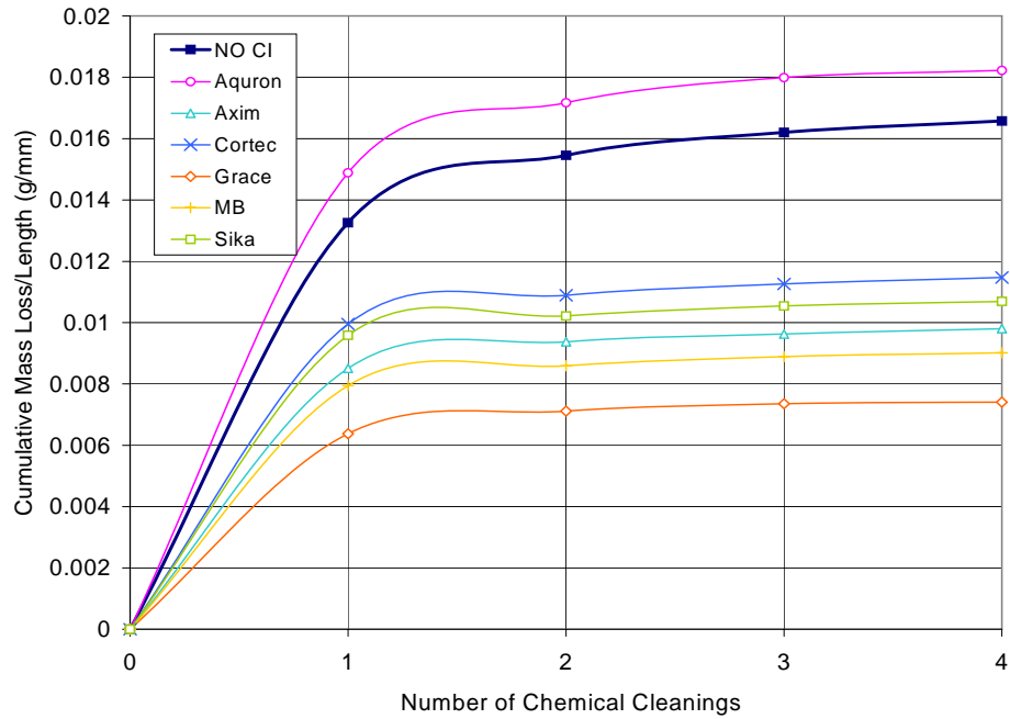
Figure F.45 – Cumulative Mass Loss/Length for Chamber Shelf 4 0.5% Chloride, Pre-Cracked Specimens
