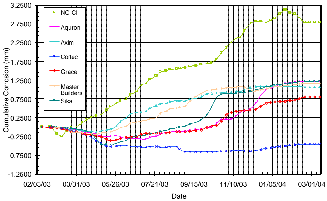
Figure 4.5 - Cumulative Corrosion Over Time for Bath 2, 0.0% Chloride, Pre-Cracked
