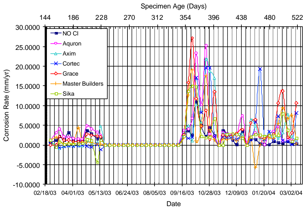
Figure A.42 – Corrosion Rate for Chamber Shelf 3, 1.5% Chloride, Post-Cracked
