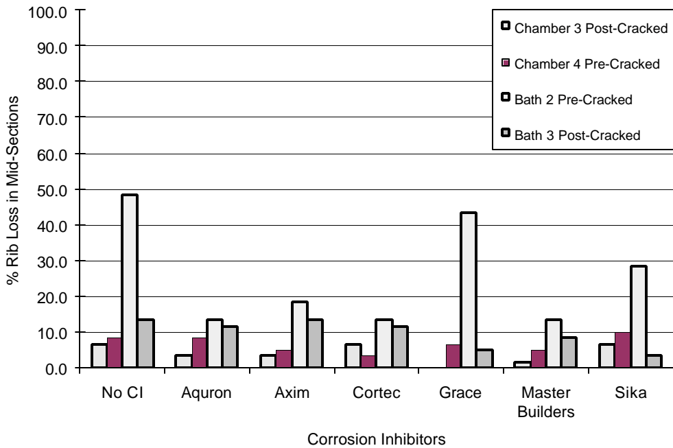
Figure 4.31 - % Rib Loss in Midsections for 0.0% Chloride (Set #2)
