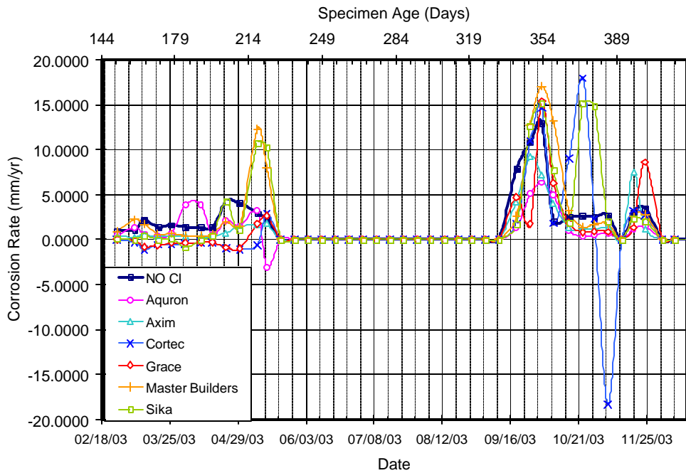
Figure A.36 – Corrosion Rate for Chamber Shelf 2, 1.5% Chloride, Pre-Cracked
