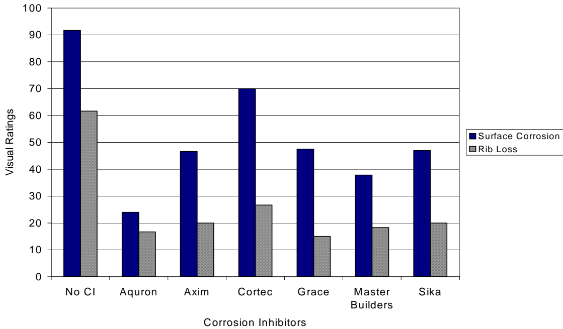
Figure G.43 – Visual Ratings for Bath 4, 1.5% Chloride, Post-Cracked
