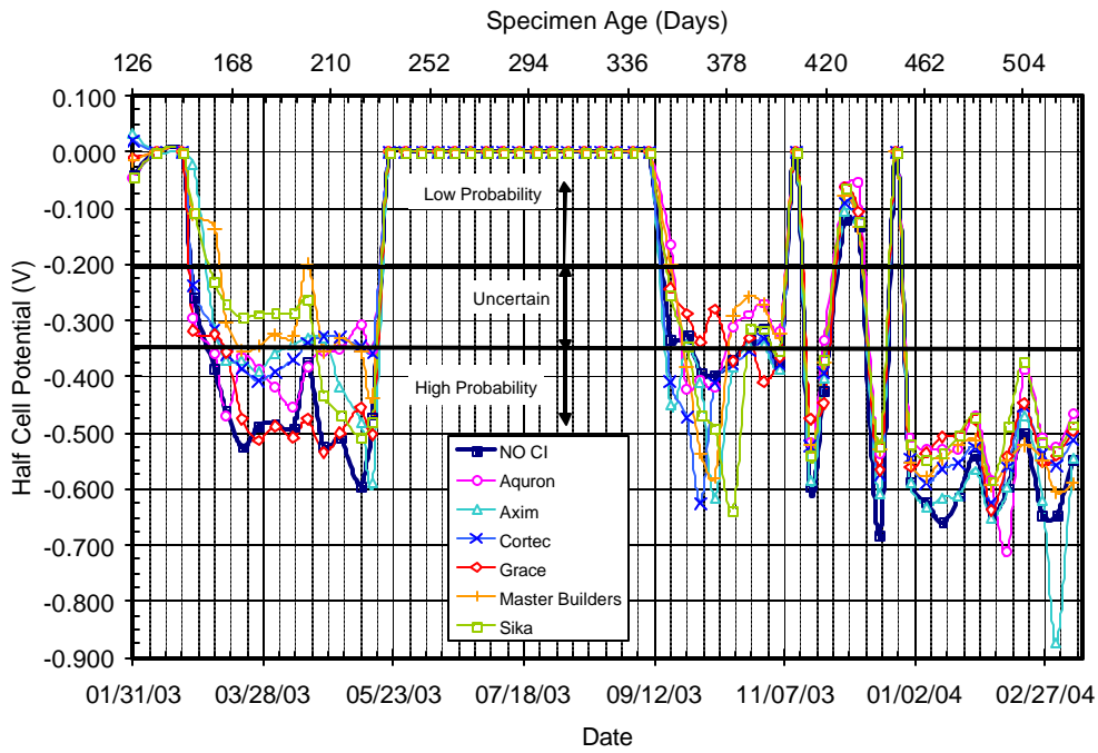
Figure C.47 – Half Cell Potential Readings for Chamber Shelf 4, 1.0% Chloride, Pre-Cracked
