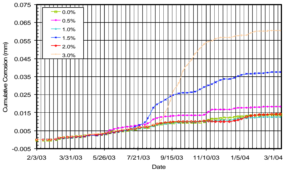
Figure B.2 – Cumulative Corrosion Over Time for Control Set #2
