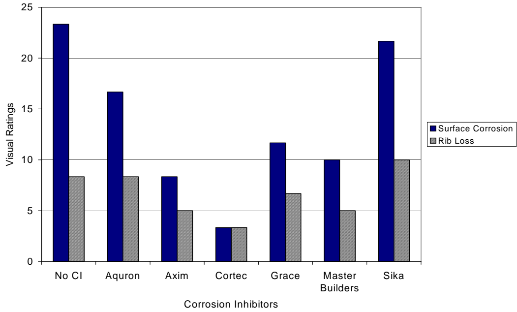
Figure G.85 – Visual Ratings for Chamber Shelf 4, 0.0% Chloride, Pre-Cracked
