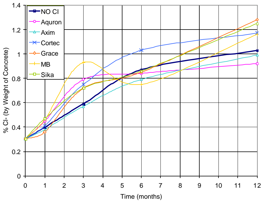
Figure D.7 – Chloride Content for Bath Specimens – 3.0% Chloride
