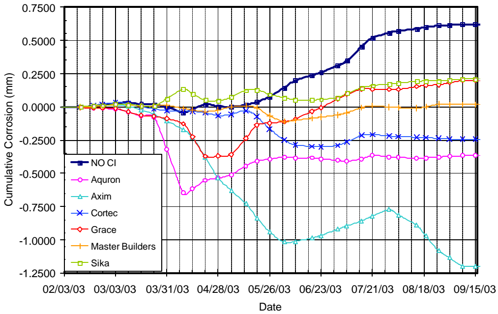
Figure B.7 – Cumulative Corrosion Over Time for Bath 1, 2.0% Chloride, Pre-Cracked
