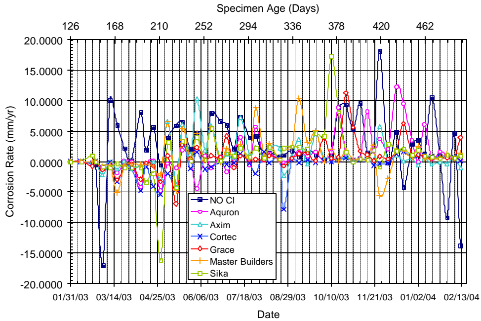
Figure A.9 – Corrosion Rate for Bath 2, 0.0% Chloride, Pre-Cracked
