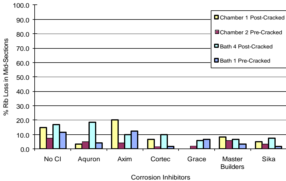
Figure E.2 Rib Loss at Mid Section for 0.0% Chloride (Set #1)
