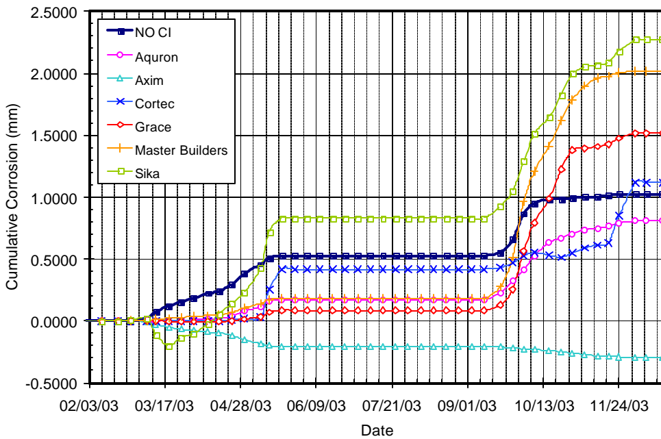
Figure B.34 – Cumulative Corrosion Over Time for Chamber Shelf 2, 0.5% Chloride, Pre-Cracked
