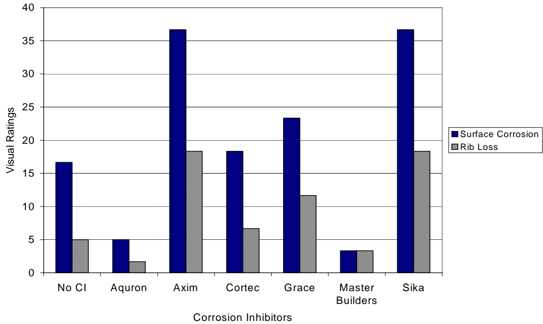
Figure G.89 – Visual Ratings for Chamber Shelf 4, 1.0% Chloride, Pre-Cracked
