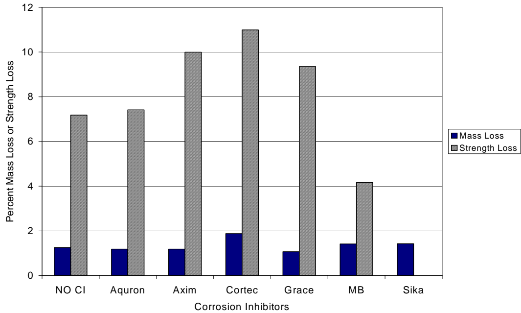
Figure G.78 – Mass Loss and Strength Loss for Chamber Shelf 3, 1.0% Chloride, Post-Cracked
