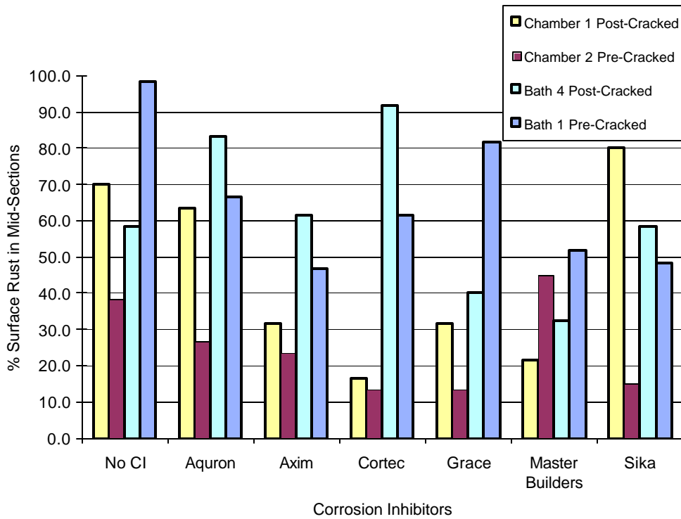
Figure E.9 Surface Corrosion at Mid Section for 2.0% Chloride (Set#1)
