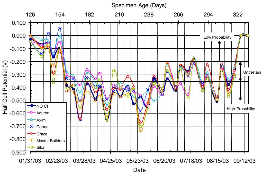
Figure C.4 – Half Cell Potential Readings for Bath 1, 0.5% Chloride, Pre-Cracked
