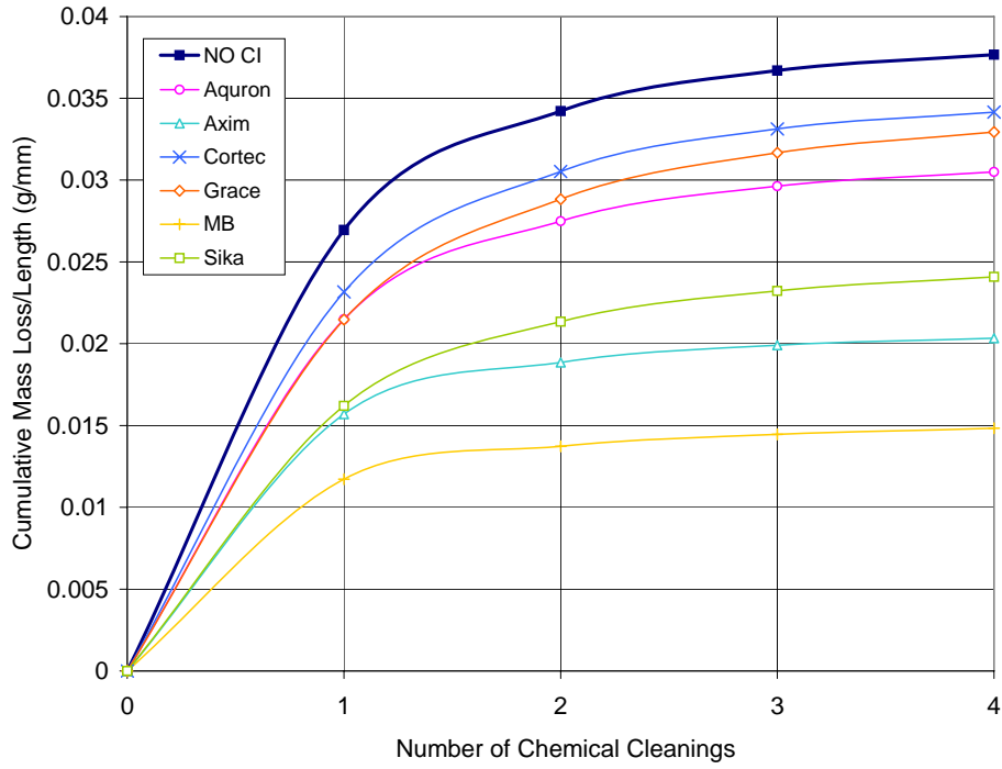
Figure F.9 – Cumulative Mass Loss/Length for Bath 2, 0.5% Chloride Pre-Cracked Specimens
