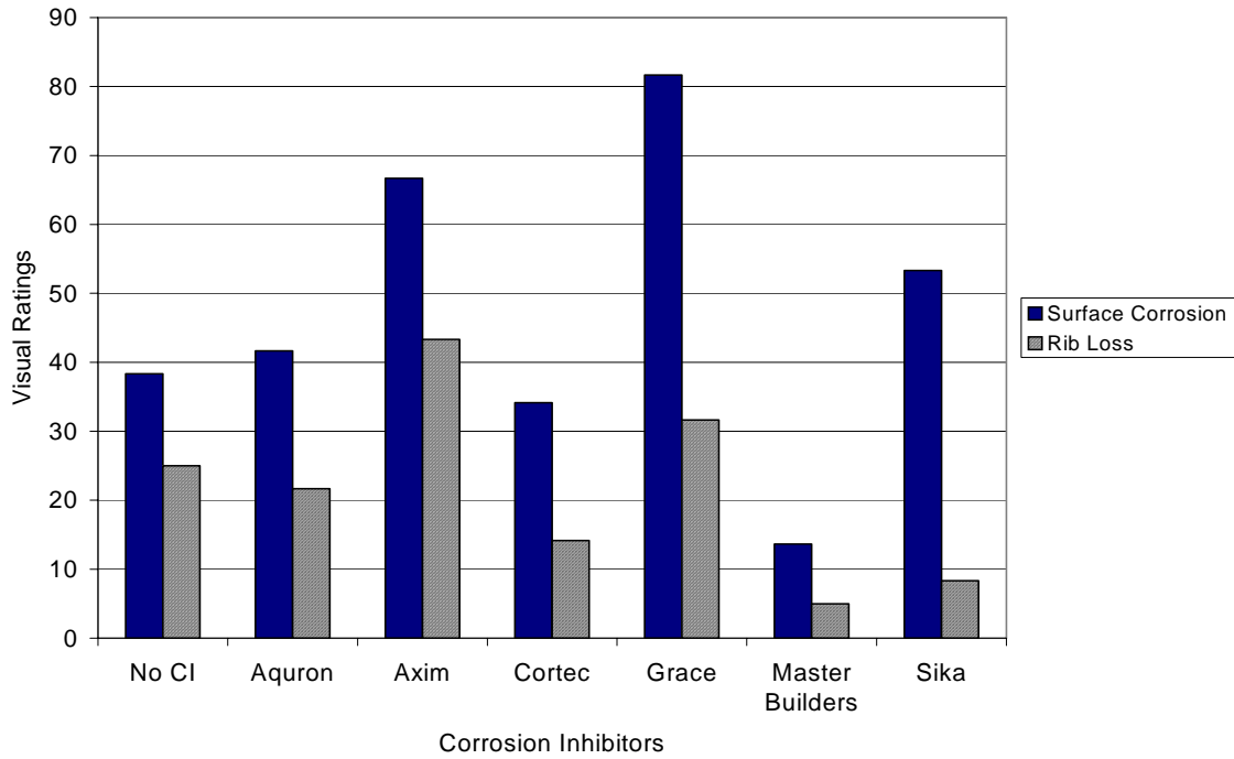
Figure G.47 – Visual Ratings for Bath 4, 3.0% Chloride, Post-Cracked
