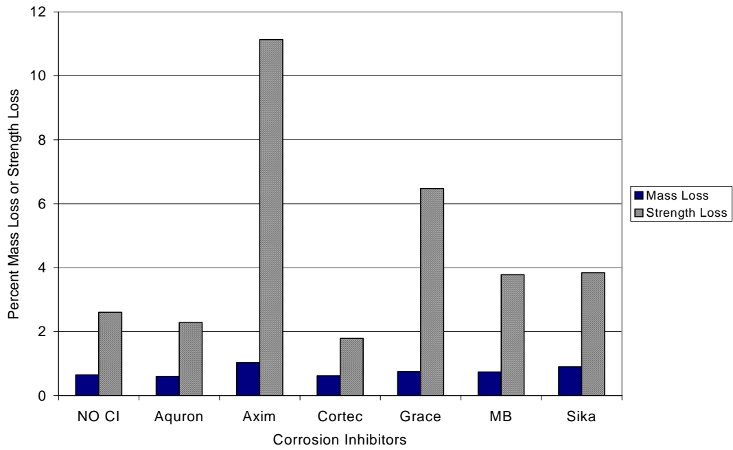
Figure G.66 – Mass Loss and Strength Loss for Chamber Shelf 2, 1.0% Chloride, Pre-Cracked
