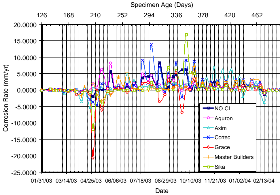
Figure A.15 – Corrosion Rate for Bath 3, 0.0% Chloride, Post-Cracked
