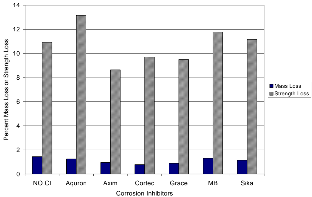
Figure G.68 – Mass Loss and Strength Loss for Chamber Shelf 2, 1.5% Chloride, Pre-Cracked
