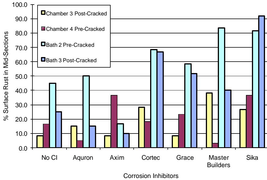
Figure E.19 Surface Corrosion at Mid Section for 1.0% Chloride (Set#2)
