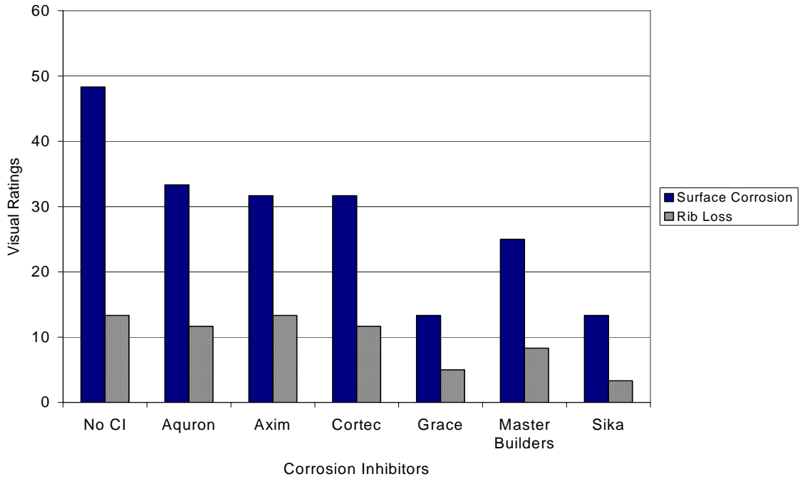
Figure G.25 – Visual Ratings for Bath 3, 0.0% Chloride, Post-Cracked
