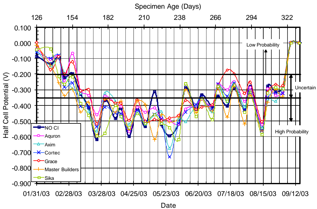
Figure C.6 – Half Cell Potential Readings for Bath 1, 1.5% Chloride, Pre-Cracked
