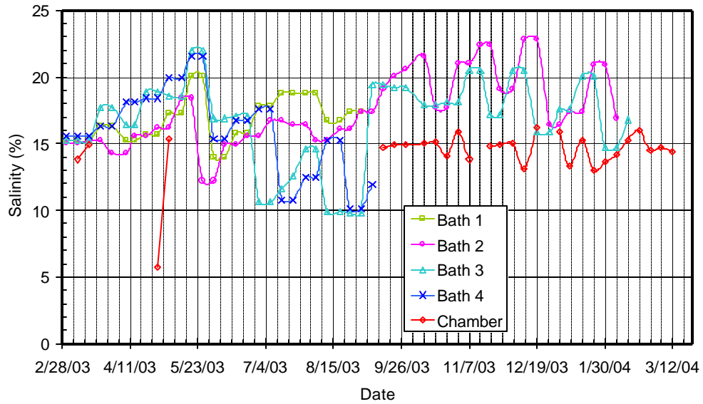
Figure 4.10 - Salinity Over Time for Bath and Chamber Environments
