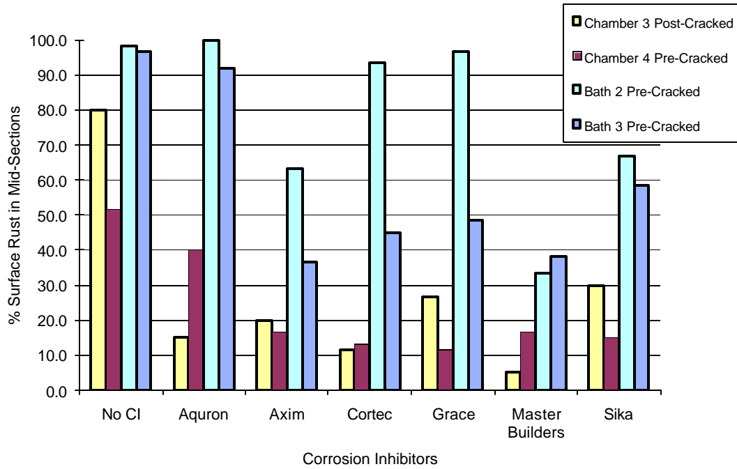
Figure E.17 Surface Corrosion at Mid Section for 0.5% Chloride (Set#2)
