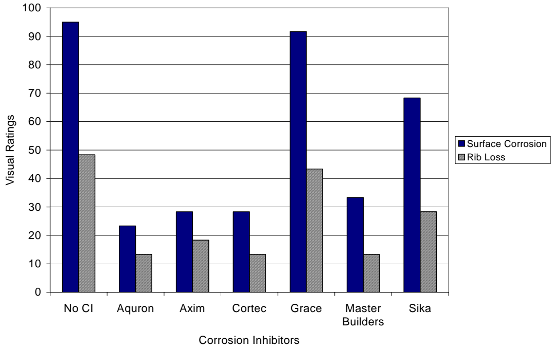
Figure G.13 – Visual Ratings for Bath 2, 0.0% Chloride, Pre-Cracked
