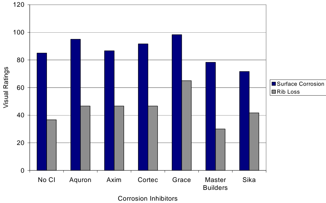
Figure G.33 – Visual Ratings for Bath 3, 2.0% Chloride, Post-Cracked
