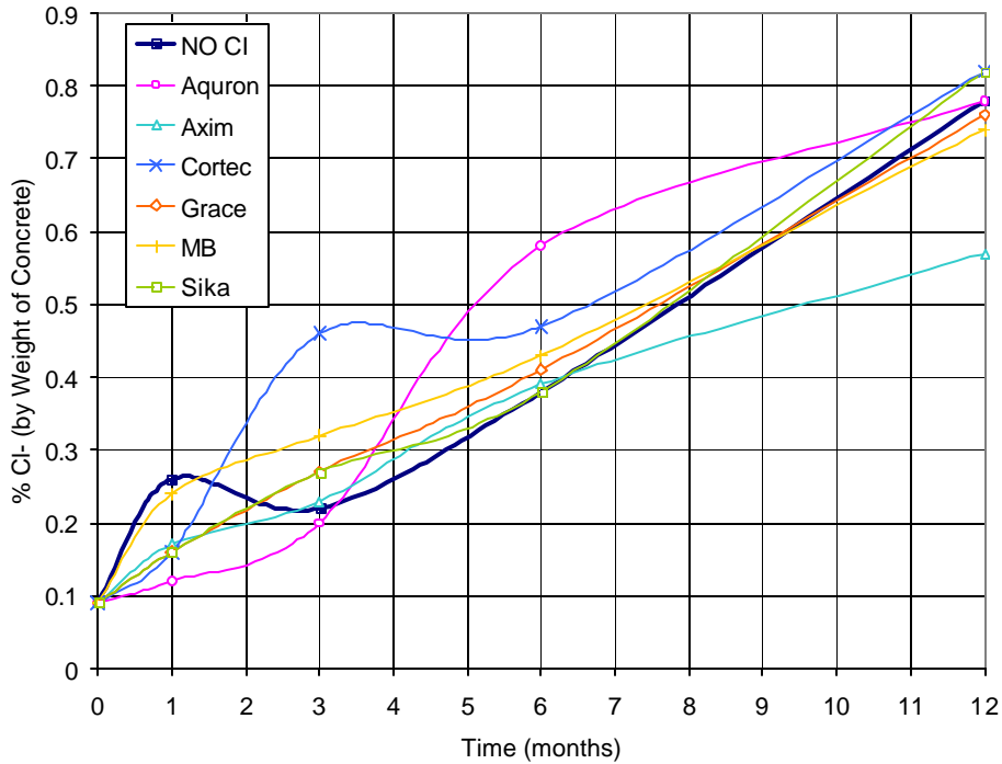
Figure D.4 – Chloride Content for Bath Specimens – 1.0% Chloride
