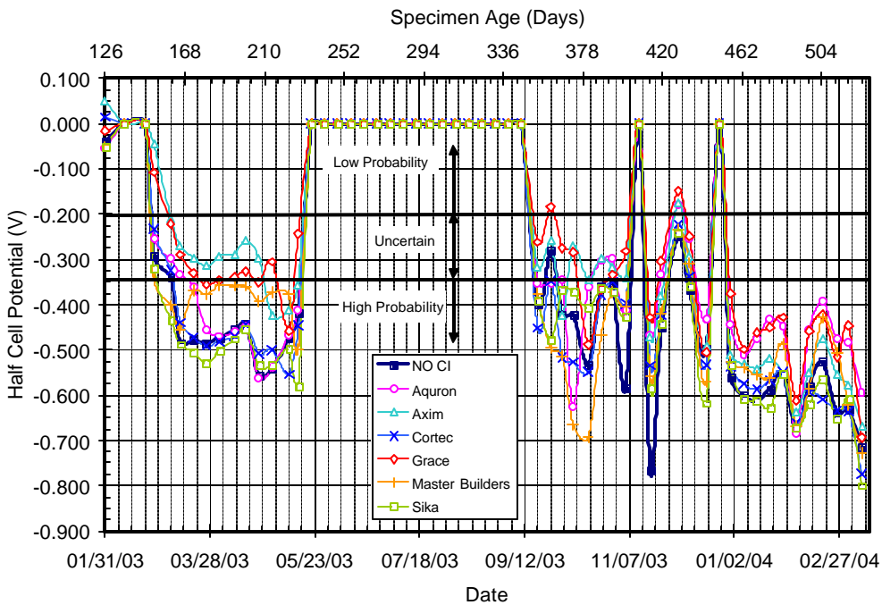
Figure C.48 – Half Cell Potential Readings for Chamber Shelf 4, 1.5% Chloride, Pre-Cracked
