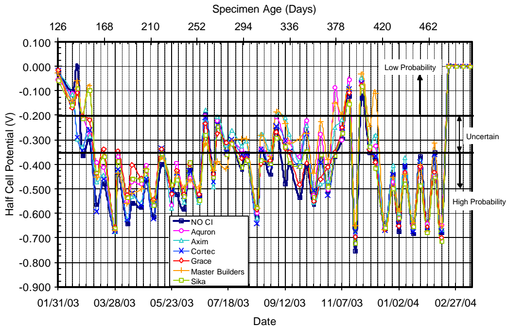
Figure C.18 – Half Cell Potential Readings for Bath 3, 1.5% Chloride, Post-Cracked
