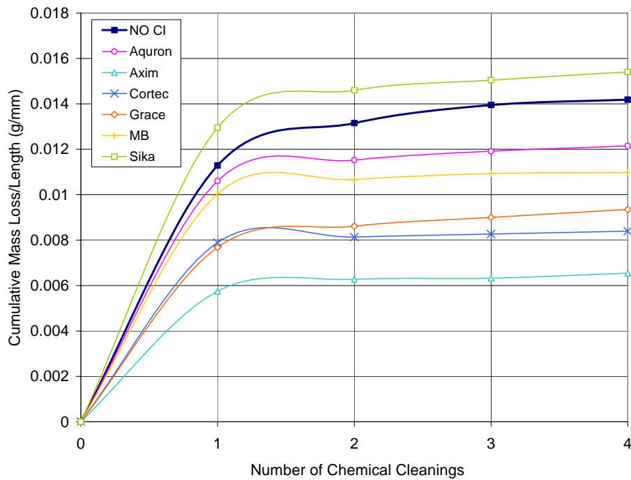
Figure F.43 – Cumulative Mass Loss/Length for Chamber Shelf 3 3.0% Chloride, Post-Cracked Specimens
