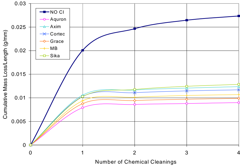
Figure F.23 – Cumulative Mass Loss/Length for Bath 4, 1.5% Chloride Post-Cracked Specimens
