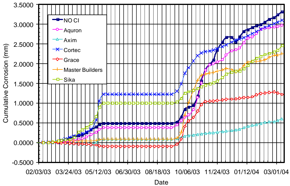
Figure B.48 – Cumulative Corrosion Over Time for Chamber Shelf 4, 1.5% Chloride, Pre-Cracked
