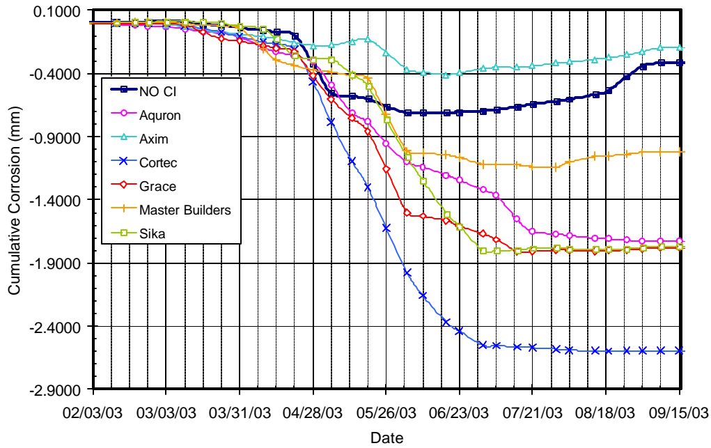
Figure B.3 – Cumulative Corrosion Over Time for Bath 1, 0.0% Chloride, Pre-Cracked
