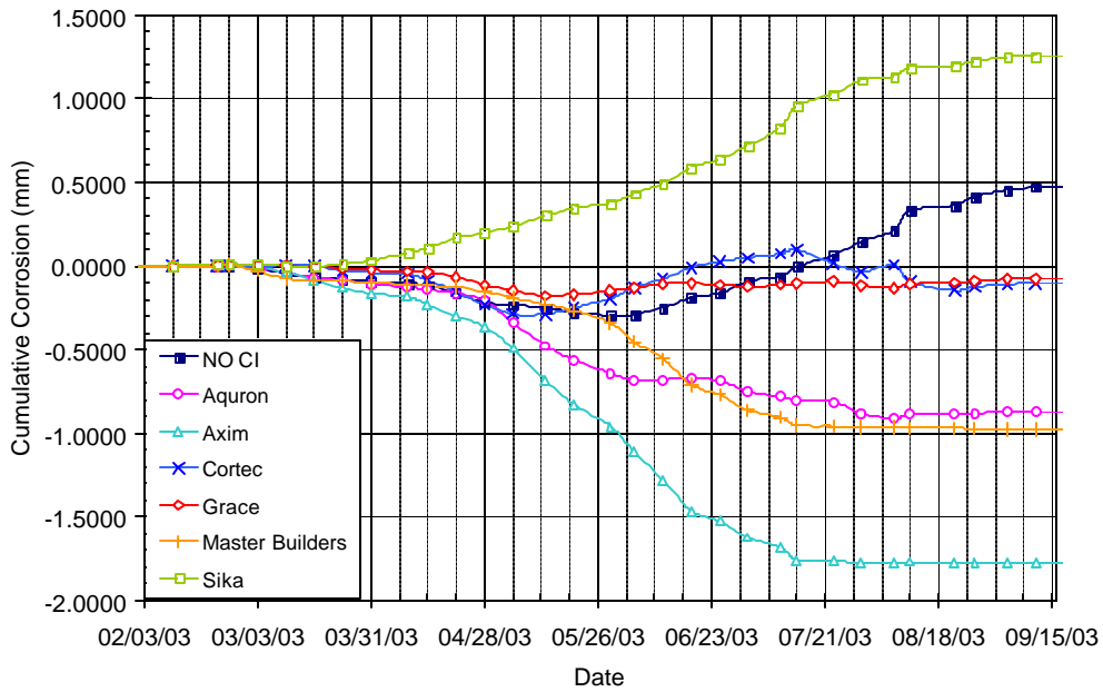
Figure B.23 – Cumulative Corrosion Over Time for Bath 4, 1.0% Chloride, Post-Cracked
