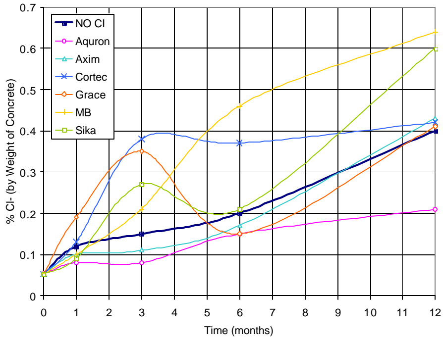
Figure D.3 – Chloride Content for Bath Specimens – 0.5% Chloride
