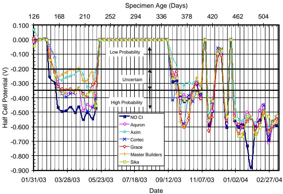
Figure C.46 – Half Cell Potential Readings for Chamber Shelf 4, 0.5% Chloride, Pre-Cracked
