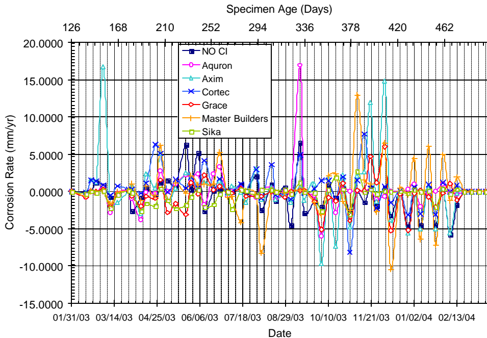
Figure A.18 – Corrosion Rate for Bath 3, 1.5% Chloride, Post-Cracked
