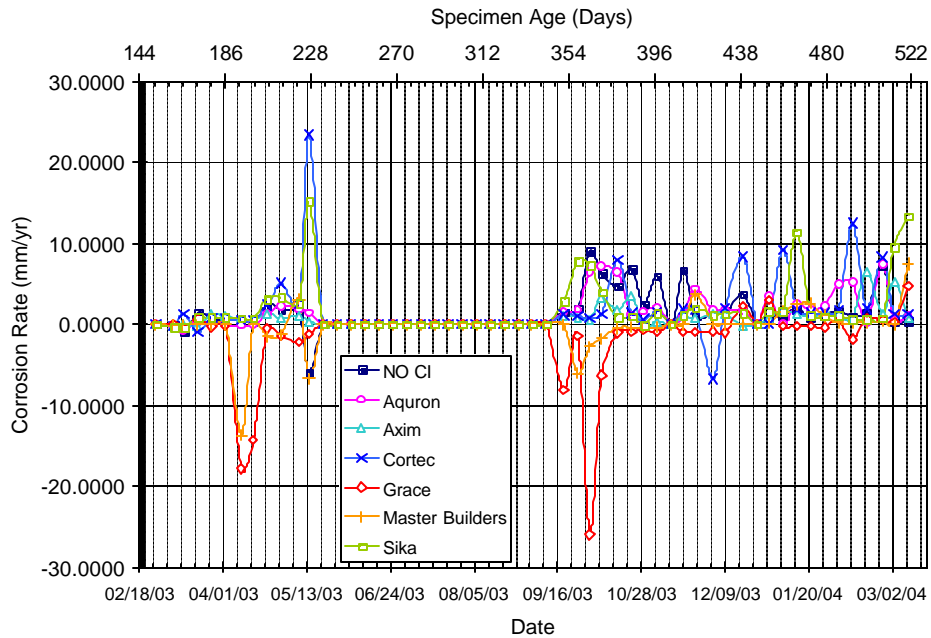
Figure A.39 – Corrosion Rate for Chamber Shelf 3, 0.0% Chloride, Post-Cracked
