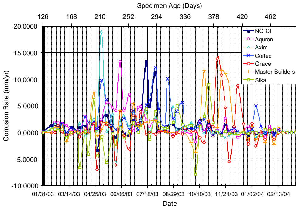
Figure A.20 – Corrosion Rate for Bath 3, 3.0% Chloride, Post-Cracked
