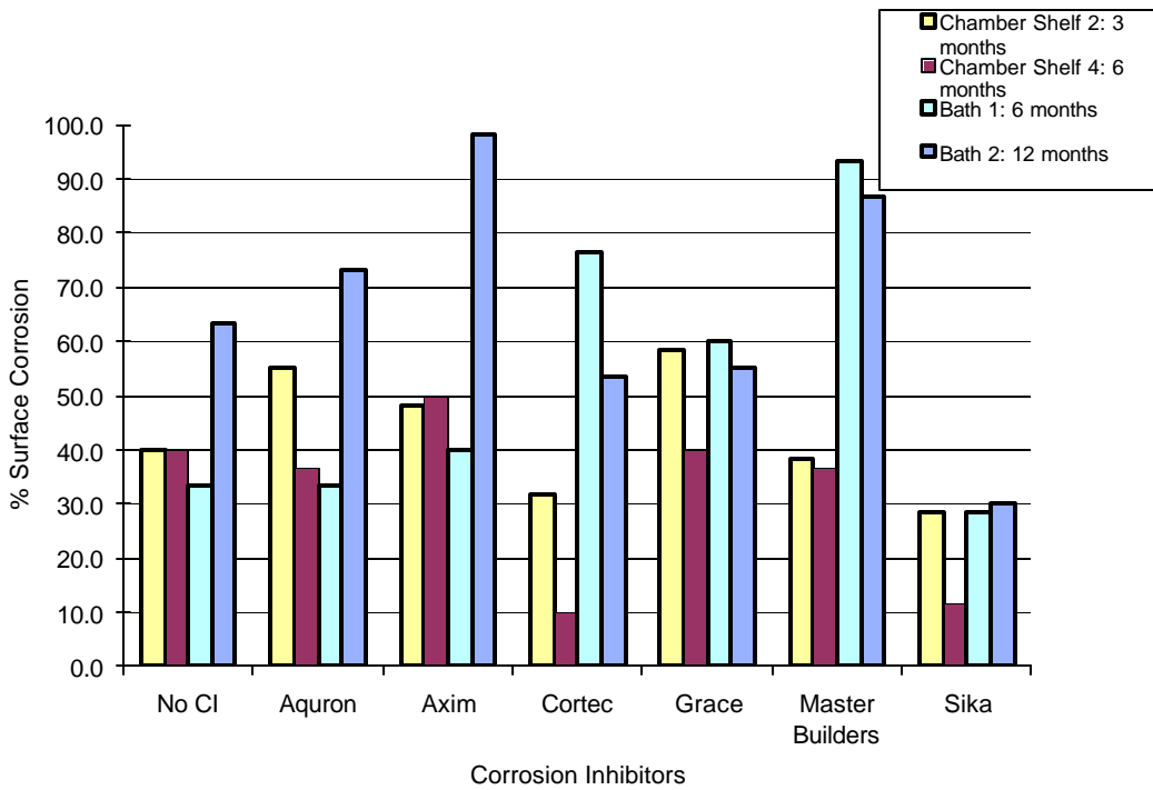
Figure E.39 Time Step of Surface Corrosion for 3.0% Chloride Pre-Cracked Specimens
