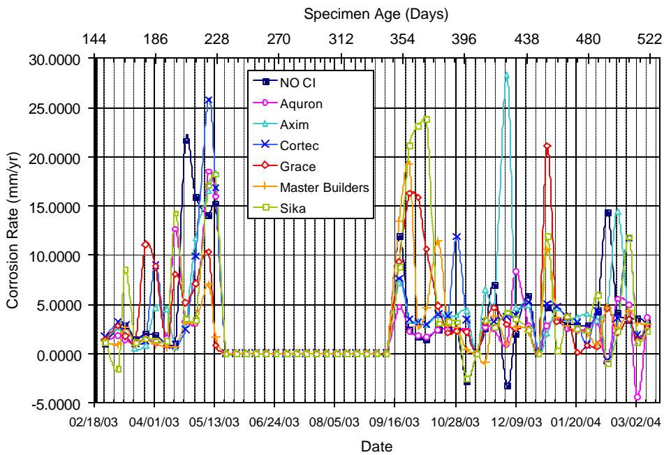
Figure A.44 – Corrosion Rate for Chamber Shelf 3, 3.0% Chloride, Post-Cracked
