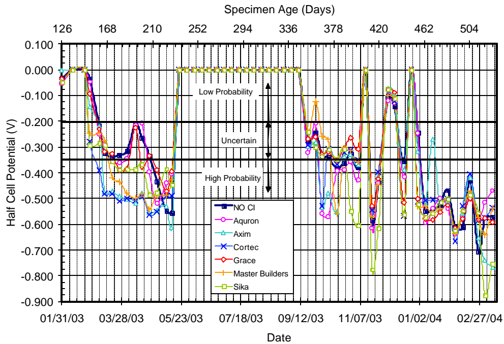
Figure C.41 – Half Cell Potential Readings for Chamber Shelf 3, 1.0% Chloride, Post-Cracked
