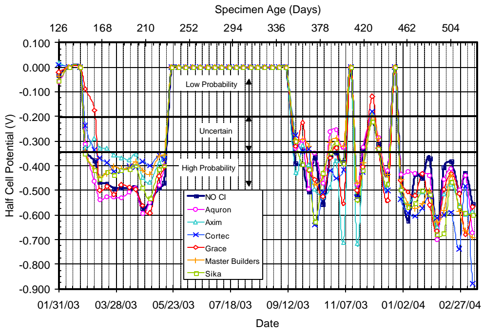
Figure C.42 – Half Cell Potential Readings for Chamber Shelf 3, 1.5% Chloride, Post-Cracked
