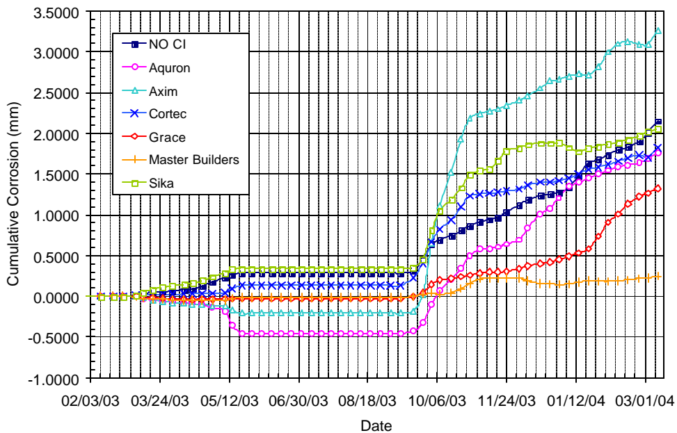
Figure B.40 – Cumulative Corrosion Over Time for Chamber Shelf 3, 0.5% Chloride, Post-Cracked
