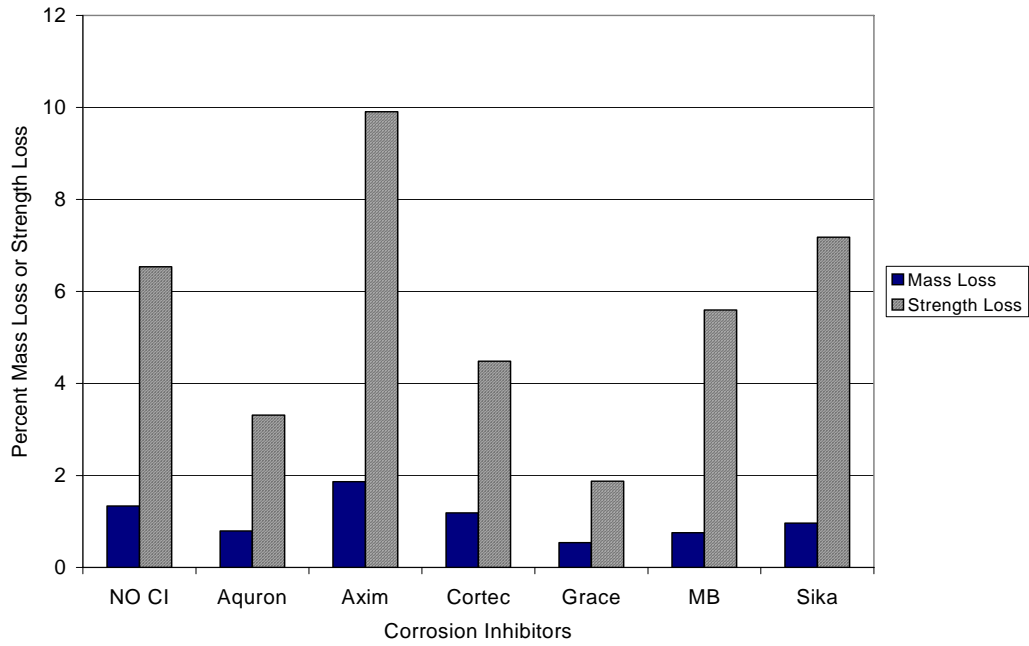
Figure G.50 – Mass Loss and Strength Loss for Chamber Shelf 1, 0.0% Chloride, Post-Cracked
