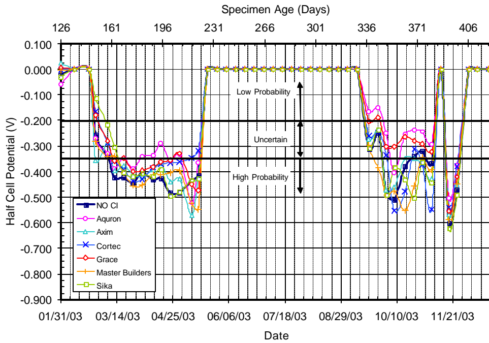
Figure C.35 – Half Cell Potential Readings for Chamber Shelf 2, 1.0% Chloride, Pre-Cracked
