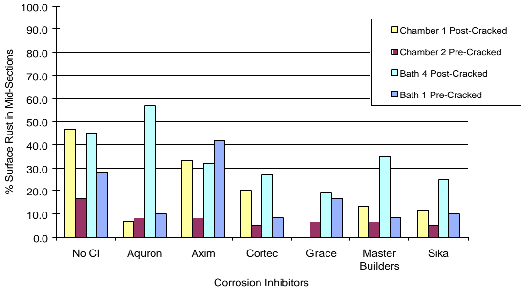
Figure E.1 Surface Corrosion at Mid Section for 0.0% Chloride (Set#1)
