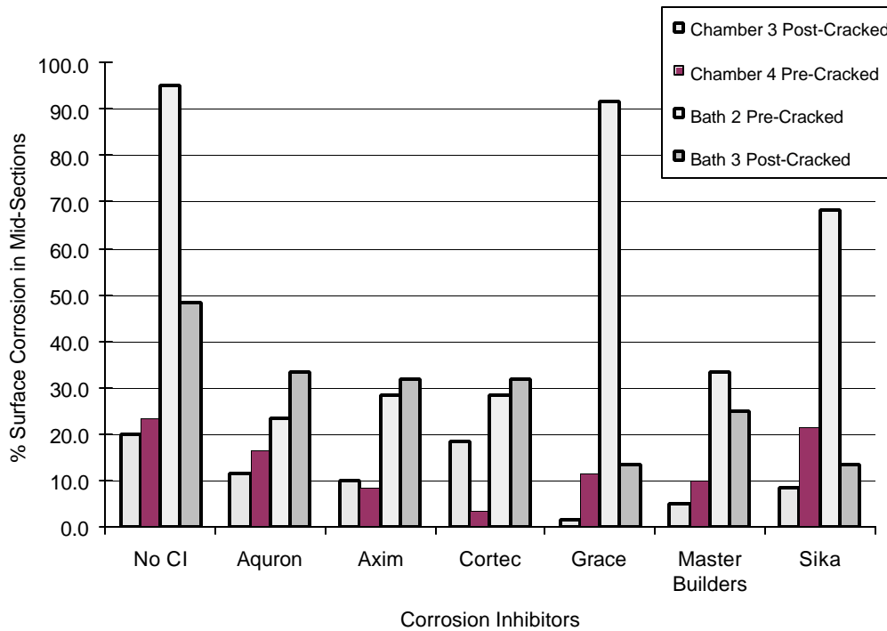
Figure 4.24 - % Surface Corrosion at Midsection for 0.0% Chloride (Set #2)
