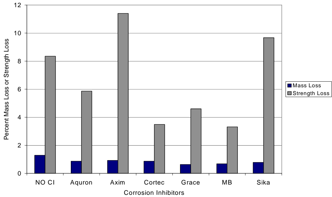
Figure G.74 – Mass Loss and Strength Loss for Chamber Shelf 3, 0.0% Chloride, Post-Cracked
