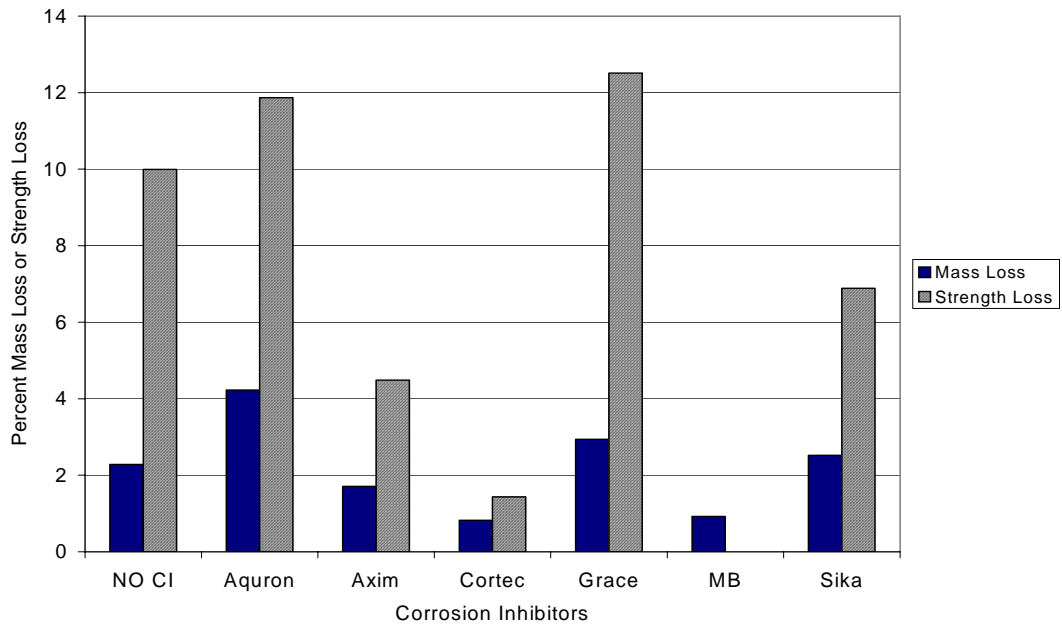
Figure G.80 – Mass Loss and Strength Loss for Chamber Shelf 3, 1.5% Chloride, Post-Cracked
