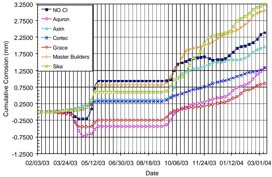
Figure B.41 – Cumulative Corrosion Over Time for Chamber Shelf 3, 1.0% Chloride, Post-Cracked
