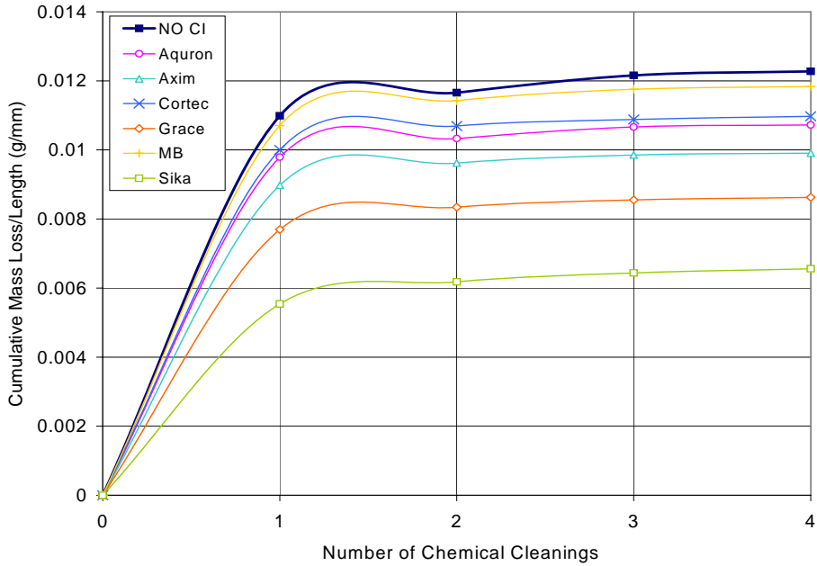
Figure F.13 – Cumulative Mass Loss/Length for Bath 2, 3.0% Chloride Pre-Cracked Specimens
