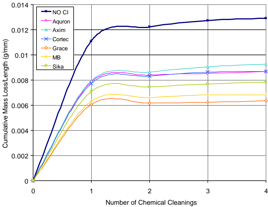
Figure 4.37 – Cumulative Mass Loss/Length for Chamber 0.0% Chloride, Shelf 3, Post-Cracked Specimens
