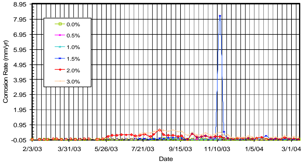
Figure A.1 – Corrosion Rate for Control Set #1
