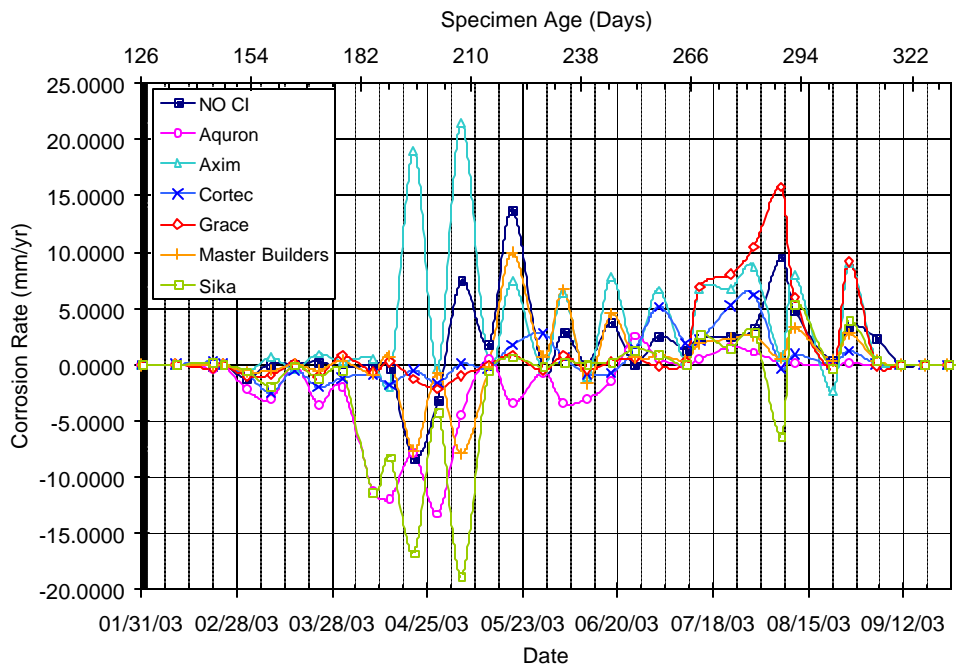
Figure A.21 – Corrosion Rate for Bath 4, 0.0% Chloride, Post-Cracked
