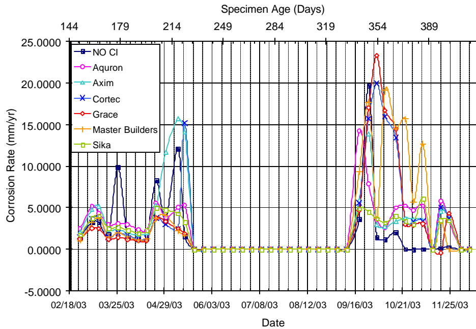
Figure A.32 – Corrosion Rate for Chamber Shelf 1, 3.0% Chloride, Post-Cracked
