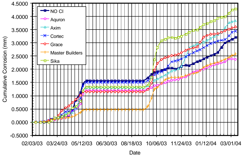
Figure B.44 – Cumulative Corrosion Over Time for Chamber Shelf 3, 3.0% Chloride, Post-Cracked
