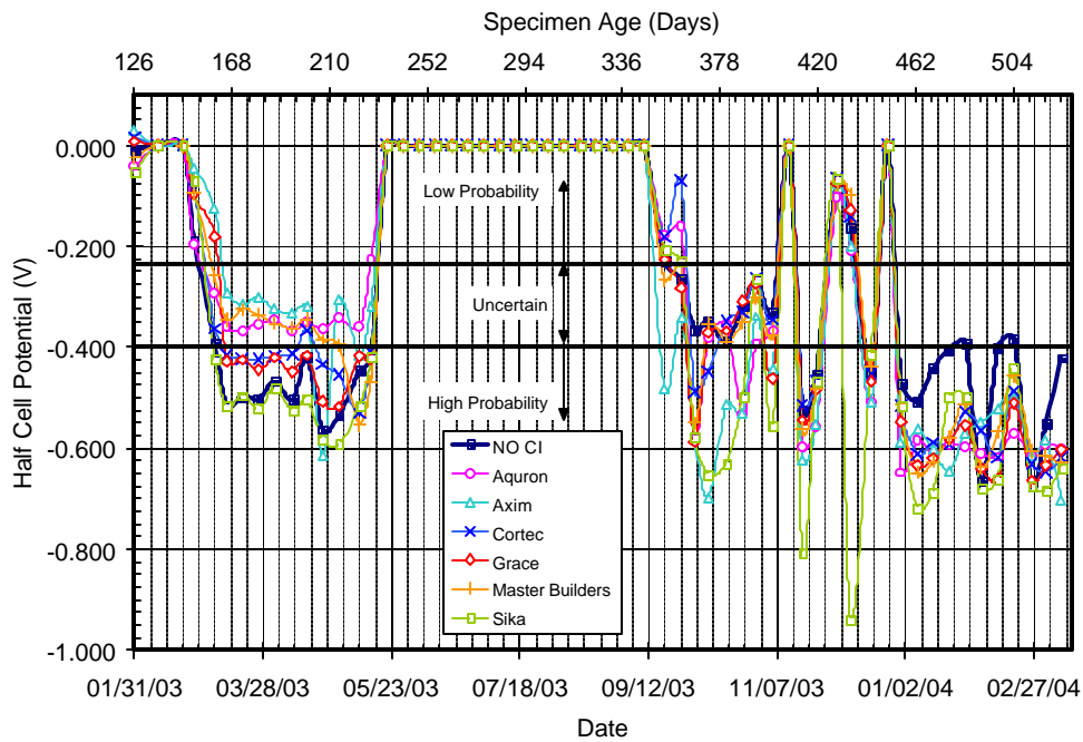
Figure C.40 – Half Cell Potential Readings for Chamber Shelf 3, 0.5% Chloride, Post-Cracked
