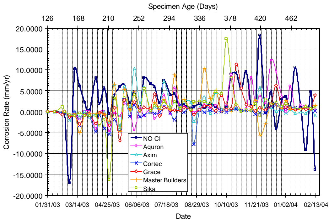
Figure 4.2 - Corrosion Rate for Bath 2, 0.0% Chloride, Pre-Cracked
