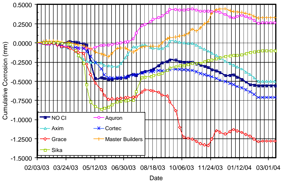
Figure B.16 – Cumulative Corrosion Over Time for Bath 3, 0.5% Chloride, Post-Cracked
