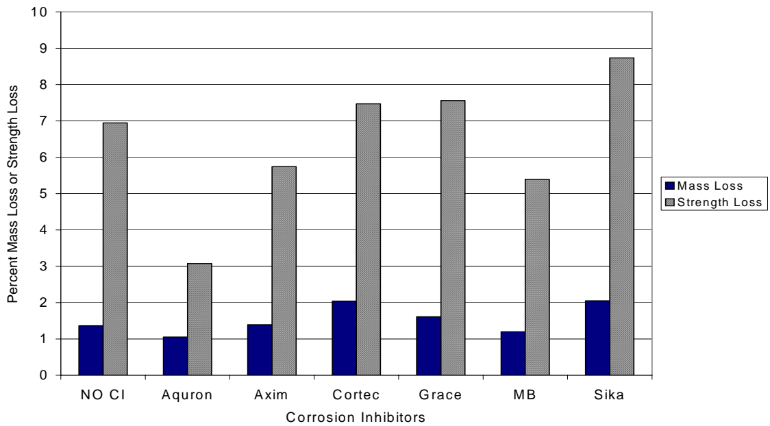
Figure G.30 – Mass Loss and Strength Loss for Bath 3, 1.0% Chloride, Post-Cracked
