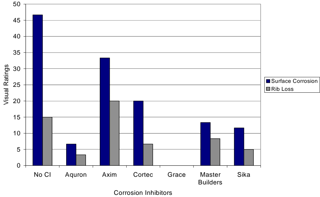
Figure G.49 – Visual Ratings for Chamber Shelf 1, 0.0% Chloride, Post-Cracked
