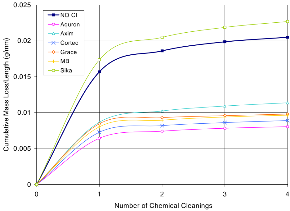
Figure F.29 – Cumulative Mass Loss/Length for Chamber Shelf 1 1.5% Chloride, Post-Cracked Specimens
