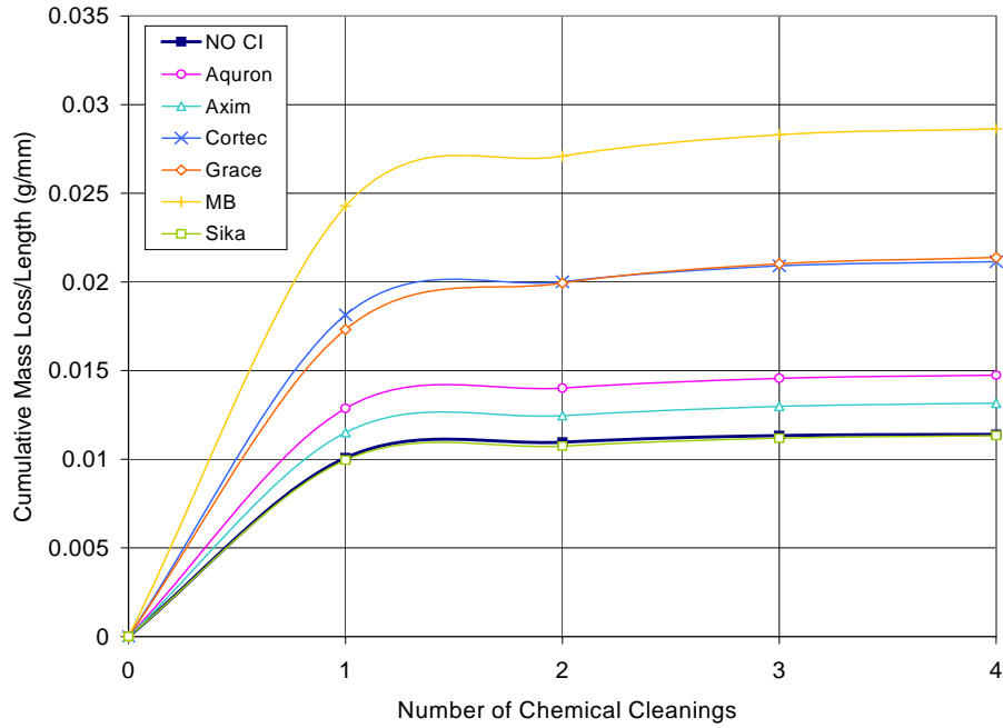
Figure F.7 – Cumulative Mass Loss/Length for Bath 1, 3.0% Chloride Pre-Cracked Specimens
