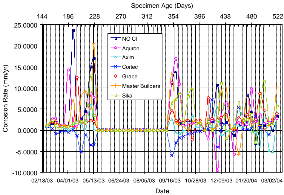
Figure A.43 – Corrosion Rate for Chamber Shelf 3, 2.0% Chloride, Post-Cracked
