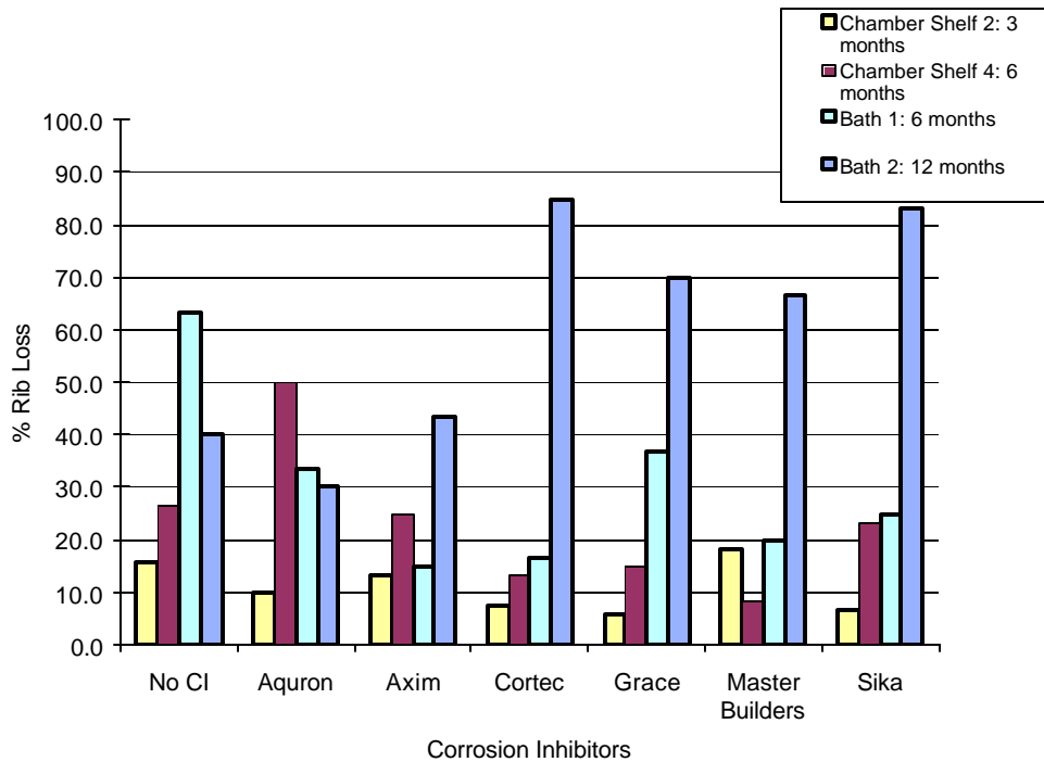
Figure E.38 Time Step of Rib Loss for 2.0% Chloride Pre-Cracked Specimens
