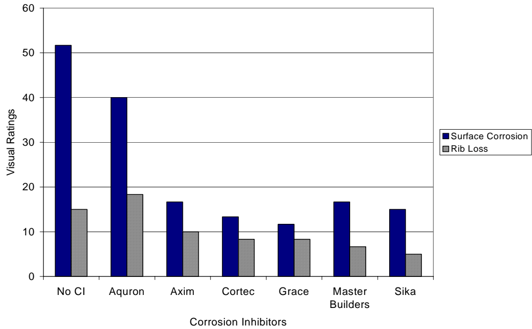
Figure G.87 – Visual Ratings for Chamber Shelf 4, 0.5% Chloride, Pre-Cracked
