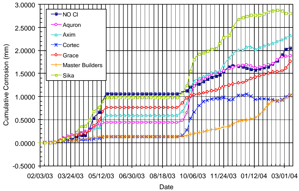
Figure B.49 – Cumulative Corrosion Over Time for Chamber Shelf 4, 2.0% Chloride, Pre-Cracked
