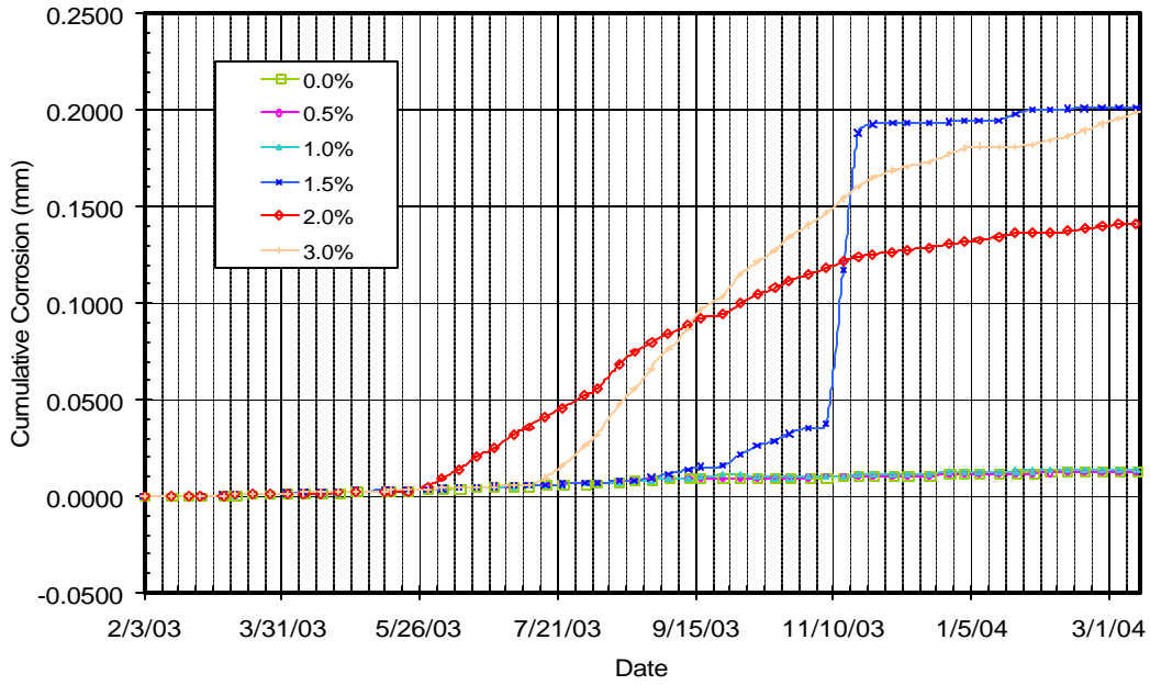
Figure B.1 – Cumulative Corrosion Over Time for Control Set #1
