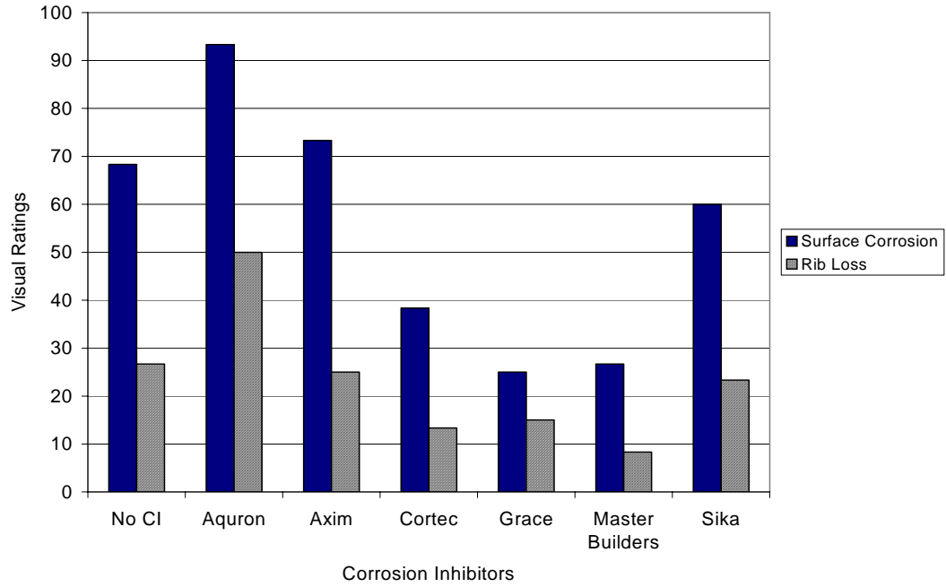
Figure G.93 – Visual Ratings for Chamber Shelf 4, 2.0% Chloride, Pre-Cracked
