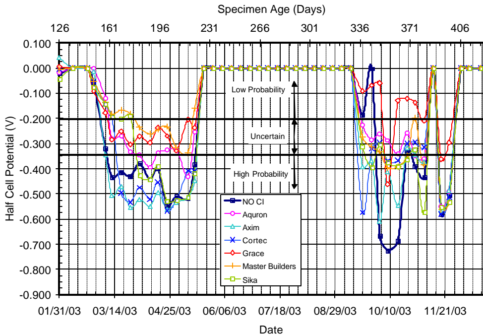
Figure C.27 – Half Cell Potential Readings for Chamber Shelf 1, 0.0% Chloride, Post-Cracked
