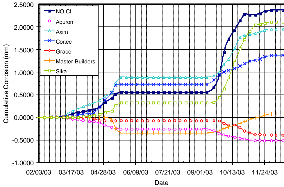
Figure B.27 – Cumulative Corrosion Over Time for Chamber Shelf 1, 0.0% Chloride, Post-Cracked
