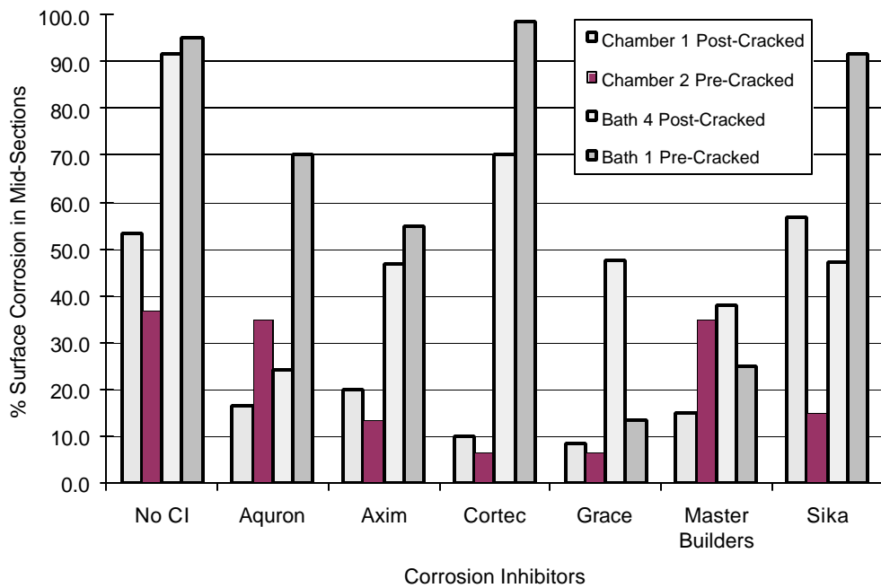
Figure 4.22 - % Surface Corrosion at Midsection for 1.5% Chloride (Set #1)
