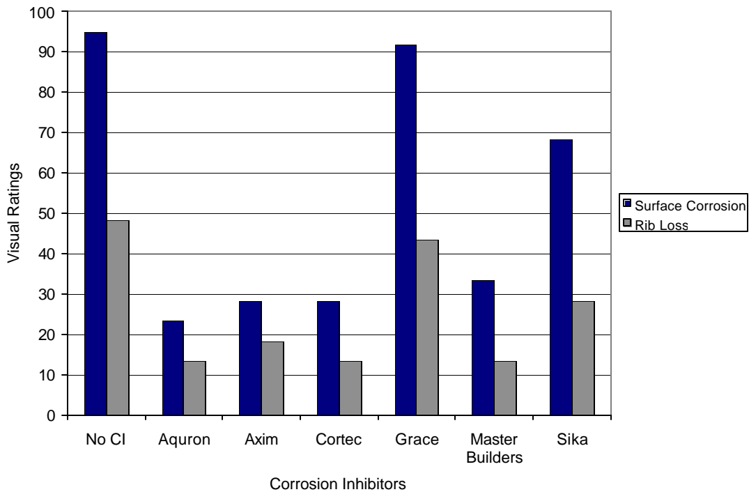
Figure 4.41 – Visual Ratings for Bath 2, 0.0% Chloride, Pre-Cracked Specimens
