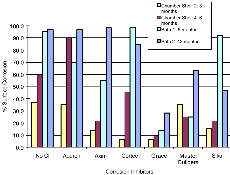
Figure E.35 Time Step of Surface Corrosion for 1.5% Chloride Pre-Cracked Specimens
