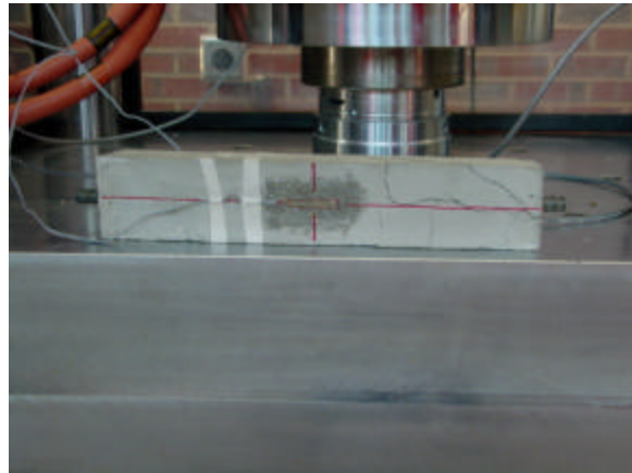
Figure 3.10 – Failed Specimen
