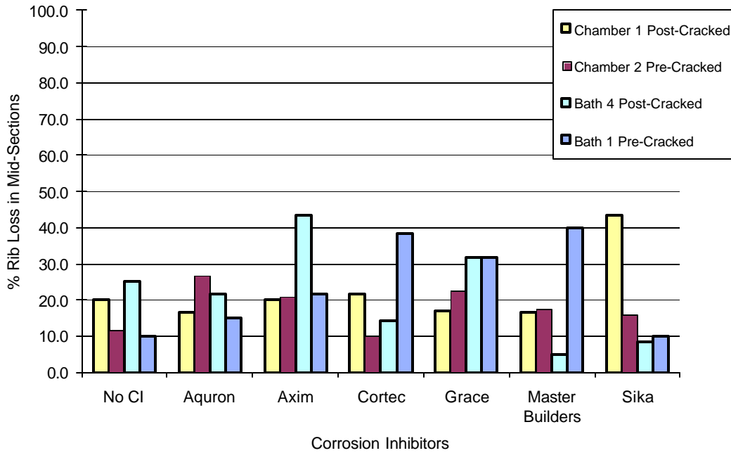
Figure E.12 Rib Loss at Mid Section for 3.0% Chloride (Set #1)
