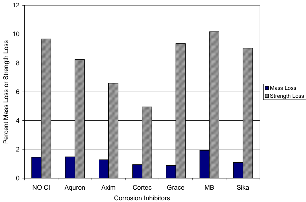
Figure G.70 – Mass Loss and Strength Loss for Chamber Shelf 2, 2.0% Chloride, Pre-Cracked
