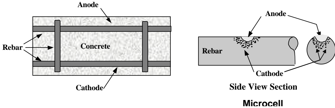
Figure 2.2 - Mechanism of Corrosion in Macrocell and Microcell
