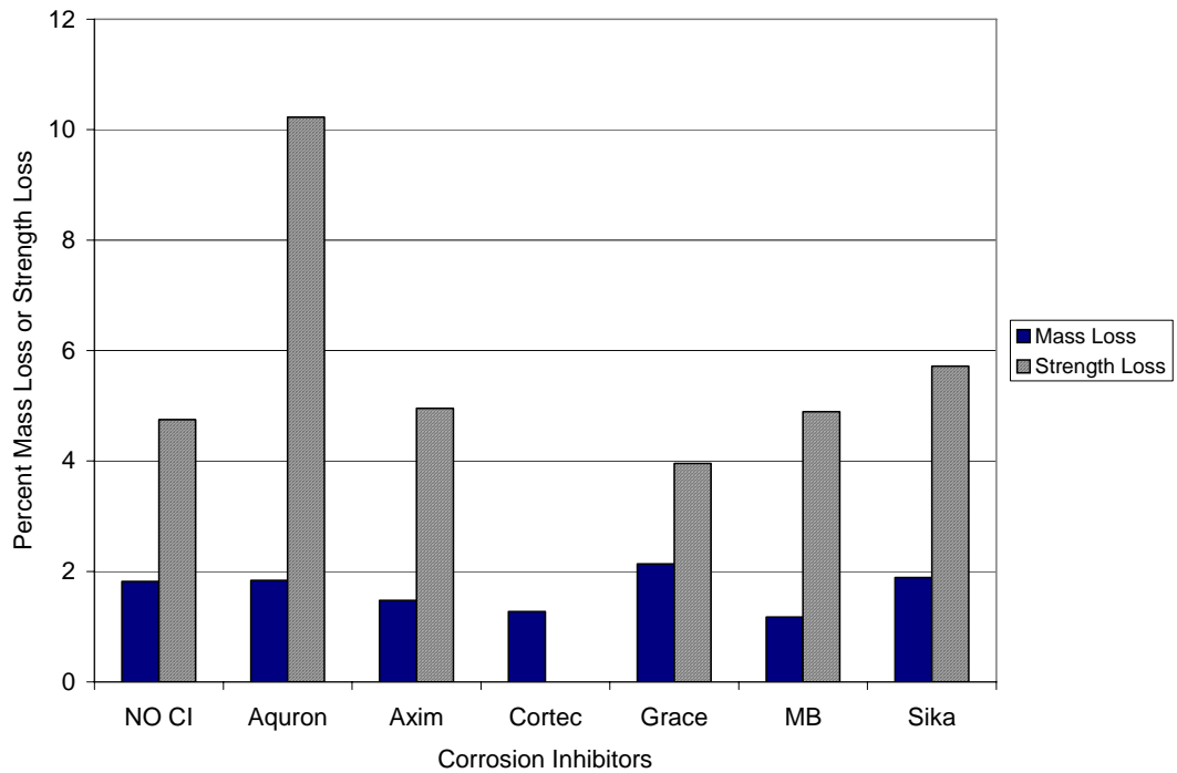
Figure G.82 – Mass Loss and Strength Loss for Chamber Shelf 3, 2.0% Chloride, Post-Cracked
