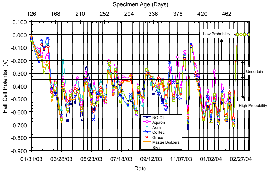
Figure C.17 – Half Cell Potential Readings for Bath 3, 1.5% Chloride, Post-Cracked
