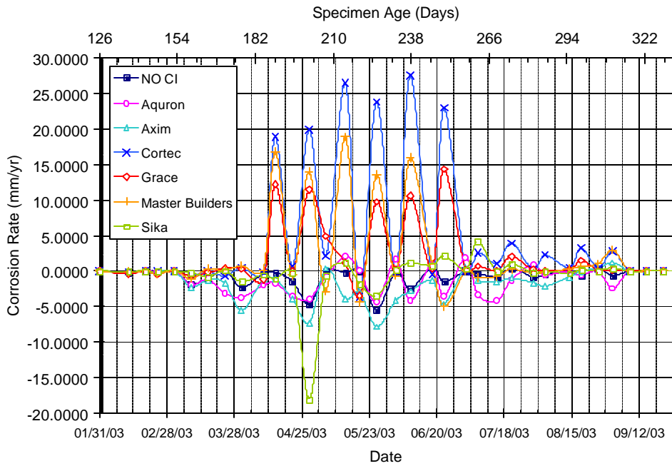
Figure A.4 – Corrosion Rate for Bath 1, 0.5% Chloride, Pre-Cracked
