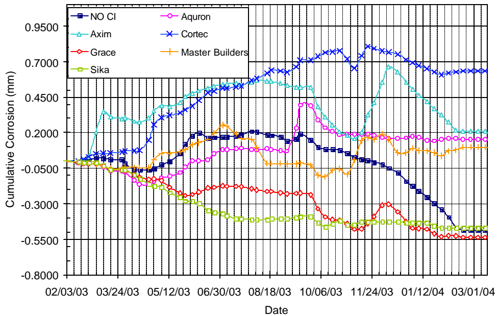
Figure B.18 – Cumulative Corrosion Over Time for Bath 3, 1.5% Chloride, Post-Cracked
