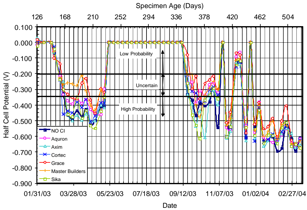
Figure C.39 – Half Cell Potential Readings for Chamber Shelf 3, 0.0% Chloride, Post-Cracked
