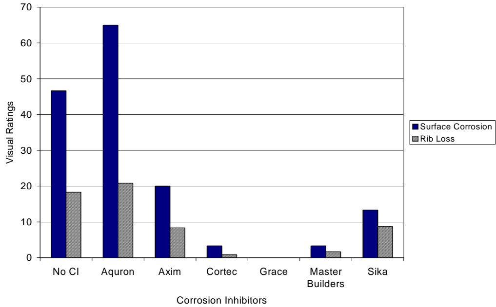
Figure G.51 – Visual Ratings for Chamber Shelf 1, 0.5% Chloride, Post-Cracked
