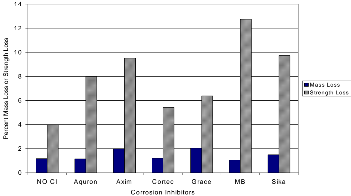
Figure G.48 – Mass Loss and Strength Loss for Bath 4, 3.0% Chloride, Post-Cracked
