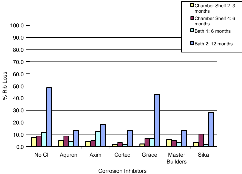
Figure E.30 Time Step of Rib Loss for 0.0% Chloride Pre-Cracked Specimens
