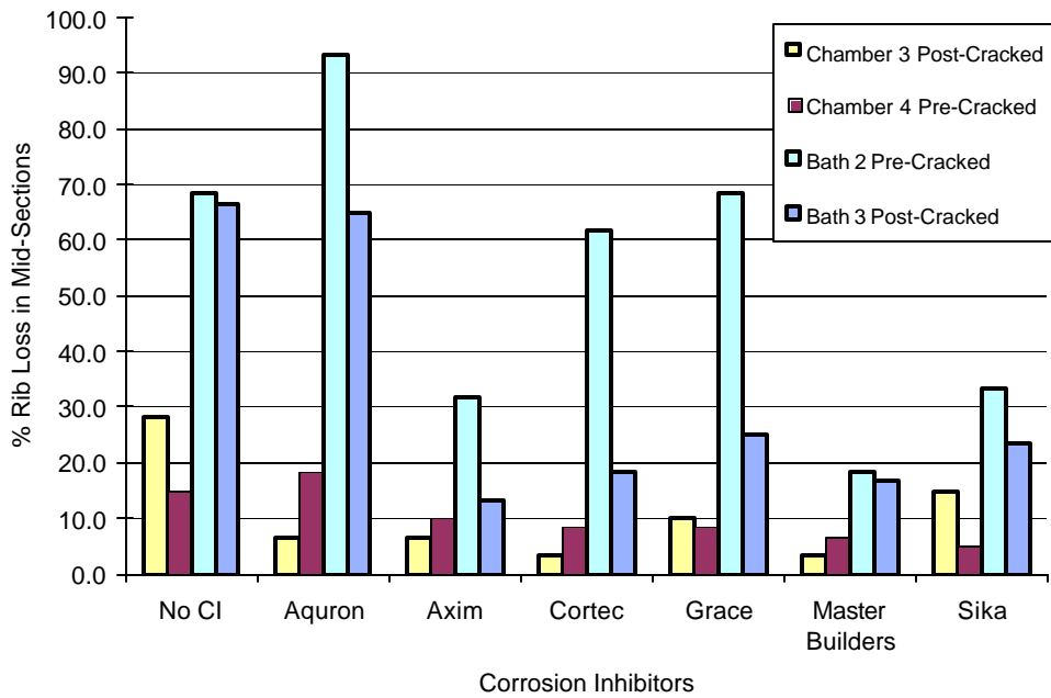
Figure E.18 Rib Loss at Mid Section for 0.5% Chloride (Set #2)
