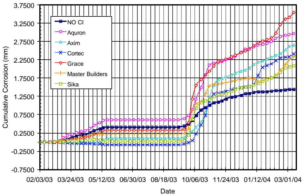
Figure B.42 – Cumulative Corrosion Over Time for Chamber Shelf 3, 1.5% Chloride, Post-Cracked
