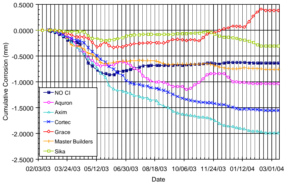
Figure B.10 – Cumulative Corrosion Over Time for Bath 2, 0.5% Chloride, Pre-Cracked
