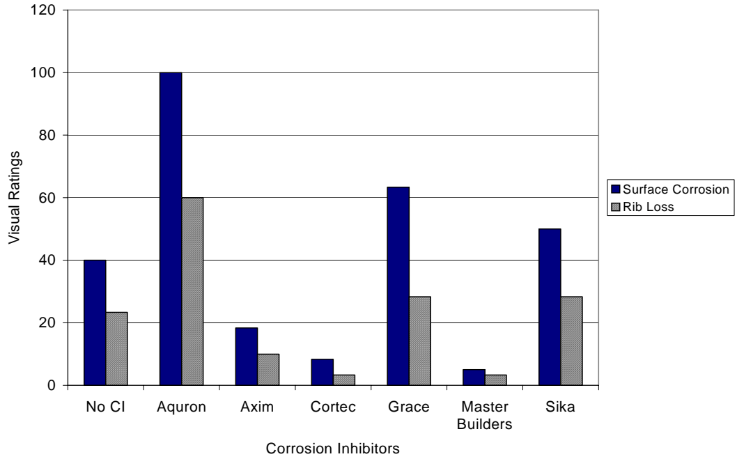
Figure G.79 – Visual Ratings for Chamber Shelf 3, 1.5% Chloride, Post-Cracked
