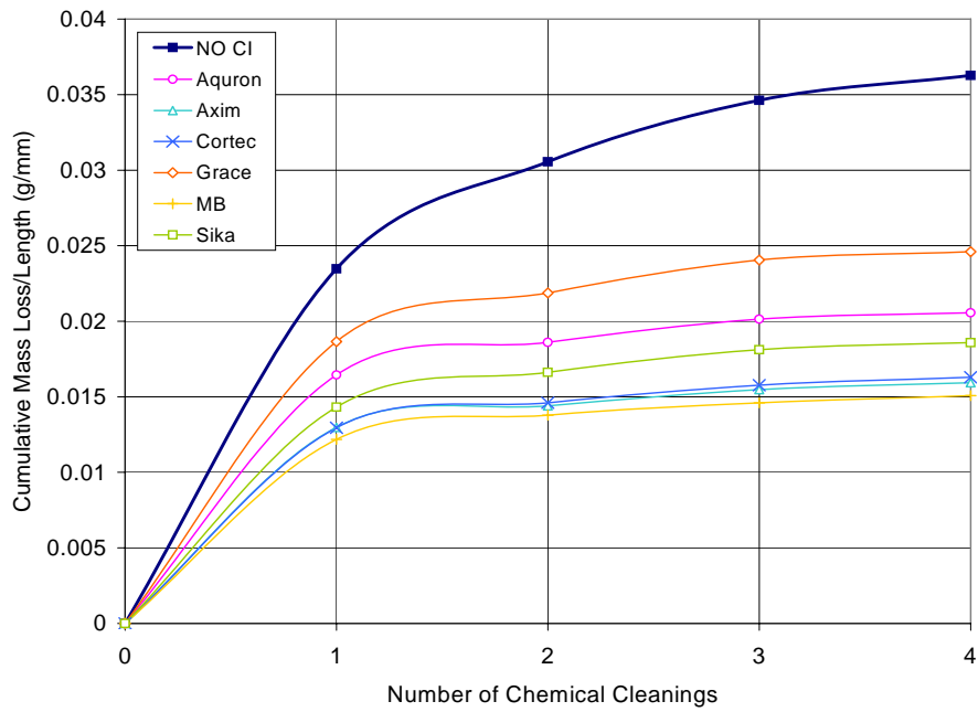
Figure F.5 – Cumulative Mass Loss/Length for Bath 1, 1.5% Chloride Pre-Cracked Specimens
