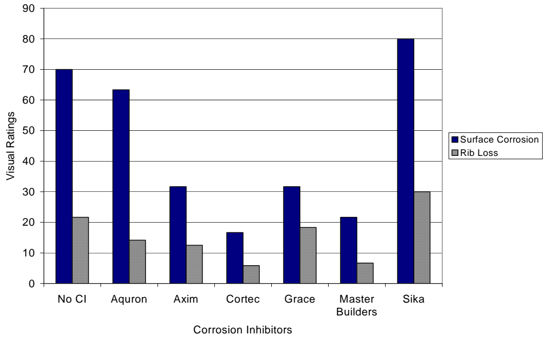
Figure G.57 – Visual Ratings for Chamber Shelf 1, 2.0% Chloride, Post-Cracked
