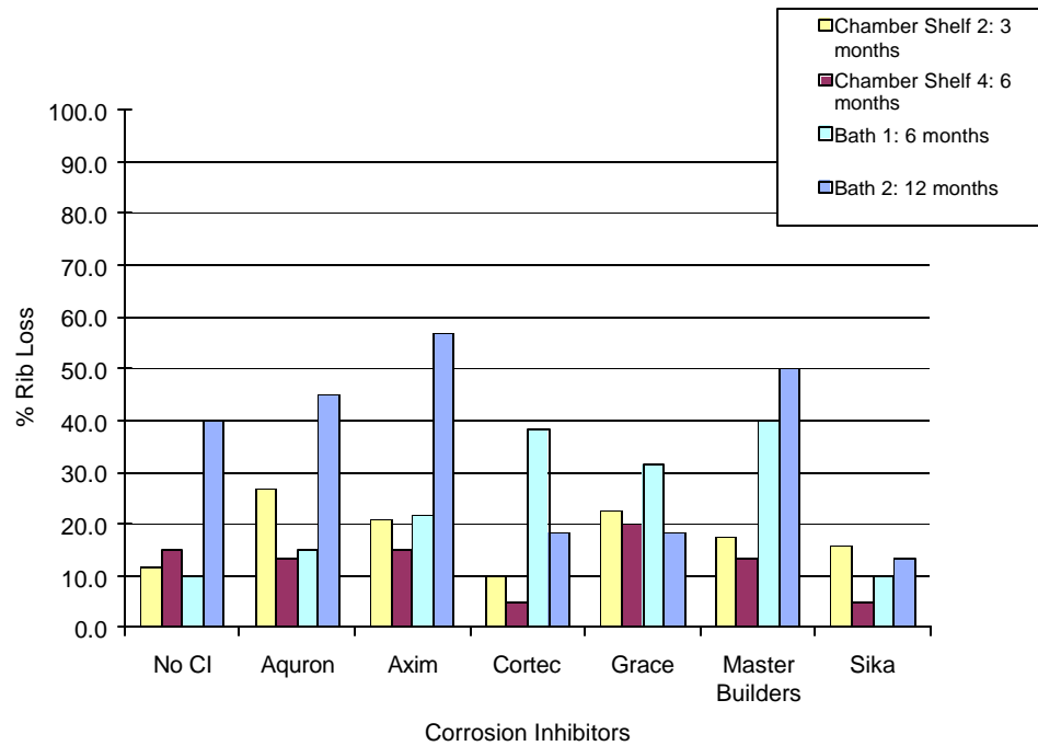
Figure E.40 Time Step of Rib Loss for 3.0% Chloride Pre-Cracked Specimens
