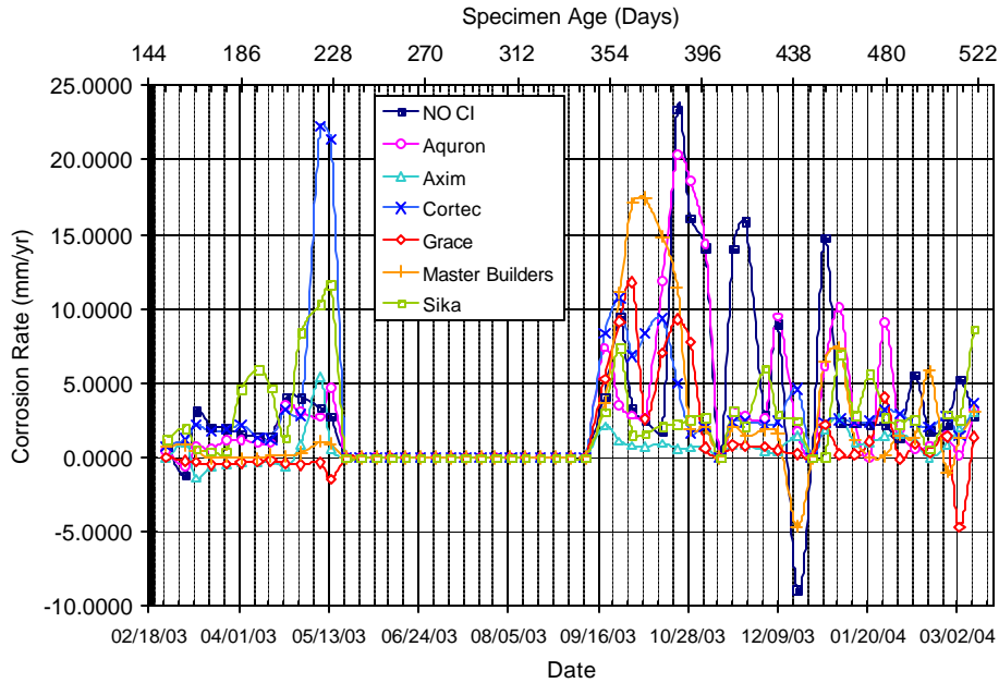
Figure A.48 – Corrosion Rate for Chamber Shelf 4, 1.5% Chloride, Pre-Cracked
