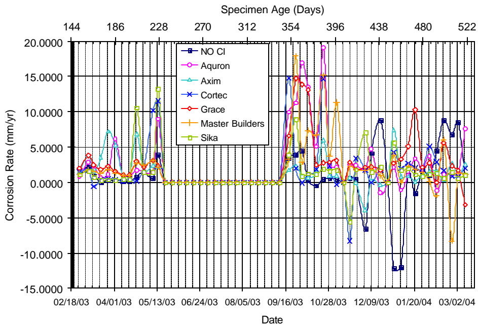
Figure A.50 – Corrosion Rate for Chamber Shelf 4, 3.0% Chloride, Pre-Cracked
