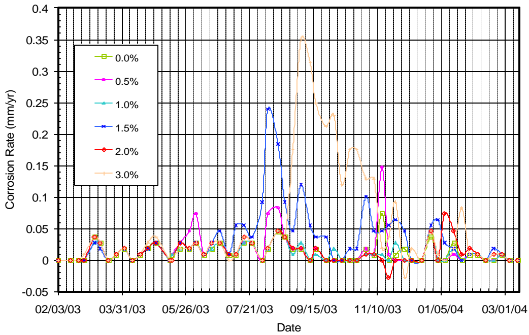
Figure A.2 – Corrosion Rate for Control Set #2
