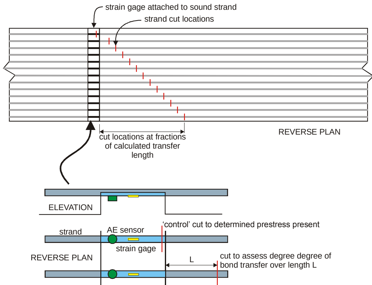
Figure 7.2 Schematic representation of proposed test program.
