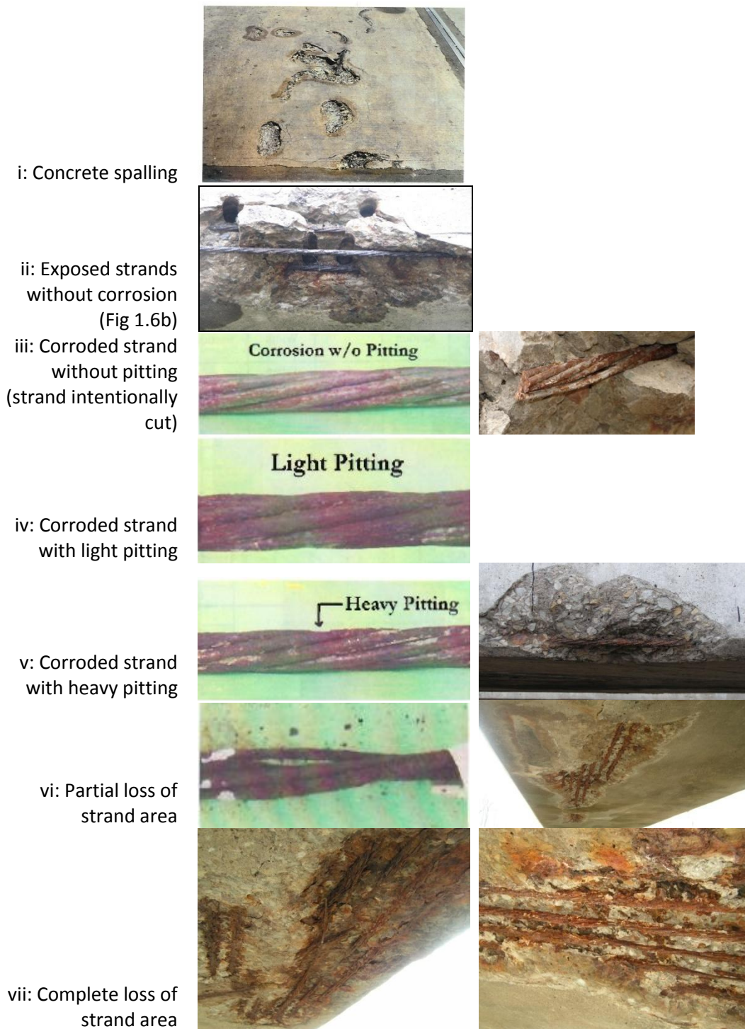
Figure 1.11 Continuum of corrosion damage (Naito et al 2006; Harries 2006)
