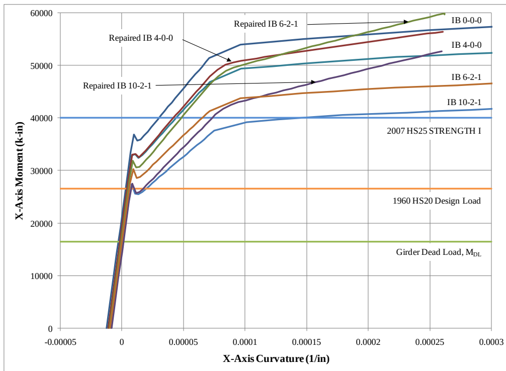
Figure 5.14 NSM repair moment-curvature plot.
