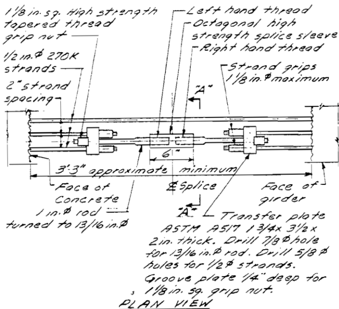
Figure 3.4 Strand splicing methods. (Shananfelt and Horn 1980)
