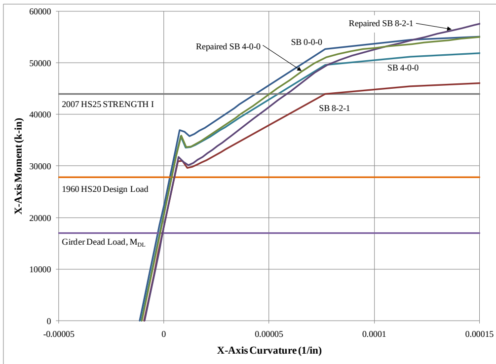
Figure 5.8 Preform CFRP strip repaired SB moment-curvature plot.
