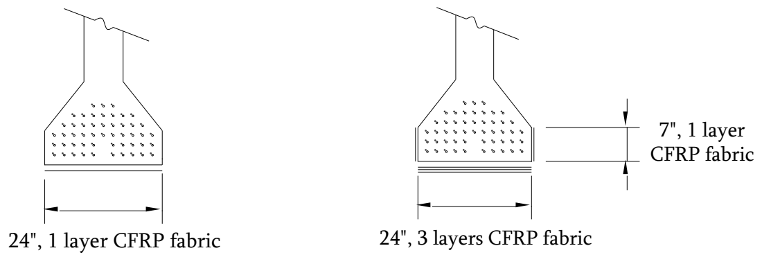
Figure 5.11 CFRP fabric repairs.
