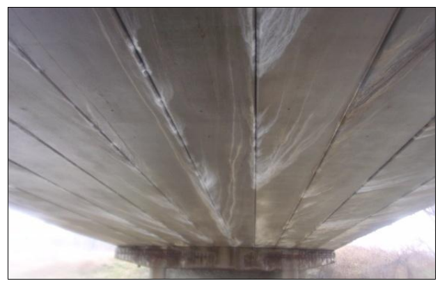
(b) water leaking between adjacent box girders (PennDOT).
