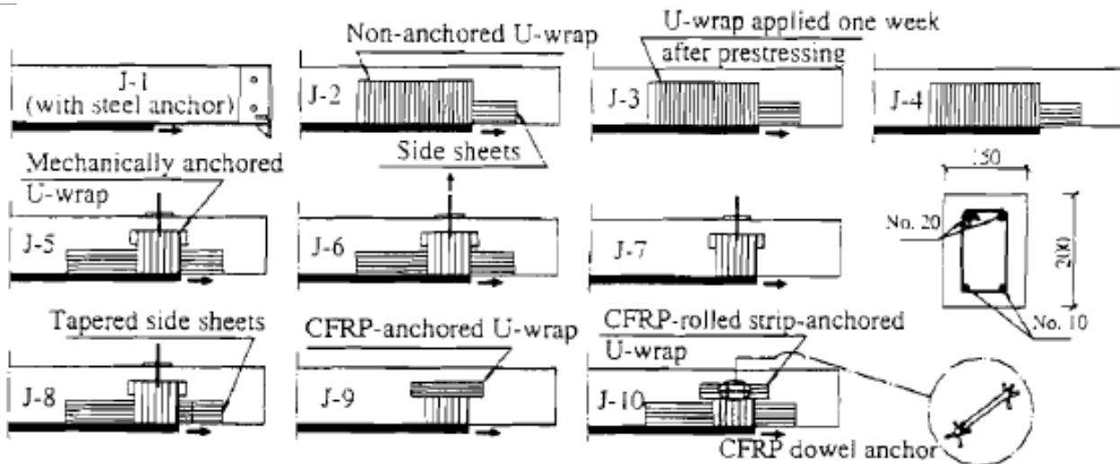
Figure 3.6 Non-metallic anchoring systems (Kim et al. 2008a).
