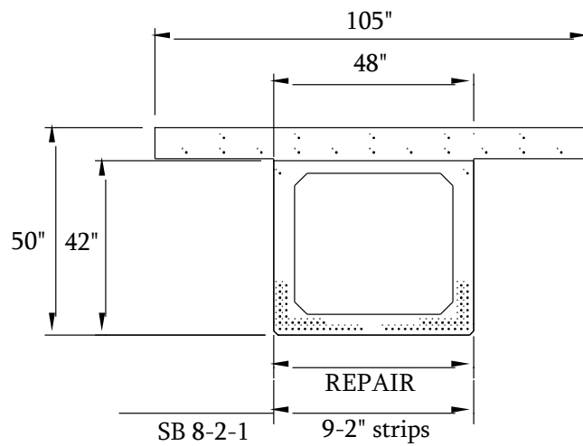
Figure 5.16 Prestressed CFRP repaired SB.
