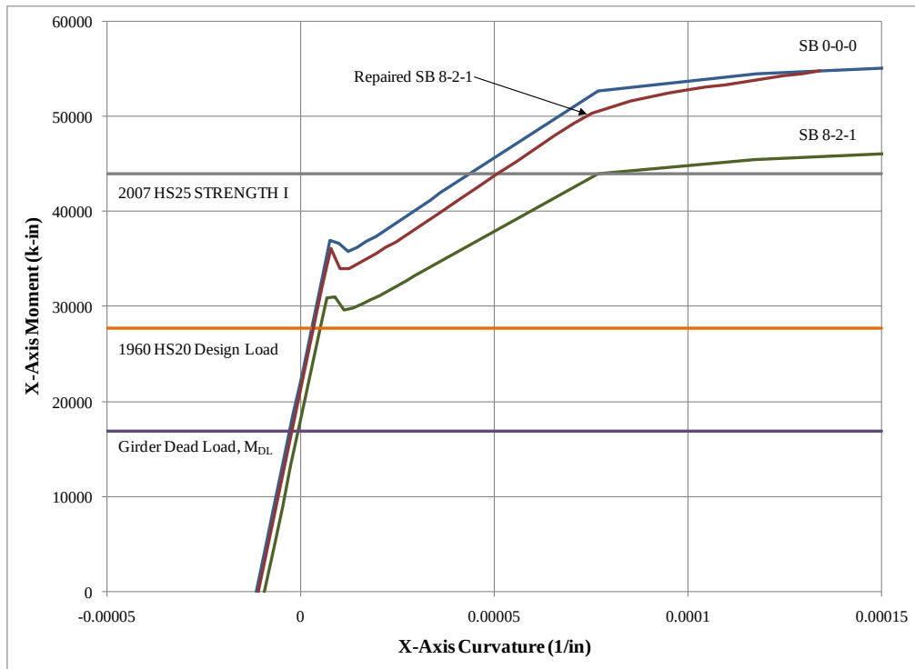
Figure 5.19 Prestressed CFRP repaired SB moment-curvature plot.
