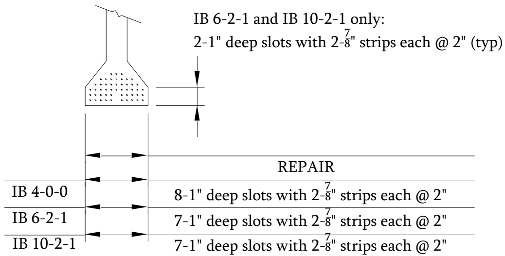
Figure 5.13 NSM repairs.
