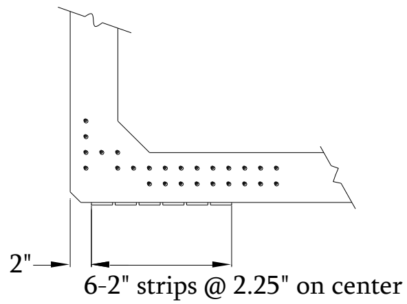
Figure 5.9 Suggested strip location for AB 4-0-0.
