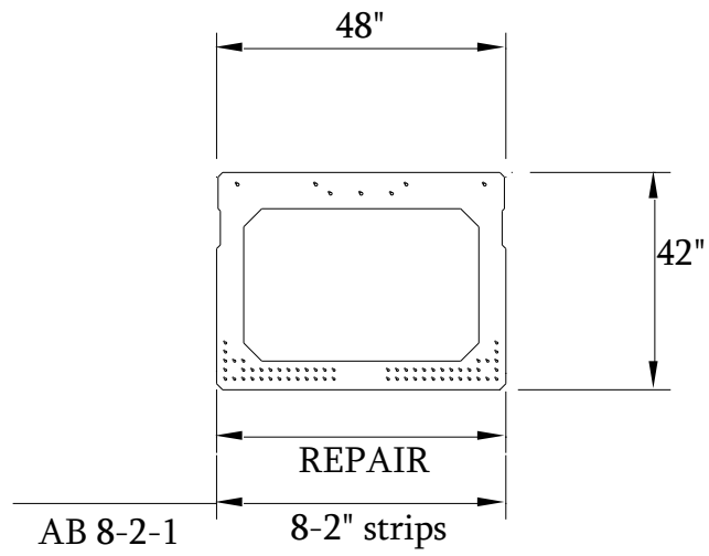
Figure 5.15 Prestressed CFRP repaired AB.
