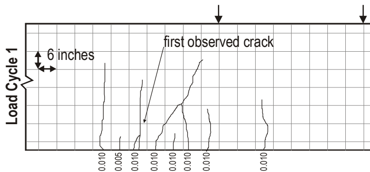
Figure 1.13 Representative flexural distress (Lake View Drive INTERIOR test girder; Harries 2006).
