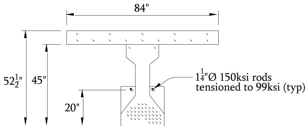
Figure 5.28 External post-tensioned steel repaired IB 6-2-1 drawing.
