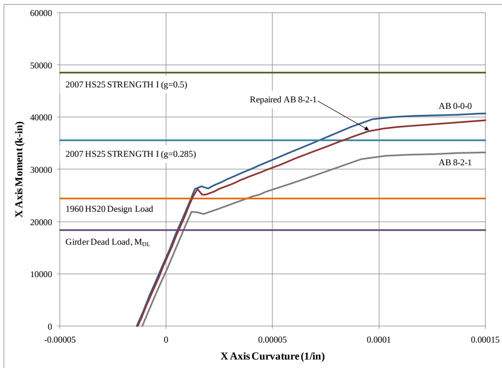
Figure 5.24 Post-tensioned CFRP repaired AB moment-curvature plot.
