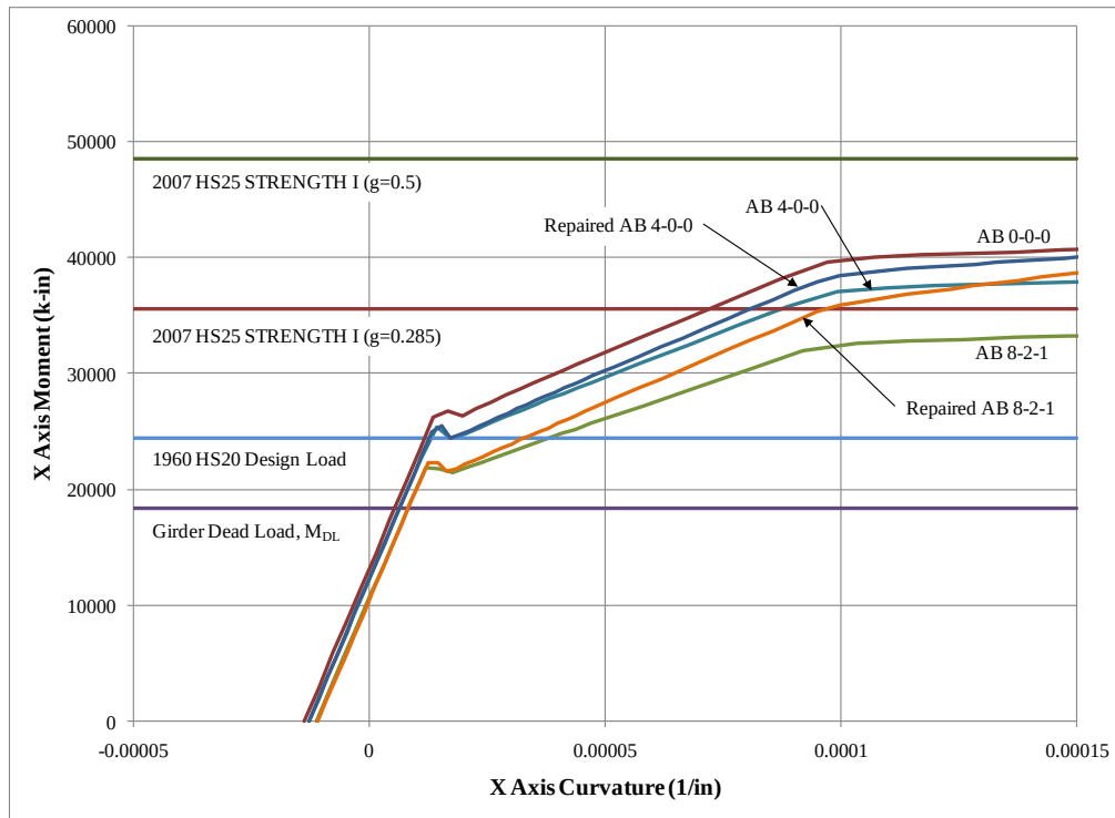
Figure 5.7 Preform CFRP strip repaired AB moment-curvature plot.
