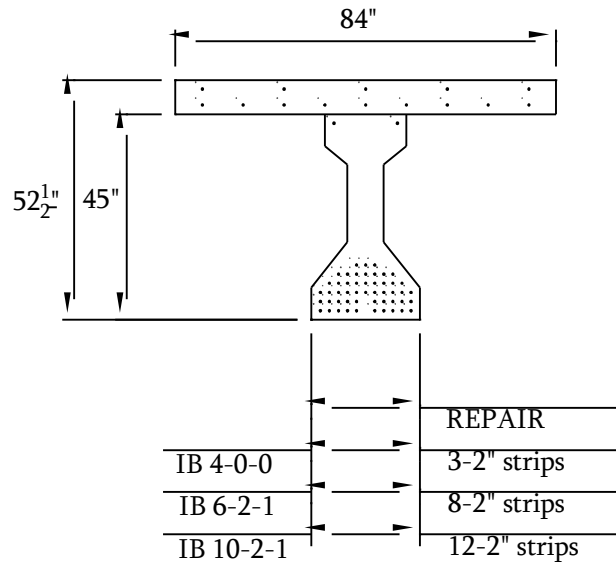
Figure 5.23 Post-tensioned CFRP repaired IB.
