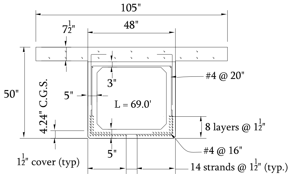
Figure 5.2 Prototype SB girder cross section.
