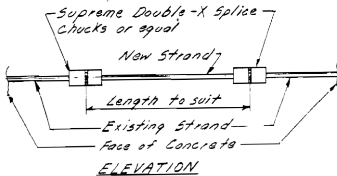
(a) Splice 6: Splice chucks used to splice strand. Prestressing reintroduced by heating strand during installation.
