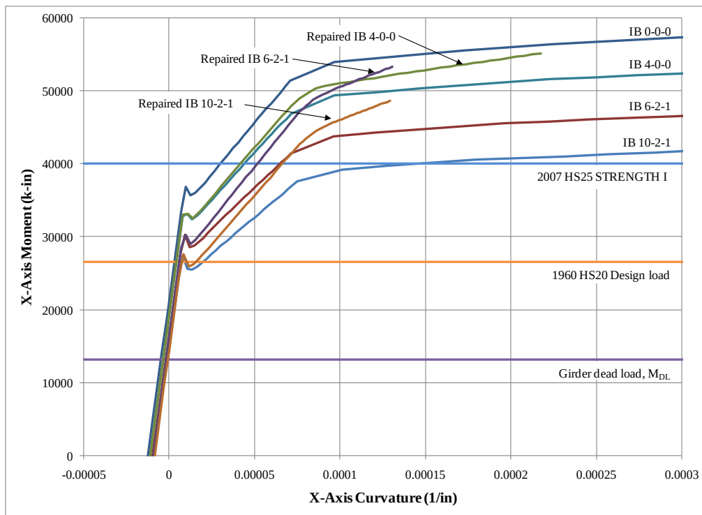
Figure 5.12 CFRP fabric repair moment-curvature plot.
