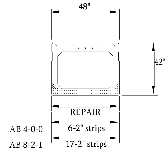
(a) AB CFRP strip repair.
