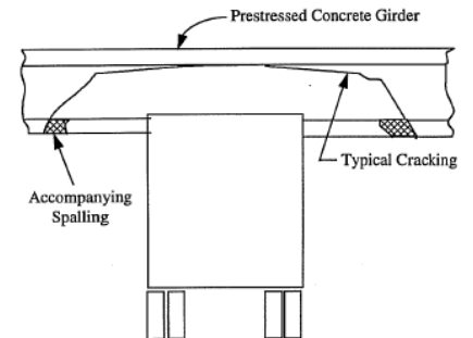
(c) typical impact damage due to side impact (Feldman et al. 1996).
