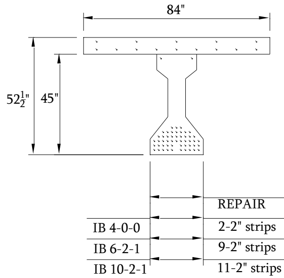
Figure 5.17 Prestressed CFRP repaired IB.
