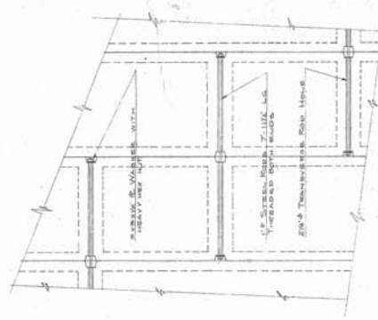
DETAIL SHOWING TRANSVERSE ROD CONNECTIONS AT DIAPHRAGM 16'-10"
