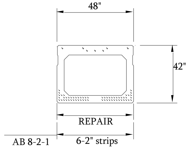
Figure 5.21 Post-tensioned CFRP repaired AB.
