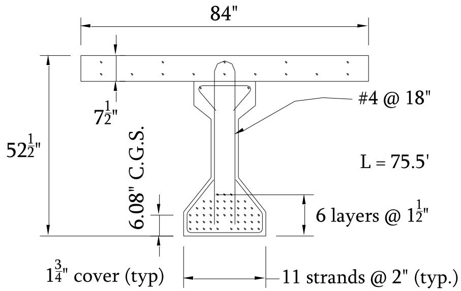
Figure 5.3 Prototype IB girder cross section.
