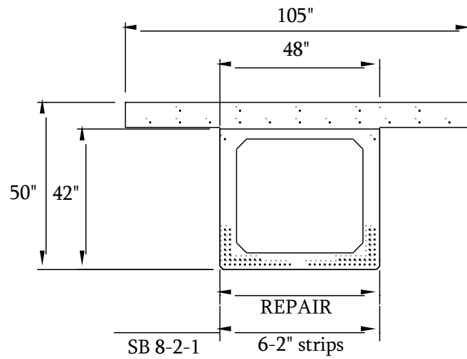
Figure 5.22 Post-tensioned CFRP repaired SB.
