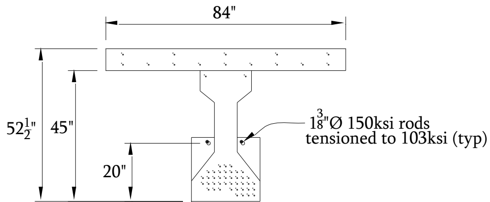
Figure 5.29 External post-tensioned steel repaired IB 10-2-1 drawing.
