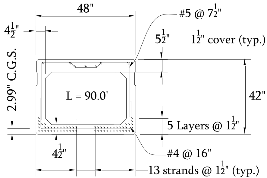
Figure 5.1 Prototype AB girder cross section.
