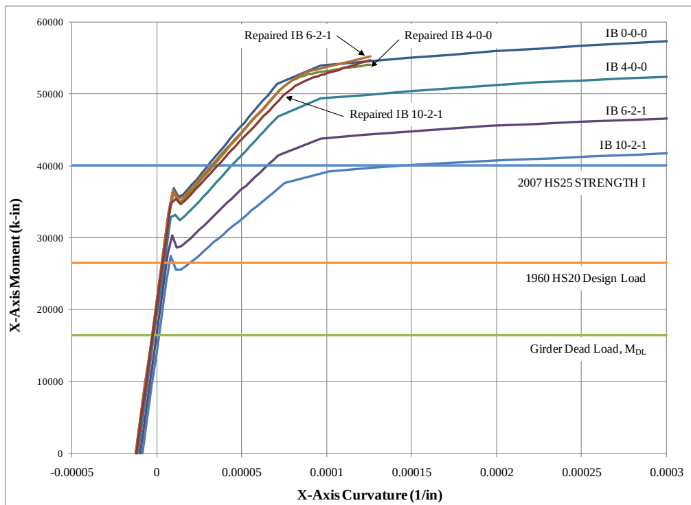
Figure 5.26 Post-tensioned CFRP repaired IB moment-curvature plot.
