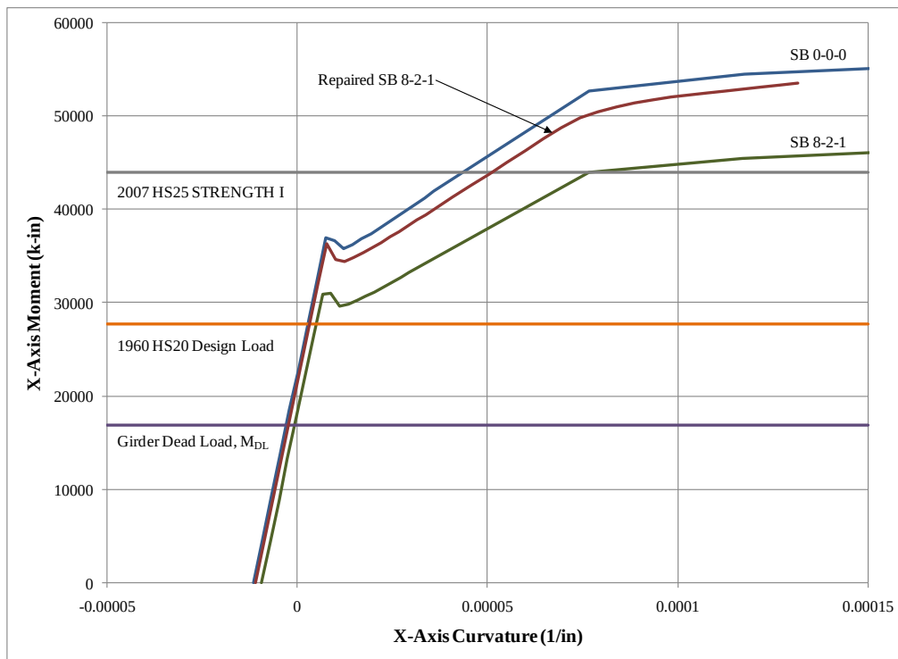
Figure 5.25 Post-tensioned CFRP repaired SB moment-curvature plot.
