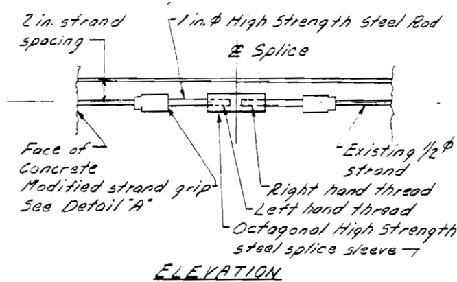
(b) Splice 7: 'Turnbuckle' style strand splice. Coupler draws strand ends together.
