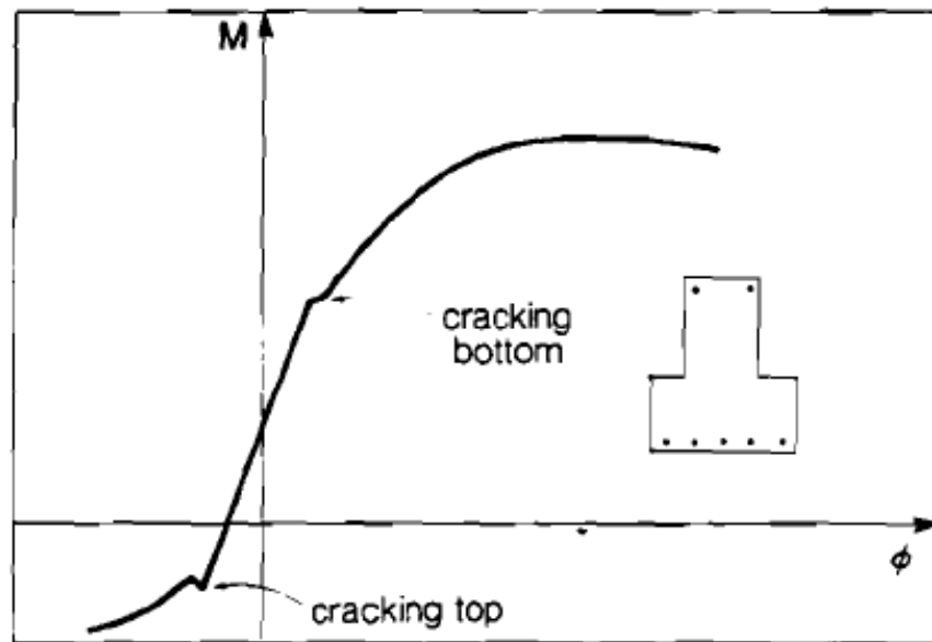
Figure 5.10 Flexural behavior of prestressed girders (Collins and Mitchell 1997).
