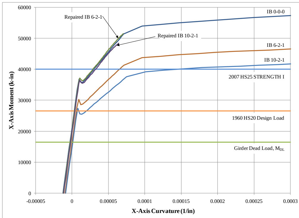
Figure 5.30 External post-tensioned steel repaired IB moment-curvature plot.
