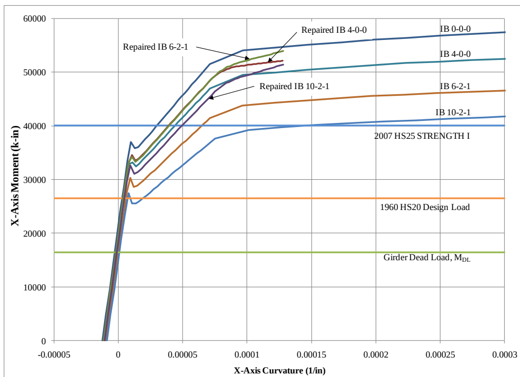
Figure 5.19 Prestressed CFRP repaired SB moment-curvature plot.
