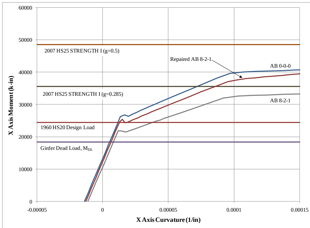
Figure 5.18 Prestressed CFRP repaired AB moment-curvature plot.
