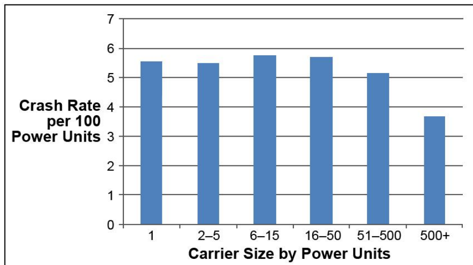
Figure 3. Bar Chart. Crash Rates per 100 Power Units by Fleet Size
