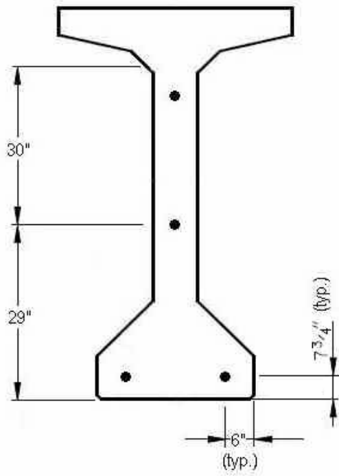
(a) 132 ft. girder
