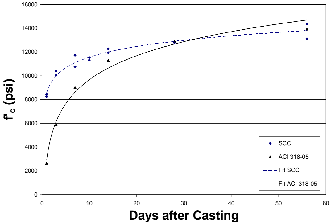
Figure 3-8 Measured and calculated compressive strength values
