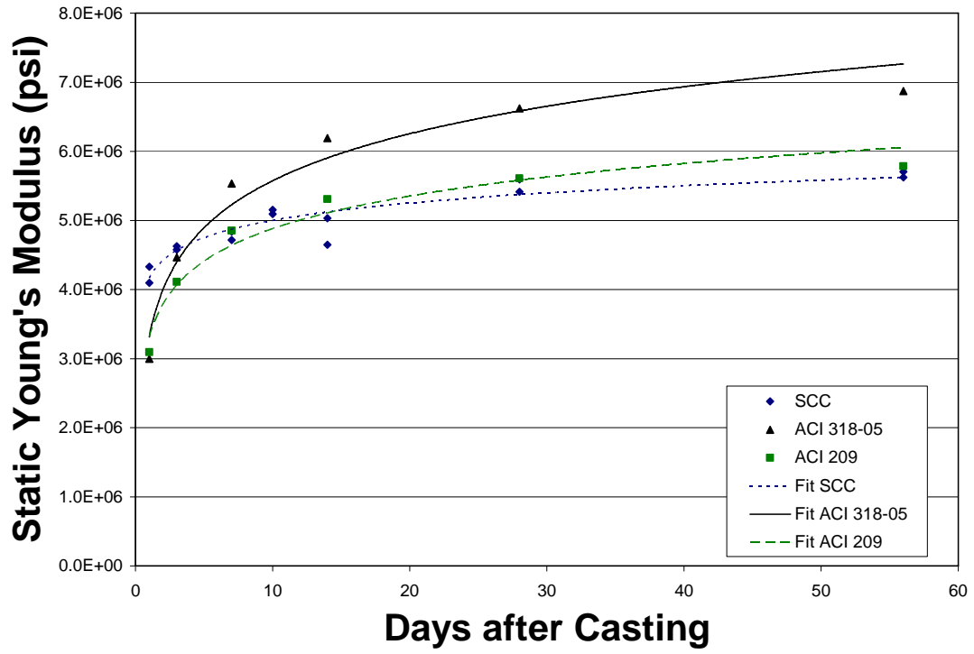
Figure 3-9 Measured and calculated static Young's modulus values
