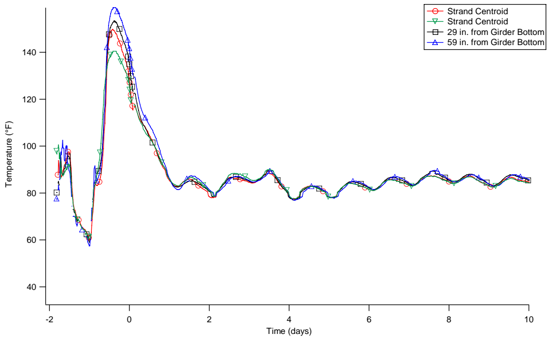
(b) Short term temperature readings
