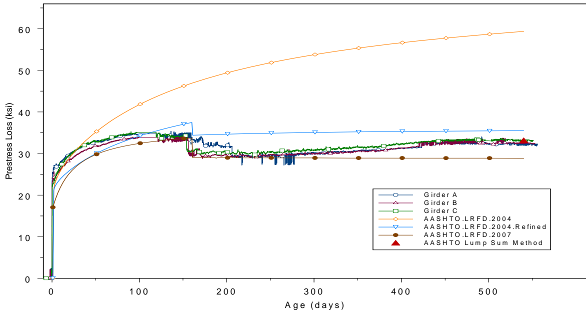
Figure 3-13 Measured and calculated (using specified values) prestress losses for the 132 ft. girders
