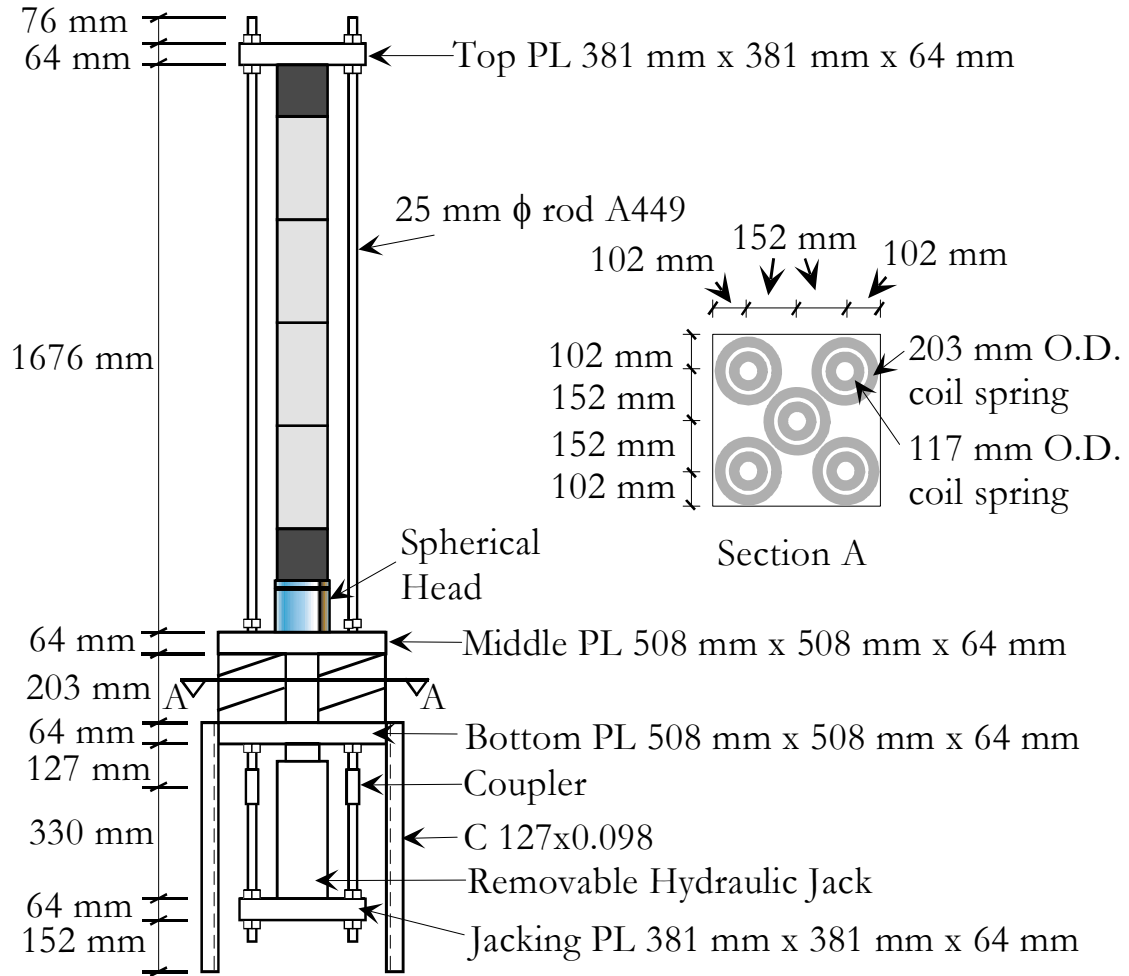
Figure 2-8 Creep Rig Design
