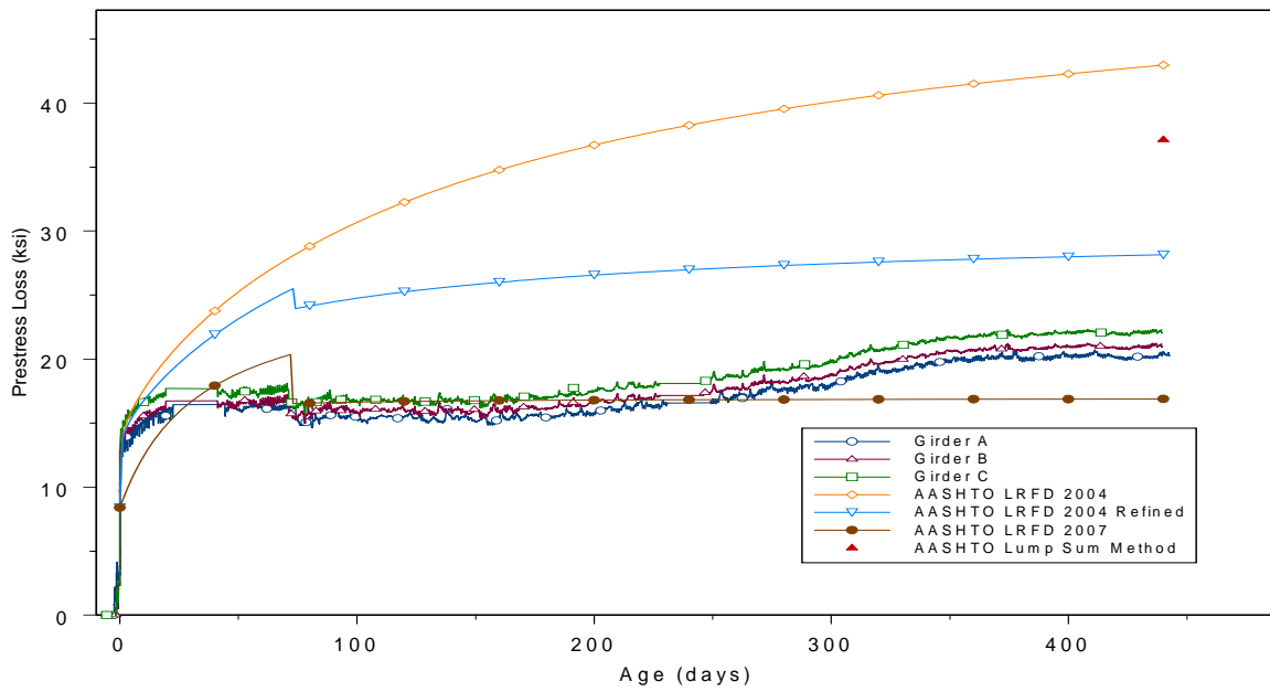
Figure 3-14 Measured and calculated (using specified values) prestress losses for the 82 ft. girders
