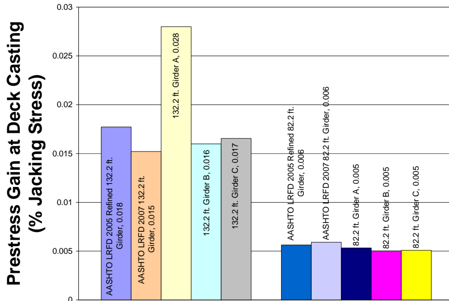
Figure 3-17 Measured and calculated prestress gains at deck placement
