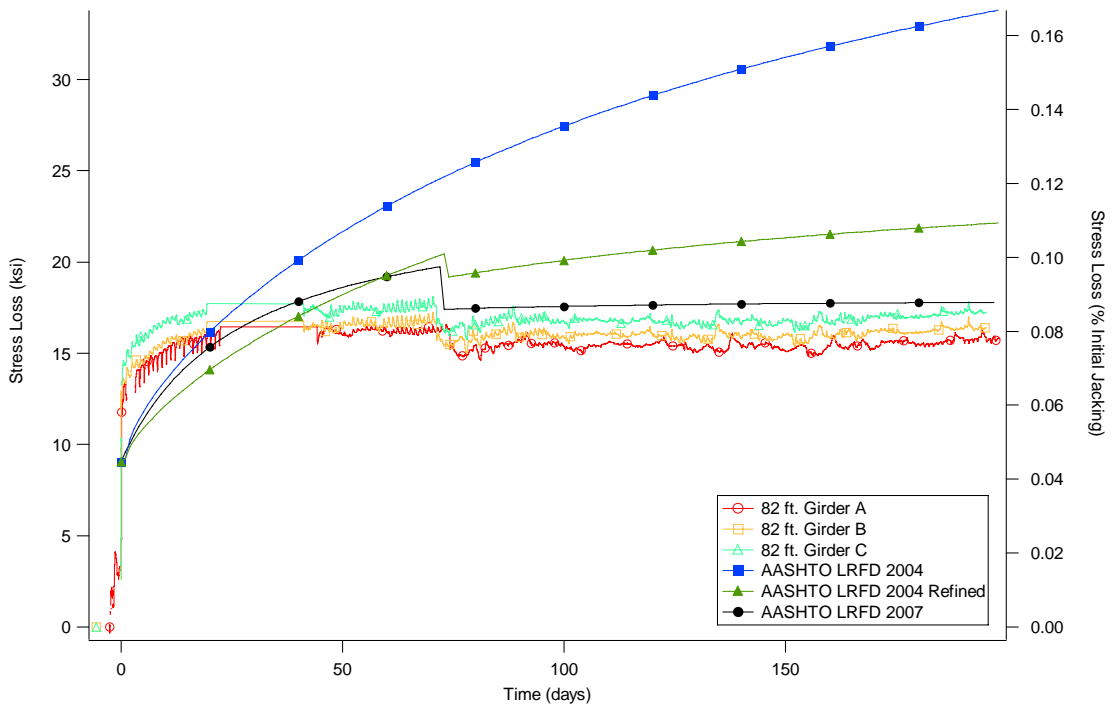
Figure 3-12 Measured and calculated (using measured values) prestress losses for the 82 ft. girders
