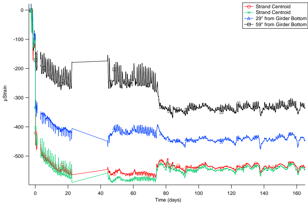
Figure 3-5 Measured strains
