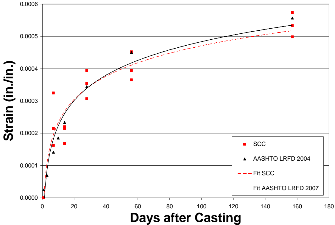
Figure 3-10 Measured and calculated shrinkage values
