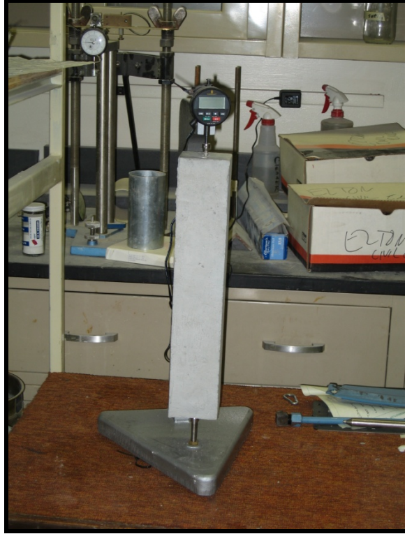
Figure 2-6 Shrinkage Test
