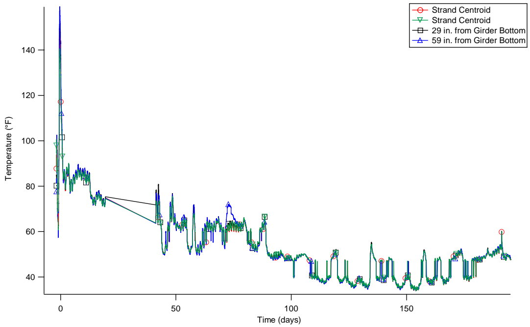
(a) Long term temperature readings
