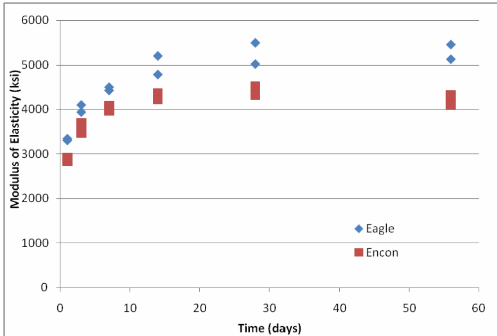
Figure 2-5 Modulus of Elasticity versus Time
