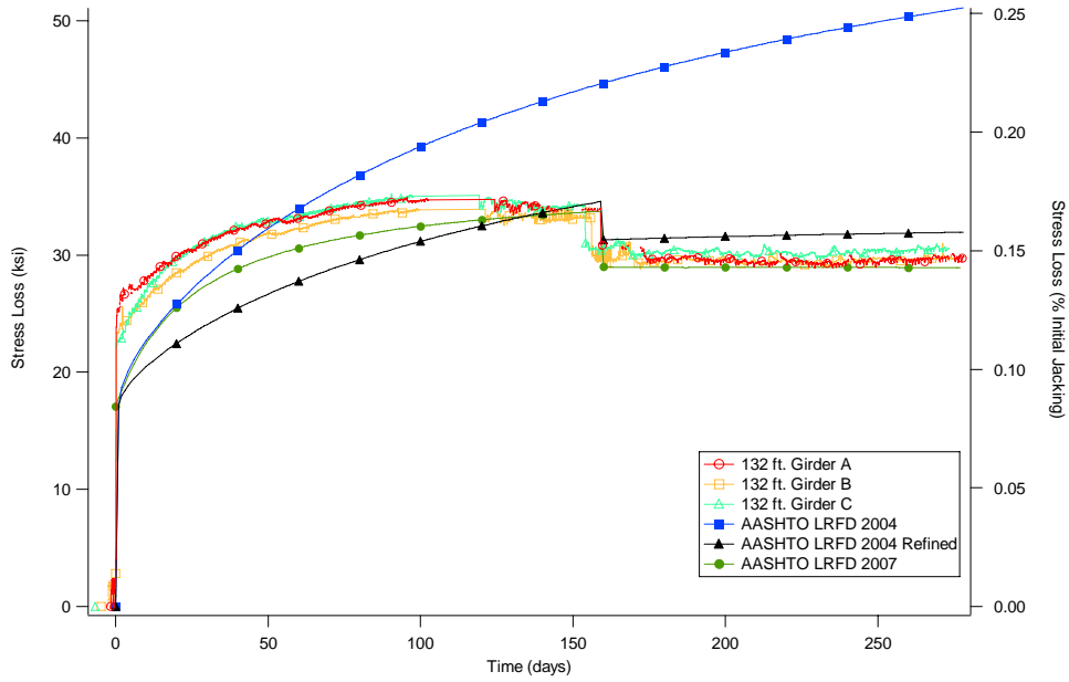
Figure 3-11 Measured and calculated (using measured values) prestress losses for the 132 ft. girders
