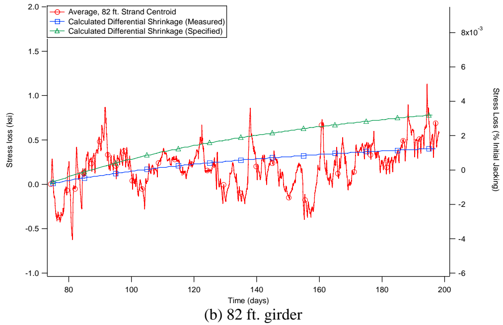
Figure 3-18 Measured and calculated prestress losses due to differential shrinkage
