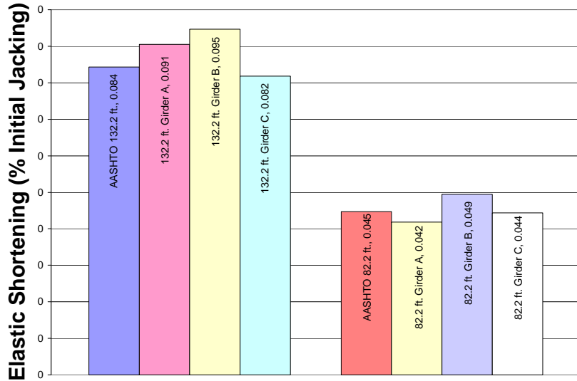
Figure 3-15 Measured and calculated prestress losses due to elastic shortening
