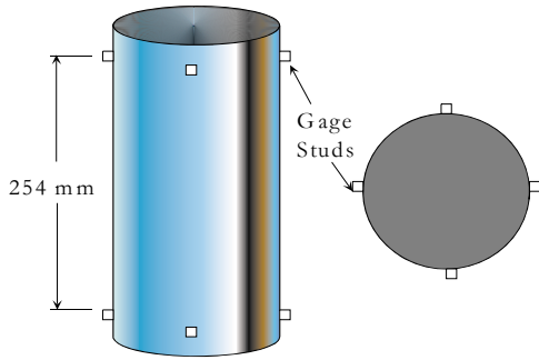
Figure 2-9 Gage Stud Locations
