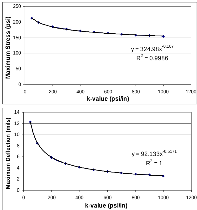
Figure 49. Maximum Stress and Deflection of One-Layer System.
