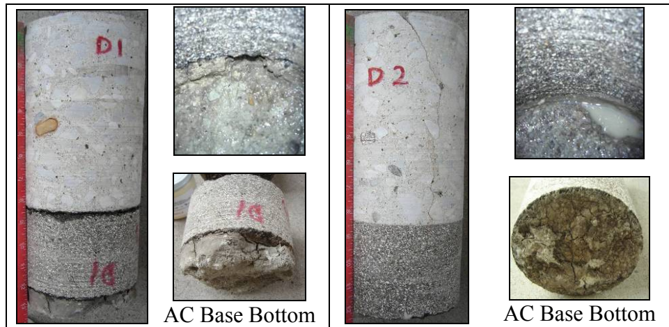
Figure 14. Cored Samples and Subgrade Condition of Section 1 on US 81/287.
