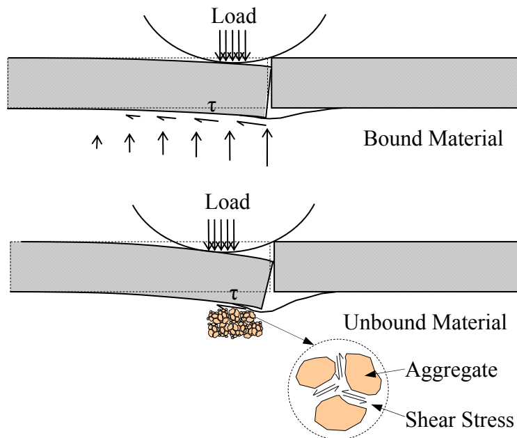
Figure 34. Shear Induced Erosion.
