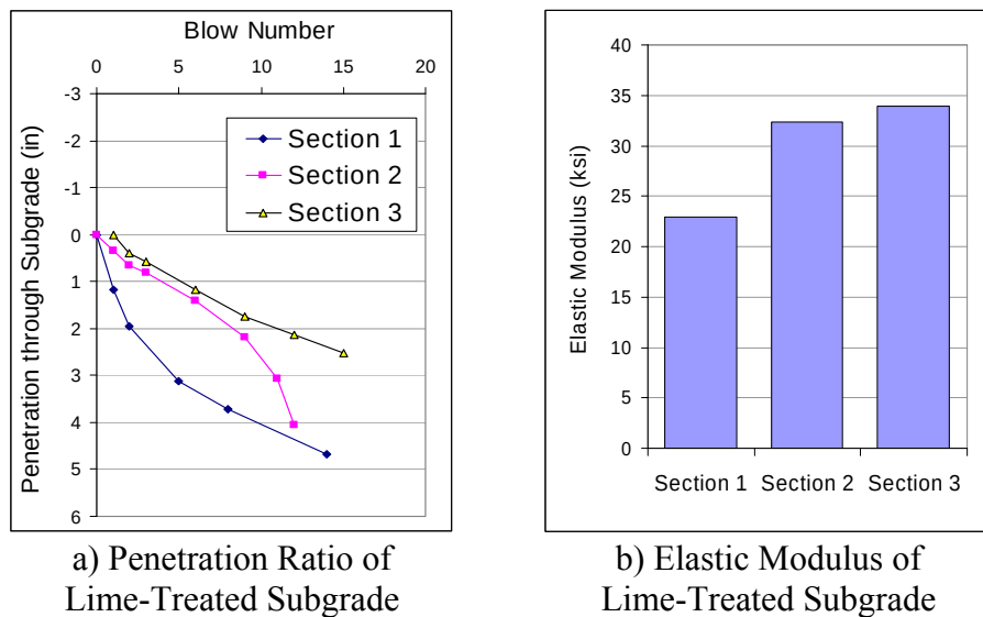
Figure 13. DCP Testing Results of Test Sections on US 81/287.
