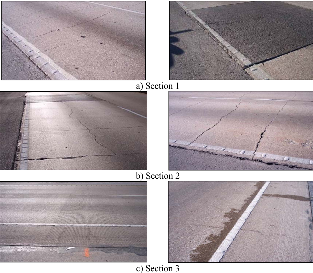
Figure 8. Test Sections on US 81/287.
