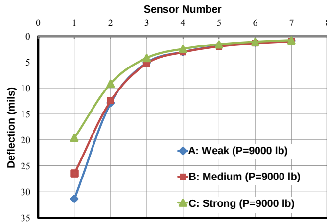
Figure 59. FWD Result along Sensors.
