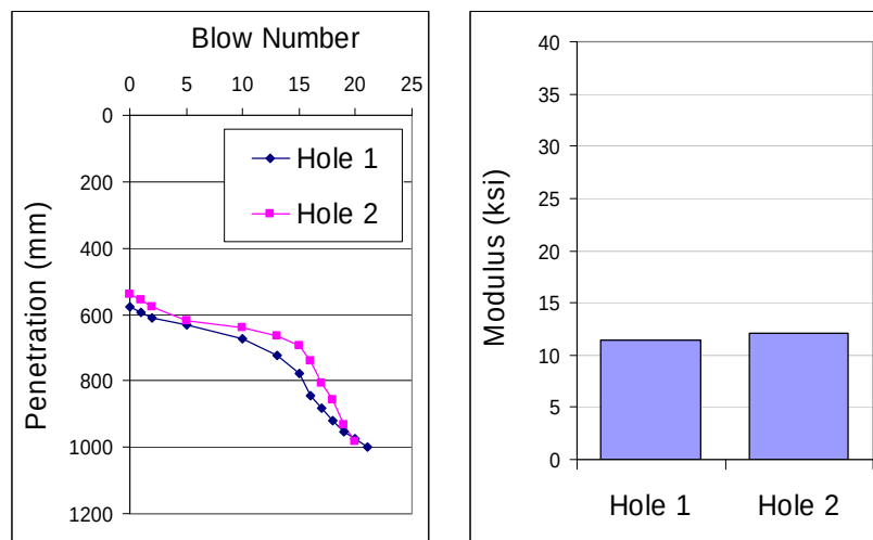
Figure 20. DCP Testing Results of Test Section on FM 364.
