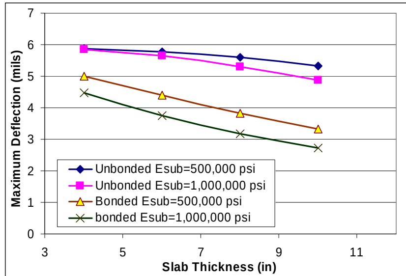
Figure 48. Maximum Deflection.
