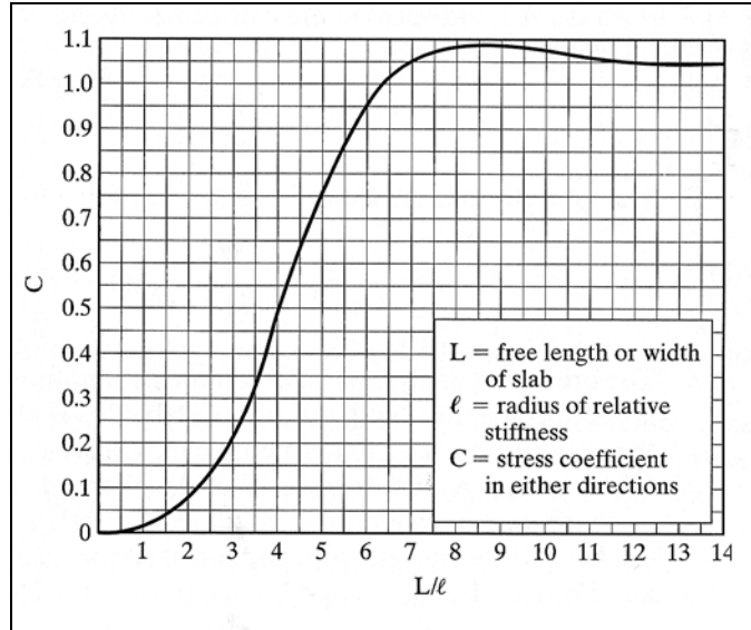
Figure 53. Stress Coefficient at the Center of Slab for the Curling Ratio L/\ell (16).
